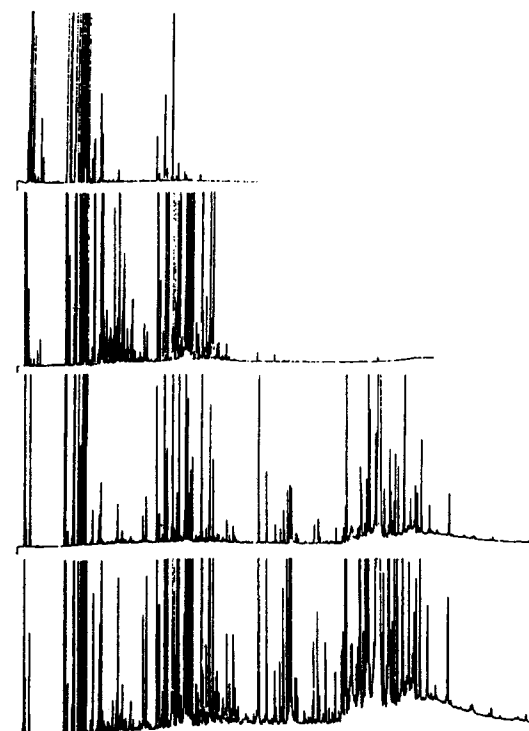
Fig. 9.2. Chromatograms of black pepper volatiles produced by (top to bottom) (1) direct injection of 200 \mu L of headspace vapor, (2) simultaneous steam distillation-extraction (Nickerson Likens), and Soxhlet extractions with (3) dichloromethane, and (4) high pressure liquid carbon dioxide. Column, 30 m \times 0.25 mm, 0.25 \mu m film of polydimethylsiloxane; 40–280°C @ 4°/min, headspace injection on-column, all other injections split 1:100. From [3], and reprinted by permission of the American Chemical Society.
