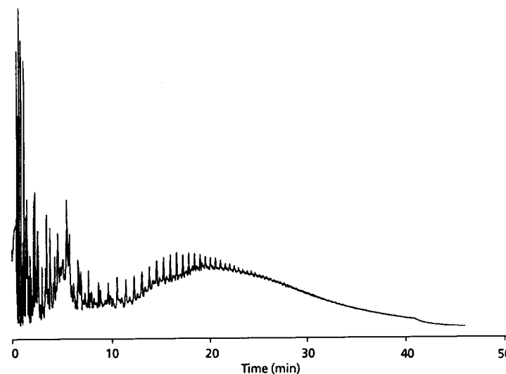
Fig. 9.40. Reference crude oil chromatographed on a 5 m \times 0.53 mm I.D. metal capillary column with a 0.15 \mu m film of bonded methylpolysiloxane. The oven was programmed from -30 to 430^\circ\text{C} at 10^\circ\text{C} per minute. The sample was in \text{CS}_2 solution. The PTV injector used was programmed from 55 to 450^\circ\text{C} at 1^\circ\text{C} per second.
