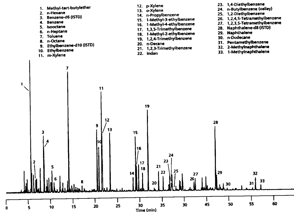
Fig. 9.32. A thick film dimethylpolysiloxane column, 60 m \times 0.25 mm I.D. with a 1.0 \mu m film, coupled with MS detection used to quantitate aromatic compounds in gasoline. Deuterated benzene (d6), ethylbenzene (d10) and naphthalene (d8) served as internal standards. Courtesy of J&W Scientific.
