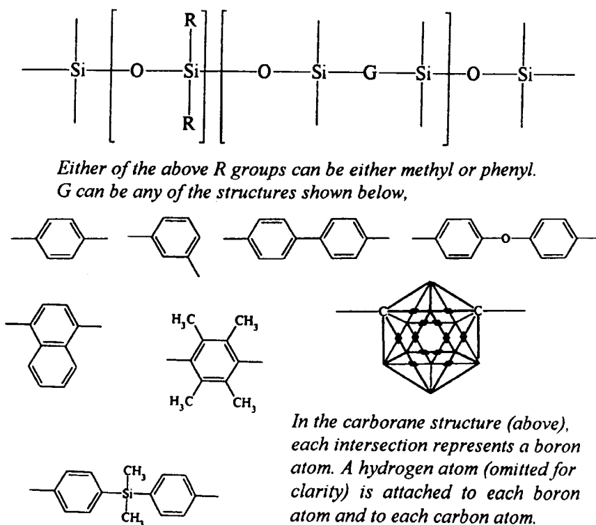
Fig. 4.2. Groups suggested as inclusions in the polysiloxane chain to effect “stiffening” [10].
