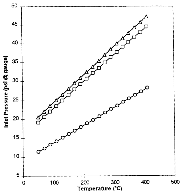
Fig. 5.1. Inlet pressure required to maintain a 1.0 mL/min volumetric flow of carrier gas through a 60 m \times 0.25 mm \times 1.0 \mu m column; helium ( \Delta ); nitrogen ( \square ); and hydrogen ( \circ ).
