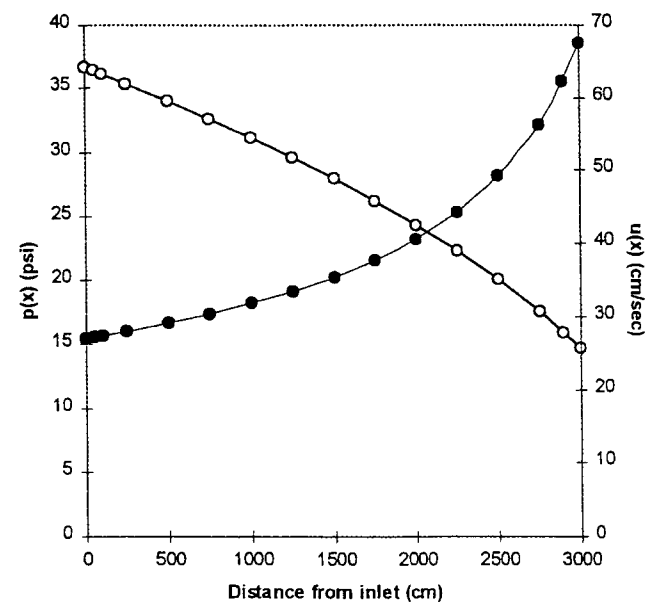
Fig. 5.4. Linear velocity ( \bullet ) and pressure ( \circ ) as a function of distance from the inlet of a 30 m \times 0.25 mm \times 1.0 \mu m DB-1 column operated with helium carrier gas at a temperature of 175°C, an inlet pressure of 22 psig, and an outlet pressure of 14.690. Under these conditions, the carrier gas viscosity is 0.0026 cP, volumetric flow is 1.99 mL/min (measured as 1.30 mL/min at 20°C), column hold-up time is 1.378 min, and the average linear velocity of carrier gas is 36.34 cm/sec.
