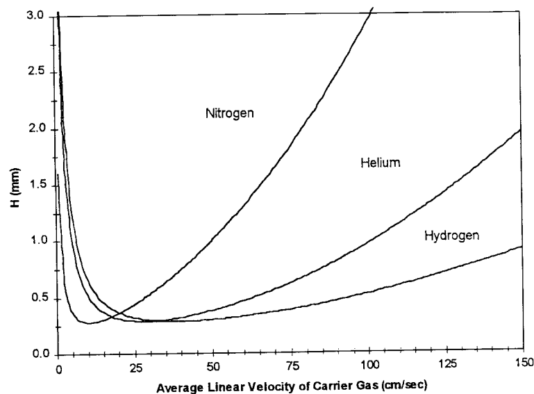
Fig. 5.7. Variation in H as a function of \bar{u} for different carrier gases on a 30 m \times 0.32 mm \times 2.25 \mu m SE-30 column operated isothermally at 115°C. In all cases k = 6.237 .
