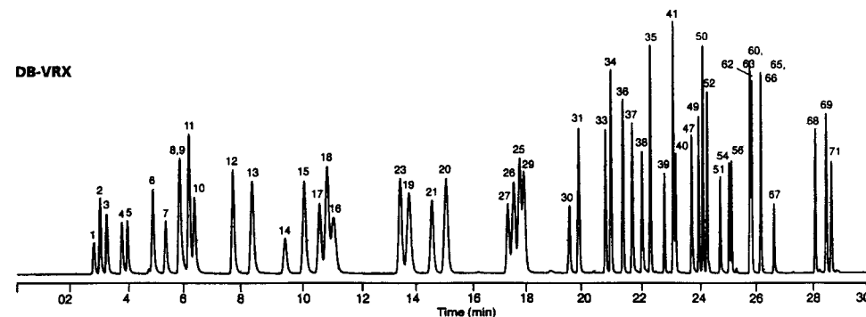
Fig. 9.48. US EPA Method 8021 is a general method for the analysis of volatile priority pollutants in industrial waste. A dual column application with tandem PID-ELCD detection is presented here. The result being four chromatograms from a single sample. The columns are a 75 m \times 0.45 mm I.D. DB-VRX and DB-624, with 2.55 \mu m films. Purge and trap injection without cryofocusing is used to inject the sample. The combination of dissimilar selectivities of both stationary phases and detectors provides an ambiguous assignment of peaks.
