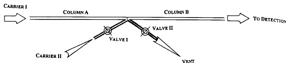
Fig. 8.11. The concept of "selectivity tuning," adapted from Hinshaw and Ettre [40, 41]. Columns A and B are coupled together, with a "Y" providing a port at the point of junction. To gain a higher contribution from column A (and a lesser contribution from column B), the micro-metering valve I is opened, introducing a controlled amount of additional carrier gas (carrier II is at a slightly higher pressure than carrier I). This increases the residence time in (and the contribution from) column A, and decreases the time in (and the contribution from) column B. The degree to which these contributions are affected is controlled by valve I. To gain a higher contribution from column B (and a lesser contribution from column A), valve I is closed, and valve II is opened. This decreases the time in (and the contribution from) column A, and increases the time in (and the contribution from) column B. Again, the magnitude of these effects is controlled by valve II.
