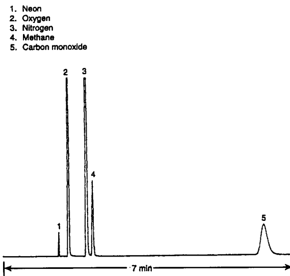
Fig. 9.29. Separation of permanent gases at 50°C on a 30 m \times .53 mm I.D., molecular sieve PLOT column.
