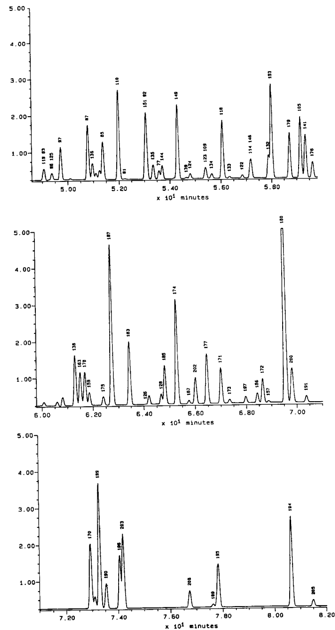
Fig. 9.54. A chromatogram of poly chlorinated biphenyls, listed by IUPAC #, on a 60 m × 0.18 mm I.D. DB-XLB with a 0.18 μm film. The oven was programmed from 75°C (2 min.) at 15°C/min to 150°C, then at 1.5°C/min to 285°C. The carrier was H 2 with an average linear velocity of 40 cm/sec. The sample was a dilute mixture of Aroclor 1232, 1248 and 1262. Courtesy of Jack Cochran, Hazardous Waste Research and Information Center, Champaign, IL, USA.
