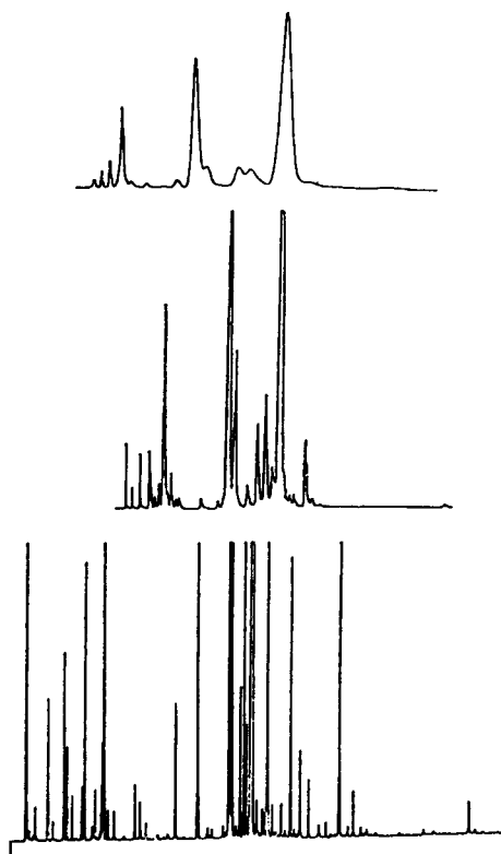
Fig. 1.2. Chromatograms of a peppermint oil on (top) a 6\text{ ft} \times 1/4 in packed column, (center) a 500\text{ ft} \times 0.03 in stainless steel open tubular column, and (bottom) a 30\text{ m} \times 0.25 mm fused silica open tubular (capillary) column. Adapted from [12], p. 445, and reprinted with permission.
