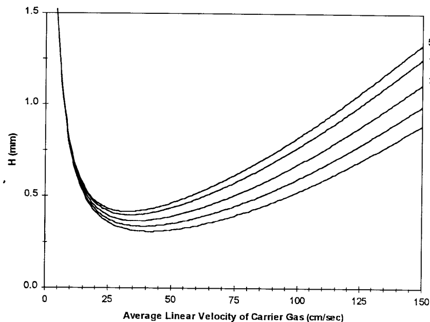
Fig. 5.14. Variation in H as a function of \bar{u} for several 30 m \times 0.32 mm \times 1.00 \mu m columns operating isothermally at 150°C with hydrogen carrier gas: 1) D_S = 1.292 \times 10^{-5} cm 2 /sec; 2) D_S = 6.252 \times 10^{-6} cm 2 /sec; 3) D_S = 3.941 \times 10^{-6} cm 2 /sec; 4) D_S = 2.752 \times 10^{-6} cm 2 /sec; and 5) D_S = 2.342 \times 10^{-6} cm 2 /sec.
