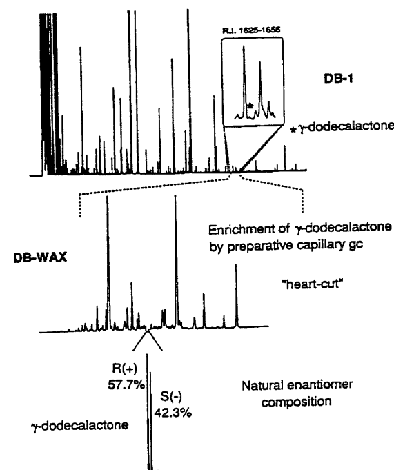
Fig. 8.5. Diversion of a single peak from a DB-WAX column to a second chiral column, which resolved the enantiomers [15].
