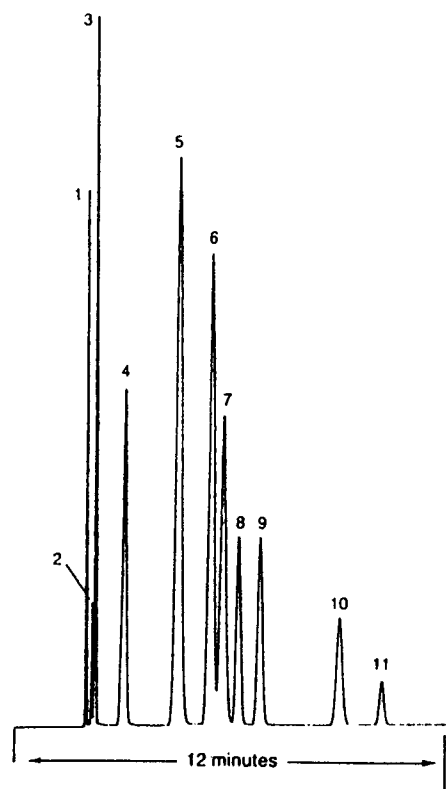
Fig. 9.26. Refinery gas on a thick-film column. Column, 30 m \times 0.32 mm, d_i 5.0 \mu m dimethyl polysiloxane. One mL gas injected directly on column; 0°C (3 min) to 50°C @ 10°/min. Solutes: 1) methane; 2) ethylene; 3) ethane; 4) propane; 5) isobutane ; 6) 1-butene; 7) n -butane; 8) trans -2-butene; 9) cis -2-butene; 10) isopentane ; 11) n -pentane. Courtesy of J&W Scientific.
