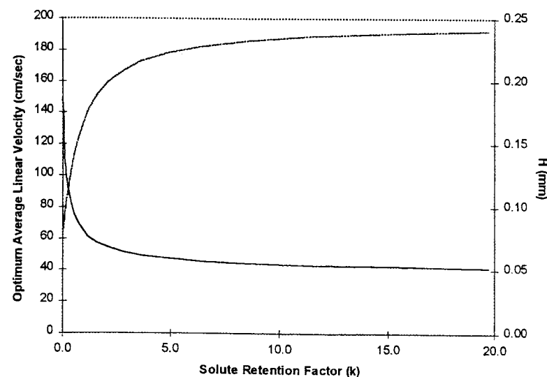
Fig. 5.9. Variation in H at \bar{u}_{\text{opt}} as a function of the solute retention factor. Parameters for calculation included a 30 \text{ m} \times 0.25 \text{ mm} \times 0.50 \mu\text{m} SE-30 WCOT column operating isothermally at 250^\circ\text{C} with hydrogen carrier gas. The upper curve illustrates the variation in H , while the lower curve shows the variation in \bar{u}_{\text{opt}} .
