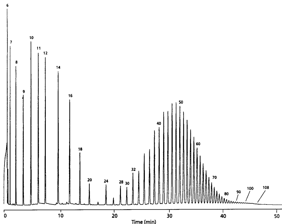
Fig. 9.38. Standard n -alkanes chromatographed on a 5 m \times 0.53 mm I.D. metal capillary column with a 0.15 \mu m film of bonded methylpolysiloxane [66]. The oven was programmed from -30 to 430^\circ\text{C} at 10^\circ\text{C} per minute. The sample was in \text{CS}_2 solution. The PTV injector used was programmed from 55 to 450^\circ\text{C} at 1^\circ\text{C} per second.
