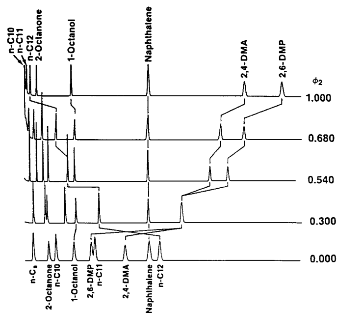
Fig. 8.12. Selectivity tuning, as applied to a sample of lime oil [41].
