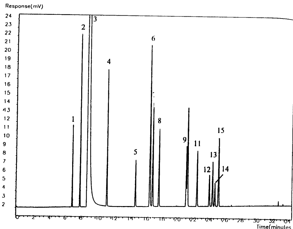
Fig. 9.28. Ethylene separated from impurities on a 50 meter \text{Al}_2\text{O}_3 PLOT column with KCl deactivation coupled to a 30 meter thick film ( 5\ \mu\text{m} ) methyl silicone column. Both columns have a 0.53 mm I.D. The methyl silicone column improves the separation of methyl acetylene, iso-pentane and n -pentane. The components are: (1) methane, (2) ethane, (3) ethylene, (4) propane, (5) propylene, (6) acetylene, (7) isobutane , (8) n -butane, (9) trans -2-butene, (10) 1-butene, (11) cis -2-butene, (12) isopentane , (13) methylacetylene, (14) n -pentane, (15) 1,3-butadiene.
