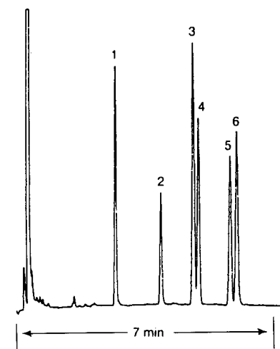
Fig. 9.62. Sedative and hypnotic drugs; conditions as in Fig. 9.60 except 70\text{ ng} per component, 150^\circ\text{C} to 250^\circ\text{C} @ 10^\circ/\text{min} . Solutes: 1) aprobarbital; 2) meprobamate; 3) diphenhydramine; 4) mephobarbital; 5) methapyrilene; 6) chlorpheniramine.
