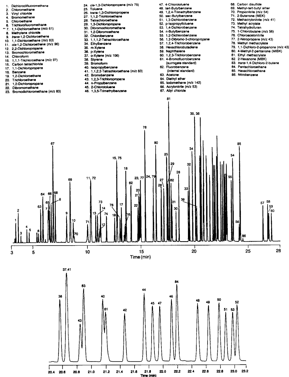
Fig. 9.47. US EPA Method 524.2, Revision 4, volatile organic compounds on a 60 m x 0.25 mm I.D. DB-VRX with a 1.4 μm film thickness. For this method of drinking water analysis, the purge and trap unit desorbs into a cryofocusing module (−160°C) at the head of the column. The method calls for the analysis of 82 compounds plus internal standards. The lower chromatogram is an expanded portion of the upper chromatogram.
