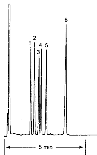
Fig. 9.60. Underivatized barbiturates on a 30\text{ m} \times 0.53\text{ mm} column, 1.5\text{ }\mu\text{m} film of dimethylpolysiloxane; 175^\circ\text{C} to 210^\circ\text{C} @ 8^\circ/\text{min} . Direct injection of one \mu\text{L} methanol containing one \mu\text{g} each analyte. Solutes: 1) aprobarbital; 2) butabarbital; 3) amobarbital; 4) pentobarbital; 5) secobarbital; 6) phenobarbital.
