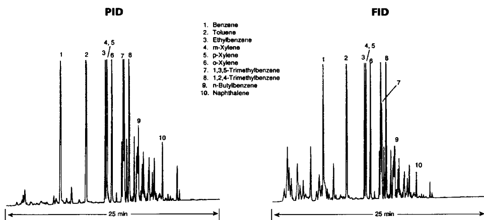
Fig. 9.55. The analysis of a contaminated water (5 ppm gasoline) sample for BTEX using a PID and FID in tandem. The PID is selective for unsaturated and aromatic compounds and the FID detects all of the hydrocarbons in the sample. The sample was chromatographed on a 30 m \times 0.53 mm I.D. DB-624 column with a 3 \mu m film. The sample was collected and injected with a purge and trap concentrator.
