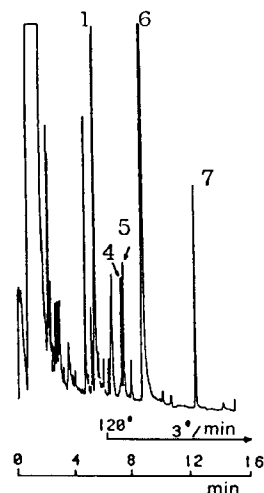
Fig. 9.67. Extract of human plasma following oral administration of isosorbide dinitrate [94]. Column, 30 m \times 0.32 mm, 0.25 \mu m film of 5%-phenyl-95%-methylpolysiloxane; 60° during injection, ballistic rise to 120°C (3 min) to 195°C @ 3°/min. Solutes: 1) isosorbide-2-mononitrate; 4) isomannide mononitrate; 5) isoidide mononitrate; 6) isosorbide-5-mononitrate; 7) isosorbide dinitrate. Reprinted with permission of Huethig Publishing Co.
