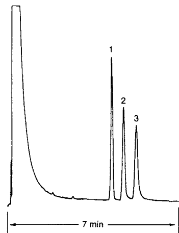
Fig. 9.59. Underivatized antidepressant drugs on a 15\text{ m} \times 0.53\text{ mm} column, 1\text{ }\mu\text{m} 50%-dimethyl-50%-diphenylpolysiloxane; 150 to 220^\circ\text{C} @ 20^\circ/\text{min} . Solutes: 1) amitriptyline; 2) nortriptyline; 3) protriptyline.
