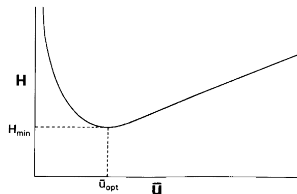
Fig. 1.9. Total effect of the average linear carrier gas velocity ( \bar{u} ) on column efficiency ( H ), the van Deemter curve represents the summation of the curves shown in Figs. 1.7 and 1.8.
