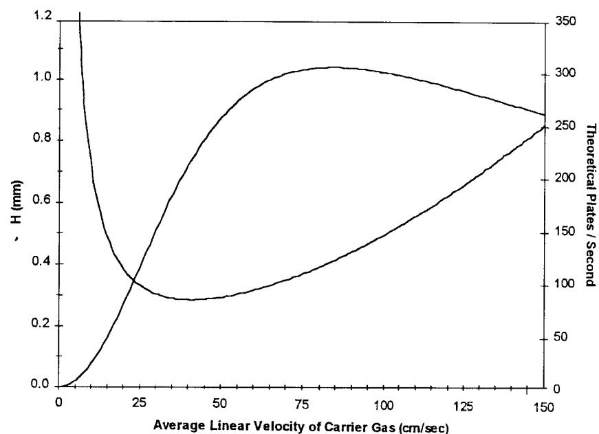
Fig. 5.16. Variation in H and N/\text{sec} as a function of \bar{u} for a particular solute on several 30 \text{ m} \times 0.32 \text{ mm} \times 0.50 \text{ }\mu\text{m} columns under isothermal conditions at 120^\circ\text{C} with hydrogen carrier gas.
