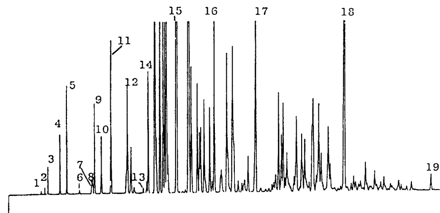
Fig. 9.30. Chromatogram produced by injection of one mL neat naphtha on a 30 m \times 0.32 mm column, d_f 1.0 \mu\text{m} dimethylpolysiloxane. Hydrogen carrier @ 38 cm/sec (100°C); 28°C (4 min) to 100°C @ 2.5°/min. Analysis time 28 min. Solutes (attenuation \times 1): 1) propane; 2) methylpropane; 3) n -butane; 4) (attenuation to \times 4) 2-methylbutane; 5) n -pentane; 6) 2,2-dimethylbutane; 7) cyclopentane; 8) 2,3-dimethylbutane; 9) 2-methylpentane; 10) 3-methylpentane; 11) (attenuation to \times 8) n -hexane; 12) methylcyclopentane; 13) (attenuation to \times 16) benzene; 14) cyclohexane; 15) n -heptane; 16) toluene; 17) n -octane; 18) n -nonane; 19) n -decane. Courtesy of J&W Scientific.
