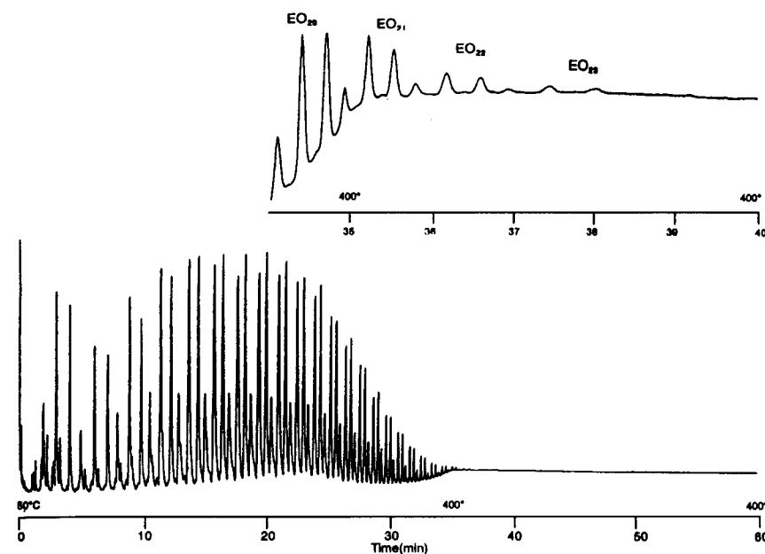
Fig. 4.5. A 3 m segment of a 0.25 mm DB-XLB column programmed to 400°C and held. The molecular weight of the last discernable solute eluting at 38 min in the expanded printout is 1238. From reference [11].
