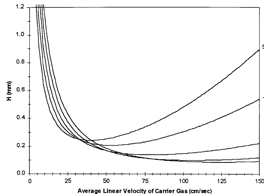
Fig. 5.15. Variation in H as a function of \bar{u} for a particular solute on several 30 m \times 0.250 mm \times 0.50 \mu m columns operated under isothermal conditions with hydrogen carrier gas. 1) T = 300^\circ\text{C} , k = 0.044 , D_S = 1.039 \times 10^{-4} cm 2 /sec, D_M = 0.677 cm 2 /sec; 2) T = 250^\circ\text{C} , k = 0.126 , D_S = 6.267 \times 10^{-5} cm 2 /sec, D_M = 0.577 cm 2 /sec; 3) T = 200^\circ\text{C} , k = 0.460 , D_S = 3.395 \times 10^{-5} cm 2 /sec, D_M = 0.484 cm 2 /sec; 4) T = 150^\circ\text{C} , k = 0.2276 , D_S = 1.592 \times 10^{-5} cm 2 /sec, D_M = 0.398 cm 2 /sec; 5) T = 100^\circ\text{C} , k = 0.17263 , D_S = 6.089 \times 10^{-6} cm 2 /sec, D_M = 0.319 cm 2 /sec.
