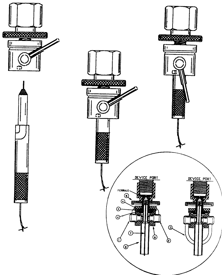
Fig. 6.2. A "Quick Connector" for column installation, using standard graphitized Vespe l ™ ferrules. Courtesy of Quadrex, Inc.
