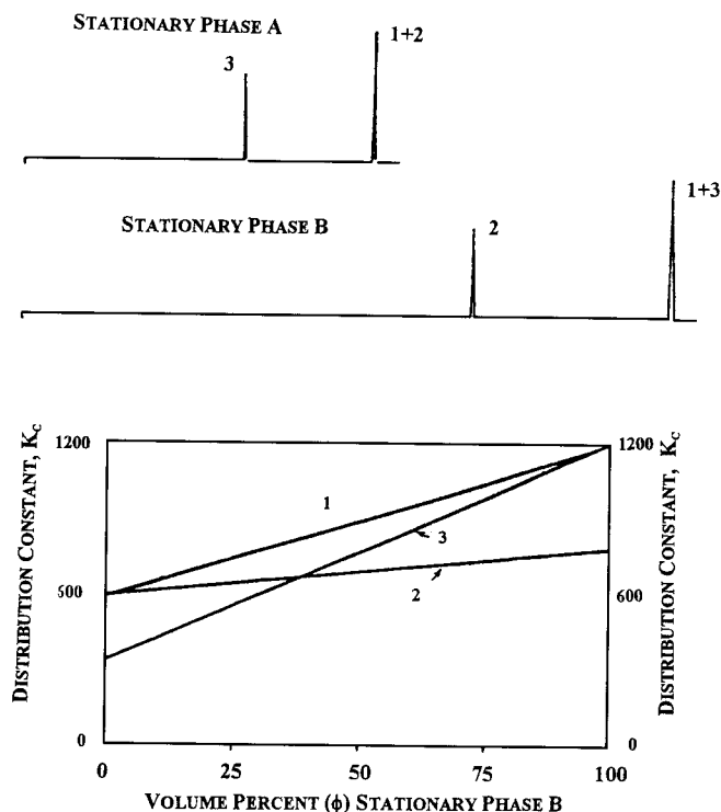
Fig. 8.8. Simplified explanation of the Maier and Karpthy [26] approach to utilization of binary mixtures of stationary phases. Distribution constants ( K_c ) for each solute are calculated from the isothermal chromatogram on stationary phase A, and plotted on the left ordinate of the bottom graph. Similarly, K_c s of each solute on the isothermal chromatogram (same temperature) on stationary phase B; these are plotted on the right ordinate of the bottom graph. K_c for each of these solutes in any specified mixture of A + B can now be predicted from a line connecting the two values for that solute.
