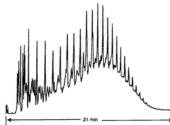
Fig. 9.39. A reference gas oil chromatographed according to ASTM D2887E. The 10 m \times 0.53 mm I.D., 3 \mu m film column was programmed only to 350^\circ\text{C} , limiting the range to \text{C}_{60} . The sample was introduced by Megabore direct injection.
