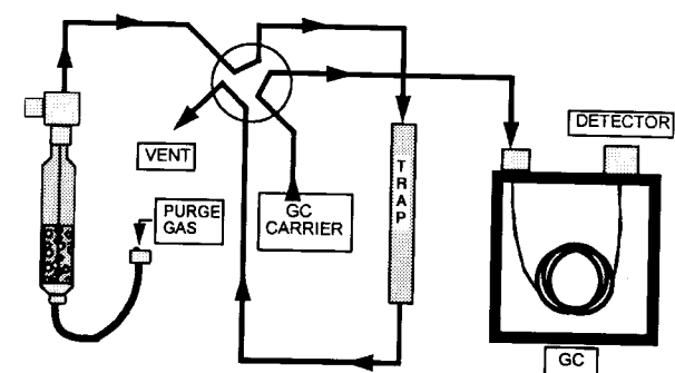
PURGE STATE
