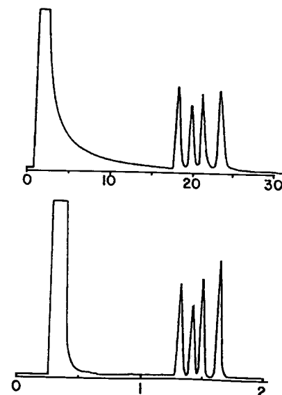
Fig. 1.3. Off-line monitoring of a mixture of methyl benzoates. Top, packed column analysis (25 min), and bottom, 1.7\text{ m} \times 0.25 mm glass capillary analysis (1.7 min).
