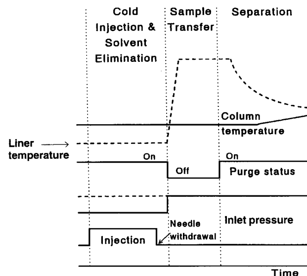
Fig. 3.10. Parameters to be optimized for a large volume PTV injection in the solvent split mode. Adapted from C. Cramers and H. Jannsen with permission.
