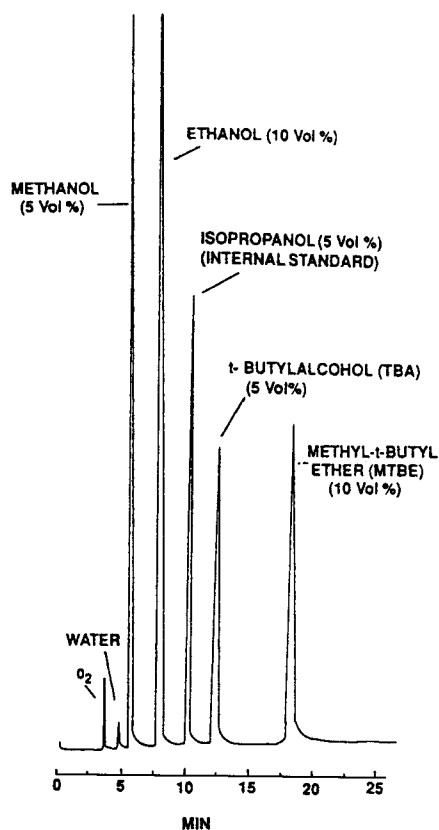
Fig. 9.33. The GC-OFID chromatogram of typical oxygenated compounds found in reformulated gasoline. The separation was performed on a 30 \text{ m} \times 0.32 \text{ mm} I.D. methylpolysiloxane column with a 3 \mu\text{m} film thickness [53].
