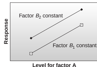
Figure 14.4 Factor effect plot for two independent factors.
