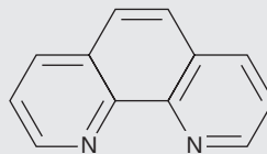
o-Phenanthroline
