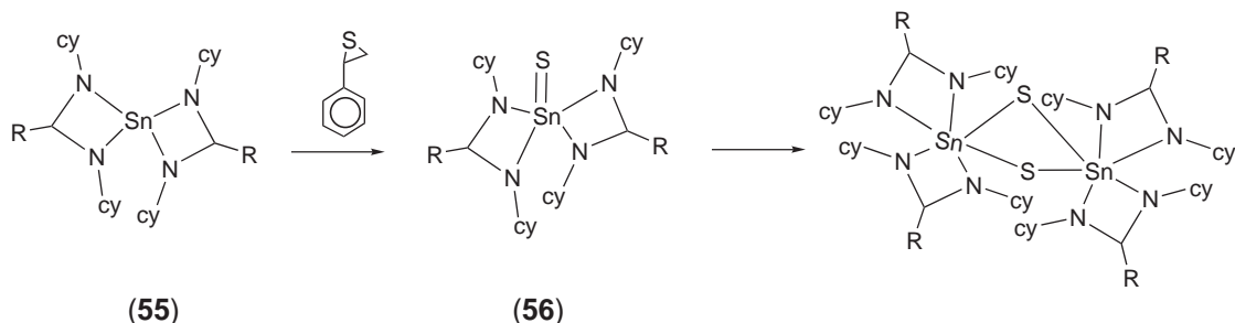
Scheme 18
