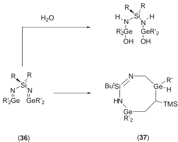
Scheme 13
