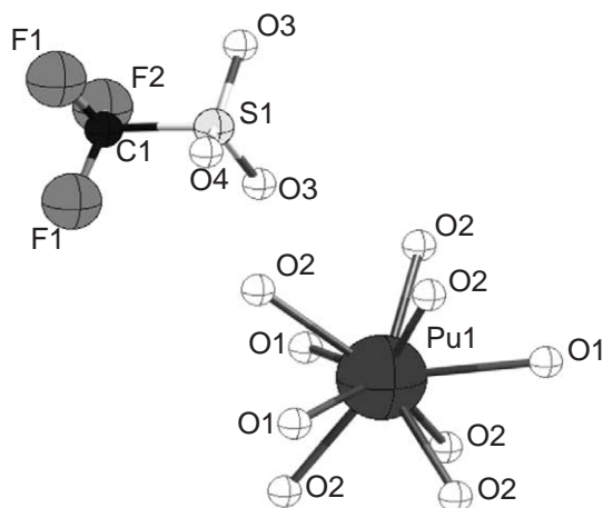
Figure 5 Crystal structure of [Pu(H_2O)_9][CF_3SO_3]_3 , showing Pu^{III} aqua with ideal tricapped trigonal prismatic geometry (Matonic, Scott et al. Inorg. Chem. 2000 , 40 , 2638).
