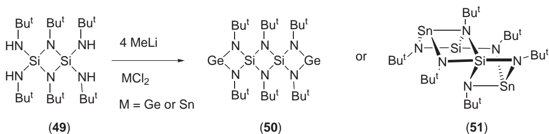
Scheme 17
