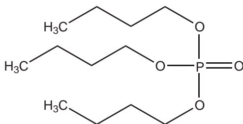
Figure 54 Tributylphosphate (TBP).
