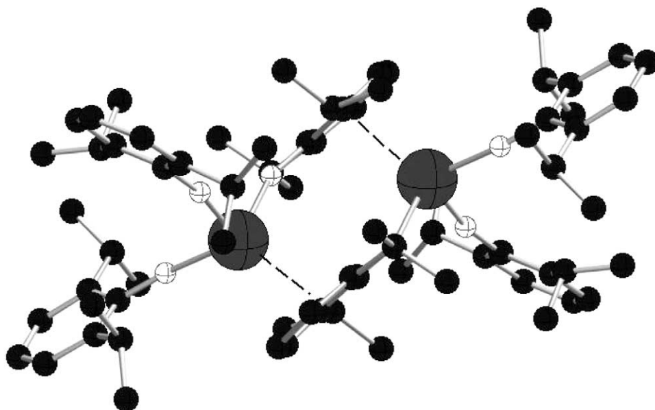
Figure 3 Crystal structure of [\text{U}(\text{O}-2,6\text{-Pr}^i_2\text{C}_6\text{H}_3)_2]_2 (Van Der Sluys, Burns et al. Inorg. Chem. 1998 , 110 , 5924).
