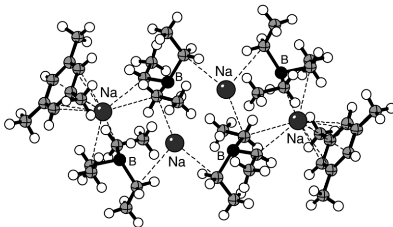
Figure 24 The structure of the sodium derivative of the “superhydride” anion, \text{Na}[\text{HB}(\text{Et})_3] .
