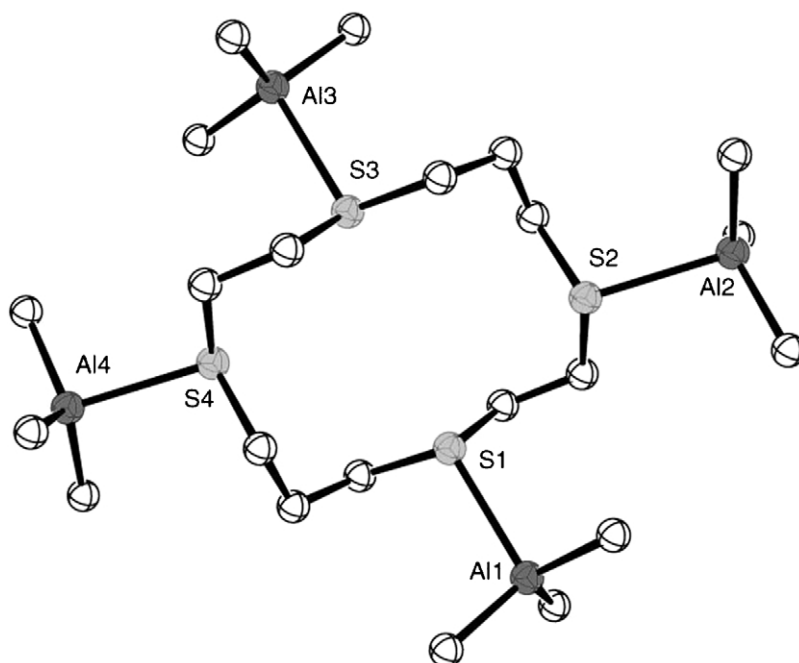
Figure 14 Solid-state structure of [\text{Me}_3\text{Al}]_4[14]\text{aneS}_4 .
