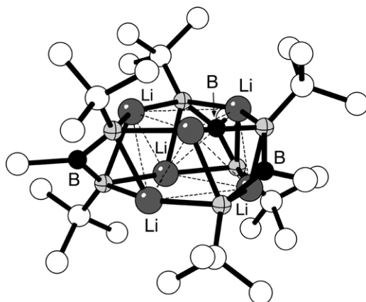
Figure 44 The structure of the hexametallic boraamidinate complex \{[\text{MeB}(\text{NBu}^t_2)_2]\text{Li}_2\}_3 .
