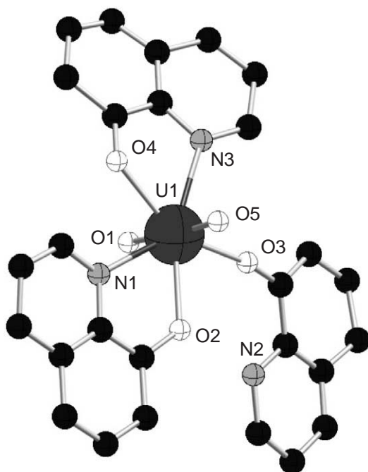
Figure 61 The structure of \text{UO}_2(\text{Ox})_2\text{HOx} \cdot \text{CHCl}_3 (Hall, Rae et al. Acta. Cris. 1987 , 22, 258).
