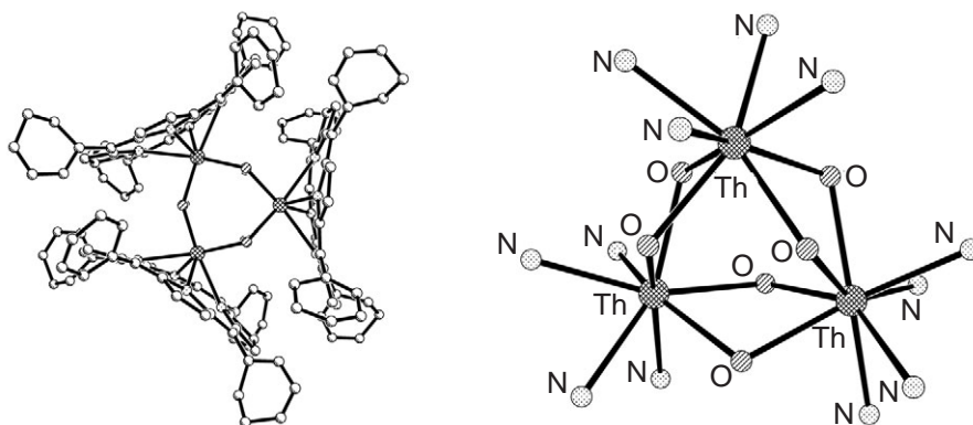
Figure 37 Crystal structure of [(\text{C}_{44}\text{H}_{28}\text{N}_4)_3\text{Th}(\text{OH})_2]_3 \cdot 2\text{H}_2\text{O} \cdot 3\text{C}_7\text{H}_6 (Kadish, Liu et al. J. Am. Chem. Soc. 1988 , 110, 6455–6462).
