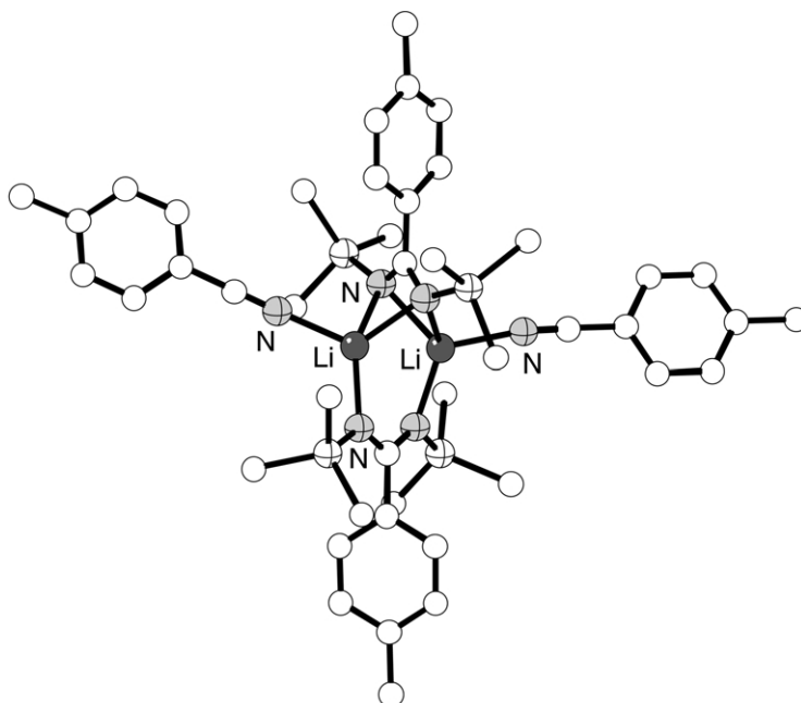
Figure 42 The structure of [4\text{-MeC}_6\text{H}_4\text{C}(\text{NSiMe}_3)_2]\text{Li}(\text{NCC}_6\text{H}_4\text{Me-4})_2 .
