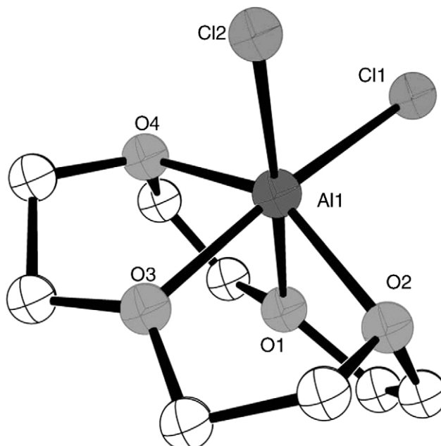
Figure 10 Solid-state structure of [\text{Cl}_2\text{Al}\cdot 12\text{-crown-4}]^+ cation.
