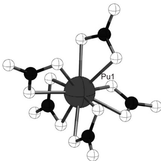
Figure 10 The pentacarboxato \text{Pu}^{\text{IV}} anion from the crystal structure of the hydrated sodium salt (Clark, Conradson et al. Inorganic Chemistry 1998 , 37, 2893–2899).
