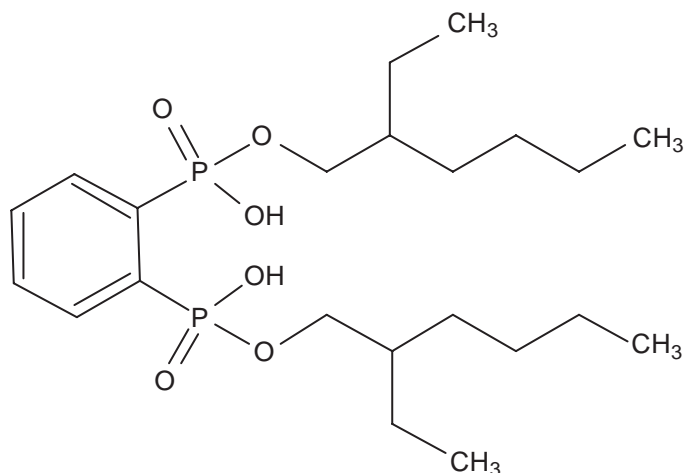
Figure 95 \text{H}_2\text{DEH}[1,2\text{-BzDP}] .
