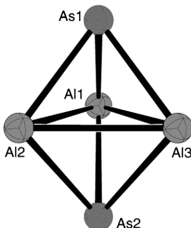
Figure 7 Solid-state structure of \text{As}_2\text{Al}_3 core of \text{As}_2[\text{AlCp}^*]_3 .
