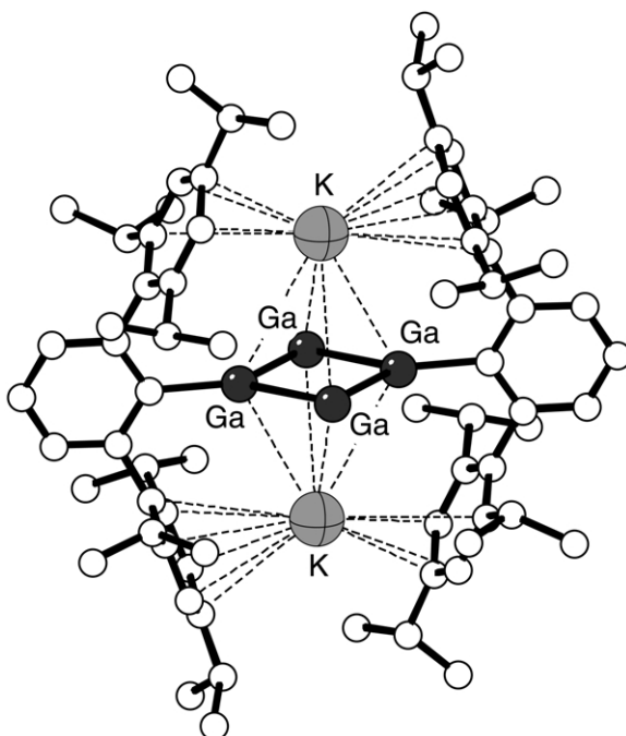
Figure 4 The structure of \text{K}_2[\text{Ga}_4(\text{C}_6\text{H}_3\text{-}2,6\text{-(}2,4,6\text{-(Pr}^i\text{)}_3\text{C}_6\text{H}_2)_2] , illustrating the \text{K}^+ –phenyl interactions.
