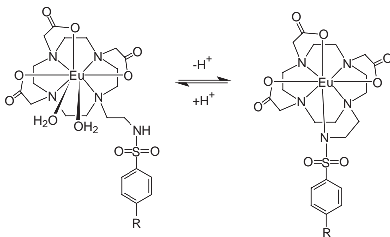
Scheme 6
