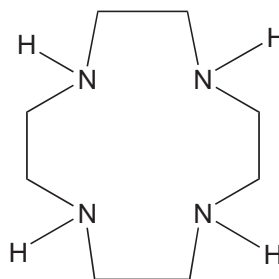
cyclen
