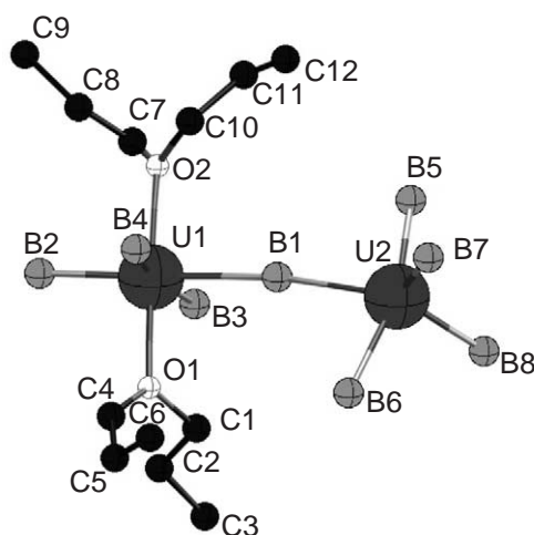
Figure 39 Crystal structure of (n\text{-Pr}_2\text{O})_2(\eta^3\text{-BH}_4)_3\text{U}(\mu\text{-}\eta^2, \eta^2\text{-BH}_4)\text{U}(\eta^3\text{-BH}_4)_4 (Zalkin, Rietz et al. Inorg. Chem. 1978 , 17, 661).
