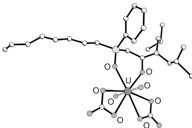
Figure 70 Crystal structure of \text{UO}_2(\text{NO}_3)_2(\text{C}_{24}\text{H}_{42}\text{PO}_2\text{N}) (Cherfa, Pécaut et al. Z. Kristallogr.-New Crys. Struct. 1999 , 214, 523–525).
