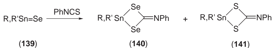
Scheme 25
