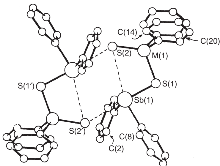
Figure 40 The structure of [Ph 2 Sb(S 2 SPPH 2 )] (reproduced by permission of the Royal Society of Chemistry from J. Chem. Soc., Dalton Trans. 1986 , 1031–1034).
