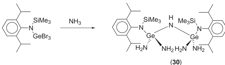
Scheme 11
