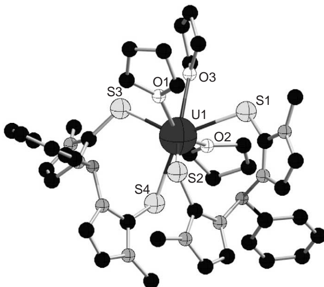
Figure 4 Crystal structure of \{U[H(R)B(timMe)_2]_2(THF)_2\}\{BPh_4\} (Maria, Domingos et al. Inorg. Chem. 2001 , 40 , 6863).
