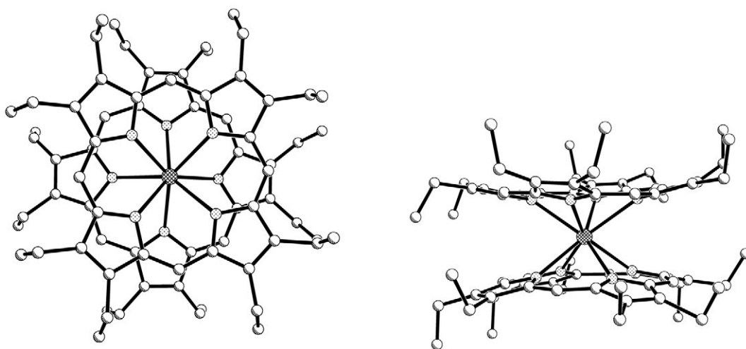
Figure 35 Crystal structure of \text{Th}(\text{C}_{36}\text{H}_{44}\text{N}_4)_2 (top and side views) (Girolami, Gorlin et al. Journal of Coordination Chemistry 1994 , 32, 173–212).
