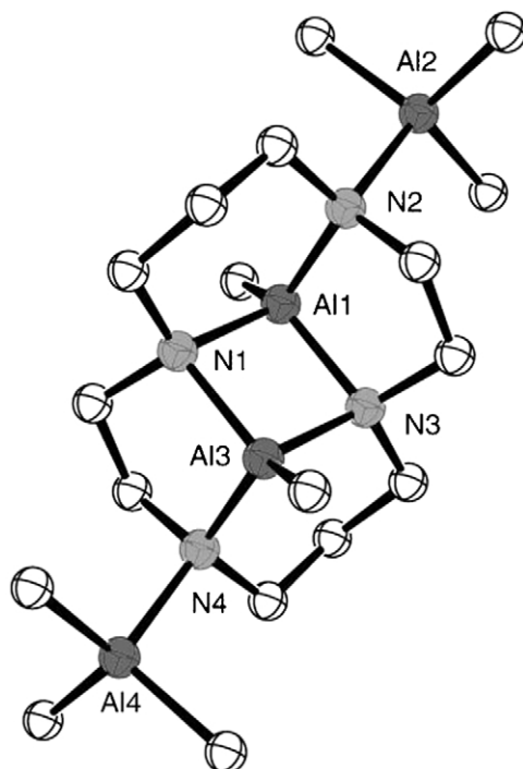
Figure 6 Solid-state structure of [Me 3 Al] 2 [14]aneN 4 [AlMe 2 ].
