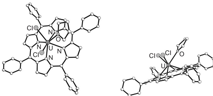
Figure 36 Crystal structure of \text{U}(\text{C}_{44}\text{H}_{28}\text{N}_4)\text{Cl}_2(\text{C}_4\text{H}_8\text{O}) (top and side views) (Girolami, Milam et al. Inorganic Chemistry 1987 , 26, 343–344).
