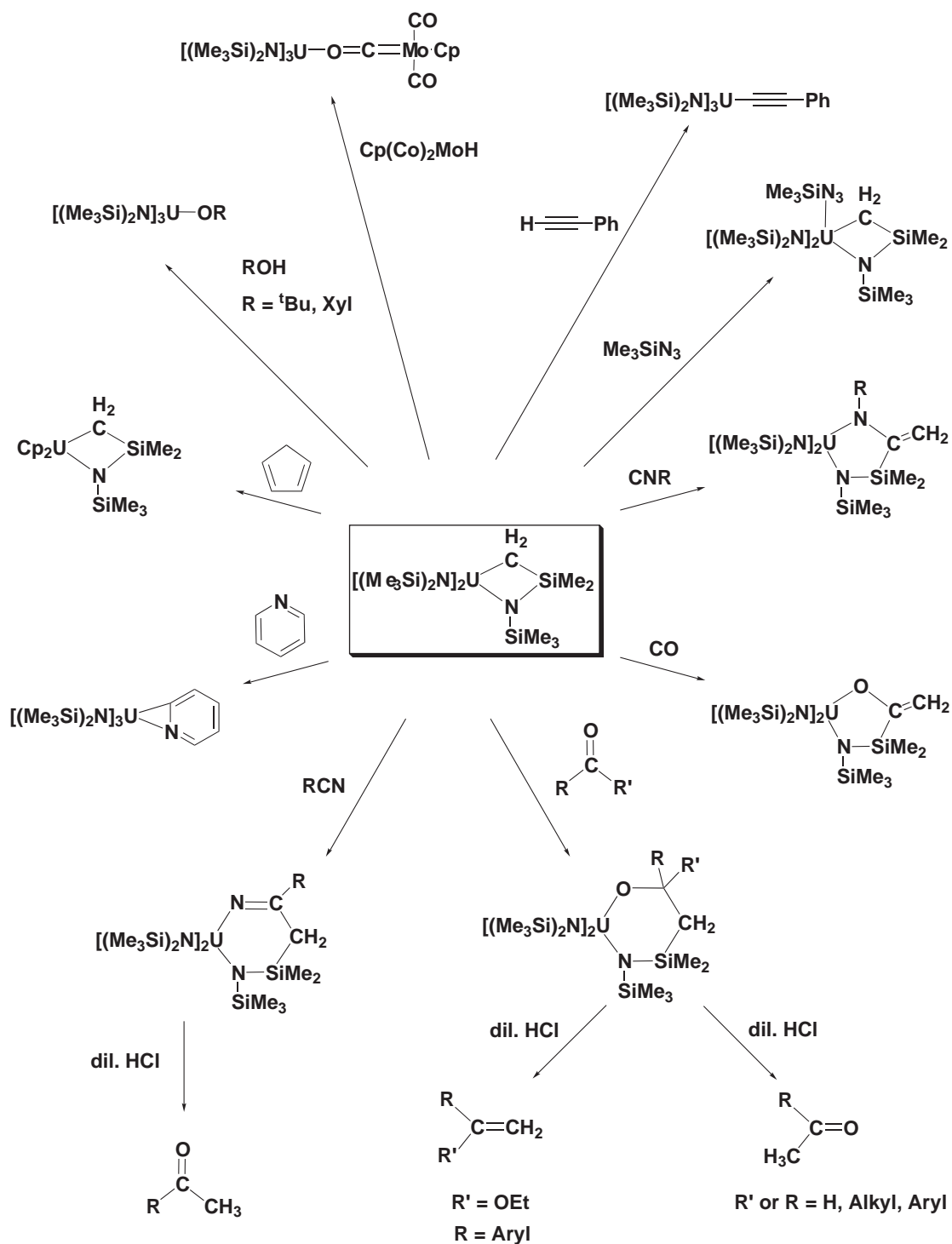
Figure 6 Reactions of uranium metallacycle \text{Ux}[\text{N}(\text{SiMe}_3)(\text{SiMe}_2\text{CH}_2)]_2[\text{N}(\text{SiMe}_3)_2]_2 .
