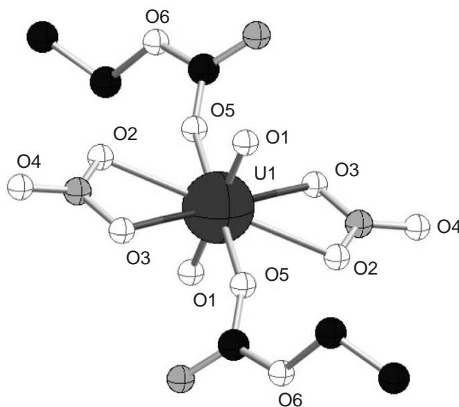
Figure 62 Structure of \text{UO}_2(\text{NO}_3)_2\text{L}_2 L = ethylcarbamate (Graziani, Bombieri et al. J. Chem. Soc., Dalton Trans. 1973, 451–454).
