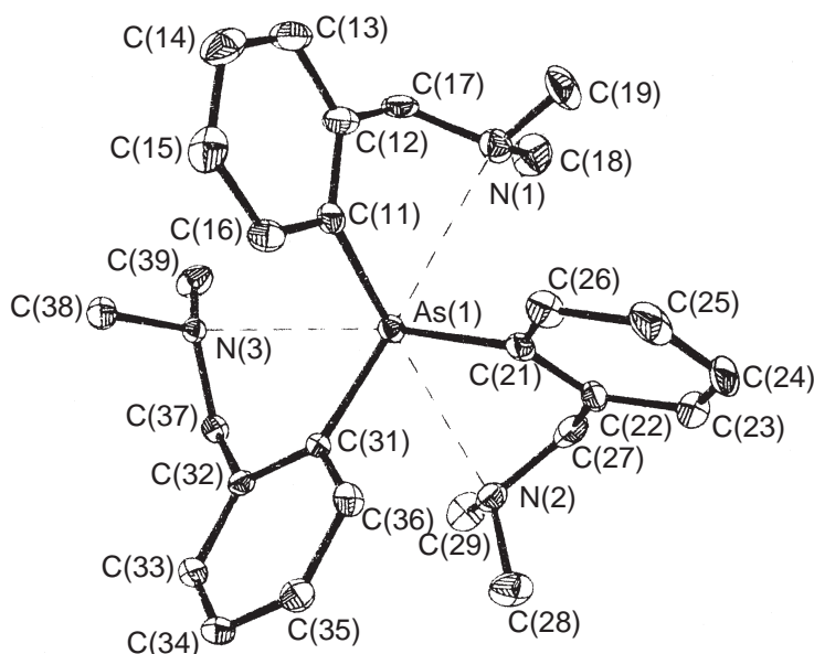
Figure 1 The structure of [\text{As}(\text{2-Me}_2\text{NCH}_2\text{C}_6\text{H}_4)_3] (reproduced by permission of the American Chemical Society from Inorg. Chem. 1996 , 35, 6179–6183).
