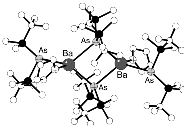
Figure 56 The structure of \{\text{Ba}[\text{As}(\text{SiMe}_2(\text{Bu}^t))_2]_2(\text{THF})\}_2 .
