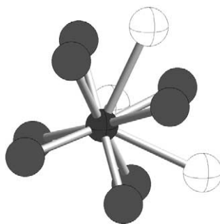
Figure 47 An unusual 11-coordinate \text{U}^{\text{IV}} within the extended structure of \text{U}_4\text{O}_9 with a pseudotricapped cubic geometry, where the longer, “capping” oxygens are shown in white (Bevan, Grey et al. J. Solid State Chem. 1986 , 61(1), 1–7).
