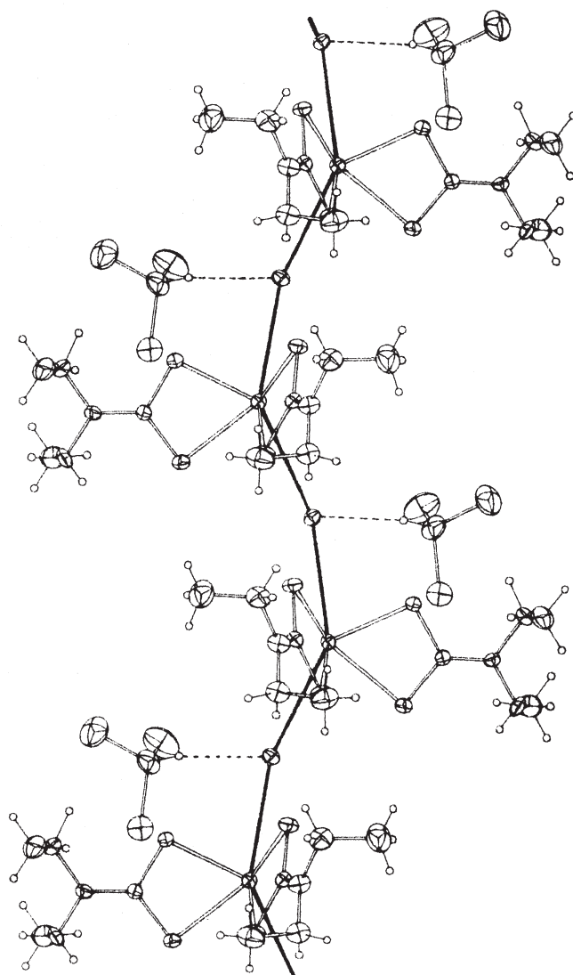
Figure 39 The polymeric chain in [\text{Sb}(\text{S}_2\text{CNEt}_2)_2\text{I}]\cdot\text{CHCl}_3 (reproduced by permission of the Royal Society of Chemistry from J. Chem. Soc., Dalton Trans. 1981 , 1360–1365).
