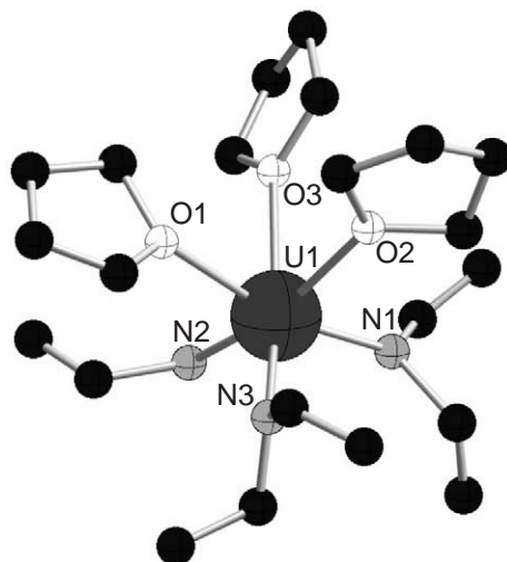
Figure 7 Crystal structure of [\text{U}(\text{NEt}_2)_3(\text{THF})_3][\text{BPh}_4] (Berthet, Boisson et al. J. Chem. Soc., Dalton Trans. 1995 , 3019).
