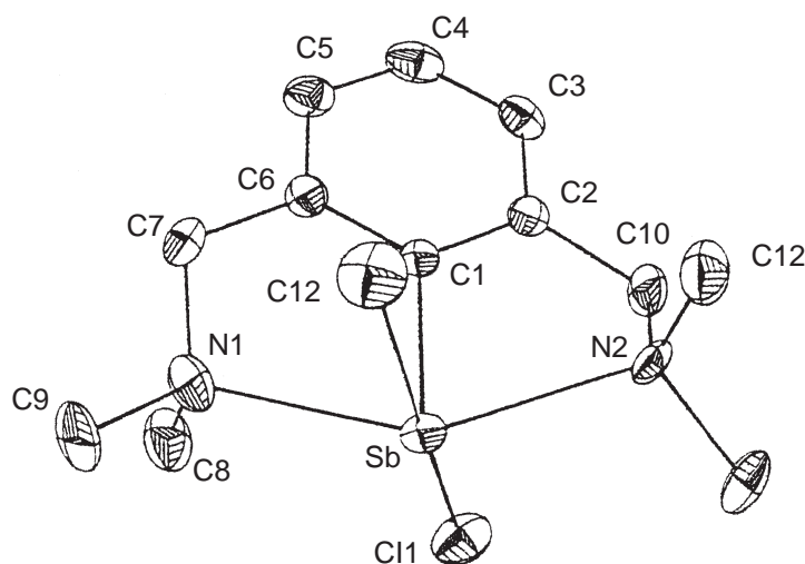
Figure 17 The structure of [\text{SbCl}_2\{2,6\text{-(Me}_2\text{NCH}_2)_2\text{C}_6\text{H}_3\}] (reproduced by permission of Elsevier Science from Inorg. Chim. Acta 1992 , 198–200, 271–274).
