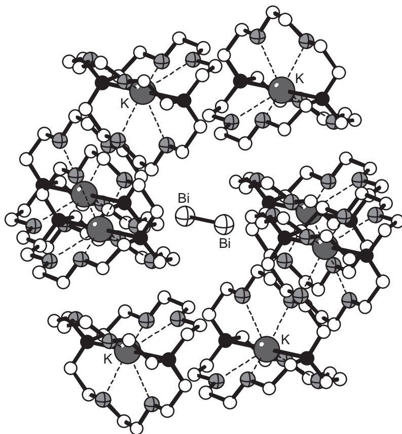
Figure 15 The [K([2.2.2]crypt)] salt of the Bi_2^{2-} anion.
