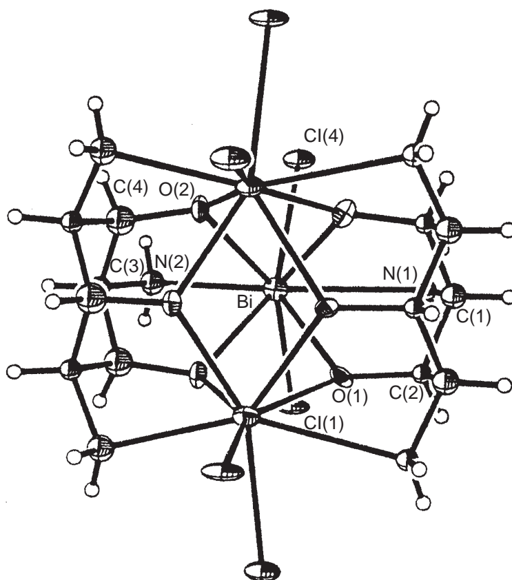
Figure 68 The structure of [\text{Bi}_3(\text{taci})_2]\text{Cl}_3 (reproduced by permission of the American Chemical Society from Inorg. Chem. 1993 , 32, 2699–2704).
