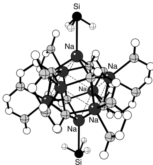
Figure 26 The structure of [\text{Na}_8(\text{OCH}_2\text{CH}_2\text{OCH}_2\text{CH}_2\text{OMe})_6(\text{SiH}_3)_2] , with its inverted \text{SiH}_3 moieties.
