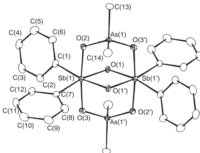
Figure 30 The structure of [(\text{Ph}_2\text{Sb})_2(\text{O})_2(\text{O}_2\text{AsMe}_2)_2] (reproduced by permission of the Royal Society of Chemistry from J. Chem. Soc., Dalton Trans. 1997 , 2785–2792).
