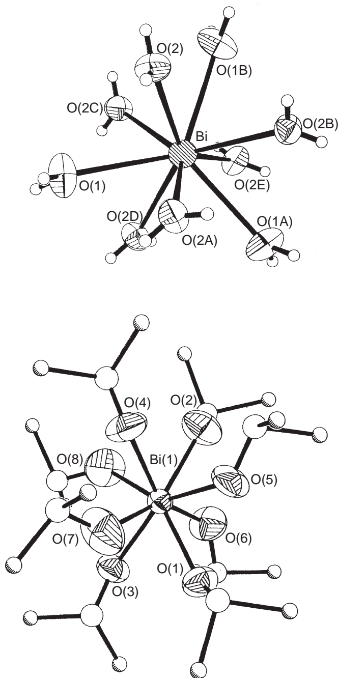
Figure 61 The structures of [\text{Bi}(\text{H}_2\text{O})_9]^{3+} and [\text{Bi}(\text{DMSO})_8]^{3+} (reproduced by permission of the American Chemical Society from Inorg. Chem. 2000 , 39, 4012–4021).
