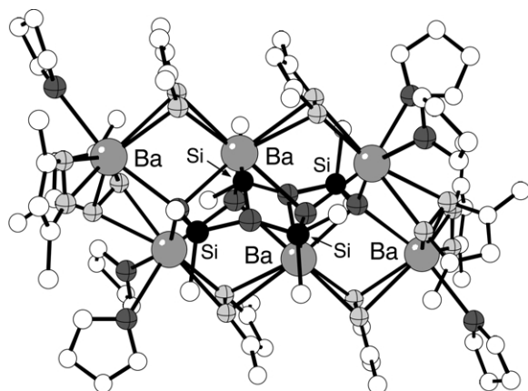
Figure 40 The structure of [(\text{THF})_6\text{Ba}_6(3,5\text{-dimethylpyrazolato})_8\{(\text{OSiMe}_2)_2\text{O}\}_2] .
