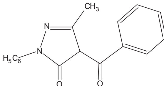
Figure 93 1-phenyl-3-methyl-4-benzoylpyrazolone-5 (HPMBP).
