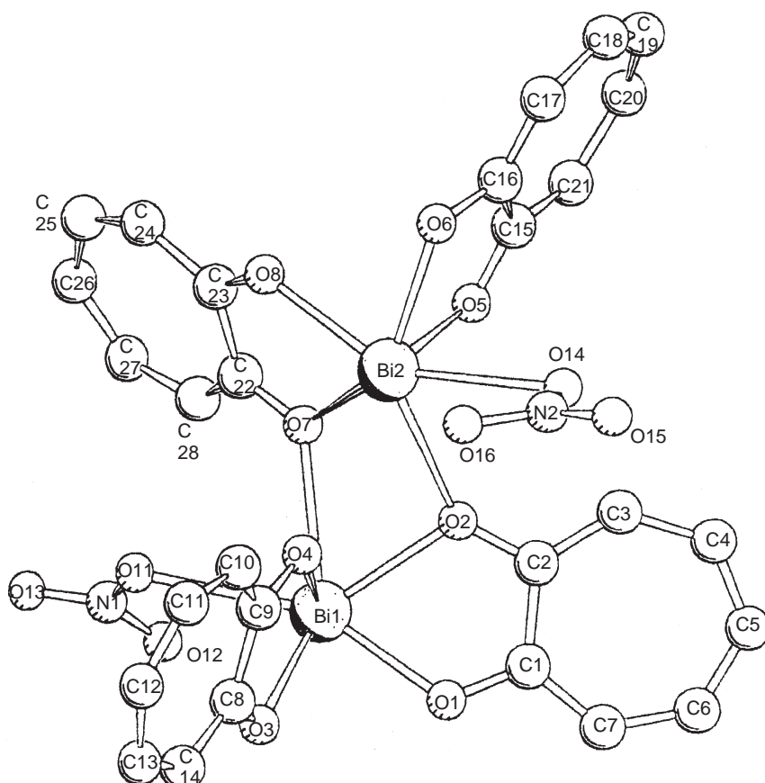
Figure 64 The structure of [\text{Bi}_2(\text{NO}_3)_2(\text{trop})_4] (reproduced by permission of Wiley-VCH from Chem. Ber. 1995 , 128, 335–342).
