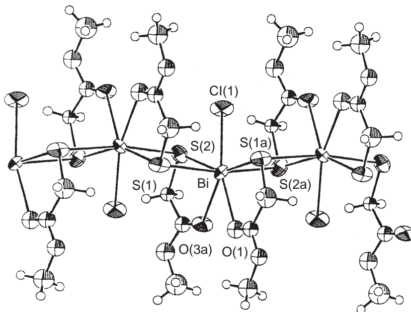
Figure 78 The polymeric unit in [\text{Bi}(\text{SCH}_2\text{CO}_2\text{Me})_2\text{Cl}] (reproduced by permission of the Royal Society of Chemistry from Chem. Commun. 2000 , 13–14).
