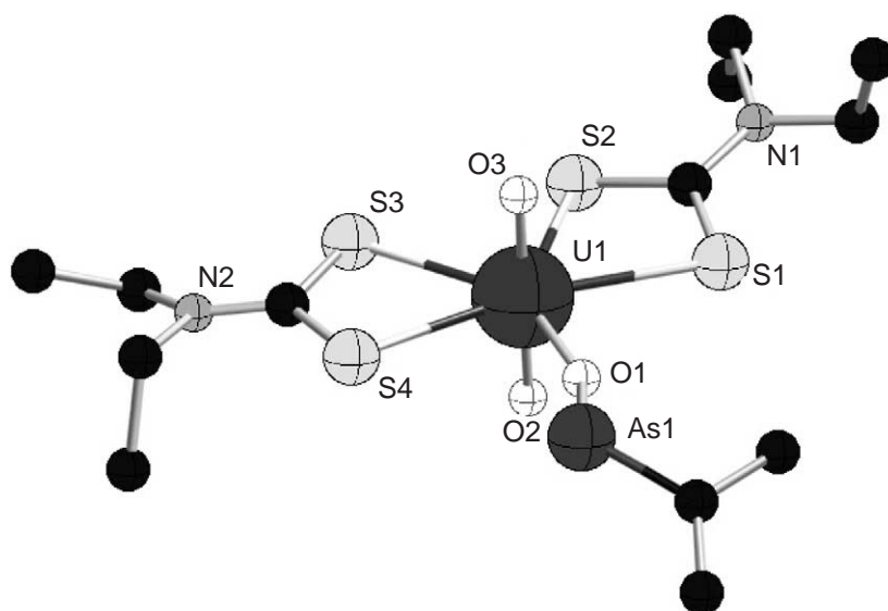
Figure 64 Structure of \text{UO}_2(\text{Et}_2\text{NCS}_2)_2 \cdot \text{L} , \text{L} = (\text{C}_6\text{H}_5)_3\text{AsO} , (\text{C}_6\text{H}_5)_3\text{PO} , and (\text{CH}_3)_3\text{NO} (Graziani, Zarli et al. Inorg. Chem. 1970 , 9 , 2116–1124; Forsellini, Bombieri et al. Inorg. Nucl. Chem. Lett. 1972 , 8 , 461–463).
