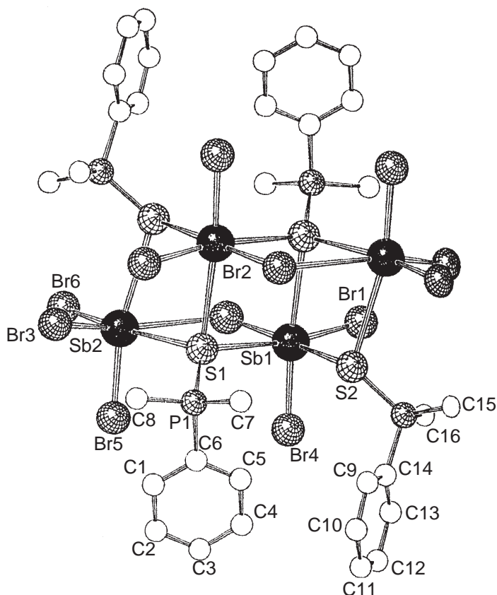
Figure 37 The tetrameric structure of [SbBr 3 (SPMe 2 Ph)] (reproduced by permission of the publishers from Z. Naturforsch., B 1990 , 45, 1355–1362).
