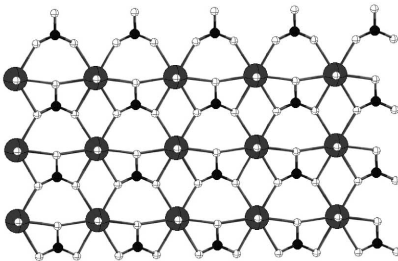
Figure 50 Uranyl carbonate layers in the crystal structure of the mineral rutherfordine, \text{UO}_2\text{CO}_3 (Finch, Cooper et al. Canadian Mineralogist 1999 , 37, 929–938).
