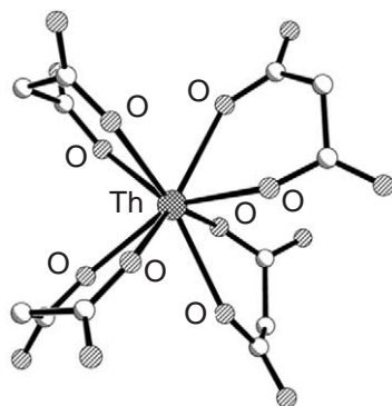
Figure 11 Crystal structure of (\text{C}_4\text{H}_{12}\text{N}_2)_2[\text{Th}(\text{C}_3\text{H}_2\text{O}_4)_4]\cdot\text{H}_2\text{O} (Zang, Collison et al. Polyhedron 2000 , 19, 1757–1767).
