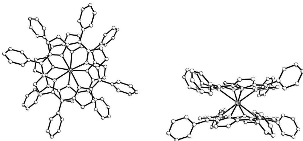
Figure 34 Crystal structure of [\text{Th}(\text{C}_{44}\text{H}_{28}\text{N}_4)_2] \cdot \text{C}_7\text{H}_8 (top and side views) (Girolami, Gorlin et al. Journal of Coordination Chemistry 1994 , 32, 173–212).
