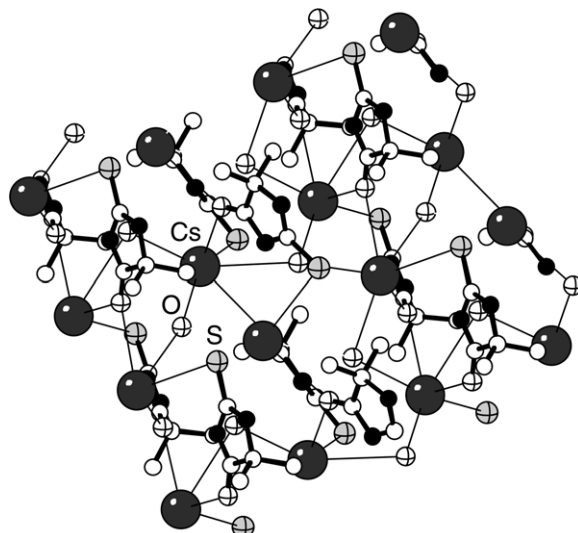
Figure 89 Portion of the lattice of (\text{Cs}(5,5\text{-dimethyl-4-oxoimidazolidine-2-thione})\text{OH})_\infty .
