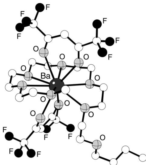
Figure 82 The structure of \text{Ba}(\text{HFA})_2 \cdot \text{CH}_3\text{O}(\text{CH}_2\text{CH}_2\text{O})_6\text{-}n\text{-C}_4\text{H}_9 .
