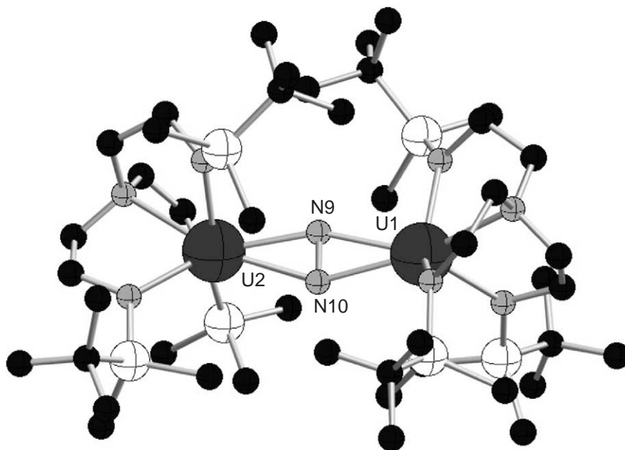
Figure 1 Crystal structure of \{N[CH_2CH_2N(Si(Bu^t)Me_2)U]_2(\mu^2-\eta^2: \eta^2-N_2)\} (Roussel and Scott J. Am. Chem. Soc. 1998 , 120 , 1070).
