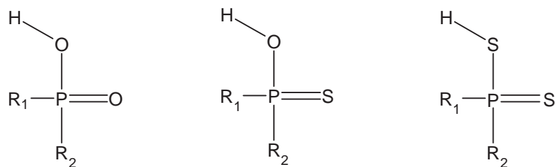
Figure 88 General diagrams of phosphinic acid, monothiophosphinic acid and dithiophosphinic acid, respectively.
