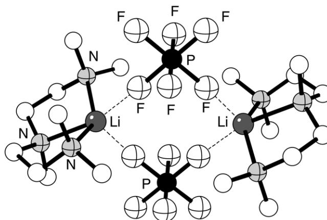
Figure 101 The structure of [(\text{PMDETA})\text{LiPF}_6]_2 .
