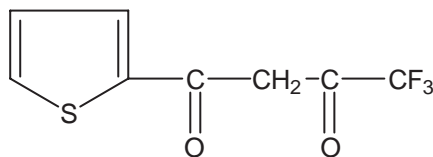
Figure 92 Thenoyltrifluoroacetone (HTTA).
