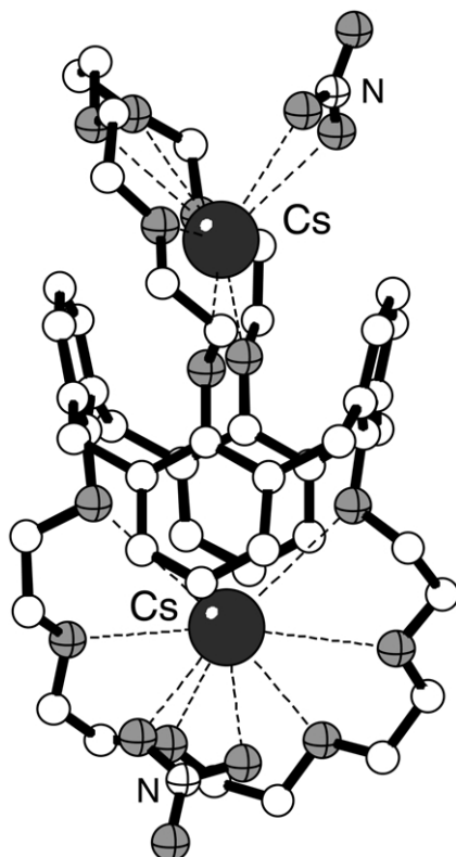
Figure 17 Dinitrato derivative of \text{Cs}^+ and 1,3-calix[4]-bis-crown-6.
