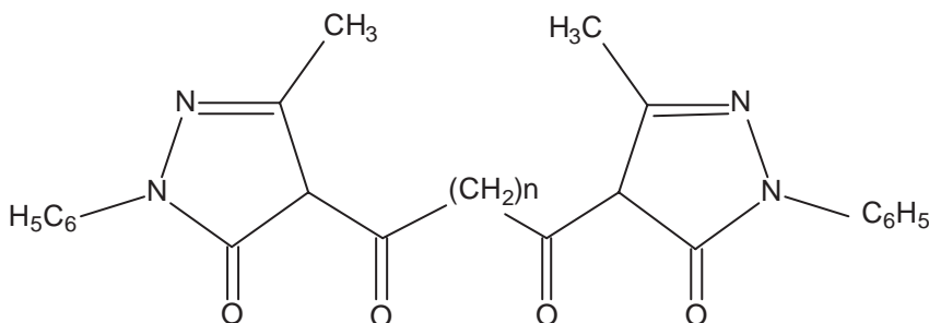
Figure 94 Bis(1-phenyl-3-methyl-4-acylpyrazol-5-one) ( \text{H}_2\text{BP}_n ) ( n = 3-8, 10 or 22 ).
