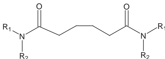
Figure 72 General diagram of an adipicamide.
