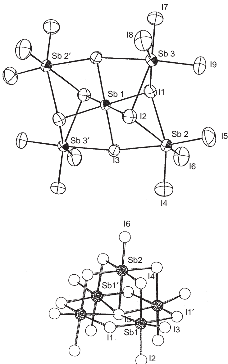
Figure 52 The structures of two forms of [\text{Sb}_5\text{I}_{18}]^{3-} (reproduced by permission of (a) Elsevier Science from Polyhedron 1993 , 12, 2081–2090, and (b) Wiley-VCH from Angew. Chem. Int. Ed. Engl. 1989 , 28, 344–345).
