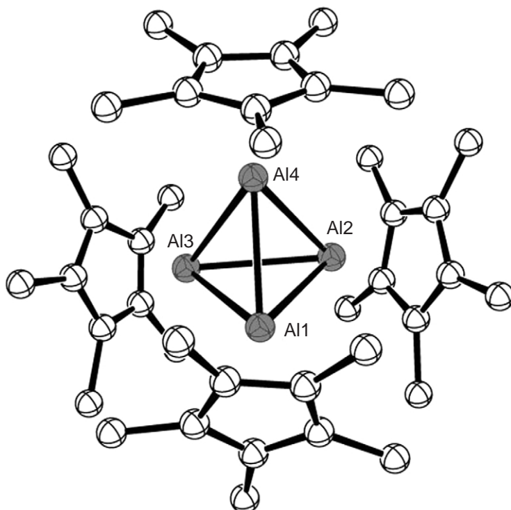
Figure 19 Solid-state structure of [(\text{C}_5\text{Me}_5)\text{Al}]_4 .
