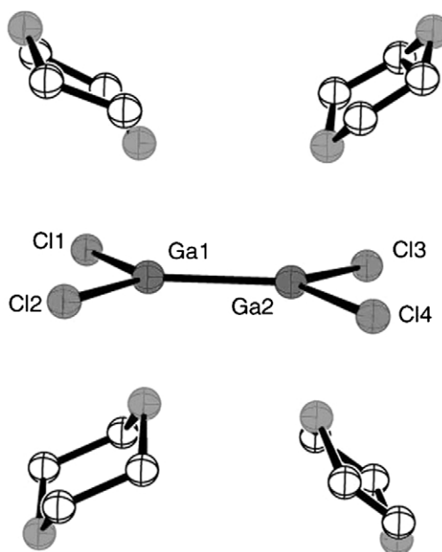
Figure 29 Solid-state structure of \text{Cl}_2\text{Ga-GaCl}_2(\text{dioxane})_4 .
