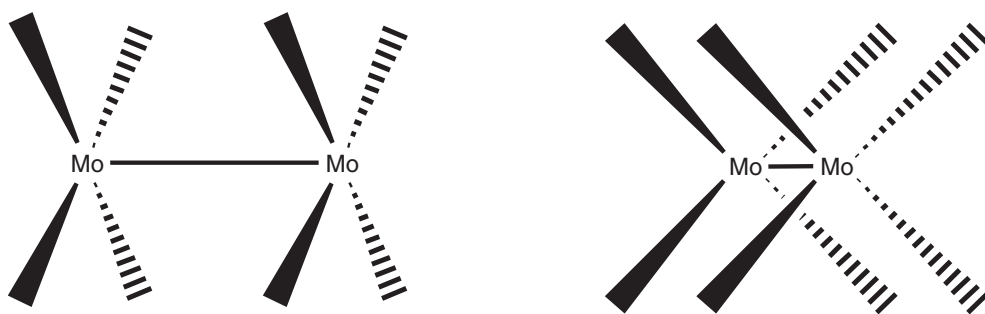
Figure 53 Structural motif of \text{Mo}_2^{\text{II,II}} complexes both perpendicular to and along the metal–metal axis.
