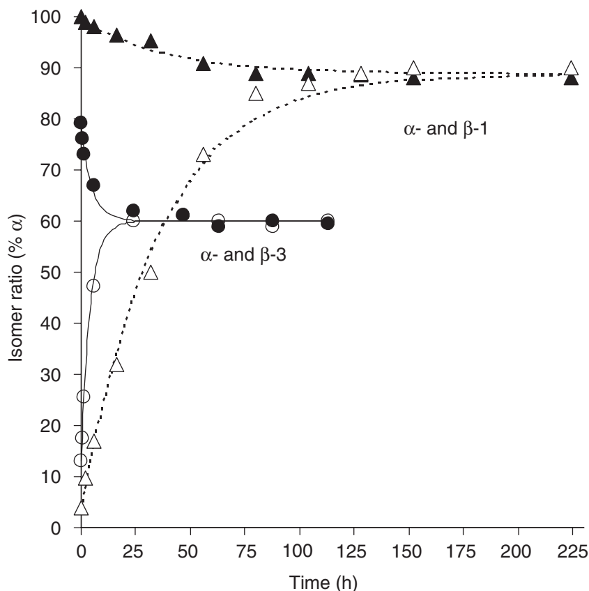
Figure 8 Isomerization of \alpha - \text{AlW}_{12}\text{O}_{40}^{5-} ( \alpha -(1); black triangles) and \beta - \text{AlW}_{12}\text{O}_{40}^{5-} ( \beta -(1); open triangles) and of \alpha - \text{Na}_9\text{AlW}_{11}\text{O}_{39} ( \alpha -(3); black circles) and \beta - \text{Na}_9\text{AlW}_{11}\text{O}_{39} ( \beta -(3); open circles). Approach to equilibrium between \alpha -(1) and \beta -(1) shown by dashed curves; approach to equilibrium between solutions initially containing mostly \alpha -(3) (82% \alpha , 18% \beta ) and mostly \beta -(3) (87% \beta , 13% \alpha ) in \text{D}_2\text{O} is shown by solid curves (reprinted with permission from J. Am. Chem. Soc. 1999 , 121, 4608–4617; © American Chemical Society).
