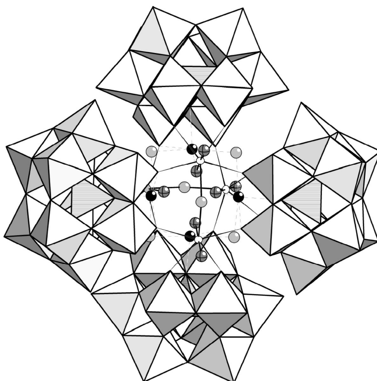
Figure 26 [\{\text{M}(\text{OH}_2)\}_4(\text{UO}_2)_4(\text{OH})_2(\gamma\text{-SiW}_{10}\text{O}_{36})_4]^{22-} .
