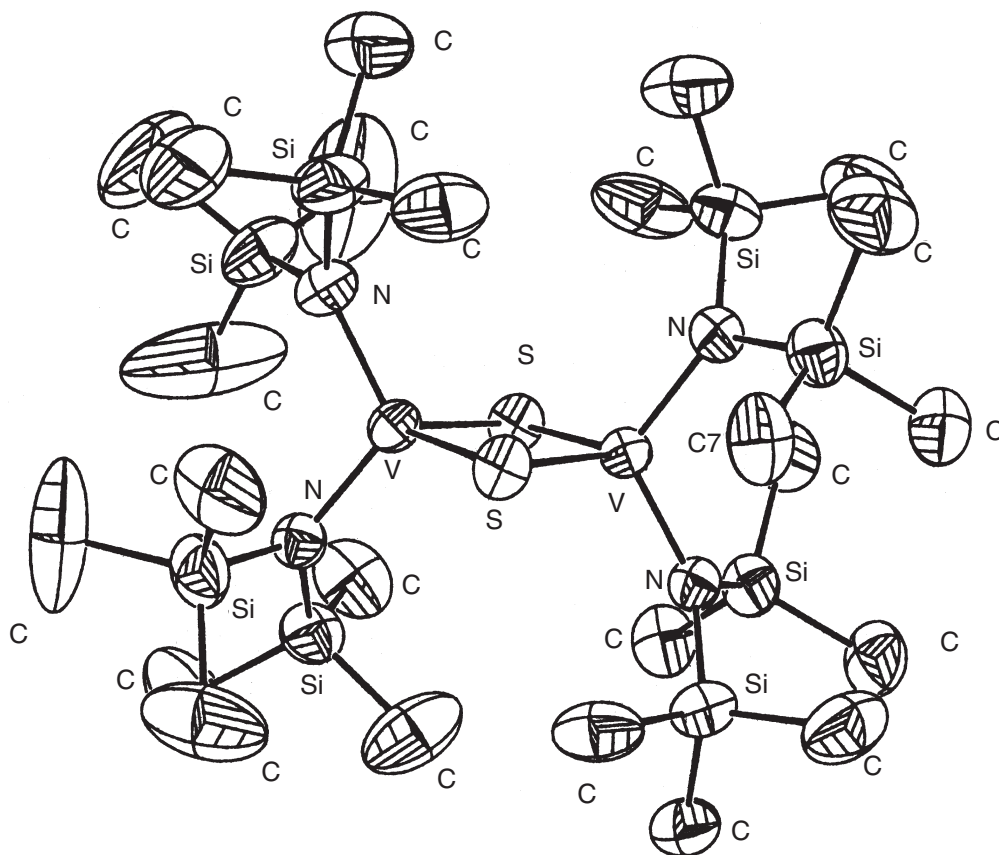
Figure 6 ORTEP drawing of V_2(\mu\text{-S})_2[\text{N}(\text{Si}(\text{CH}_3)_3)_2] (reproduced by permission of the American Chemical Society from Inorg. Chem. 1997 , 36, 2191–2194).
