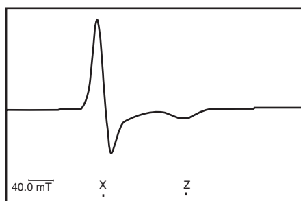
Figure 42 ESR spectrum of [Mo 4 S 4 (H 2 O) 12 ] 5+ (2 mM) in 2.0 M Hpts at 3.8 K, with microwave frequency 9.25 GHz, power 20 mV and gain 1.25 \times 10^{-3} . 6
