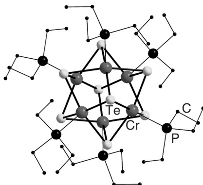
Figure 24 Structure of the [\text{Cr}_6\text{Te}_8(\text{PET}_3)_6] molecule.
