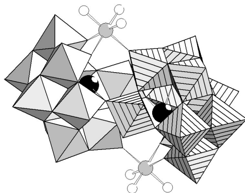
Figure 13 The structure of [X 2 W 22 O 74 (OH) 2 ] 12− . Two (or all four) of the sandwiched tungsten atoms can be replaced by other metal cations; see Table 17.
