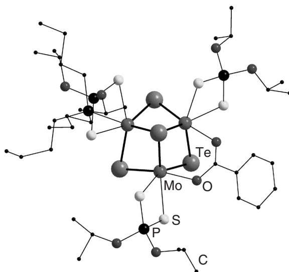
Figure 32 Structure of the [\text{Mo}_3\text{Te}_4((i\text{PrO})_2\text{PS}_2)_3(\mu\text{-C}_6\text{H}_5\text{CO}_2)(\text{PBu}_3)] molecule.
