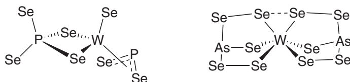
Figure 16 Schematic drawing [(\text{PSe}_2)\text{W}(\text{Se})(\text{PSe}_4)]^{2-} and [\text{W}(\text{AsSe}_5)_2]^{2-} .
