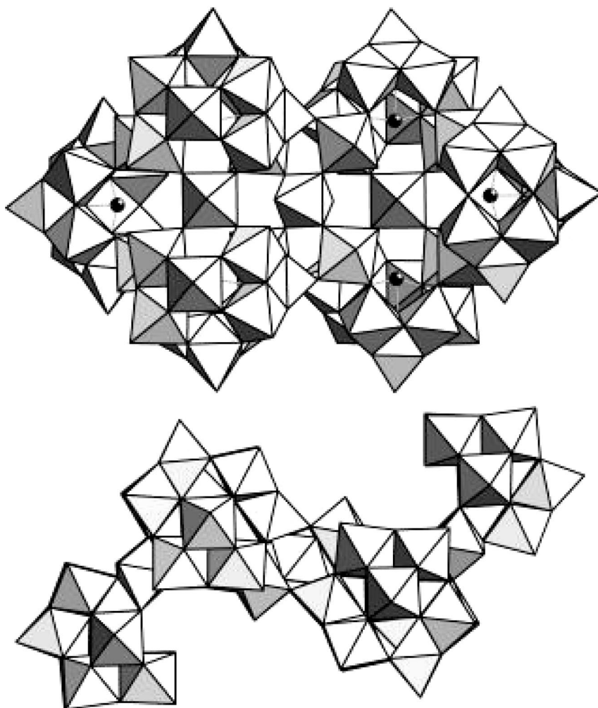
Figure 29 [\text{As}_6\text{W}_{65}\text{O}_{217}(\text{H}_2\text{O})_7]^{26-} .
