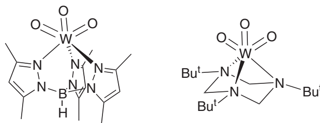
Figure 8 Schematic drawing of [LWO_3]^- ( L = \text{hydrotris}(3,5\text{-dimethylpyrazol-1-yl})\text{borate} ) and [(t-Bu_3tach)W(O)_3] ( t-Bu_3tach = 1,3,5 -tri- tert -butyl-1,3,5-triazacyclohexane).
