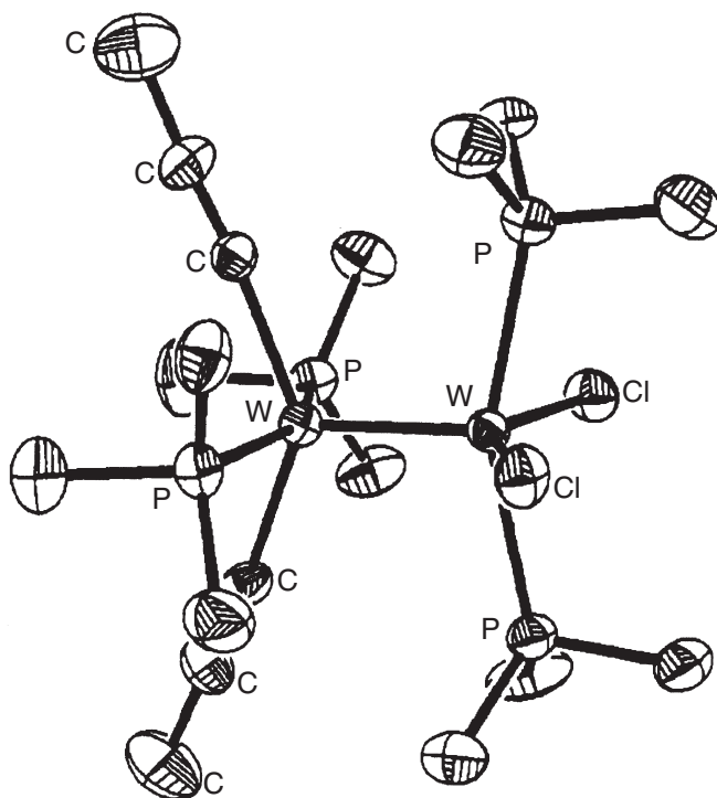
Figure 66 ORTEP drawing of W_2(CCCH_3)_2Cl_2(P(CH_3)_3)_4 (reproduced by permission of the American Chemical Society from J. Am. Chem. Soc. 1992 , 114, 4201–4204).
