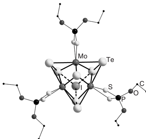
Figure 39 Structure of the [\text{Mo}_3\text{Te}_7((\text{EtO})_2\text{PS}_2)_3]\text{I} molecule.
