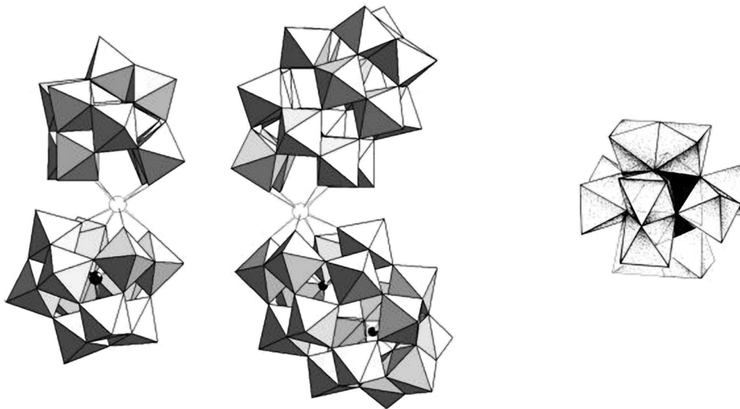
Figure 19 (a) Weakley-type [\text{LnL}_2]^{n-} complexes; (b) [\text{X}^{\text{IV}}\text{Mo}_{12}\text{O}_{42}]^{8-} .
