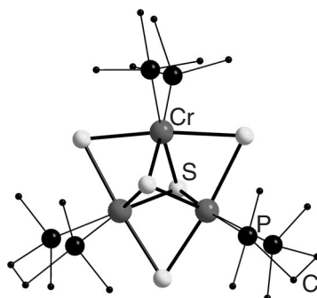
Figure 22 Structure of the [\text{Cr}_3\text{S}_5(\text{dmpe})_3] molecule.
