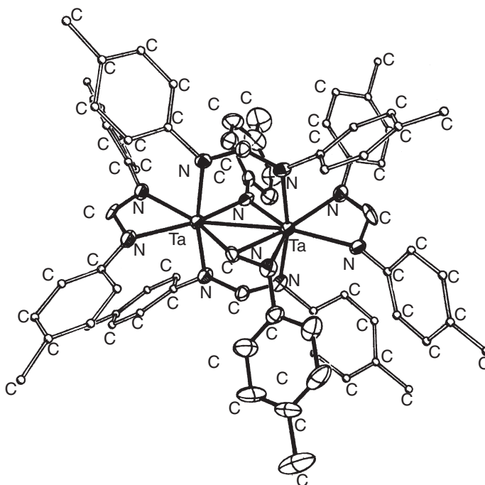
Figure 24 ORTEP drawing of (\eta^2\text{-C}_6\text{H}_5\text{NC(H)NC}_6\text{H}_5)_2\text{Ta}(\mu\text{-NC}_6\text{H}_5)(\mu\text{-}\eta^2\text{-C}_6\text{H}_5\text{NC(H)NC}_6\text{H}_5)_2(\mu\text{-}\eta^2\text{-CNC}_6\text{H}_5)_2\text{Ta}(\eta^2\text{-C}_6\text{H}_5\text{NC(H)NC}_6\text{H}_5) (reproduced by permission of the American Chemical Society from Inorg. Chem. 1997 , 36, 896–901).
