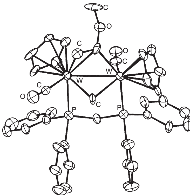
Figure 63 CAMERON drawing of the structure of the cation of [\text{W}_2(\mu\text{-CH}_2)\{\mu\text{-}\eta^1:\eta^2\text{-C}(\text{OCH}_3)\text{CH}_2\}(\eta^5\text{-C}_5\text{H}_5)_2(\text{CO})_2(\mu\text{-dppm})]\text{BF}_4 (reproduced by permission of the American Chemical Society from Organometallics 2002 , 21, 1177–1183).
