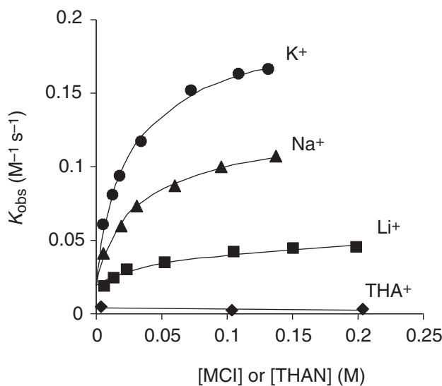
Figure 5 Rate of the outer-sphere electron-transfer oxidation of an organic substrate by a POM (oxidation of 3,3',5,5'-tetra-Bu t -biphenyl-4,4'-diol by \alpha -SiVW 11 O 40 5- to form \alpha -SiV IV W 11 O 40 6- and the DPQ in ~100% selectivity; Equation (12)) as a function of the cation concentration (counterions + added MCl), M^+ = K^+ (top curve); Na^+ (second curve from top); Li^+ (third curve from top), and THA + (the nitrate salt of the nonpairing cation, tetra- n -heptylammonium; bottom curve) (reprinted with permission from J. Am. Chem. Soc. 2001 , 123, 5292–5307; © American Chemical Society).
