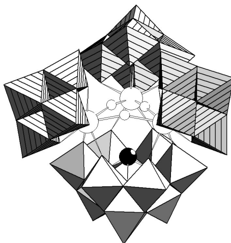
Figure 21 [\text{Eu}_3(\text{H}_2\text{O})_3(\text{SbW}_9\text{O}_{33})(\text{W}_5\text{O}_{18})_3]^{18-} .
