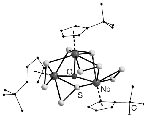
Figure 15 Structure of the [(\eta^5\text{-}^t\text{BuC}_5\text{H}_4)_3\text{Nb}_3(\mu_3\text{-O})(\text{S}_2)_5] molecule.
