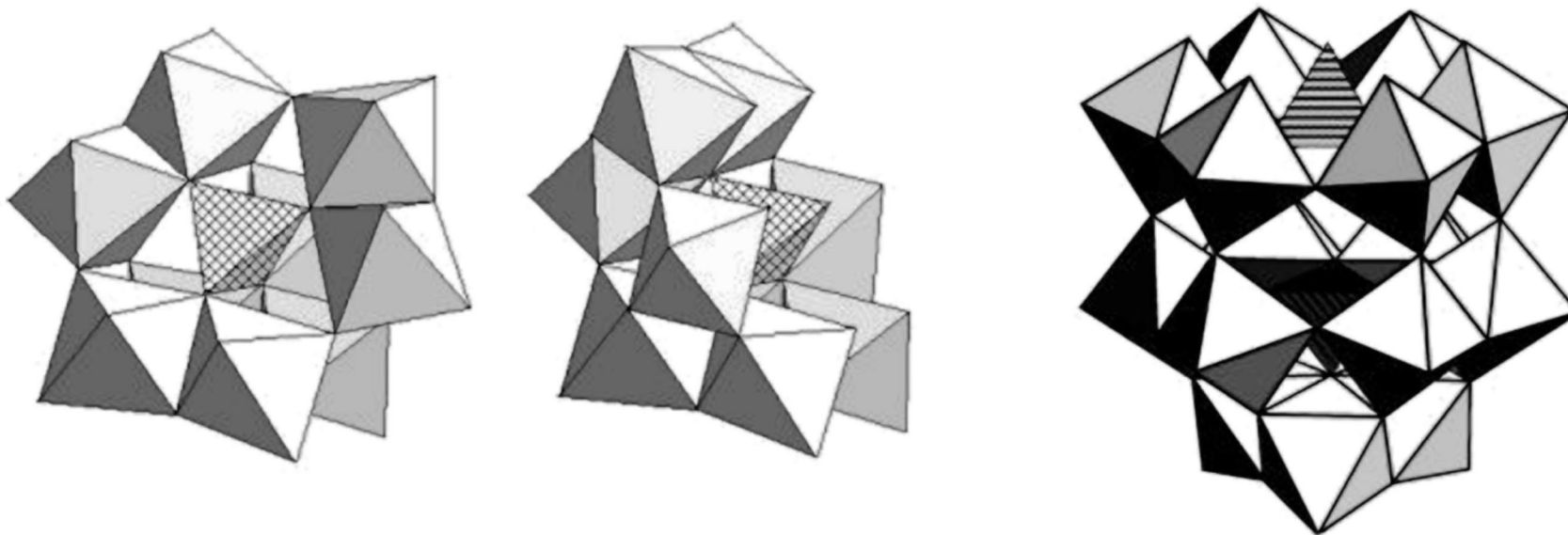
Figure 12 Trivalent \alpha -Keggin (A- and B-type) and Wells-Dawson structures.
