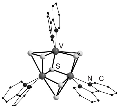
Figure 10 Structure of the [V_3S_7(bpy)_3]^+ cation.
