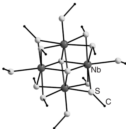
Figure 18 Structure of the [\text{Nb}_4(\text{S})_2(\text{SPh})_{12}]^{4-} anion. Only C atoms bonded to S are shown.
