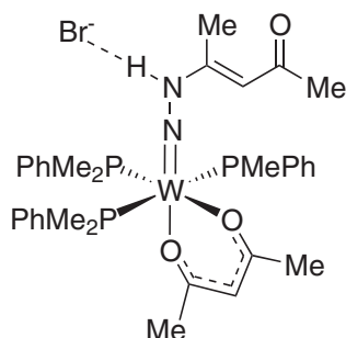
Figure 17 Schematic drawing of mer - [\text{W}(\text{acac})(\text{NNHCOMeCHCOMe})(\text{PMe}_2\text{Ph})_3]\text{Br} .
