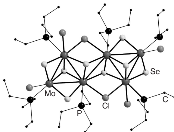
Figure 58 Structure of the [\text{Mo}_6\text{Se}_8\text{Cl}_6(\text{PEt}_3)_6] molecule.
