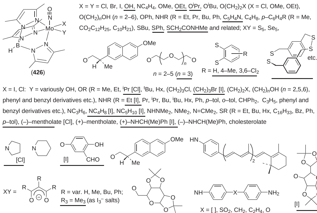
Figure 2 Nitrosyl- \text{Mo}^{\text{II}} complexes of \text{Tp}^* .
