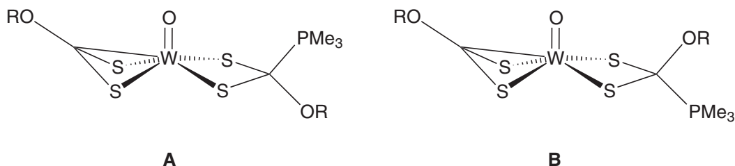
Figure 20 Two isomers of [WO\{S_2C(PMe_3)OR-S,S'\}(S_2COR-S,S',C)] ( R = ME, Et, i -Pr).
