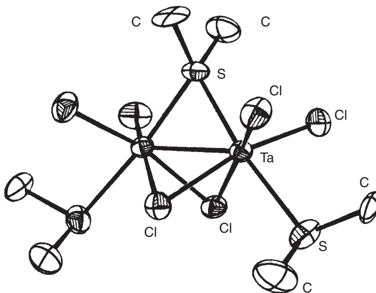
Figure 32 ORTEP drawing of \text{Ta}_2\text{Cl}_6(\text{S(CH}_3)_2)_3 (reproduced by permission of the American Chemical Society from Inorg. Chem. 1981 , 20, 2716–2719).
