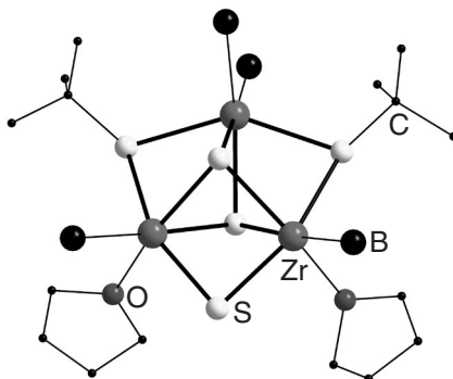
Figure 2 Structure of the [\text{Zr}_3(\mu_3\text{-S})_2(\mu\text{-}^t\text{BuS})_2(\mu\text{-S})(\text{BH}_4)_4(\text{THF})_2] molecule.
