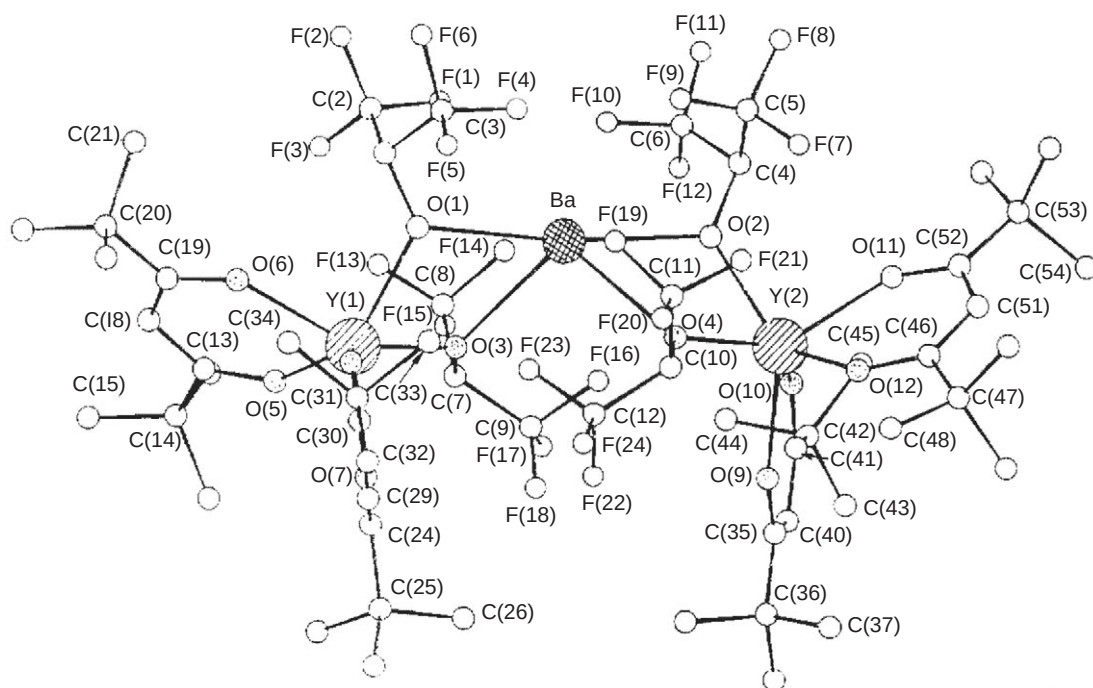
Figure 11 The molecular structure of \text{Y}_2\text{Ba}[\text{OCH}(\text{CF}_3)_2]_4(\text{dmp})_4 (where \text{dmp} = \text{Bu}^t\text{C}(\text{O})\text{CHC}(\text{O})\text{Bu}^t ) (reproduced by permission of The Royal Society of Chemistry from J. Chem. Soc., Chem. Commun. , 1993 , 1556–1558).
