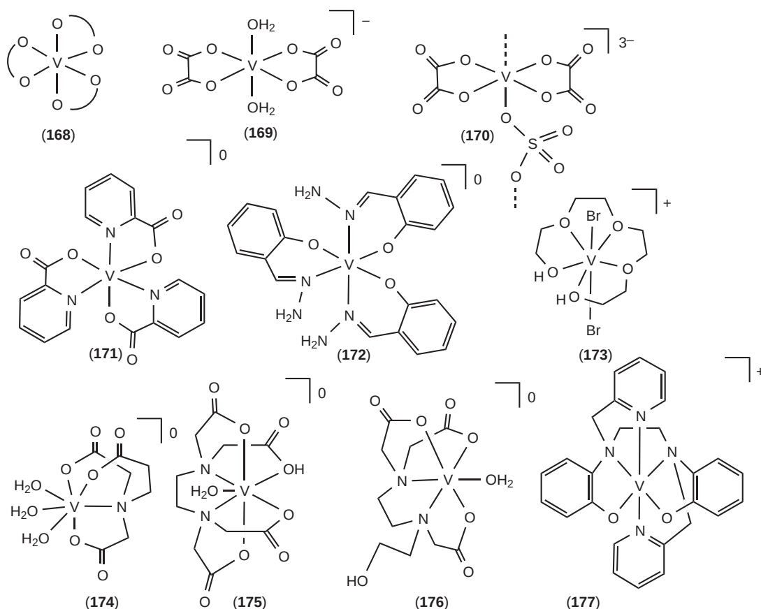
Figure 15 Structural illustrations of (168–177). The charges are given for structures and for structure types in which all the complexes have the same charge. For structure types that have differently charged ligands, no charge is given.
