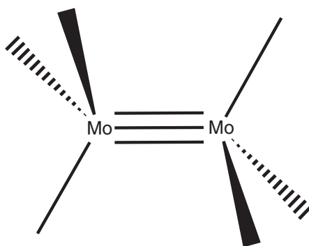
Figure 50 Triply bonded ethane-like d^3\text{--}d^3 molecules
