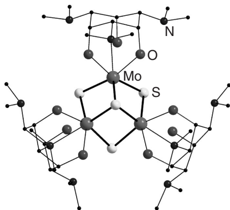
Figure 28 Structure of the [Mo_3S_4(L-4H)_4] (L = 1,3-diamino-5-(isopropylidenamino)-1,3,5-trideoxy-cis-inositol) molecule.
