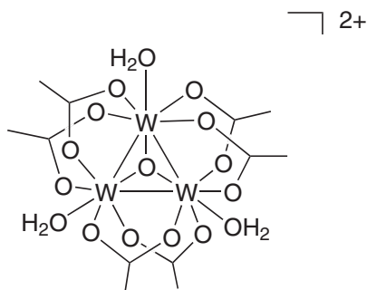
Figure 34 Hemicapped trinuclear structure in [W_3(\mu_3-O)(O_2CCH_3)_6(H_2O)_3][ZnBr_4] \cdot 8H_2O .
