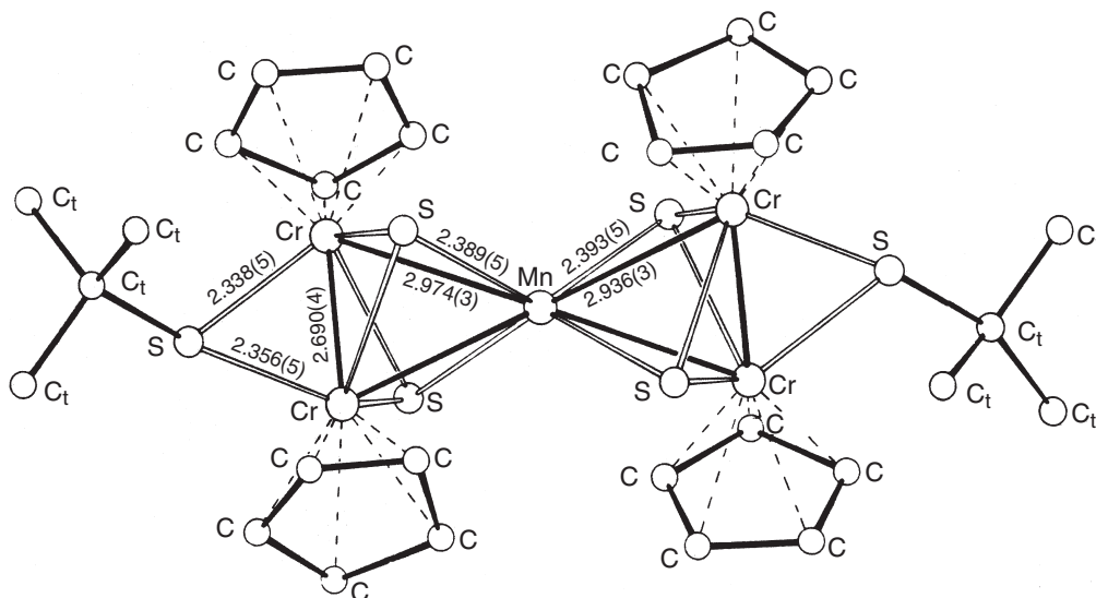
Figure 35 The structure of [(\eta^5\text{-C}_5\text{H}_5)_2\text{Cr}_2(\text{SC}(\text{CH}_3)_3)(\mu_3\text{-S})_2]\text{Mn} (reproduced by permission of Elsevier Science from J. Organomet. Chem. 1984 , 275, 183–189).
