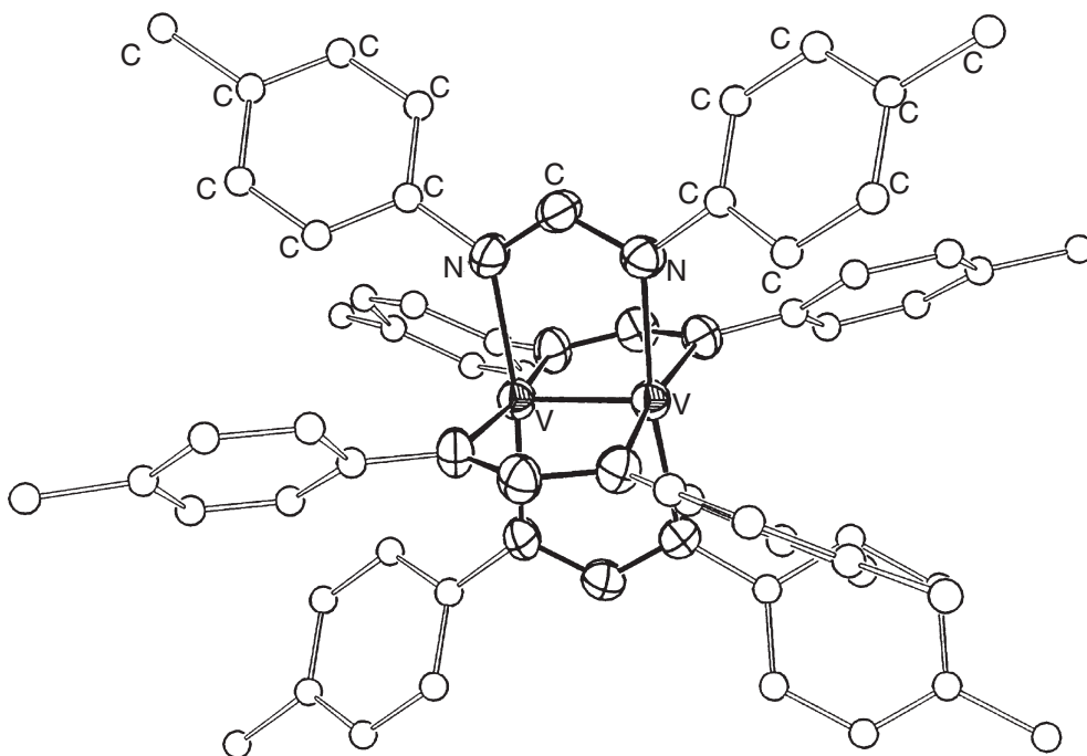
Figure 11 ORTEP drawing of V_2[((p-CH_3C_6H_4)_2N)_2C(H)]_4 (reproduced by permission of Wiley-VCH from Angew. Chem., Int. Ed. Engl. Engl. 1992 , 31, 737–738).
