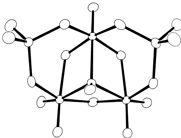
Figure 4 [\text{Mo}_3\text{O}_8(\text{OMe})(\text{MoO}_4)_2]^{3-} (reprinted with permission from Chen, Q.; Ma, L.; Liu, S.; Zubieta, J. J. Am. Chem. Soc. 1989 , 111 , 5944–5946. © 1989 American Chemical Society).
