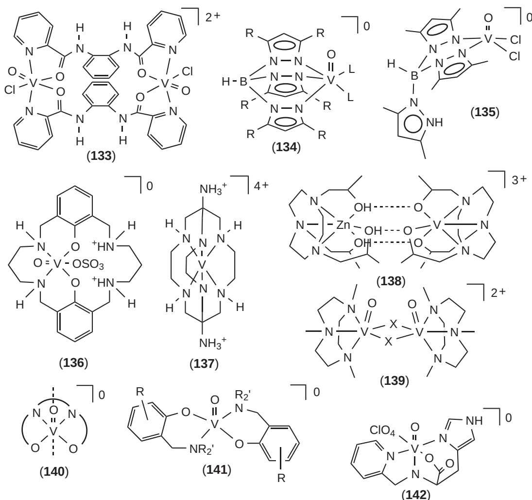
Figure 12 Structural illustrations of (133–142).
