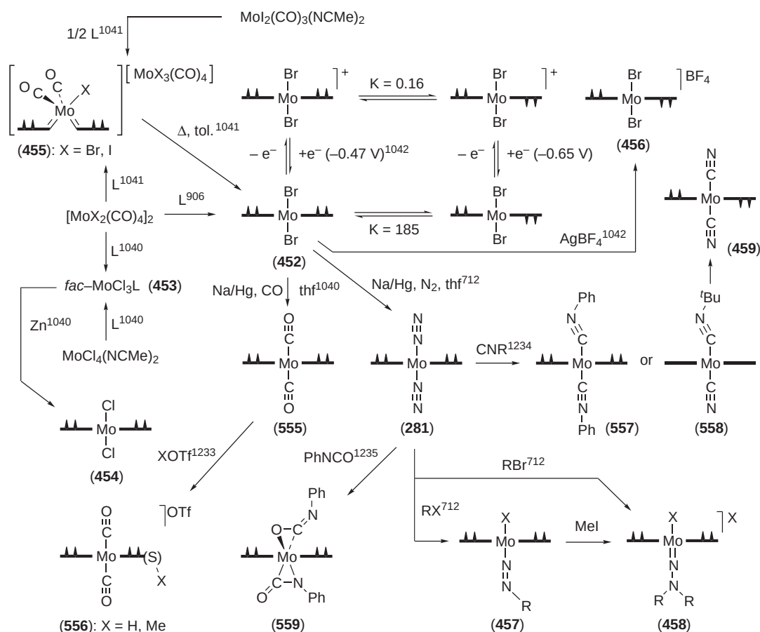
Scheme 19 (L = \text{Me}_8[16]\text{aneS}_4 279)
