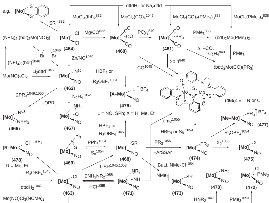
Scheme 20 [\text{Mo}] = \text{Mo}(\text{dttt}) fragment; [\text{X-Mo}] = \text{S-alkylated} or \text{S-protonated Mo}(\text{dttt}) fragment
