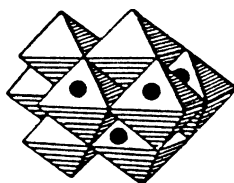
Figure 5 [\text{Mo}_4\text{V}_5\text{O}_{27}]^{5-} .
