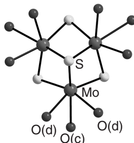
Figure 25 Structure of the [\text{Mo}_3\text{S}_4(\text{H}_2\text{O})_9]^{4+} cation showing c- and d-positions of coordinated \text{H}_2\text{O} ligands.
