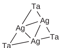
\text{Ag}_3\text{Ta}_3 core of \text{Ag}_3\text{Ta}_3(\text{CO})_{12}(\text{dmpe})_3
