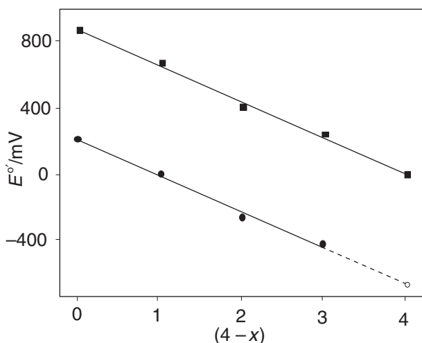
Figure 44 Reduction potentials E^\circ vs. nhe for [\text{Mo}_x\text{W}_{4-x}\text{S}_4(\text{H}_2\text{O})_{12}]^{6+/5+} (■) and [\text{Mo}_x\text{W}_{4-x}\text{S}_4(\text{H}_2\text{O})_{12}]^{5+/4+} (●) couples, x = 0-4 . 119,270
