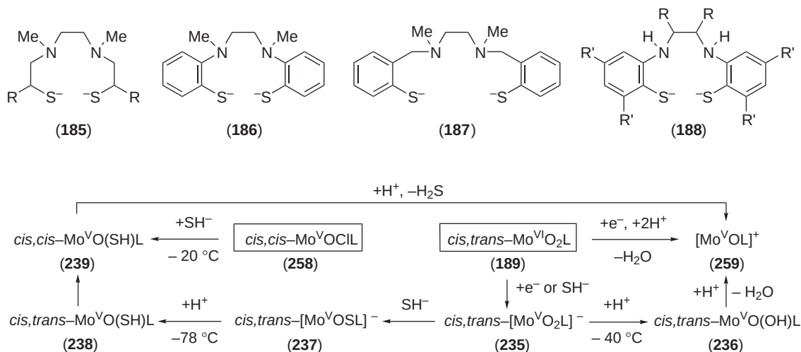
Scheme 9 ( L = L - N_2S_2 = 186 )
