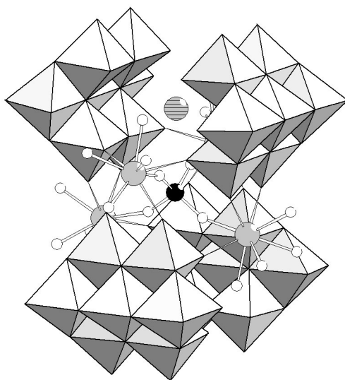
Figure 27 [\text{Ln}_4(\text{H}_2\text{O})_{16}(\text{MoO}_4)(\text{Mo}_7\text{O}_{24})_4]^{14-} .
