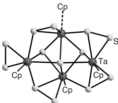
Figure 17 Structure of the [(\eta^5\text{-C}_5\text{H}_5)_4\text{Ta}_4(\mu_4\text{-S})(\mu_3\text{-S})_2(\mu_2\text{-S}_2)_4(\text{S}_2)] molecule.
