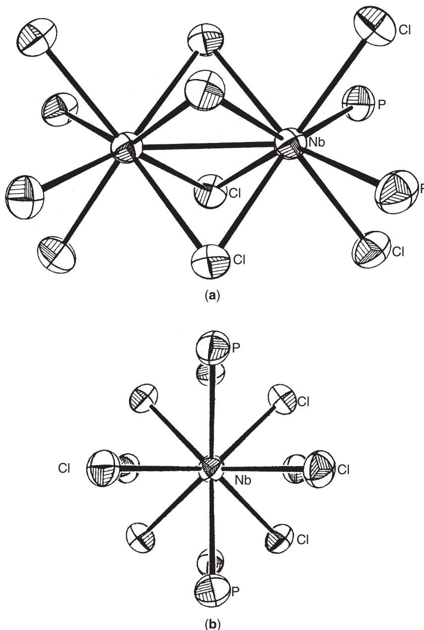
Figure 16 ORTEP drawing of the core structure of the [NbCl 2 (P(CH 3 ) 2 (C 6 H 5 )) 2 ](μ-Cl) 4 molecule both perpendicular to and along the Nb–Nb axis (reproduced by permission of the American Chemical Society from Inorg. Chem. 1984 , 23, 945–947).
