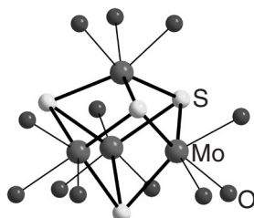
Figure 41 Structure of the [Mo 4 S 4 (H 2 O) 12 ] 5+ cation.
