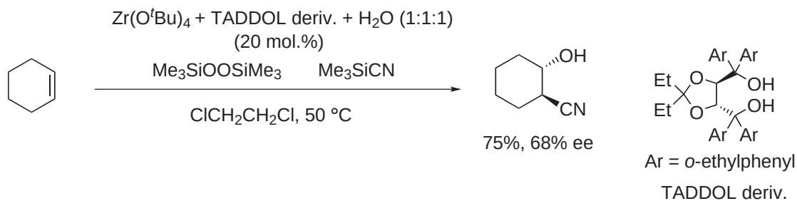
Scheme 39
