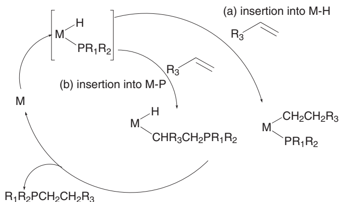
Scheme 45
