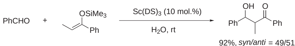
Scheme 16
