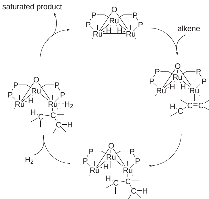
Scheme 73
