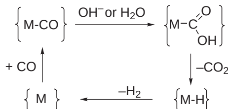
Scheme 64
