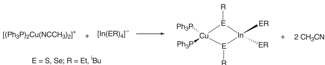
Figure 44 Preparation of [(\text{Ph}_3\text{P})_2\text{Cu}(\mu\text{-ER})_2\text{In}(\text{ER})_2] ( \text{E} = \text{S}, \text{Se}; \text{R} = \text{Et}, \text{Bu}^i ).
