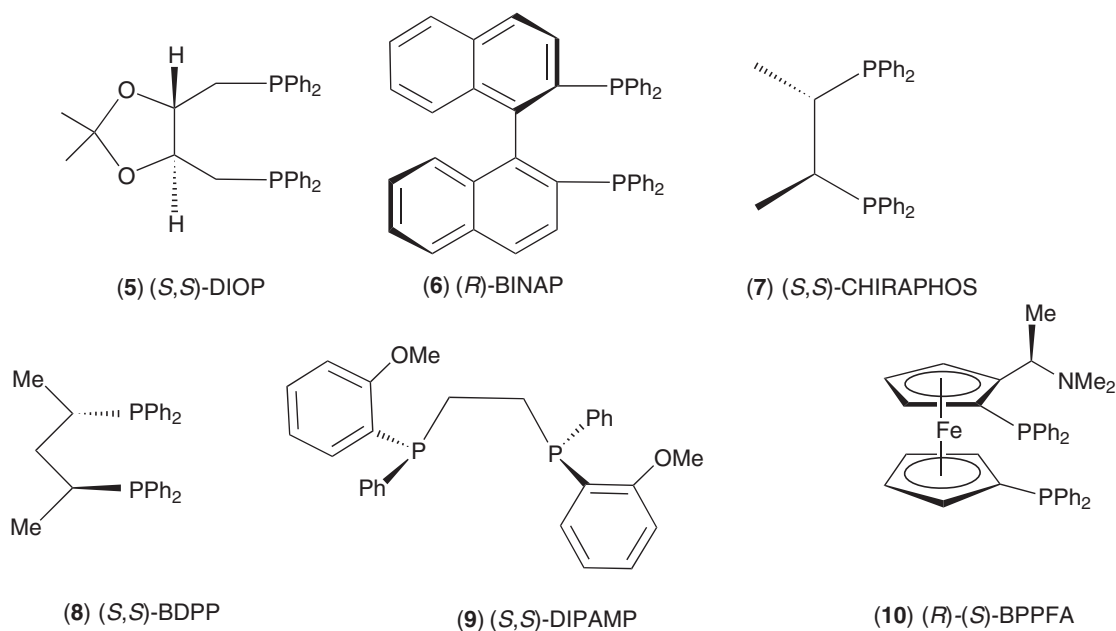
Scheme 8
