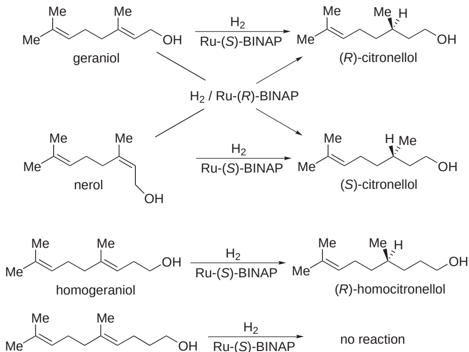
Scheme 11
