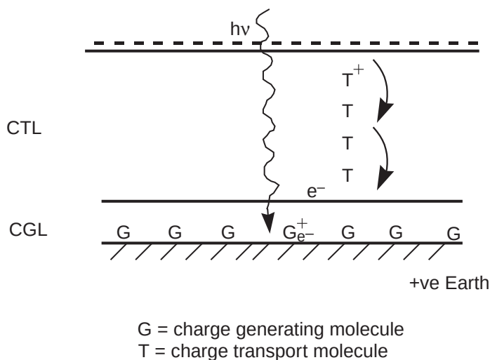
Figure 6 How an OPC works.
