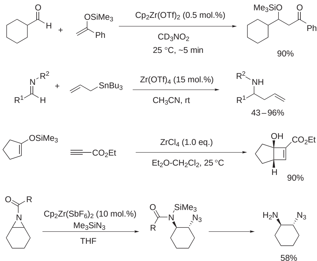
Scheme 37
