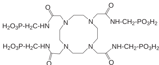
Scheme 12
