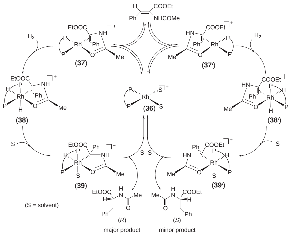
Scheme 10
