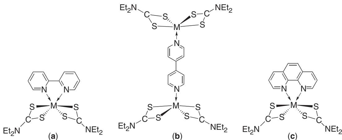
Figure 26 Structures of (a) [M(S_2CNEt_2)_2(2,2'\text{-bipy})] ( M = \text{Cd}, \text{Zn} ); (b) [\{M(S_2CNEt_2)_2\}_2(\mu\text{-}4,4'\text{-bipy})] ; (c) [M(S_2CNEt_2)_2(\text{phen})] ( M = \text{Cd}, \text{Zn} ).
