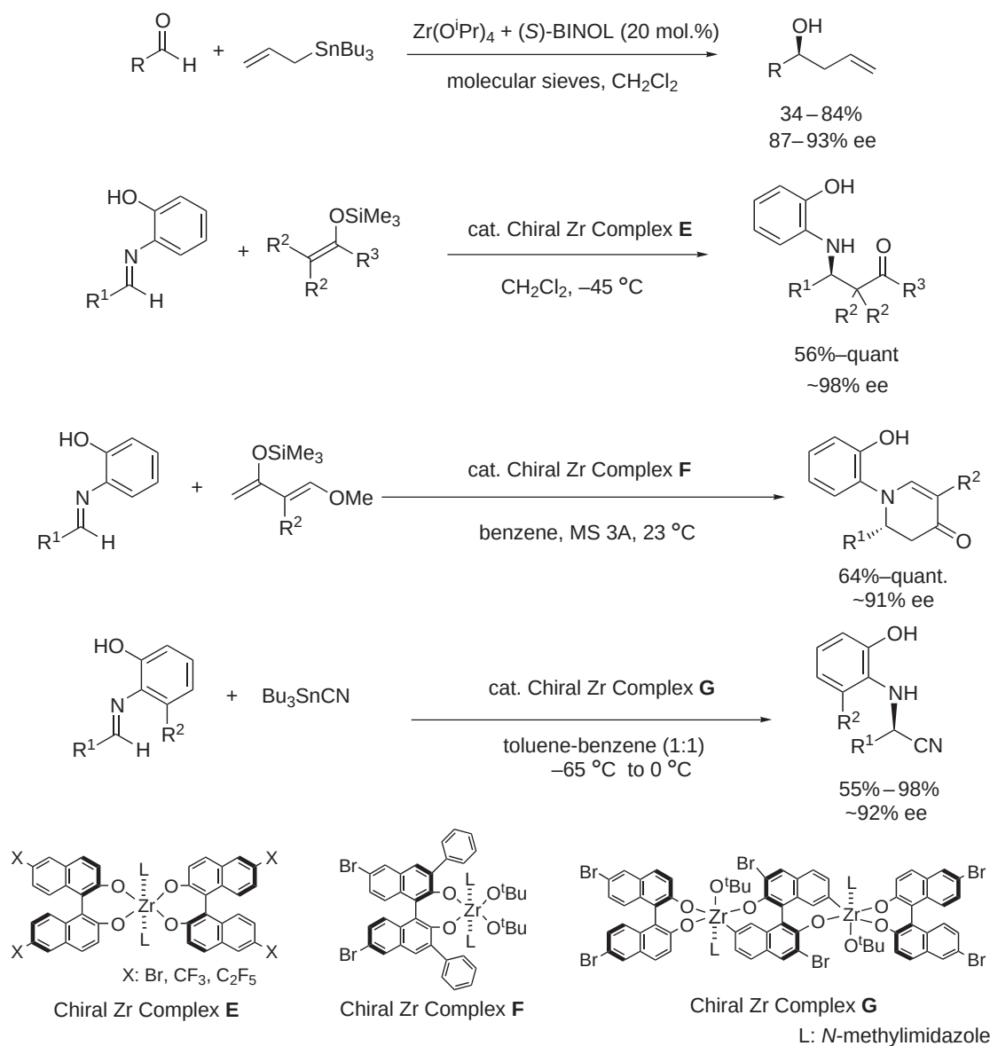
Scheme 38
