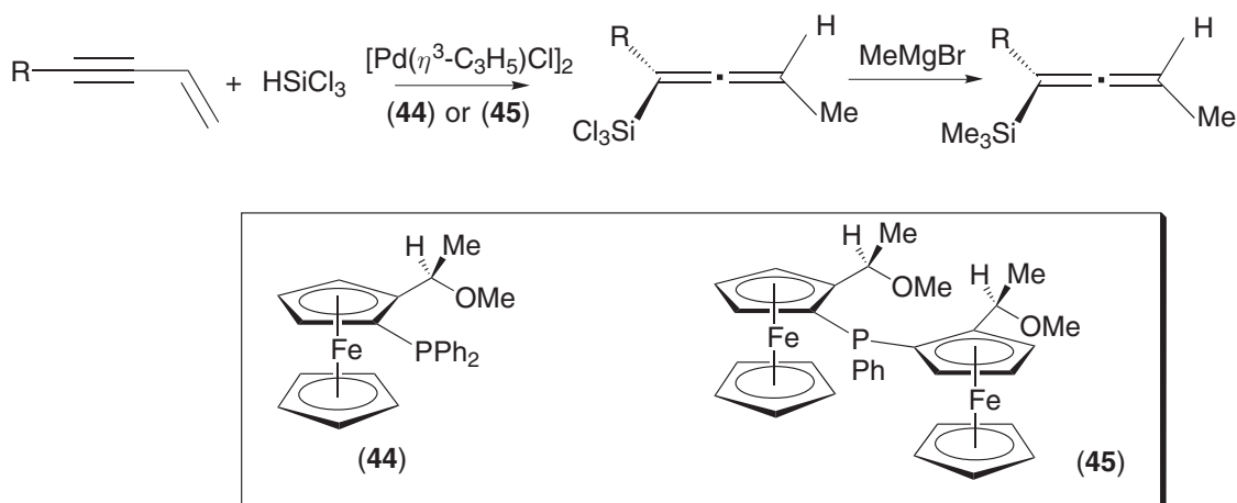
Scheme 27
