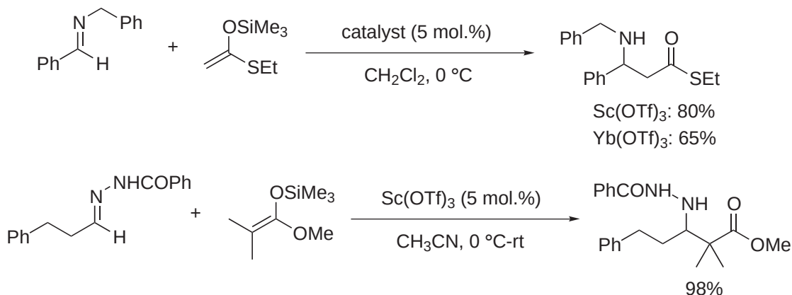
Scheme 11
