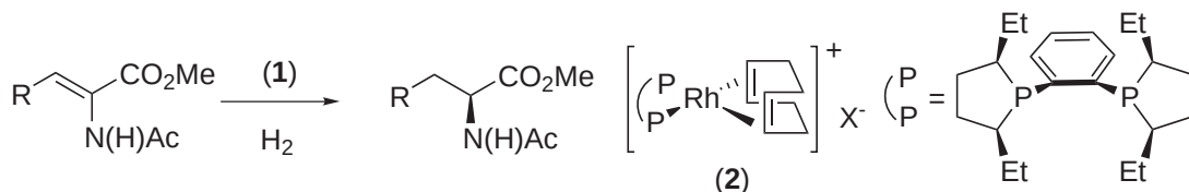
Scheme 67
