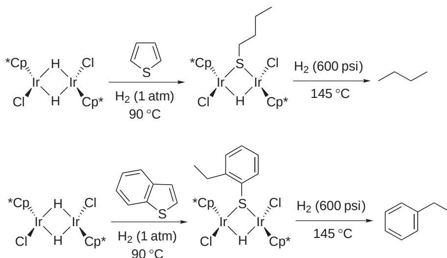
Scheme 38
