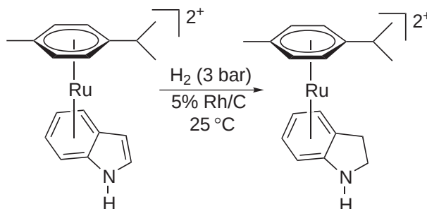
Scheme 48
