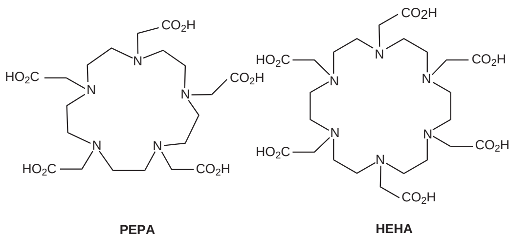
Figure 13 Macrocyclic polyaminocarboxylate ligands for Ac III .
