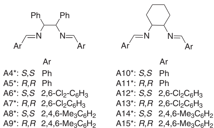
Scheme 13
