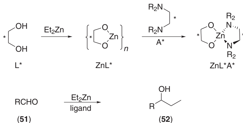
Scheme 11
