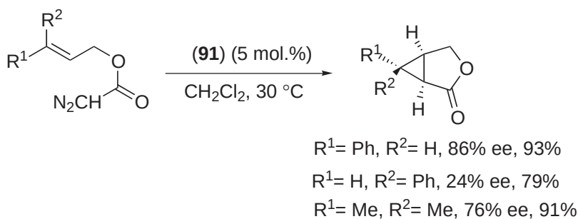
Scheme 80
