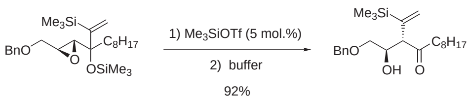
Scheme 77
