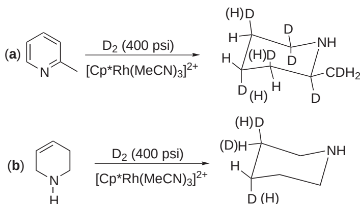
Scheme 51
