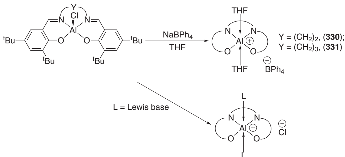
Scheme 22
