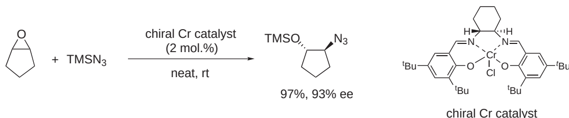
Scheme 58
