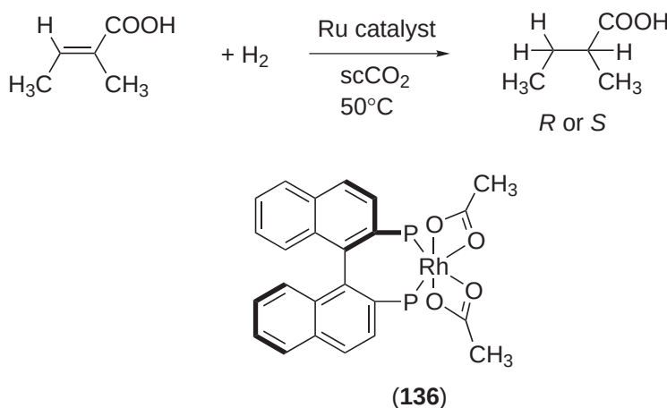
Scheme 68
