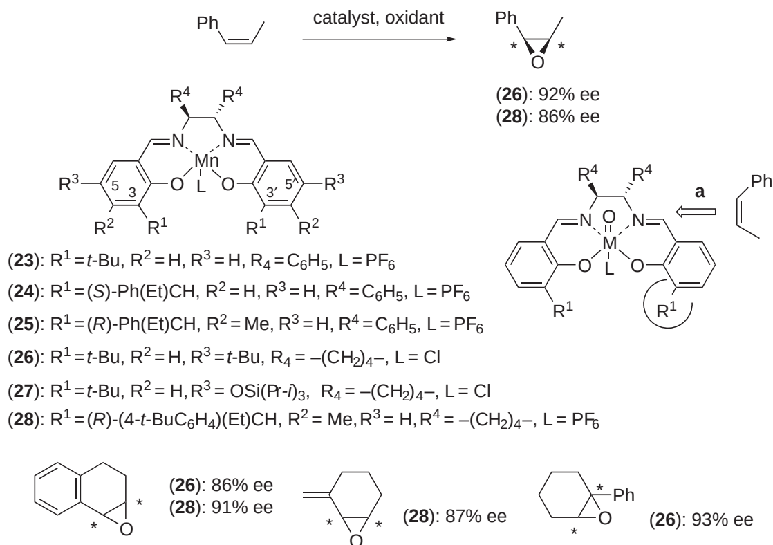
Scheme 14
