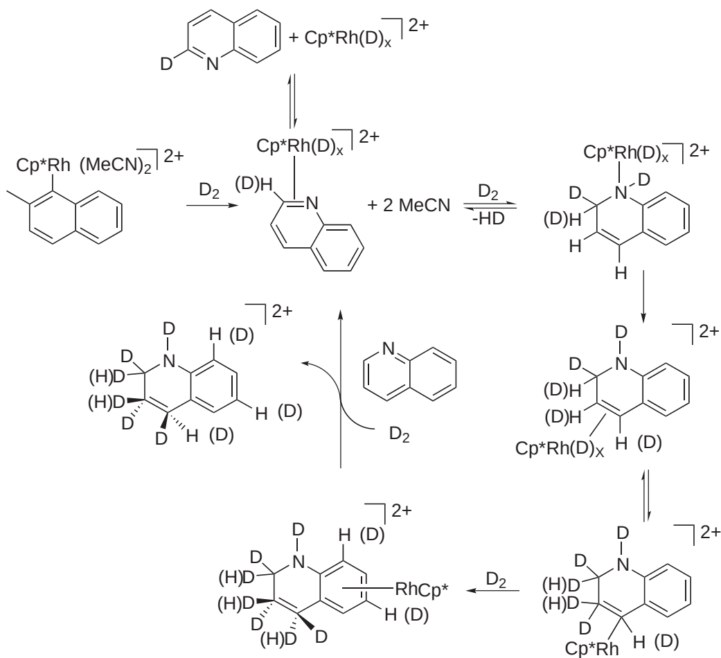
Scheme 52
