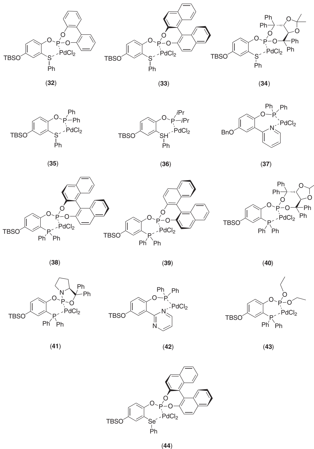
Scheme 9
