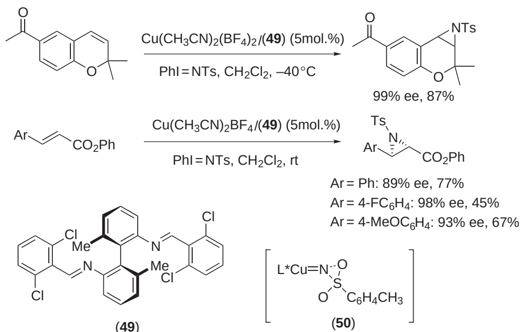
Scheme 36
