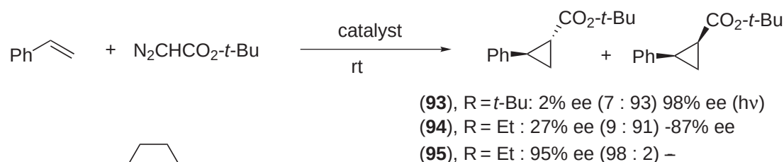
Scheme 67
