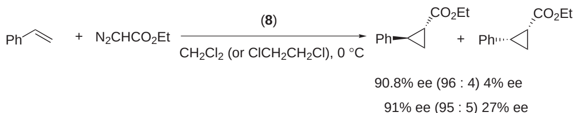
Scheme 67
