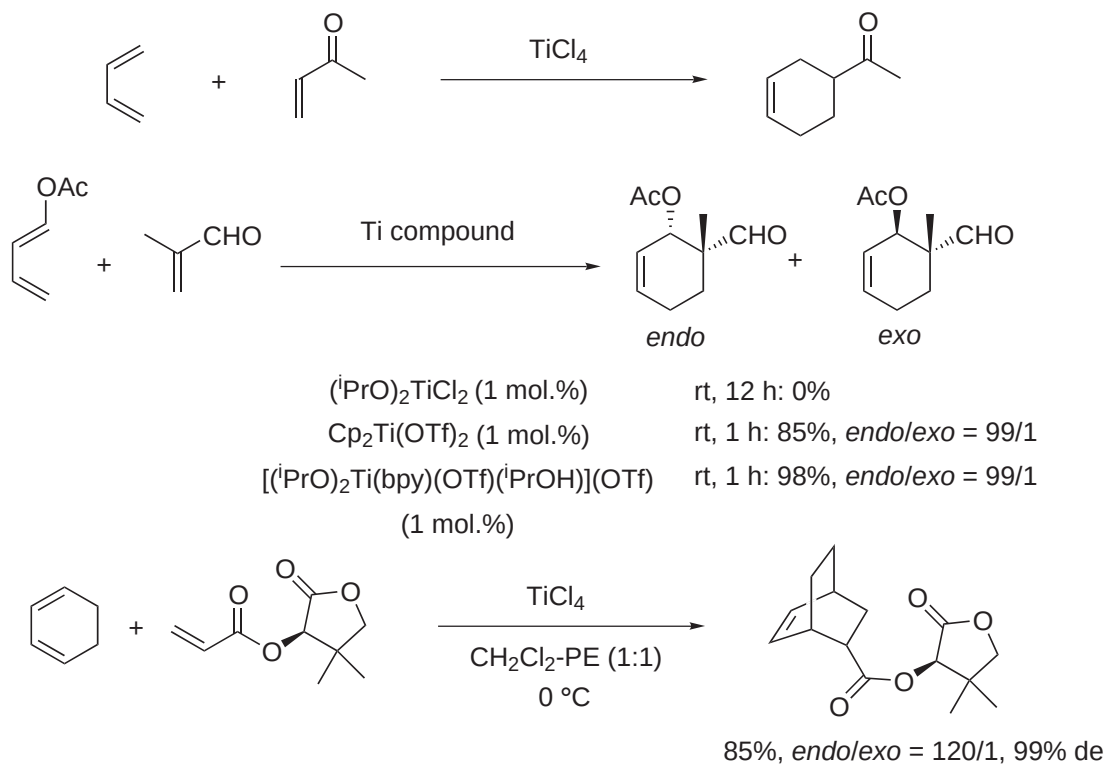
Scheme 25
