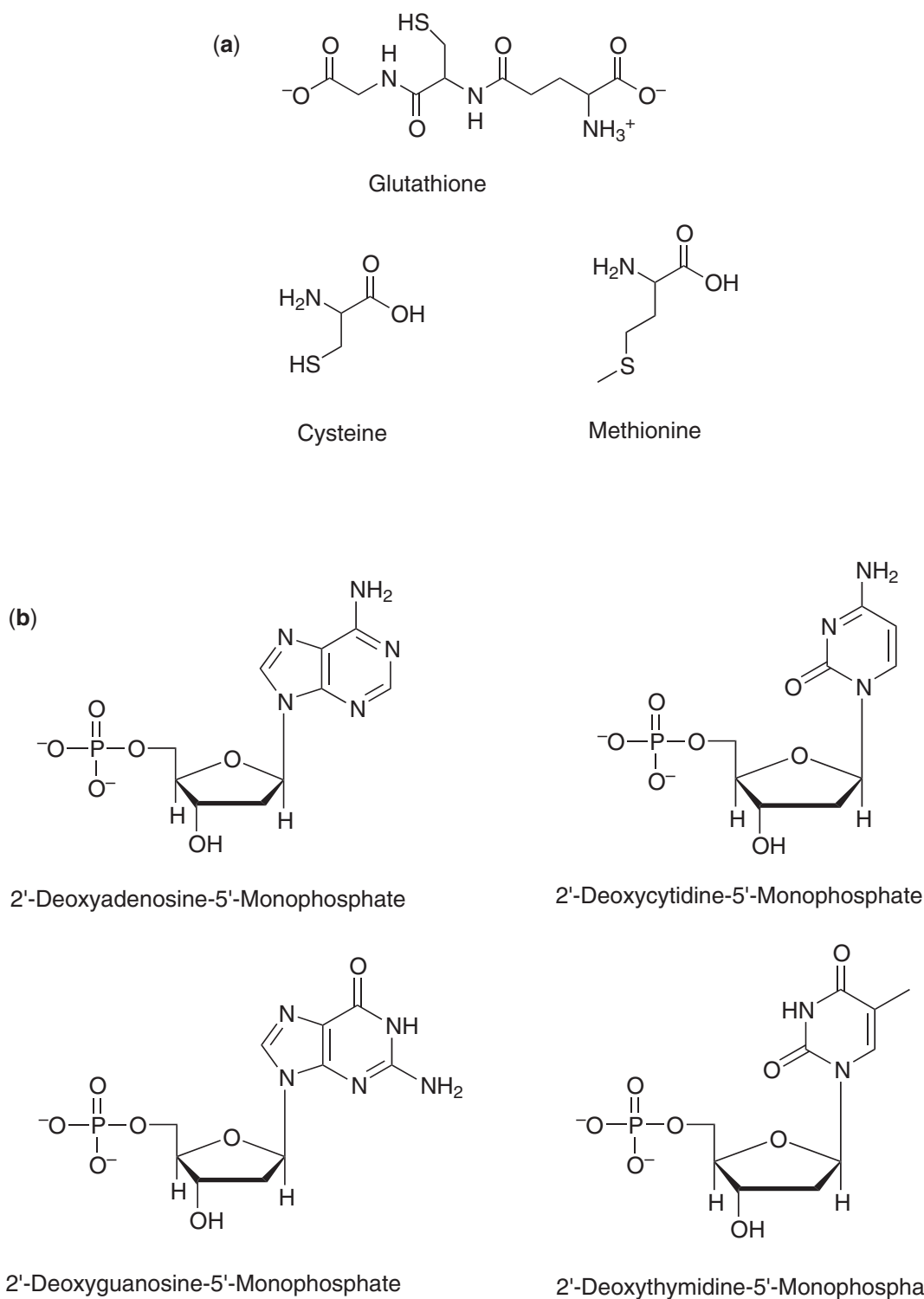
Figure 1 (a) Structures of common sulfur-based amino acids and tripeptides. (b) Structures of nucleic acid monophosphates capable of metal binding.
