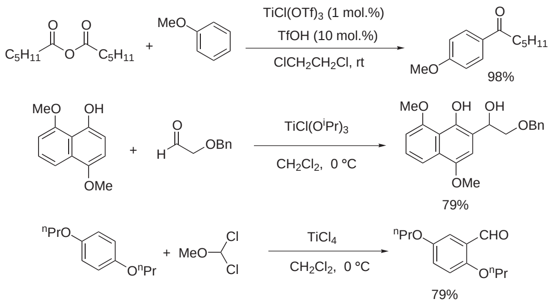
Scheme 28
