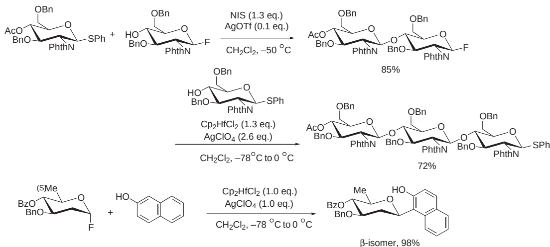
Scheme 41
