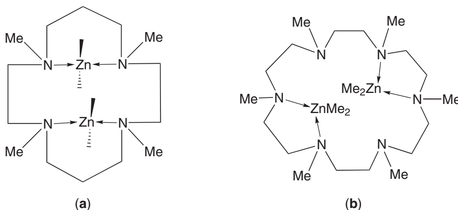
Figure 11 Structures of (a) [(\text{Me}_2\text{Zn})_2(\text{Me}_4\text{-14-ane-N}_4)] ; (b) [(\text{Me}_2\text{Zn})_2(\text{Me}_6\text{-18-ane-N}_6)] .
