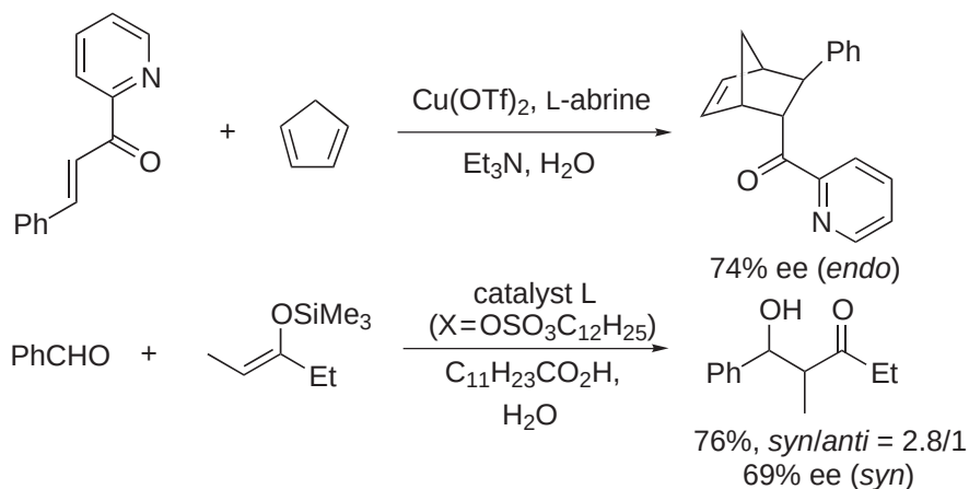
Scheme 49
