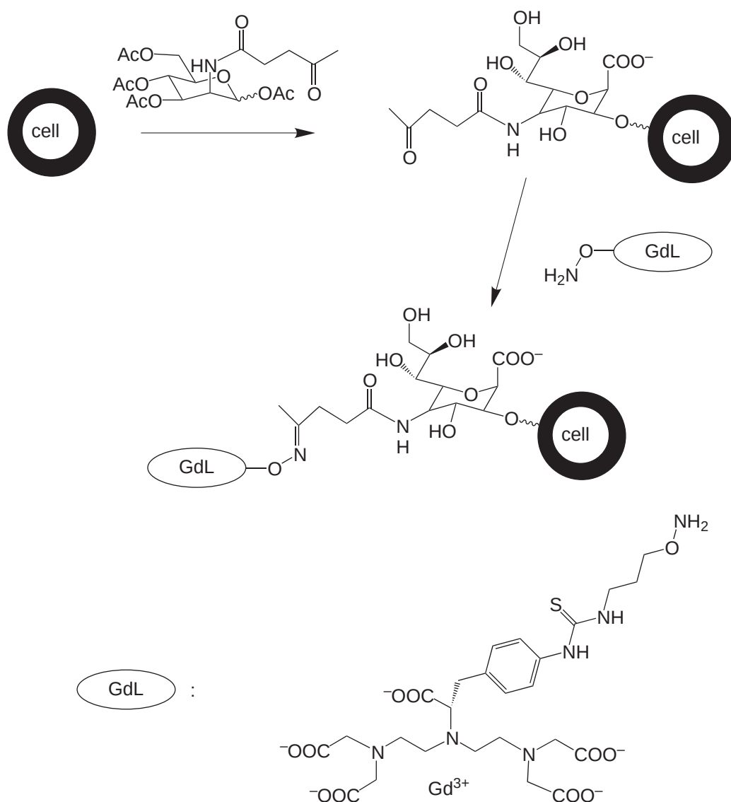
Scheme 20
