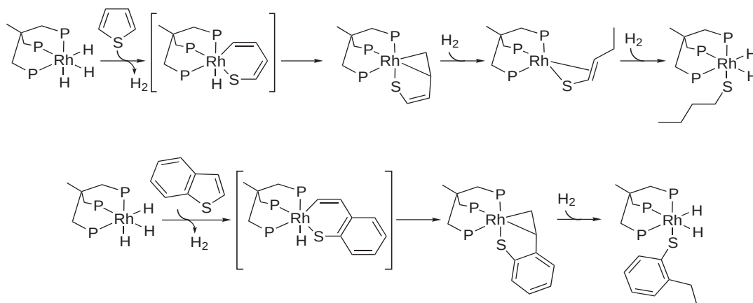
Scheme 39
