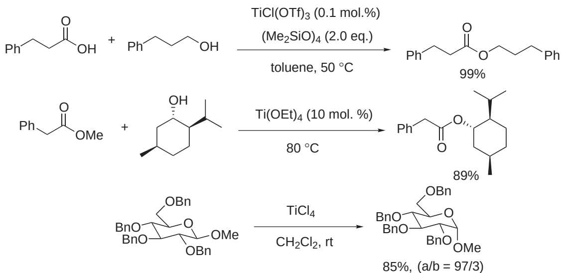
Scheme 30
