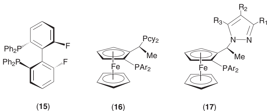
Scheme 11
