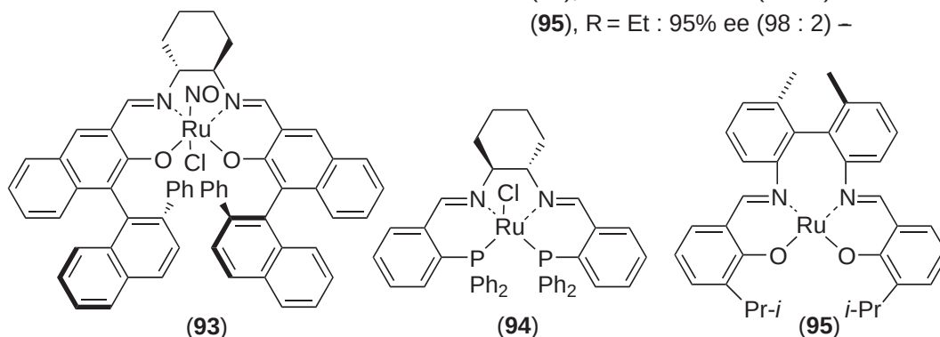
Scheme 68
