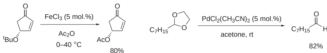
Scheme 57
