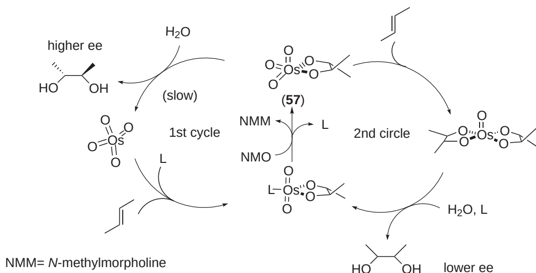
Scheme 45
