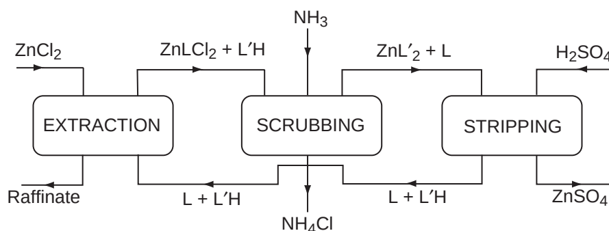
Figure 8 An outline flowsheet to transport zinc from chloride to sulfate media using a mixture of an acidic (pH-swing) extractant L'H and a solvating extractant L. 187
