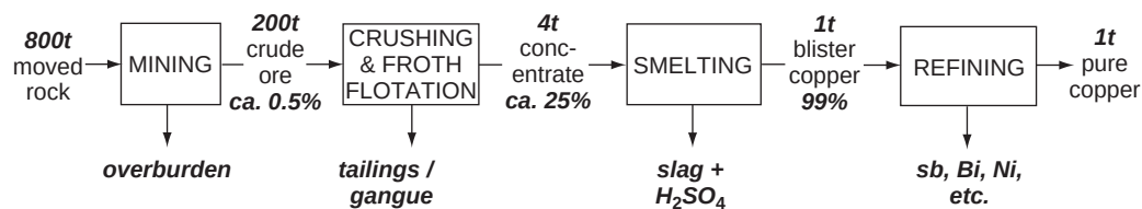
Figure 1 Typical quantities involved in the concentration of copper from sulfide ores.
