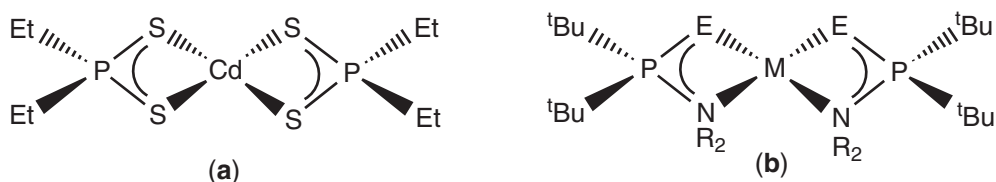
Figure 34 Structures of dithiophosphinate derivatives: (a) \text{M} = \text{Cd} , \text{R} = \text{Et} ; (b) [\text{M}\{(\text{Bu}^t)_2\text{PE}(\text{NR})_2\}_2] ( \text{M} = \text{Zn}, \text{Cd} ; \text{E} = \text{Se}, \text{Te} ; \text{R} = \text{Pr}^i , c - \text{C}_6\text{H}_{11} ).
