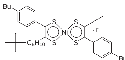
(162) : n_2 = -4.6 \cdot 10^{-9} \text{ cm}^2 \text{ kW}^{-1} , \alpha = 240 \text{ cm}^{-1} , W = 0.5 , n_2/\phi = 4.3 (PMMA film) 436
