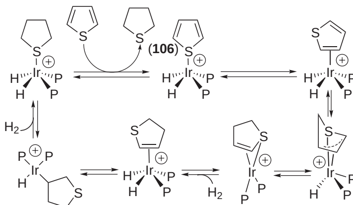
Scheme 34
