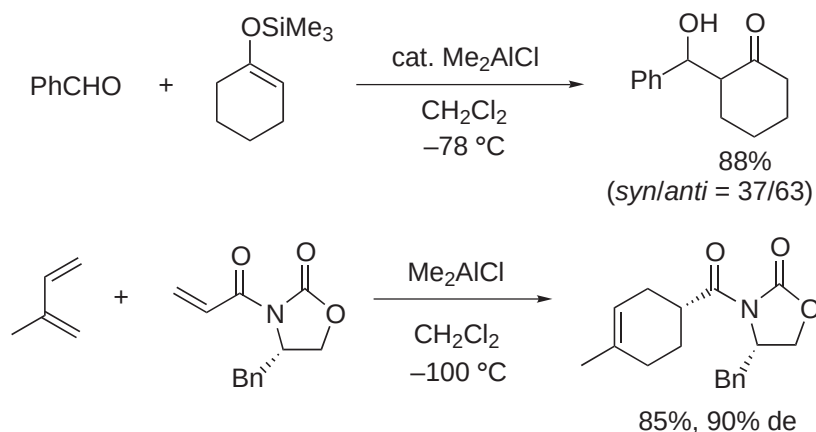
Scheme 71
