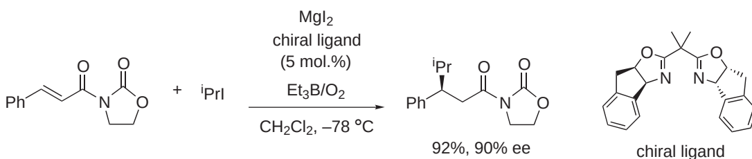
Scheme 8
