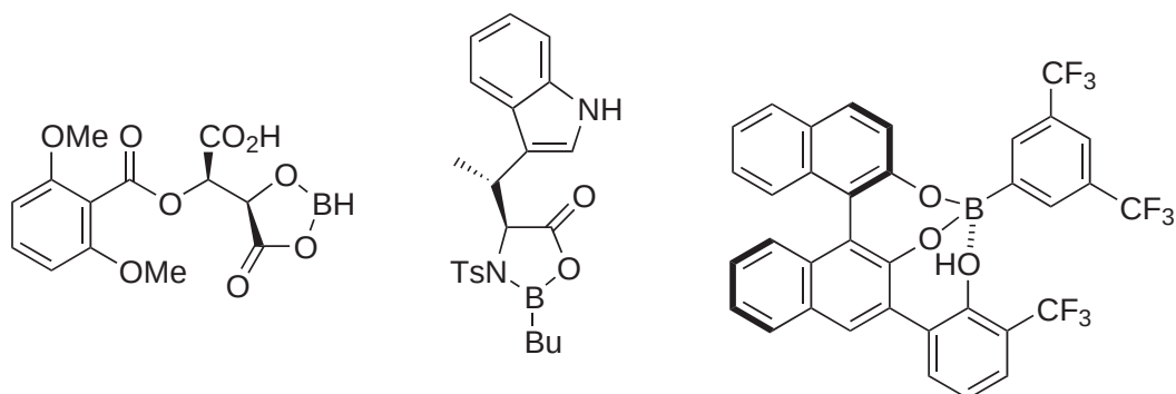
Figure 2 Chiral Lewis-acidic boron compounds.
