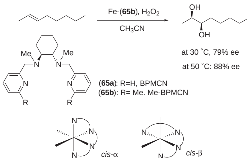
Scheme 53
