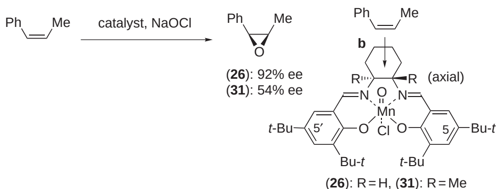
Scheme 16
