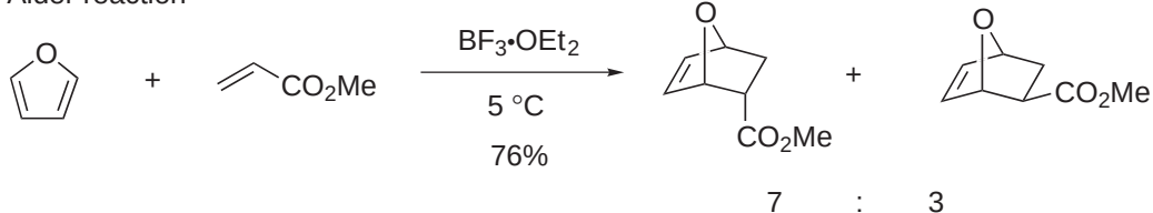
Scheme 63
