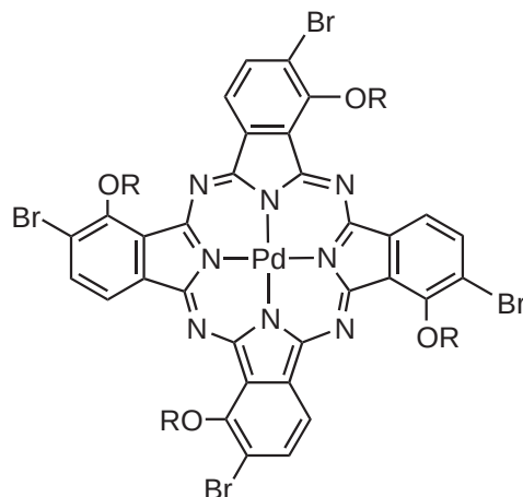
Scheme 7
