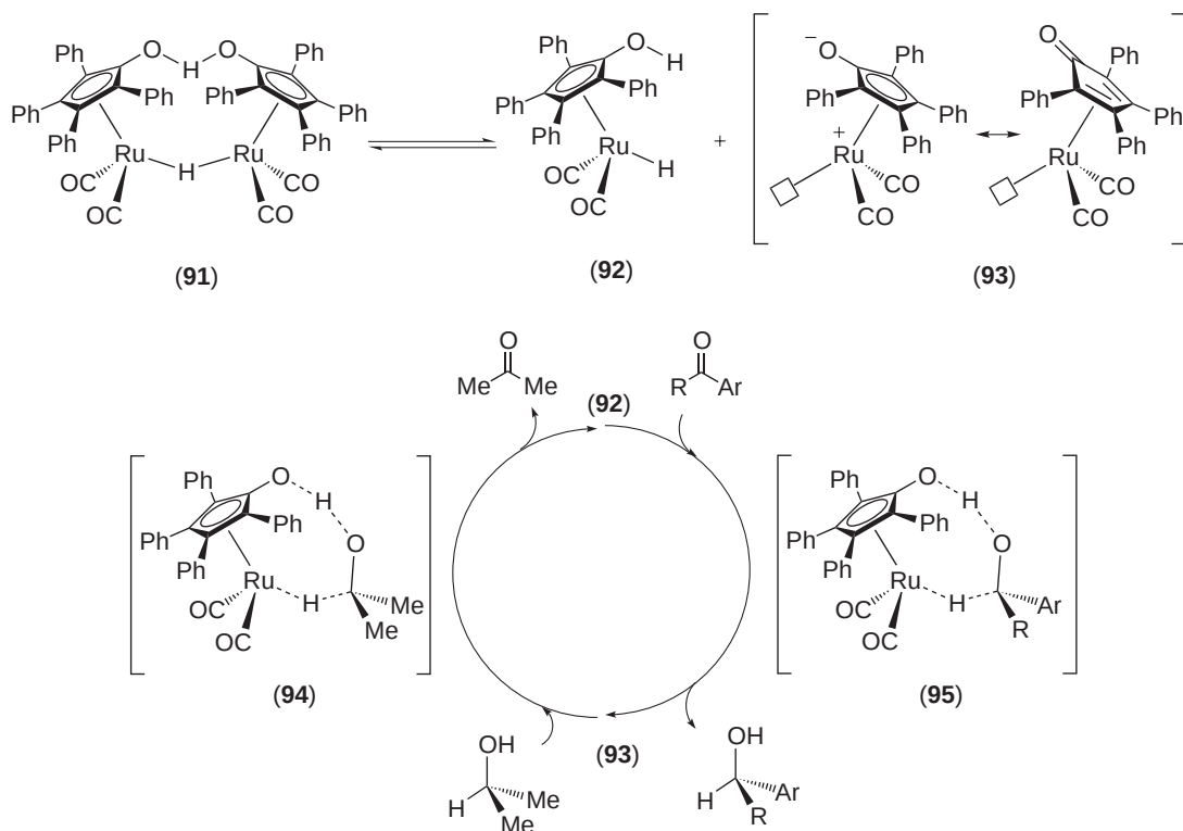
Scheme 30
