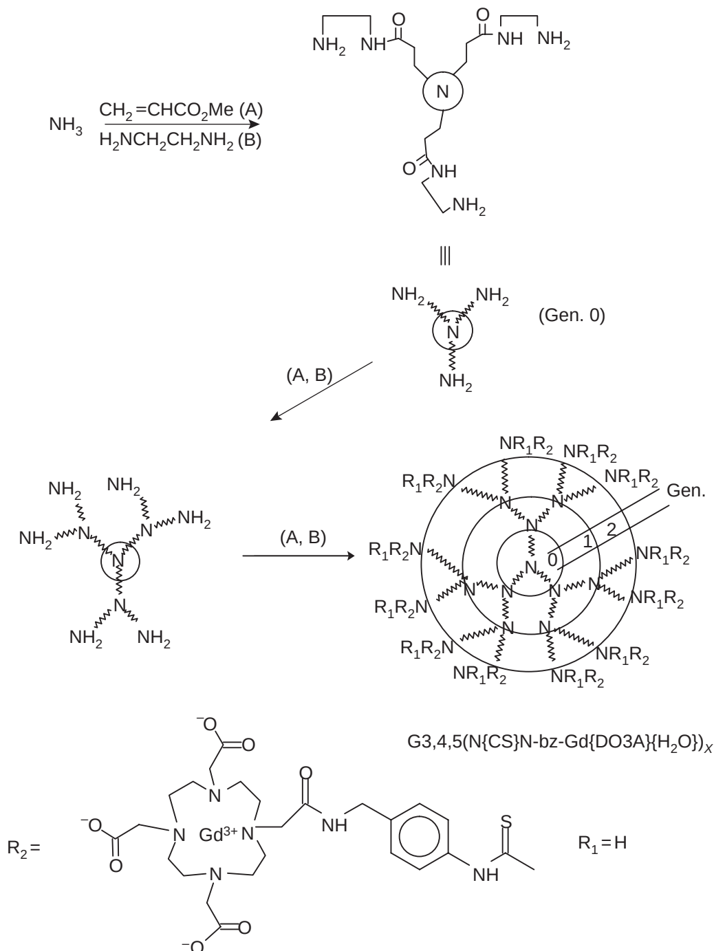
Scheme 5
