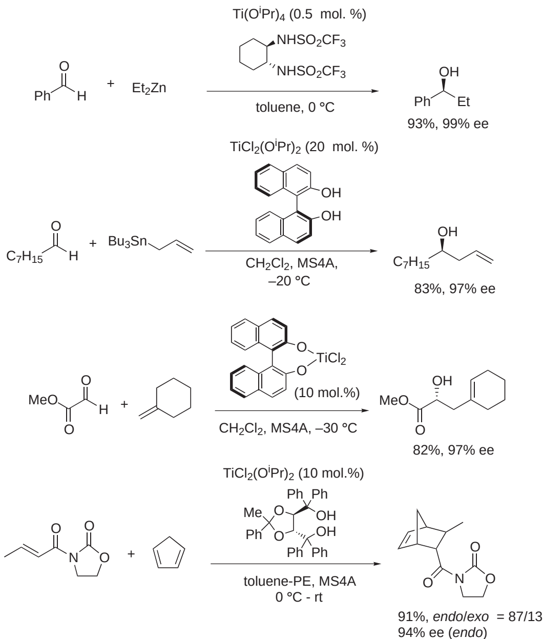
Scheme 35
