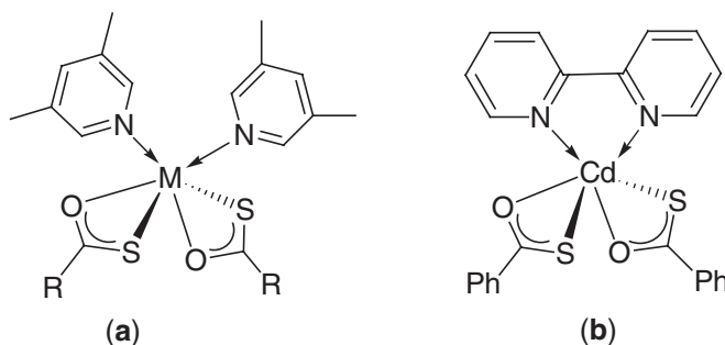
Figure 48 Structures of (a) [\text{M}(\text{SOCR})_2(\text{dmpy})_2] ( \text{M} = \text{Cd}, \text{Zn} ; \text{R} = \text{Me}, \text{Bu}^t ); (b) [\text{Cd}(\text{SOCPh})_2(2,2'\text{-bipy})] .
