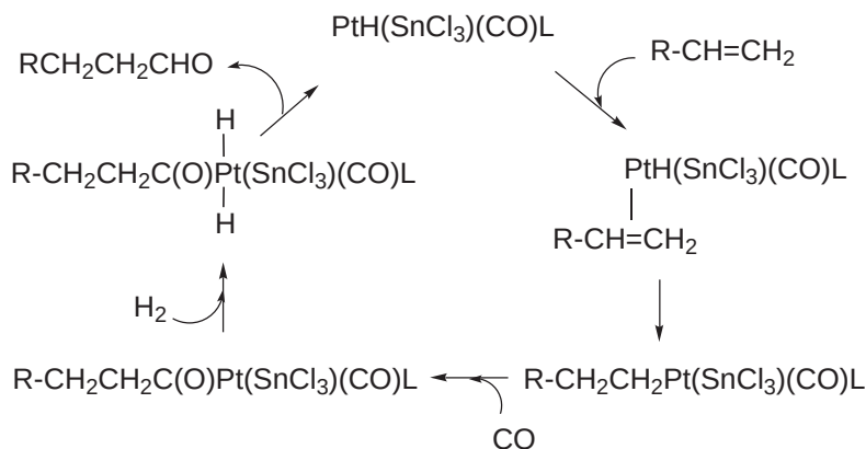
Scheme 2
