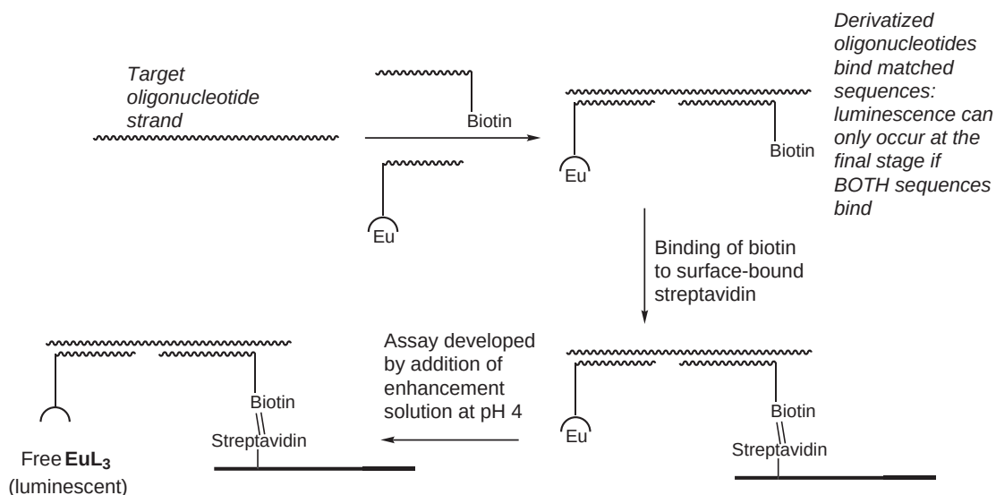
Figure 12 Split-probe oligonucleotide sequencing using DELFI.
