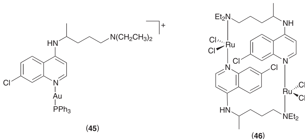
Figure 21 Gold and ruthenium complexes of antiparasitic agents.
