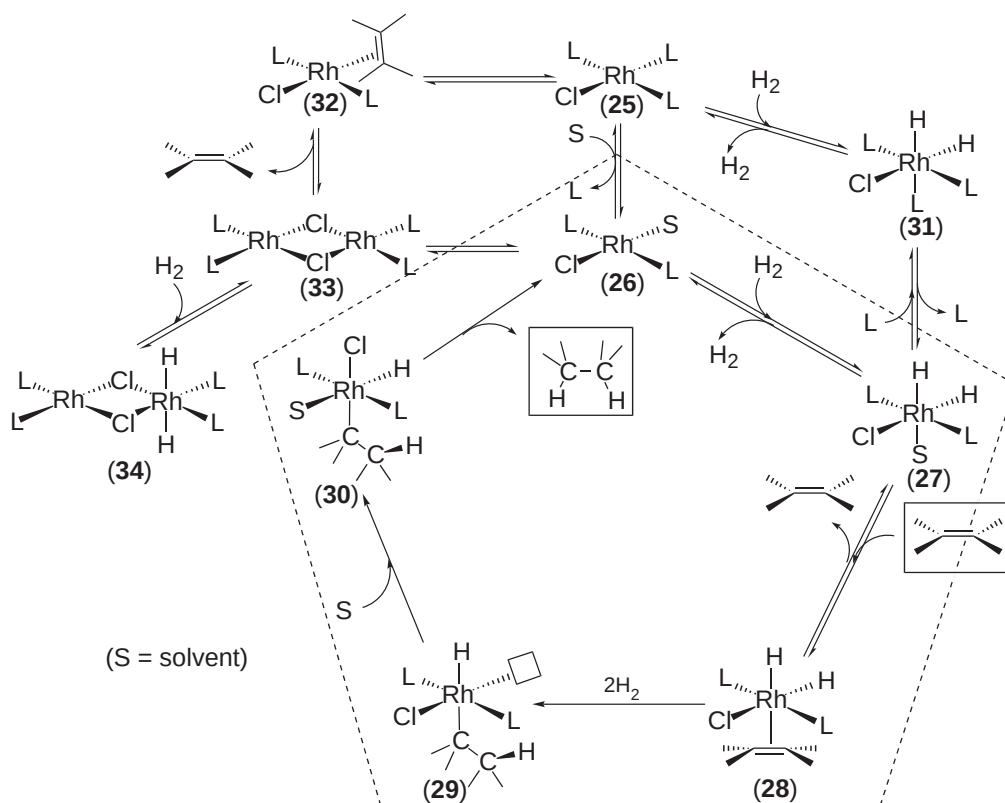
Scheme 8
