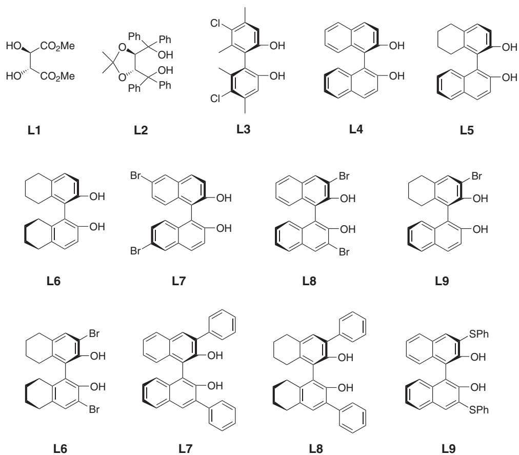
Scheme 25
