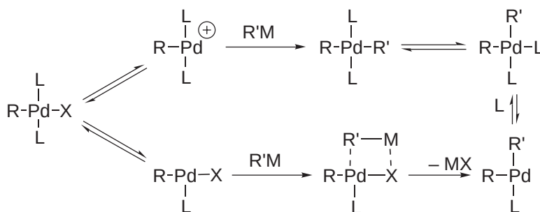
Scheme 3
