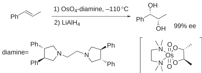
Scheme 43
