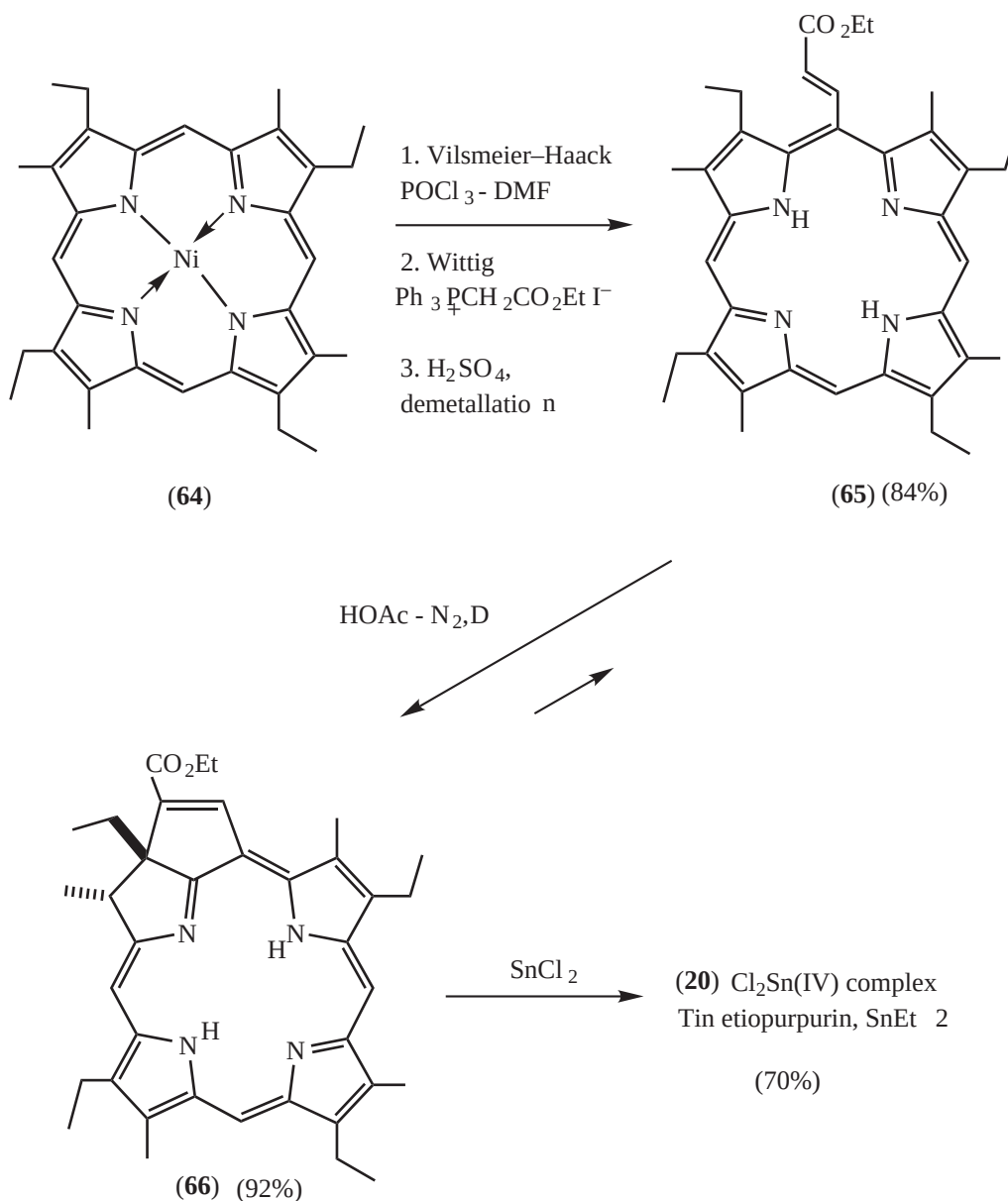
Figure 15 Synthesis of dichlorotin(IV) etiopurpurin ( \text{SnEt}_2 ) (20) from nickel(II) etioporphyrin I (64). 159,406,407
