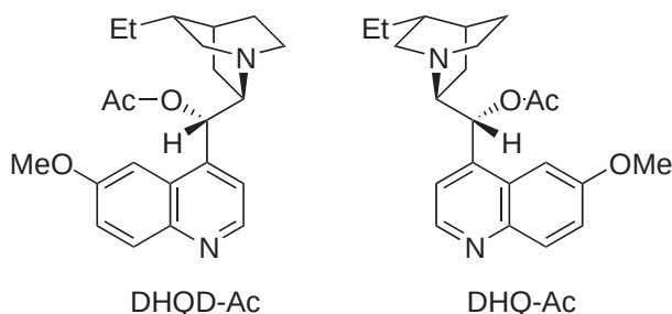
Scheme 42
