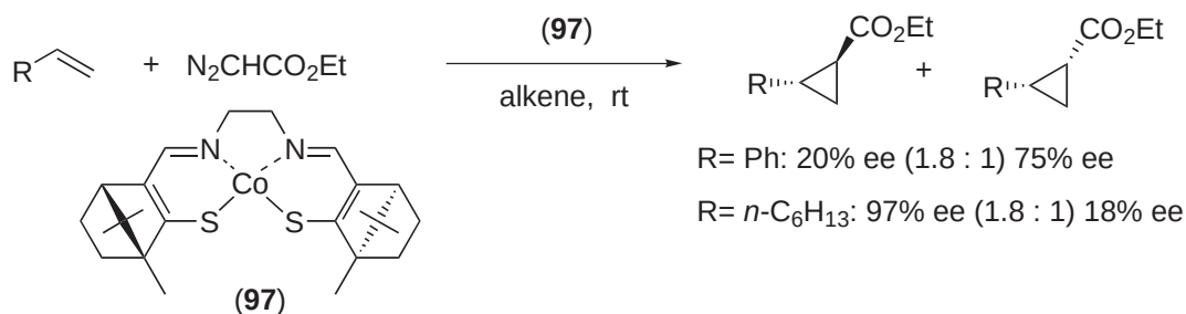
Scheme 70
