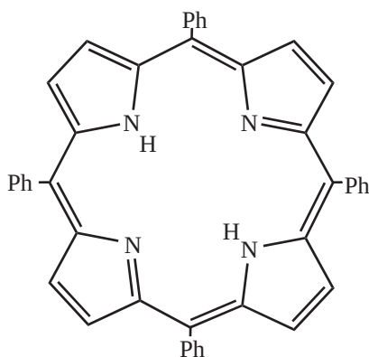
(2) 5,10,15,20-Tetraphenylporphyrin (TPP)
