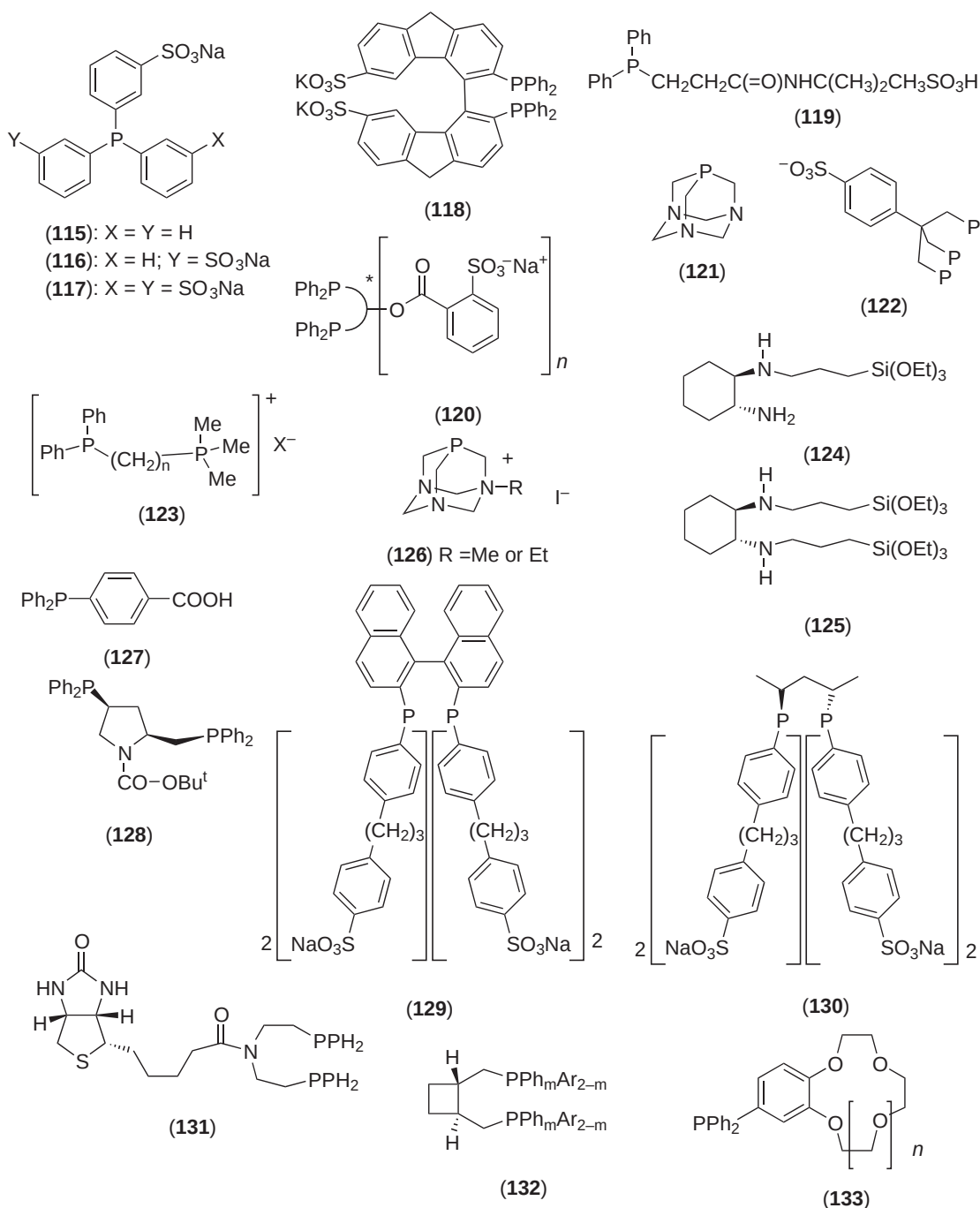
Scheme 55
