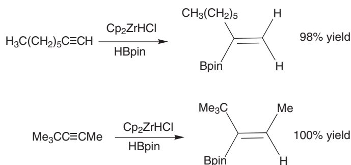
Scheme 7
