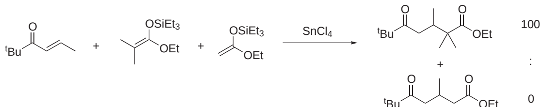
Scheme 82
