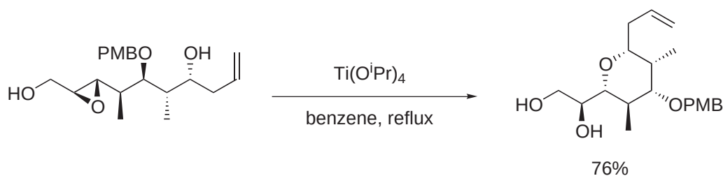
Scheme 33
