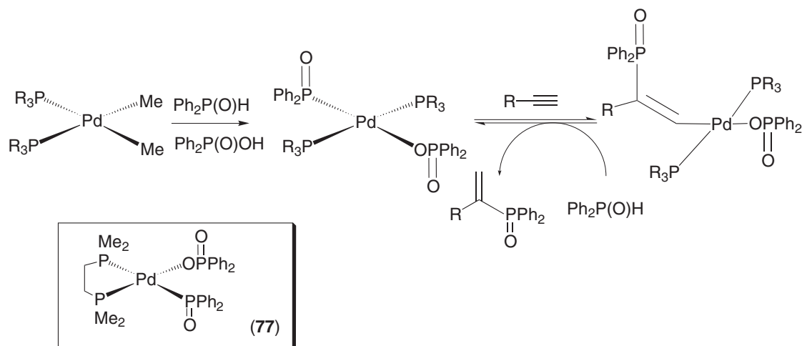
Scheme 47
