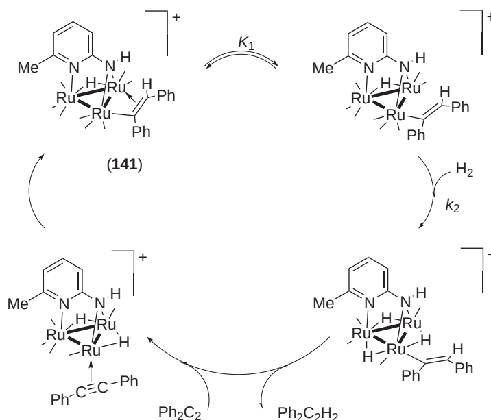
Scheme 75
