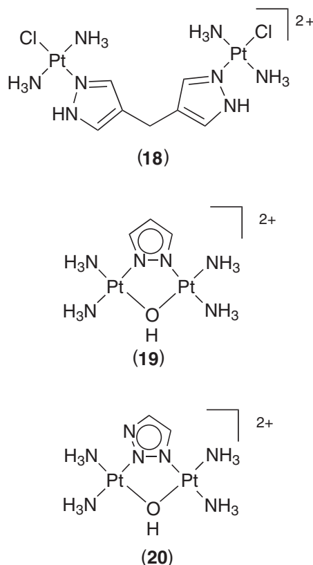
Figure 11 Dinuclear platinum compounds based on heterocycle bridges.
