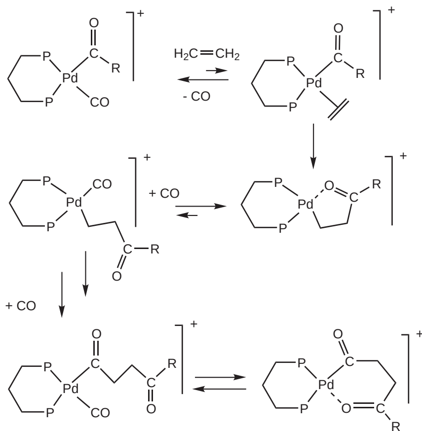
Scheme 5
