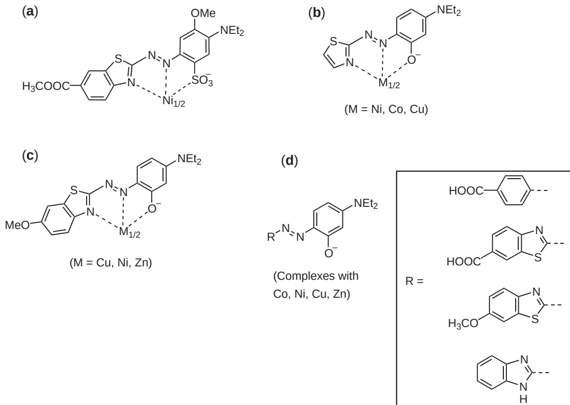
Scheme 11
