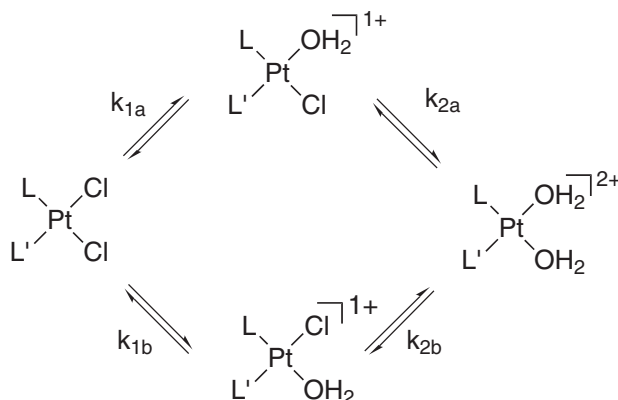
Figure 4 Hydrolysis scheme for cisplatin-based anticancer agents. Where \text{L} = \text{L}' = \text{NH}_3 cisplatin is indicated. When \text{L} = \text{NH}_3 and \text{L}' = 2\text{-picoline} or \text{cha} the rates of aquation of the trans -chloride ligands are different.
