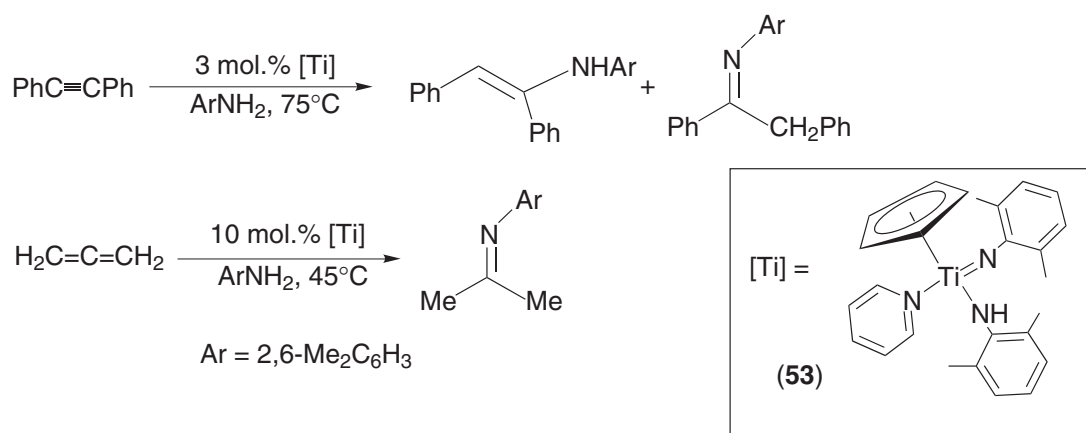
Scheme 35
