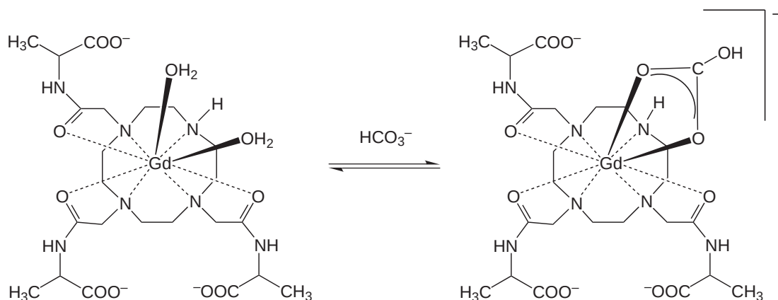
Scheme 13
