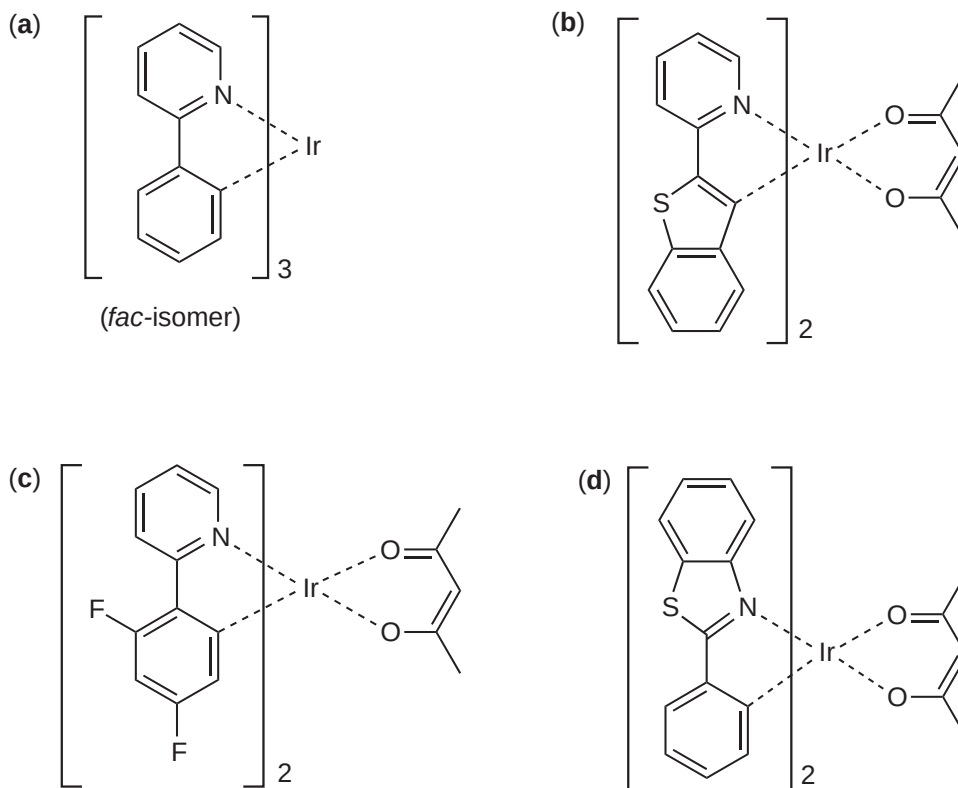
Figure 3 Structures of some \text{Ir}^{\text{III}} complex phosphors based on cyclometallating N,C -donor ligands (see Section 9.15.5.1.4).
