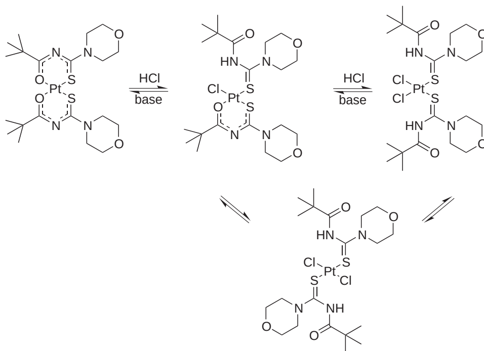
Figure 11 Interconversion of \text{Pt}^{\text{II}} complexes of N - t -pentanoyl- N' -morpholinothiourea. 386
