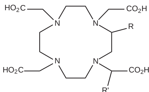
Figure 4 NOTA analogues.
