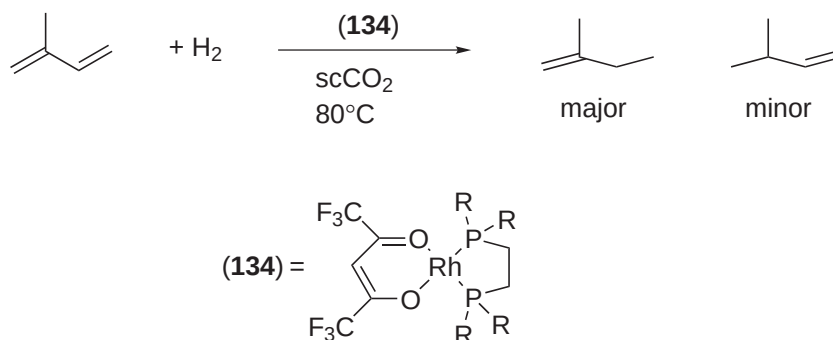
Scheme 66
