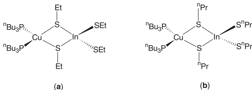
Figure 43 Structures of (a) [(Bu n 3 P) 2 Cu(μ-SEt) 2 In(SET) 2 ]; (b) [(Bu n 3 P) 2 Cu(μ-S(Pr n )) 2 In(SPr n ) 2 ].
