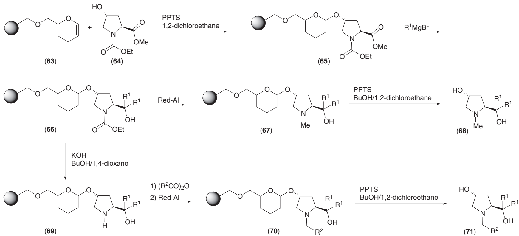
Scheme 17
