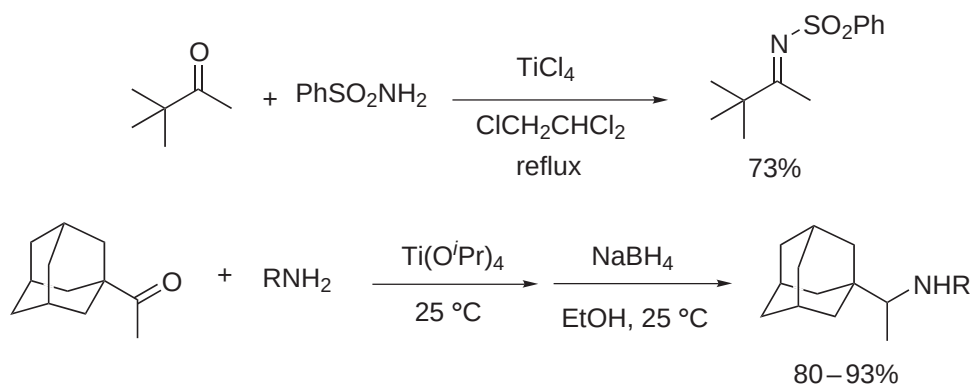
Scheme 31
