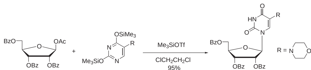
Scheme 78
