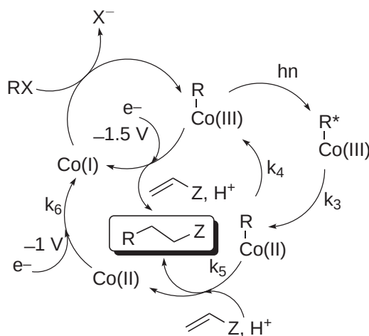
Scheme 9
