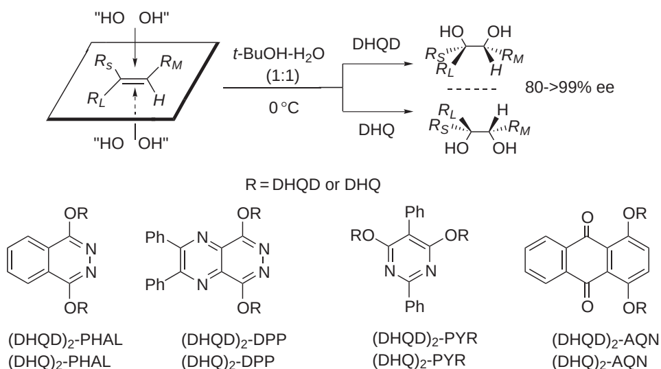
Scheme 47
