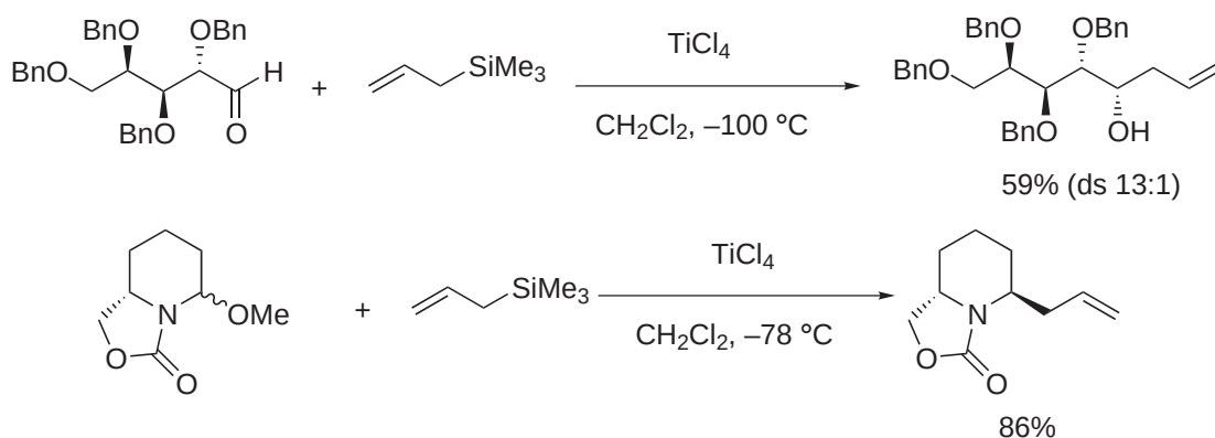
Scheme 22
