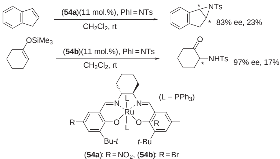
Scheme 39
