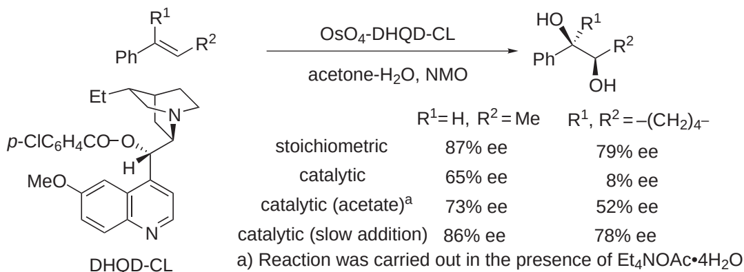
Scheme 44
