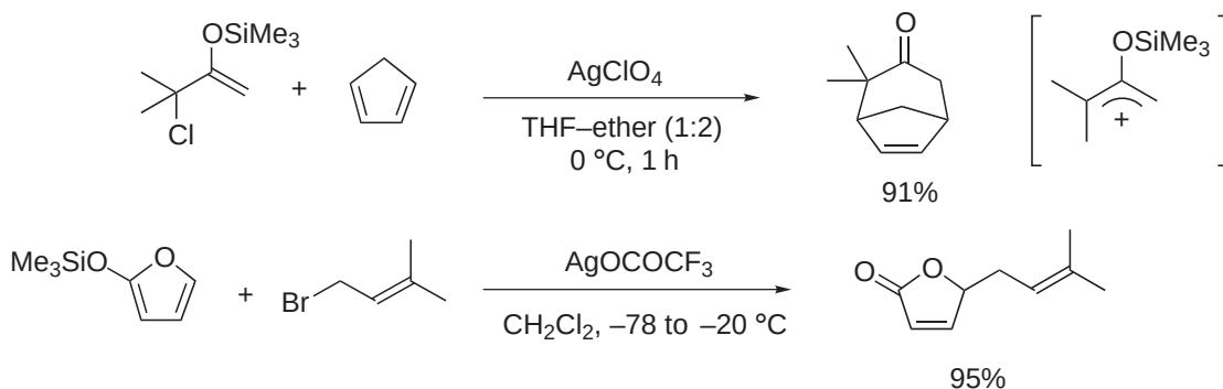
Scheme 50
