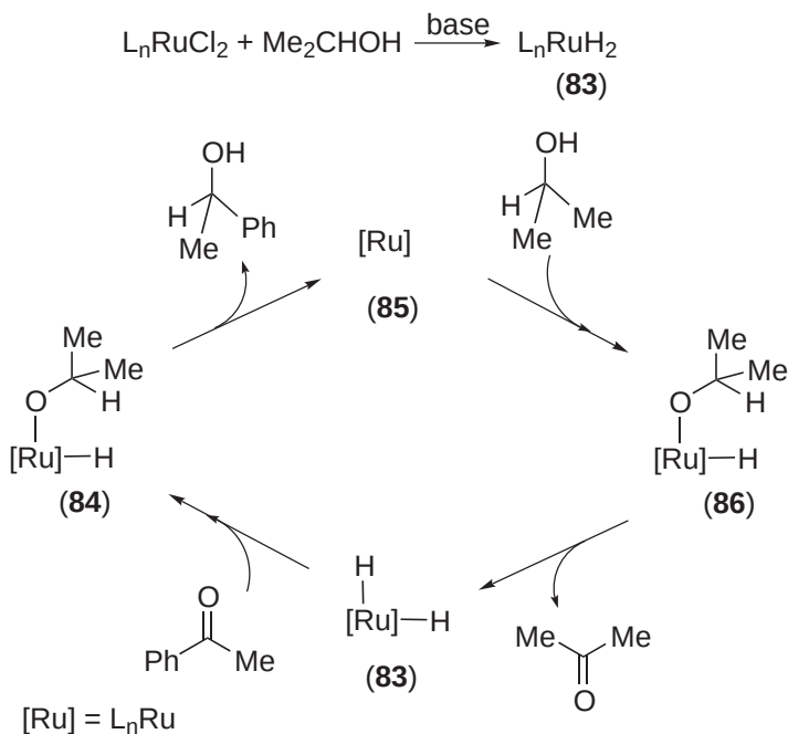
Scheme 26
