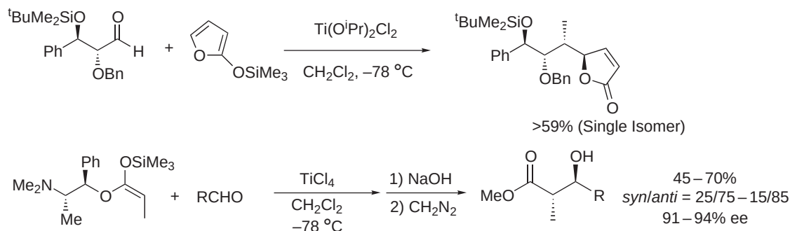
Scheme 20
