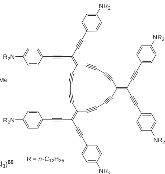
(4): \gamma[\text{THG}_{2100}] = 4.3 \cdot 10^{-32} \text{ esu} , \chi^{(3)} = 7.6 \cdot 10^{-11} \text{ esu (CHCl}_3)^{26}
