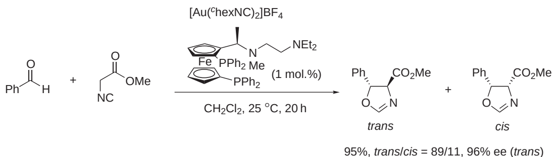
Scheme 52
