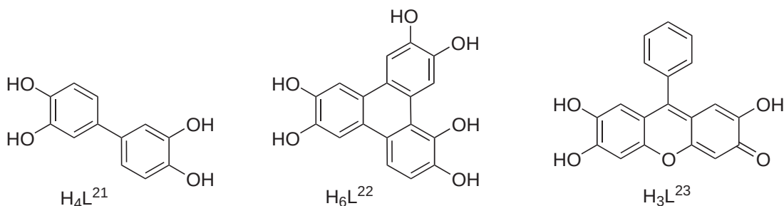
Scheme 5
