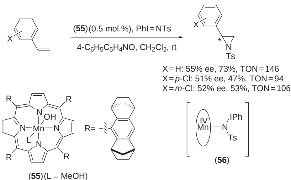
Scheme 40
