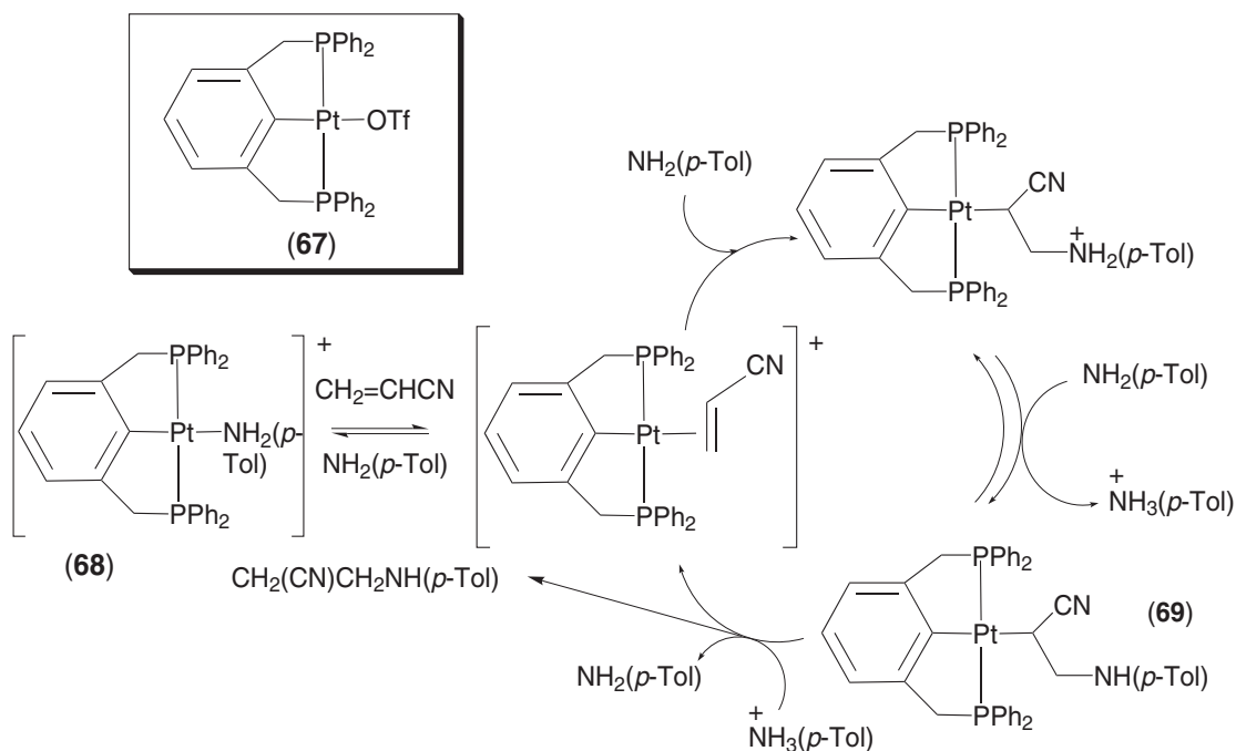
Scheme 42
