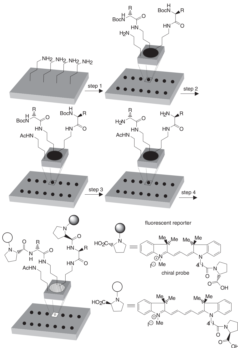
Figure 7 Reaction microarrays in high-throughput ee-determination. Reagents and conditions: step 1, \text{BocHNCH(R)CO}_2\text{H} , \text{PyAOP} , 1\text{Pr}_2\text{NEt} , \text{DMF} ; step 2, \text{Ac}_2\text{O} , pyridine; step 3, 10% \text{CF}_3\text{CO}_2\text{H} and 10% \text{Et}_3\text{SiH} in \text{CH}_2\text{Cl}_2 , then 3% \text{Et}_3\text{N} in \text{CH}_2\text{Cl}_2 ; step 4, pentafluorophenyl diphenylphosphinate, 1\text{Pr}_2\text{NEt} , 1:1 mixture of the two fluorescent proline derivatives, \text{DMF} , -20^\circ\text{C} . 99
