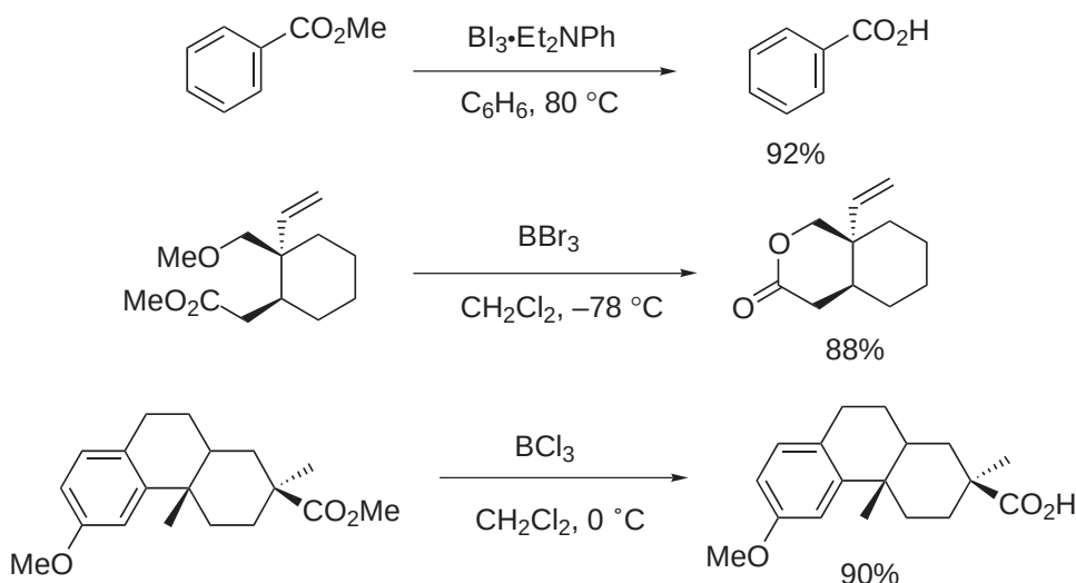
Scheme 61
