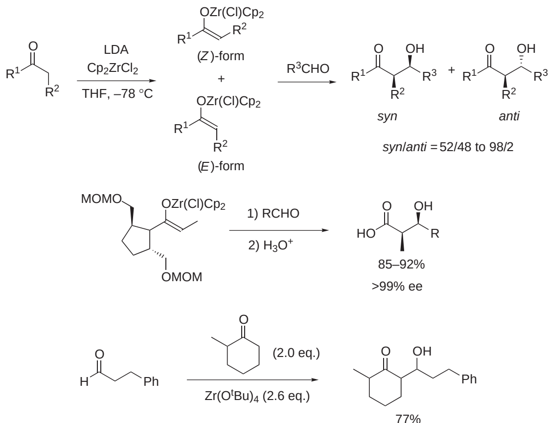
Scheme 36
