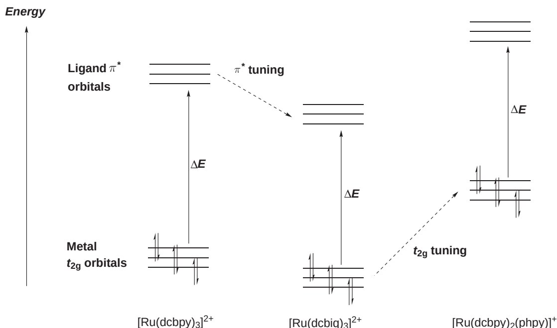
Figure 8 Tuning of HOMO ( t_{2g} ) and LUMO ( \pi^* ) orbital energy in various ruthenium polypyridyl complexes (Hphpy = 2-phenylpyridine).
