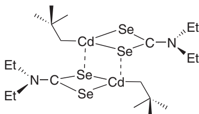
Figure 27 Structure of [\text{Me}_3\text{CCH}_2\text{Cd}(\text{Se}_2\text{CNEt}_2)]_2 .
