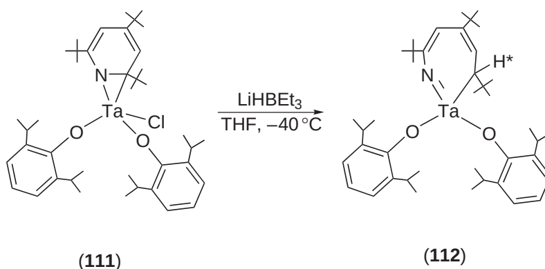
Scheme 49
