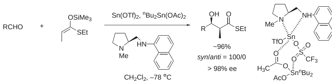
Scheme 80
