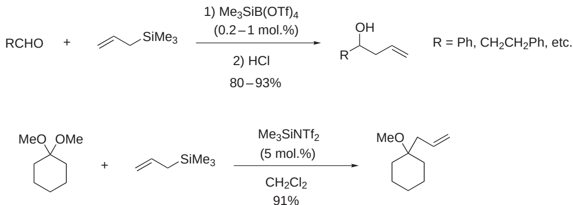
Scheme 75
