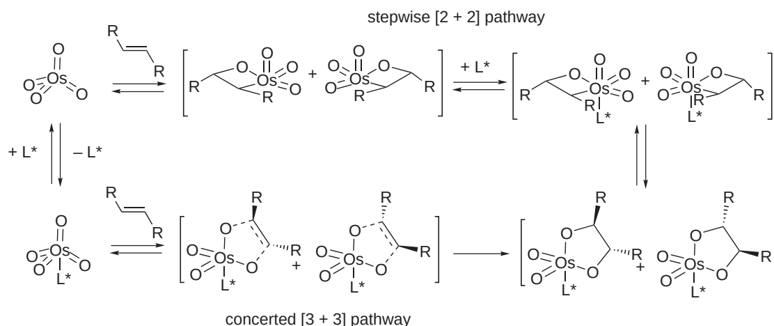
Scheme 50
