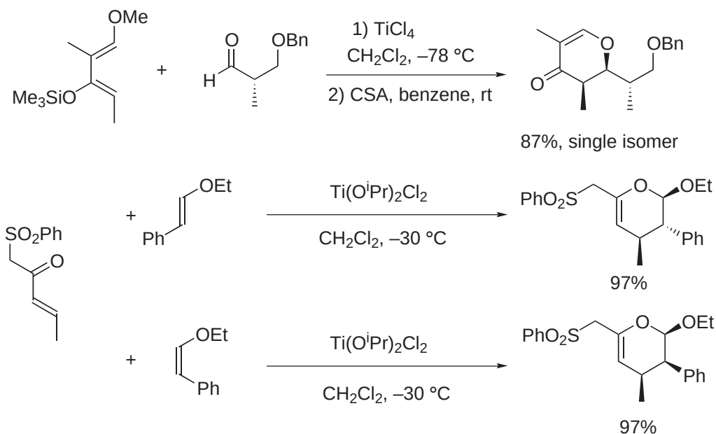
Scheme 26
