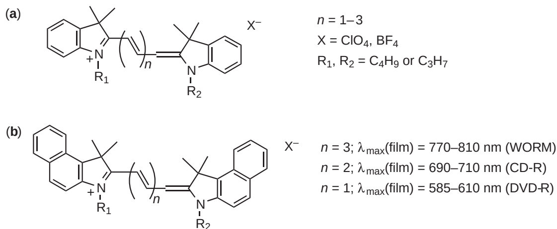
Scheme 6
