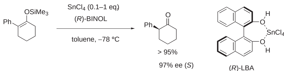
Scheme 83
