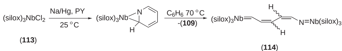
Scheme 50
