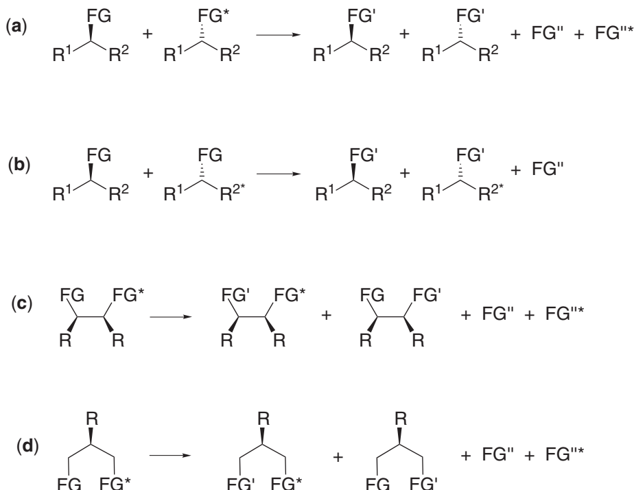
Scheme 15
