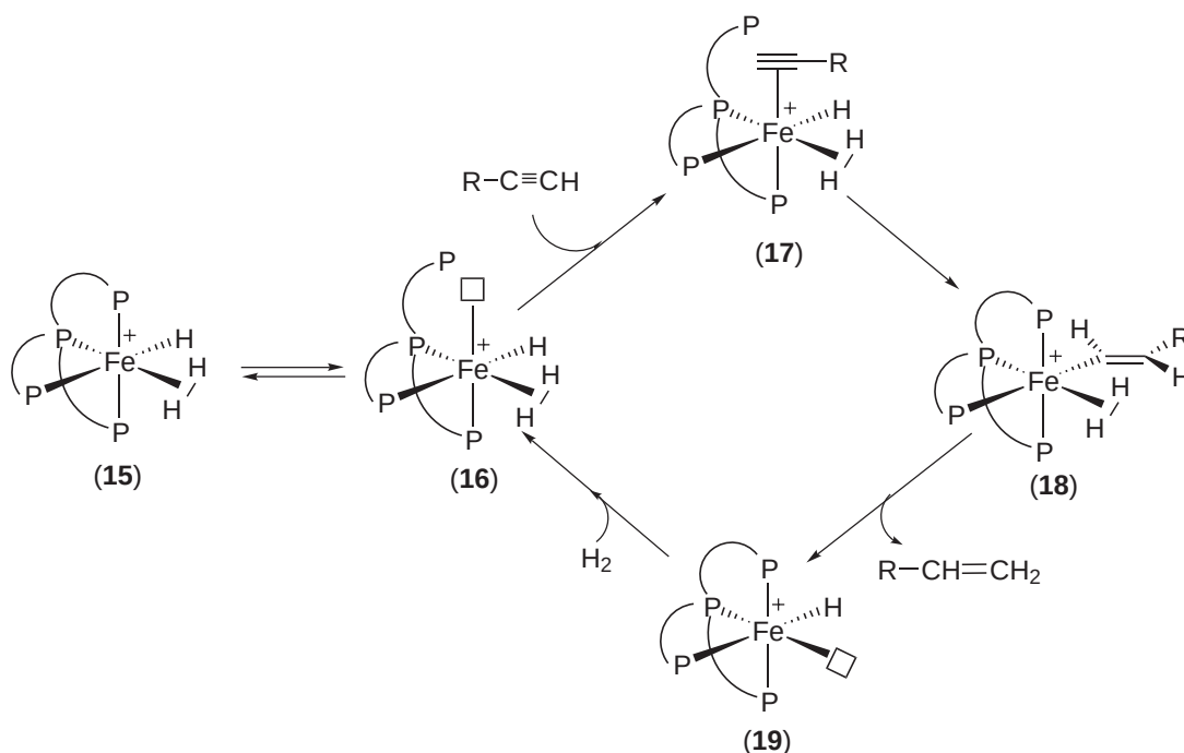
Scheme 6
