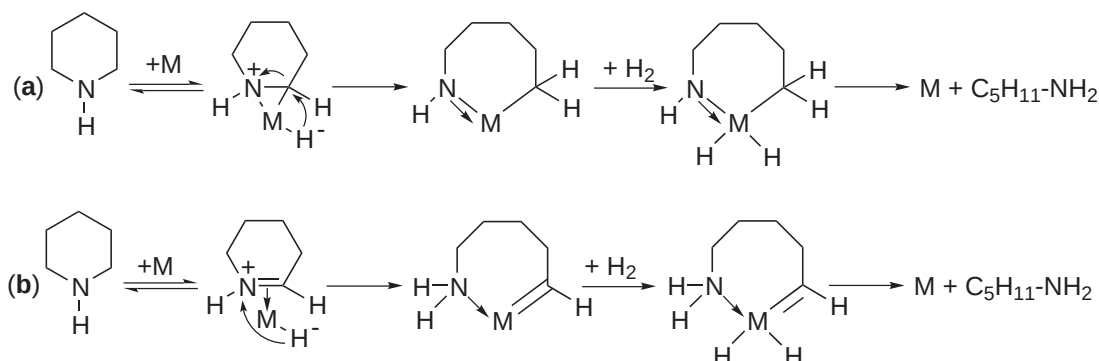
Scheme 46
