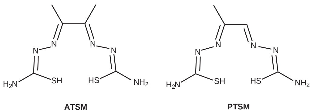
Figure 7 Bis(thiosemicarbazone) ligands for Cu II .
