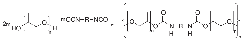
Scheme 20
