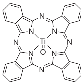
Titanyloxy phthalocyanine
