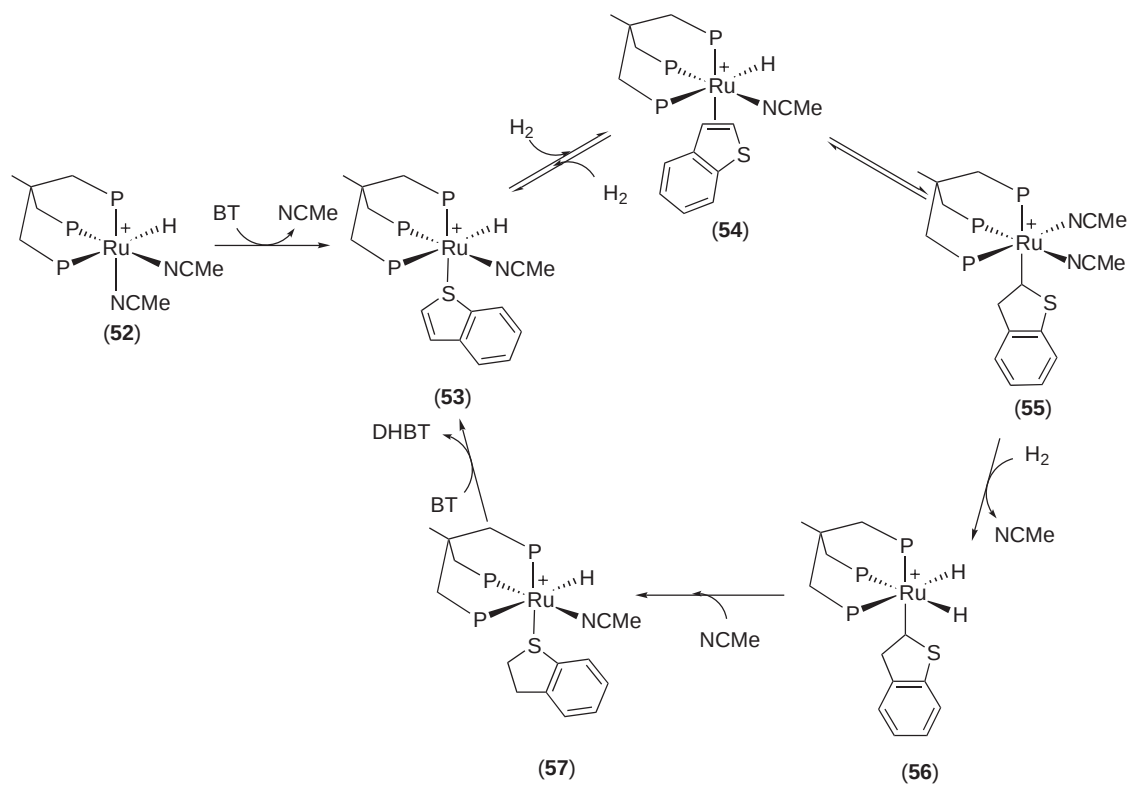
Scheme 14
