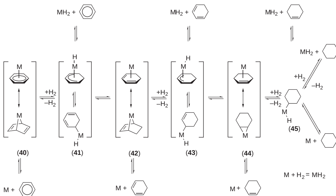
Scheme 12
