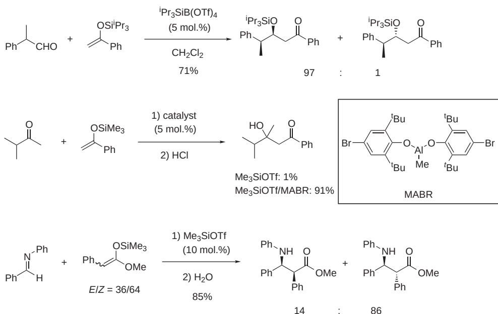
Scheme 74
