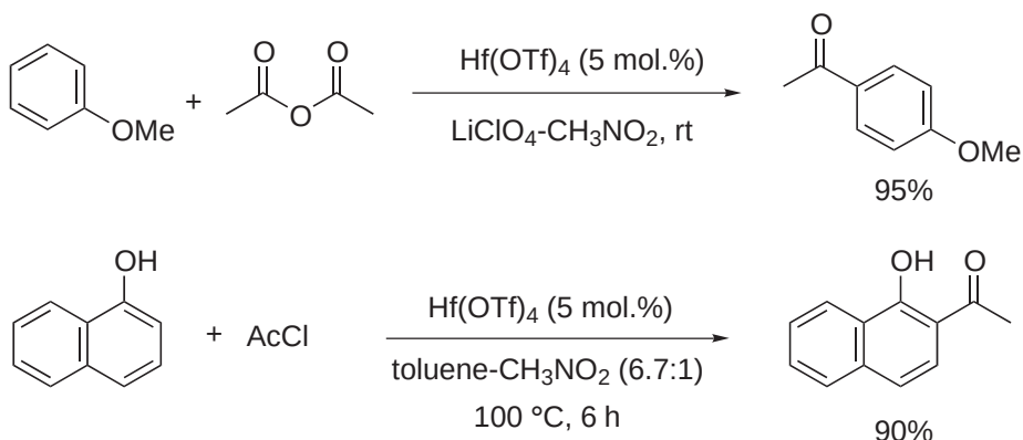
Scheme 42
