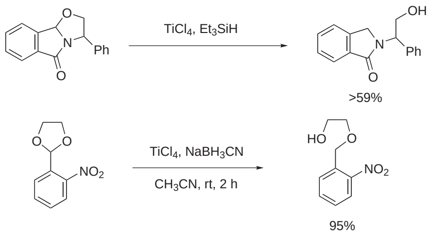
Scheme 24
