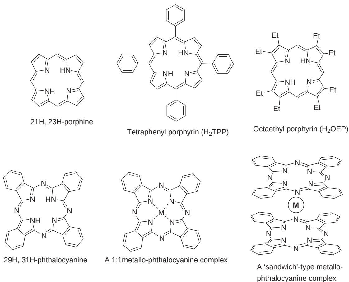
Scheme 2
