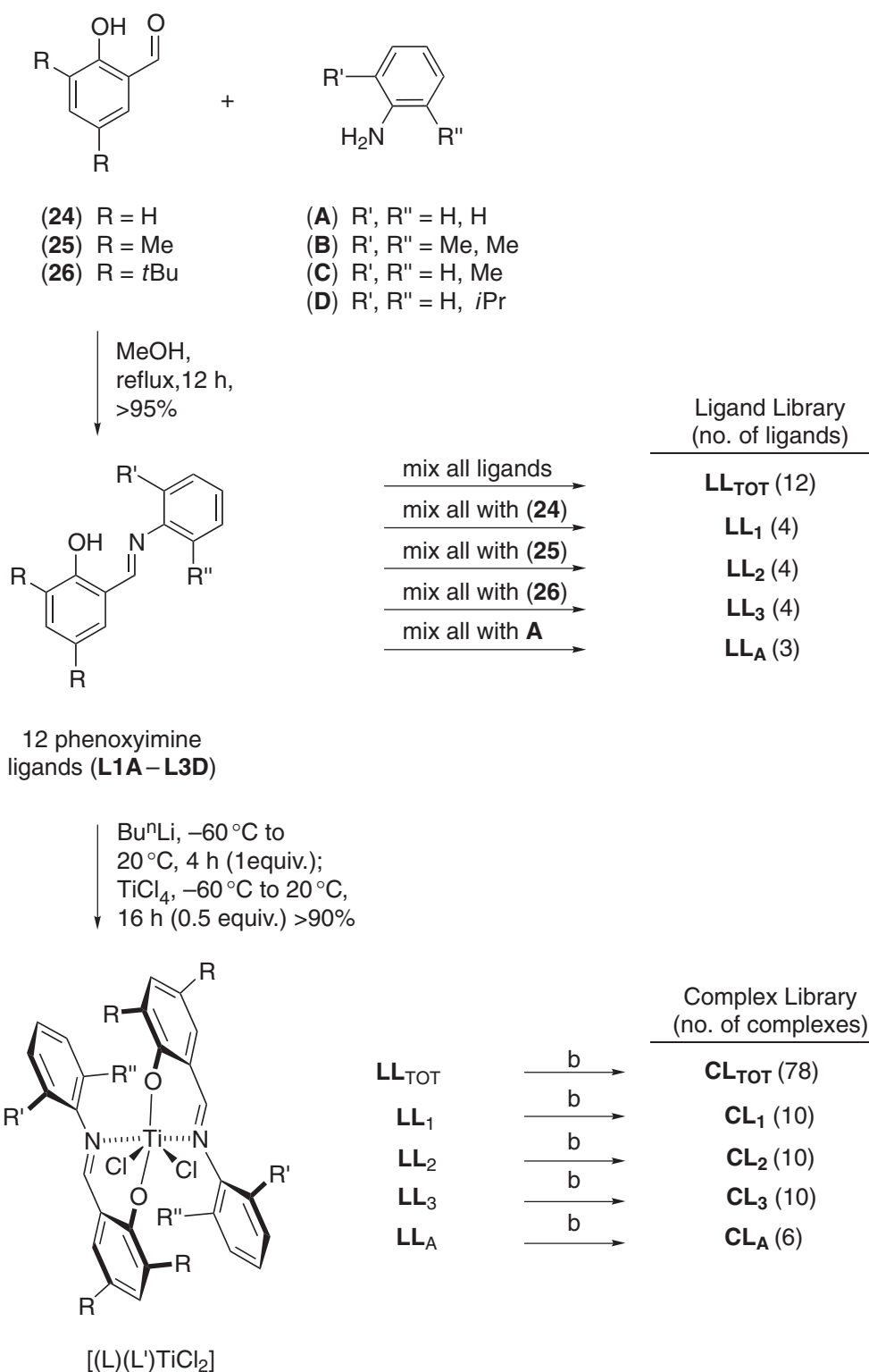
Scheme 5
