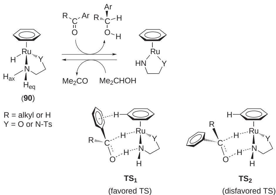
Scheme 29
