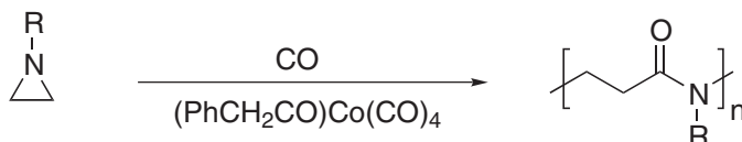
Scheme 26
