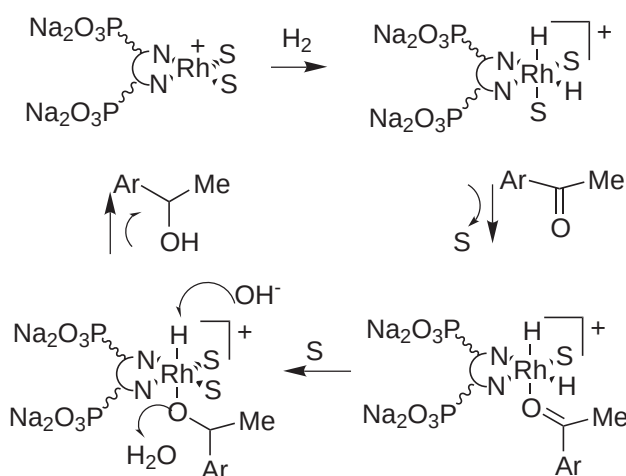
Scheme 56
