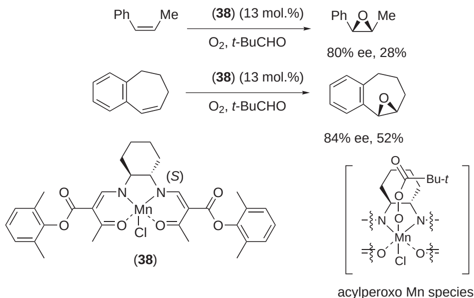
Scheme 22
