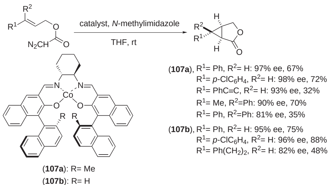
Scheme 84
