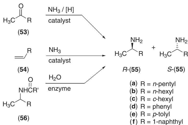
Scheme 14
