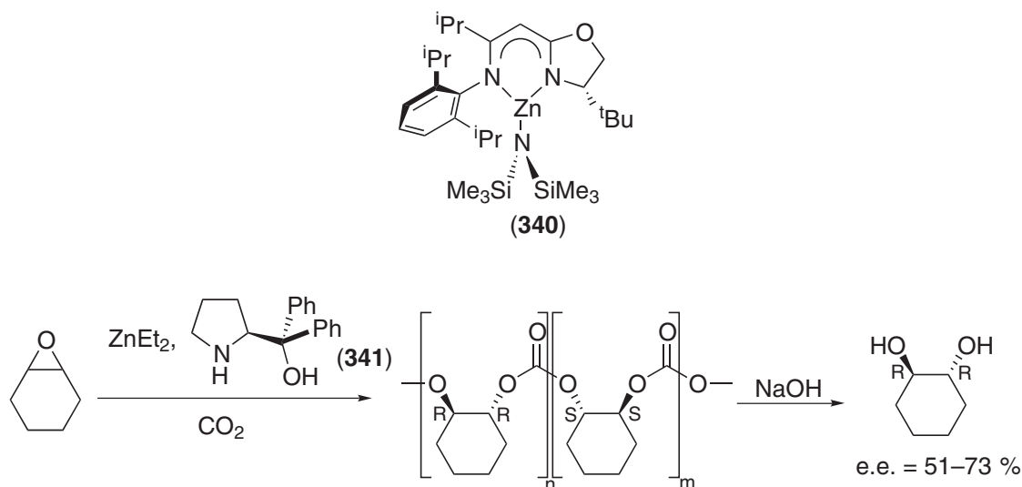
Scheme 23
