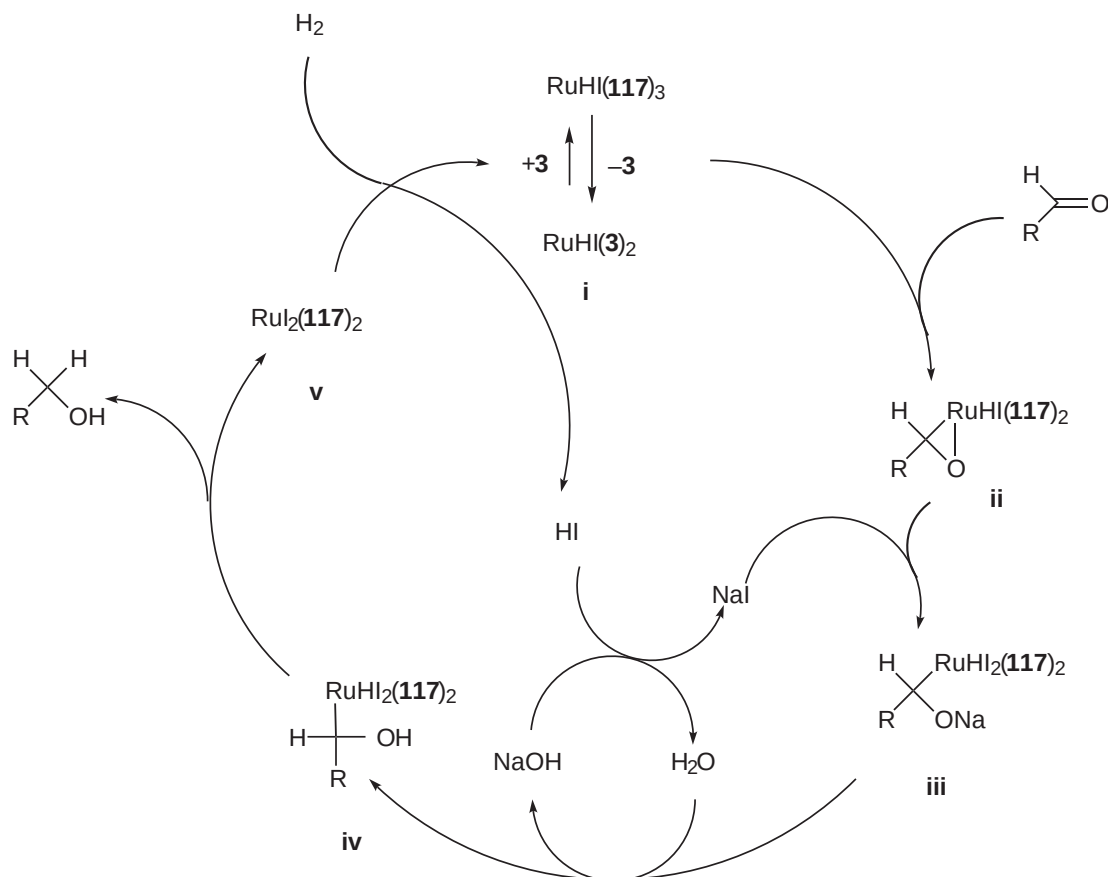
Scheme 60
