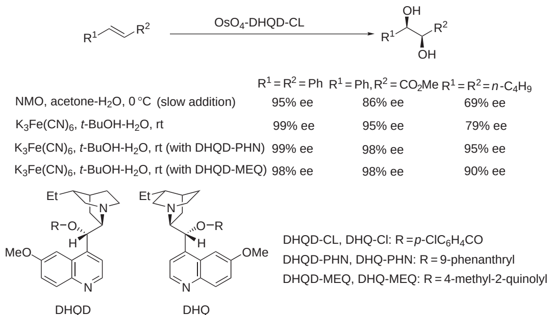
Scheme 46
