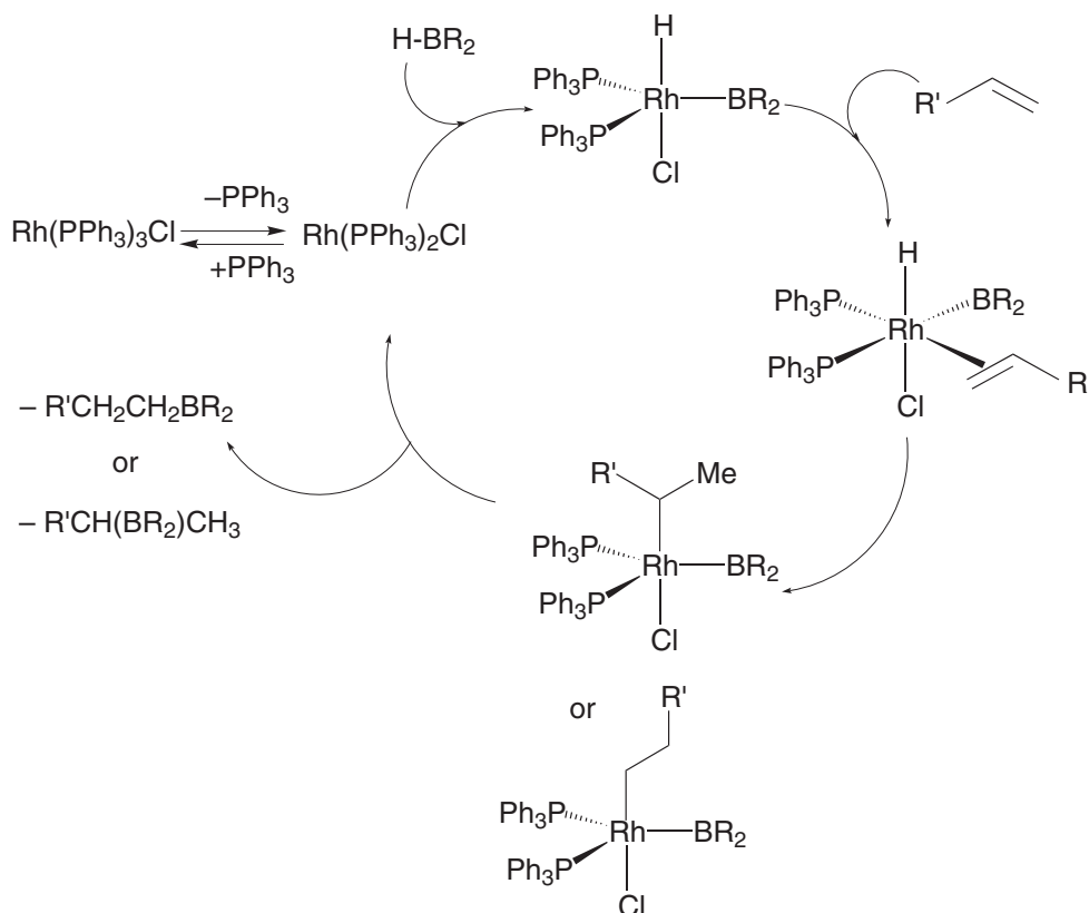
Scheme 3
