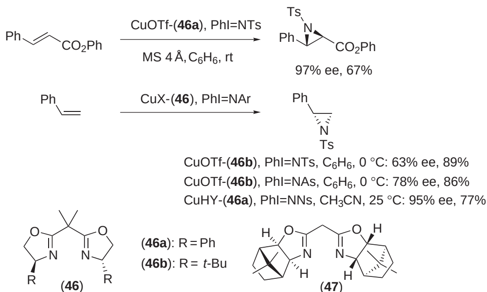
Scheme 34
