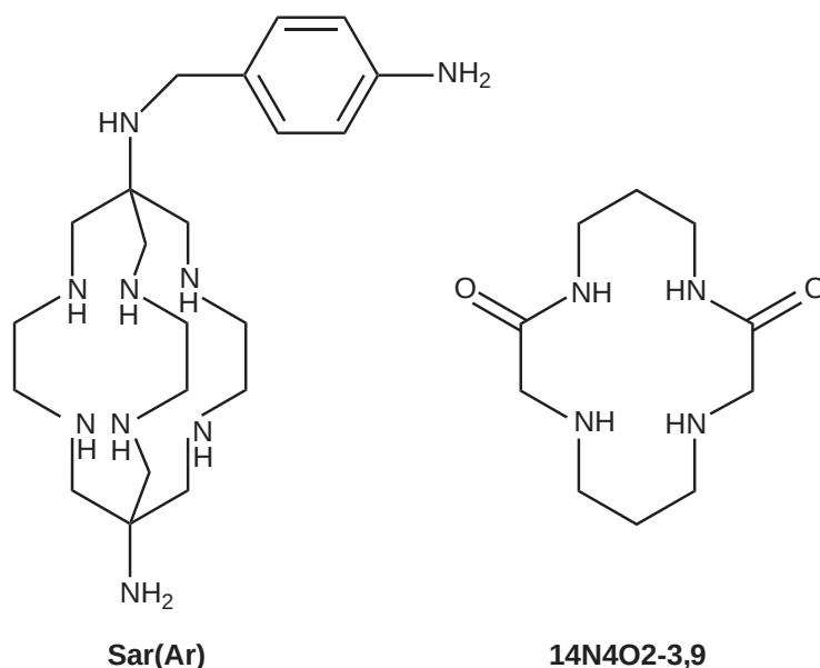
Figure 9 Macrocyclic ligands for Cu II .
