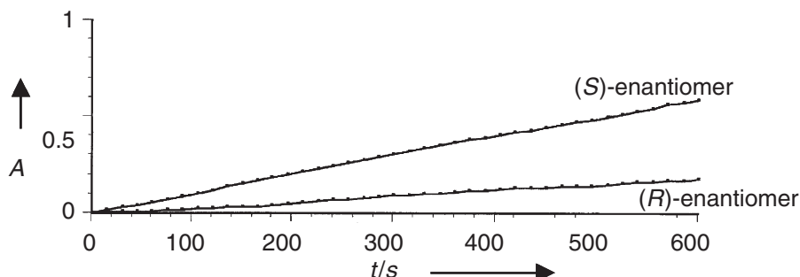
Figure 4 Course of the catalytic of the ( R )- and ( S )-ester ( 45 ) as a function of time. (a) Wildtype lipase from P. aeruginosa , (b) improved mutant in the first generation. 76
