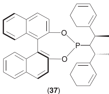
Scheme 21
