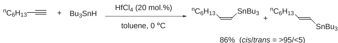
Scheme 43
