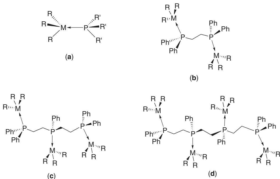
Figure 13 Structures of trialkylmetal adducts with multidentate phosphines: (a) [R_3M(PR_3)] ( M = Ga, In ; R = alkyl ); (b) [(R_3M)_2(\mu\text{-dppe})] ( M = Al, Ga, In ); (c) [(R_3M)_3(\mu^3\text{-triphos})] ( M = Al, Ga, In ); (d) [(R_3M)_4(\mu^4\text{-tetraphos})] ( M = Al, Ga, In ).
