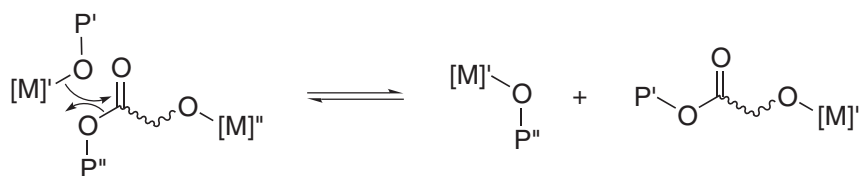
Scheme 17
