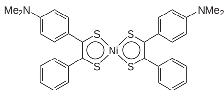
(156) : \lambda_{\text{max}} = 1064 \text{ nm} , \chi^{(3)}[\text{DFWM}] = 7.59 \cdot 10^{-11} \text{ esu (CH}_2\text{Cl}_2) 413
