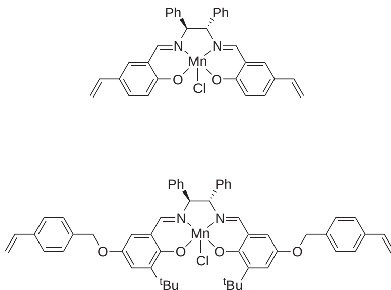
Figure 19 Polymer-supported chiral Mn(III)-salen complexes ( P = polymer support).
