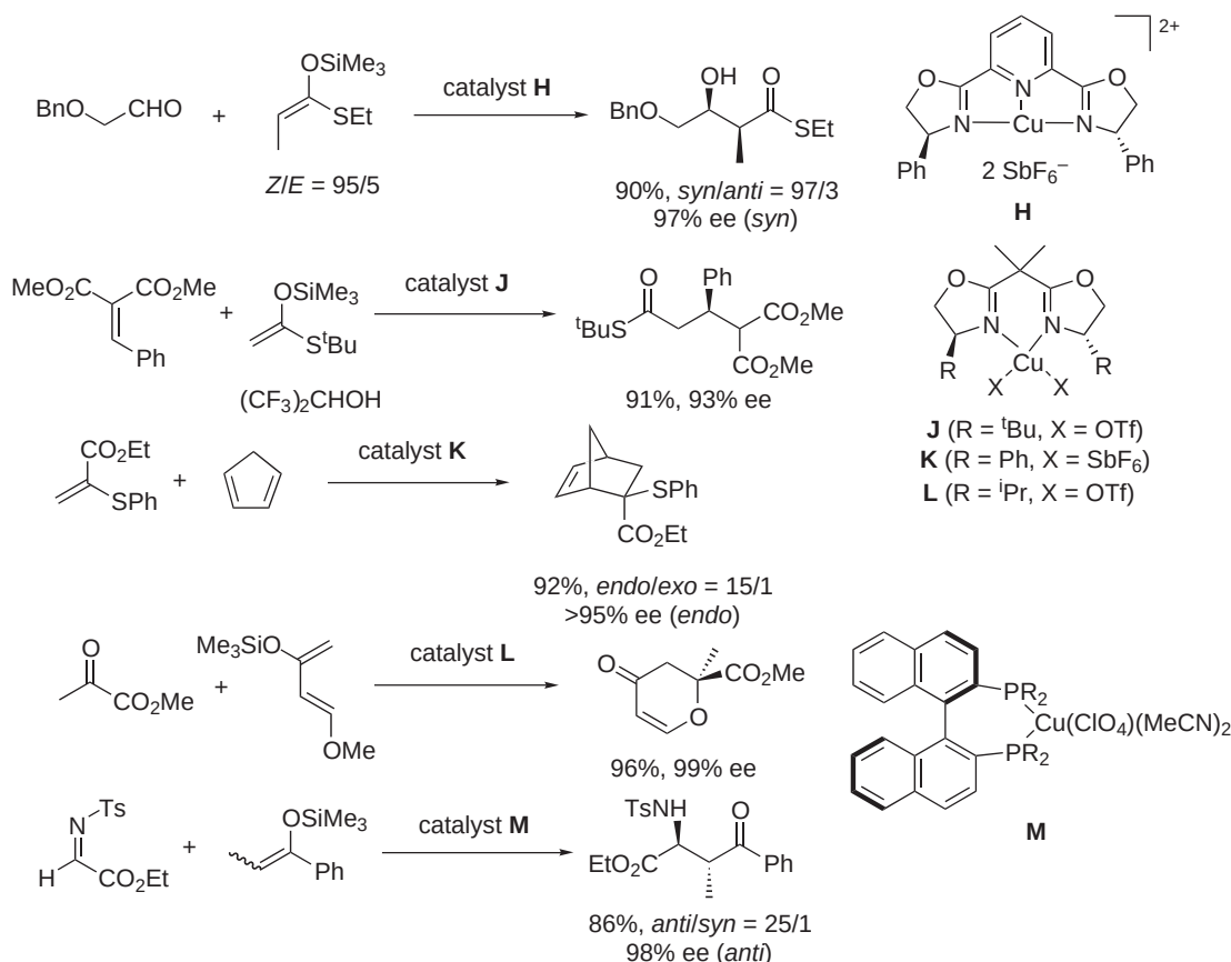
Scheme 48
