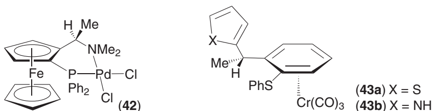
Scheme 25
