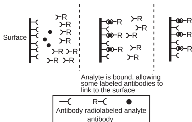
Figure 9 Representation of a typical radioimmunoassay.
