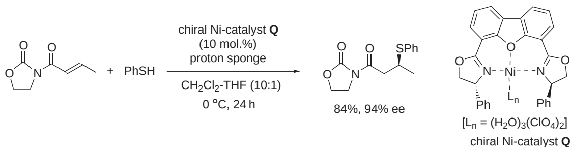
Scheme 59
