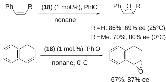
Scheme 11
