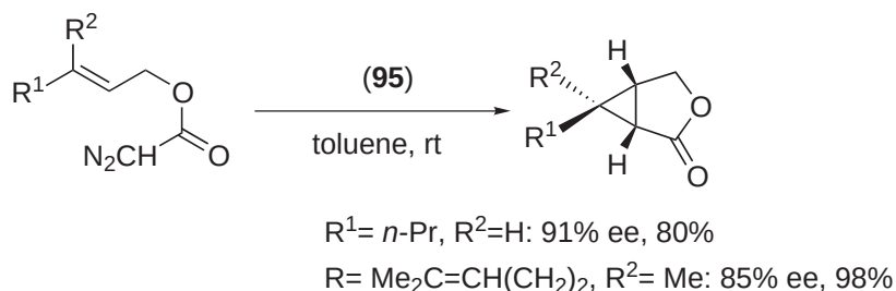
Scheme 83
