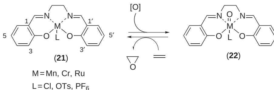
Scheme 12
