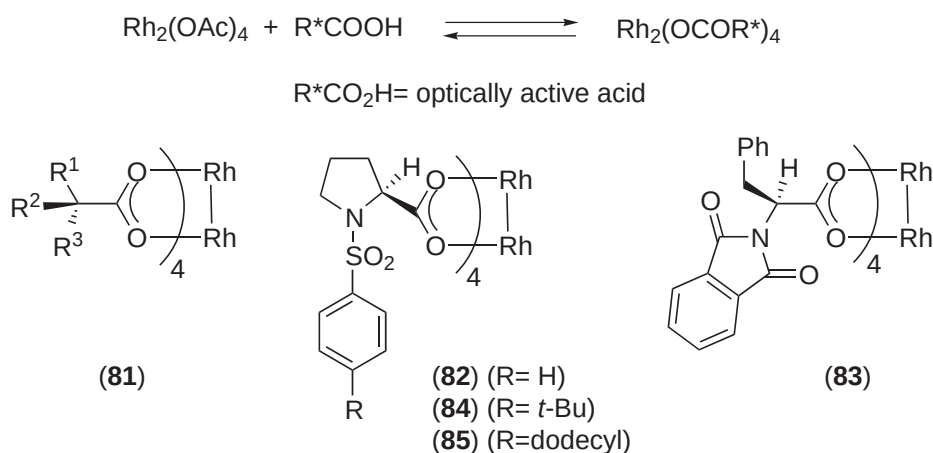
Scheme 63
