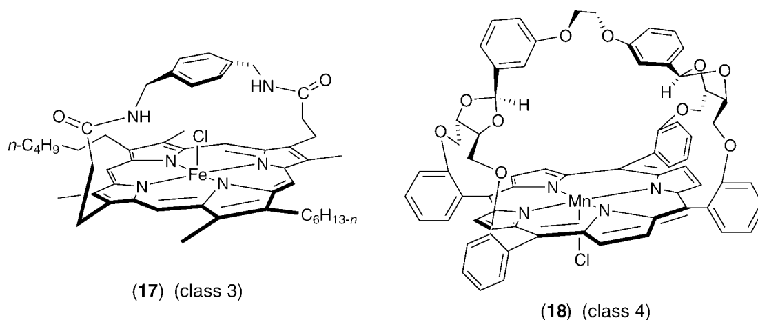
Figure 4 Metalloporphyrin complexes of classes 3 and 4.
