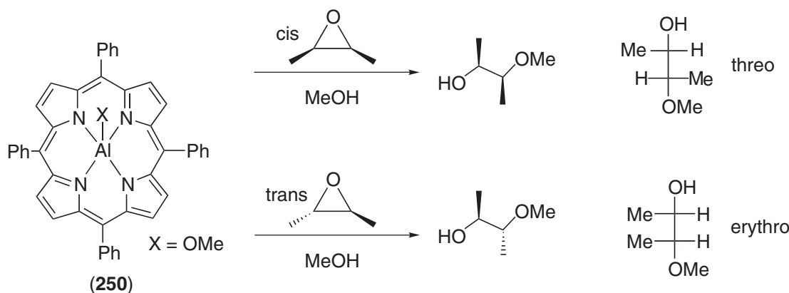
Scheme 21
