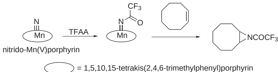
Scheme 31
