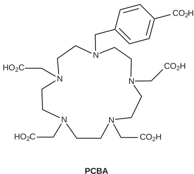
Figure 8 PCBA ligand for Cu II .
