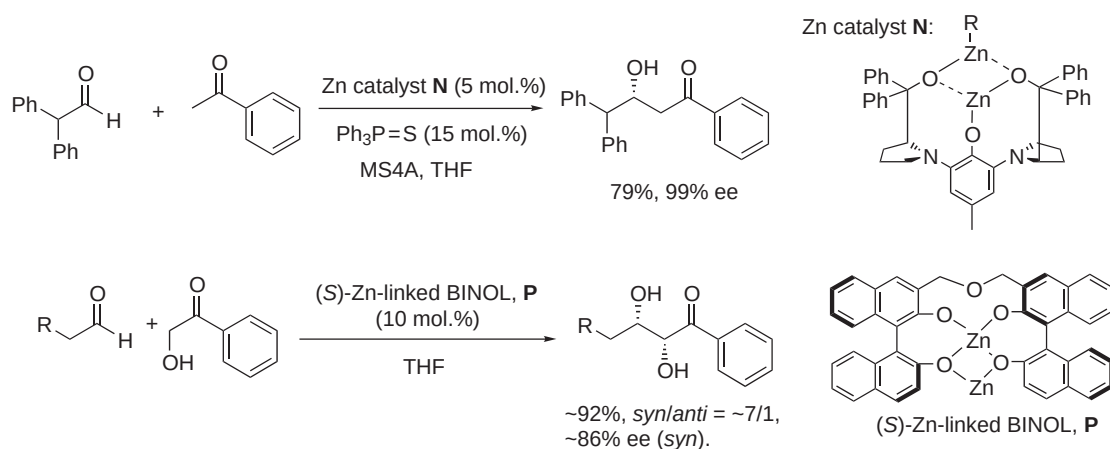
Scheme 55
