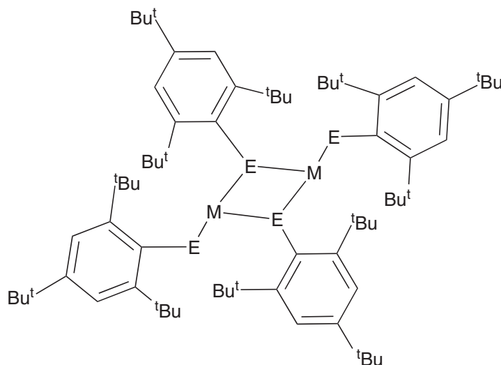
Figure 32 Structure of [M(EC_6H_2Bu^t)_2]_2 ( E = S, Se ; M = Cd ).
