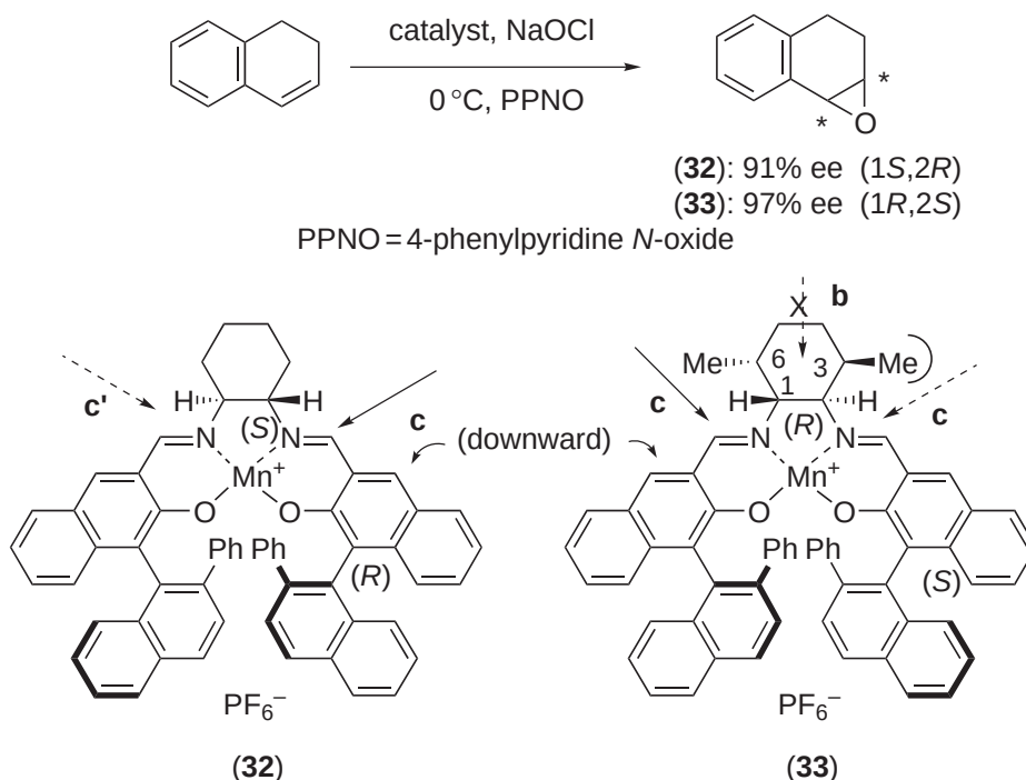
Scheme 17
