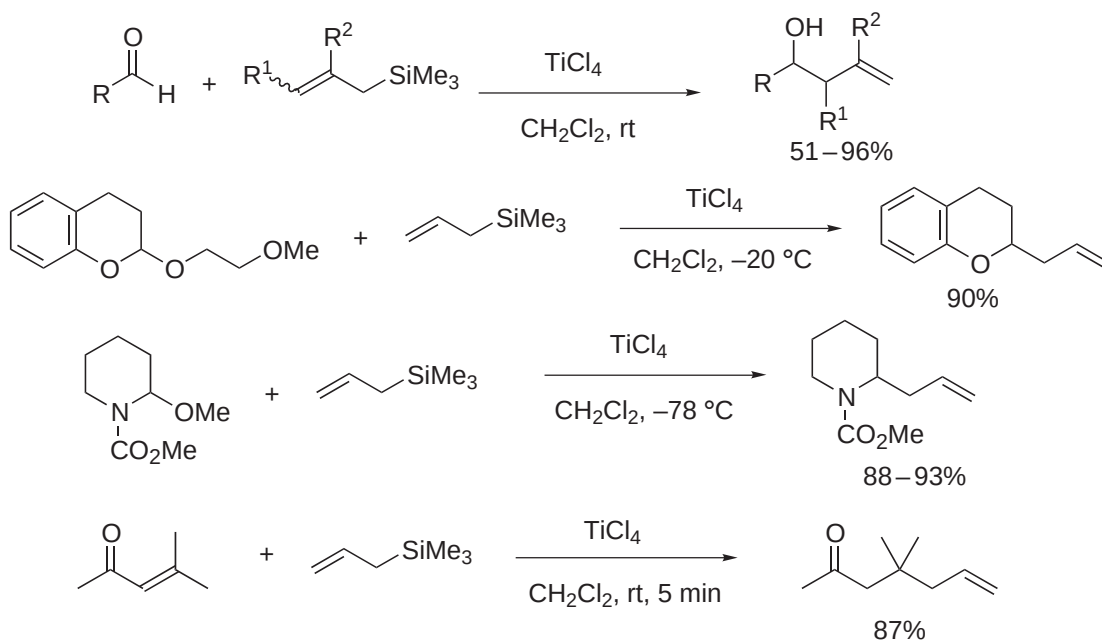
Scheme 21
