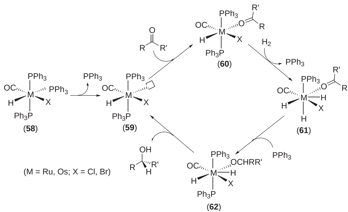
Scheme 15
