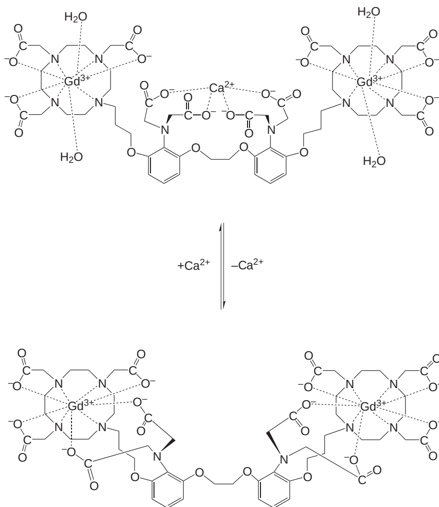
Scheme 17
