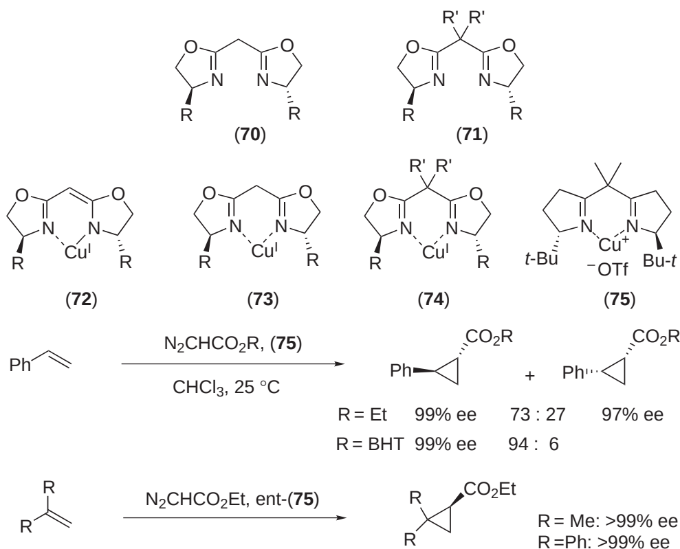
Scheme 61
