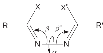
Figure 4 Conformational flexibility of open-chain diazine ( N-N ) systems.
