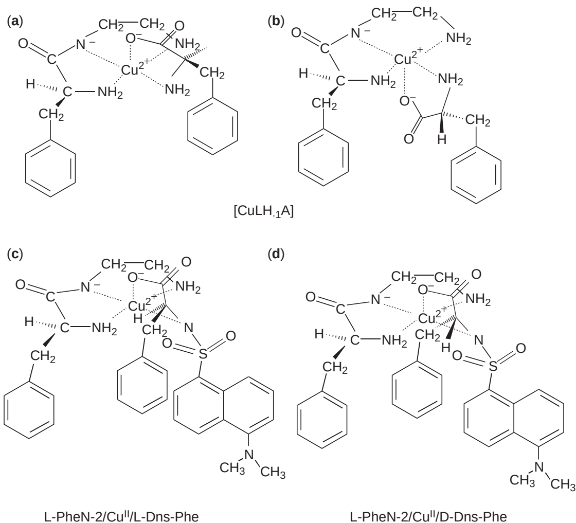
Figure 1 (a), (b) Two coordination modes of D-phenylalanine with [Cu II (N-L-phenyl-alanylethanediamine)] resolving agent; (c) Geometry of L-dansylated phenylalanine complex of [Cu II (N-L-phenylalanatoethanediamine)] resolving agent; 60 and (d) D-dansylated phenylalanine complex of [Cu II (N-L-phenylalanatoethanediamine)] resolving agent. 60
