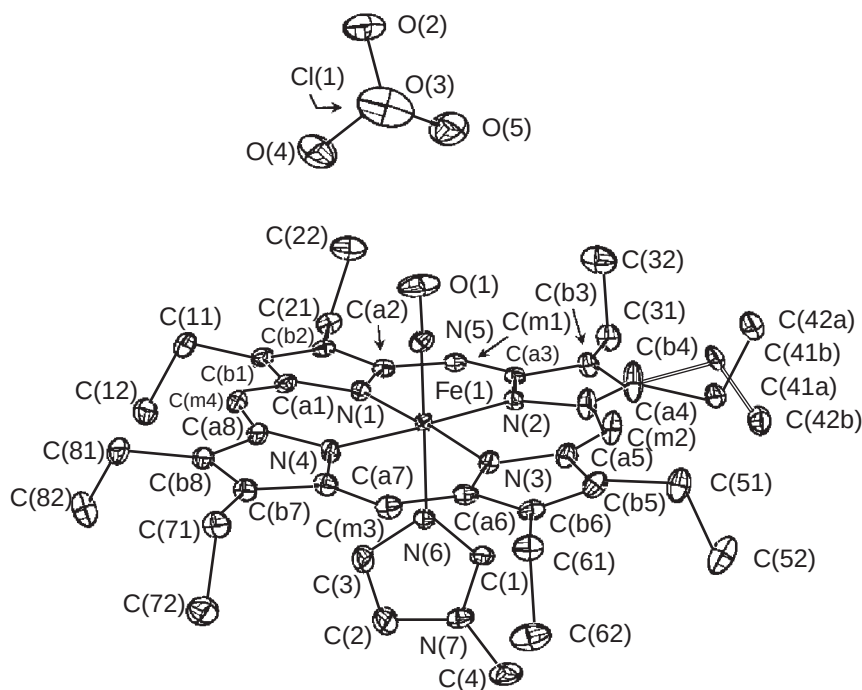
Figure 2 ORTEP diagram of [\text{Fe}(\text{OEP})(1\text{-MeIm})(\text{NO})]\text{ClO}_4 ; 50% probability ellipsoids (reproduced by permission of Ellison and Scheidt, 1999; 28 © American Chemical Society).
