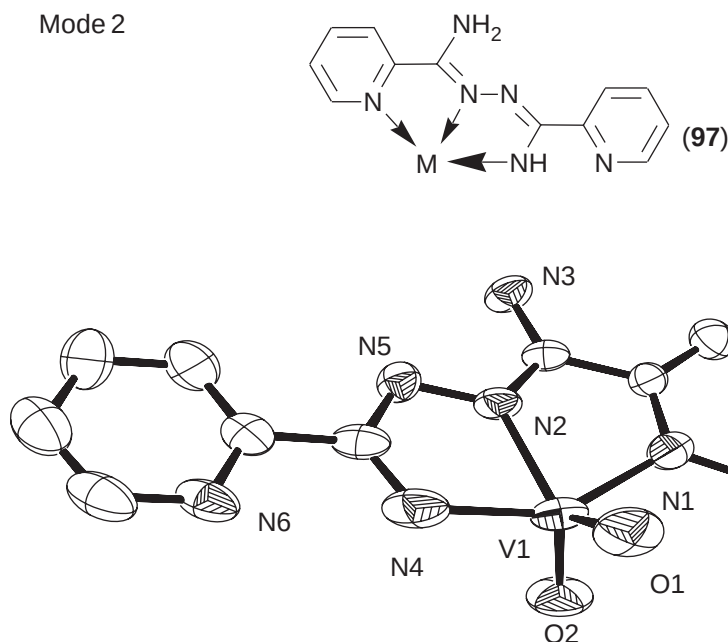
Figure 9 Structural representation of mode 2 in a mononuclear complex containing ligand (97).
