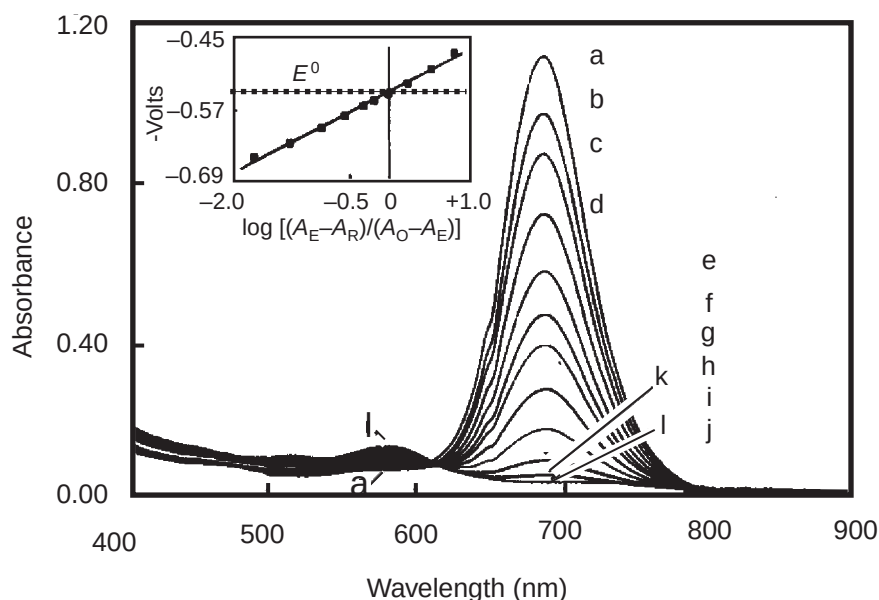
Figure 2 Absorption spectra of a 6.08 mM solution of \text{Re}_3\text{Cl}_9 in the 49 mol.% \text{AlCl}_3 -MeEtImCl salt at 40 °C in at various applied potentials (V): (a) open-circuit; (b) -0.266 ; (c) -0.303 ; (d) -0.325 ; (e) -0.340 ; (f) -0.352 ; (g) -0.364 ; (h) -0.383 ; (i) -0.405 ; (j) -0.550 . Inset: Nernst plot constructed from the spectra (redrawn with permission from S. K. D. Strubinger, I. W. Sun, W. E. Cleland, C. L. Hussey, Inorg. Chem. , 1990 , 29, 993–999; © 1990, American Chemical Society).
