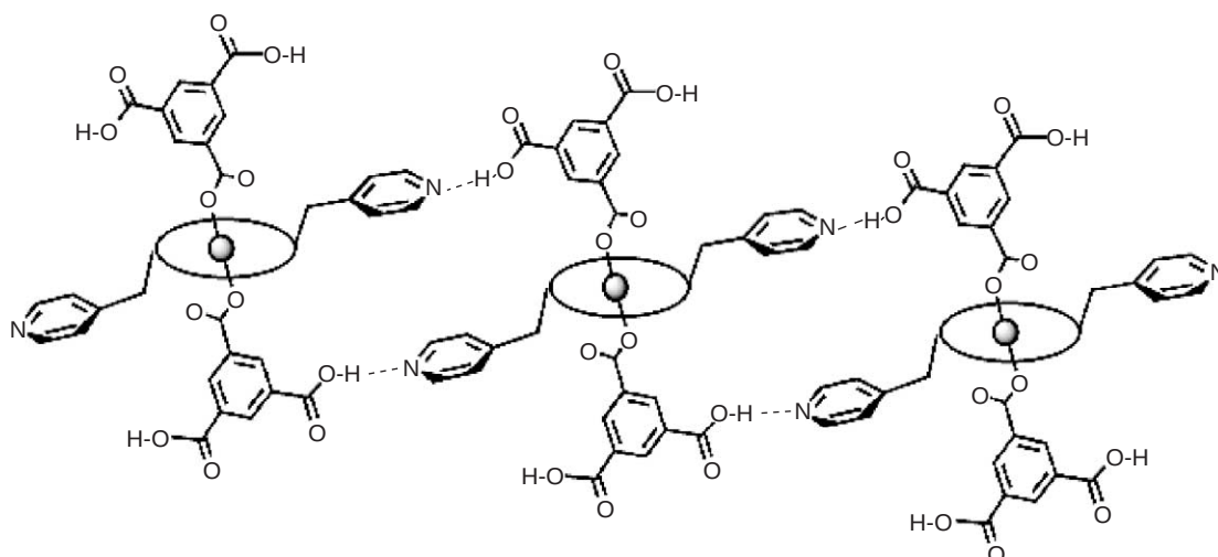
Figure 4 Macrocyclic complexes connected via carboxylic acid–pyridine hydrogen bonds.
