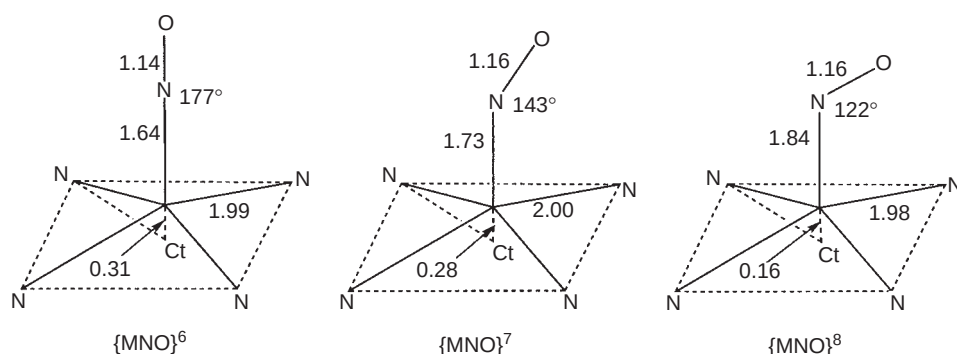
Figure 4 Formal diagrams for five-coordinate nitrosylmetalloporphyrin \{\text{MNO}\}^n , ( n=6, 7 , and 8 ). Distances and angles represent estimates of the “best” geometry (reproduced by permission of Wyllie and Scheidt, 2002; 20 © American Chemical Society).
