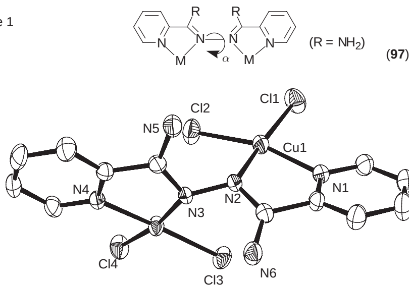
Figure 8 Structural representation of mode 1 in a dinuclear copper(II) complex containing ligand (97).
