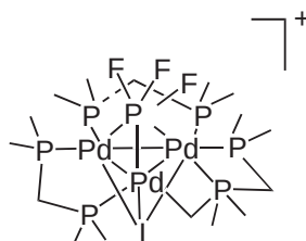
Figure 115 The cluster [\text{Pd}_3(\mu\text{-dppm})_3(\mu_3\text{-I})(\mu_3\text{-PF}_3)]\text{PF}_6 [dppm = bis-(diphenylphosphino)methane].
