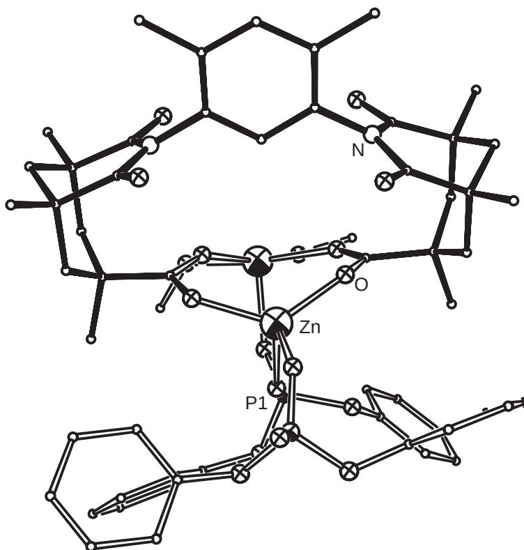
Figure 6 Molecular structure of a dimeric zinc compound with a bridging phosphodiester formed with ligands based on Kemp's triacid imide. 44†
