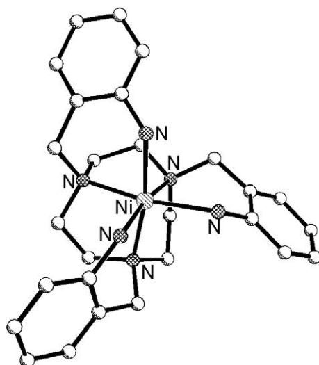
Figure 17 Molecular structure of [Ni(tabtacn)] 2+ . 1430
