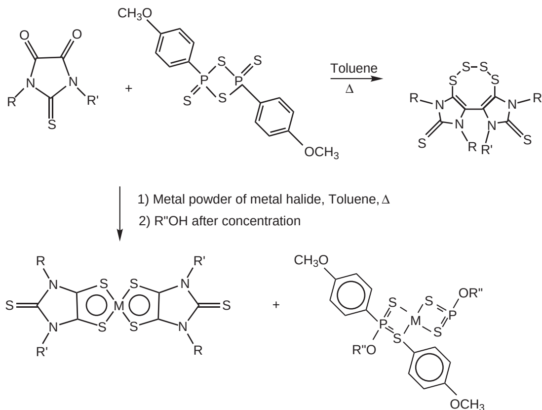
Scheme 4
