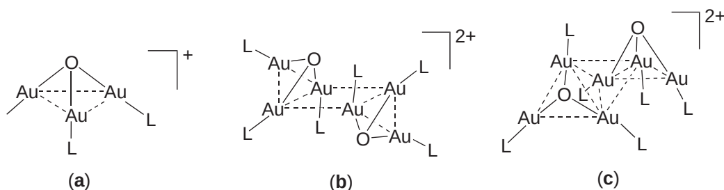
Figure 21 Different structures of [\text{O}(\text{AuL})_3]^+ cations.
