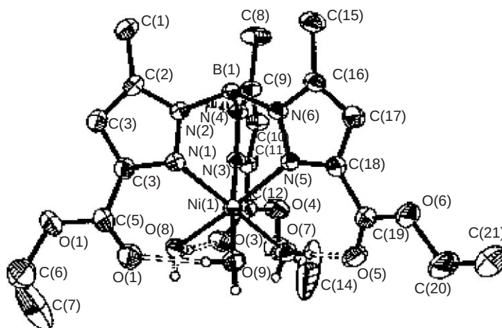
Figure 7 Molecular structure of (205) 617 (reproduced by permission of The Royal Society of Chemistry).
