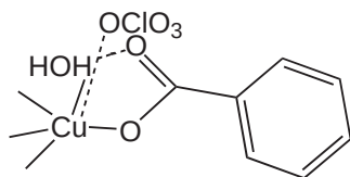
[(\text{Me}_3\text{TACN})\text{Cu}(\text{H}_2\text{O})(\text{benzoato})][\text{ClO}_4] ( 650 )
