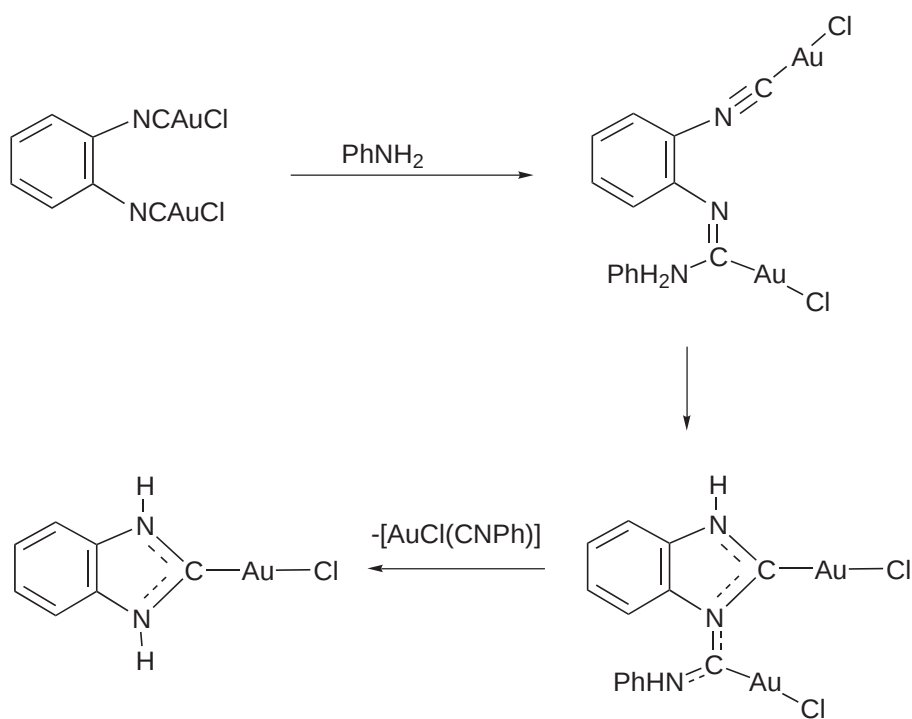
Scheme 32
