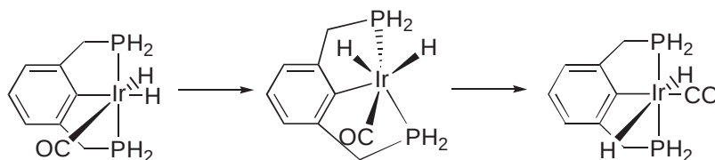
Scheme 19
