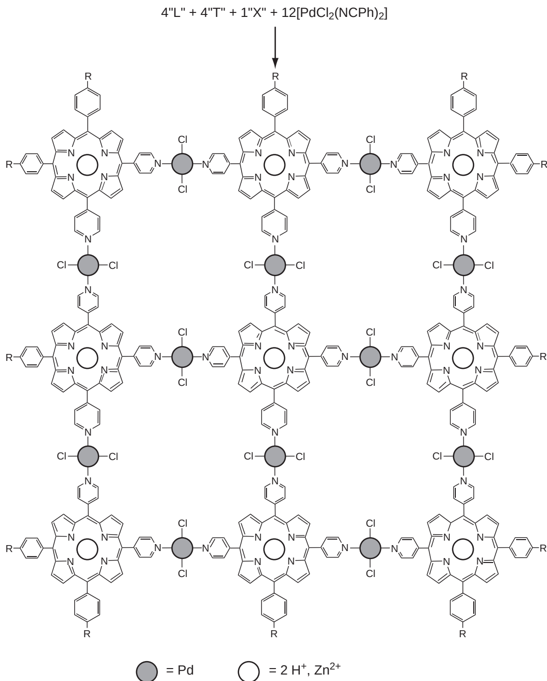
Figure 88 Nonameric arrays of porphyrins.
