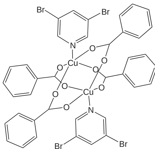
[(L)_2Cu_2(O_2CPh)_4(3,5-Br_2-pyridine)_2] ( 639 )
