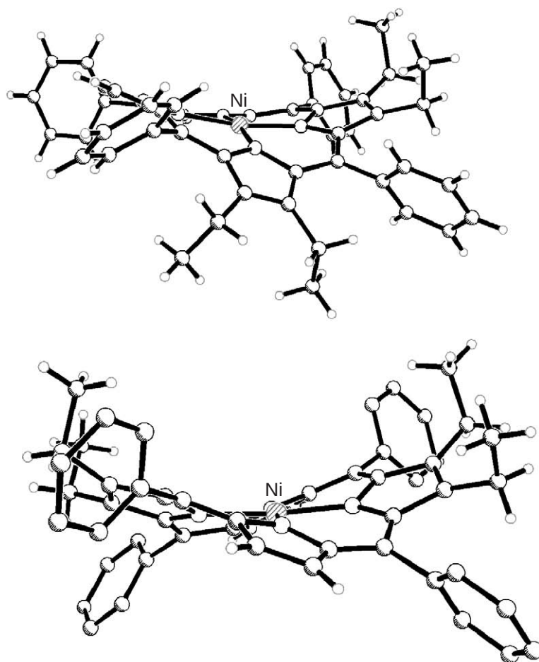
Figure 23 Side views of the molecular structures of one of the two independent molecules in the structures of \text{Ni}^{\text{II}} tTETPP (top) and \text{Ni}^{\text{II}} cTETPP (bottom). 1773
