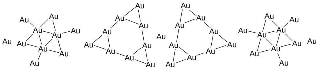
Figure 35 Layers of the cluster [\text{Au}_{39}\text{Cl}_6(\text{PPh}_3)_{14}]\text{Cl}_2 .
