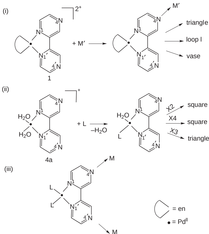
Figure 52 Use of the 2,2'-bipyrazine (2,2'-bpz) complexes [L_2Pd(2,2'-bpz-N^1, N^{1'})]^{2+} in which ( L_2 = \text{en} and L = \text{H}_2\text{O} ) as angular units for the generation of larger cationic aggregates.
