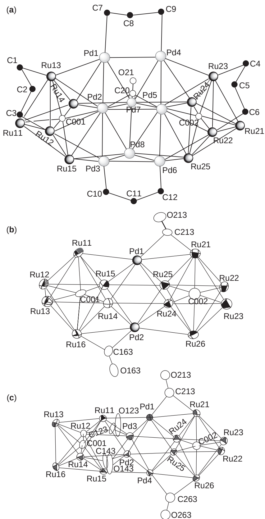
Figure 109 Structures of (a) [\text{Pd}_8\text{Ru}_{10}\text{C}_2(\text{CO})_{27}(\text{C}_3\text{H}_5)_4] ; (b) [\text{PPN}]_2[\text{Pd}_2\text{Ru}_{12}\text{C}_2(\text{CO})_{30}] ; and (c) [\text{PPN}]_2[\text{Pd}_4\text{Ru}_{12}\text{C}_2(\text{CO})_{32}] .
