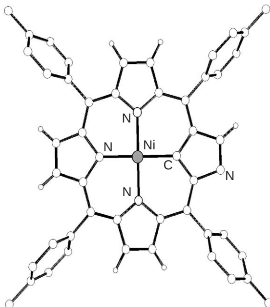
Figure 27 Molecular structure of [\text{Ni}^{\text{II}}(\text{CTPP})] .
