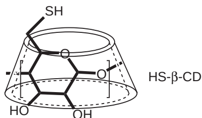
Figure 113 Structure of per -6-thio- \beta -cyclodextrin.
