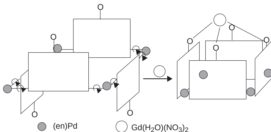
Figure 72 Generation of the cyclic species [(\text{en})\text{-Pd}(\text{dmpymo-}N^1, N^3)]_4^{4+} , by a self-assembly process.
