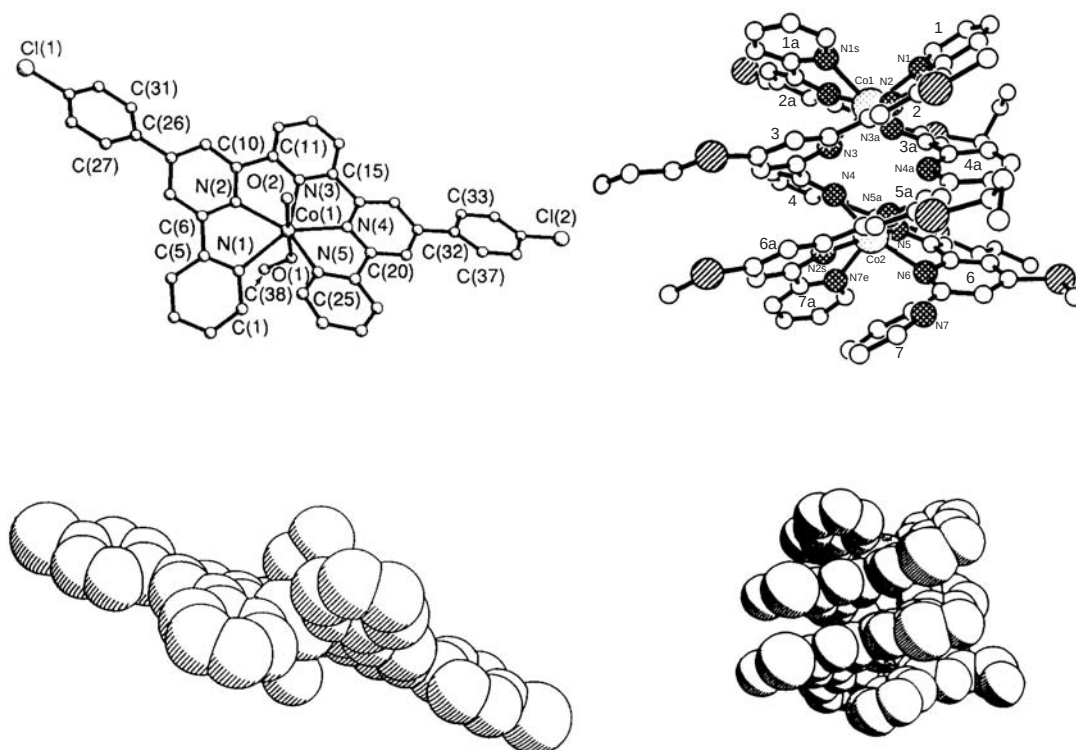
Figure 4 Mononuclear quinquenpyridine (4',4'''-bis(4-chlorophenyl) analogue) \text{Co}^{\text{II}} complex (left, reproduced with permission of the Royal Society of Chemistry from J. Chem. Soc., Chem. Commun. , 1992 , 768–771) and dinuclear septipyridine (4',4''''-bis(4-mercaptomethylphenyl)-4''''',4''''''-bis(4-mercaptopropylphenyl) derivative) dicobalt(II) complex (right, reproduced with permission of the American Chemical Society from Inorg. Chem. , 1993 , 32, 5477–5484). Space filling representations also shown.
