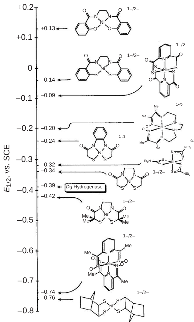
Figure 1 Comparative display of low-potential \text{Ni}^{\text{II/III}} redox couples 298 (reprinted with permission from ref. 298; © 1991, American Chemical Society).
