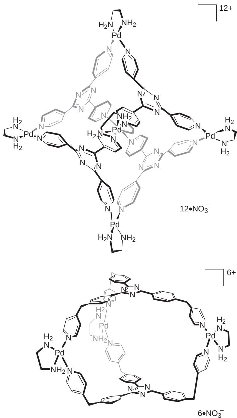
Figure 78 Two preformed \text{Pd}^{\text{II}} cage compounds that are reorganized into the three-dimensionally interlocked catenane in high yield when they are mixed in an aqueous solution.
