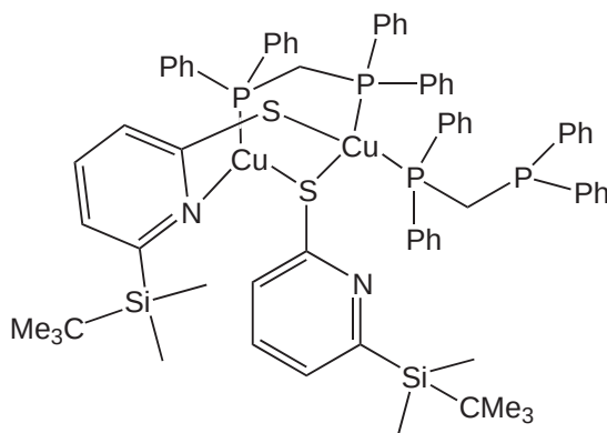
[(L)_2Cu_2(L')_2] ( 789 )
