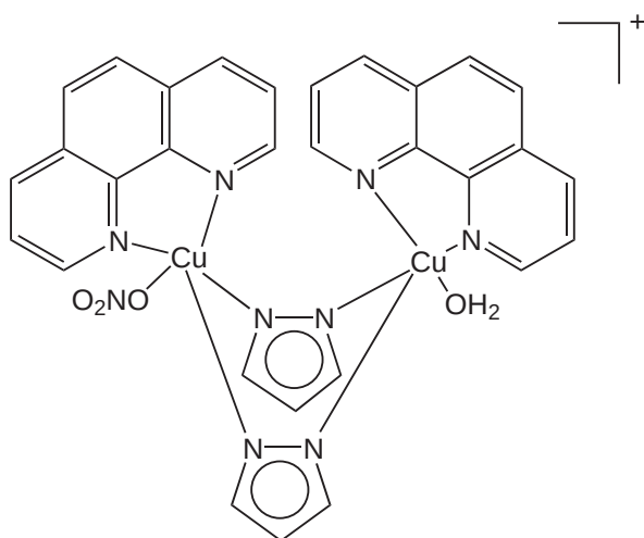
[(L)_2Cu_2(pz)_2(ONO_2)(H_2O)][NO_3] ( 603 )
