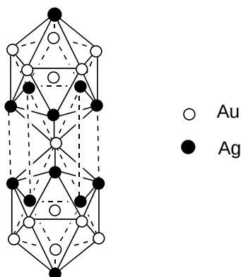
Figure 36 Core of [(\text{Ph}_3\text{P})_{19}\text{Au}_{13}\text{Ag}_{12}\text{Br}_8]^+ .
