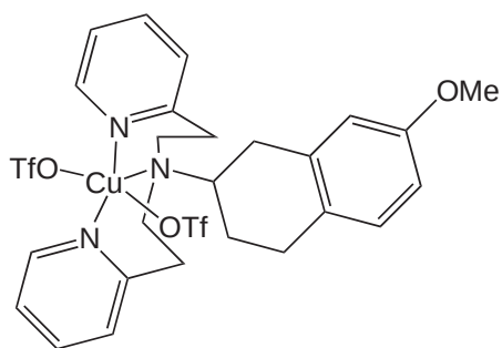
[(L)Cu(OTf)_2] ( 200 )
