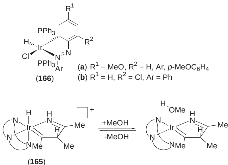
Scheme 20
