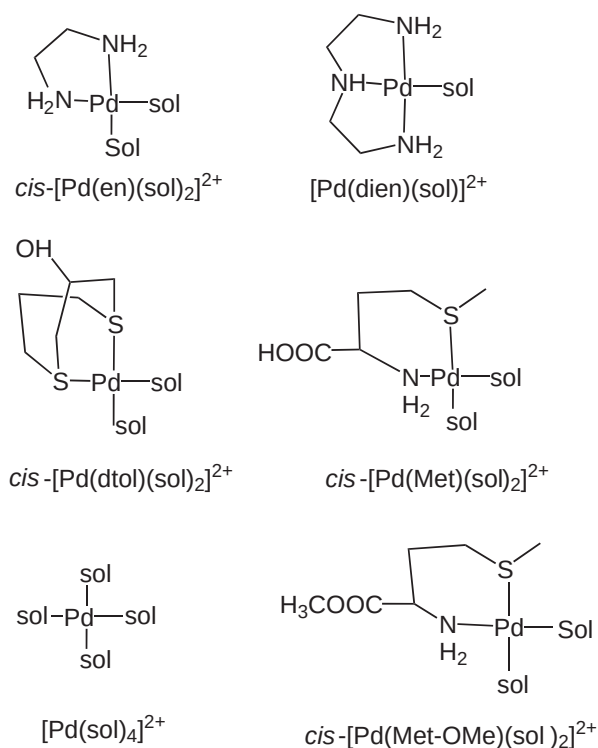
Figure 36 Complexes catalyzing hydrolytic cleavage of peptides, hydrolysis and alcoholysis of nitriles, decomposition of urea to carbon dioxide and ammonia, and alcoholysis of urea to ammonia and various carbamate esters.
