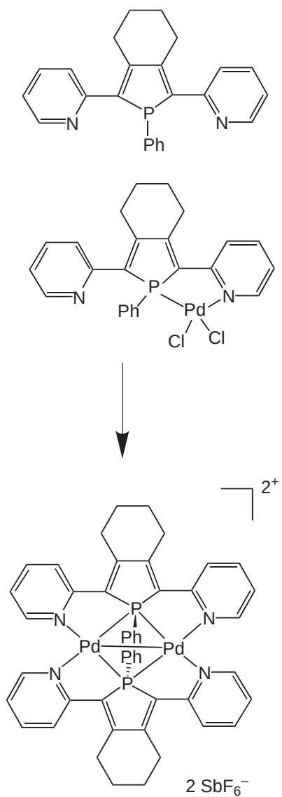
Figure 47 The new dinuclear Pd(I) complex.
