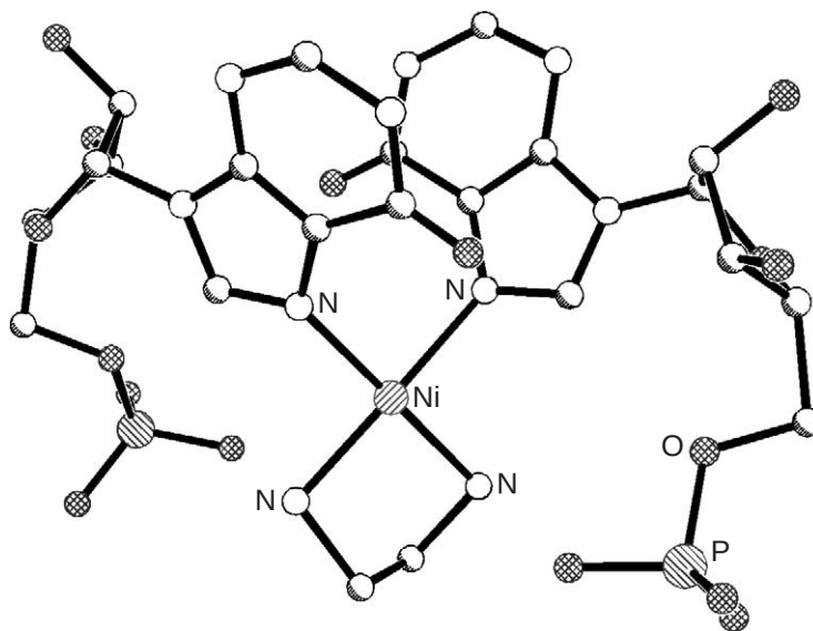
Figure 29 Molecular structure of the complex [\text{Ni}(\text{5'GMPPH})_2(\text{en})(\text{H}_2\text{O})_2] .
