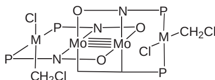
Figure 112 \text{Mo}_2\text{Pd}_2\text{Cl}_2(\text{CH}_2\text{Cl})_2(\text{pyphos})_4 .
