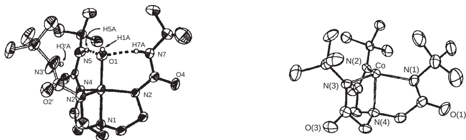
Figure 7 Tripodal triamide complexes of (left) (82) with hydroxocobalt(III) (divalent complex is similar) (reproduced with permission of the American Chemical Society from Inorg. Chem. , 2001 , 40, 4733–4741) and (right) (83) with \text{Co}^{\text{II}} (reproduced with permission of the American Chemical Society from Inorg. Chem. , 1998 , 37, 1527–1532).
