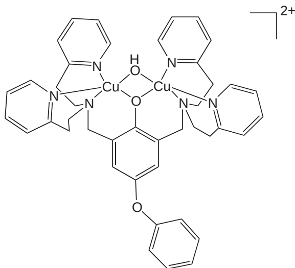
[(L)Cu 2 (OH)][BPh 4 ] 2 ( 172 )
