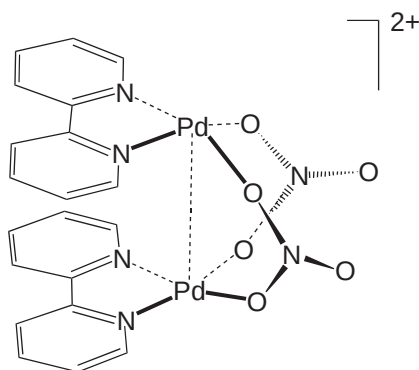
Figure 45 Structure of \{cis-[(2,2\text{-bipyridine})\text{palladium(II)}]_2(\mu\text{-}1,3\text{-NO}_3)_2\}^{2+} .
