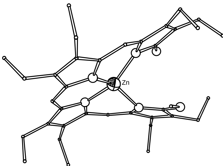
Figure 14 Molecular structure showing the helical nature of the zinc complex with a 19-methoxyoctaethylbilinone ligand formed on ring opening of the oxaporphyrin macrocycle. 828
