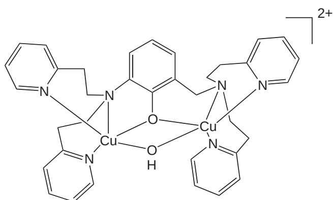
[(\text{L})\text{Cu}_2(\text{OH})][\text{PF}_6]_2 ( 176 )
