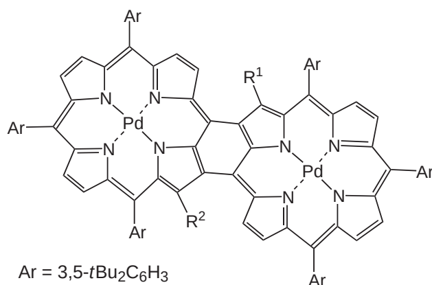
Figure 43 Doubly meso- \beta -linked diporphyrin products obtained in the reaction of \text{Pd}^{\text{II}} -porphyrin with 1.2 equivalents of BAHA.
