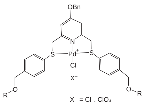
Figure 39 A Pd metallodendrimer.
