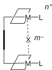
Figure 67 Cofacial disposition of the metals allowing for the incorporation of negatively charged ligands and complexes into the molecular clefts.
