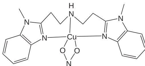
[(L)Cu(ONO)][ClO 4 ]·MeCN ( 77 )
