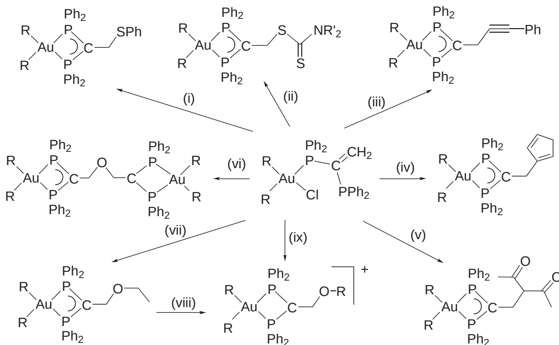
Scheme 16 \text{R} = \text{C}_6\text{F}_5 (i) \text{NaSPh} , (ii) \text{NaS}_2\text{CNR}'_2 , (iii) \text{AgCCPh} , (iv) \text{TlCp} , (v) \text{Tl}(\text{ACAC}) , (vi) 1/2 \text{Ag}_2\text{O} , (vii) \text{NaOEt} , (viii) \text{HClO}_4 , (ix) \text{AgClO}_4 + \text{OR} .
