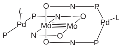
Figure 111 \text{Mo}_2\text{Pd}_2(\text{pyphos})_4(\text{L})_2 [ \text{L} = acrylonitrile, fumaronitrile, tetracyanoethylene].
