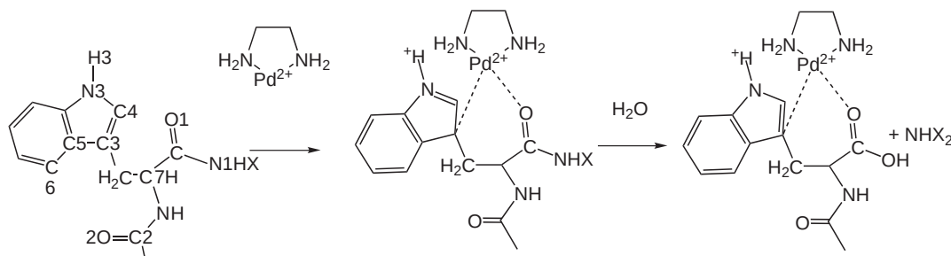
Scheme 9
