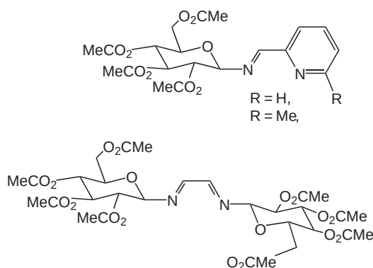
Figure 103 Improved N,N-ligands.
