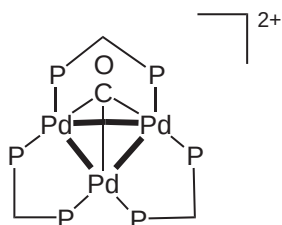
Figure 106 The complex ion [\text{Pd}_3(\text{dppm})_3(\text{CO})]^{2+} .
