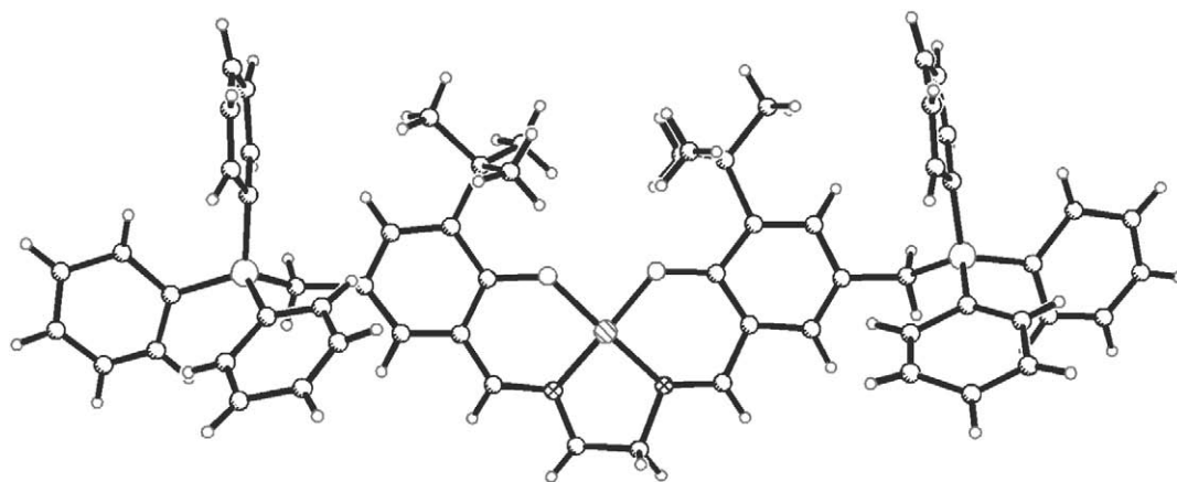
Figure 12 Crystal structure of N,N' -bis{3- t -butyl-5-[(triphenylphosphonium)methyl]salicylidene}-1,2-ethanediamine chloride with \text{Ni}^{\text{II}} ions. 1160
