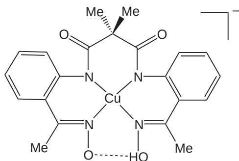
[Et 4 N][Cu(L)] ( 439 )
