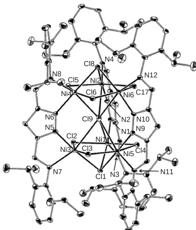
Figure 31 Hexanuclear \text{Ni}^{\text{II}} cage complex ( 832 ) with an interstitial \mu_6\text{-Cl} atom 2033 (reproduced by permission of the Royal Society of Chemistry).
