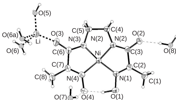
Figure 6 Structure and numbering scheme for the complex \text{Li}[\text{Ni}(\text{H}_{-1}\text{pen})]\cdot 4\text{H}_2\text{O} .
