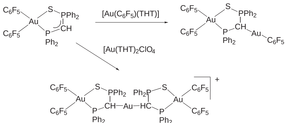
Scheme 23
