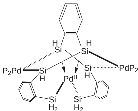
Figure 2 The alternative view of bonding for the trinuclear complex shown in Figure 1.
