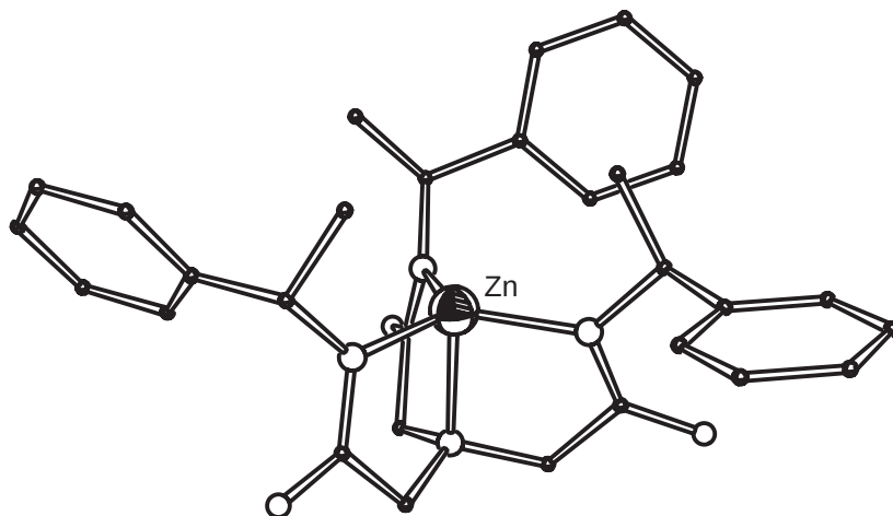
Figure 3 Molecular structure of the trigonal-monopyramidal zinc complex formed on deprotonation of tris( N -( S )-(–)-(α)-methylbenzylcarbomoylmethyl)amine. 243
