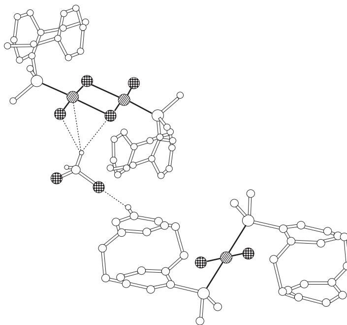
Figure 18 trans -[Pd{PPh 2 (C 16 H 15 ) 2 Cl 2 ] and [Pd{PPh 2 (C 16 H 15 ) 2 Cl 2 ] 2 .
