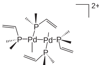
Figure 101 The cation [\{\text{Pd}[\mu\text{-Ph}_2(\text{CH})\text{CH}_2]\}[\text{PPh}_2(\text{CH})\text{CH}_2]\}_2^{2+} .
