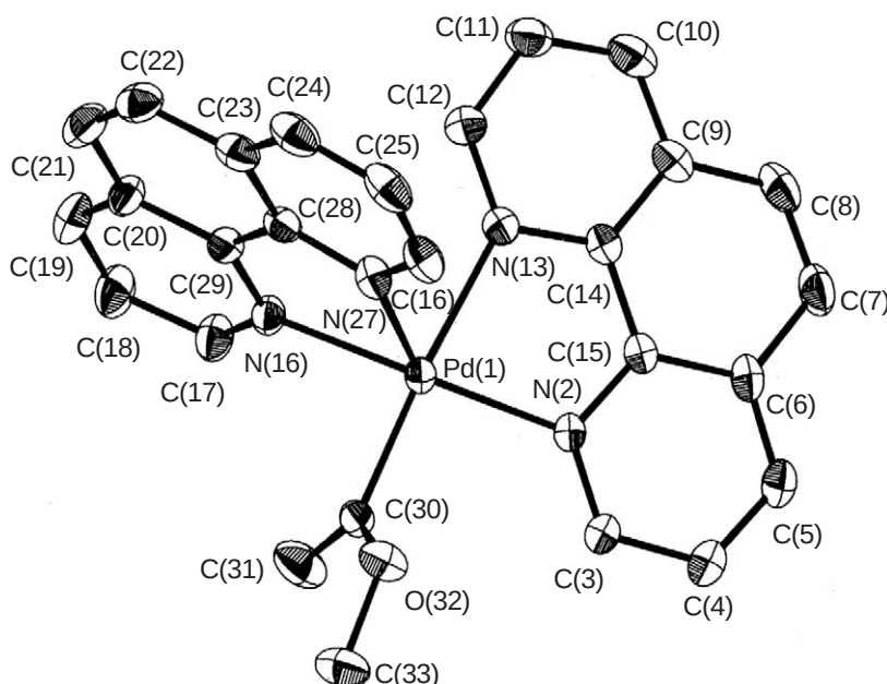
Figure 37 Structure of the five-coordinate complex [\text{Pd}(\text{phen})_2(\text{CO}_2\text{CH}_3)](\text{PF}_6) .
