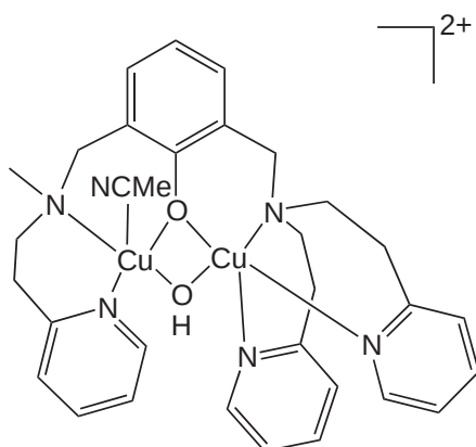
[(\text{L})\text{Cu}_2(\text{OH})(\text{MeCN})][\text{PF}_6]_2 ( 175 )
