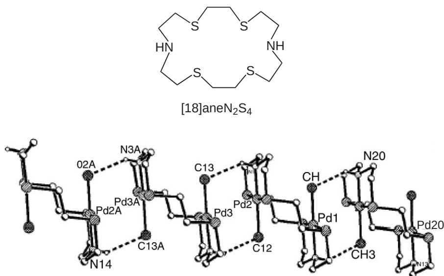
Figure 33 The two coordination planes lie parallel to each other but the overall binuclear dication adopts a stepped conformation in order to minimize steric interactions.
