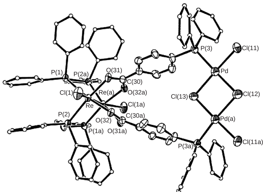
Figure 44 Structure of cis - \text{Re}_2(\mu\text{-O}_2\text{CC}_6\text{H}_4\text{-4-PPH}_2)_2\text{Cl}_2(\mu\text{-dppm})_2(\text{Pd}_2\text{Cl}_4) .
