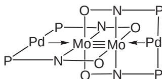
Figure 110 Tetrametal complex \text{Mo}_2\text{Pd}_2(\text{pyphos})_4 .
