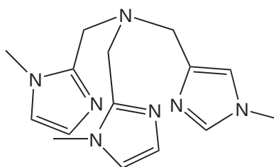
[(\text{L})\text{CuCl}][\text{PF}_6] (41)
