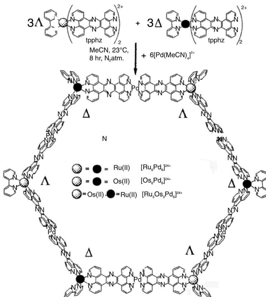
Figure 69 The molecular hexagons \text{Ru}_6\text{Pd}_6 , \text{Os}_6\text{Pd}_6 , and \text{Ru}_3\text{Os}_3\text{Pd}_6 .
