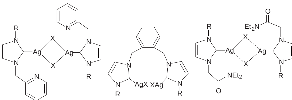
Figure 4 C-imidazolsilver compounds.
