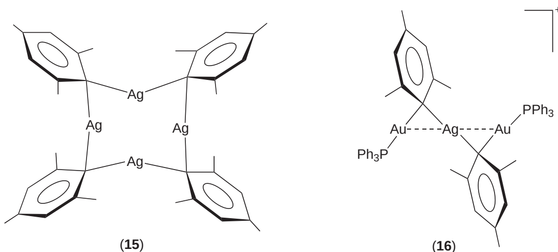
Figure 4 C-imidazolsilver compounds.
