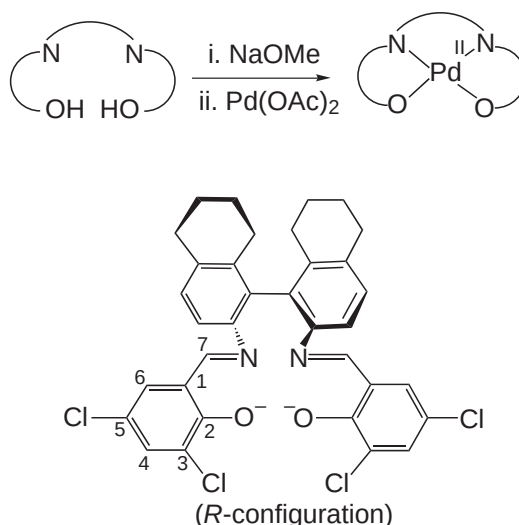
Figure 31 A Pd^{II} complex with a partially hydrogenated ligand acts as a catalyst for asymmetric epoxidation.
