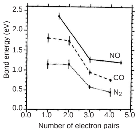
Figure 34 Trend in bond energies for loss of a ligand from [\text{Ni}(\text{CO})_x]^+ ( x = 1-4 ), [\text{Ni}(\text{N}_2)_x]^+ ( x = 1-4 ), and [\text{Ni}(\text{NO})_x]^+ ( x = 1-3 ) (reprinted with permission from ref. 2409; © 1995, American Chemical Society).
