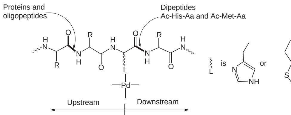
Figure 34 Palladium(II) complexes act with different regioselectivity in cleaving dipeptides and proteins.
