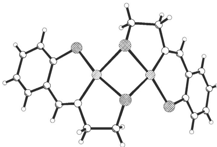
Figure 15 Molecular structure of [\text{Ni}(\text{L}^2)]_2 ( \text{HBu}^t\text{L}^2 = (515) ).
