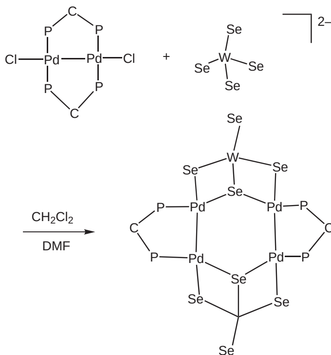
Figure 96 Preparation of neutral heterohexanuclear cluster [(\mu_3\text{-WSe}_4)_2(\text{Pd}_2)_2(\mu\text{-dppm})_2]\cdot 2\text{DMF} .
