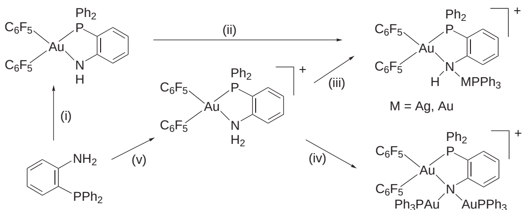
Scheme 22 (i) [Au(C 6 F 5 ) 2 (ACAC)], (ii) [Ag(OCIO 3 )(PPh 3 )], (iv) 2 [Au(ACAC)(PPh 3 )], (v) [Au(C 6 F 5 ) 2 (OEt) 2 ]ClO 4 .
