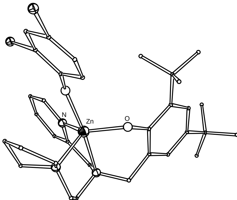
Figure 15 The molecular structure of the zinc complex formed with the unsymmetric tripod, (2-picolyl) ( N -pyrrolidinylethyl)(2-hydroxy-3,5-di- t -butylbenzyl)amine and 2,4-dibromophenoxide. 877
