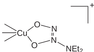
[(i\text{-Pr}_3\text{TACN})\text{Cu}\{\text{Et}_2\text{N}(\text{N}_2\text{O}_2)\}][\text{CF}_3\text{SO}_3] ( 500 )
