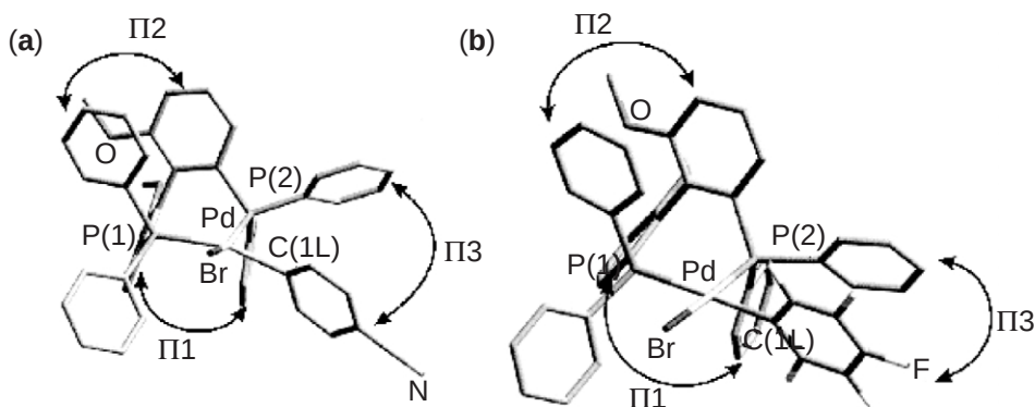
Figure 4 Chiral Pd complexes (a) \text{PdBr}(p\text{-CNC}_6\text{H}_4)(\text{S})\text{-MeO-Biphep} ; (b) \text{PdBr}(\text{C}_6\text{F}_5)(\text{S})\text{-MeO-Biphep} . Potential aromatic \pi - \pi stacking interactions are indicated by arrows.
