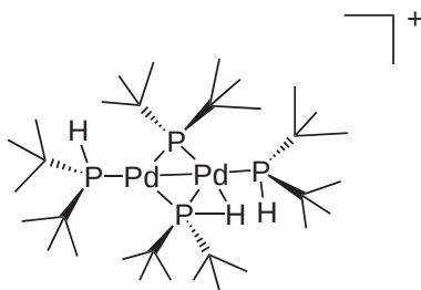
Figure 100 The structure of the complex [\text{Pd}_2(\mu\text{-P}^t\text{Bu}_2)(\mu\text{-P}^t\text{Bu}_2\text{H})(\text{P}^t\text{Bu}_2\text{H})_2]\text{BF}_4 , which contains a secondary phosphine as bridging ligand.
