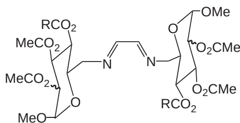
Figure 102 Chelating ligand that is derived from \alpha -D-MANOSE.
