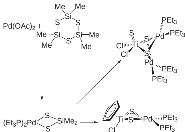
Figure 26 Synthesis of a palladium dimethylsilanedithiolato complex and its cluster forming reactions with (C_5H_5)TiCl_3 and TiCl_4(THF)_2 .
