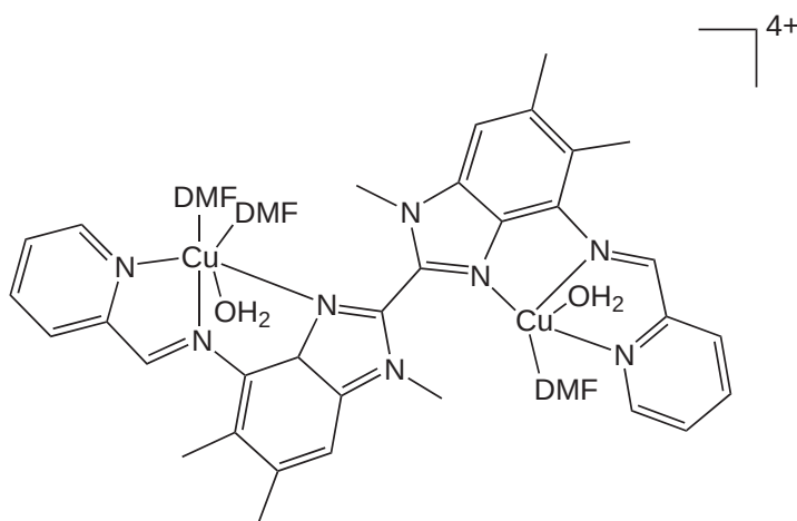
[(L)Cu_2(DMF)_3(H_2O)_2][CF_3SO_3]_4 ( 96 )
