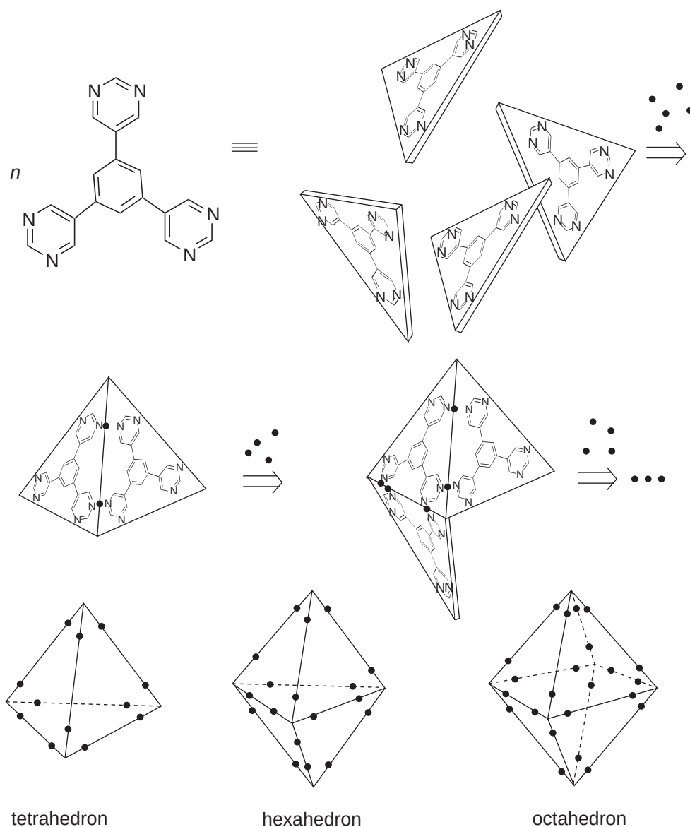
Figure 79 Assembly of a polyhedron achieved by complexation of 1,3,5-tris(3,5-pyrimidyl)benzene with \text{Pd(en)}^{2+} groups.
