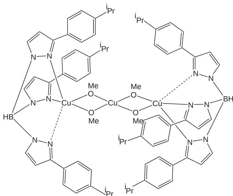
[\{(L)Cu(OMe)_2\}_2Cu] ( 331b )
