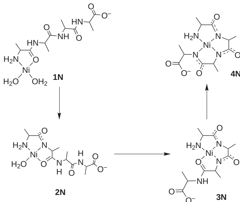
Scheme 8
