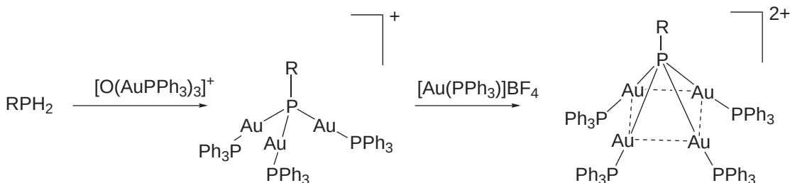
Scheme 34
