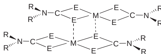
Figure 24 Dimeric structure of dialkyldichalcogenocarbamate compounds [M(E_2CNRR')_2] ( M = \text{Zn, Cd} ; E = \text{S, Se} ).
