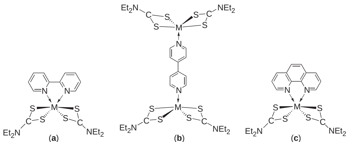
Figure 26 Structures of (a) [M(S_2CNEt_2)_2(2,2'\text{-bipy})] ( M = \text{Cd}, \text{Zn} ); (b) [\{M(S_2CNEt_2)_2\}_2(\mu\text{-}4,4'\text{-bipy})] ; (c) [M(S_2CNEt_2)(\text{phen})] ( M = \text{Cd}, \text{Zn} ).
