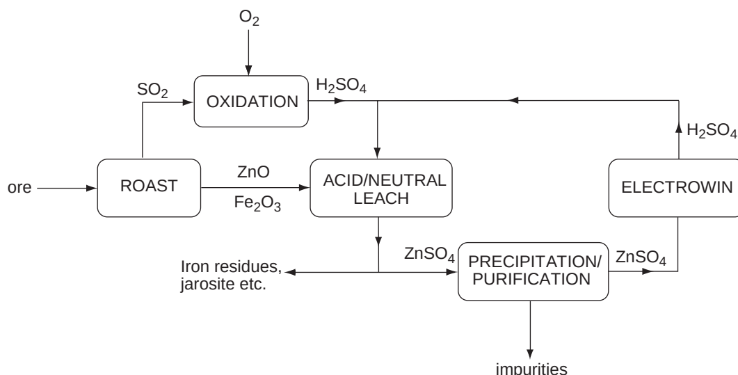
Figure 7 An outline of the flowsheet for zinc production by the conventional roast/neutral-leach/electrowinning circuit.
