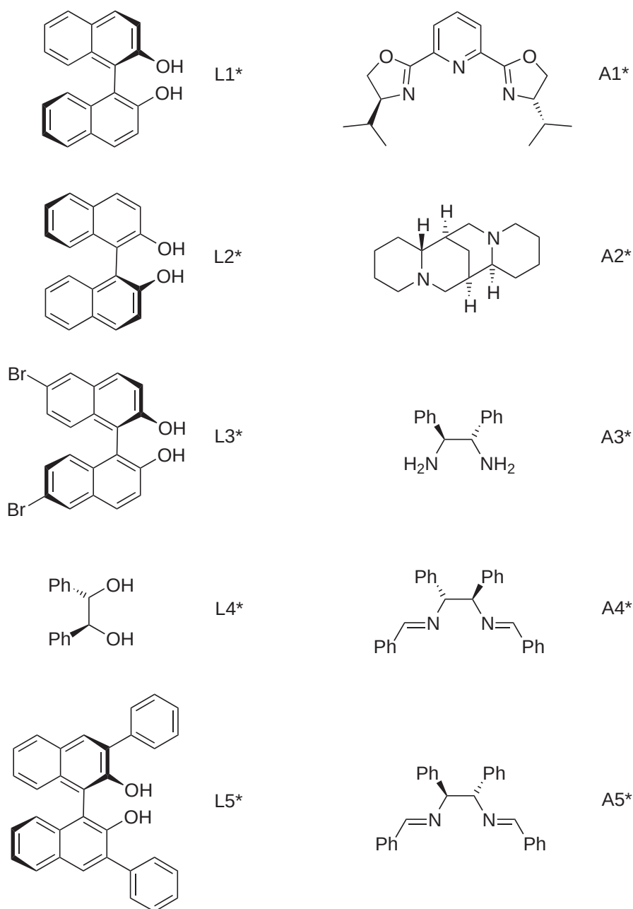
Scheme 12
