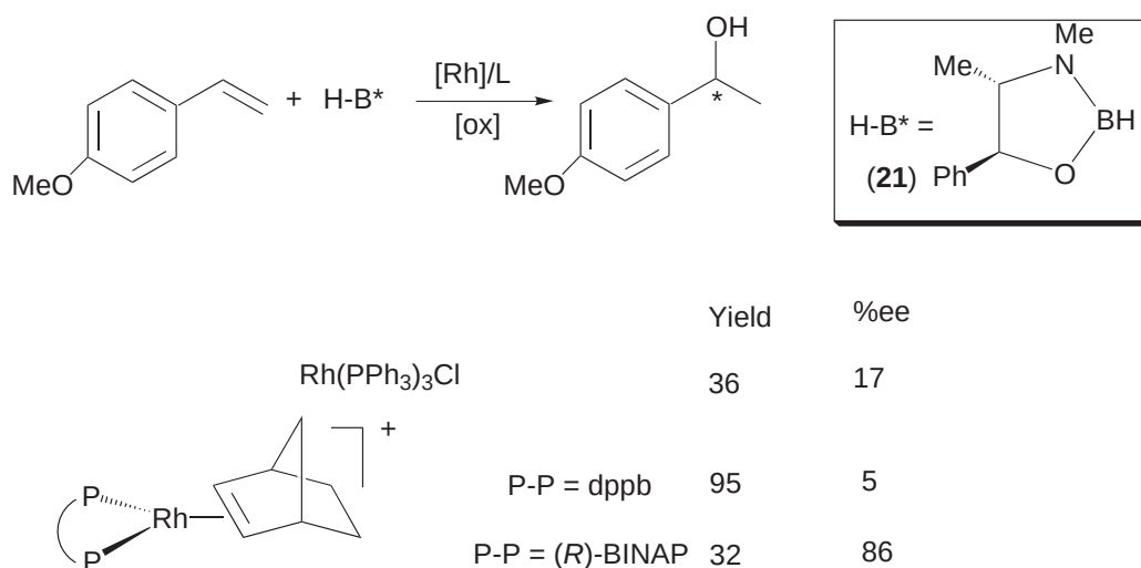
Scheme 13
