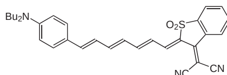
(2): \lambda_{\text{max}} = 826 \text{ nm} , \beta_0[\text{EFISHG}_{1907}] = 1,470 \cdot 10^{-30} \text{ esu} (\text{CHCl}_3)^{59}
