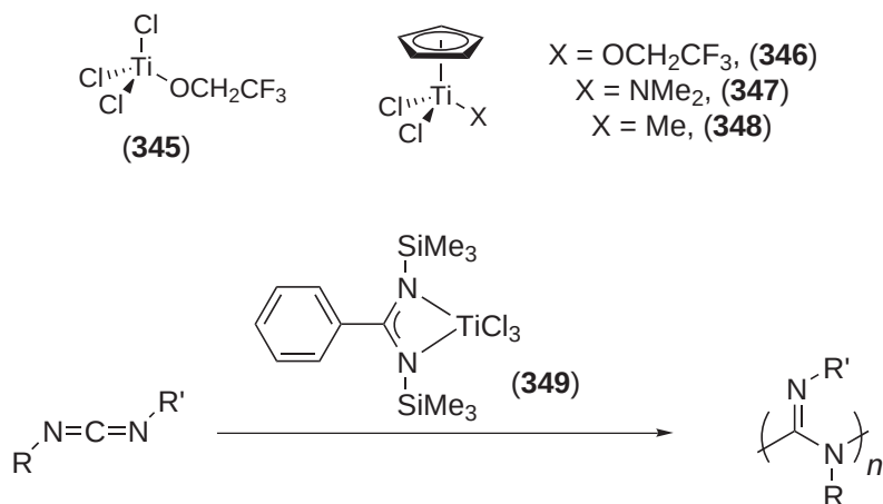
Scheme 29
