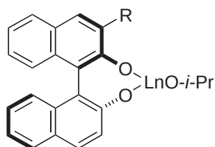
Scheme 24
