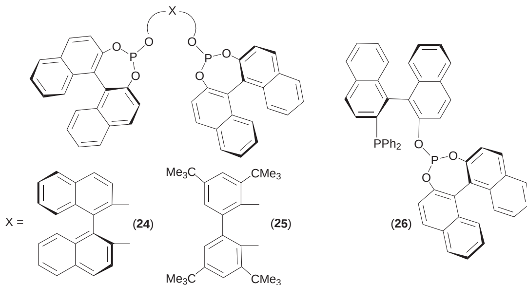
Scheme 14
