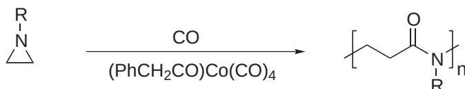
Scheme 26
