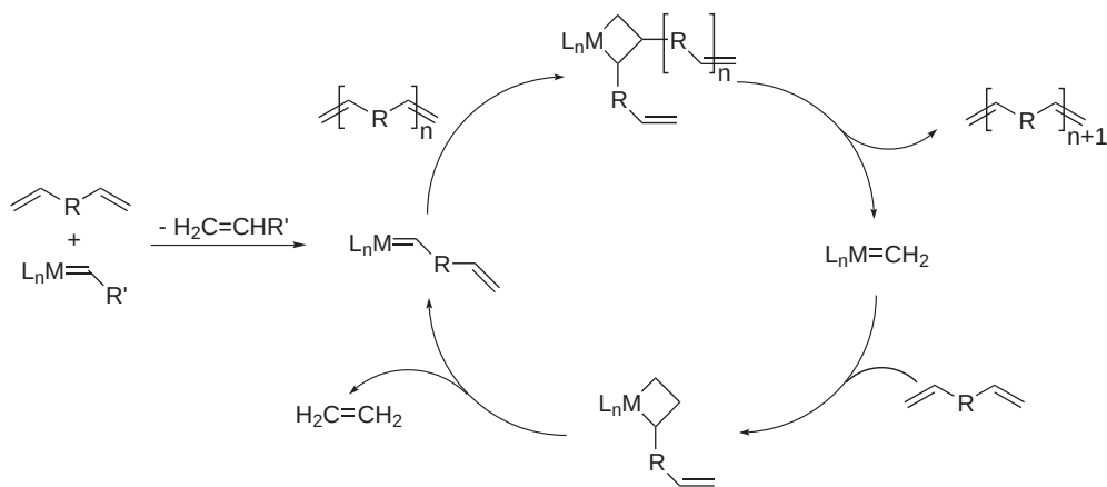
Scheme 13
