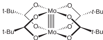
(241): \gamma [\text{DFWM}] = 1.3 \cdot 10^{-32} \text{ esu (CH}_2\text{Cl}_2) 641
