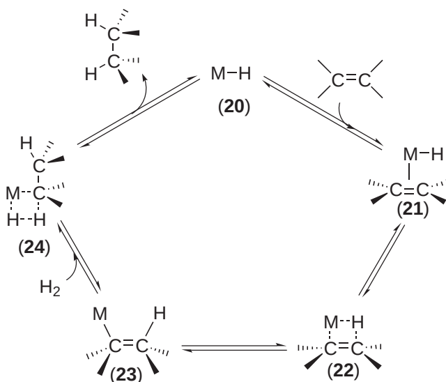
Scheme 7
