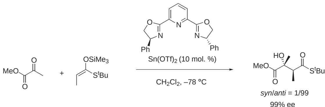
Scheme 81
