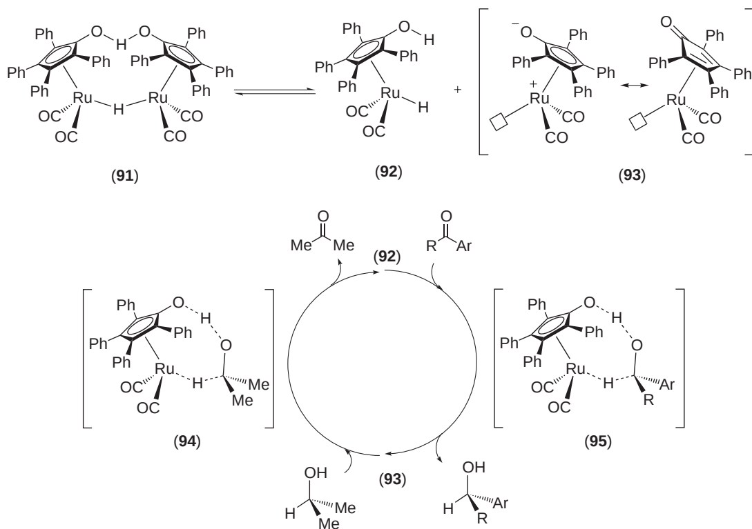
Scheme 30
