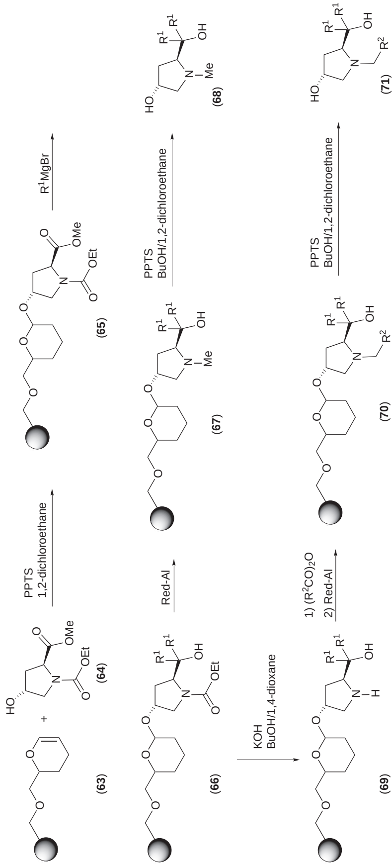
Scheme 17
