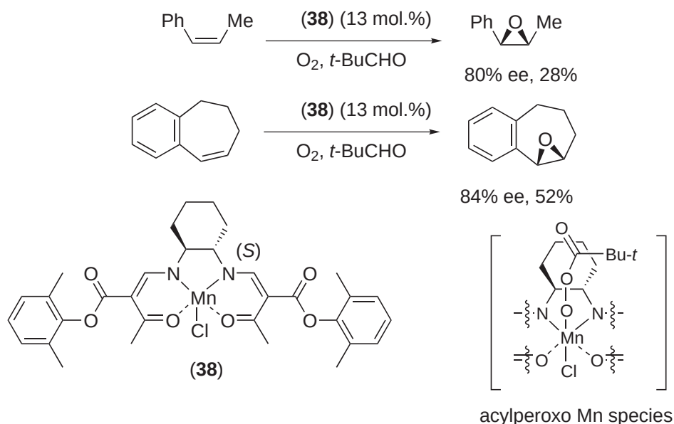
Scheme 22
