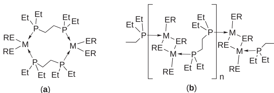
Figure 29 Structures of (a) molecular 1:1 and (b) polymeric 2:1 \text{M}(\text{ER})_2 :depe adducts ( M = \text{Zn}, \text{Cd}, \text{Hg} ; E = \text{S}, \text{Se}, \text{Te} ; R = \text{Ph}, \text{Bu}^t ).
