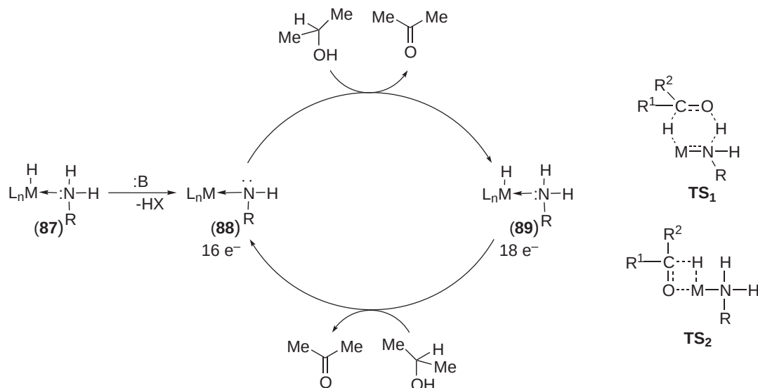
Scheme 28
