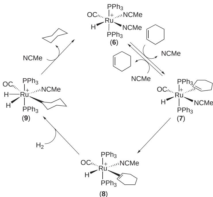
Scheme 4
