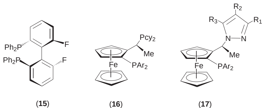
Scheme 11
