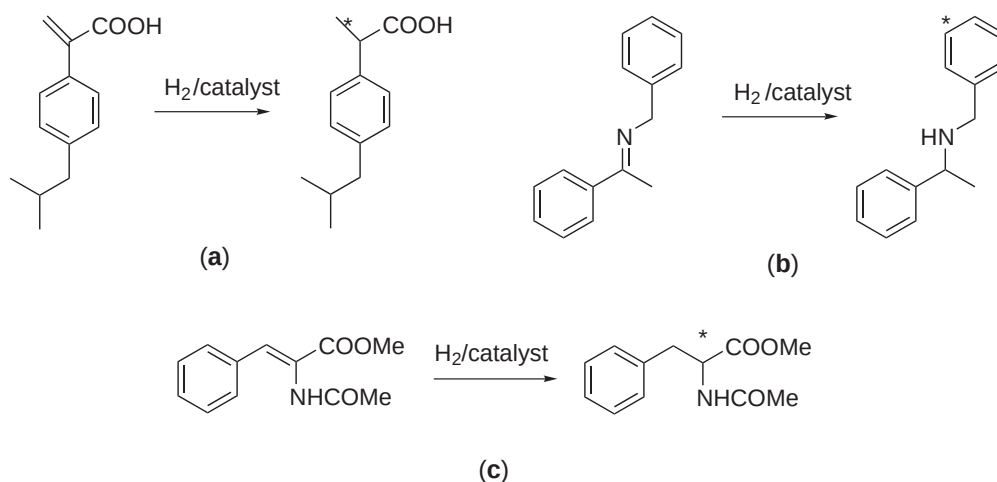
Scheme 62
