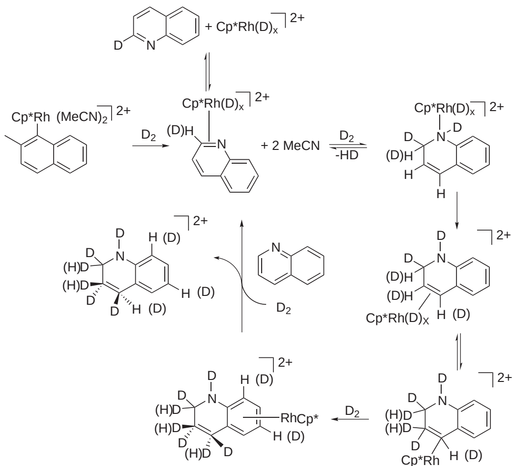
Scheme 52
