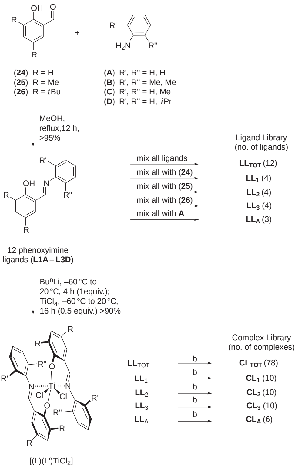
Scheme 5
