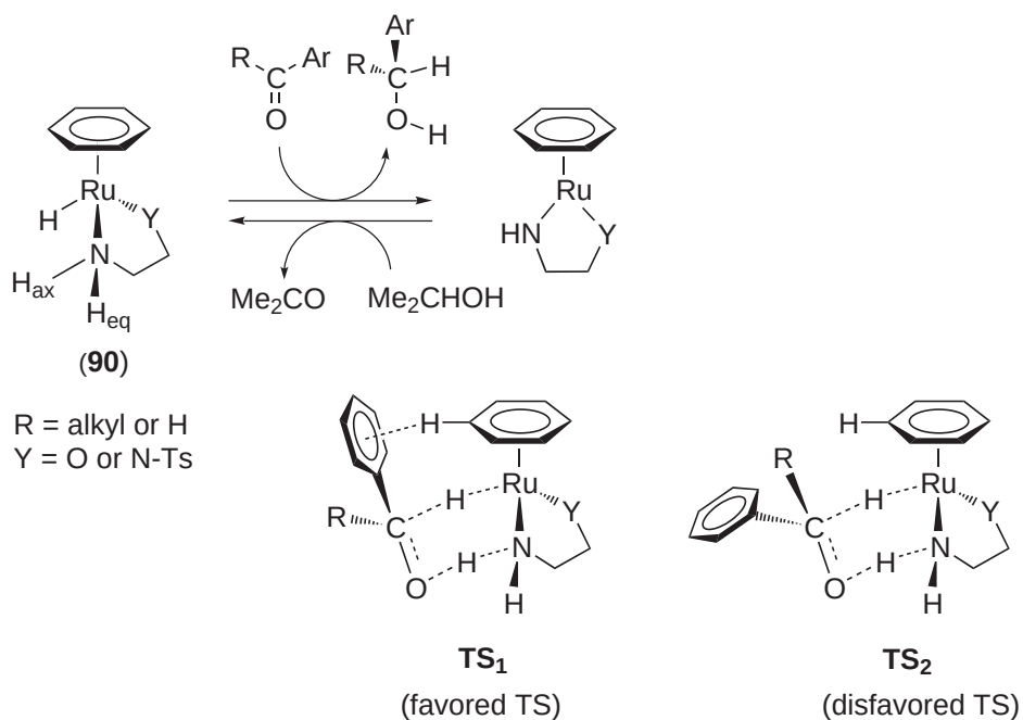
Scheme 29
