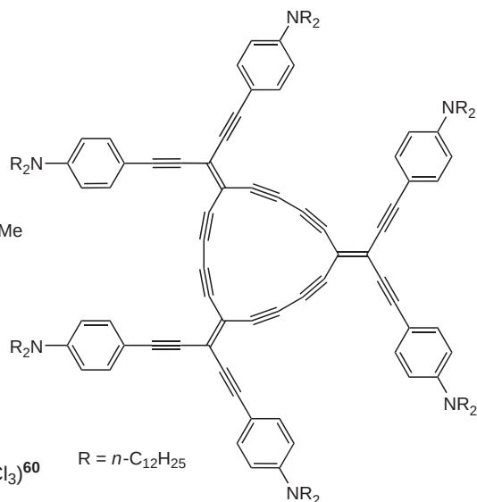
(4): \gamma[\text{THG}_{2100}] = 4.3 \cdot 10^{-32} \text{ esu} , \chi^{(3)} = 7.6 \cdot 10^{-11} \text{ esu} (\text{CHCl}_3)^{26}
