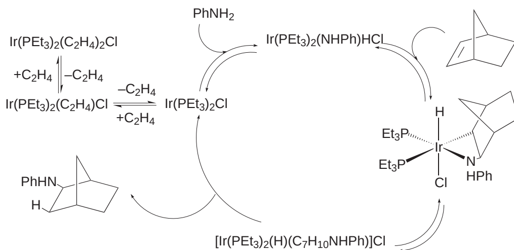
Scheme 39
