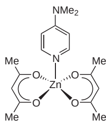
(205) : \text{SHG}_{1064} = \text{ca. } 1 \cdot \text{urea} , \beta_0[\text{AM1/TDHF}] = 4.4 \cdot 10^{-30} esu 567
