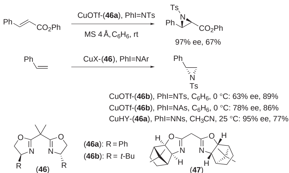
Scheme 34
