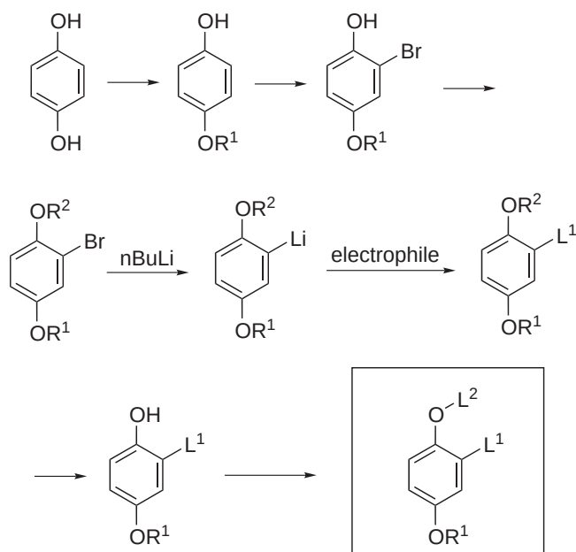
Scheme 8
