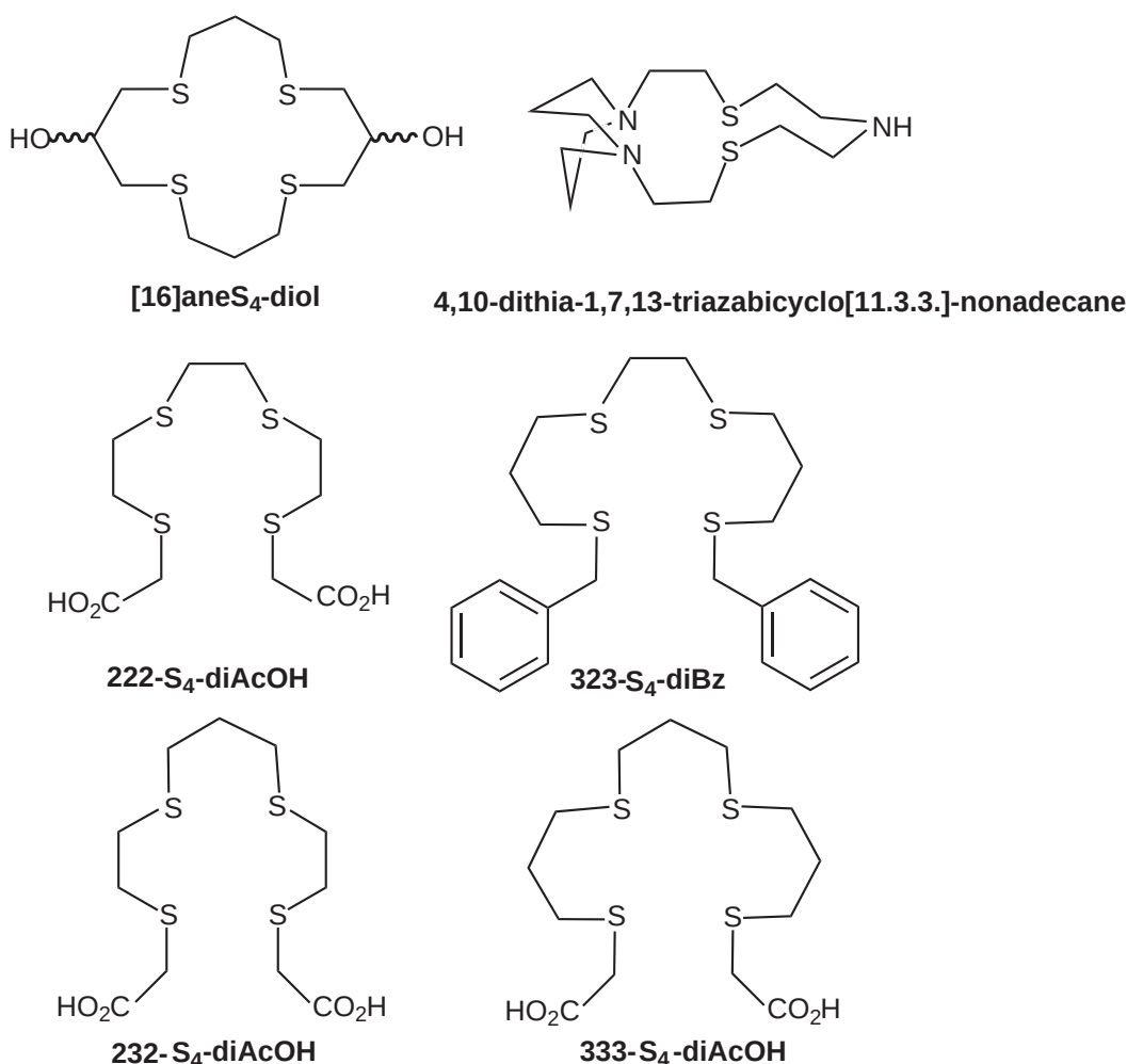
Figure 11 Ligands for \text{Rh}^{\text{III}} .
