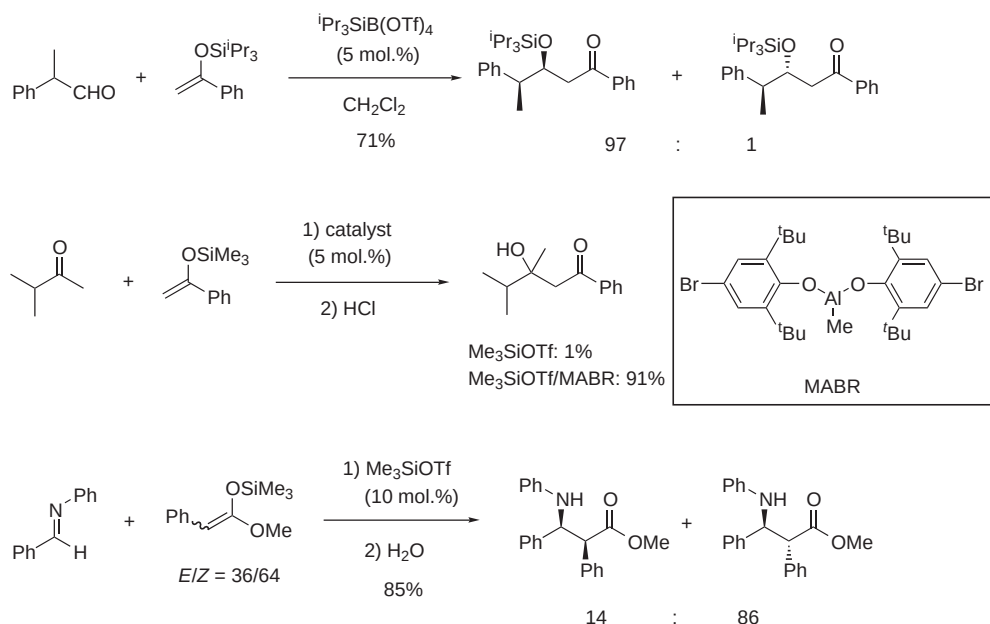
Scheme 74
