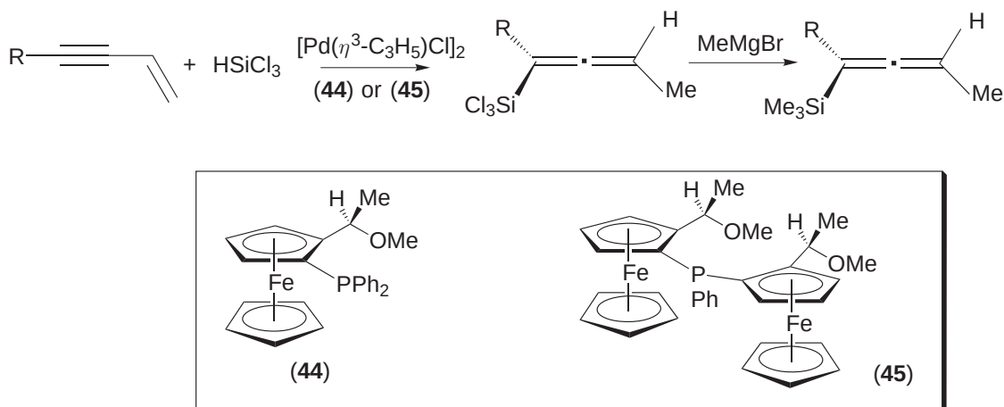
Scheme 27
