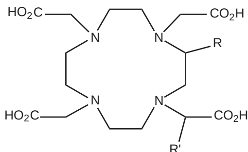
Figure 4 NOTA analogues.
