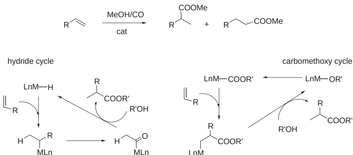
Scheme 11
