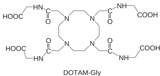
Scheme 19
