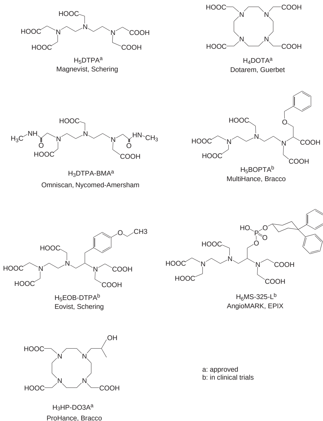
Scheme 1
