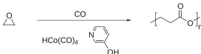
Scheme 24
