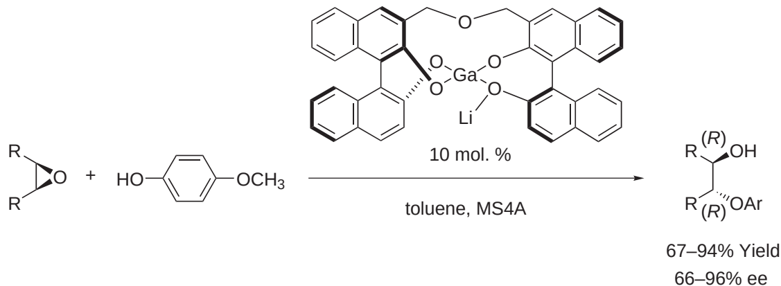
Scheme 84
