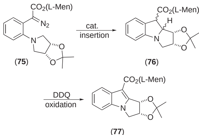
Scheme 19
