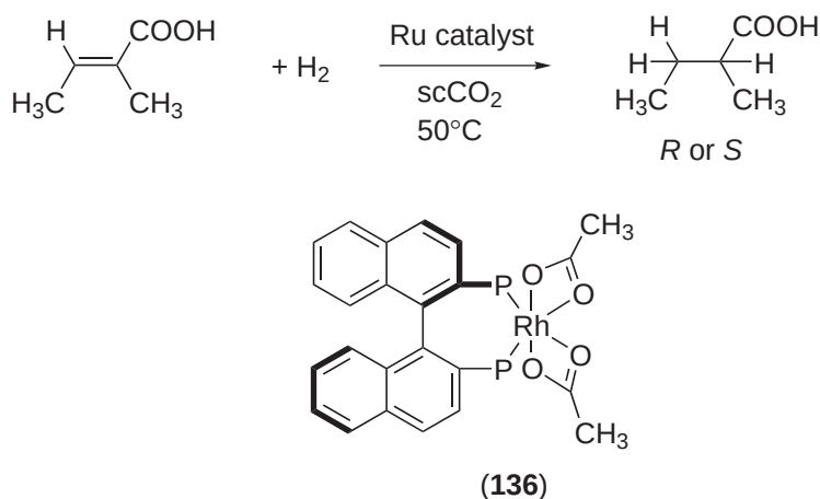
Scheme 68
