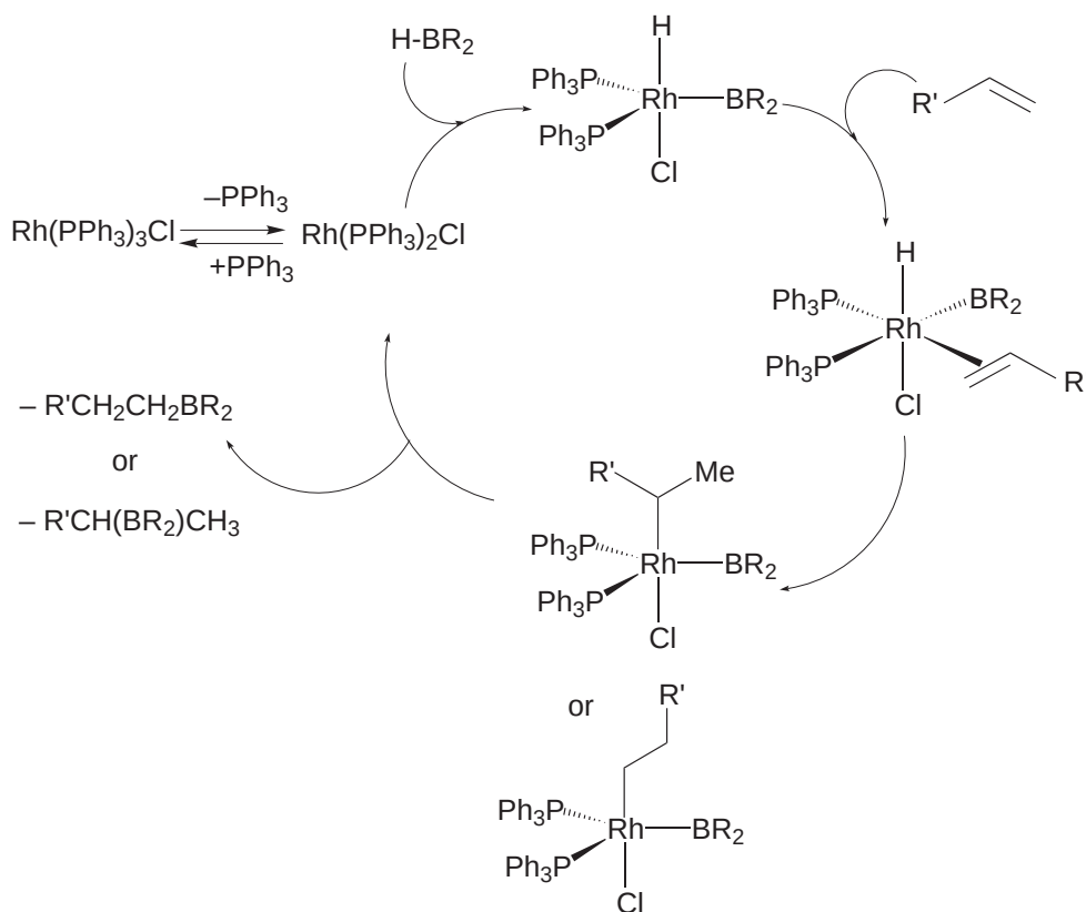
Scheme 3
