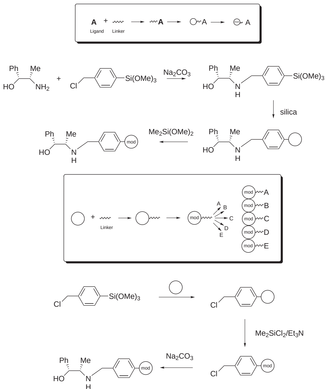
Scheme 58
