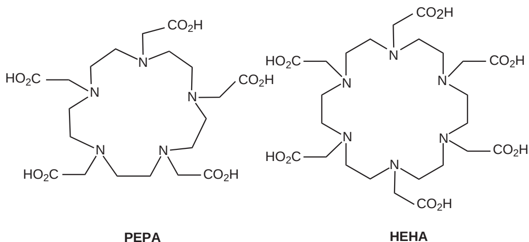
Figure 13 Macrocyclic polyaminocarboxylate ligands for Ac III .
