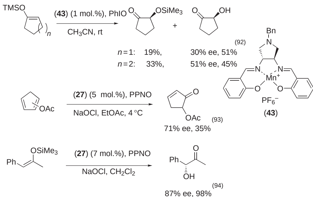
Scheme 28
