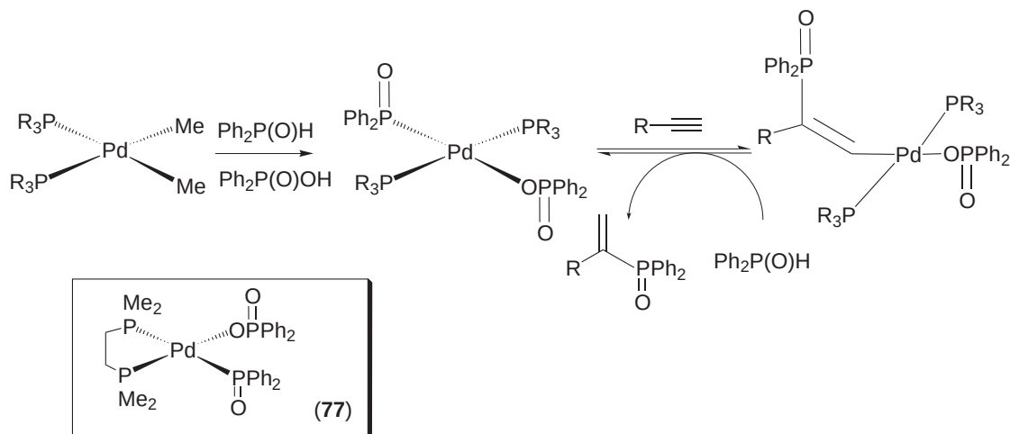
Scheme 47
