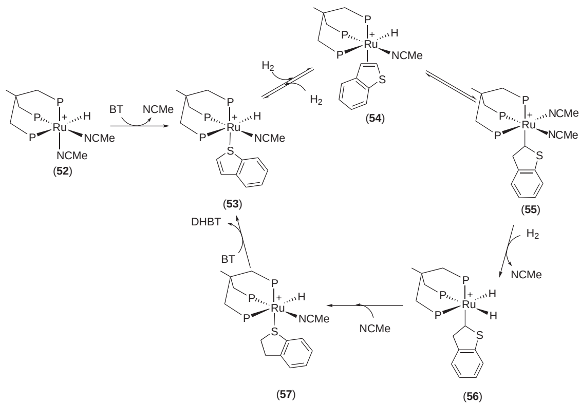
Scheme 14
