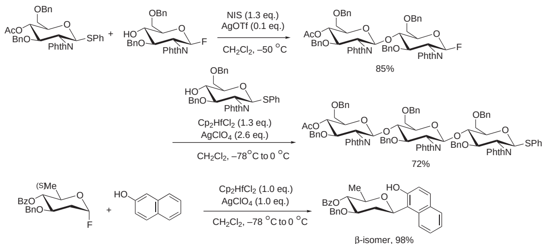
Scheme 41
