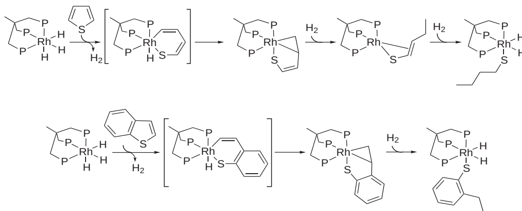
Scheme 39
