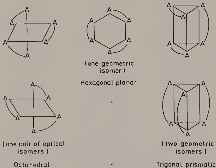
Fig. 7. Predicted isomers for compound type M(\overline{AA})_3 .
