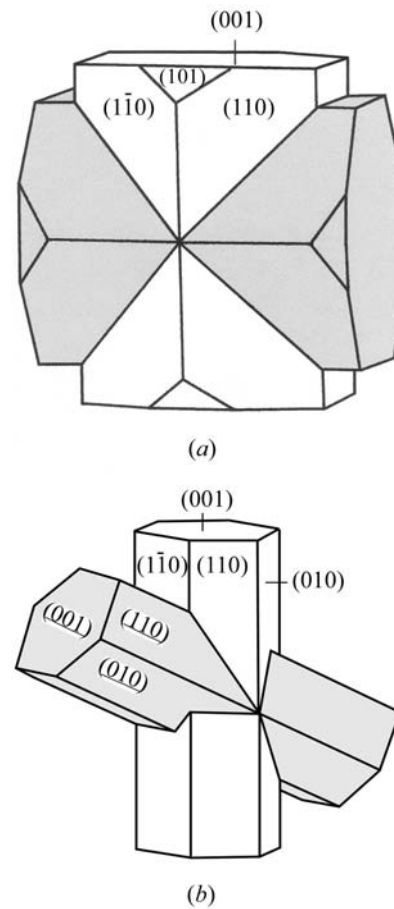
Fig. 3.3.6.13. Twinning of staurolite. (a) 90^\circ cross ('Greek cross') with twin reflection and composition planes (031) and (031̄). (b) 60^\circ cross ('St Andrew's cross') with twin reflection and composition plane (231).
