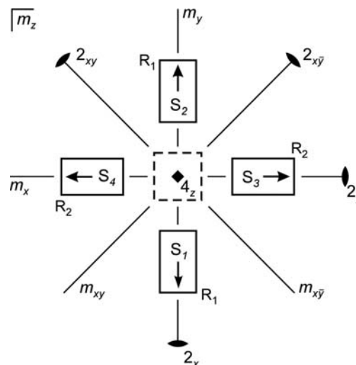
Fig. 3.4.2.2. Exploded view of single-domain states \mathbf{S}_1 , \mathbf{S}_2 , \mathbf{S}_3 and \mathbf{S}_4 (solid rectangles with arrows of spontaneous polarization) formed at a phase transition from a parent phase with symmetry G = 4_z/m_z m_x m_{xy} to a ferroic phase with symmetry F_1 = 2_x m_z m_y . The parent phase is represented by a dashed square in the centre with the symmetry elements of the parent group G = 4_z/m_z m_x m_{xy} shown.
