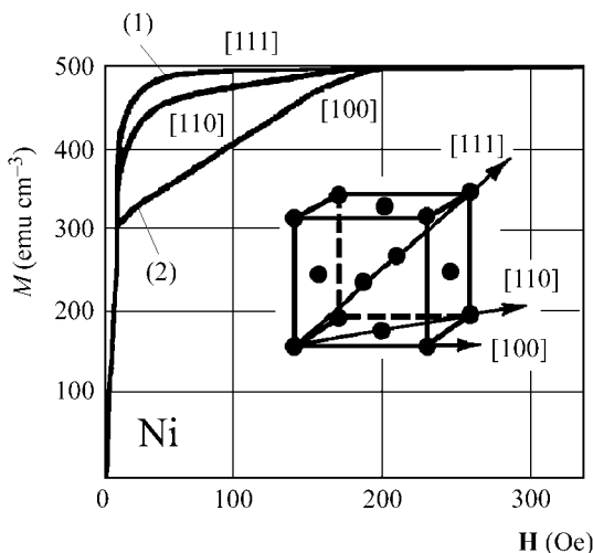
Fig. 1.5.4.2. Magnetization curves of two cubic crystals (iron and nickel) for three crystallographic directions.
