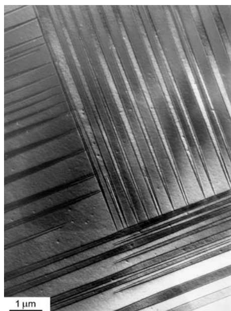
Fig. 3.4.1.4. Transmission electron microscopy image of the ferroelastic domain structure in a \text{YBa}_2\text{Cu}_3\text{O}_{7-y} crystal (Rosová, 1999). Courtesy of A. Rosová, Institute of Electrical Engineering, SAS, Bratislava. There are two systems ('complexes'), each of which is formed by almost parallel ferroelastic domain walls with needle-like tips. The domain walls in one complex are nearly perpendicular to the domain walls in the other complex.
