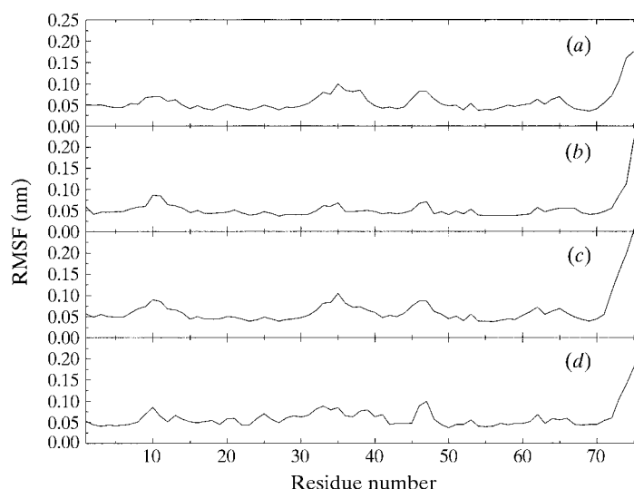
Fig. 20.1.3.6. Root-mean-square C\alpha -atom-position fluctuations (RMSFs) in nm are shown for molecule 4, with full translational and rotational fitting over the C\alpha atoms of residues 1–72. Different averaging periods are compared. (a) shows the RMSFs for the period 400–800 ps, (b) shows those for the period 800–1200 ps. In (c), the results for the previous two periods are averaged (400–1200 ps), and in (d), the results for the period 1200–2000 ps are shown.
