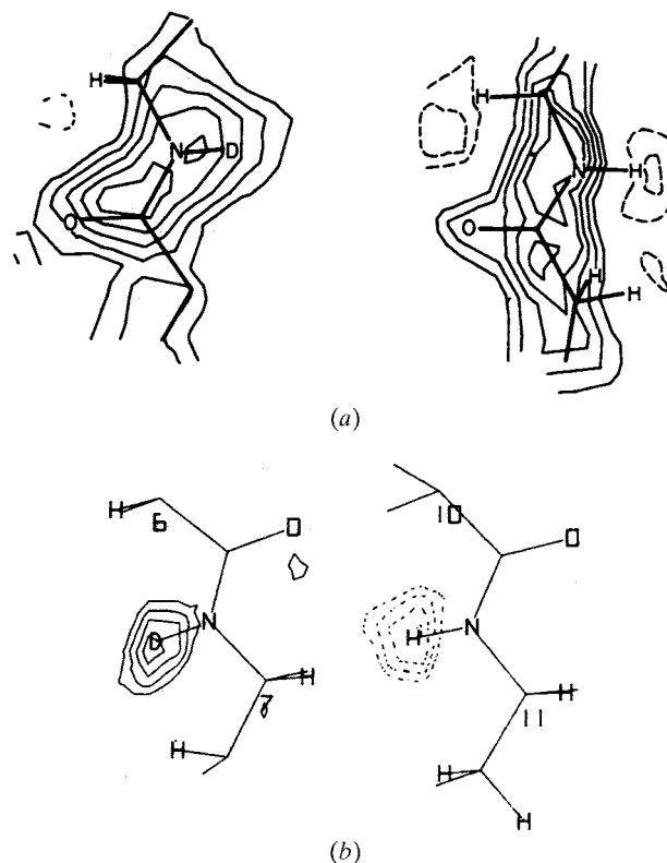
Fig. 19.1.8.1. Sections of neutron density maps taken in the plane of the peptide group. (a) 2F_o - F_c maps showing an example of an exchanged and unexchanged amide peptide group. (b) \text{D}_2\text{O} – \text{H}_2\text{O} difference density map showing the same.
