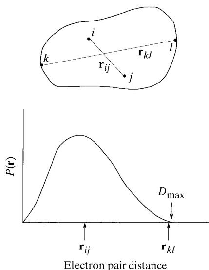
Fig. 19.3.3.4. Definition of the electron pair distance distribution function P(r) . It is a histogram of all electron pair distances within a particle as depicted here. The largest dimension of the molecule D_{\max} is determined from the point where P(r) falls to zero.
