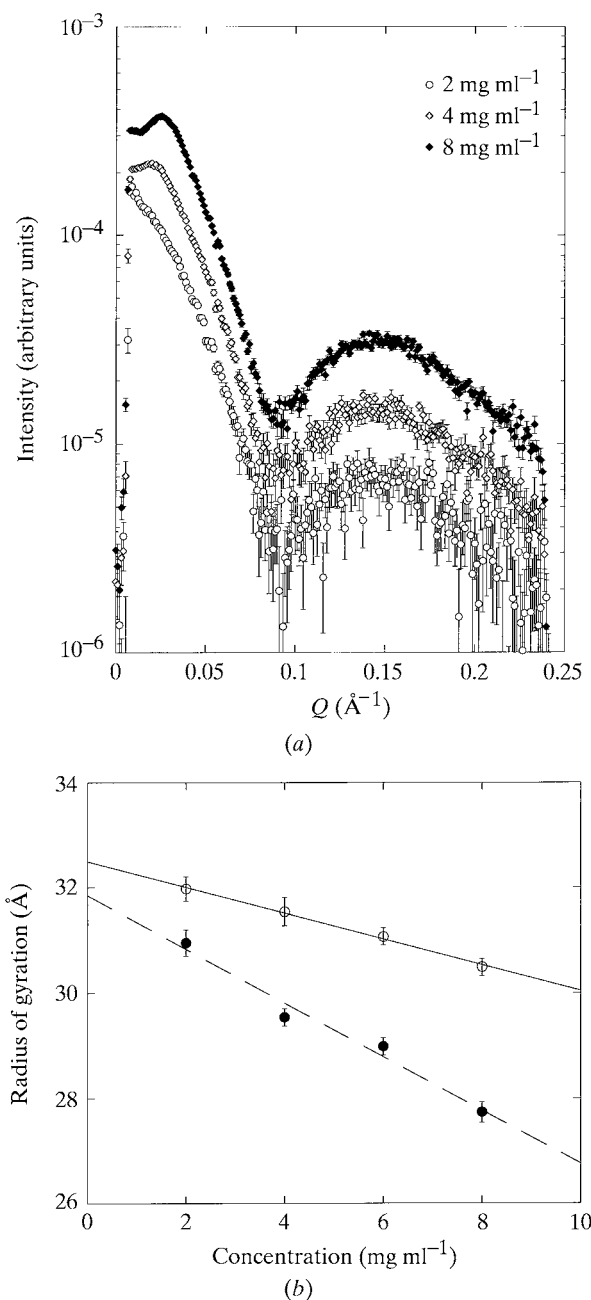
Fig. 19.3.3.3. (a). Interparticle interference in biological small-angle scattering. Scattering from myelin P0 glycoprotein solubilized in 0.1% SDS, recorded at 2, 4 and 8 mg ml -1 (Inouye et al. , 1999). (b) Plots of measured radii of gyration of E. coli aspartate transcarbamoylase catalytic trimer versus concentration in the absence (open circles) and presence (filled circles) of the bisubstrate analogue N -phosphonacetyl-L-aspartate (E. R. Johnson, H. Tsuruta & H. K. Schachman, unpublished data).
