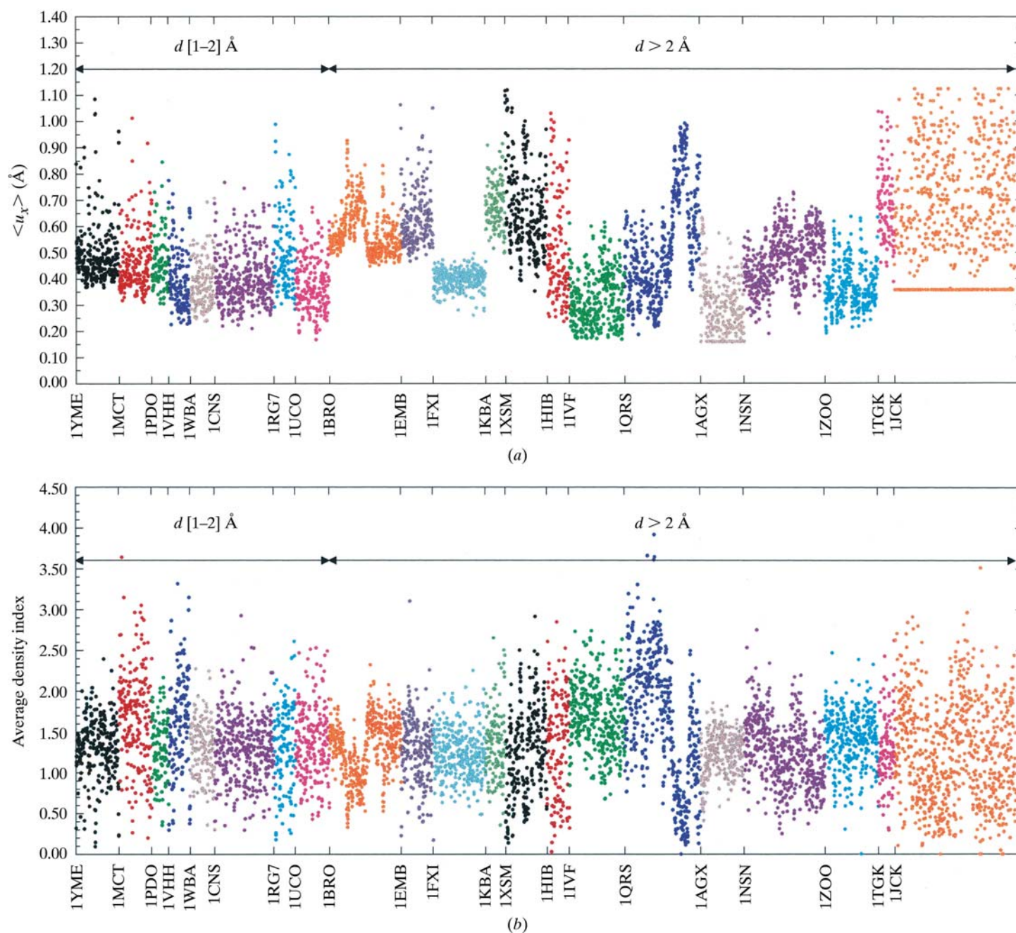
Fig. 21.2.3.6. B factors and density indices for residues across different structures. (a) Average B values in residues of 21 protein structures; (b) average density indices of the same set of residues and structures. The 21 protein structures analysed are from the following PDB entries: 1YME, 1MCT, 1PDO, 1VHH, 1WBA, 1CNS, 1RG7, 1UCO, 1BRO, 1EMB, 1FXI, 1KBA, 1XSM, 1HIB, 1IVF, 1QRS, 1AGX, 1NSN, 1ZOO, 1TGK, 1JCK.
