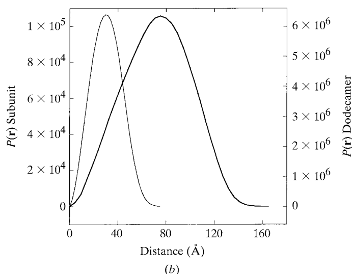
Fig. 19.3.3.2. (a) The calculated solution X-ray scattering curves from the crystal structure of Salmonella typhimurium glutamine synthetase. Glutamine synthetase is composed of 12 identical 469-residue subunits and forms a functional dodecameric assembly (PDB entry 2GLS; Yamashita et al. , 1989). The single subunit was computationally isolated, and the solution scattering curves for the subunit (thin line) and the assembled form (thick line) were calculated with a 3 Å-thick hydration layer of 0.03 \text{ e } \text{\AA}^{-3} using CRY SOL (Svergun et al. , 1995). The curves are normalized to an identical weight concentration, that is, the number concentration of the dodecamer is 1/12 of that of the subunit, giving a 12-fold increase in I(Q=0) . The inset shows Guinier plots of the calculated scattering curves. The radii of gyration determined by the Guinier plot to Q \simeq 1.0/R_g (solid-line fit) for the subunit and the assembled form are 24.1 and 55.8 Å, respectively. The 'extended' Guinier plots to Q \simeq 2.0/R_g (circles) give 23.9 and 56.5 Å. Note that both Guinier plots are quite linear beyond Q \simeq 2.0/R_g , although the Guinier approximation is theoretically valid to Q \simeq 1.0/R_g . It should be noted, however, that the 'extended' Guinier plot tends to give significantly smaller R_g for elongated shapes. (b) The electron distance distribution functions. The pair distribution functions P(\mathbf{r}) were calculated from the scattering curves in (a) using GNOM (Svergun, 1992). The maximum intramolecular distance is 75 and 160 Å for the subunit and the assembled enzyme, respectively. The P(\mathbf{r}) gives the radius of gyration as 23.6 Å for the subunit and 55.0 Å for the assembled enzyme.
