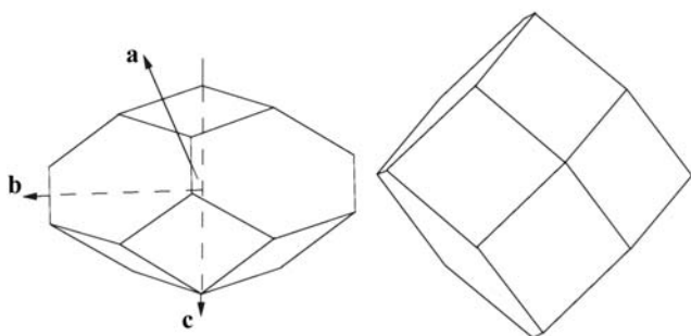
Fig. 26.1.2.1. Tetragonal lysozyme crystals with well developed \{110\} faces (left-hand crystal) and small \{110\} faces (right-hand crystal).
