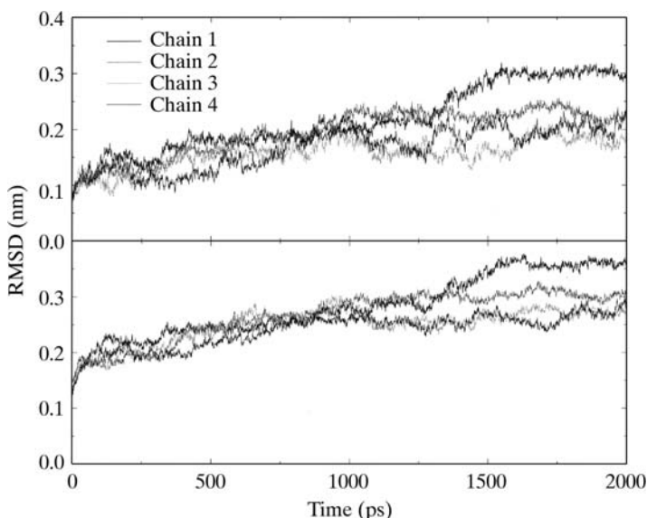
Fig. 20.1.3.2. Root-mean-square atom-positional deviations (RMSD) in nm from the X-ray structure of the four different protein molecules in the unit cell as a function of time. Rotational and translational fitting was applied using the \text{C}\alpha atoms of residues 1–72. The upper and lower graphs show the deviations for the \text{C}\alpha atoms and for all atoms, respectively.
