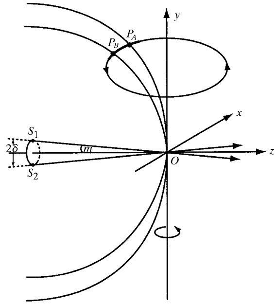
Fig. A11.5.1.1. Penetration of a reciprocal-lattice point P into the sphere of reflection by rotation around Oy. The extremes of reflecting conditions at P_A and P_B are equivalent to X-rays passing along the lines S_1O and S_2O with centres of the Ewald spheres at S_1 and S_2 and subtending an angle of 2m at O . Hence, in three dimensions, the extreme reflecting spheres will lie with their centres on a circle of radius \delta = m/\lambda at z = -1/\lambda .
