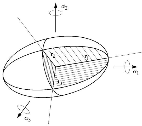
Fig. 18.4.1.1. The thermal-ellipsoid model used to represent anisotropic atomic displacement, with major axes indicated. The ellipsoid is drawn with a specified probability of finding an atom inside its contour. Six parameters are necessary to describe the ellipsoid: three represent the dimensions of the major axes and three the orientation of these axes. These six parameters are expressed in terms of a symmetric U tensor and contribute to atomic scattering through the term \exp[-2\pi^2(U_{11}h^2a^{*2} + U_{22}k^2b^{*2} + U_{33}l^2c^{*2} + 2U_{12}hka^*b^* \cos \gamma^* + 2U_{13}hla^*c^* \cos \beta^* + 2U_{23}klb^*c^* \cos \alpha^*)] .
