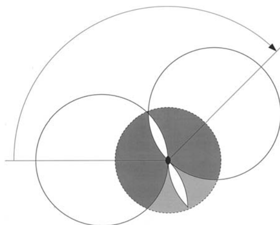
Fig. 9.1.7.2. Rotation of a triclinic crystal by 135^\circ is not sufficient to obtain totally complete data. At high resolution the completeness is higher than at low resolution, where a full 180^\circ rotation is required.
