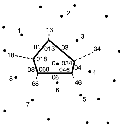
Fig. 22.1.1.2. Labelling parts of Voronoi polyhedra. The central atom is atom 0, and each neighbouring atom has a sequential index number (1, 2, 3, . . .). Consequently, in three dimensions, planes are denoted by the indices of the two atoms that form them (e.g. 01); lines are denoted by the indices of three atoms (e.g. 012); and vertices are denoted by four indices (e.g. 0123). In the 2D representation shown here, lines are denoted by two indices, and vertices by three. From a collection of points, a volume can be calculated by a variety of approaches: First of all, the volume of a tetrahedron determined by four points can be calculated by placing one vertex at the origin and evaluating the determinant formed from the remaining three vertices. (The tetrahedron volume is one-sixth of the determinant value.) The determinant can be quickly calculated by a vector triple product, \mathbf{w} \cdot (\mathbf{u} \times \mathbf{v}) , where \mathbf{u} , \mathbf{v} and \mathbf{w} are vectors between the vertex selected to be the origin and the other three vertices of the tetrahedron. Alternatively, the volume of the pyramid from a central atom to a face can be calculated from the usual formula Ad/3 , where A is the area of the face and d is the distance to the face.
