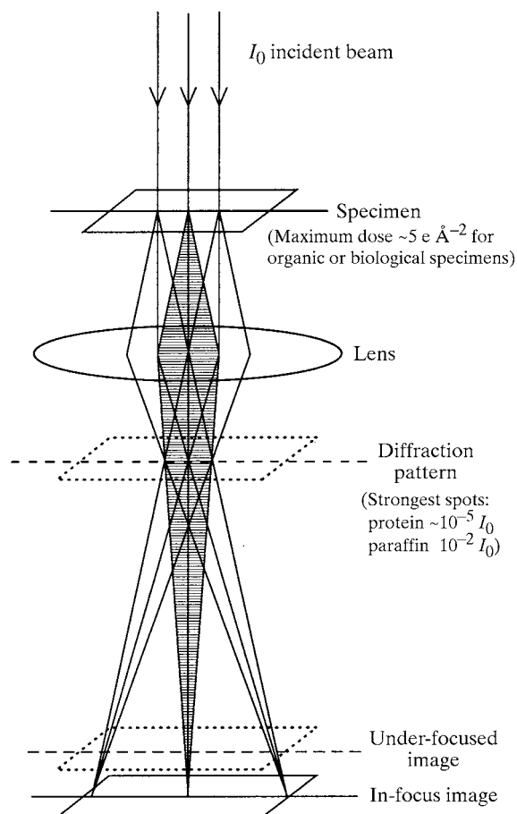
Fig. 19.6.2.1. Schematic diagram showing the principle of image formation and diffraction in the transmission electron microscope. The incident beam, I_0 , illuminates the specimen. Scattered and unscattered electrons are collected by the objective lens and focused back to form first an electron-diffraction pattern and then an image. For a 2D or 3D crystal, the electron-diffraction pattern would show a lattice of spots, each of whose intensity is a small fraction of that of the incident beam. In practice, an in-focus image has virtually no contrast, so images are recorded with the objective lens slightly defocused to take advantage of the out-of-focus phase-contrast mechanism.
