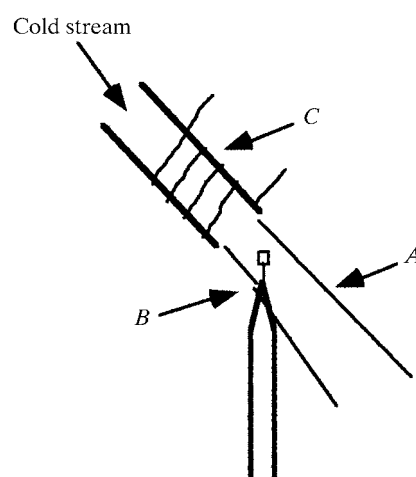
Fig. 10.1.4.4. Schematic drawing of a single-stream setup with the stream angled relative to the diffractometer \varphi axis. A represents the outline of the cold stream. At B the crystal mounting pin protrudes 1–2 mm into the cold stream. This prevents frost from forming on the mounting fibre. The tip of the outlet end is heated above the dew point with a heating coil C. The cold stream misses the goniometer head, so no shield is required. In general, the simplest operation is attained with a setup similar to that shown here.
