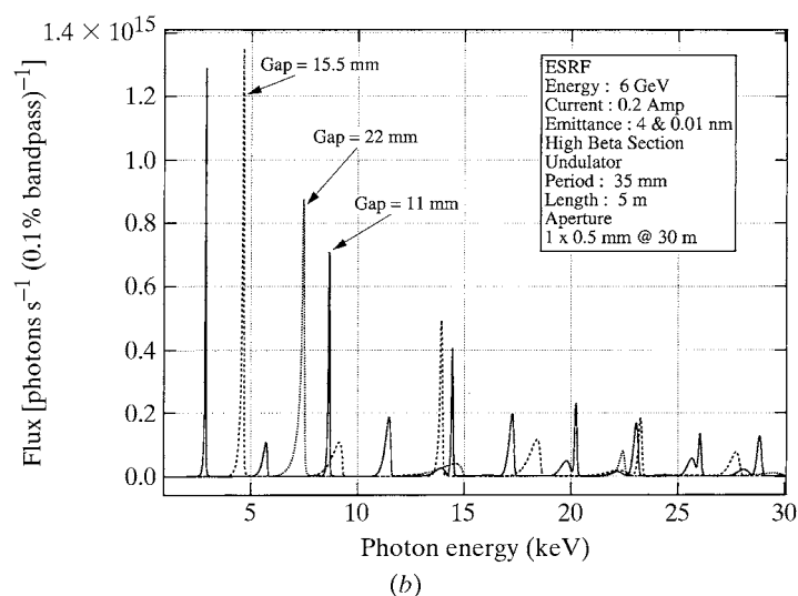
Fig. 8.1.2.4. SR spectra. (a) Brilliances of different SR source types (undulator, multipole wiggler and bending magnet) as exemplified by such sources at the ESRF. For the undulator, the tuning range ( i.e. as the magnet gap is changed) is indicated. (b) Undulator-emitted spectra at the ESRF, shown as photon fluxes through a 1 \times 0.5 mm aperture at 30 m, for three different gaps, i.e. widening the gap shifts the emitted fundamental and associated harmonics in each case to higher photon energies. Kindly provided by Dr Pascal Elleaume, ESRF, Grenoble, France.
