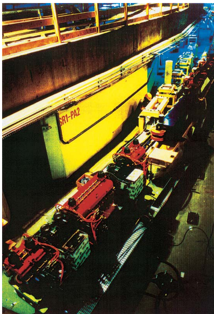
Fig. 8.1.2.3. The ring tunnel and part of the machine lattice at the ESRF, Grenoble, France.
