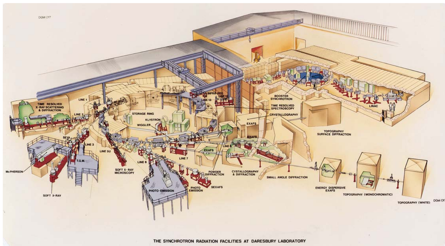
Fig. 8.1.2.2. Overall layout of the Daresbury SRS facility, including LINAC, booster synchrotron, main storage ring and experimental beamlines (as in 1985 for clarity). Reproduced with the permission of CLRC Daresbury Laboratory.
