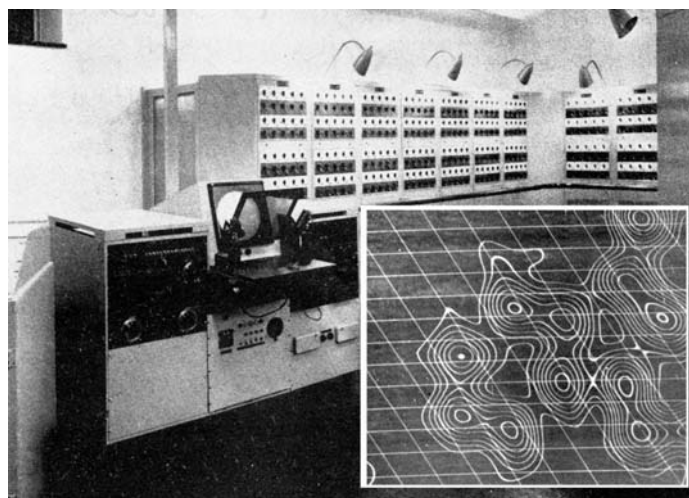
Fig. 17.2.2.1. One bay of X-RAC showing coefficient panels and the display oscilloscope. Inset: photo from the oscilloscope, showing a region of the phthalocyanine Fourier map. Reproduced from Pepinsky (1952).
