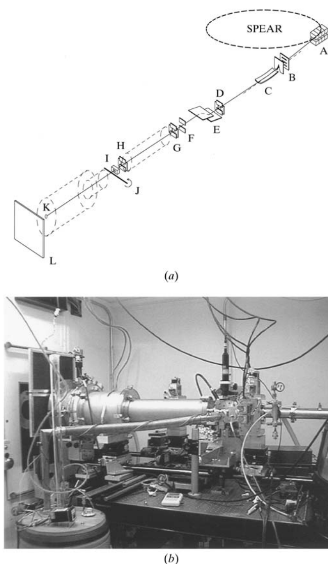
Fig. 19.3.3.5. A small-angle X-ray scattering instrument on BL 4-2 at the Stanford Synchrotron Radiation Laboratory. (a) A diagram of the instrument composed of an eight-pole wiggler source (A), mirror slits (B), toroidal focusing mirror (C), monochromator slit (D), double-crystal monochromator (E), fast beam shutter (F), beam-defining slit (G), guard slit (H), ion chamber (I), crystal spindle axis (J), which would be replaced with a solution sample cell for solution X-ray scattering, beam stop (K) and an image plate detector (L), which would be replaced with a gas-chamber detector for solution scattering. Vacuum beam flight paths are drawn in dotted lines. (b) A view of the instrument as configured for small-angle single-crystal diffraction with a crystal-to-detector distance of 1.3 m. Some of the components in (a) are also seen in (b).
