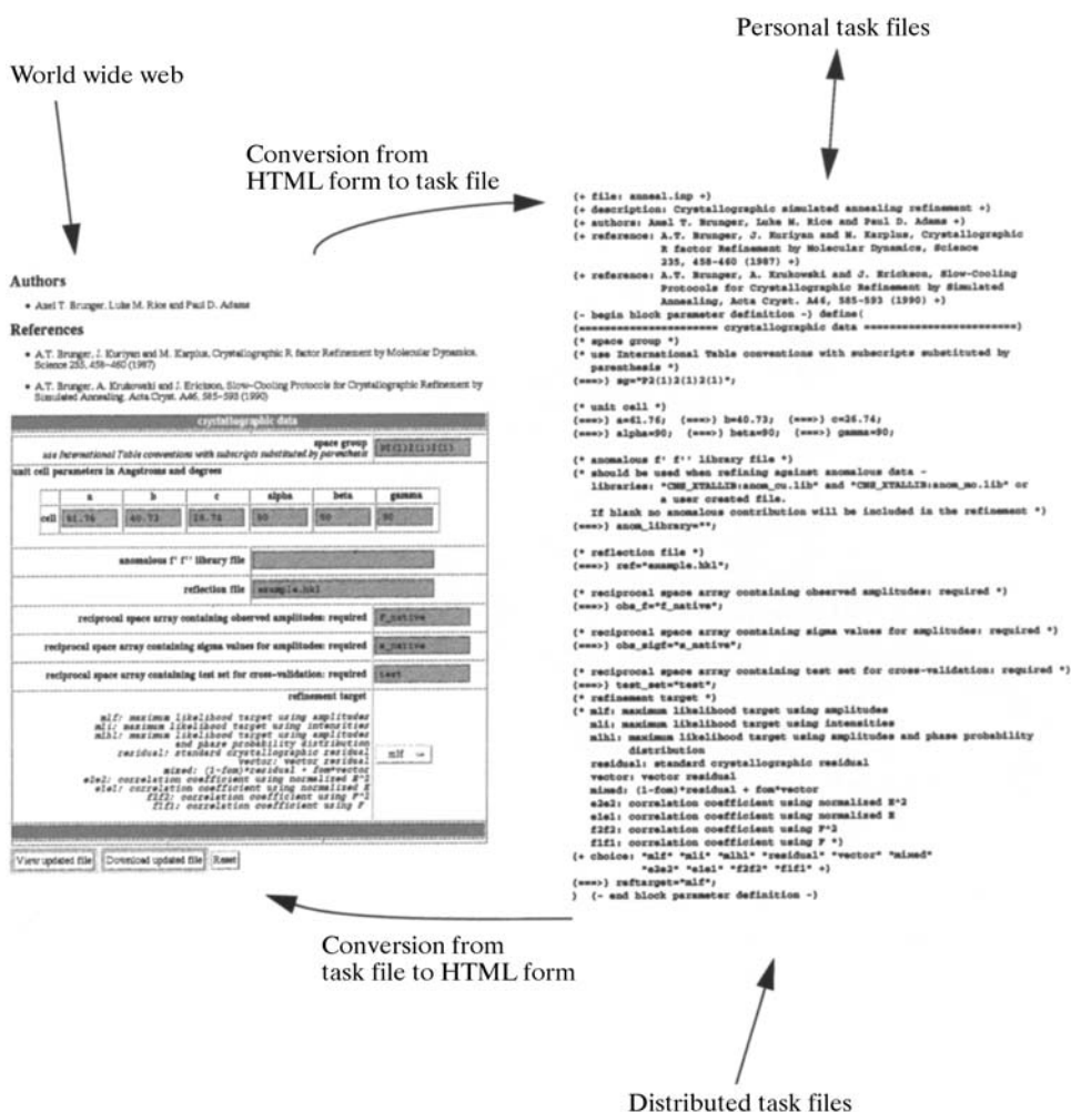
Fig. 25.2.3.10. Use of the CNS HTML form page interface, emphasizing the correspondence between input fields in the form page and parameters in the task file.
