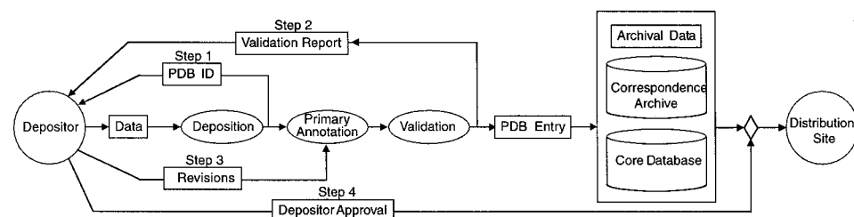
Fig. 24.5.2.1. The steps in PDB data processing. Ellipses represent actions and rectangles define content.
