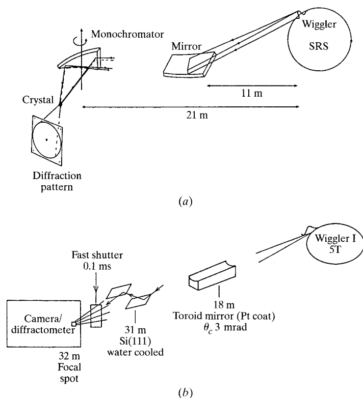
Fig. 8.1.4.1. Common beamline optics modes. (a) Horizontally focusing cylindrical monochromator and vertical focusing mirror [shown here for station 9.6 at the SRS (adapted from Helliwell et al. , 1986)]. (b) Rapidly tunable double-crystal monochromator and point-focusing toroid mirror [shown here for station 9.5 at the SRS (adapted from Brammer et al. , 1988)].
