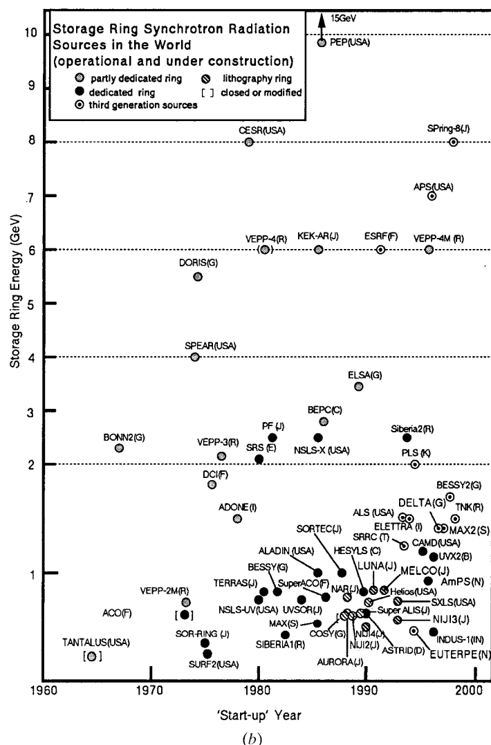
Fig. 8.1.2.1. (a) Evolution of X-ray source brilliance (photons \text{s}^{-1} \text{mrad}^{-2} \text{mm}^{-2} per 0.1% \delta\lambda/\lambda ) in the hundred years since Rontgen's discovery of X-rays in 1895. Adapted from Coppens (1992). (b) The evolution of storage-ring synchrotron-radiation sources over the decades, as illustrated by their increasing number and range of machine energies up to the present (Suller, 1998).
