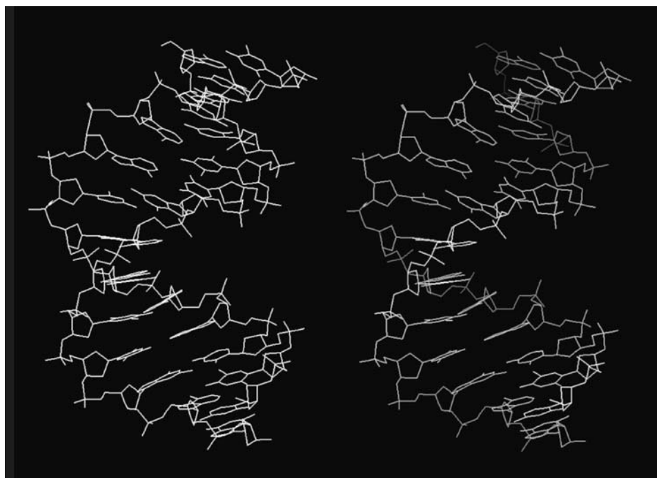
Fig. 17.2.3.3. Simple bonding diagram of a DNA structure (PDB code: 140D) (Mujeeb et al. , 1993). On the left all lines are of equal intensity. On the right the lines are depth-cued to show which parts of the structure are closer to the viewer.
