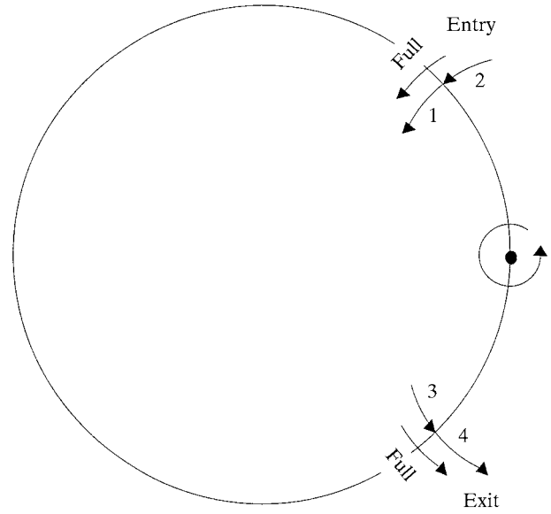
Fig. A11.5.1.3. The four conditions 1, 2, 3 and 4 for partial reflections corresponding to Table A11.5.1.1. The arrow ends and heads correspond to the start and end positions of a reciprocal-lattice point, respectively.
