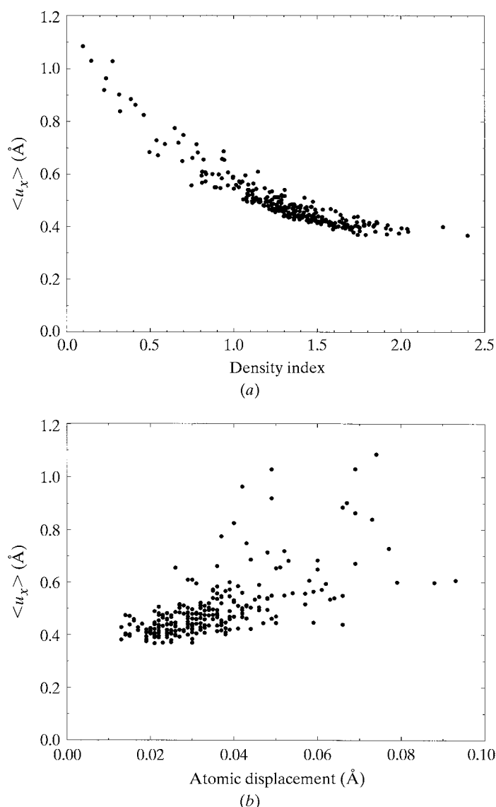
Fig. 21.2.3.5. Pairwise correlations between the various local quality indicators computed by SFCHECK . (a) Correlation between the average residue B factor and the density index, and (b) between the B factor and the atomic displacement. The values displayed were computed for residues in the crystal structure of carboxypeptidase (1YME). The meaning of the parameters displayed is given in Table 21.2.3.3.
