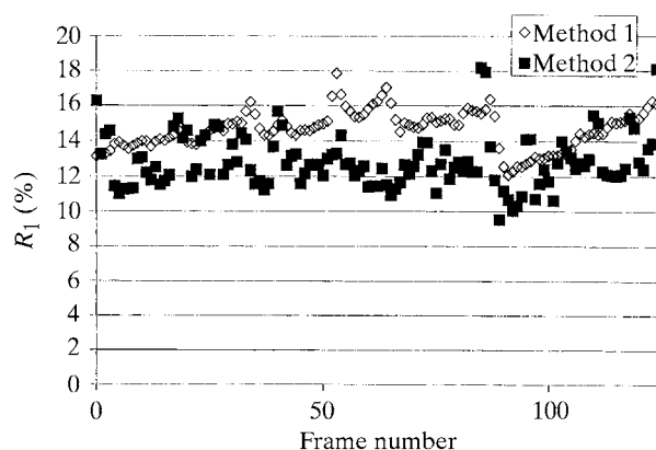
Fig. 11.5.7.5. R factor per frame as a function of frame number for a \varphi X174 data set (Dokland et al. , 1997).
