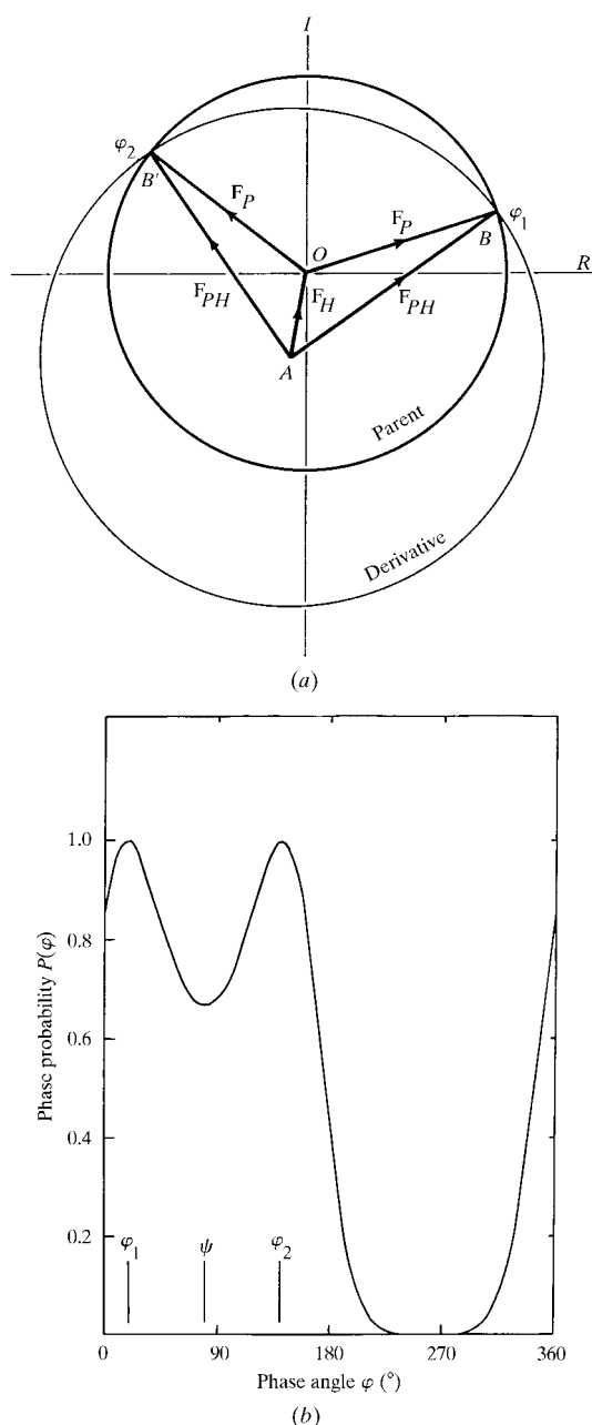
Fig. 14.1.2.1. (a) Harker construction for a single isomorphous replacement. \varphi_1 and \varphi_2 are the 'most probable' phases for \mathbf{F}_P . (b) Phase probability distribution for a single isomorphous replacement. This and subsequent probabilities are unnormalized. [All figures in this chapter are reproduced with permission from Matthews (1970). Copyright (1970) International Union of Crystallography.]
