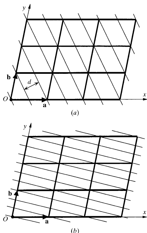
Fig. 2.1.1.3. A two-dimensional lattice with 3 \times 3 unit cells. In both (a) and (b), a set of equidistant parallel lattice planes is drawn. They pass through all lattice points. Lattice planes always divide the unit-cell axes into a whole number of equal parts – 1, 2, 3 etc. For instance, in (a), the vector a of the unit cell is cut into two parts, and the vector b into only one part. This set of planes is then given the indices h = 2 and k = 1 . In three dimensions, there would be a third index, l . In (b), the set of lattice planes has the indices h = 1 and k = 3 . In general, lattice planes have the indices (hkl) , known as Miller indices. If a set of lattice planes is parallel to an axis, the corresponding index is 0. For instance, (001) is the set of planes parallel to the unit-cell vectors a and b . Note that the projection of a/h on the line normal to the lattice plane is equal to the lattice-plane distance d . This is also true for b/k . Reproduced with permission from Drenth (1999). Copyright (1999) Springer-Verlag.
