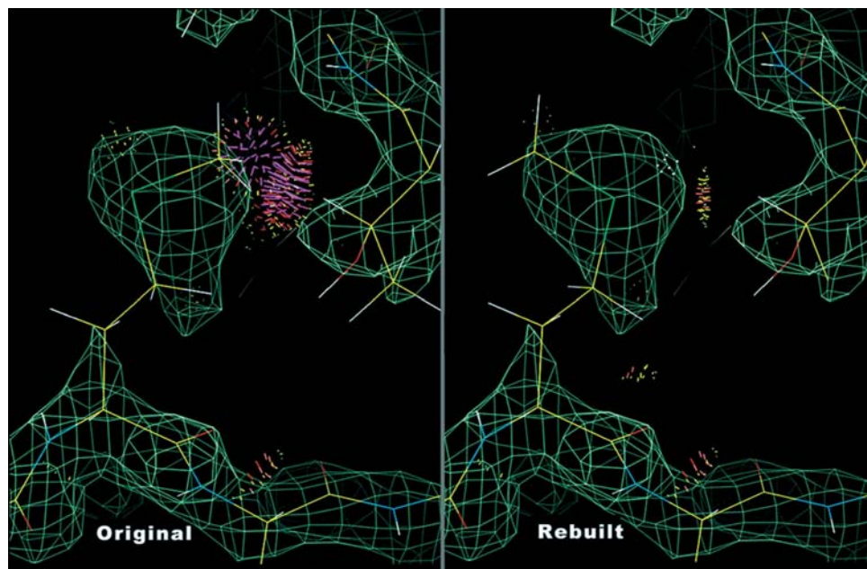
Fig. 25.2.8.4. All-atom contact dots being used in O for model rebuilding during refinement of a Trp tRNA synthetase at 2.3 Å resolution (courtesy of Charles W. Carter, University of North Carolina, Chapel Hill). The Met side-chain density is fairly round and accommodates the original fitting reasonably, but the contact dots show serious clashes (red spikes in the left panel). Rebuilding relieved all clashes (right panel), with equal or better fit to the map and to rotamer preferences. In this case, the electron density can be contoured lower to show a small but definite bulge in the direction of the rebuilt methyl.
