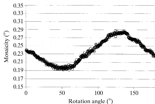
Fig. 11.5.7.7. Variation of (unconstrained) mosaicity for a monoclinic crystal of the bacterial virus alpha3 (Bernal et al. , 1998) showing the crystal anisotropy.
