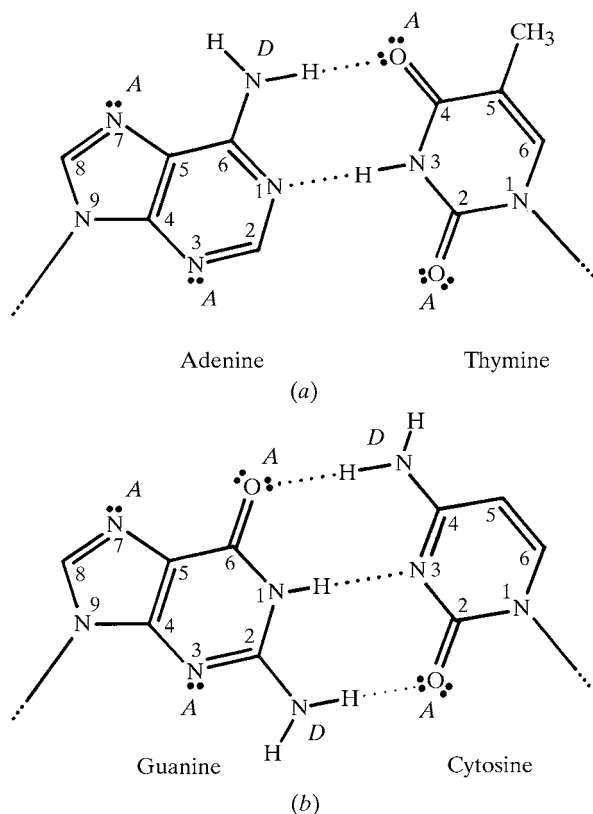
Fig. 23.3.2.7. A-T and G-C base pairs with minor groove edge below and major groove edge above. A is a hydrogen-bond acceptor, D is as hydrogen-bond donor.
