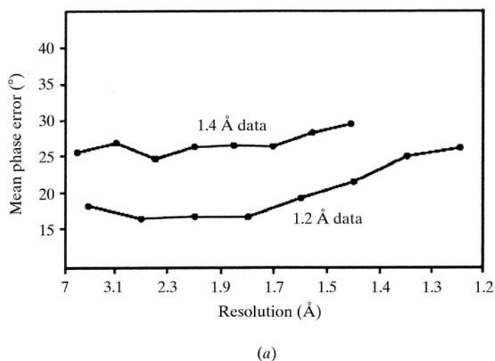
Fig. 16.1.8.2. (a) Mean phase error as a function of resolution for the two independent ab initio SHELXD solutions of the previously unsolved protein hirutasin. Either the 1.2 Å or the 1.4 Å native data set led to solution of the structure. (b) Part of the hirutasin molecule from the 1.4 Å room-temperature data after one round of B -value refinement with fixed coordinates.
