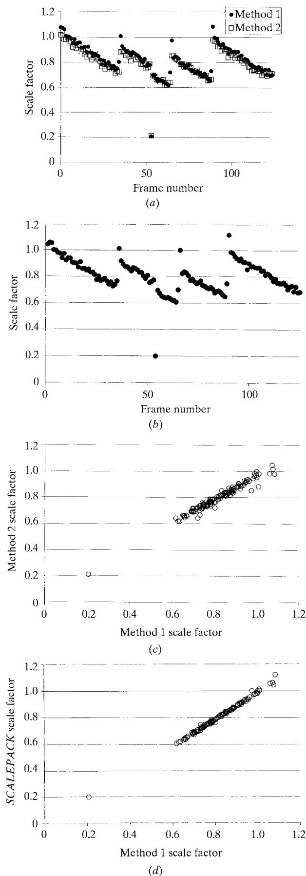
Fig. 11.5.7.1. Linear scale factors as a function of frame number for a \phi X174 data set (Dokland et al. , 1997). Results from (a) method 1 and method 2, (b) SCALEPACK. Comparison of (c) method 2 versus method 1, and (d) SCALEPACK versus method 1.
