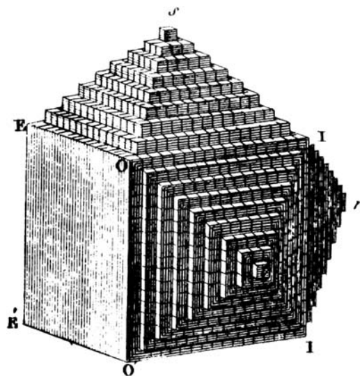
Fig. 17.2.1.1. Model of a crystal structure proposed by René Häuy in Traite elementaire de Physique , Vol. 1 [Paris: De L'Imprimerie de Delance et Lesueur, 1803]. This model, proposed in 1784, was the first to connect the external facets of a crystal with an underlying regular arrangement of building blocks.
