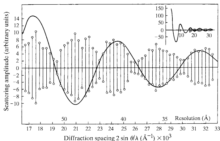
Fig. 13.4.12.1. Structure amplitudes of the type II crystals of southern bean mosaic virus, averaged within shells of reciprocal space, shown in relation to the Fourier transform of a 284 Å diameter sphere. The inset shows the complete spherical transform from infinity to 30 Å resolution. [Reproduced with permission from Johnson et al. (1976). Copyright (1976) Academic Press.]
