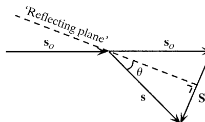
Fig. 2.1.4.3. The direction of the incident wave is indicated by \mathbf{s}_0 and that of the scattered wave by \mathbf{s} . Both vectors are of length 1/\lambda . A plane that makes equal angles with \mathbf{s} and \mathbf{s}_0 can be regarded as a mirror reflecting the incident beam. Reproduced with permission from Drenth (1999). Copyright (1999) Springer-Verlag.
