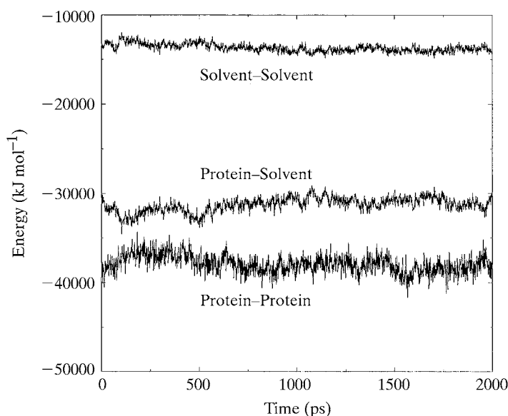
Fig. 20.1.3.1. Non-bonded energies (in \text{kJ mol}^{-1} ) of the simulated system as a function of time.
