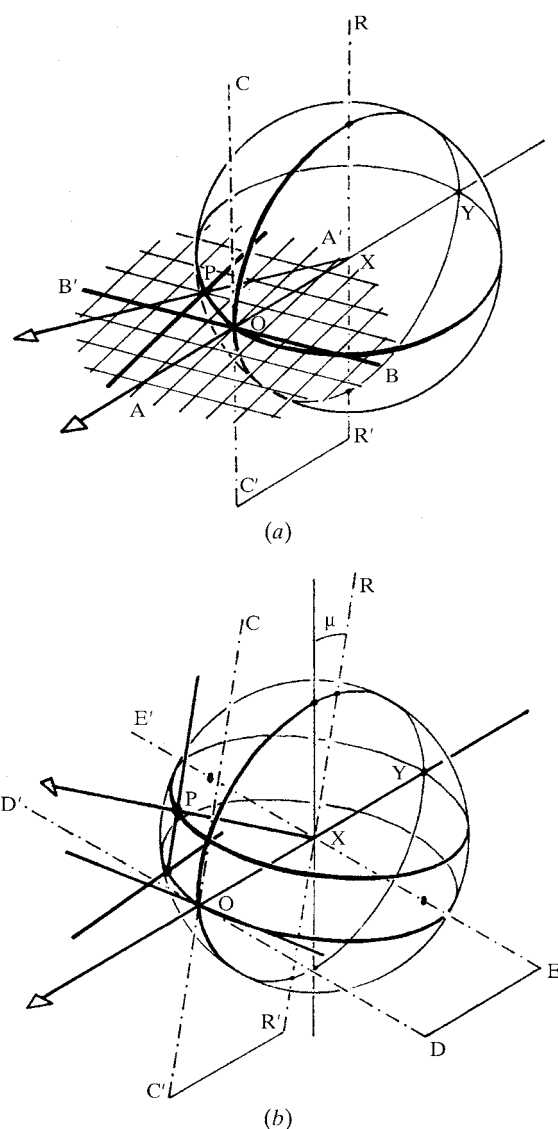
Fig. 26.1.2.4. Reciprocal-space diagrams showing the direction of the incident X-ray beam, the Ewald sphere and the genesis of a reflection (a) in an equatorial plane and (b) in the equi-inclination setting. Principal reciprocal-lattice directions are shown as thick lines. They also represent the slides in the diffractometer. The rotation of the diffractometer slide system about the axis C'OC is coupled to the rotation of the crystal about the axis R'XR by gears, pulleys and steel tapes. The counter arm of the diffractometer is represented by the fixed link XP = XO . Reproduced with permission from Arndt & Phillips (1961). Copyright (1961) International Union of Crystallography.
