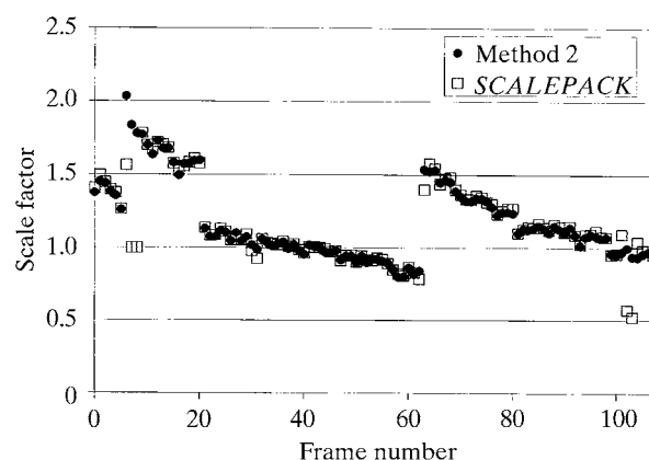
Fig. 11.5.7.2. Linear scale factor as a function of frame number for an HRV14 data set (Rossmann et al. , 1985, 1997).
