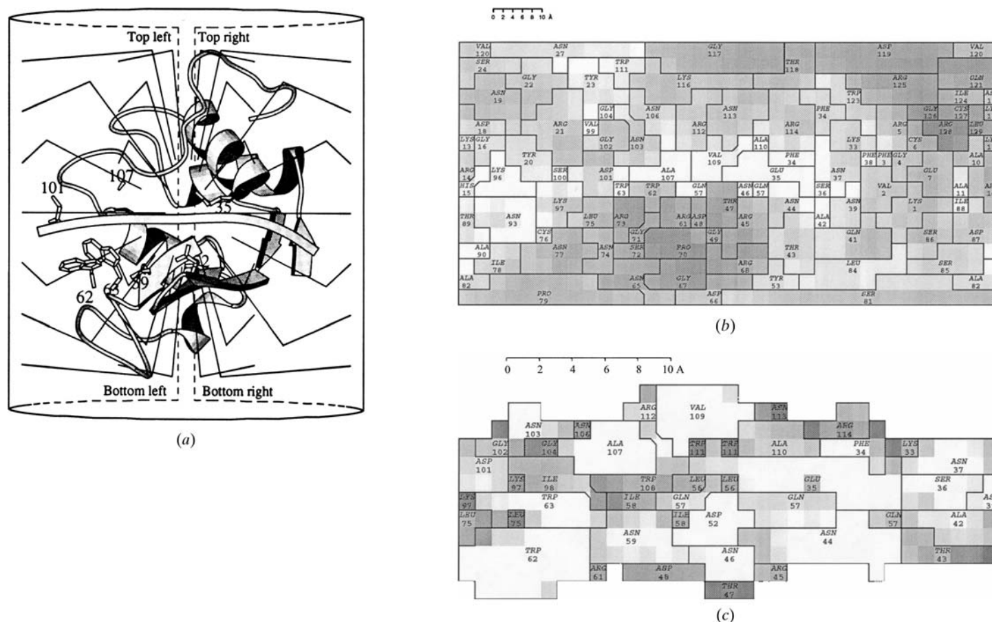
Fig. 22.1.2.4. Different projections illustrated with lysozyme. (a) Lysozyme (Blake et al. , 1965; Diamond, 1974) is sketched with MOLSCRIPT (Kraulis, 1991) and shown with a ribbon indicating the active-site cleft (Kelly et al. , 1979). A cylindrical surface shown unrolled in (b) is shown in (a) wrapped around lysozyme. Vectors orthogonal to the now cylindrical illustrative surface are extended inwards until they intersect with the sphere. Vectors then run towards the centre of the molecule, and their intersections with the solvent-accessible surface are projected back upon the cylinder [unrolled in (b)]. (b) The surface is shaded according to distance from the centre, revealing the substrate-binding cleft as lighter shading. Details of active-site residues are revealed in (c) with a different type of projection. A segmented bent cylinder was traced along the substrate-binding cleft. The surface shows the projection outwards from points on the cylindrical axis. This reveals the amino acids likely to be in most intimate contact with the substrate. Similar plots, coloured according to charge, atomic solvation parameters, or hydrophobicity, can reveal the nature of predominant chemical interactions. This figure is reproduced from Chapman (1993). Copyright (1993) The Protein Society. Reprinted with the permission of Cambridge University Press.
