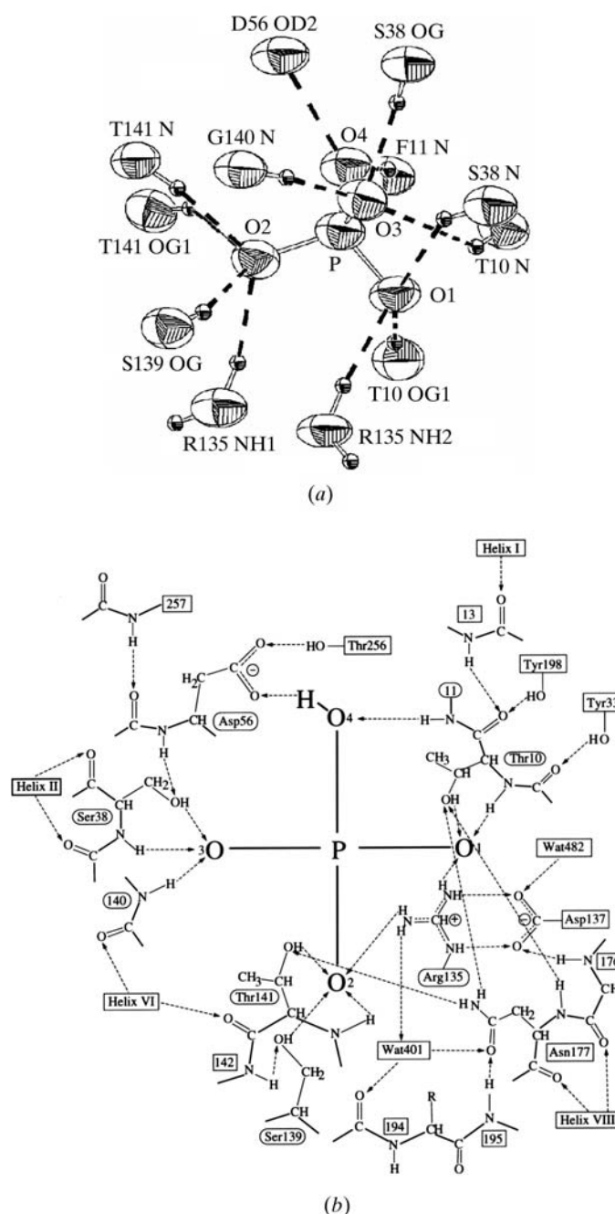
Fig. 23.2.5.1. 12 hydrogen-bonding interactions between the phosphate-binding protein (PBP) and phosphate. (a) Displacement ellipsoids of the atoms involved in the interactions from the 0.98 Å atomic structure (Wang et al. , 1997). (b) Schematic diagram of the interactions, including additional hydrogen bonds.
