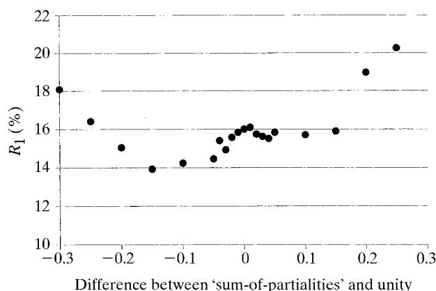
Fig. 11.5.7.4. R factor as a function of the difference of calculated 'sum-of-partialities' and unity for the estimates of full reflections when method 1 is used for the scaling and averaging of a \varphi X174 data set (Dokland et al. , 1997).
