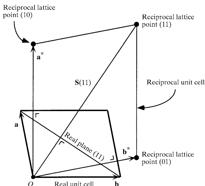
Fig. 2.1.5.1. A two-dimensional real unit cell is drawn together with its reciprocal unit cell. The reciprocal-lattice points are the endpoints of the vectors \mathbf{S}(hk) [in three dimensions \mathbf{S}(hkl) ]; for instance, vector \mathbf{S}(11) starts at O and ends at reciprocal-lattice point (11). Reproduced with permission from Drenth (1999). Copyright (1999) Springer-Verlag.
