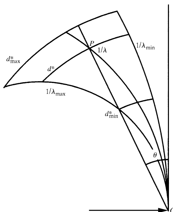
Fig. 8.2.2.1. Laue diffraction geometry. The volume element dV stimulated in a Laue experiment lies between d^* and d^* + dd^* , between the Ewald spheres corresponding to \lambda and \lambda + d\lambda , and between \varphi and \varphi + d\varphi , where \varphi denotes rotation about the incident X-ray beam direction. The entire volume stimulated in a single Laue exposure lies between 0 and d_{\max}^* , between the Ewald spheres corresponding to \lambda_{\min} and \lambda_{\max} , and between values of \theta ranging from 0 to 2\pi .
