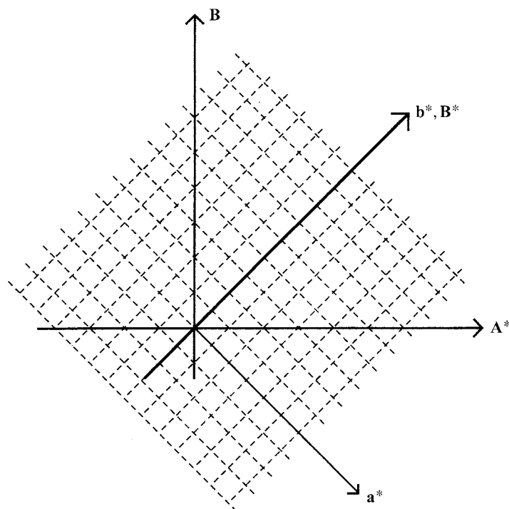
Fig. 26.1.3.2. The a^*b^* plane of the reciprocal lattice oriented to rotate about the [110] axis. The indexing of reflections in a monoclinic unit cell with axes A^* and B^* is also shown. A^* coincides with [110] in the tetragonal lattice and B^* coincides with b^* . The rotation axis is the B axis in the monoclinic cell. The reciprocal-lattice dimensions with Cu K\alpha radiation are a^* = b^* = 0.0195 ; c^* = 0.0406 r.l.u., while the cell diagonal in the a^*b^* plane is 0.0276 r.l.u.
