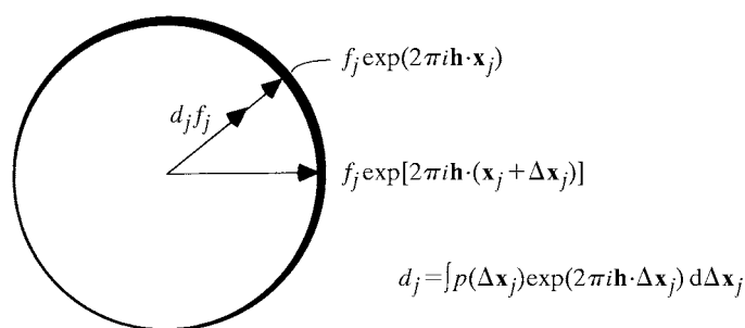
Fig. 15.2.3.1. Centroid of the structure-factor contribution from a single atom. The probability of a phase for the contribution is indicated by the thickness of the line.
