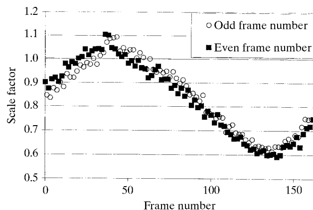
Fig. 11.5.7.3. Linear scale factor determined by method 2 as a function of frame number for an SCP(114–264) data set (Choi et al. , 1991, 1996). The sine-like pattern reflects the anisotropy of a thin plate-shaped crystal.
