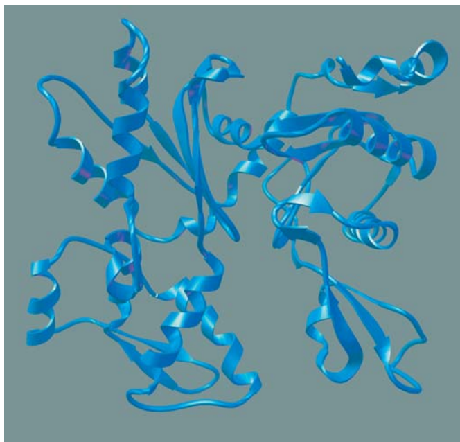
Fig. 17.2.3.2. Ribbon diagram of actin monomer (PDB code: 1atn) (Kabsch et al. , 1990).
