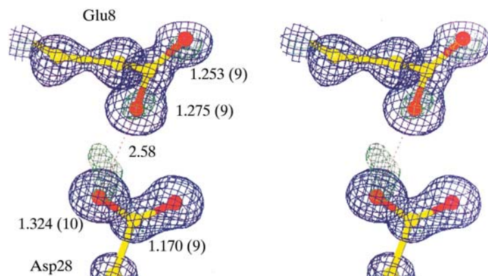
Fig. 8.1.8.1. Determination of the protonation states of carboxylic acid side chains in proteins via hydrogen atoms and resolved single and double bond lengths. After Deacon et al. (1997) using CHESS. Reproduced by permission of The Royal Society of Chemistry.
