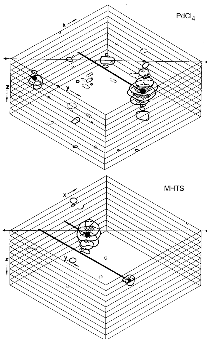
Fig. 26.1.2.11. Electron-density difference syntheses showing the main sites of substitution and subsidiary sites with low occupancy in the \text{PdCl}_4 and MHTS derivatives (Fenn, 1964).
