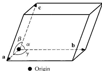
Fig. 2.1.1.1. One unit cell with axes a , b and c . The angles between the axes are \alpha , \beta and \gamma . Note that the axial system is right-handed. Reproduced with permission from Drenth (1999). Copyright (1999) Springer-Verlag.
