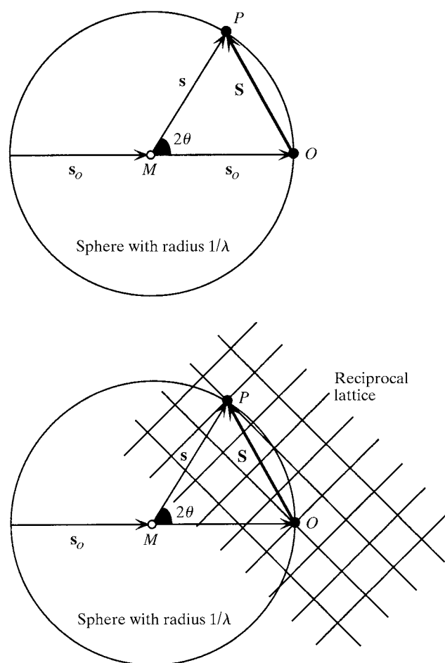
Fig. 2.1.5.2. The circle is, in fact, a sphere with radius 1/\lambda . \mathbf{s}_0 indicates the direction of the incident beam and has a length 1/\lambda . The diffracted beam is indicated by vector \mathbf{s} , which also has a length 1/\lambda . Only reciprocal-lattice points on the surface of the sphere are in a reflecting position. Reproduced with permission from Drenth (1999). Copyright (1999) Springer-Verlag.
