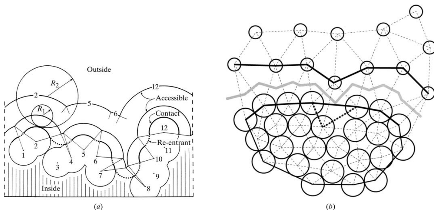
Fig. 22.1.1.7. Definitions of the protein surface. (a) The classic definitions of protein surface in terms of the probe sphere, the accessible surface and the molecular surface. (This figure is adapted from Richards, 1977). (b) Voronoi polyhedra and Delaunay triangulation can also be used to define a protein surface. In this schematic, the large spheres represent closely packed protein atoms and the smaller spheres represent the small loosely packed water molecules. The Delaunay triangulation is shown by dotted lines. Some parts of the triangulation can be used to define surfaces. The outermost part of the triangulation of just the protein atoms forms the convex hull. This is indicated by the thick line around the protein atoms. For the convex-hull construction, one imagines that the water is not present. This is highlighted by the thick dotted line, which shows how Delaunay triangulation of the surface atoms in the presence of the water diverges from the convex hull near a deep cleft. Another part of the triangulation, also indicated by thick black lines, connects the first layer of water molecules (those that touch protein atoms). A time-averaged version of this line approximates the accessible surface. Finally, the light thick lines show the Voronoi faces separating the protein surface atoms from the first layer of water molecules. Note how this corresponds approximately to the molecular surface (considering the water positions to be time-averaged). These correspondences between the accessible and molecular surfaces and time-averaged parts of the Voronoi construction are understandable in terms of which part of the probe sphere (centre or point of tangency) is used for the surface definition. The accessible surface is based on the position of the centre of the probe sphere while the molecular surface is based on the points of tangency between the probe sphere and the protein atoms, and these tangent points are similarly positioned to Voronoi faces, which bisect interatomic vectors between solvent and protein atoms.
