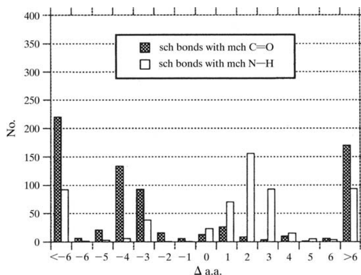
Fig. 22.2.5.1. Distribution of side-chain-main-chain hydrogen bonds as a function of the separation ( \Delta a.a.) along the polypeptide between the side-chain (sch) and main-chain (mch) groups involved, i.e. \Delta a.a. = -n means that a side chain interacts with a main-chain group n residues earlier in the polypeptide (towards the N-terminus). Reproduced with permission from Bordo & Argos (1994). Copyright (1994) Academic Press.
