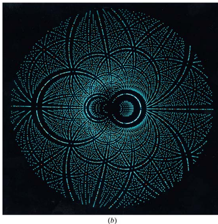
Fig. 8.1.4.2. Single-crystal SR diffraction patterns. (a) Rhinovirus monochromatic oscillation photograph recorded at CHESS (Arnold et al. 1987; see also Rossmann & Erickson, 1983). Copyright (1987) International Union of Crystallography. (b) Prediction of a protein crystal Laue diffraction pattern (for an illuminating bandpass, without monochromator, \sim 0.4 < \lambda < 2.6 Å). The colour coding is according to the multiplicity of each spot: turquoise for singlet reflections, yellow for doublets, orange for triplets and blue for quartet or higher-multiplicity Laue spots. Reproduced with permission from Cruickshank et al. (1991). Copyright (1991) International Union of Crystallography.
