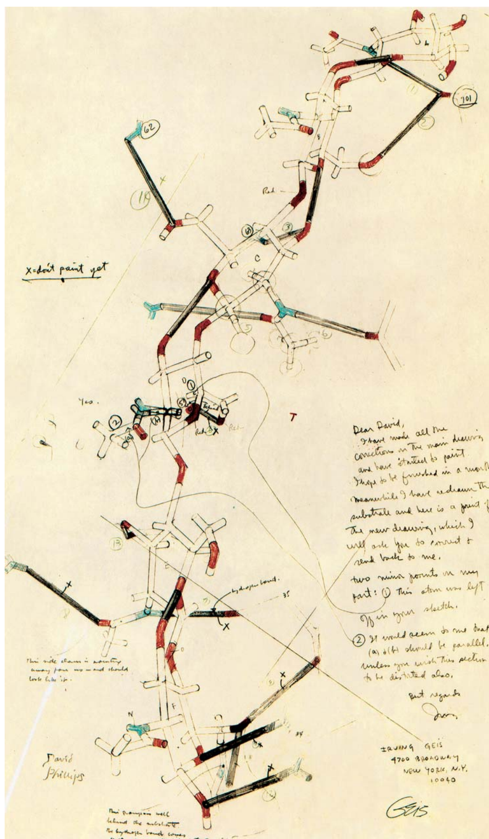
Fig. 26.1.4.5. Draft sketch of the lysozyme-hexasaccharide substrate complex prepared by Irving Geis and annotated by David Phillips for an article published in Scientific American in 1966 (Phillips, 1966).
