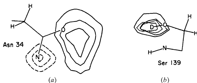
Fig. 19.1.5.1. Difference map of Asn34 in the trypsin structure. (a) In a protein X-ray analysis, the difference in scattering intensity between O and \text{NH}_2 is much too small to be detected. In contrast, the neutron-scattering magnitudes of oxygen and nitrogen (5.8 f versus 9.4 f) are quite dissimilar, and there is additional scattering at the nitrogen site from the two bound deuterium atoms. The resulting differential is over 350%, quite large enough to be detected for well ordered side chains. The nitrogen and oxygen positions shown are from the X-ray model. The difference density indicates that the orientation of the nitrogen and oxygen atoms is incorrect and should be rotated by 180^\circ around the \text{C}_\beta\text{--C}_\gamma bond. (b) Difference map for Ser139. On well ordered hydroxyl side chains, the orientation of deuterium atoms can sometimes be assigned.
