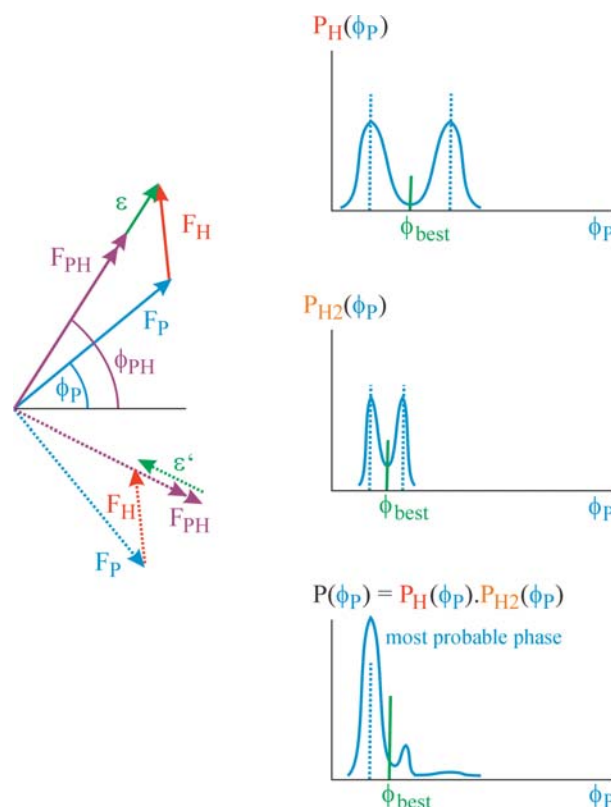
Fig. 12.2.4.1. The treatment of phase errors. The calculated heavy-atom structure results in a calculated value for both the phase and magnitude of F_H (red). According to the value of \varphi_P , the triangle F_P - F_H - F_{PH} will fail to close by an amount \epsilon , the lack of closure (green). This gives rise to a phase distribution which is bimodal for a single derivative. The combined probability from a series of derivatives has a most probable phase (the maximum) and a best phase (the centroid of the distribution), for which the overall phase error is minimum.
