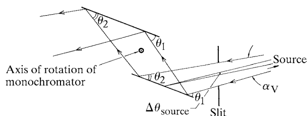
Fig. 8.1.7.2. Double-crystal monochromator illuminated by SR. The contributions of the source divergence, \alpha_v [less than or equal to \gamma_v^{-1} , equation (8.1.2.4), depending on the monochromator vertical entrance slit aperture; see also Colapietro et al. , 1992], and angular source size, \Delta\theta_{\text{source}} , to the range of energies reflected by the monochromator are shown. From Helliwell (1984). Reproduced with the permission of the Institute of Physics.
