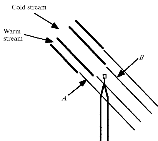
Fig. 10.1.4.2. Schematic drawing of a dual-stream setup with the streams angled relative to the diffractometer \varphi axis. A and B are the same as in Fig. 10.1.4.1. The cold stream misses the goniometer head, so no shield is required.
