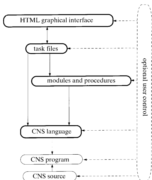
Fig. 25.2.3.1. CNS consists of five layers which are under user control. The high-level HTML graphical interface interacts with the task-oriented input files. The task files use the CNS language and the modules. The modules contain CNS language statements. The CNS language is interpreted by the CNS Fortran77 program. The program performs the data manipulations, data operations and 'hard-wired' algorithms.
