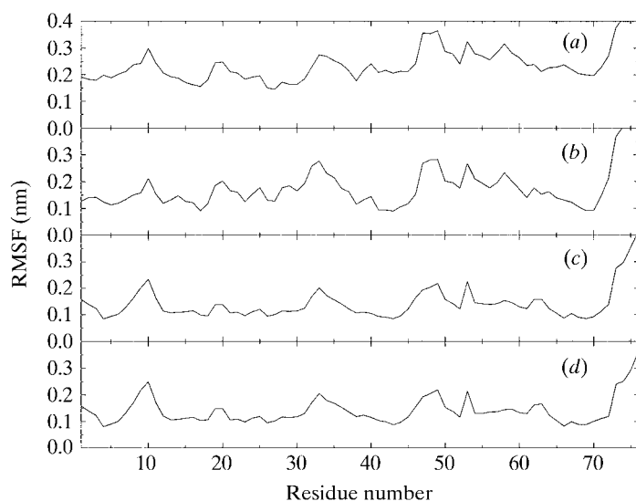
Fig. 20.1.3.5. Root-mean-square C\alpha -atom-position fluctuations (RMSFs) in nm are shown using the same fitting protocols as in Fig. 20.1.3.4, but averaged over all four protein molecules in the unit cell.
