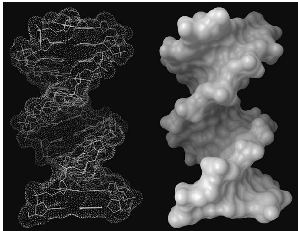
Fig. 17.2.3.5. Solvent-excluded surface of the DNA structure using a water probe radius of 1.5 Å. The figure on the left shows a depth-cued dot surface, while the figure on the right shows a Gouraud-shaded triangulated surface.
