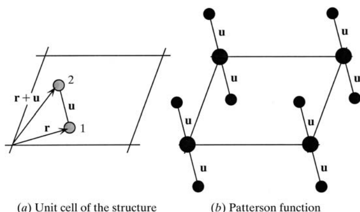
Fig. 2.1.9.1. (a) A two-dimensional unit cell with two atoms. (b) The corresponding Patterson function. Reproduced with permission from Drenth (1999). Copyright (1999) Springer-Verlag.
