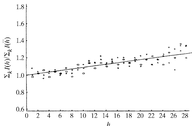
Fig. 26.1.3.6. Plot of the ratio \sum_k I(h) / \sum_k I(-h) against h . In this example, a linear correction may be safely applied to equalize the average intensities in opposite rows (North et al. , 1968).
