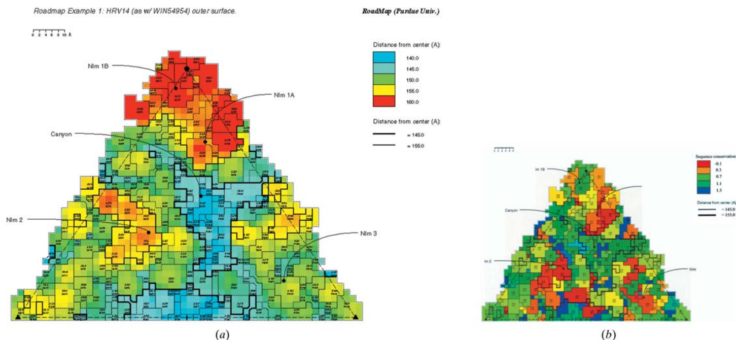
Fig. 22.1.2.3. (a) Solvent-accessible surface topology of a rhinovirus 14–drug complex (Kim et al. , 1993). The triangle shows one of the 60 symmetry-equivalent faces of an icosadeltahedron that constitute the entire virus surface. The surface is coloured and contoured according to distance from the centre of the virus, red being the most elevated. Residues are marked with dotted lines and labelled with residue type and number. A letter starting the residue label indicates a symmetry equivalent. The first numeral indicates the protein number (1 to 4), which is followed by the three-digit residue number. A depression, the ‘canyon’, is where the cellular receptor is bound (Olson et al. , 1993). The locations of the dominant neutralizing immunogenic (NIm) sites were determined through the sequencing of escape mutants (Sherry & Rueckert, 1985; Sherry et al. , 1986) and are labelled ‘NIm’. (b) The same view is coloured according to sequence similarity (Palmenberg, 1989; Chapman, 1994), with blue being the most conserved rhinoviral amino acids and red being the most variable. Comparison of diagrams like these suggested the ‘canyon hypothesis’ (Rossmann, 1989). The prediction has proved largely true in that the sites of receptor attachment in several picornaviruses would be depressed areas whose sequences could be more highly conserved because they were partially inaccessible to antibodies and therefore not under the same selective pressure to mutate. In this and other applications, the schematic nature of these diagrams has helped in the collation of structure with data arising from the known phenotypes of site-directed or natural mutants. Part (b) is reproduced from Chapman (1993). Copyright (1993) The Protein Society. Reprinted with the permission of Cambridge University Press.
