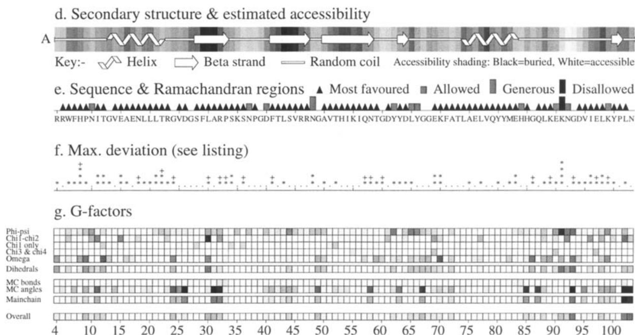
Fig. 25.2.6.3. Schematic plots of various residue-by-residue properties, showing (d) the protein secondary structure, with the shading behind it giving an approximation to each residue's accessibility, the darker the shading the more buried the residue; (e) the protein sequence plus markers identifying the region of the Ramachandran plot in which the residue is located; (f) a histogram of asterisks and plus signs showing each residue's maximum deviation from one of the ideal values, as shown on the residue-by-residue listing; and (g) the residue 'G factor' values for various properties, where the darker the square the more 'unusual' the property.
