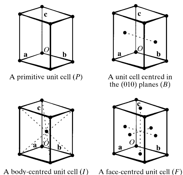
Fig. 2.1.1.4. Non-centred and centred unit cells. Reproduced with permission from Drenth (1999). Copyright (1999) Springer-Verlag.
