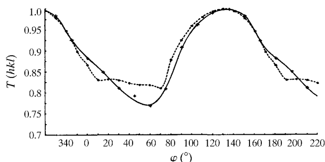
Fig. 26.1.2.6. Absorption curve. Variation of relative transmission T(hkl) = I(\varphi_{hkl})/I_{\max}(\varphi) [= 1/A(hkl)] with rotation angle \varphi for the 200 reflection and the crystal rotating about the normal to (200). Solid line: measured curve; broken line: calculated curve, neglecting effect of mother liquor and capillary. Reproduced with permission from North et al. (1968). Copyright (1968) International Union of Crystallography.
