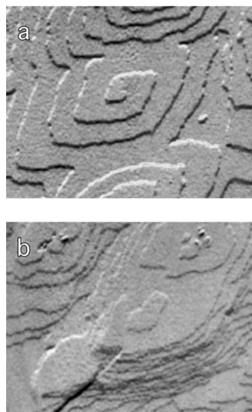
Fig. 4.1.5.1. Visualization of the surface of yeast tRNA Phe crystals by AFM. (a) Spiral growth with screw dislocations occurring at lower supersaturation and (b) growth by two-dimensional nucleation occurring at higher supersaturation, showing growth and coalescence of islands and expansions of stacks. Notice that supersaturation and type of growth mechanisms are very temperature-sensitive and are modulated by temperature variation, since in (a), crystals grew at 15 °C and in (b), at 13 °C. Reproduced with permission from Ng, Kuznetsov et al. (1997). Copyright (1997) Oxford University Press.
