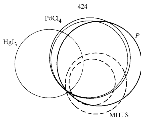
Fig. 26.1.2.10. Phase determination for reflection 424. In this Harker diagram, the heavily traced protein circle (with radius |F_P| ) is labelled P . The circles with radii |F_{HP}| obtained with PdCl 4 , MHTS and HgI 3 are shown. Values of the anomalous-scattering pairs hkl and khl were used for PdCl 4 and MHTS. The position of the protein vector, weighted by its figure of merit, is shown as a small open circle (R. J. Poljak, unpublished results).
