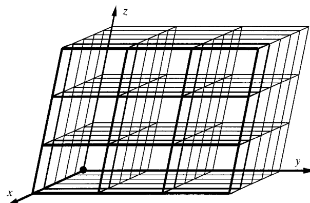
Fig. 2.1.1.2. A set of 5 \times 3 \times 3 unit cells. The points where the lines intersect are called lattice points. The axes x and y form a (001) plane, which is one member of the set of parallel and equidistant (001) planes; y and z form a (100) plane, and z and x a (010) plane. Reproduced with permission from Drenth (1999). Copyright (1999) Springer-Verlag.
