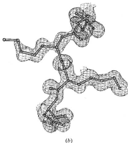
Fig. 16.1.8.2. (a) Mean phase error as a function of resolution for the two independent ab initio SHELXD solutions of the previously unsolved protein hirutasin. Either the 1.2 Å or the 1.4 Å native data set led to solution of the structure. (b) Part of the hirutasin molecule from the 1.4 Å room-temperature data after one round of B -value refinement with fixed coordinates.
