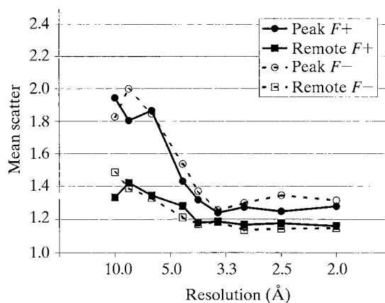
Fig. 11.5.7.8. Quality of anomalous-dispersion data for an SeMet derivative of dioxxygenase Rieske ferredoxin (Colbert & Bolin, 1999).
