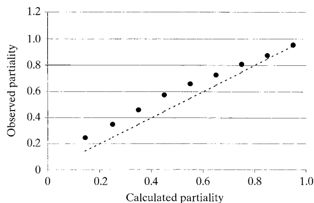
Fig. 11.5.7.6. The observed partialities plotted against calculated partialities for a \varphi X174 data set (Dokland et al. , 1997) processed by method 2. The observed partialities for individual partial reflections were averaged in bins of calculated partialities. The broken line represents the ideal relationship p_{\text{obs}} = p_{\text{calc}} .
