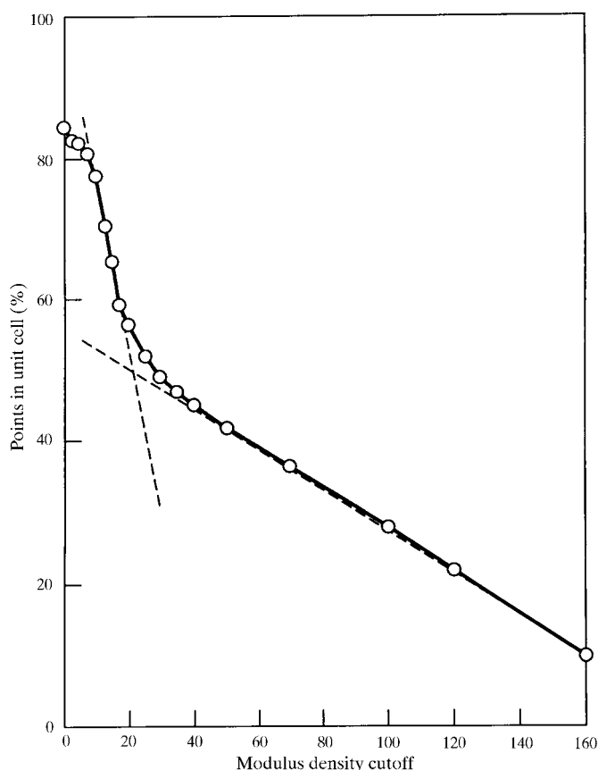
Fig. 13.4.6.1. The volume of the molecular mask expressed as a percentage of the volume of the p -cell asymmetric unit, as determined by the density cutoff in the h -cell. When the modulus of the density cutoff is decreased to less than the mean smeared electron density within the protein, the mask volume increases rapidly. Intersection of the tangents suggests the most appropriate density cutoff value for mask generation. [Reproduced with permission from McKenna, Xia, Willingmann, Ilag & Rossmann (1992). Copyright (1992) International Union of Crystallography.]
