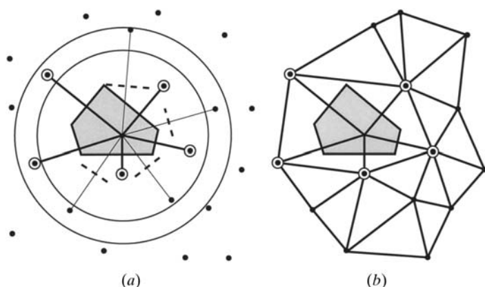
Fig. 22.1.1.5. Delaunay triangulation and its relation to the Voronoi construction. (a) A standard schematic of the Voronoi construction. The atoms used to define the Voronoi planes around the central atom are circled. Lines connecting these atoms to the central one are part of the Delaunay triangulation, which is shown in (b). Note that atoms included in the triangulation cannot be selected strictly on the basis of a simple distance criterion relative to the central atom. The two circles about the central atoms illustrate this. Some atoms within the outer circle but outside the inner circle are included in the triangulation, but others are not. In the context of protein structure, Delaunay triangulation is useful in identifying true 'packing contacts', in contrast to those contacts found purely by distance threshold. The broken lines in (a) indicate planes that were initially included in the polyhedron but then removed by the 'chopping-down' procedure (see Fig. 22.1.1.4).
