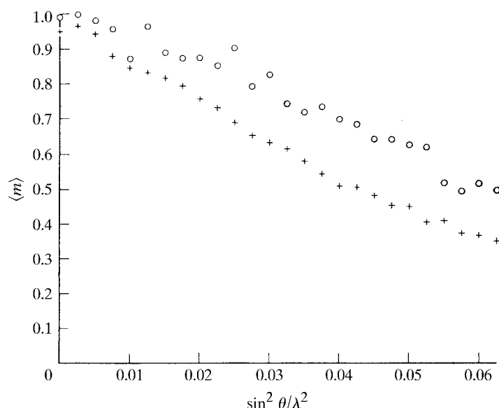
Fig. 26.1.3.8. Variation of the mean figure of merit \langle m \rangle with \sin^2 \theta / \lambda^2 . (crosses represent acentric reflections, open circles represent centric reflections).
