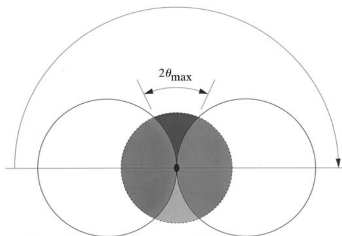
Fig. 9.1.7.1. Rotation of a triclinic crystal by 180^\circ in the X-ray beam, represented as rotating the Ewald sphere with a stationary crystal, projected along the rotation axis. For the purpose of analysing the relation of data completeness to crystal symmetry and orientation both representations are equivalent.
