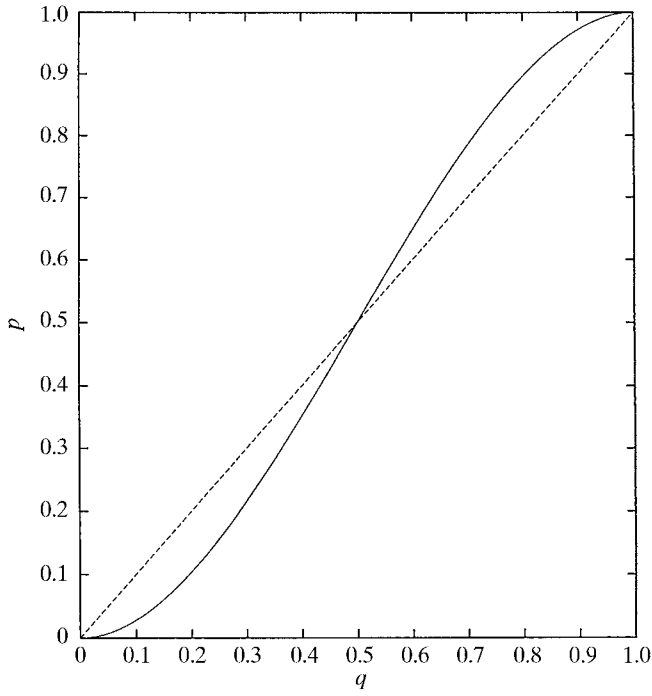
Fig. A11.5.1.2. Relationship between the fraction of the path travelled, q , by a reciprocal-lattice point across an Ewald sphere of finite thickness and the fraction of the total scattered intensity, p . The curve shown is for p = 3q^2 - 2q^3 . As an extreme case, the line p = q is also shown.
