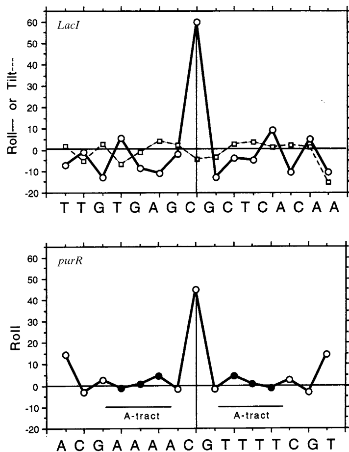
Fig. 23.3.4.6. Roll-angle plots for sequence-specific DNA-protein complexes with lacI (top) and purR (bottom). In each case, bending occurs via localized roll at a C-G step. Other steps of the sequence have random rolls of ca 10° or less. Note that, as with IHF, A-tracts are especially straight and unbent. Dashed lines in the lacI plot demonstrate the unimportance of tilt in production of helix bending.
