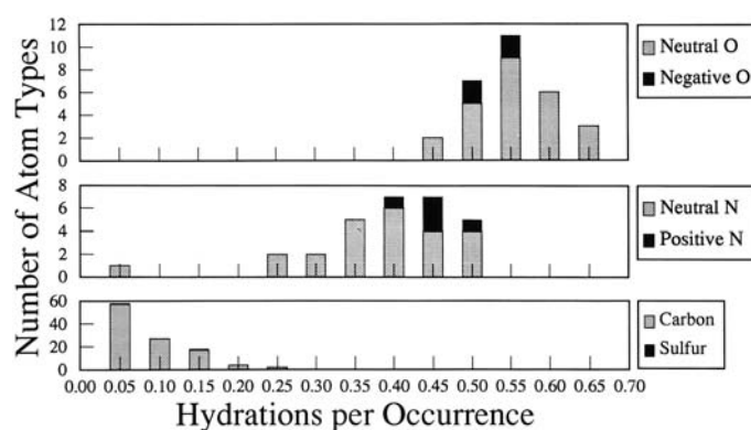
Fig. 23.4.3.2. Distribution of atomic hydration values. To determine which atoms are similar or distinct with respect to water binding, we plotted the number of atom types (e.g. Ala amide nitrogen, Ala C\alpha , . . .) at each hydration per occurrence value. Each atom type contributed one vertical unit to the graph. Oxygen atoms were the most hydrated (top graph), with negatively charged oxygen (black bars) slightly less hydrated on average than neutral oxygen (grey bars). Nitrogens (middle graph) were the next most hydrated, overlapping the oxygen distribution, and positively charged nitrogens (black bars) were somewhat more hydrated than neutral nitrogens (grey bars). Proline's amide nitrogen, with no hydrogen-bonding capacity, had the lowest nitrogen hydration value (leftmost bar). Carbon and sulfur atoms (bottom graph; note change of y-axis scale) were the least hydrated, with sulfur values at 0.05 and 0.15 hydrations per occurrence. Reproduced from Kuhn et al. (1995). Copyright (1995) Wiley-Liss, Inc. Reprinted by permission of Wiley-Liss, Inc., a division of John Wiley & Sons, Inc.
