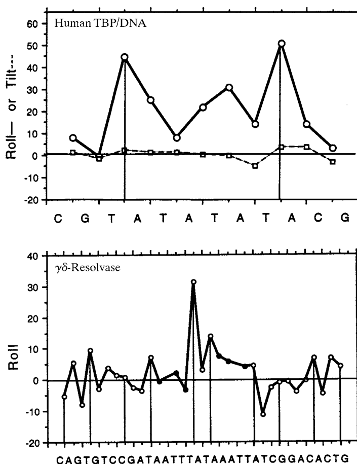
Fig. 23.3.4.7. Bending via roll at T-A steps in TBP or the TATA-binding protein (top) and in \gamma\delta -resolvase (bottom). Note that not every T-A step in TBP or \gamma\delta -resolvase is necessarily bent. Note also in \gamma\delta -resolvase that C-A = T-G steps, which in proteins such as CAP are used to generate sharp roll bends, here, frequently, are local roll maxima, even though they contribute little to the overall bending. They have a bending potential that is not used in this particular setting.
