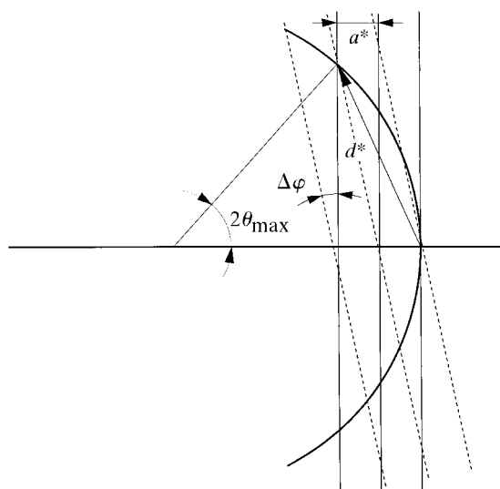
Fig. 9.1.6.7. The largest allowed rotation range per exposure depends on the dimension of the primitive unit cell oriented along the X-ray beam; this is diminished by high mosaicity.
