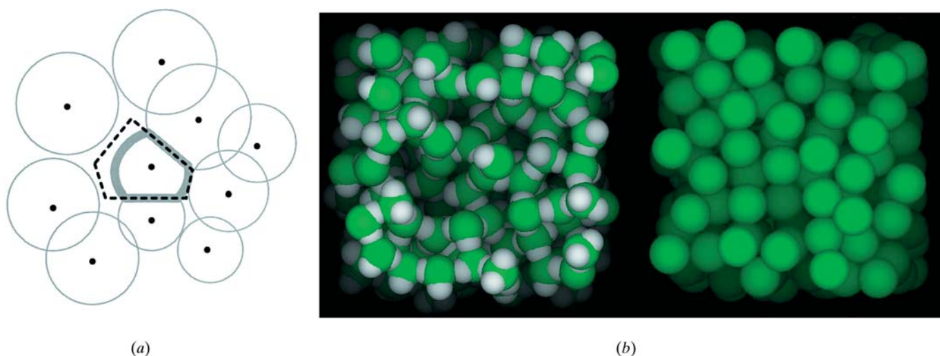
Fig. 22.1.1.8. Packing efficiency. (a) The relationship between Voronoi polyhedra and packing efficiency. Packing efficiency is defined as the volume of an object as a fraction of the space that it occupies. (It is also known as the 'packing coefficient' or 'packing density'.) In the context of molecular structure, it is measured by the ratio of the VDW volume ( V_{VDW} , shown by a light grey line) and Voronoi volume ( V_{Vor} , shown by a dotted line). This calculation gives absolute packing efficiencies. In practice, one usually measures a relative efficiency, relative to the atom in a reference state: (V_{VDW}/V_{Vor})/[V_{VDW}/V_{Vor}(\text{ref})] . Note that in this ratio the unchanging VDW volume of an atom cancels out, leaving one with just a ratio of two Voronoi volumes. Perhaps more usefully, when one is trying to evaluate the packing efficiency P at an interface, one computes P = p \sum V_i / \sum v_i , where p is packing efficiency of the reference data set (usually 0.74), V_i is the actual measured volume of each atom i at the interface and v_i is the reference volume corresponding to the type of atom i . (b) A graphical illustration of the difference between tight packing and loose packing. Frames from a simulation are shown for liquid water (left) and for liquid argon, a simple liquid (right). Owing to its hydrogen bonds, water is much less tightly packed than argon (packing efficiency of 0.35 versus ~0.7). Each water molecule has only four to five nearest neighbours while each argon atom has about ten.
