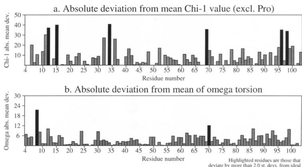
Fig. 25.2.6.2. Two of the residue-property plots generated by PROCHECK . The plots shown here are (a) the absolute deviation from the mean of the \chi_1 torsion angle (excluding prolines) and (b) the absolute deviation from the mean of the \omega torsion angle. Usually, three such plots are shown per page and can be selected from a set of 14 possible plots. On each graph, unusual values (usually those more than 2.0 standard deviations away from the 'ideal' mean value) are highlighted.
