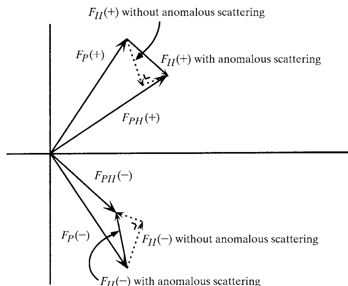
Fig. 2.1.7.1. An Argand diagram for the structure factors of the two members of a Friedel pair. (+) represents hkl and (-) represents \bar{h}\bar{k}\bar{l} . F_P is the contribution to the structure factor by the non-anomously scattering protein atoms and F_H is that for the anomalously scattering atoms. F_H consists of a real part with an imaginary part perpendicular to it. The real parts are mirror images with respect to the horizontal axis. The imaginary parts are rotated counterclockwise with respect to the real parts (Section 2.1.4.4). The result is that the total structure factors, F_{PH}(+) and F_{PH}(-) , have different amplitudes and phase angles. Reproduced with permission from Drenth (1999). Copyright (1999) Springer-Verlag.
