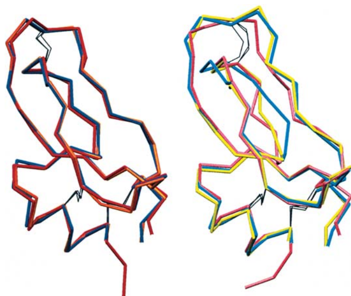
Fig. 20.2.8.1. \alpha tracings of BPTI. Left: crystallographic structures determined from data at three different resolutions: 1.1 (red), 1.7 (blue) and 2.7 Å (orange). Right: 10 ps average MD structures from simulations initiated with the energy-minimized crystallographic structure determined at 1.1 (pink), 1.7 (cyan) or 2.7 Å (yellow) resolution. The 10 ps average is over coordinates from 290 to 300 ps.
