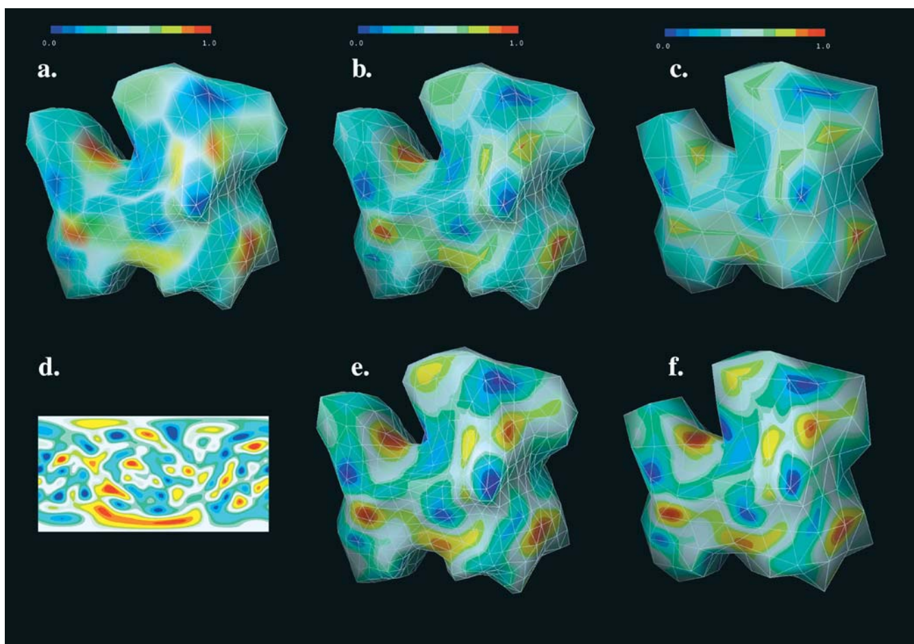
Fig. 17.2.3.6. Hydrophobicity mapped onto a molecular surface. A spherical-harmonic approximation of the actin monomer solvent-excluded surface is shown. (a) Vertex colouring of a medium-mesh tessellated surface. The hydrophobicity colour scale is shown above. Notice that the colours blend between vertices, producing colour artifacts in relationship to the property scale. (b) The same medium-mesh representation as in (a) but using a property-based (one-dimensional) texture map, applying the same colour scale. Notice that the boundaries between the colours are distinct, even when they intersect vertices. Here the property value is interpolated. (c) A coarser mesh showing the same texture-mapping technique used in (b). Since the properties are only sampled at the vertices of the mesh, the finer details of the mapping are lost at this coarse triangulation. (d) A two-dimensional texture map created as a 'Mercator-like' projection in spherical coordinates ( \theta , \varphi ) from the same hydrophobicity scale used in (a)–(c). (e) The 2-D texture map shown in (d) mapped onto the medium-mesh actin surface. Notice that the linear nature of the interpolation seen in (b) using the same mesh is no longer present. (f) The same 2-D texture map applied to the coarse-mesh surface of actin. Notice that, unlike in (c), the detail of the texture map is preserved independent of the mesh.
