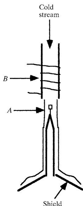
Fig. 10.1.4.3. Schematic drawing of a single-stream setup with the stream parallel to the diffractometer \varphi axis. A represents the outline of the cold stream. The tip of the outlet end is heated above the dew point with a heating coil B. The goniometer head (not shown) is protected by a shield.
