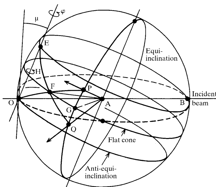
Fig. 26.1.3.1. Perspective drawing of the sphere of reflection showing inclination geometry with simultaneous reflections (reciprocal-lattice points P and Q) from levels symmetrically related by the flat-cone setting. Reproduced with permission from Phillips (1964). Copyright (1964) Institute of Physics.
