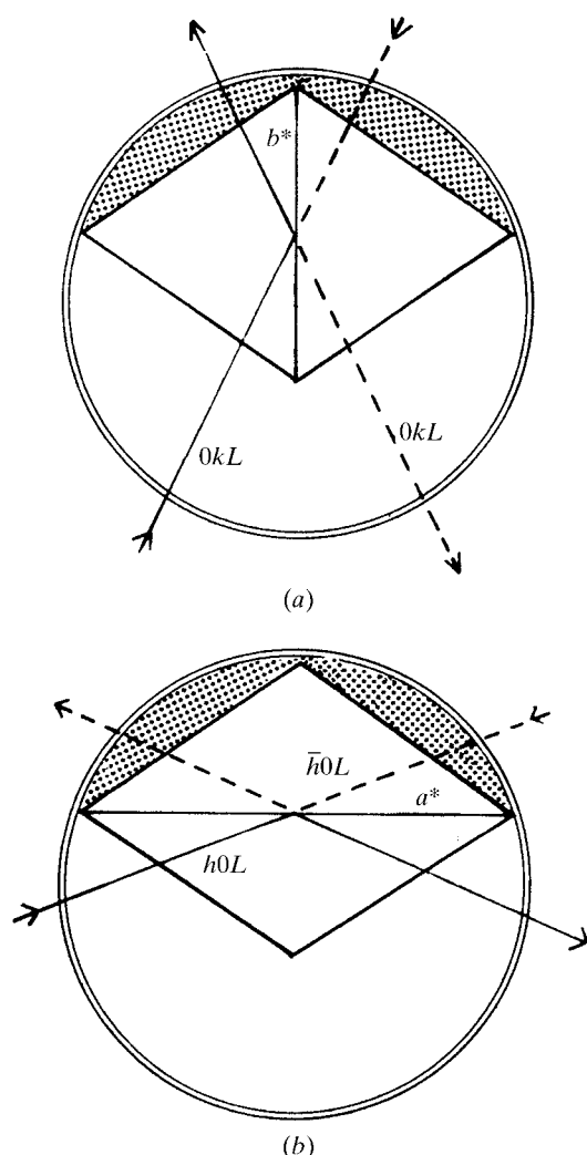
Fig. 26.1.3.5. Asymmetric mounting of a protein crystal with its mother liquor in a capillary tube. Anomalous-scattering differences would be seriously affected in (b) but not in (a). Reproduced with permission from North et al. (1968). Copyright (1968) International Union of Crystallography.
