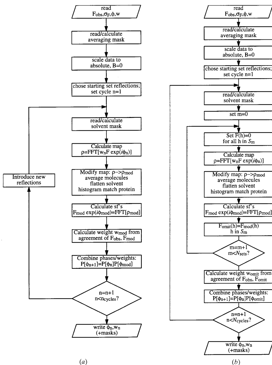
Fig. 25.2.2.2. (a) Flow chart for a simple DM calculation with free-Sim phase combination. (b) Flow chart for a simple DM calculation with reflection-omit phase combination.
