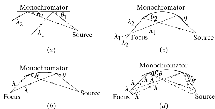
Fig. 8.1.7.1. Single-crystal monochromator illuminated by SR. (a) Flat crystal. (b) Guinier setting. (c) Overbent crystal. (d) Effect of source size (shown at the Guinier setting for clarity). From Helliwell (1984). Reproduced with the permission of the Institute of Physics.
