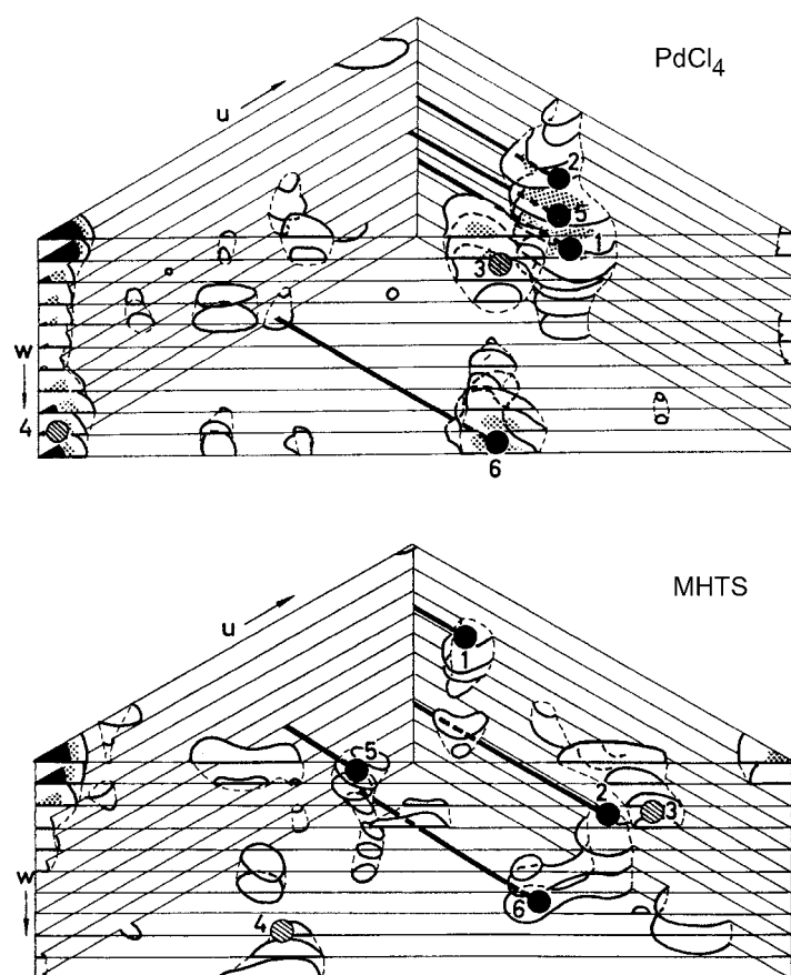
Fig. 26.1.2.9. Three-dimensional |\Delta F|^2 syntheses for the \text{PdCl}_4 and MHTS derivatives. The positions of peaks in the Harker sections are marked and numbered (Fenn, 1964).
