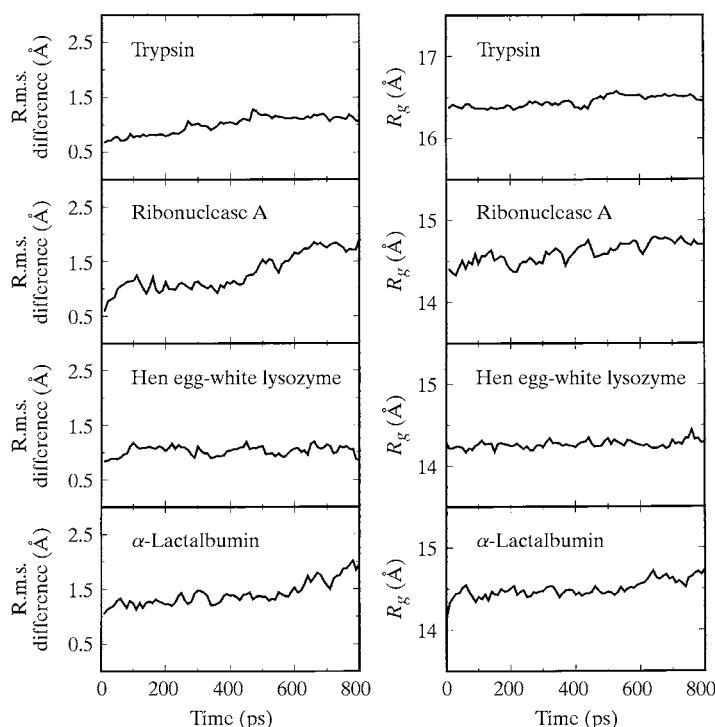
Fig. 20.2.7.1. Structural comparison and radii of gyration of various proteins as a function of time in the molecular-dynamics simulation. Left: r.m.s. coordinate differences averaged over main-chain atoms (N, C \alpha , C) between the energy-minimized crystallographic structure and the simulation snapshot. Right: radii of gyration ( R_g ).
