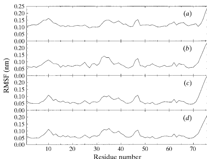
Fig. 20.1.3.4. Root-mean-square C\alpha -atom-position fluctuations (RMSFs) in nm are shown for molecule 4 as a function of residue number. RMSFs are averaged over the final 1.6 ns. In (a), no fitting was applied; in (b), translational fitting was applied using the C\alpha atoms of residues 1–72; and in (c), the rotational component of motion was also removed. In (d), translational and rotational fitting was applied over all C\alpha atoms (1–76).
