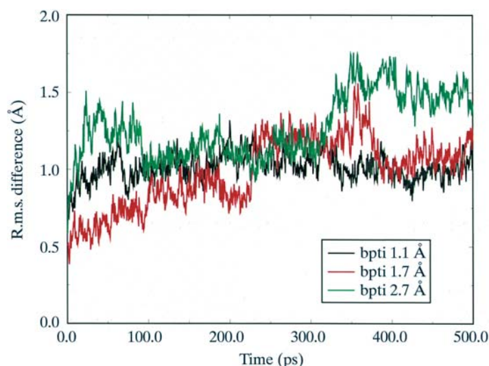
Fig. 20.2.8.2. BPTI r.m.s. coordinate differences between the energy-minimized crystallographic structure and MD snapshots from three simulations. A simulation was initiated from the energy-minimized crystallographic structure determined at 1.1 (black), 1.7 (red) or 2.7 Å (green) resolution. The r.m.s.d. is averaged over the main-chain atoms N, C \alpha and C.
