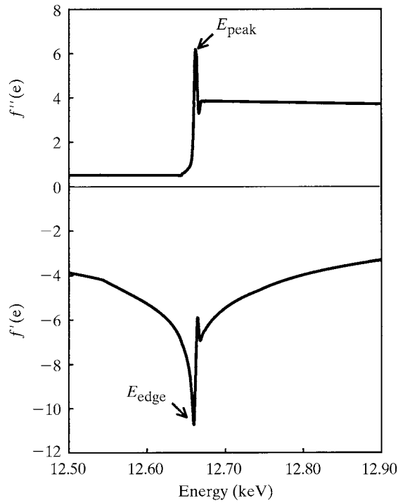
Fig. 14.2.1.1. Anomalous scattering factors for Se in a protein labelled with selenomethionine. The spectra are a hybrid of experimental values derived from an absorption spectrum of a SeMet protein for energies near the Se K absorption edge and calculated values for energies remote from the edge. The Se K edge occurs at 12 660 eV, corresponding to a wavelength of 0.9800 Å. Anomalous-scattering effects are enhanced by a white line just above the edge. The position of the absorption edge ( E_{\text{edge}} ) is the inflection point of the \mu_a (and f'' ) spectrum, and E_{\text{peak}} is the energy of peak absorption just above the edge. These energies correspond to the wavelengths \lambda_{\text{edge}} and \lambda_{\text{peak}} in a MAD experiment because the magnitudes of f' and f'' are greatest at E_{\text{edge}} and E_{\text{peak}} , respectively.
