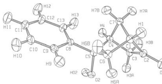
Fig. 17.2.3.1. ORTEP plot of phenylhydroxynorbornanone showing atomic thermal ellipsoids (from Thermal ellipsoid analysis: the fossil footprints of restless atoms , by Carroll K. Johnson and Michael N. Burnett, Buerger Award Lecture at the ACA meeting in St. Louis, July 20–26, 1997).
