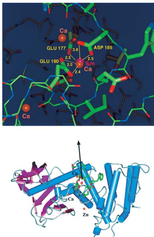
Fig. 12.1.6.1. The displacement of calcium by samarium in thermolysin. The samarium of the heavy-atom derivative is shown superposed on the parent crystal structure.
