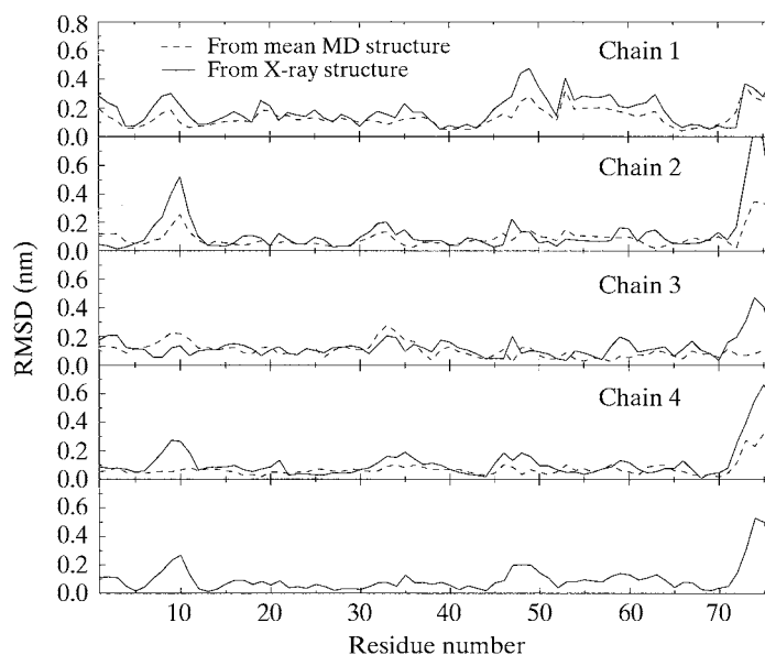
Fig. 20.1.3.3. Root-mean-square C \alpha -atom-position deviation (RMSD) in nm from a reference structure as a function of the residue number using the final 1.6 ns of the simulation. RMSDs of the four protein molecules in the unit cell from the mean molecular-dynamics structure (dashed line) and from the X-ray structure (solid line) are shown in the first four graphs. The bottom graph shows the RMSD of the mean (over the four molecules) MD structure from the X-ray structure.
