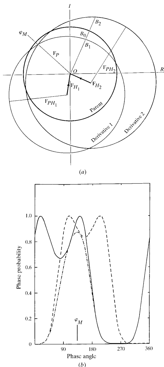
Fig. 14.1.3.1. (a) Harker construction for a double isomorphous replacement. \varphi_M is the 'most probable' phase for F_P . (b) Phase probability distribution corresponding to the double isomorphous replacement shown in part (a). The curve for derivative 1 is solid, that for derivative 2 is dashed, and that for the combined distribution is drawn as a dotted-and-dashed line.
