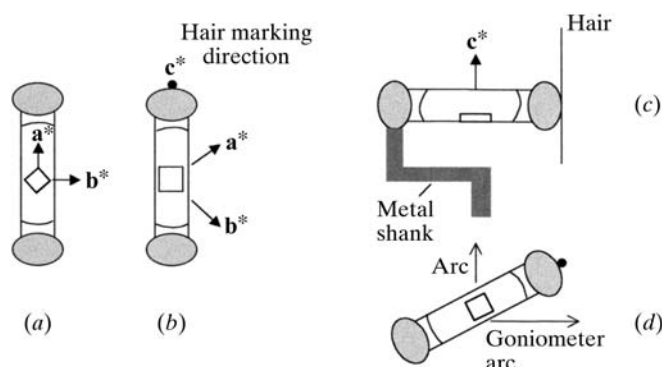
Fig. 26.1.2.5. Crystal mounting. (a) Rotation about the a^* axis; (b) rotation about [110] , preliminary to c^* mounting; (c) rotation about the c^* axis (elevation); and (d) rotation about the c^* axis (plan).
