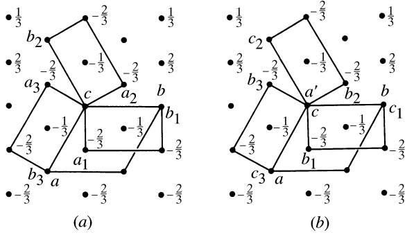
Fig. 5.1.3.9. Rhombohedral lattice with a triple hexagonal unit cell a, b, c in obverse setting (i.e. unit cell a_1, b_1, c in Fig. 5.1.3.6c) and the three centred monoclinic cells. (a) C-centred cells C_1 with a_1, b_1, c ; C_2 with a_2, b_2, c ; and C_3 with a_3, b_3, c . The unique monoclinic axes are b_1, b_2 and b_3 , respectively. Origin for all four cells is the same. (b) A-centred cells A_1 with a', b_1, c_1 ; A_2 with a', b_2, c_2 ; and A_3 with a', b_3, c_3 . The unique monoclinic axes are c_1, c_2 and c_3 , respectively. Origin for all four cells is the same.
