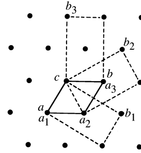
Fig. 5.1.3.7. Hexagonal lattice projected along [00\bar{1}] . Primitive hexagonal cell P with a, b, c and the three C -centred (orthohexagonal) cells a_1, b_1, c ; a_2, b_2, c ; a_3, b_3, c . Origin for all cells is the same.
