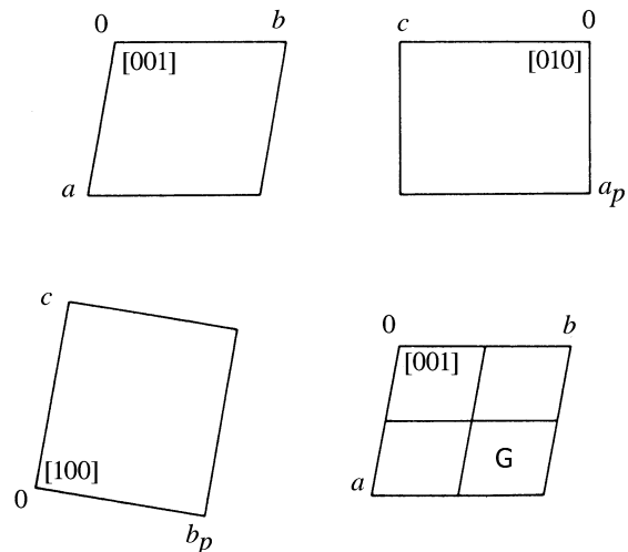
Fig. 2.2.6.3. Monoclinic space groups, setting with unique axis c .
