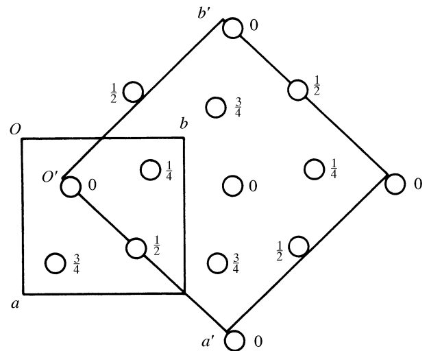
Fig. 5.2.3.1. Positions of silicon atoms in the low-cristobalite structure, projected along [00\bar{1}] . Primitive tetragonal cell a, b, c ; C-centred tetragonal cell a', b', c' . Shift of origin from O to O' by the vector \mathbf{p} = \frac{1}{4}\mathbf{a} + \frac{1}{4}\mathbf{b} .
