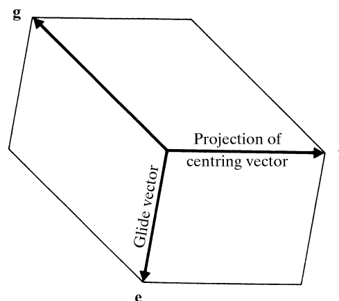
Fig. 2.2.16.1. The three primitive two-dimensional cells which are spanned by the shortest three translation vectors e , f , g in the monoclinic plane. For the present discussion, the glide vector is considered to be along e and the projection of the centring vector along f .
