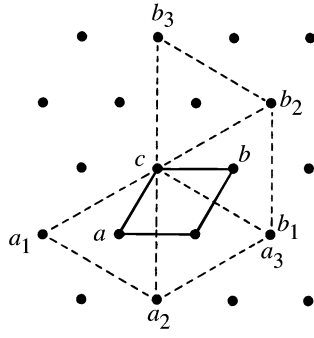
Fig. 5.1.3.8. Hexagonal lattice projected along [00\bar{1}] . Primitive hexagonal cell P with a, b, c and the three triple hexagonal cells H with a_1, b_1, c ; a_2, b_2, c ; a_3, b_3, c . Origin for all cells is the same.
