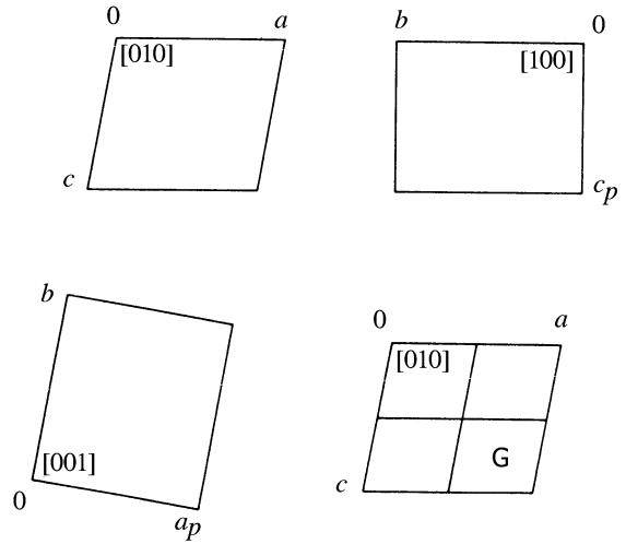
Fig. 2.2.6.2. Monoclinic space groups, setting with unique axis b (G = general-position diagram).
