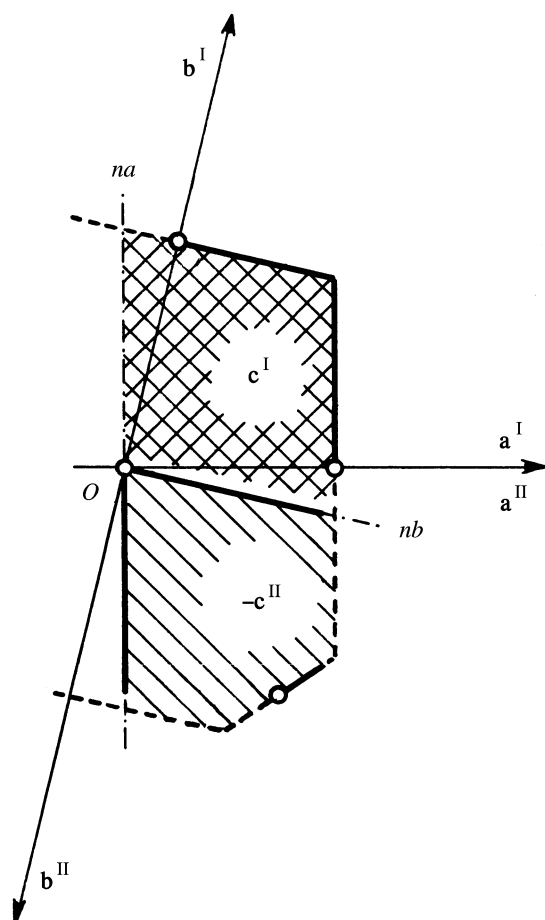
Fig. 9.2.4.3. The effect of the special conditions. Border lines of type-I and type-II regions are drawn as heavy lines if included. Type-I and type-II regions are marked as in Fig. 9.2.4.1. n_b belongs to the type-II region. A heavy border line of a region stops short of an end point if the latter is not included in the region to which the border belongs. a , b net oblique; special conditions (9.2.2.3c), (9.2.2.3d), (9.2.2.5f).
