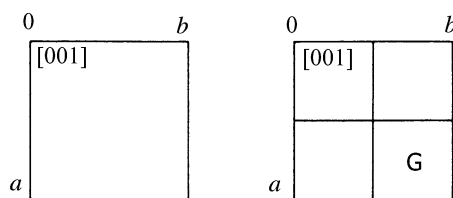
Fig. 2.2.6.7. Tetragonal space groups (G = general-position diagram).
