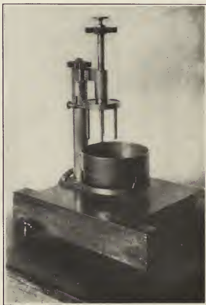
FIGURE 2. — LABORATORY MIXER.
