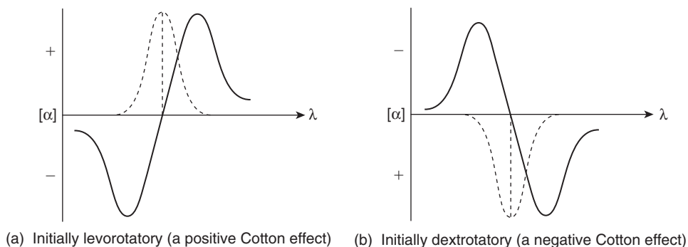
■ FIGURE 16.6 Variation of optical rotation with wavelength in the region of a hypothetical absorption band (shown as the dashed line).
