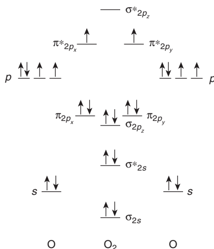
■ FIGURE 13.10 Molecular orbital diagram for the \text{O}_2 molecule.
