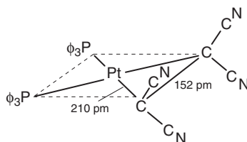
■ FIGURE 21.9 The structure of [\text{Pt}(\text{P}\phi_3)_2\text{C}_2(\text{CN})_4] (where \phi = \text{C}_6\text{H}_5 ).
