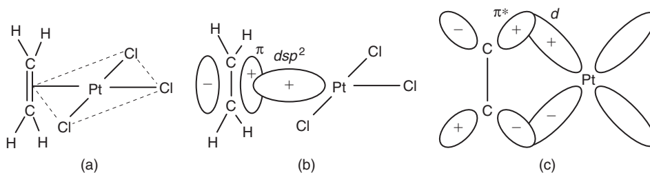
■ FIGURE 16.10 The structure and bonding in the anion of Zeise's salt. A \sigma -bond results from the overlap of a dsp^2 hybrid orbital on the metal and the \pi orbital on ethylene. Back donation from a d orbital on the metal to the \pi^* orbital on ethylene gives some \pi bonding (shown in (c)).
