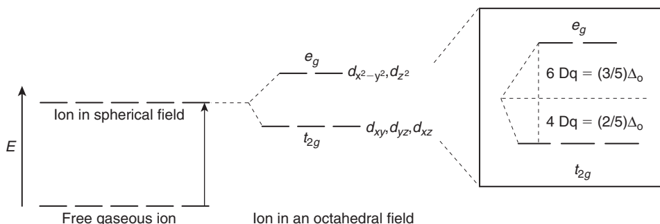
■ FIGURE 17.3 Splitting of the d orbitals in a crystal field of octahedral symmetry.
