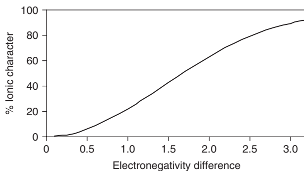
■ FIGURE 3.10 The variation in percent ionic character to a bond and the difference in the electronegativities of the atoms.
