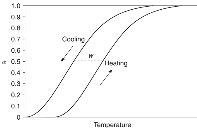
■ FIGURE 8.5 The thermal hysteresis that occurs when the rate of the phase change on cooling is lower than that on heating at the same temperature.
