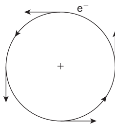
■ FIGURE 1.6 As the electron moves around the nucleus, it is constantly changing direction.
