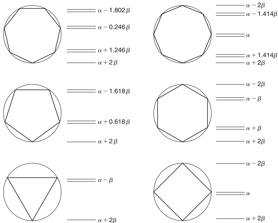
■ FIGURE 5.20 Frost–Musulin diagrams for cyclic systems having 3-, 4-, 5-, 6-, 7-, and 8-membered rings.
