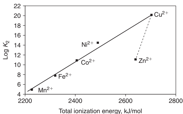
■ FIGURE 19.6 Variation in \ln K_2 for M(en)_3^{2+} complexes with total ionization potential of the metal.
