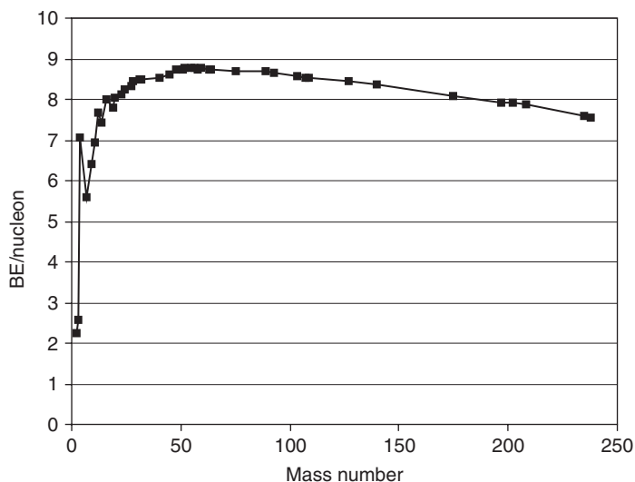
■ FIGURE 1.12 The average binding energy per nucleon as a function of mass number.
