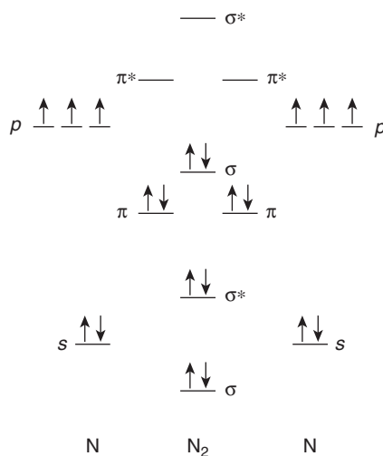
■ FIGURE 14.3 The molecular orbital diagram for the \text{N}_2 molecule.
