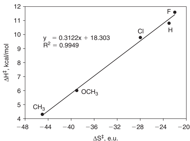
■ FIGURE 22.4 An isokinetic plot for the reaction of \text{trans-}[\text{IrCl}(\text{CO})\text{P}(\text{p-C}_6\text{H}_4\text{Y})_3]_2 . The identity of Y is indicated for each point on the graph. (Constructed from data given in Atwood, 1985, p. 168.)
