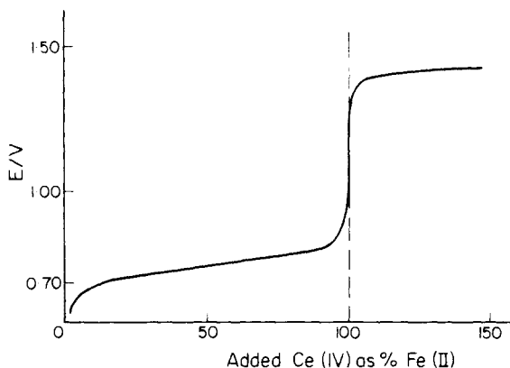
Figure 4.7. Potentiometric titration of \text{Fe(II)} with \text{Ce(IV)}
