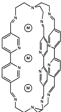
The crystal structure of the \text{M} = \text{Ag}^+ species with this ligand has been determined
