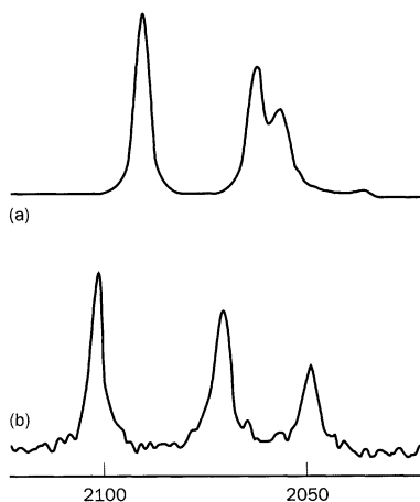
Fig. 12.3 The Raman spectra of crystalline samples of (a) K_4[Fe(CN)_6] and (b) Na_4[Fe(CN)_6] . This figure illustrates several of the points made in the text. In the [Fe(CN)_6] anion the \nu(C\equiv N) vibrations are coupled. The higher frequency bands in both spectra are the A_{1g} (totally symmetric, 'breathing' mode) and the lower E_g , the components of which are split apart. This latter splitting—and all the frequency differences between the two spectra—show the importance of solid-state effects, in which they originate. (Adapted and reproduced with permission from T. N. Day, P. J. Hendra, A. J. Rest and A. J. Rowlands, Spectrochim. Acta A (1991) 47A, 1251).
