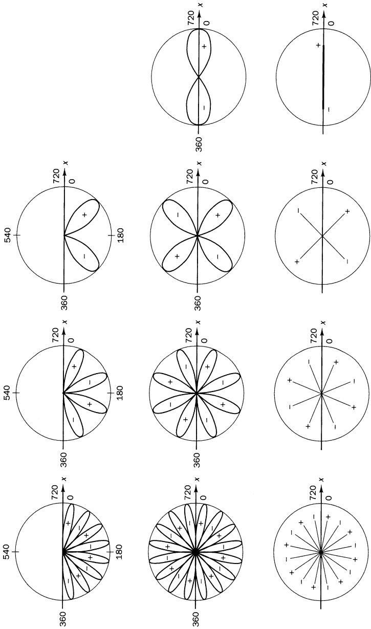
Fig. 11.6 The identity operation = 720° representation of the orbitals of Fig. 11.5, together with the spin = 1/2 function.
