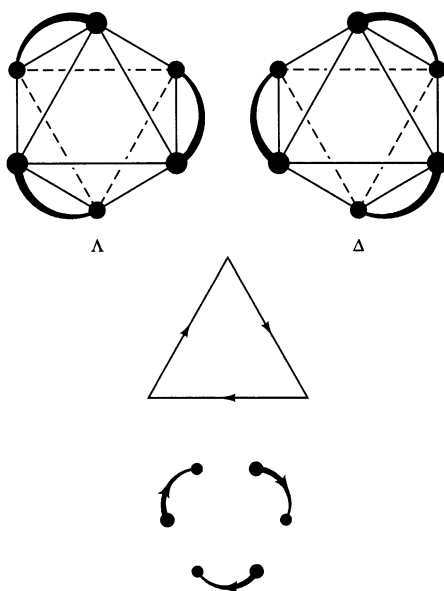
Fig. A1.3 The \Lambda and \Delta configurations of three chelate rings in an octahedral complex.
