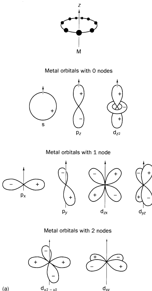
Fig. 10.2 A classification of orbitals according to the number of their nodal planes which contain the z axis for metal and planar cyclic C_n , R_n systems. The z axis is the axis of highest rotational symmetry (top).
