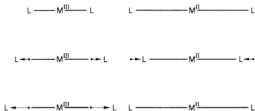
Fig. 14.2 For simplicity, this figure shows two centrosymmetric \text{ML}_2 molecules. The \text{M}^{\text{III}}\text{--L} (top left) is drawn much shorter than the \text{M}^{\text{II}}\text{--L} (top right). By appropriate totally symmetric (breathing) M–L extensions or contractions the two molecules become of identical size (centre). The totally symmetric mode can involve just one molecule but then the amplitude is greater (bottom). Evidently, a continuous range of matching bond lengths exists.
