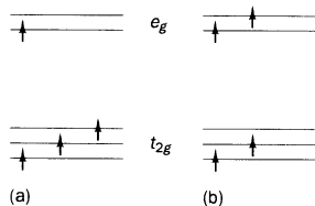
Fig. 7.12 (a) Ground and (b) an excited state with the same spin multiplicity, derived from the d^4 configuration in an octahedral crystal field. In the ground state there is a hole in the e_g orbitals; in the excited state the hole is in the t_{2g} orbitals.
