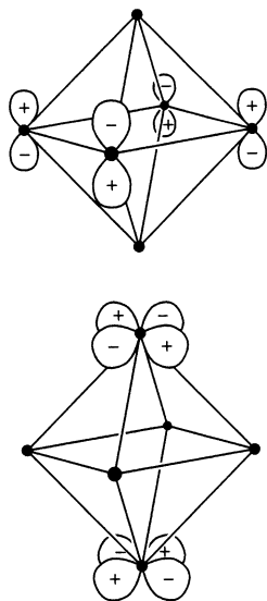
Fig. 15.24 The T_{20} combinations of \pi - and \delta -type functions that are shown as interacting in Fig. 15.23. Note that, for simplicity, the \pi -type function shown is p_{x_i} ; in fact, a d_{xy} is the one involved in Fig. 15.23.
