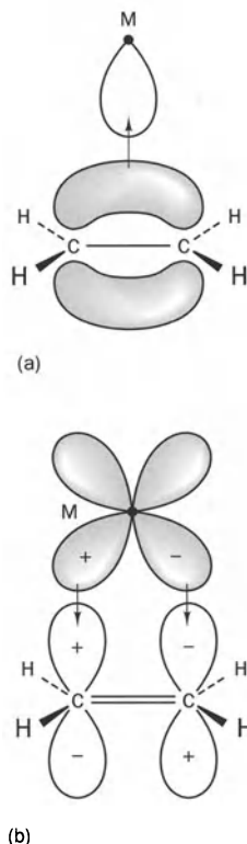
Fig. 2.2 (a) The \sigma donation \text{C}_2\text{H}_4 \pi \rightarrow \text{metal} empty orbital. (b) The \pi back-donation \text{metal} \rightarrow \text{C}_2\text{H}_4 \pi^* antibonding orbital.
