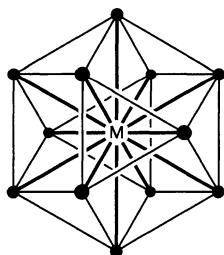
Fig. 3.24 There are several modes of 12-coordination, all of high symmetry (although no complex containing the twelve monodentate ligands needed to give these symmetries is known). That shown is the cuboctahedron ( O_h ). It is best known as the cubic close packing arrangement in metals. The solid figure may be regarded as derived from the octahedron (Fig. 3.12). The equilateral triangular face evident in the cuboctahedron is derived from a face of the parent octahedron, but is smaller. This is because a square face has been obtained by cutting the solid octahedron perpendicular to each fourfold axis to give the cuboctahedron. This has the effect of removing the corners of the octahedron face, so that the corners of the triangular faces of the cuboctahedron are at the mid-points of faces of the parent octahedron.
