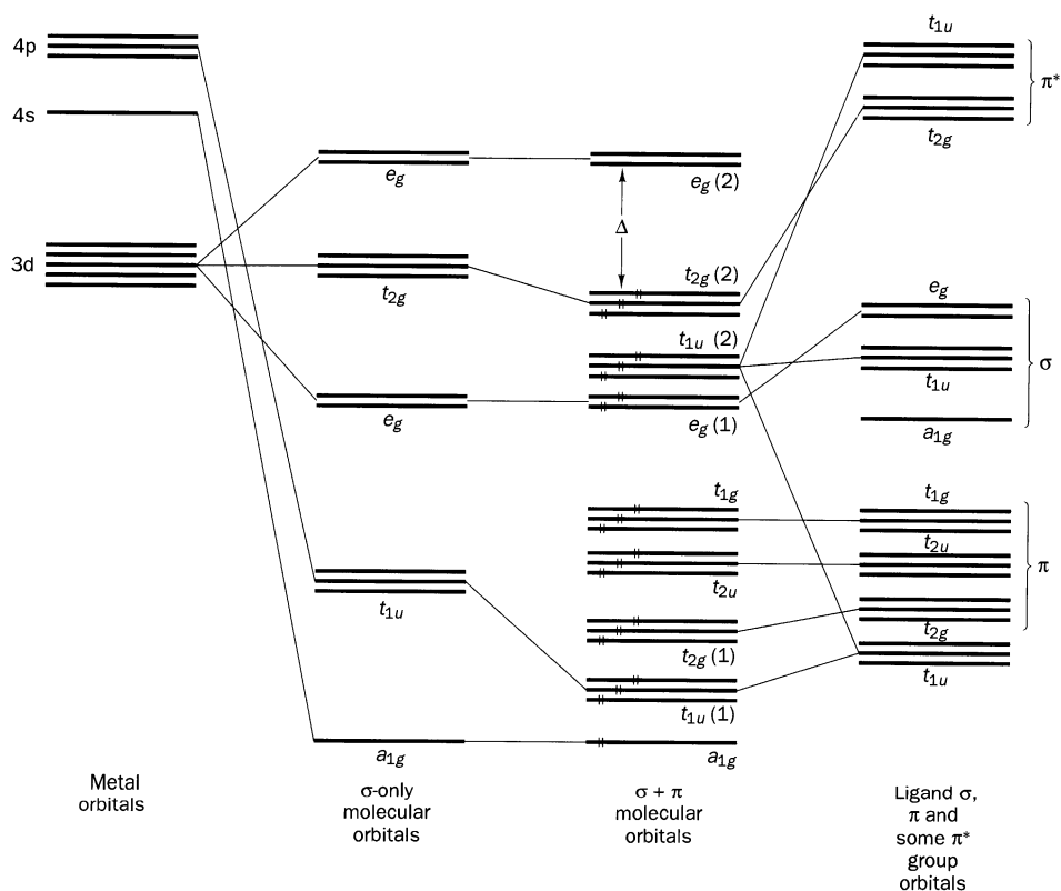
Fig. 10.5 A qualitative \sigma + \pi bonding molecular orbital energy level diagram for \text{Cr(CO)}_6 based on Figs. 6.11 and 6.16(c) together with the associated discussion. This schematic diagram may be compared with Fig. 10.10 which is a more accurate molecular energy level diagram for \text{Cr(CO)}_6 .
