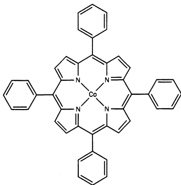
The \text{Co}^{\text{II}} complex of tpp: one of two equivalent structures (canonical forms) of the ligand is shown
