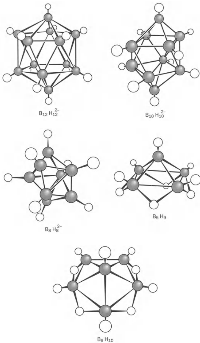
Fig. 15.12 Representative boron hydride molecules. Three are closo and two are nido .
