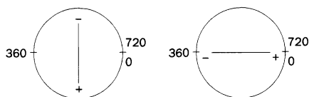
The two static functions corresponding to angular momentum = \pm \frac{1}{2}
