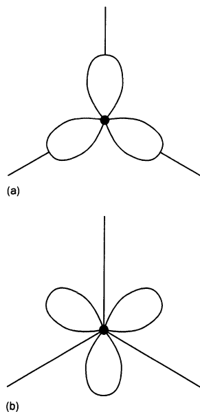
Fig. 15.5 A set of sp^2 or sp^3 hybrids viewed down a threefold axis of P_4 . They may be orientated towards (a) the tetrahedron edges or (b) faces. Although these alternatives appear rather different, they both correspond to cylindrical symmetry of electron density distribution around the threefold axis.
