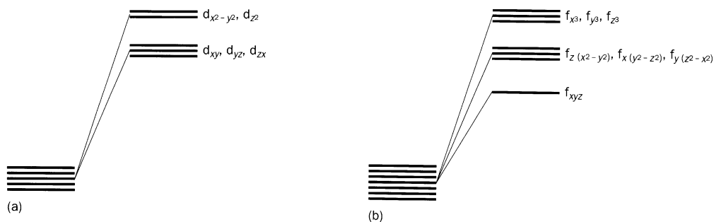
Fig. 7.8 The combined repulsive and splitting effect of an octahedral crystal field on the energies of (a) a set of metal d orbitals and (b) a set of f orbitals.
