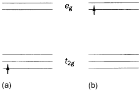
Fig. 7.11 (a) Ground and (b) excited states derived from the d^1 configuration in an octahedral crystal field.
