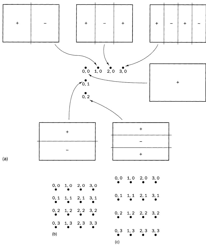
Fig. 17.5 (a) Some of the nodal patterns of the two-dimensional crystal of Fig. 17.3 with all nodes perpendicular to either x or y , together with a dot-map representation of them. (b) The dot map of Fig. 17.5(a) extended to include nodal patterns inclined to x and y . (c) Figure 17.5(b) corrected for the fact that the magnitude of the translation along y is 1.5 times that along x in Fig. 17.3. Here, the separations are in the inverse ratio, 0.67:1.
