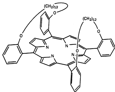
A basket-handle porphyrin
