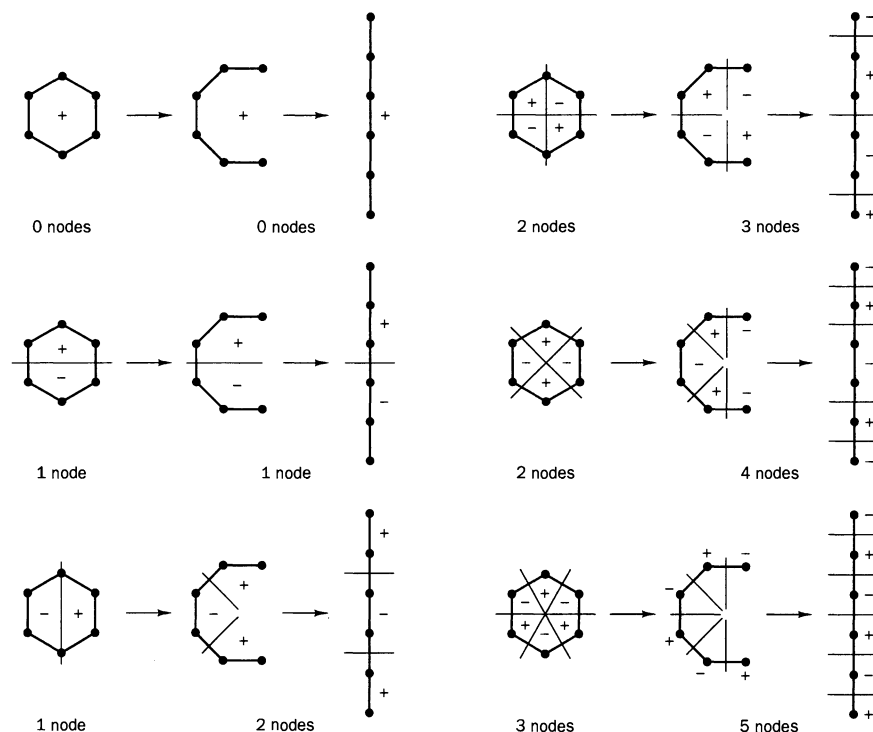
Fig. 17.2 On the left are shown the nodal patterns of the six molecular orbitals of benzene (they are shown in more detail in Fig. 17.6). These patterns carry over into the diradical generated when a C–C bond is broken (centre) and thus into the linear structure (right). The actual numbers of nodes in the initial and final patterns should be compared.
