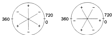
The two static functions corresponding to angular momentum = \pm \frac{3}{2}
