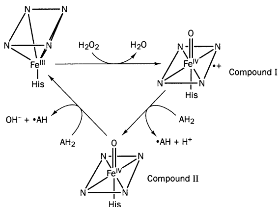
Fig. 16.14 The current view of the catalytic cycle in which peroxidase (top left-hand) is oxidized by hydrogen peroxide to give compound I. This oxidizes the substrate \text{AH}_2 to give \text{AH}^\bullet (dots indicate free radicals), \text{H}^+ and compound II. This similarly oxidizes more substrate to regenerate the starting material (His = histidine).
