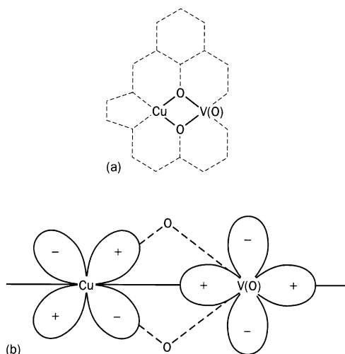
Fig. 9.10 (a) A \text{Cu}^{\text{II}}\text{-VO} complex showing ferromagnetic interaction between the copper and vanadyl ions. The ligand skeleton which holds the two ions together is shown dotted. (b) On the d^9 ion \text{Cu}^{2+} an unpaired electron is in an e_g type of orbital; on the d^1 ion \text{VO}^{2+} an unpaired electron is in a t_{2g} type of orbital. These orbitals are, respectively, antisymmetric and symmetric with respect to the vertical mirror plane shown as a solid line, and are therefore orthogonal.
