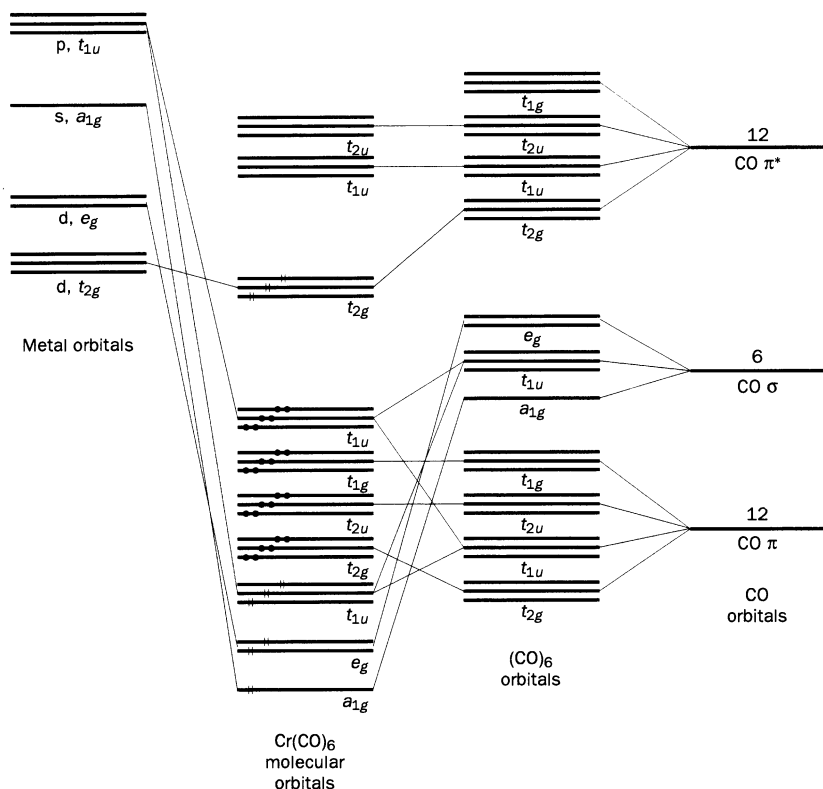
Fig. 10.10 Schematic X\alpha molecular orbital energy level diagram for \text{Cr(CO)}_6 (data from R. Arratia-Perez and C. Y. Yang, J. Chem. Phys. (1985) 83, 4005). Electrons which would be counted in an application of the 18-electron rule are shown as lines, those that would be excluded are shown as dots.
