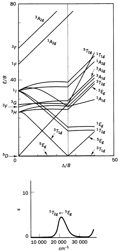
Fig. A7.3 d^4 ; \gamma = 4.61 and the spectrum of [\text{Mn}(\text{H}_2\text{O})_6]^{3+} .
