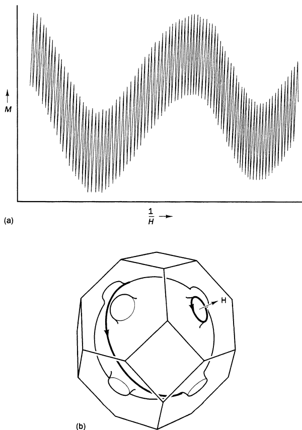
Fig. 17.18 (a) The de Haas-van Alphen oscillations in metallic copper when the magnetic field is orientated as indicated as shown in (b). The two periods of oscillation may be correlated with the concurrent existence of the two different circulatory pathways shown. A different orientation of the crystal with respect to the magnetic field would lead to a different oscillation pattern and thus provide information on the topology of the Fermi surface (adapted from Ashcroft and Mermin).
