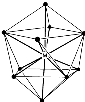
Fig. 3.22 One mode of 10-coordination—the bicapped square antiprism ( D_{4d} ). The two capping ligands are those at the top and bottom of the diagram. At the present time no complex is known which contains ten monodentate ligands.
