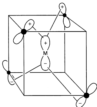
Fig. 6.25 A ligand \pi group orbital of T_2 symmetry together with the metal p_2 with which it overlaps. The dominant orbital overlaps are indicated. The form of this ligand group orbital is particularly simple for the reason given in the caption to Fig. 6.24. Note carefully the phases of the overlap—they are not incorrect!
