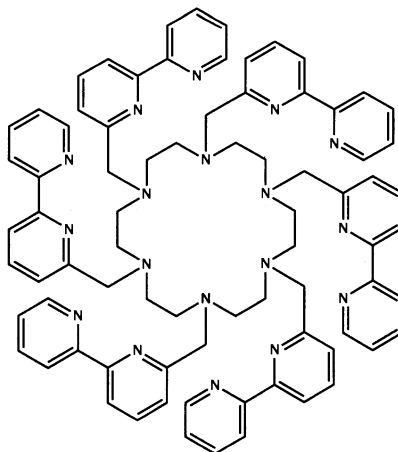
Bipyrilid groups grafted onto a cyclic hexamine
