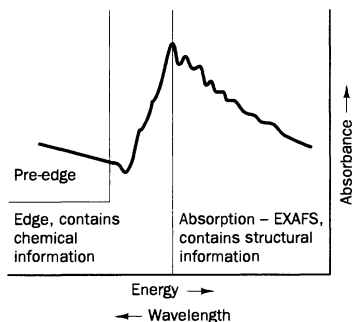
Fig. 16.8 The absorption of white X-rays at a wavelength chosen because it is one characteristic of the element one wishes to study. The fine details contain useful information.
