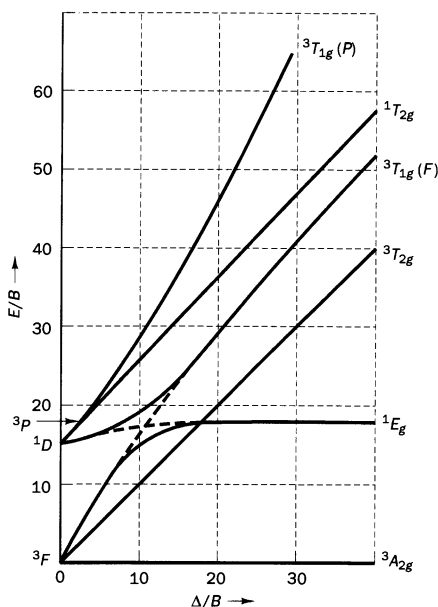
Fig. 8.16 Spin-orbit coupling causes an interaction between the {}^1E_g low-lying excited state of an octahedral d^8 complex with two of the wavefunctions of a {}^3T_{1g} . This interaction leads to mutual repulsion and a non-crossing of the energy levels.
