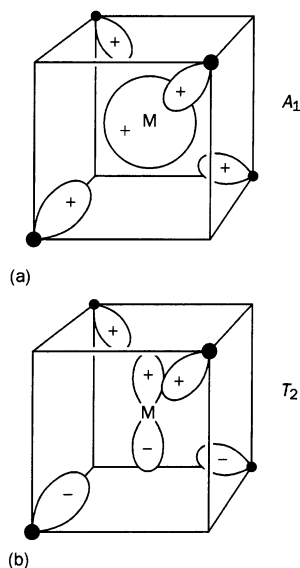
Fig. 6.20 (a) Interaction of the ligand a_1 group orbital of Table 6.3 with the metal s orbital. (b) Interaction of the first ligand t_2 \sigma group orbital listed in Table 6.4 with the corresponding metal p orbital.
