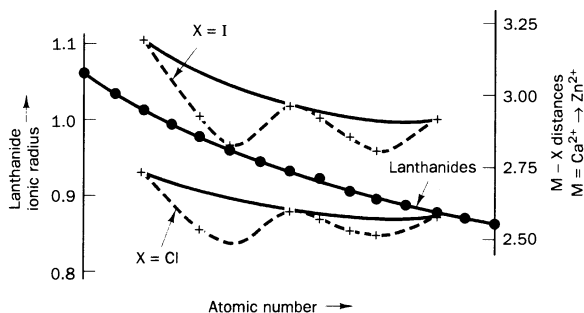
Fig. 13.1 The lanthanide contraction and metal-halogen distances for divalent first-row transition and related metal ions. The thin solid lines indicate the probable values for the M-X distances corrected for crystal field effects.
