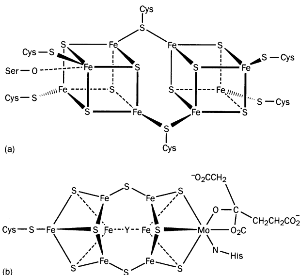
Fig. 16.20 (a) The structure of the FeMo cofactor \text{Fe}_7\text{Mo} cluster in nitrogenase. (b) The structure of the so-called P-cluster ( \text{Fe}_7\text{Mo} ) in nitrogenase (the identity of Y is not known).
