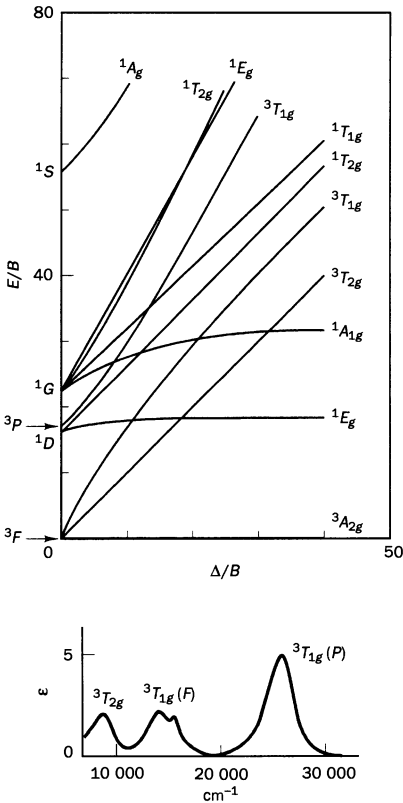
Fig. A7.7 d^8 ; \gamma = 4.71 and the spectrum of [\text{Ni}(\text{H}_2\text{O})_6]^{2+} .
