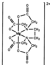
The \text{Mg}^{2+} EDTA complex
