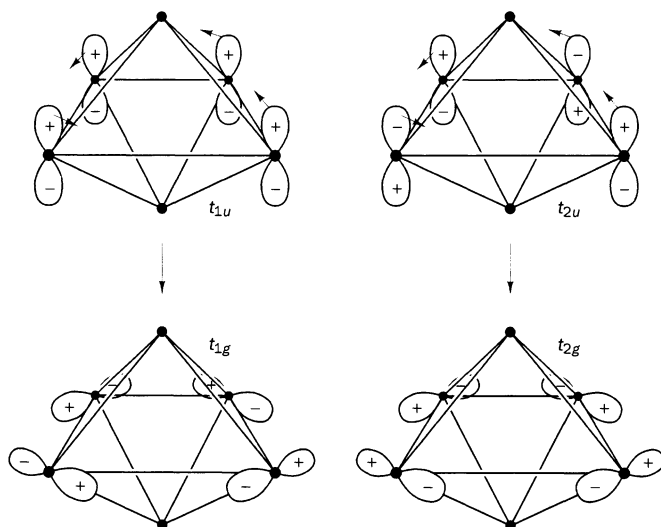
Fig. 15.18 Rotation in the same sense by 90^\circ (indicated by small arrows in the upper diagrams) converts a (bonding) t_{1u} combination into an (antibonding) t_{1g} . Conversely, an (antibonding) t_{2u} is rotated into a (bonding) t_{2g} .
