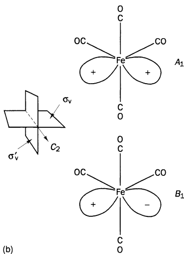
Fig. 10.13 (a) The \text{Fe}(\text{CO})_4 unit regarded as a fragment of an octahedron (drawn from the same viewpoint as Fig. 10.12). The Fe orbitals required to complete the octahedron are shown. (b) The A_1 and B_1 combinations of the octahedron-completing Fe orbitals. The symmetry elements of the C_{2v} point group are shown inset. The orbital combinations are drawn from a viewpoint lying in the \sigma_v mirror plane.
