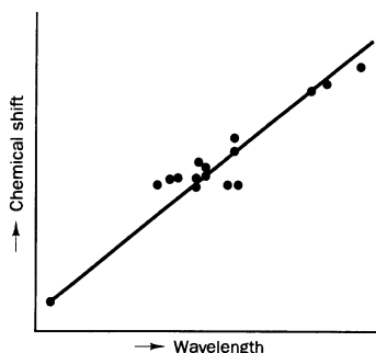
Fig. 12.15 The ^{59}\text{Co} chemical shifts shown by cobalt(III) complexes plotted against the wavelength of the corresponding ^1T_{1g} \leftarrow ^1A_{1g} electronic transition.
