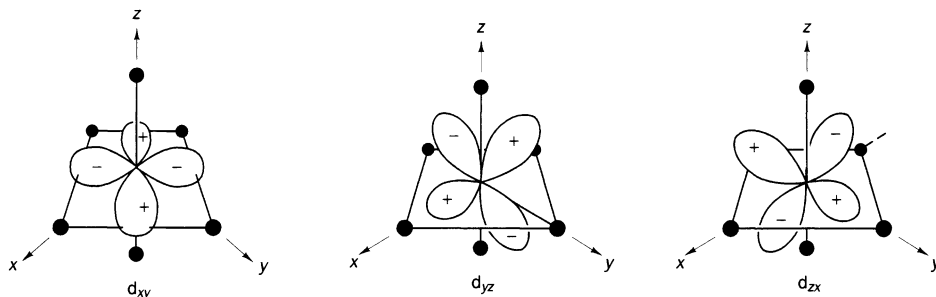
Fig. 7.4 The d_{xy} , d_{yz} and d_{xz} metal orbitals in an octahedral crystal field. Because they are all equivalent (they can be interconverted by rotating around the threefold axis approximately perpendicular to the plane of the paper) they remain triply degenerate.
