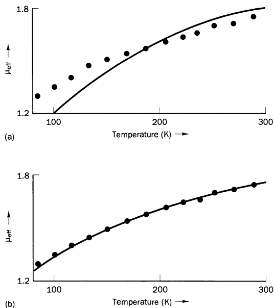
Fig. 9.4 (a) A simple Kotani plot for [\text{VCl}_6]^{2-} ( \zeta = 190 \text{ cm}^{-1} ). (b) A Kotani plot including best-fit tetragonal distortions and orbital reduction factors. In both cases experimental data are given as dots.
