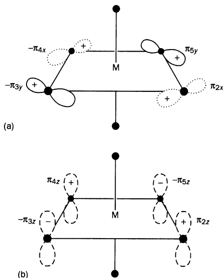
Fig. 6.13 (a) One of the three ligand \pi group orbitals of T_{1g} symmetry. Notice that of the 12 \pi ligand orbitals only four are involved in this particular combination. The remaining eight \pi ligand orbitals similarly divide into two sets of four, with no member common to any two sets. A similar pattern holds for all the other \pi combinations shown in the following figures. (b) One of the three ligand \pi group orbitals of T_{2u} symmetry. As for all other \pi combinations in adjacent figures, the combination shown is the first listed in the appropriate section of Table 6.3.
