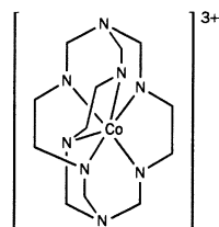
[\text{Co}(\text{sepulchrate})]^{3+}
