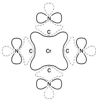
Fig. 6.31 Spin density distribution in the [\text{Cr}(\text{CN})_6]^{3-} anion in the \text{CrC}_4 plane. The solid contour defines a region of spin-up electron density and the dotted contour of spin-down. This diagram is from a model of the experimental data which over-sharpens some features so that fine detail is not reliable. Adapted and reproduced with permission from B. B. Figgis, S. B. Forsyth and P. A. Reynolds, Inorg. Chem. (1987) 26, 101.
