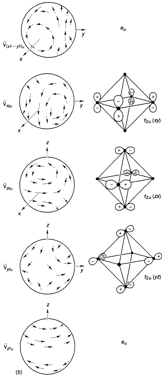
Fig. 15.21 (continued) (b) The corresponding \bar{D}_\pi(1) set of surface tensor harmonics and (right) their application to an octahedral cluster. Note the 90^\circ rotation patterns between corresponding D_\pi(1) and \bar{D}_\pi(1) functions.
