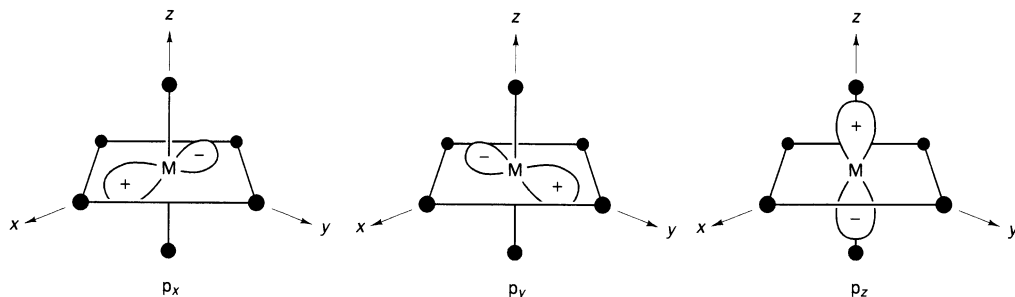
Fig. 7.3 A set of metal p orbitals in an octahedral crystal field. Because the coordinate axes of the octahedron are equivalent so too are the p orbitals. They remain triply degenerate.
