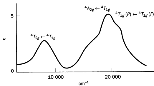
Fig. A7.6 d^7 ; \gamma = 4.63 and the spectrum of [\text{Co}(\text{H}_2\text{O})_6]^{2+} .
