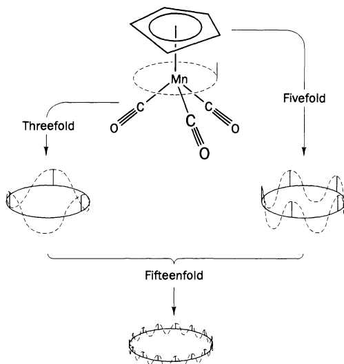
Fig. 3.27 Potential energy profiles in \eta^5\text{-C}_5\text{H}_5\text{Mn(CO)}_3 . Consider a microscopic probe, shown at the right hand side of the dotted circle surrounding the manganese atom. If the molecule is held rigid and the probe rotated around the dotted circle, the top end of the probe will experience five bumps per circuit and the bottom end will experience three. That is, the \eta^5\text{-C}_5\text{H}_5 and \text{Mn(CO)}_3 units generate fivefold and threefold potentials, respectively. Now forget the probe and consider just one carbon atom of the \text{C}_5\text{H}_5 ring as the ring is rotated against a rigid \text{Mn(CO)}_3 unit. The carbon atom will experience three bumps per circuit. So too will each of the other four carbon atoms in the \text{C}_5\text{H}_5 ring. But the geometry is such that, although all of these bumps will be equal, none will coincide. That is, in a complete circuit there will be a total of 5 \times 3 = 15 bumps, a 15-fold potential.
