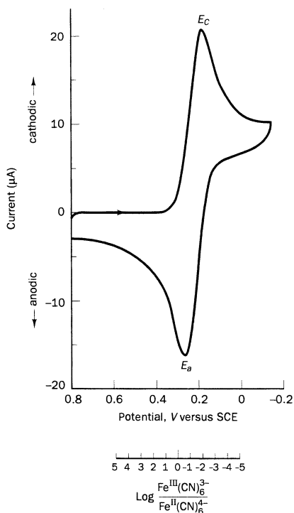
Fig. 12.25 A cyclic voltammogram of 6 mM K_3[Fe(CN)_6] in 1 M KNO_3 . Adapted and reproduced with permission from P. T. Kissinger and W. R. Heineman, J. Chem. Educ. (1983) 60, 702.
