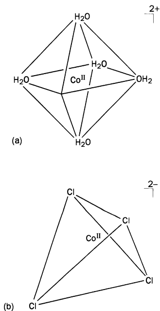
Fig. 3.5 When cobalt(II) salts dissolve in water they commonly give pale pink solutions, normally associated with the octahedral hexaqua species (a). Addition of concentrated hydrochloric acid gives a deeper, beautiful blue colour, 'cobalt blue', normally associated with the tetrahedral tetrachloro species (b). In fact, the colours are perhaps more associated with the two different geometries than ligands—replacing an \text{H}_2\text{O} by \text{Cl}^- in (a), for example, does not greatly change the observed colour of the solution.
