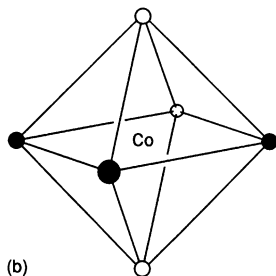
Fig. 3.3 (a) The complex (OC-6-22)-triamminotrininitrocobalt(III)—this is commonly referred to as the fac (facial) isomer, i.e. fac -triamminotrininitrocobalt(III). (b) The complex (OC-6-21)-triamminotrininitrocobalt(III)—this isomer is commonly referred to as the mer (meridional) isomer.
