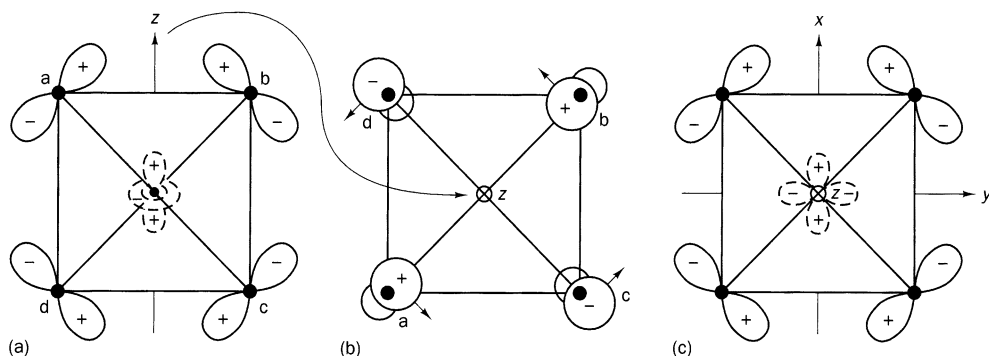
Fig. 15.19 (a) An e orbital combination which transforms like the d_{z^2} of a (hypothetical) atom at the centre of the tetrahedron. It is viewed perpendicular to the z axis. (b) The same combination but viewed along z . The direction of rotation (see the text) is indicated by small arrows. This rotation, by 90^\circ , gives (c), a combination which transforms as d_{x^2-y^2} of an atom at the centre of the tetrahedron.
