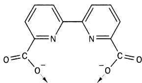
Fig. 13.7 The 2,2'-bipyridine-6,6'-dicarboxylate anion.
