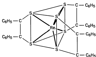
Fig. 3.13 An example of a molecule showing the trigonal prismatic mode of six-coordinate.
