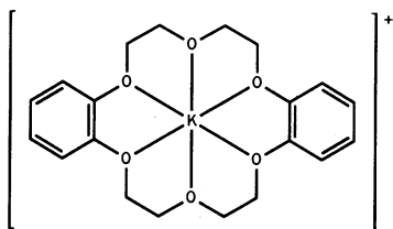
The \text{K}^+ complex of dibenzo-18-crown-6
