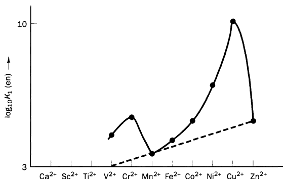
Fig. 13.4 Variation of \log_{10} K_1 across the first transition series for the reaction [\text{M}(\text{H}_2\text{O})_6]^{2+} + \text{en} \rightarrow [\text{M}(\text{H}_2\text{O})_4(\text{en})]^{2+} + 2\text{H}_2\text{O}
