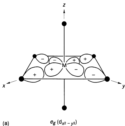
Fig. 6.10 The interaction (a) between metal d_{x^2-y^2} and (b) d_{z^2} orbitals and the corresponding ligand group orbitals.
