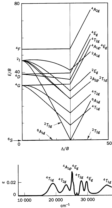
Fig. A7.4 d^5 ; \gamma = 4.48 and the spectrum of [\text{Mn}(\text{H}_2\text{O})_6]^{2+} (the ground state for all the transitions in the spectrum is 6A_{1g} ).
