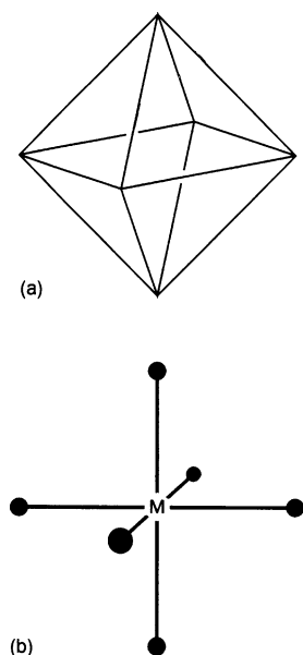
Fig. 6.1 (a) An octahedron. (b) An octahedral complex. The perspective adopted here is the same as that for (a), and was chosen to make (a) as easy as possible to visualize. The way that an octahedral complex is drawn will vary, the perspective adopted depending on the point under discussion.
