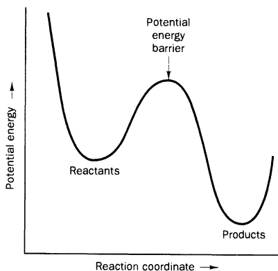
Fig. 14.6 A simple potential energy diagram relating reactants and products. The reaction coordinate can involve quite a complicated set of atomic motions, of which minor variants are admissible. It follows that this diagram is just one of a large family, of which all the acceptable variants are members.
