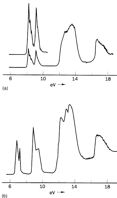
Fig. 12.24 The He I PES of (a) Mg(C 5 H 5 ) 2 and (b) Fe(C 5 H 5 ) 2 . Adapted and reproduced with permission from S. Evans, M. C. H. Green, B. Jewitt, A. F. Orchard and C. F. Pygall, J. Chem. Soc. Faraday Trans. 2 (1972) 68, 1847.
