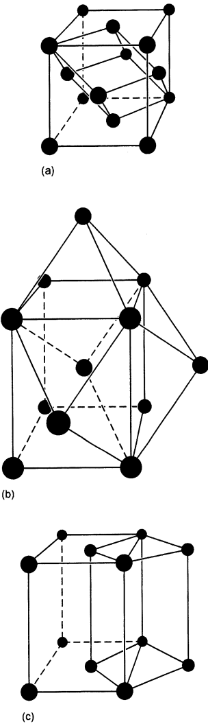
Fig. 17.1 Three centred lattices and associated primitive unit cells. The primitive is one-quarter of the volume of the face-centred cubic (a). For the body-centred tetragonal (b) and end-centred orthorhombic (c) it is one-half the volume.
