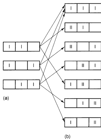
Fig. 7.22 (a) The three orbital arrangements associated with the triple orbital degeneracy of the {}^3T_{2g} ground state of the d^2 ( t_{2g}^2 ) configuration (cf. Fig. 7.15). (b) The seven different orbital arrangements corresponding to the t_{2g}^3 configuration may be derived from those of the t_{2g}^2 as indicated. It will be noticed that there are three arrows connecting with the top line of (b). One spin arrangement associated with this top line is 'all spins parallel'— {}^4A_{2g} . The other two must be spin doublets, which, together with the six below, give a total of eight spin doublet functions, corresponding to the {}^2E_g + {}^2T_{1g} + {}^2T_{2g} terms (cf. Table 7.5).
