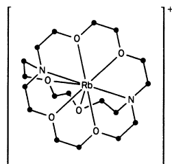
\text{Rb}^+ 2,2,2-cryptate: oxygen and nitrogen donor atoms are shown, black dots indicate \text{CH}_2 groups
