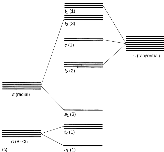
Fig. 15.10 (continued) (c) Figure 15.10(a) adapted to B_3Cl_4 , where the e(1) level is empty.
