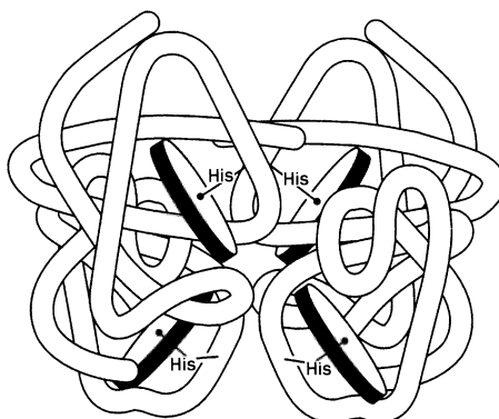
Fig. 16.2 The hemoglobin molecule; the attachment of the iron (black dots) to the protein through histidines is indicated.
