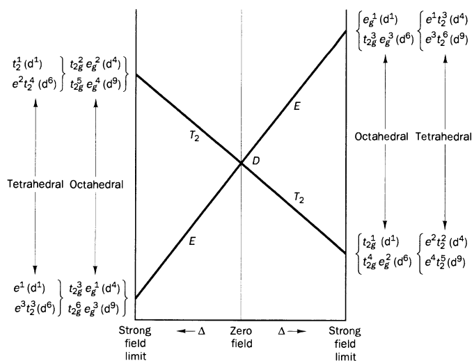
Fig. 7.23 A modified Orgel diagram for weak field complexes with free ion D terms as ground state ( d^1 , d^4 , d^6 and d^9 ).
