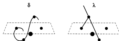
Fig. A1.2 The \lambda and \delta ring configurations.
