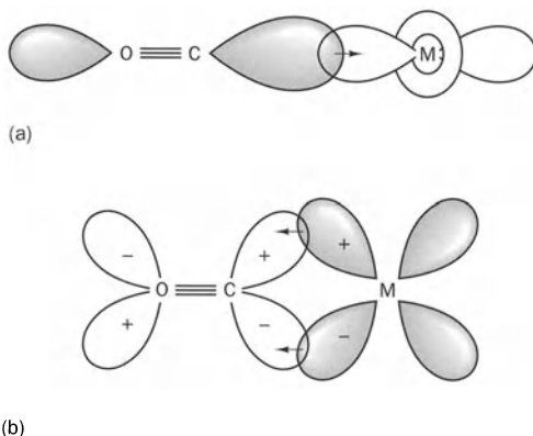
Fig. 2.1 (a) The \sigma donation \text{OC} \rightarrow \text{metal} : here, the transition metal d_{z^2} orbital is shown as the acceptor but it could be some mixture of s , p_z and d_{z^2} . Note that there is lone-pair \sigma electron density on both O and C. That on C is the larger and so has the greater overlap with the empty metal orbital. In this, and all other figures in this chapter, filled orbitals are shaded; the phases of orbitals are given explicitly. (b) The \pi back-donation \text{metal} \rightarrow \text{CO} : the metal orbital is almost pure d , the CO orbital is an empty antibonding \pi orbital. Note that for a linear triatomic OCM system there is second, equivalent, interaction to that shown above (it is like that shown but rotated 90^\circ about the OCM axis and so is located above and below the plane of the paper).
