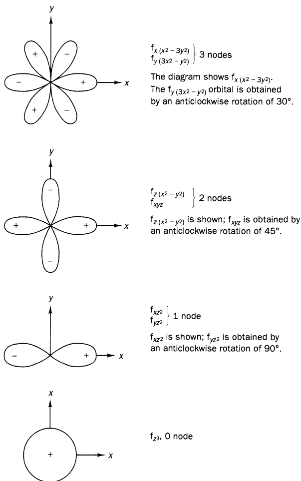
Fig. 11.4 The nodal patterns of the general set of f orbitals, viewed down the z axis (cf. Fig. 10.2(a)).
