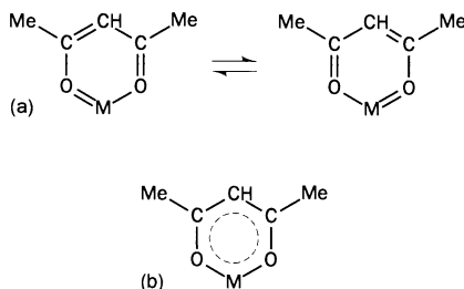
Fig. 5.4 (a) Two equivalent resonance hybrids (canonical forms) of coordinated acac. However, the conjugated nature of the system is more commonly represented as shown in (b).
