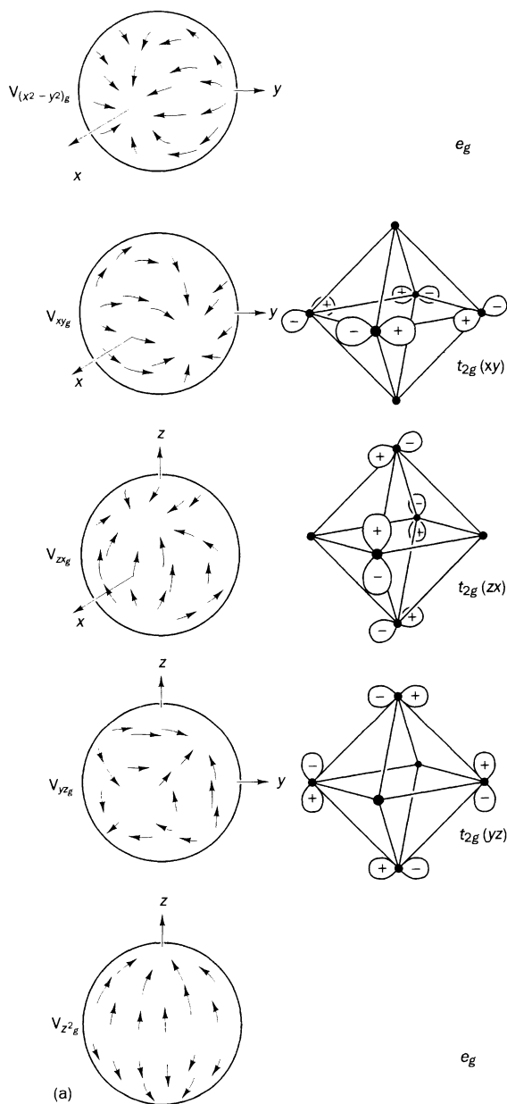
Fig. 15.21 (a) The D_{4h}(1) set of tensor surface harmonics together with, where appropriate (right) their application to an octahedral cluster.
