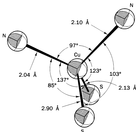
Fig. 16.17 The coordination environment of the copper in blue copper proteins.
