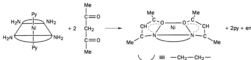
Fig. 4.8 Reaction between bisethylenediaminenickel(II) chloride and acetylacetone.
