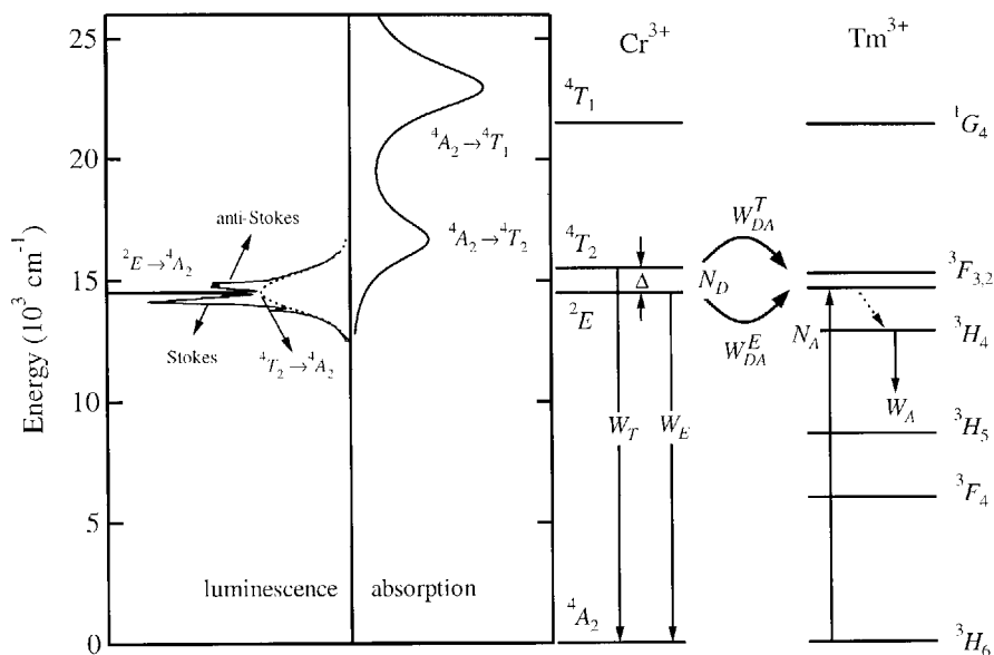
Fig. 28. Energy levels of \text{Cr}^{3+} and \text{Tm}^{3+} in \text{Y}_3\text{Al}_5\text{O}_{12} . Energy transfer occurs from the ^2\text{E} and ^4\text{T}_2 levels of the donor, \text{Cr}^{3+} , to the ^3\text{F}_2 and ^3\text{F}_3 levels of the acceptor, \text{Tm}^{3+} . W_{\text{DA}}^{\text{E}} and W_{\text{DA}}^{\text{T}} represent the rates of energy transfer from the ^4\text{T}_2 and ^2\text{E} states of \text{Cr}^{3+} , respectively. W_{\text{T}} and W_{\text{E}} are the decay rates (radiative+non-radiative) of the ^4\text{T}_2 and ^2\text{E} states of \text{Cr}^{3+} , respectively. W_{\text{A}} is the decay rate (radiative+non-radiative) of the ^3\text{H}_4 state of \text{Tm}^{3+} . The left side of the figure shows the ^4\text{T}_2 , ^2\text{E} \rightarrow ^4\text{A}_2 emission and ^4\text{A}_2 \rightarrow ^4\text{T}_2 , ^4\text{T}_1 absorption bands of \text{Cr}^{3+}
