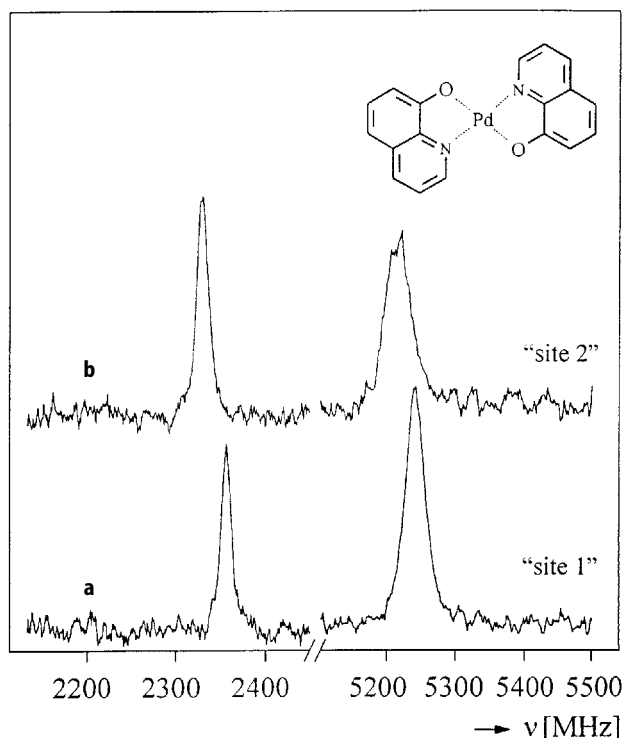
Fig. 22 a, b. Zero-field ODMR spectrum of \text{Pd}(\text{qol})_2 , in an n -octane Shpol'skii matrix, in the excited triplet state. Excitation at 457 nm, T = 1.4 K, for: a site "1", detection wavelength 621.5 nm ( 16090\text{ cm}^{-1} ); b site "2", detection wavelength 618.7 nm ( 16167\text{ cm}^{-1} )
