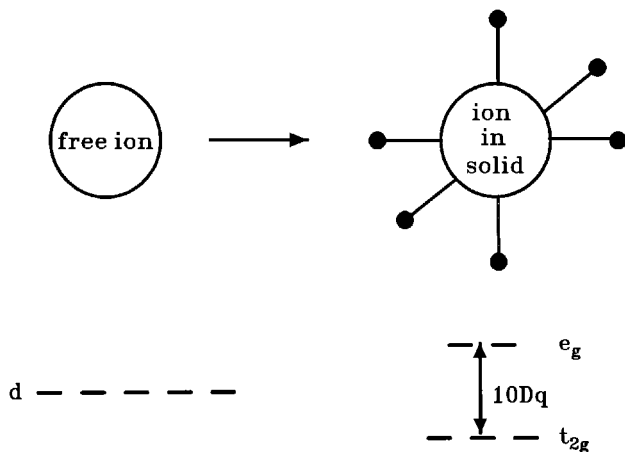
Fig. 3. Schematic depiction of the octahedral point charge crystal field model. In the free ion, the set of five d orbitals is degenerate. When the ion is placed in a solid and bonds to six nearest neighbor ligands arranged in an octahedral geometry, the d orbitals split into e_g ( d_{x^2-y^2} , d_{z^2-y^2} ) and t_{2g} ( d_{xy} , d_{yz} , d_{zx} ) subsets separated by an energy 10Dq
