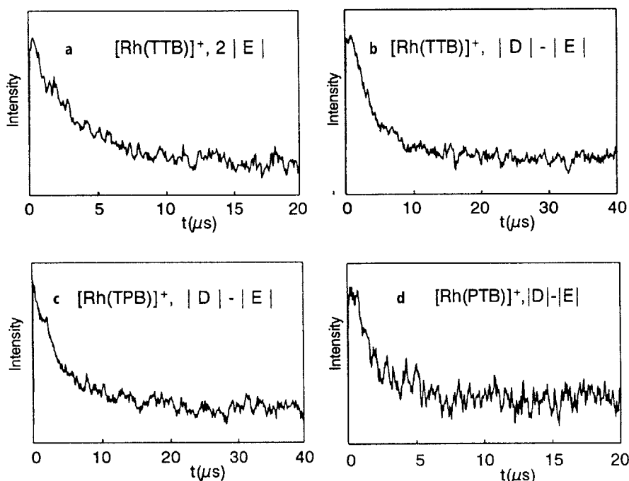
Fig. 18 a–d. Optically detected spin echo decay curves in zero magnetic field for: a the 2|E| transition at 1725 MHz of [\text{Rh}(\text{thpy})_2(\text{bpy})]^+ ; b the |D| - |E| transition at 2580 MHz of [\text{Rh}(\text{thpy})_2(\text{bpy})]^+ ; c the |D| - |E| transition at 3970 MHz of [\text{Rh}(\text{thpy})(\text{phpy})(\text{bpy})]^+ ; d the |D| - |E| transition at 1485 MHz of [\text{Rh}(\text{phpy})(\text{thpy})(\text{bpy})]
