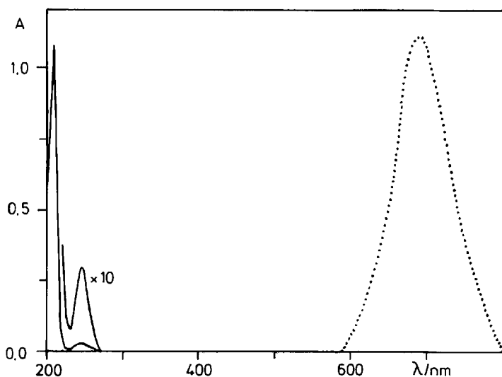
Fig. 2. Electronic absorption (continuous line) and emission (dotted line) spectra of \text{NBu}_4[\text{AuCl}_2] . Absorption: in \text{CH}_3\text{CN} , 1.64 \times 10^{-4} \text{ mol l}^{-1} , at room temperature, 1-cm cell. Emission: in \text{EtOH} , at 77 K, \lambda_{\text{exc}} = 250 \text{ nm} ; intensity in arbitrary units
