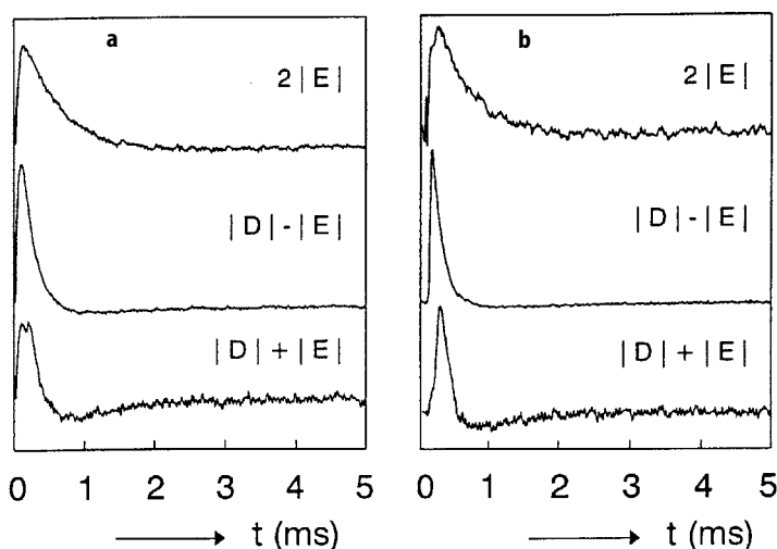
Fig. 15a,b. a Optically detected microwave recovery transients for the three zero-field ODMR transitions of [\text{Rh}(\text{thpy})_2(\text{bpy})]^+ in the excited triplet state. Detection is at 520.7 nm. b Optically detected adiabatic rapid passage transients for the three zero-field ODMR transitions of [\text{Rh}(\text{thpy})(\text{phpy})(\text{bpy})]^+ in the excited triplet state. Detection is at 519.9 nm, T = 1.4 K
