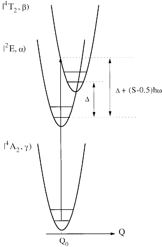
Fig. 16. Energy levels of \text{Cr}^{3+} in the context of the single configuration coordinate model. \alpha , \beta , and \gamma label the vibrational levels of the ^2E , ^4T_2 , and ^4A_2 states, respectively. \Delta is the zero phonon energy difference between the ^4T_2 and ^2E states and S is the Huang-Rhys factor
