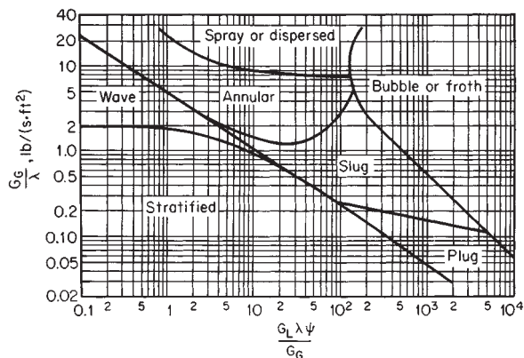
FIG. 6-25 Flow-pattern regions in cocurrent liquid/gas flow through horizontal pipes. To convert lbm/(ft 2 · s) to kg/(m 2 · s), multiply by 4.8824. (From Baker, Oil Gas J. , 53 [12], 185–190, 192, 195 [1954].)
