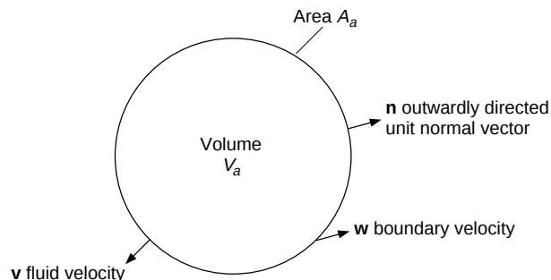
FIG. 6-3 Arbitrary control volume for application of conservation equations.
