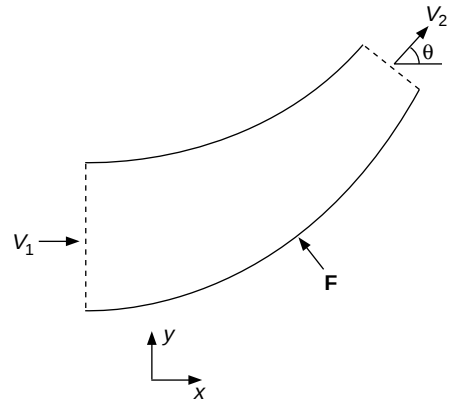
FIG. 6-5 Force at a reducing bend. \mathbf{F} is the force exerted by the bend on the fluid. The force exerted by the fluid on the bend is -\mathbf{F} .
