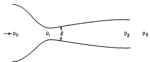
FIG. 6-23 Converging/diverging nozzle.
