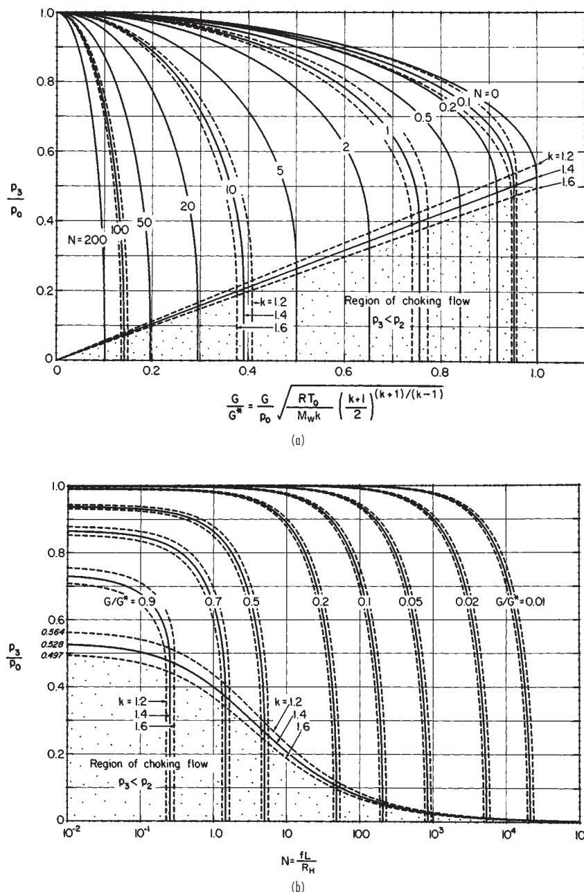
FIG. 6-21 Design charts for adiabatic flow of gases; (a) useful for finding the allowable pipe length for given flow rate; (b) useful for finding the discharge rate in a given piping system. (From Levenspiel, Am. Inst. Chem. Eng. J. , 23 , 402 [1977].)
