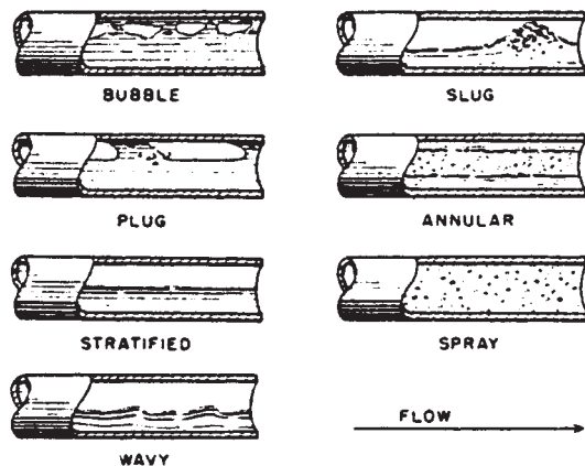
FIG. 6-24 Gas/liquid flow patterns in horizontal pipes. (From Alves, Chem. Eng. Progr. , 50 , 449–456 [1954].)
