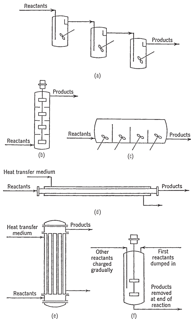
FIG. 7-4 Types of flow reactors: (a) stirred tank battery, (b) vertically staged, (c) compartmented, (d) single-jacketed tube, (e) shell and tube, (f) semibatch stirred tank.
