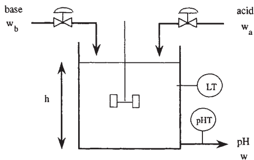
pH neutralization process
