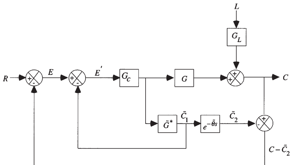
FIG. 8-37 Block diagram of the Smith predictor. The process model used in the controller is \tilde{G} = \tilde{G}^* e^{-\tilde{\theta}_s} ( \tilde{G}^* = model without delay; e^{-\tilde{\theta}_s} = time delay element).
