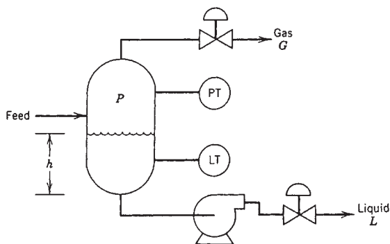
Gas liquid separator
