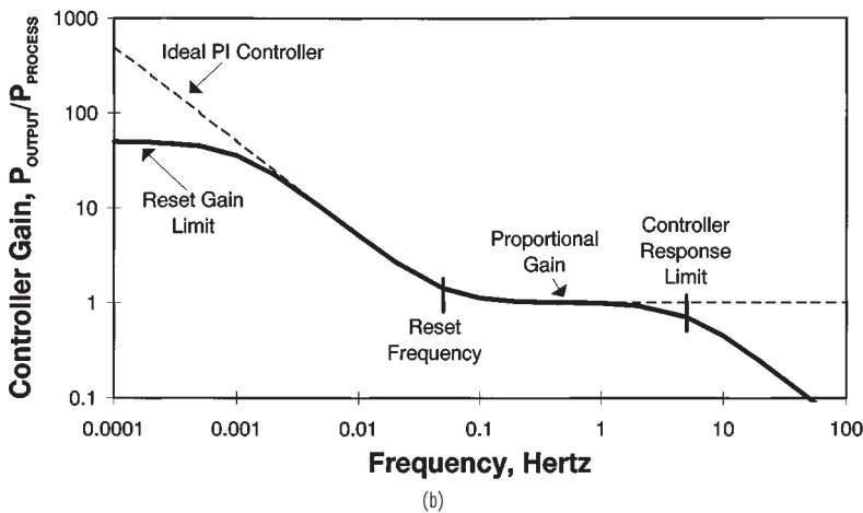
FIG. 8-64 Pneumatic controller: (a) example; (b) frequency response characteristic.
