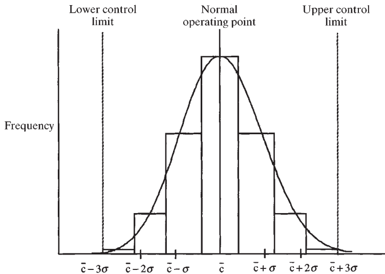
FIG. 8-38 Histogram plotting frequency of occurrence. c = mean, \sigma = rms deviation. Also shown is fit by normal probability distribution.
