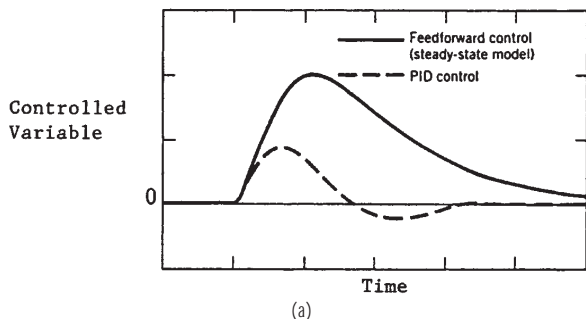
FIG. 8-33 (a) Comparison of FF (steady state model) and PID FB control for load change; (b) comparison of FF (dynamic model) and combined FF/FB control.
