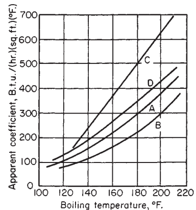
FIG. 11-27 Kerr's tests with full-sized sugar evaporators. ^{\circ}\text{C} = (^{\circ}\text{F} - 32)/1.8 ; to convert British thermal units per hour-square foot-degrees Fahrenheit to joules per square meter-second-kelvins, multiply by 5.6783.
