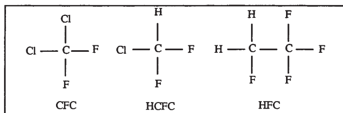
FIG. 11-109 Halocarbon refrigerants.
