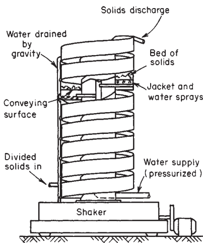
FIG. 11-63 Elevator type as heat-transfer equipment. (Courtesy of Carrier Conveyor Corp.)
