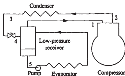
FIG. 11-77 Recirculation system.
