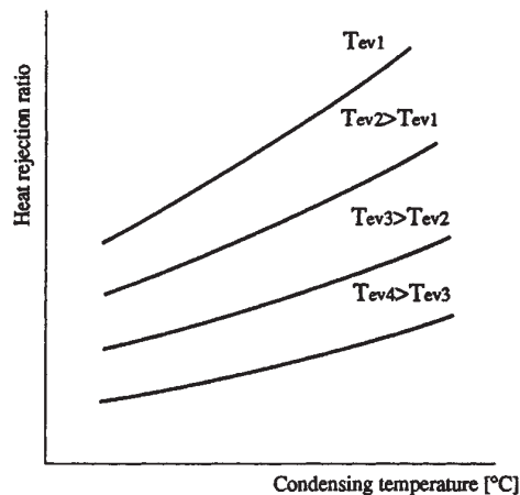
FIG. 11-94 Heat-rejection ratio.
