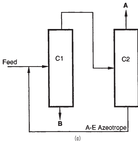
FIG. 13-64 Feasible distillation region diagrams for breaking homogeneous binary azeotrope A-B. (a) Low-boiling entrainer.
