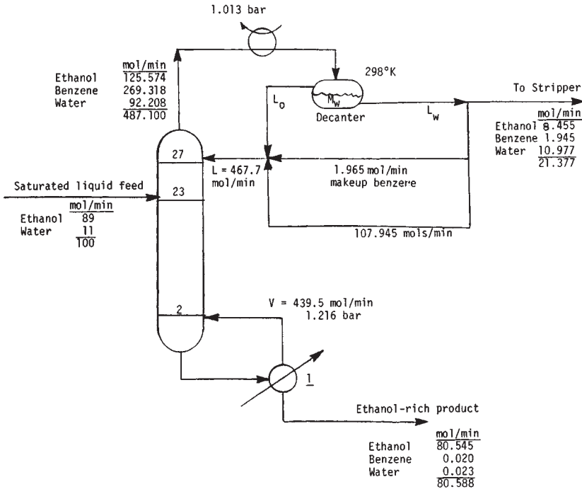
FIG. 13-108 Initial steady state for dynamic azeotropic distillation of ethanol-water with benzene.
