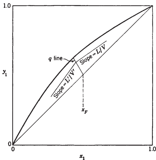
FIG. 13-31 Typical intersection of the two operating lines at the q line for a feed stage. The q line shown is for a partially flashed feed.
