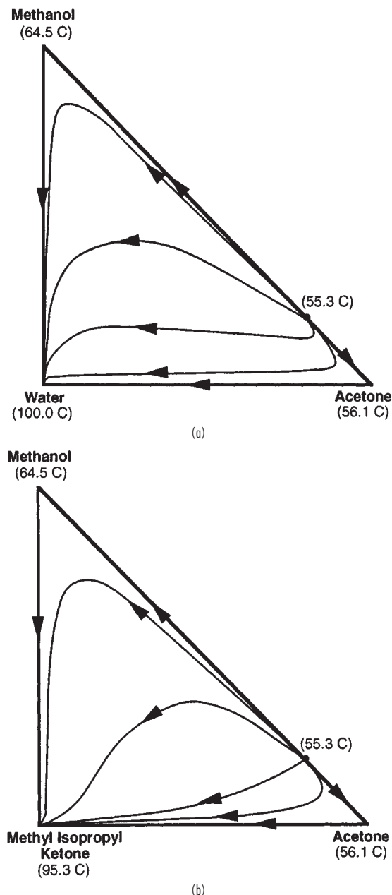
FIG. 13-73 Residue curve maps for acetone-methanol systems. (a) With water. (b) With MIPK.
