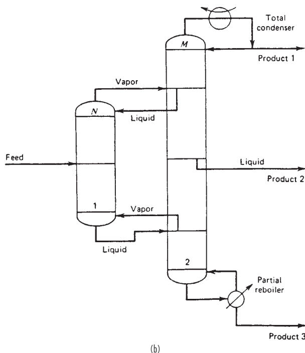
FIG. 13-6 Thermally coupled systems for separation into three products. (a) Fractionator with vapor sidestream and side-cut rectifier. (b) Petlyuk towers.
