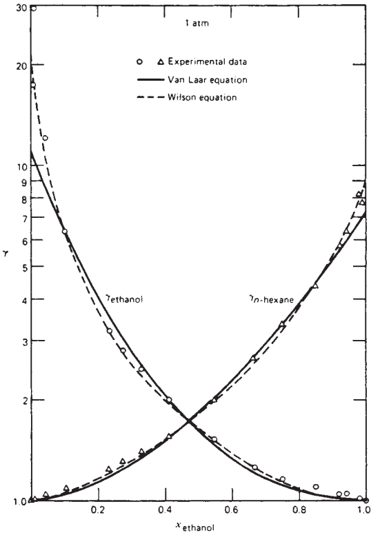
FIG. 13-20 Liquid-phase activity coefficients for an ethanol-n-hexane system. [Henley and Seader, Equilibrium-Stage Separation Operations in Chemical Engineering , Wiley, New York, 1981; data of Sinor and Weber, J. Chem. Eng. Data, 5, 243-247 (1960).]
