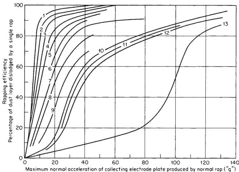
FIG. 17-73 Normal (perpendicular) rapping efficiency for various precipitated dust layers having about 0.03 \text{ g dust/cm}^2 ( 0.2 \text{ g dust/in}^2 ) as a function of maximum acceleration in multiples of g. Curve 1, fly ash, 200 or 300°F, power off. Curve 2, fly ash, 70°F, power off; also 200 or 300°F, power on. Curve 3, fly ash, 70°F, power on. Curve 4, cement-kiln feed, 300°F, power off. Curve 5, cement dust, 300°F, power off. Curve 6, same as 5, except power on. Curve 7, cement-kiln feed, 300°F, power on. Curve 8, cement dust, 200°F, power off. Curve 9, same as 8, except power on. Curve 10, cement-kiln feed, 200°F, power off. Curve 11, same as 10, except at 70°F. Curve 12, cement-kiln feed, 200°F, power on. Curve 13, cement-kiln feed, 70°F, power on. ^{\circ}\text{C} = (^{\circ}\text{F} - 32) \times \frac{5}{9} . [Sproull, Air Pollut. Control Assoc. J., 15 , 50 (1965).]
