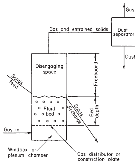
FIG. 17-7 Noncatalytic fluidized-bed system.
