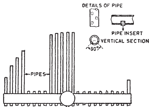
FIG. 17-11 Multiple-pipe gas distributor. [From Stermerding, de Groot, and Kuypers, Soc. Chem. Ind. J. Symp. Fluidization Proc., 35-46, London (1963).]
