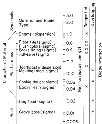
FIG. 18-42 Typical application and power for double-arm kneaders. To convert horsepower per gallon to kilowatts per cubic meter, multiply by 197.3. [Parker, Chem. Eng. , 72 (18): 125 (1965); excerpted by special permission of the copyright owner, McGraw-Hill, Inc.]
