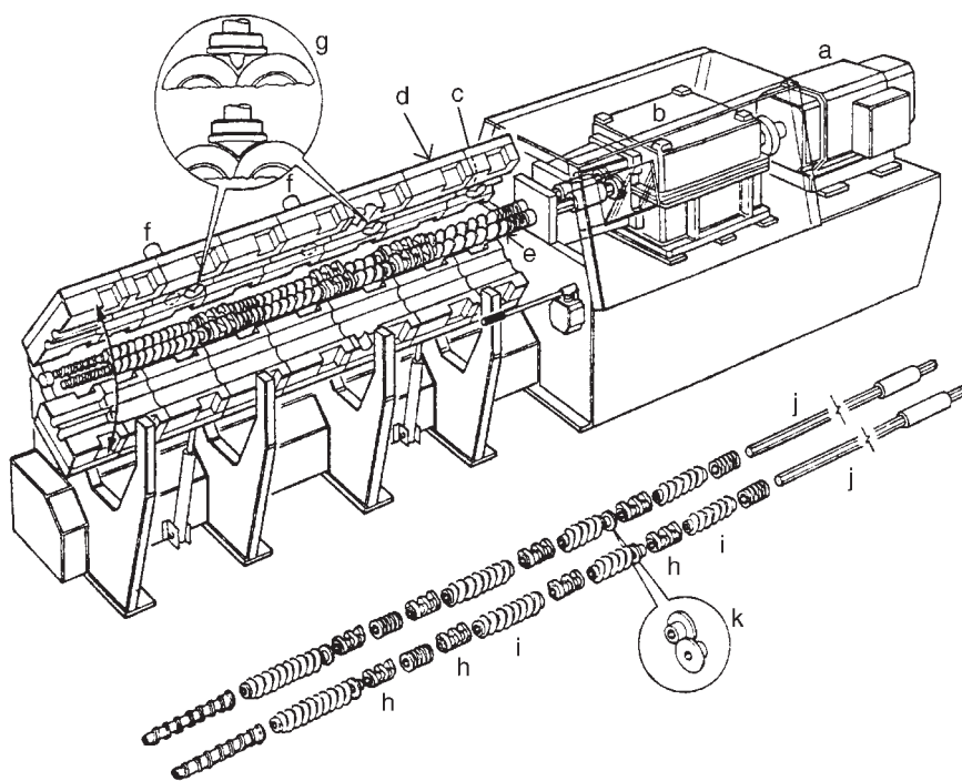
FIG. 18-50 Internmeshing corotating twin screw extruder: (a) drive motor; (b) gearbox; (c) feed port; (d) barrel; (e) assembled rotors; (f) vent; (g) barrel valve; (h) kneading paddles; (i) conveying screws; (j) splined shafts; (k) blister rings. (APV Chemical Machinery, Inc.)
