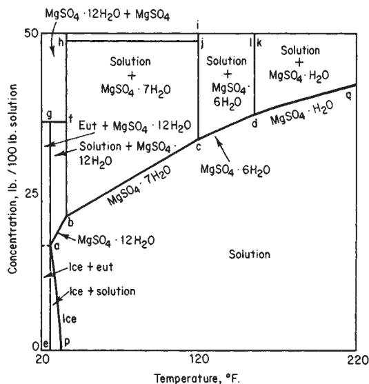
FIG. 18-56 Phase diagram. \text{MgSO}_4\text{-H}_2\text{O} . To convert pounds to kilograms, divide by 2.2; K = (^{\circ}\text{F} + 459.7)/1.8 .
