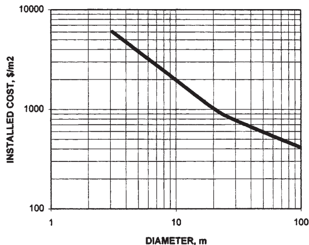
FIG. 18-93 Approximate installed cost of single-compartment thickeners (1995 dollars). To convert to ft and ft² units, multiply diameter in meters by 3.28 and divide cost by 10.76.
