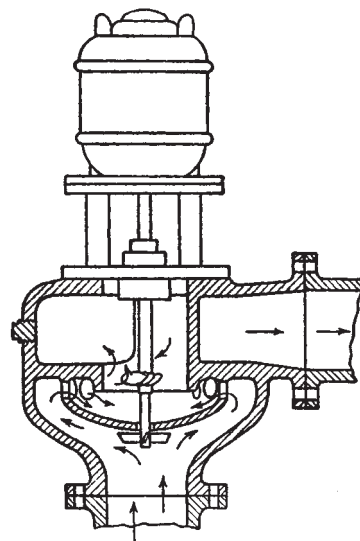
FIG. 18-32 Netto Corp. Flomix.
