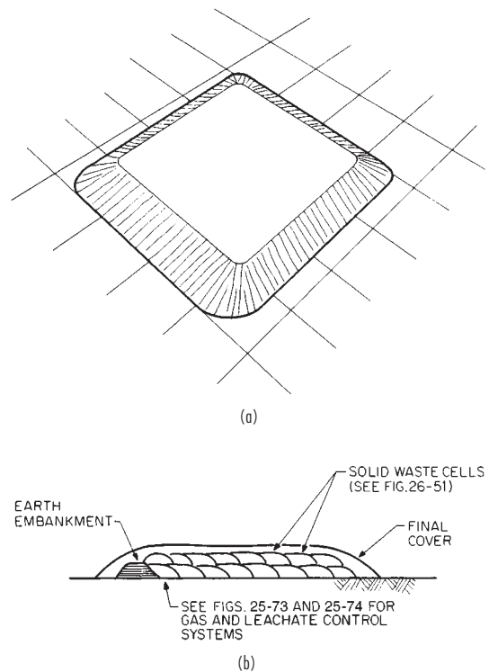
FIG. 25-68 Area method for landfilling solid wastes. (a) Pictorial view of completed landfill. (b) Section through landfill.
