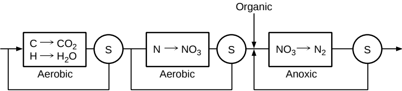
Three-sludge system
