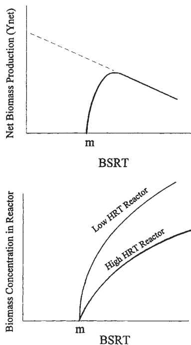
FIG. 25-50 Biomass production.
