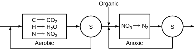
Two-sludge system
