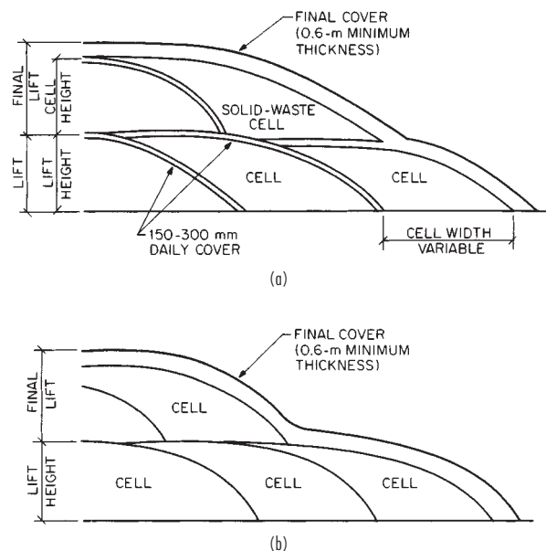
FIG. 25-69 Typical section through a landfill. (a) With daily or intermediate cover. (b) Without daily or intermediate cover.
