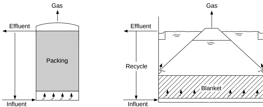
FIG. 25-57 Anaerobic processes.
