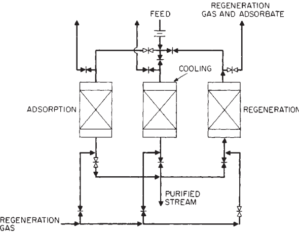
FIG. 25-11 Typical three-bed adsorption system.
