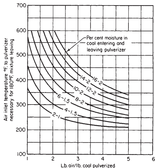
FIG. 27-20 Effect of moisture in coal on pulverizer capacity. Sufficient drying can be accomplished to restore capacity if air temperatures are high enough. [K = (^{\circ}\text{F} + 459.7)/1.8] (Combustion Engineer, Combustion Engineering Inc., New York, 1966.)
