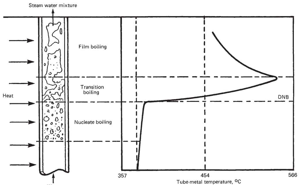
FIG. 27-40 Effect of departure from nucleate boiling (DNB) on tube-metal temperature.
