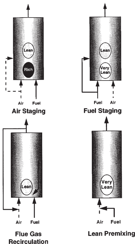
FIG. 27-15 Combustion modifications for NO x control.
