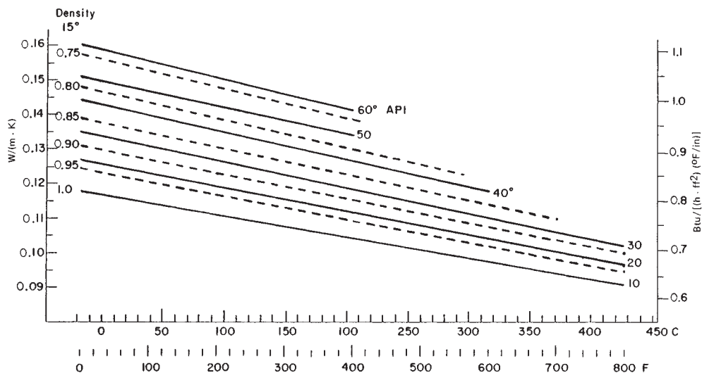
FIG. 27-4 Thermal conductivity of petroleum liquids. The solid lines refer to density expressed as degrees API; the broken lines refer to relative density at 288 K (15°C). ( K = [^{\circ}\text{F} + 459.7]/1.8 )
