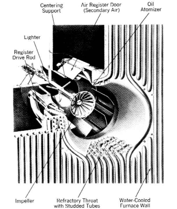
FIG. 27-29 Circular register burner with water-cooled throat for oil firing. (Babcock & Wilcox Co.)
