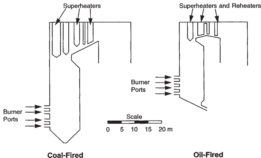
FIG. 27-42 Comparison of the sizes and shapes of typical 500-MW e coal- and oil-fired boilers. (Adapted with permission from Lawn, Principles of Combustion Engineering for Boilers , Academic Press, London, 1987.)
