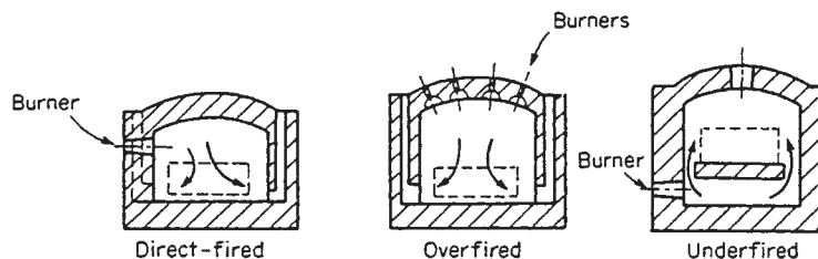
FIG. 27-53 Methods of firing direct-heated furnaces. (From Marks' Standard Handbook for Mechanical Engineers, 9th ed., McGraw-Hill, New York, 1957. Reproduced with permission.)
