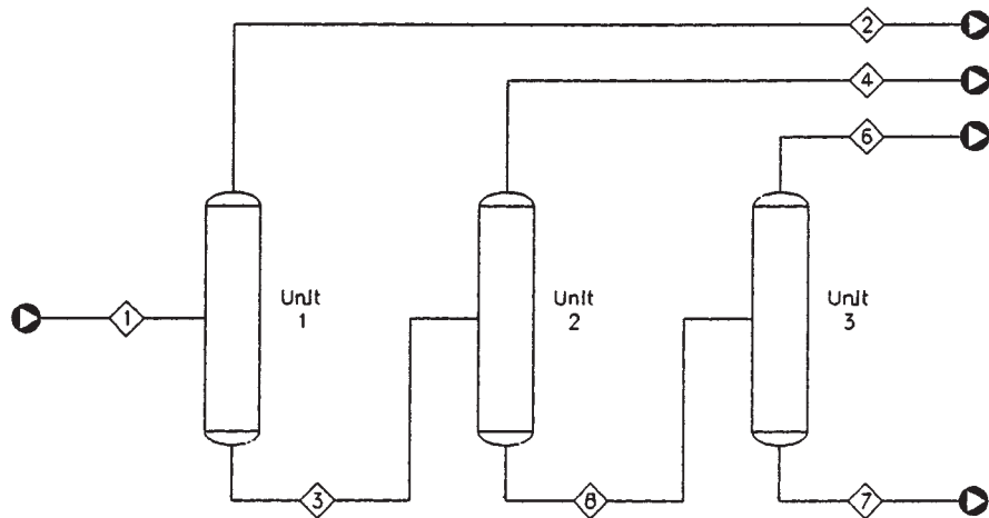
FIG. 30-21 Three-module unit.
