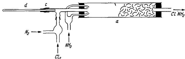
Fig. 184. Preparation of monochloramine. a ) Reaction tube, half filled with glass wool; d ) glass rod for removal of NH_4Cl plugs.
