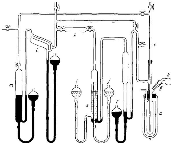
Fig. 232. Preparation of germanium hydrides.
