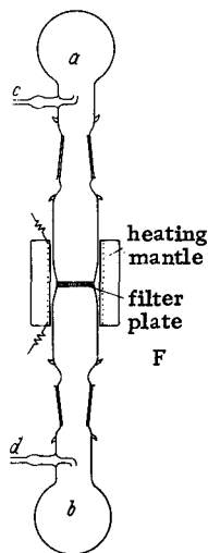
Fig. 49. Apparatus for dissolving and recrystallizing (the tube attachments c and d can also be located in the center sections).
