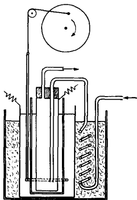
Fig. 188. Preparation of hydroxylammonium chloride by electrolysis.
