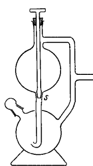
Fig. 58. Gasgenerator with Bodenstein dropping funnel. May be evacuated.
