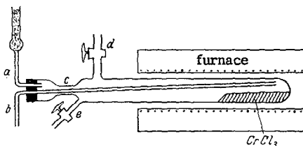
Fig. 313. Preparation of chromium (II) chloride. b inlet tube for hydrogen, \text{H}_2 -HCl mixture, or nitrogen; d stopcock with 10-mm. bore for withdrawal of reaction product.
