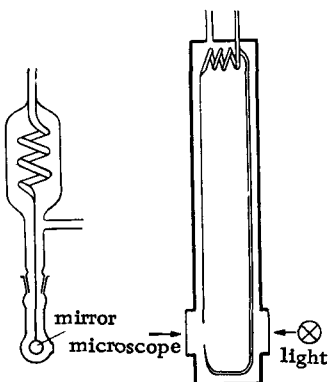
Fig. 26. Quartz-spiral manometer, Bodenstein type.
