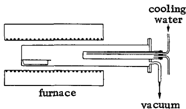
Fig. 78. Sublimation onto a cold finger.
