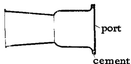
Fig. 53. Observation port for reaction tube.
