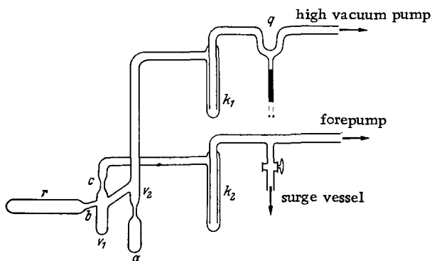
Fig. 261. Preparation of alkali metals from azides. r ) Decomposition tube; v 1 , v 2 ) receivers; a ) ampoule for storing the metal; b , c ) fused joints; k 1 , k 2 ) cooling traps; g ) mercury valve.
