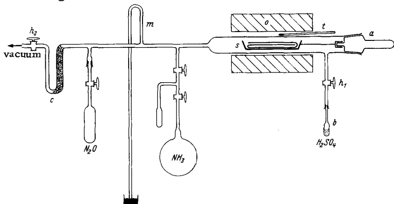
Fig. 178. Preparation of sodium amide with \text{N}^{15} . a) ground glass stopper; b) ampoule with \text{H}_2\text{SO}_4 ; c) condensation trap; h_1 , h_2 stopcocks; m) manometer; o) electric furnace; s) iron boat; t) thermocouple.
