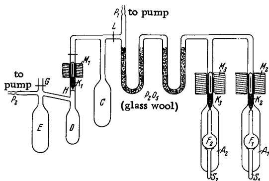
Fig. 100. Preparation of D_2S . F_1, F_2 ) ampoules containing SO_3 ; A_1, A_2 ) containers for SO_3 ampoules; K_1, K_2, K_3 ) seal breakers; M_1, M_2, M_3 ) electromagnets; H ) break-seal valve; C, D, E ) receivers (can be cooled); G, L ) sealing points.
