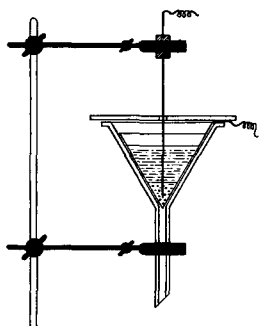
Fig. 190. Preparation of colloidal phosphorus.
