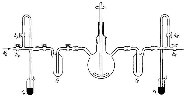
Fig. 240. Preparation of \text{LiBH}_4 from \text{LiH} and \text{B}_2\text{H}_6 .
