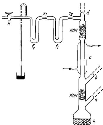
Fig. 176. Preparation of \text{N}^{15}\text{H}_3 from labeled ammonium salt. a , b , d ) Inlet tubes; \mathcal{J}_1 , \mathcal{J}_2 ) condensation traps; k ) reaction flask; s_1 , s_2 ) constricted sealing-off points.
