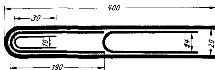
Fig. 300. Synthesis of lower titanium oxides (dimensions in mm.).
