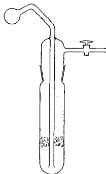
Fig. 332. Preparation of iron (II) oxide.
