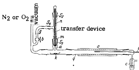
Fig. 277. Charging and heating of the \text{KO}_x\text{-CuO} mixture.
