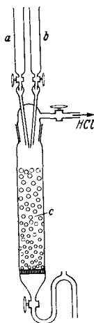
Fig. 144. Preparation of hydrogen chloride. a , b ) Dropping tubes for concentrated HCl and concentrated \text{H}_2\text{SO}_4 ; c ) reaction tube packing (silica or glass beads, diameter 2–5 mm.).
