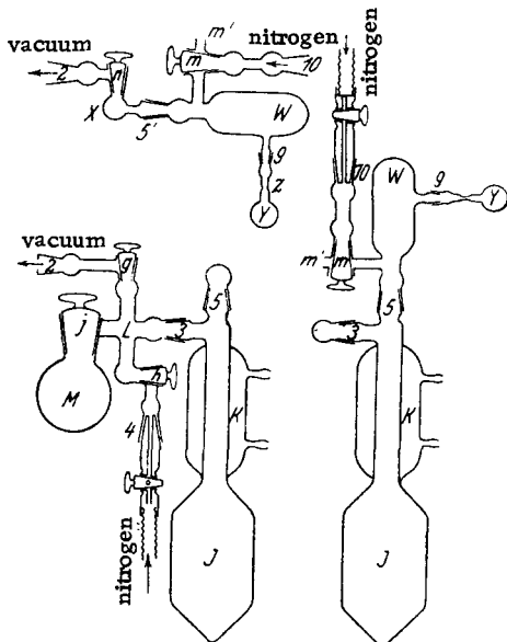
Fig. 51. Apparatus for precipitation in the absence of air. Arrangement for drying and transfer of the precipitates: W —transfer vessel with adapter X ; Y —storage vessel with sealing constriction Z ; 2-10—ground joints; g - n —stopcocks.
