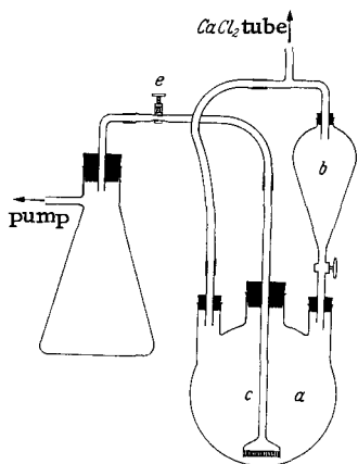
Fig. 230. Preparation of silicon tetraacetate.
