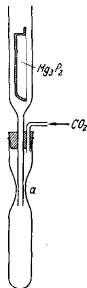
Fig. 258. Bottling of magnesium phosphide under \text{CO}_2 blanket.
