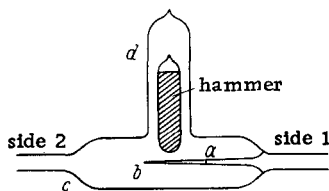
Fig. 34. Briscoe break-seal valve. The capillary point b is still open during sealing to side 1, but several scratches have been made at a . Then b is fused by means of a very small flame introduced through c , with air entering at d . Next the valve is sealed to the other side, the Hg-filled hammer bar is carefully introduced and d is sealed. A sharp movement applied from the outside will shatter the valve.
