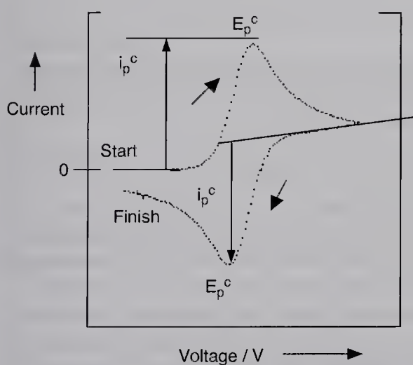
Fig. 1.2-5 Theoretical cyclic voltammogram for a single one-electron oxidation process.
