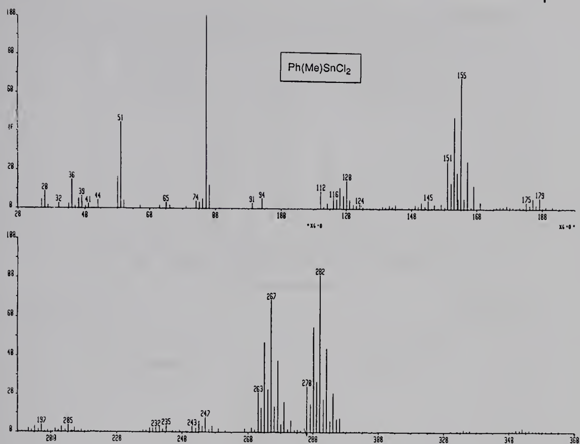
Fig. 3.17-3 Mass spectrum of \text{Ph (Me)SnCl}_2 .
