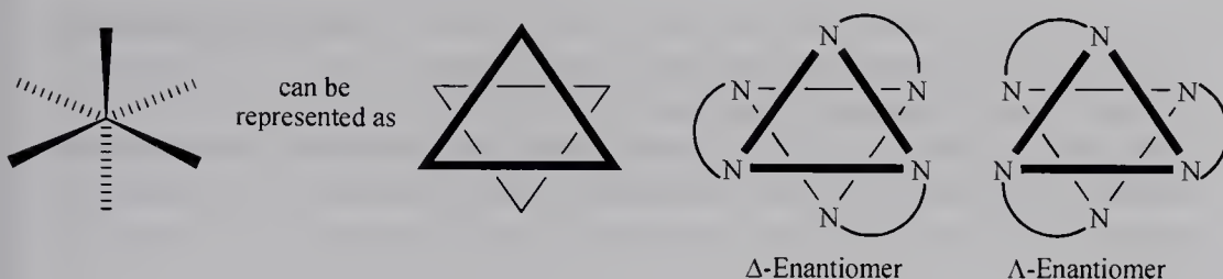
Scheme 4.2-2 The formation of enantiomers in a tris(chelate) complex.
