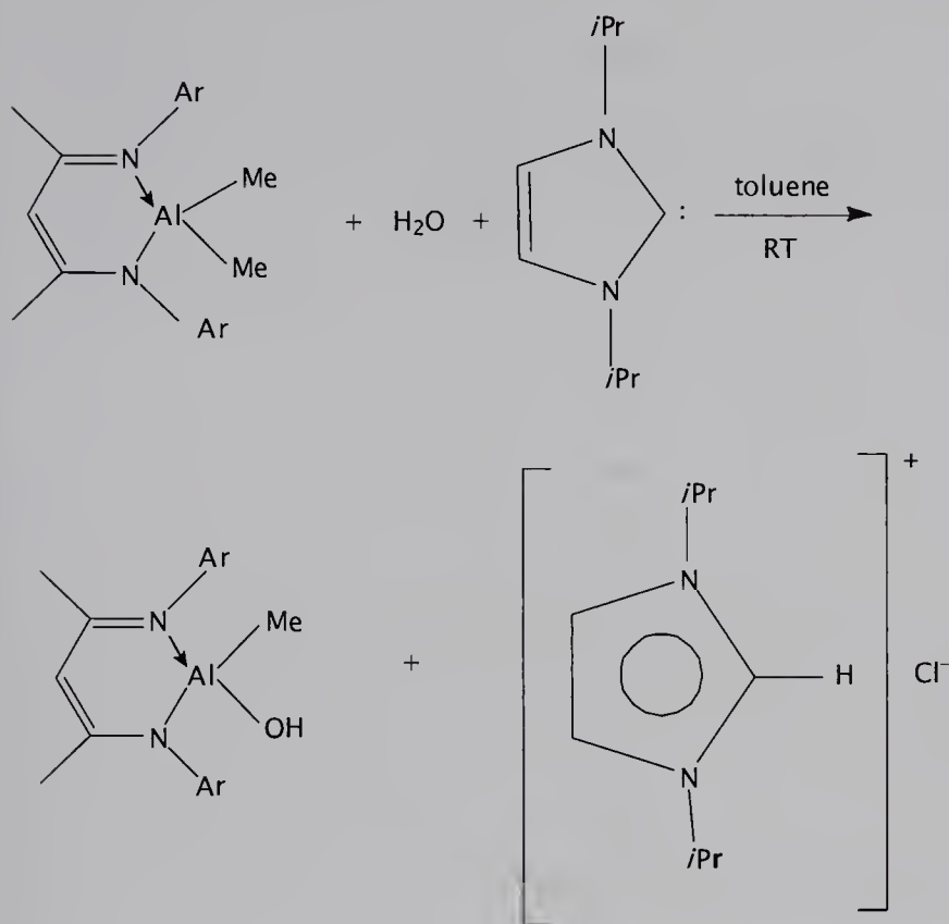
Scheme 4.25-2
