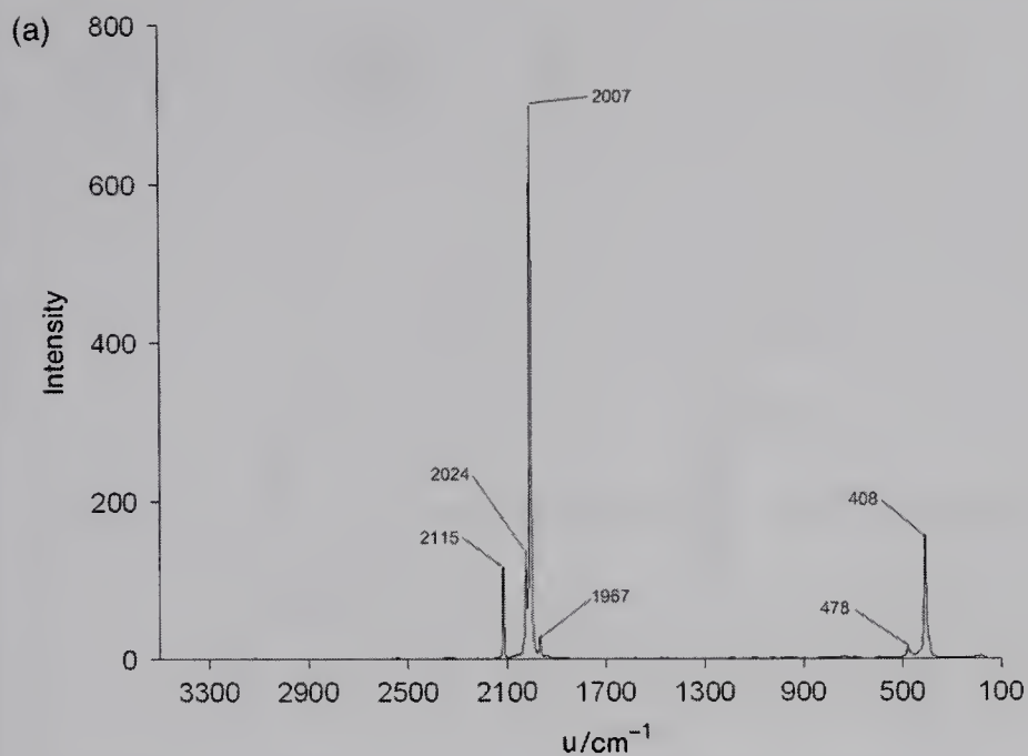
Fig. 4.16-1 (a) Raman spectrum of \text{Mo(CO)}_6 .
