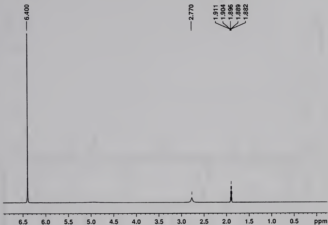
Fig. 4.16-3 ^1\text{H} NMR spectrum of cycloheptatrienyl molybdenum tricarbonyl tetrafluoroborate in acetone- d_6 .
