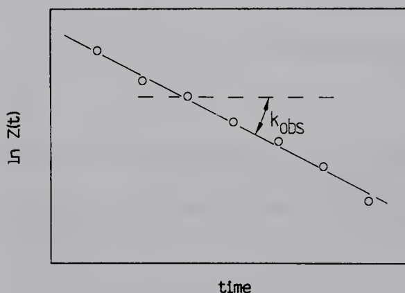
Fig. 3.32-4. Linearization of a first-order kinetic curve. Semi-log plot: Z(t) = |\gamma_t - \gamma_\infty| . Guggenheim plot: Z(t) = |\gamma_{t+\Delta} - \gamma_t| . In both cases, k_{\text{obs}} is calculated from the slope of the straight line.
