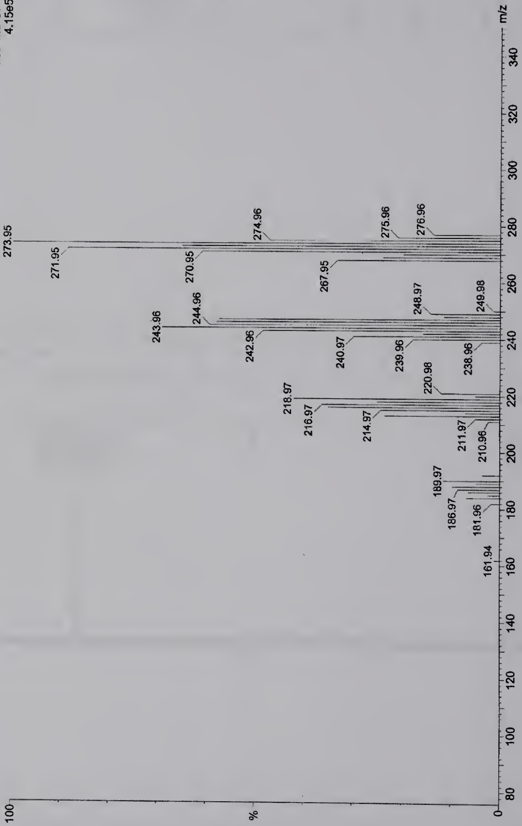
Fig. 4.16-5 Mass spectrum (chemical ionization, positive) of cycloheptatriene molybdenum tricarbonyl.
