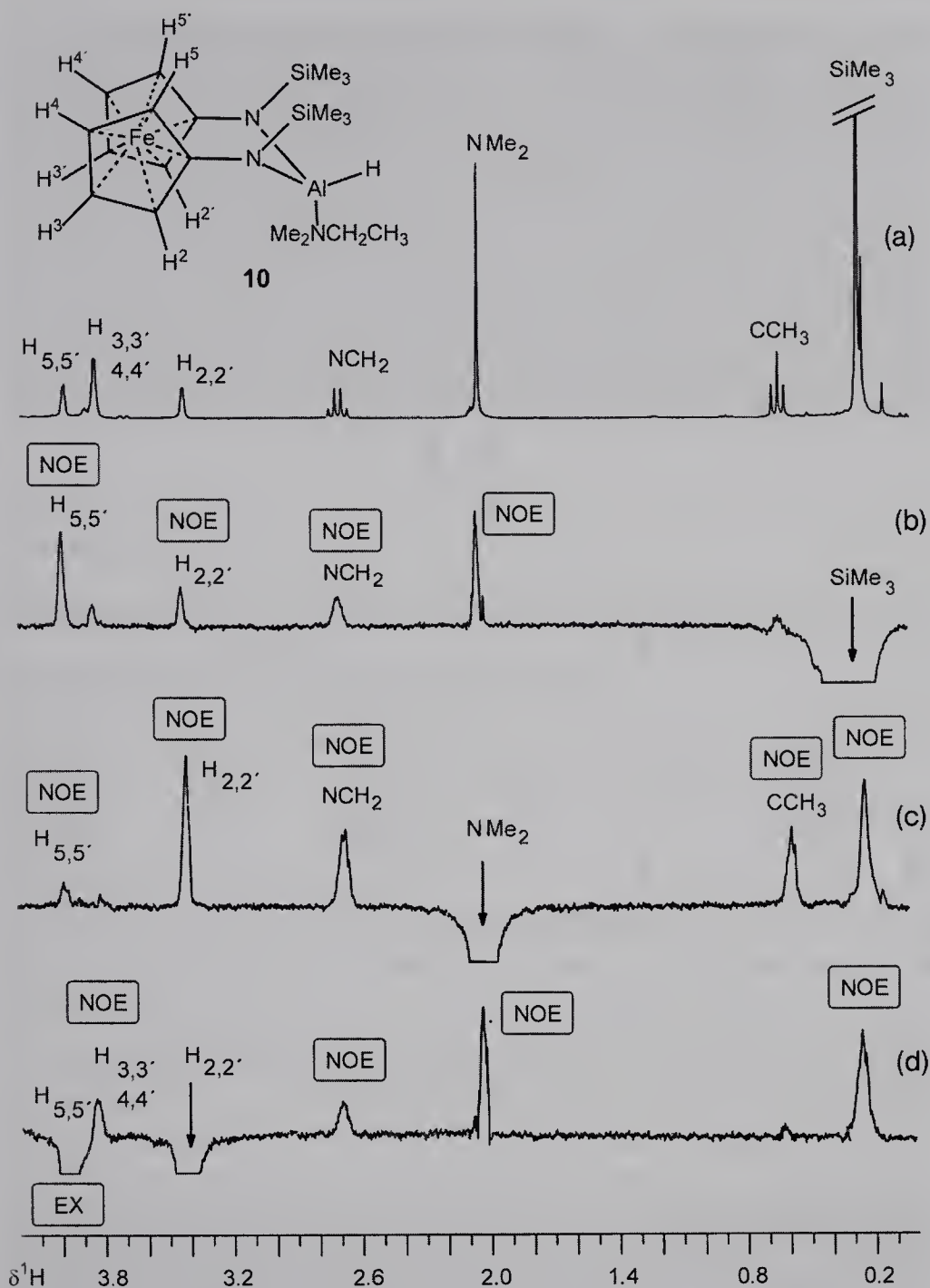
Fig. 4.15-2 400 MHz 1 H{ 1 H} NOE difference spectra (gradient enhanced [19a]) of 10 (10% in toluene- d 8 at 23 °C; relaxation delay 1.5 seconds; mixing time 0.6 seconds; 30 minutes of spectrometer time). The irradiated resonance signals are marked by arrows; the intensities as response arising from NOE or exchange (magnetisation transfer) are marked. (a) Normal 1 H NMR spectrum. (b) The NSiMe 3 resonance was irradiated. (c) The NMe 2 resonance was irradiated. (d) The H 2,2' resonance of the cyclopentadienyl groups was irradiated.
