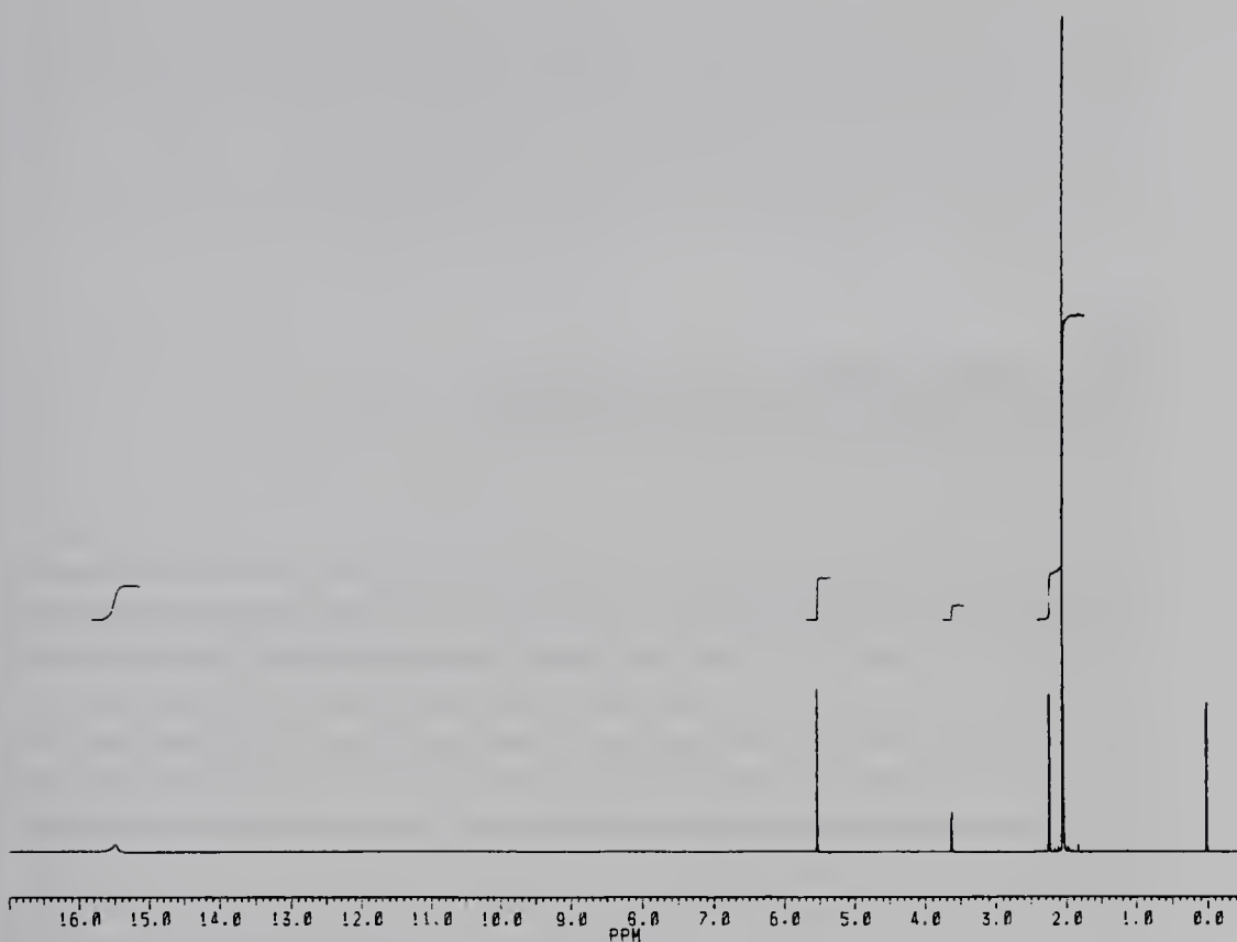
Fig. 3.1-4 The ^{13}\text{C} NMR spectrum of \text{CH}_3\text{COCH}_2\text{COCH}_3 containing both keto and enol forms.
