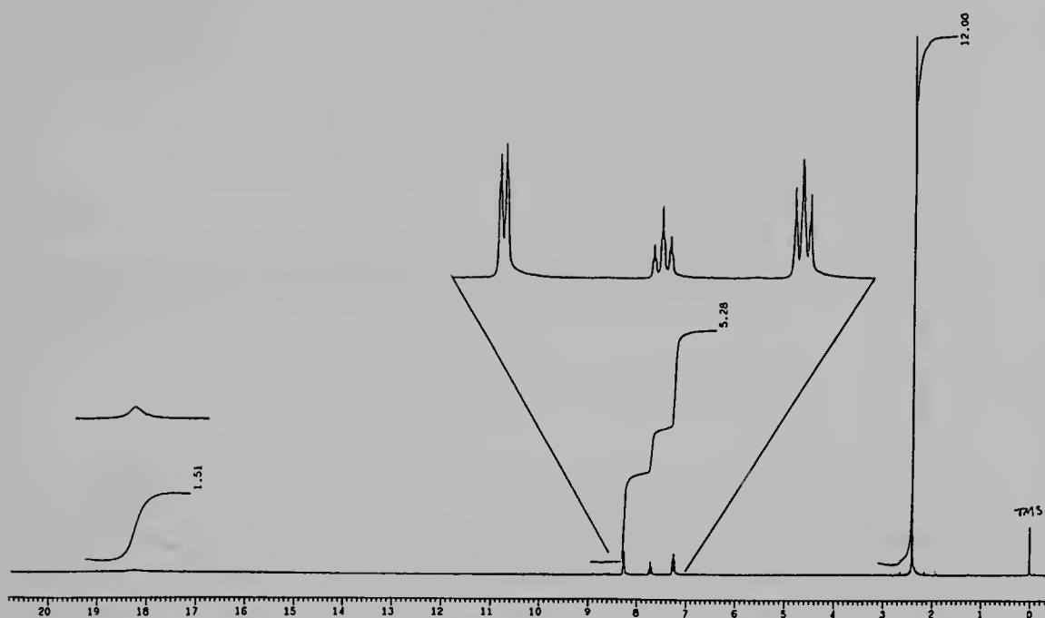
Fig. 3.18-5 The 270 MHz {}^1\text{H} NMR spectrum of chloropyridinecobaloxime recorded in \text{CDCl}_3 solution.
