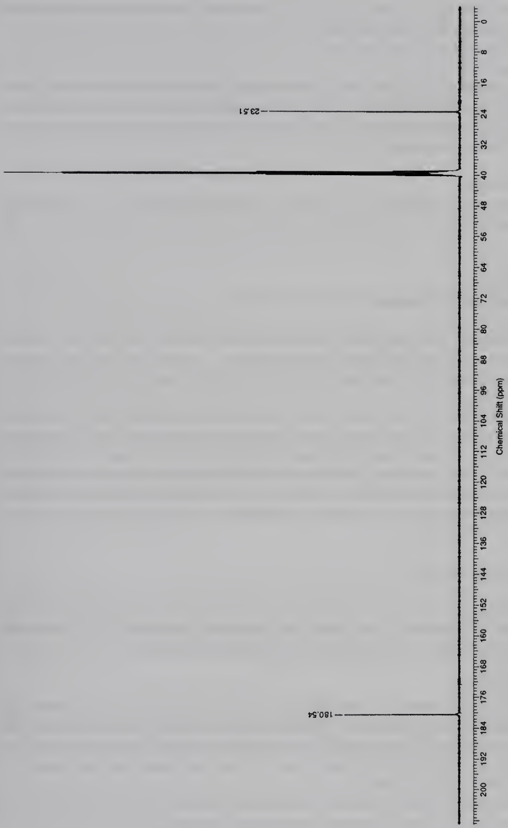
Fig. 3.12-1 ^{13}\text{C}\{^1\text{H}\} NMR spectrum (400 Hz, DMSO- d_6 ) of [\text{Mo}_2(\text{O}_2\text{CMe})_4] .
