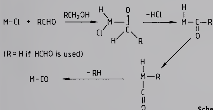
Scheme 3.18-2
