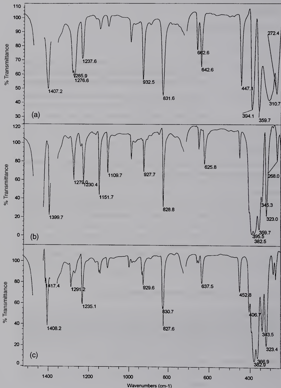
Fig. 4.31-1 FT-IR spectra obtained as Nujol mulls between CsI plates on a Nicolet 510P spectrometer, Nujol regions have been blanked. a) 2-chloro-cyclo-1,3-dithia-2-arsapentane (1). b) Bis(1,3-dithia-2-arsolidinium tetrachlorogallate), [2][GaCl 4 ] 2 . c) 2-chloro-cyclo-1,3-dithia-2-arsapentane-1,3-dithia-2-arsolidinium tetrachlorogallate, [3][GaCl 4 ].
