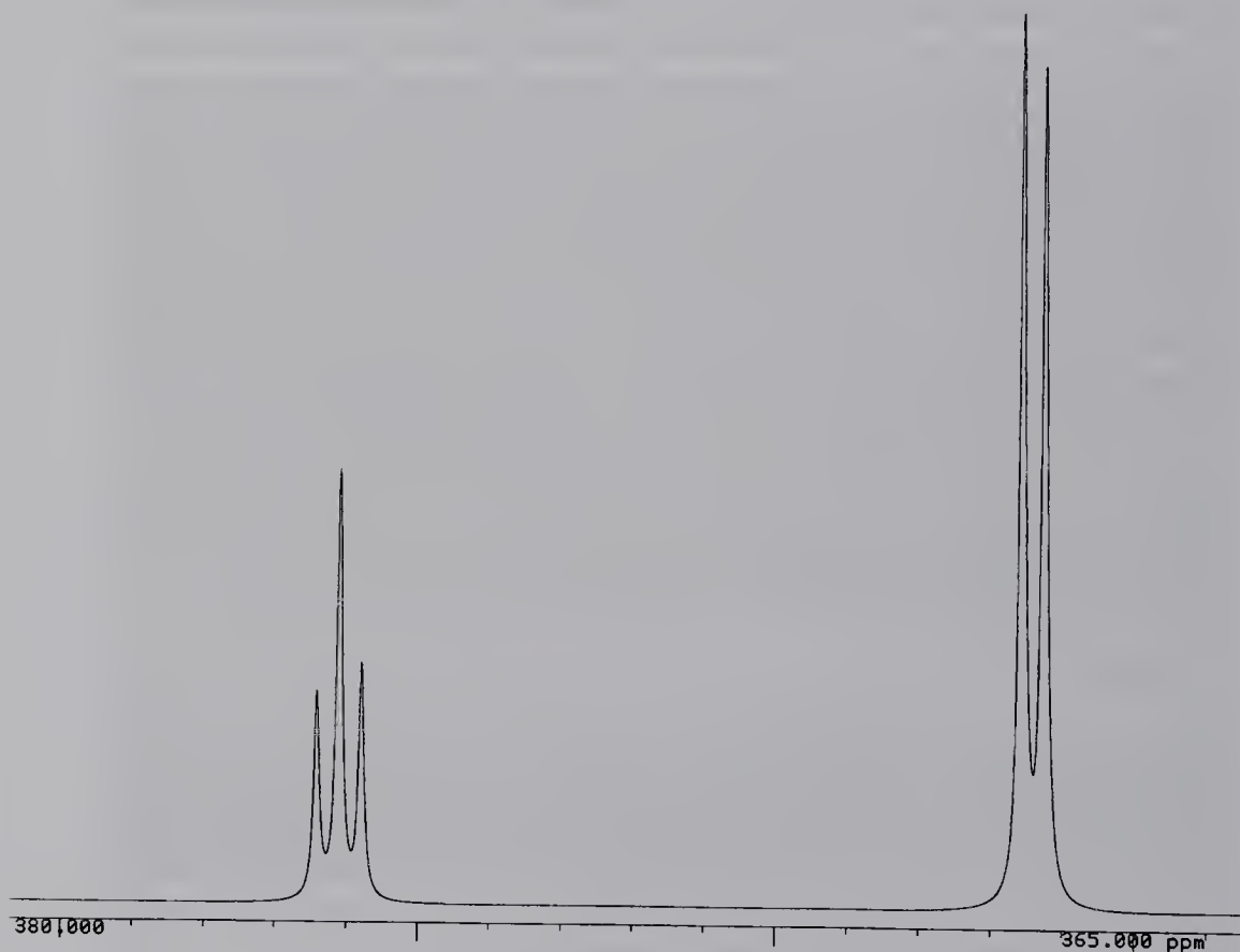
Fig. 4.34-1 ^{15}\text{N} NMR of 100% ^{15}\text{N} labelled [\text{S}_4\text{N}_3]\text{Cl} in conc. \text{HCl} at 27.36 MHz.
