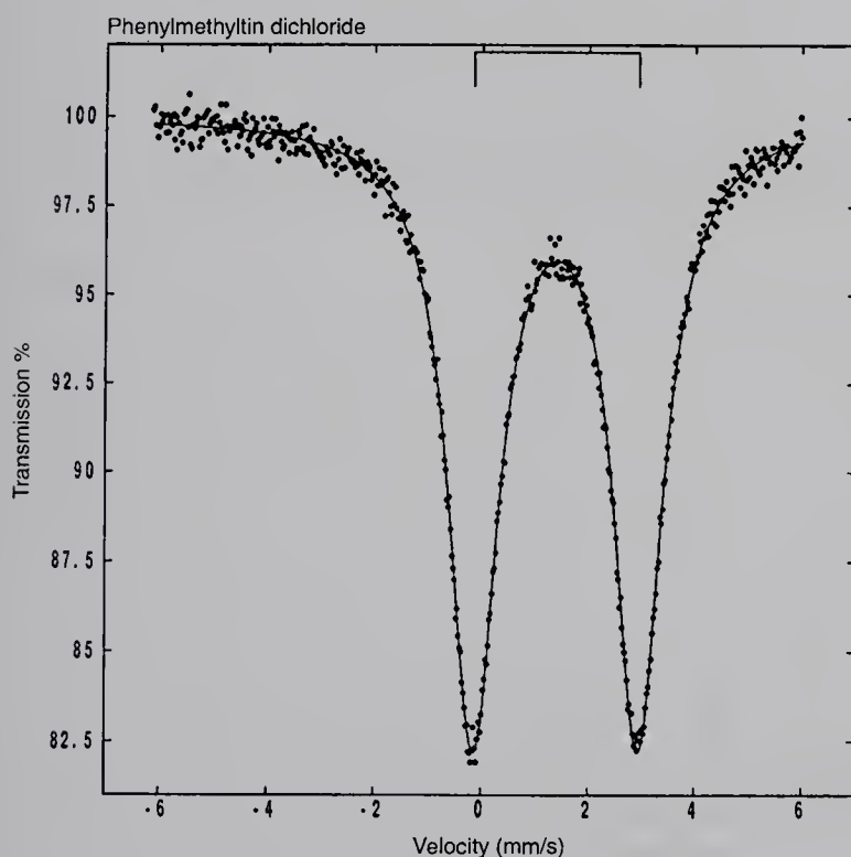
Fig. 3.17-4 Mössbauer spectrum of \text{Ph (Me)SnCl}_2 .
