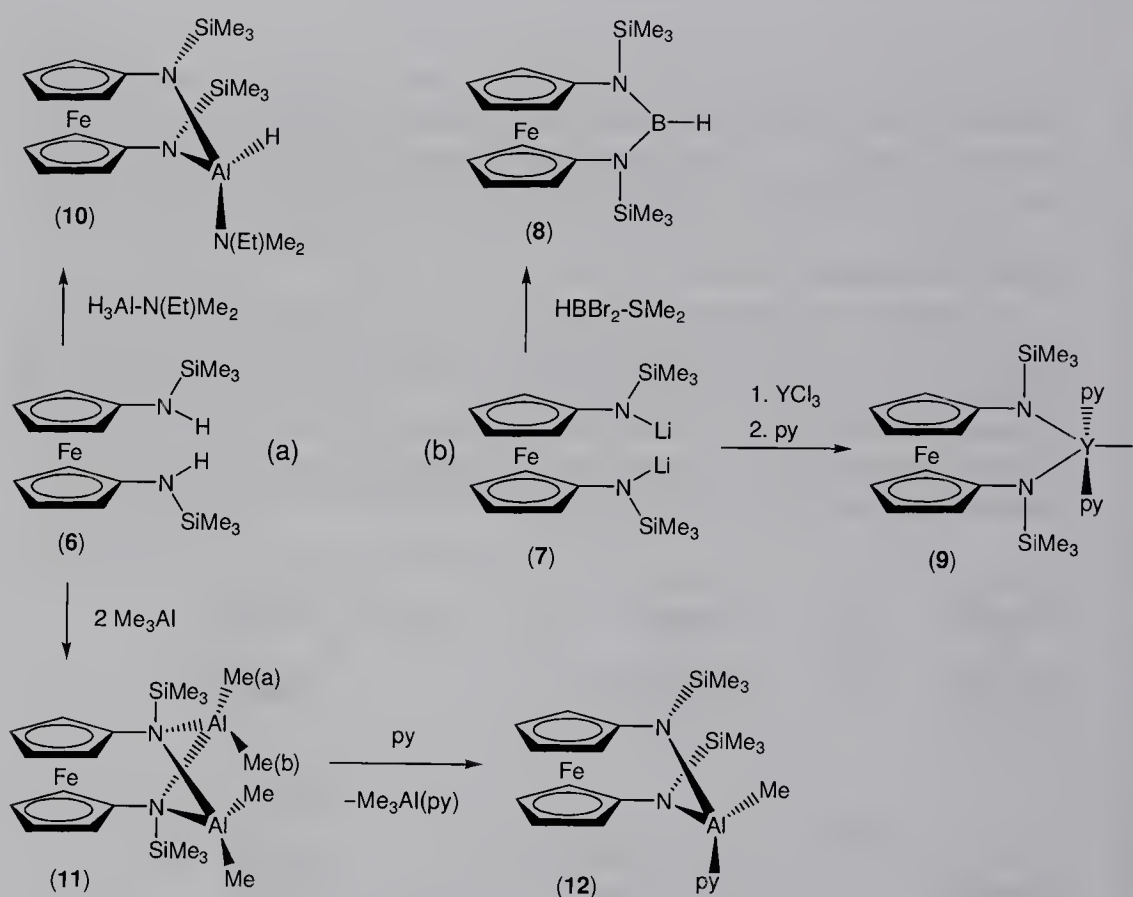
Scheme 4.15-2
