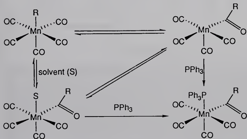
Scheme 4.17-1
