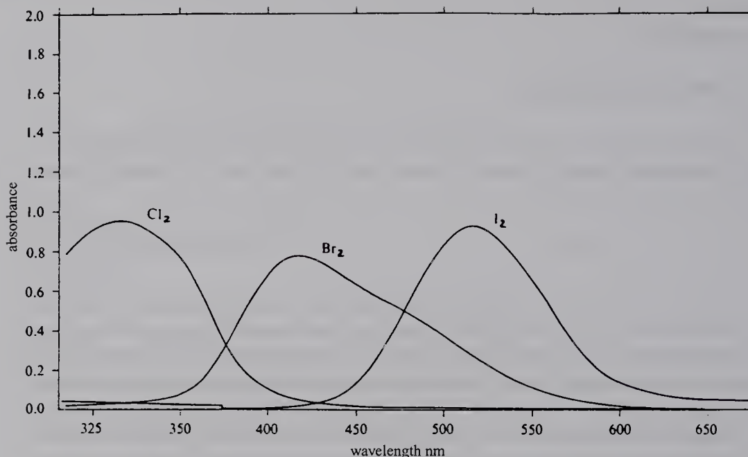
Fig. 2.24-2 Electronic spectra of chlorine (0.013 3 M in \text{CCl}_4 ), bromine (0.004 4 M in \text{CCl}_4 ) and iodine (0.000 9 M in \text{CCl}_4 ). For all three spectra the path length was 10 mm.
