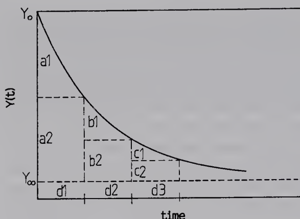
Fig. 3.32-3. First-order decay leading to a good estimation of \gamma_\infty . Half-time method ( a_1 = a_2 ; b_1 = b_2 ; c_1 = c_2 ). Note the regularity of the successive half-time ( d_1 = d_2 = d_3 ).
