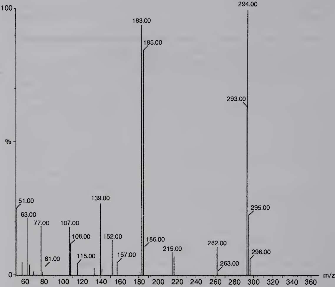
Mass Spectrum of \text{Ph}_3\text{P}=\text{S}
