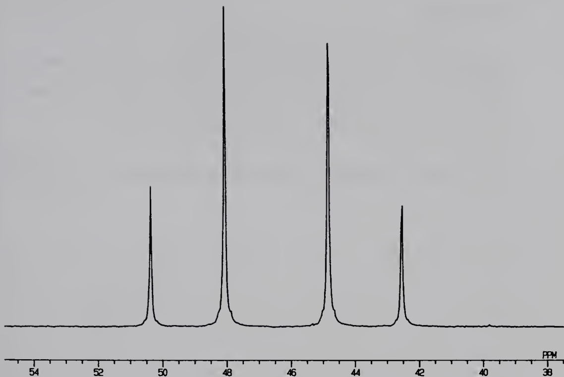
Fig. 4.27-2 ^{31}P\{-^1H\} NMR spectrum (at 109.3 MHz) of RuH(B_3H_8)CO(PPh_3)_2 .
