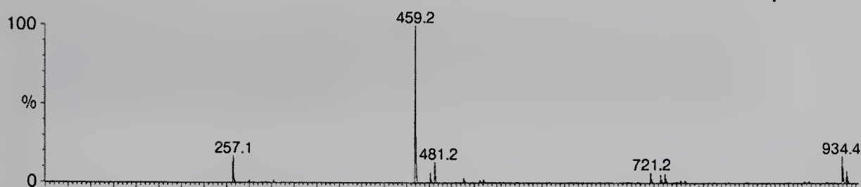
Fig. 3.24-1 Electrospray mass spectrum of \text{Ph}_2\text{P}(\text{O})\text{C}_4\text{H}_8\text{P}(\text{O})\text{Ph}_2 .
