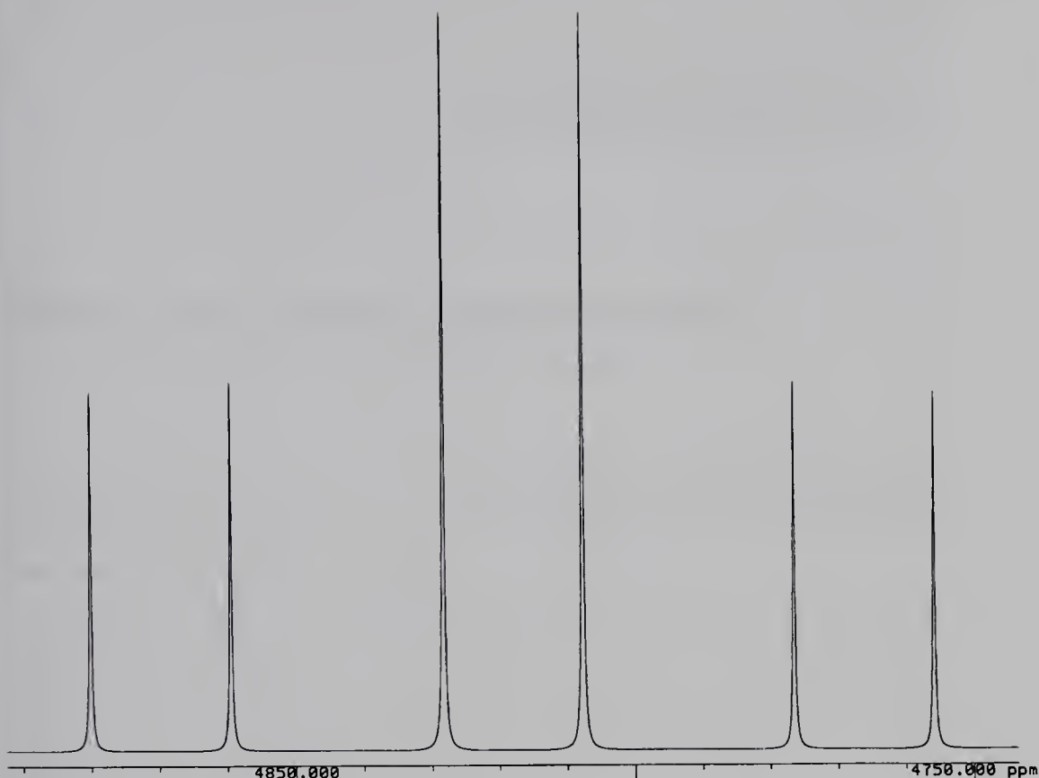
Fig. 3.8-2. 58.05 MHz ^{195}\text{Pt} NMR spectrum of trans -PtHCl(PPh 3 ) 2 .
