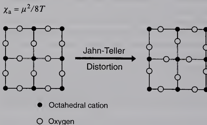
Fig. 4.9-2 Cooperative Jahn-Teller distortions in a layer of the perovskite structure.
