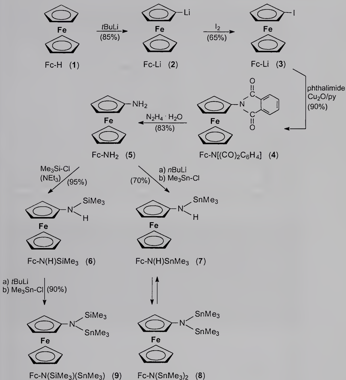
Scheme 4.14-1
