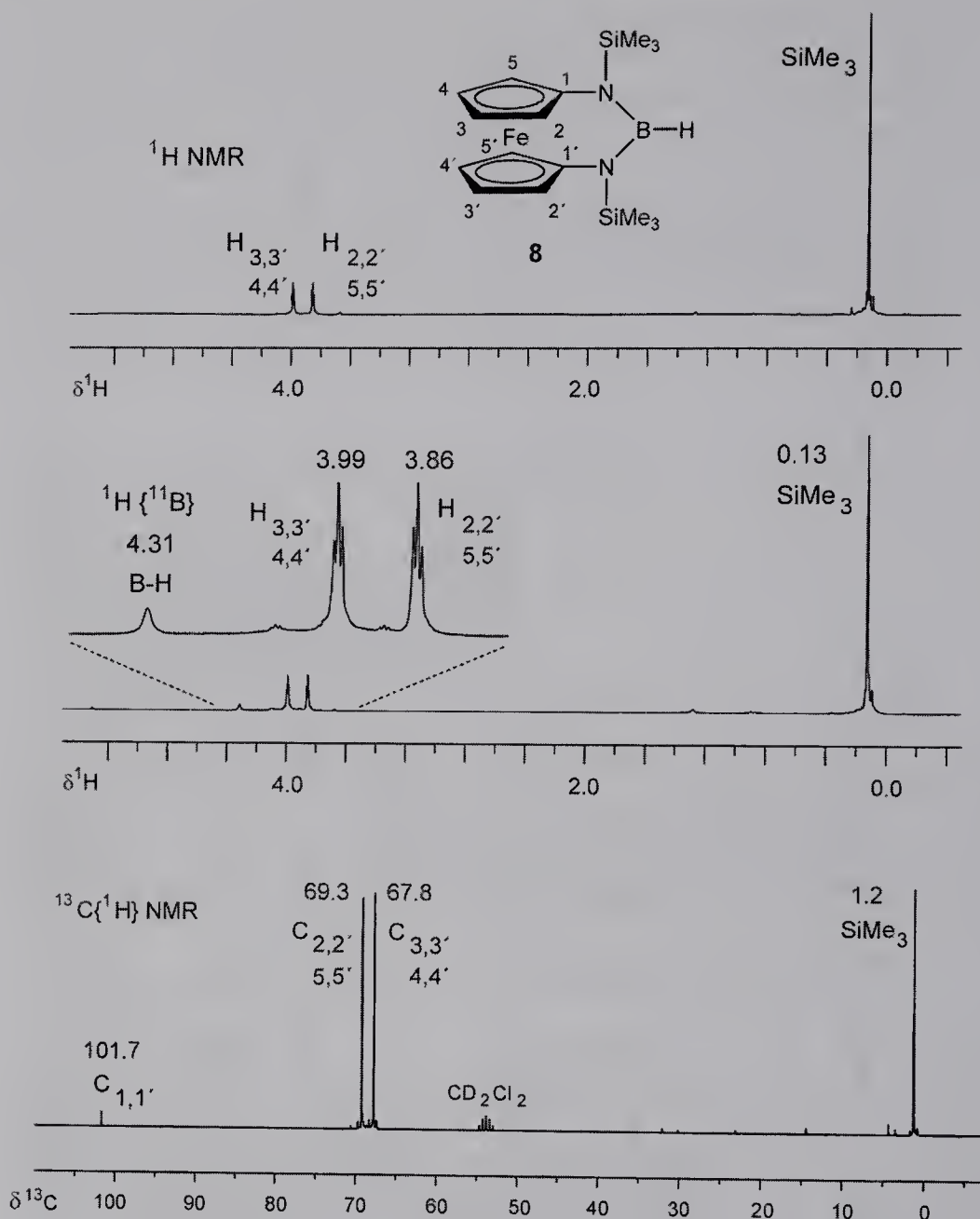
Fig. 4.15-1 250.1 MHz ^1\text{H} NMR and 62.9 MHz ^{13}\text{C}\{^1\text{H}\} NMR spectra of ( 8 ) in \text{CD}_2\text{Cl}_2 .
