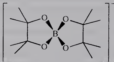
(4) Complex ion
