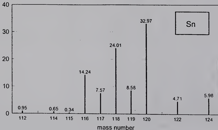
Fig. 3.17-5 Isotope distribution patterns for \text{Sn} , \text{SnX} and \text{SnX}_2 ( \text{X} = \text{Br}, \text{Cl} ).
