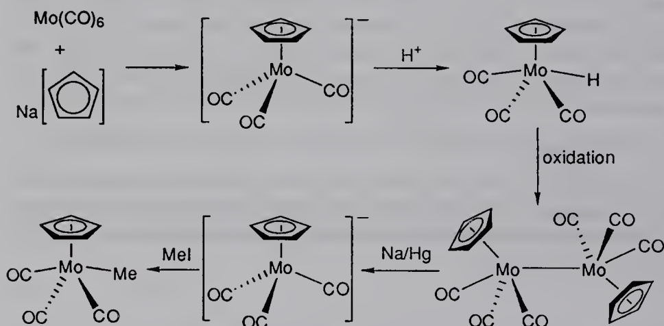
Scheme 4.17-2
