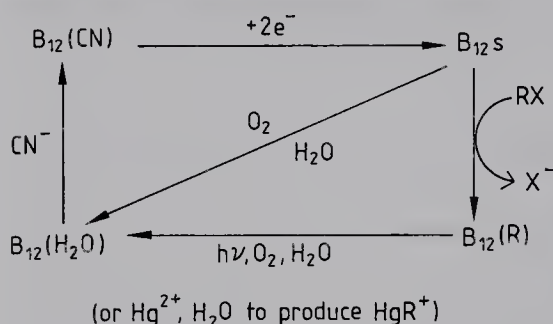
Scheme 3.18-1
