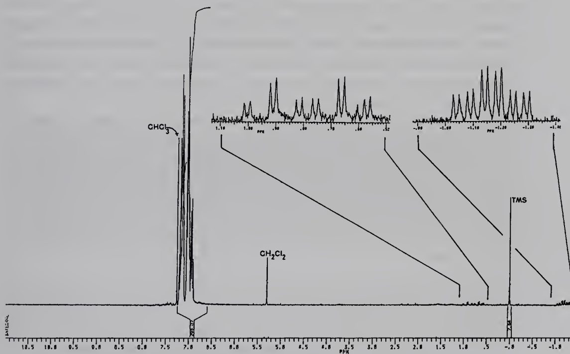
Fig. 3.18-6 {}^1\text{H} NMR spectrum of [\text{Ru}(\text{H})_2(\text{CO})(\text{PPh}_3)_3] in \text{CDCl}_3 at 300 MHz.
