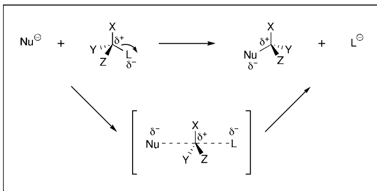
Scheme 5.6 Stereochemical course of S_N2 reactions are defined by the stereochemical configuration of the starting materials. One product is formed.
