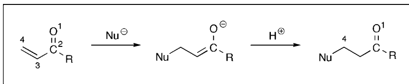
Scheme 7.17 Addition of nucleophiles to \alpha,\beta -unsaturated carbonyls can result in 1,4-additions.
