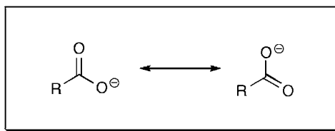
Scheme 2.3 Resonance forms of the carboxylate anion.
