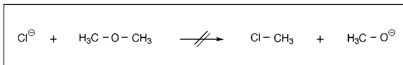
Scheme 4.4 S_N2 reactions do not proceed when incoming nucleophiles are less nucleophilic than outgoing leaving groups.
