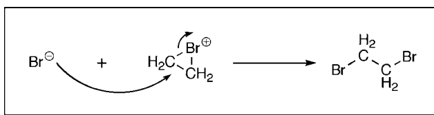
Scheme 7.4 Nucleophilic reaction between a bromide anion and a bromonium ion generates 1,2-dibromoalkanes.
