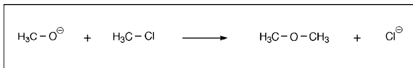
Scheme 4.3 S_N2 reactions proceed when incoming nucleophiles are more nucleophilic than outgoing leaving groups.
