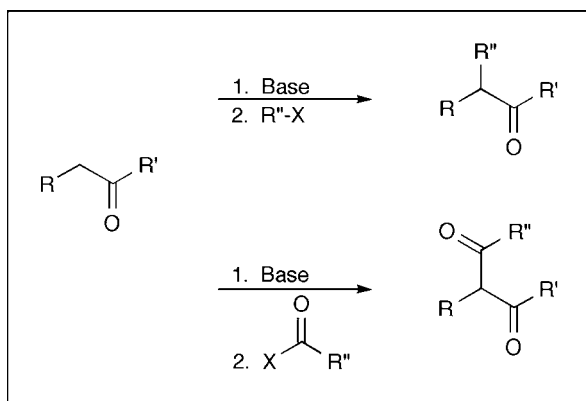
Scheme 8.11 Alkylation and acylation reactions adjacent to carbonyls.
