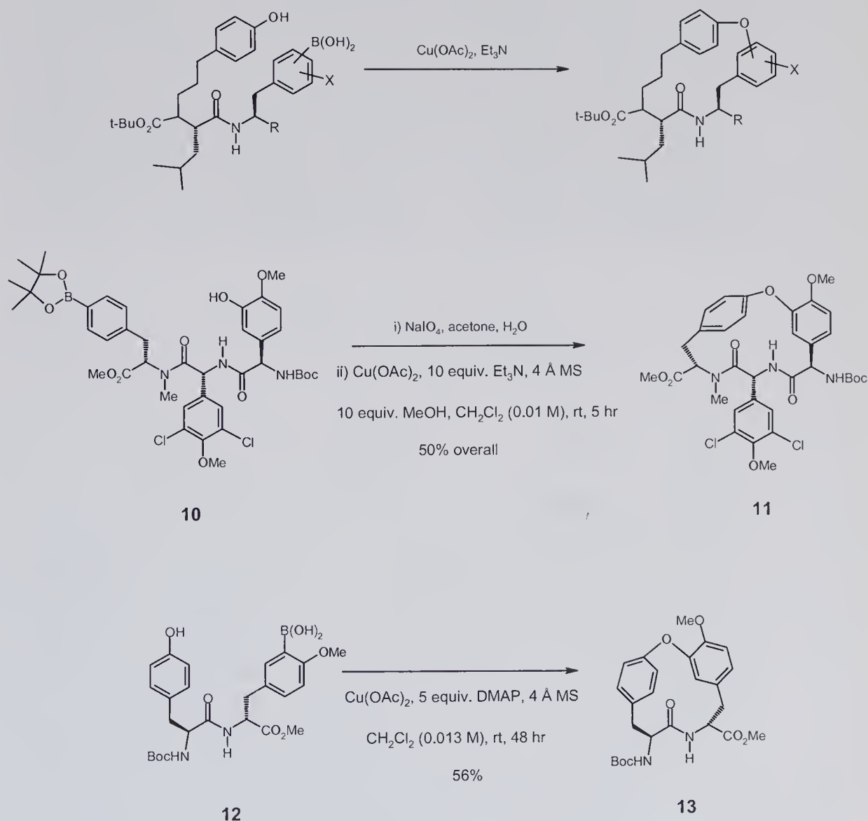
Scheme 5.5 Examples of intramolecular C–O cross-coupling.
