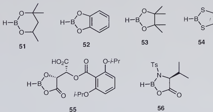
Figure 1.13 Common dialkoxyboranes and heterocyclic analogues.
