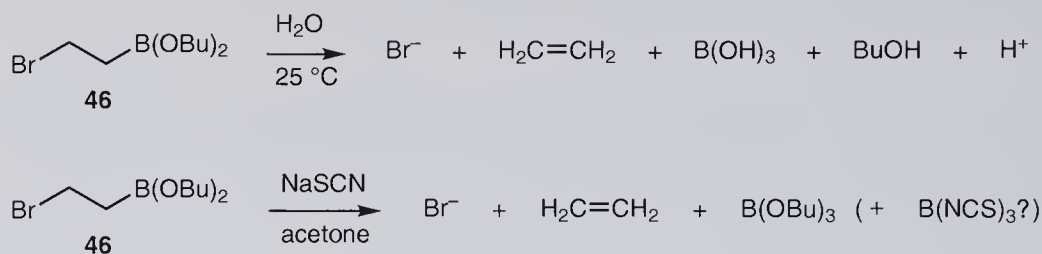
Scheme 8.10 Elimination of ethylene from dibutyl (2-bromoethyl)boronate.
