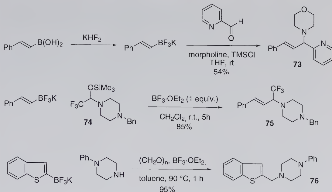
Scheme 7.16 Application of trifluoroborate salts in the Petasis borono-Mannich reaction.
