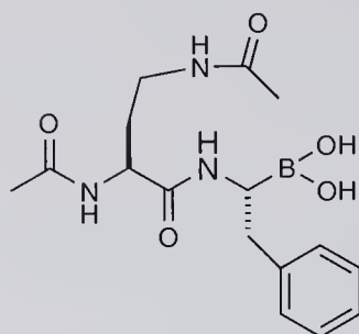
Figure 13.5 Macrocyclic peptidyl boronic acids as potential chymotrypsin inhibitors.
