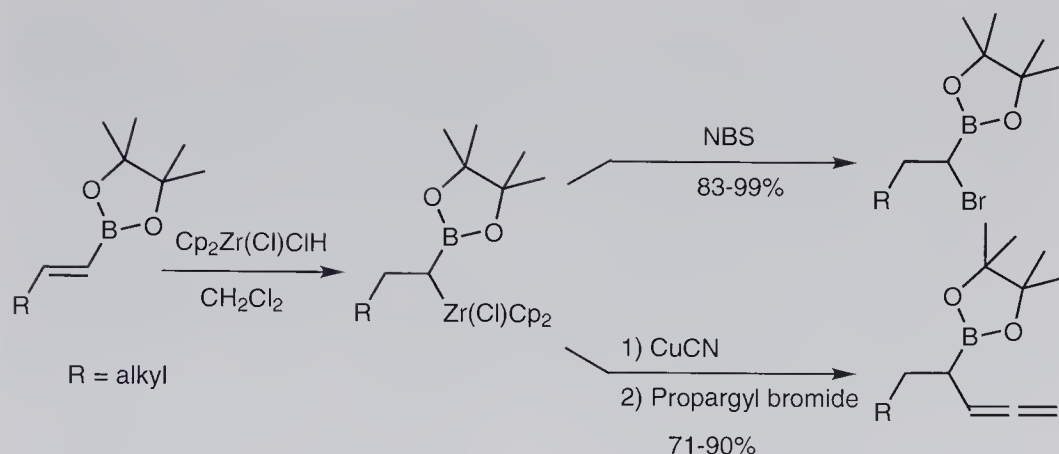
Scheme 9.56 Hydrozirconation of alkenylboronates and further transformations.
