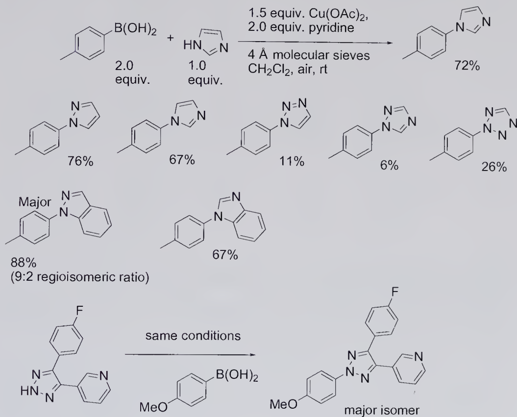
Scheme 5.15 N-Arylation of azoles.
