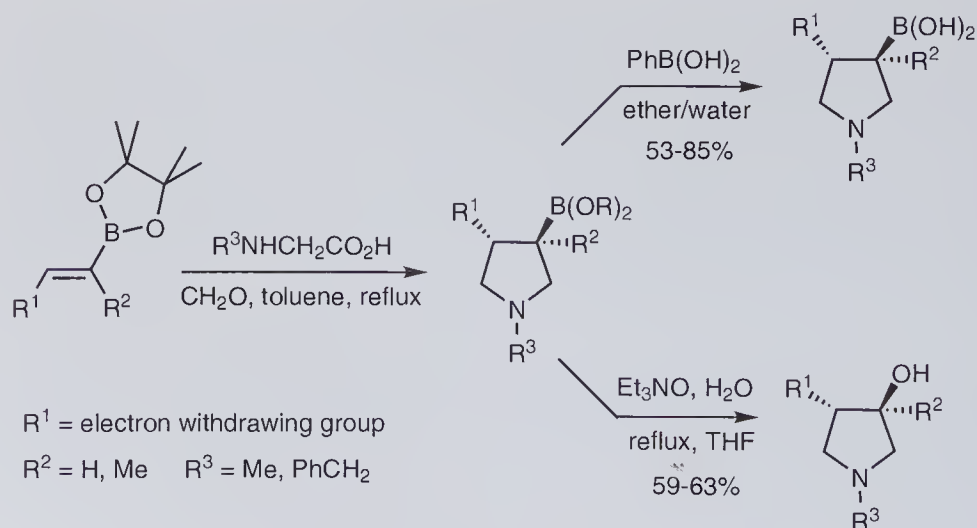
Scheme 9.46 1,3-Dipolar cycloadditions of azomethyne ylides to alkenylboronates.
