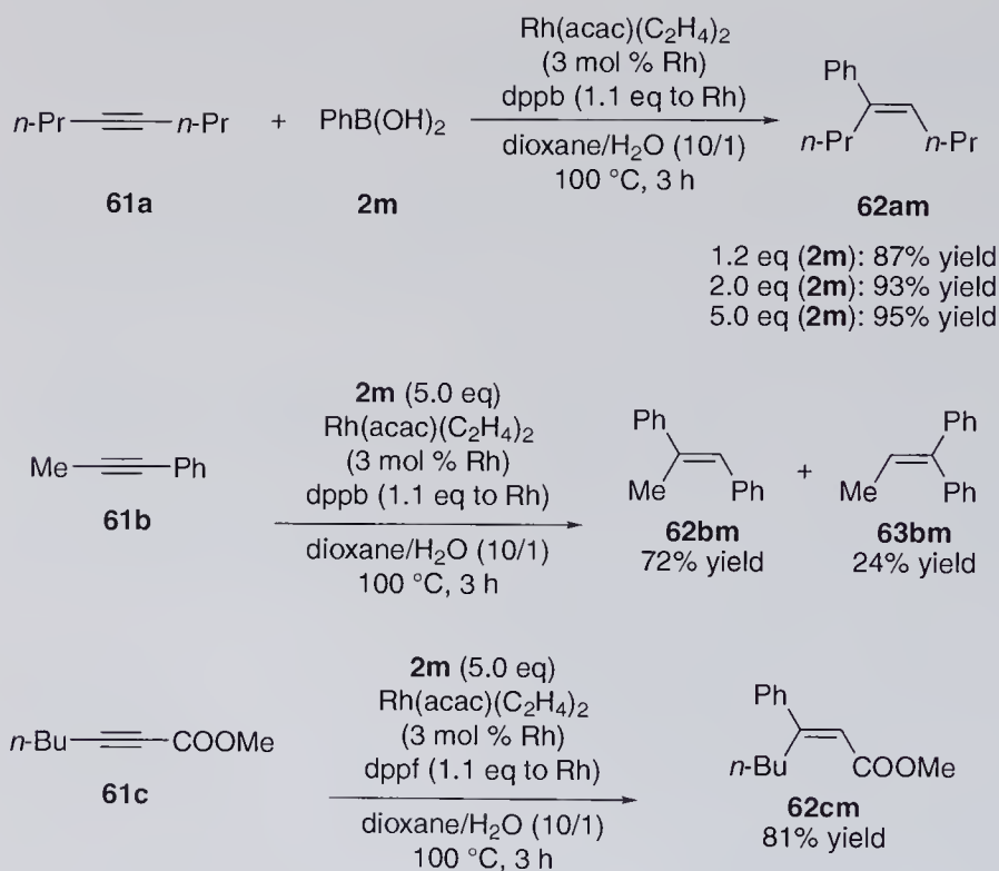
Scheme 4.27 Rhodium-catalyzed hydroarylation of alkynes with arylboronic acids.
