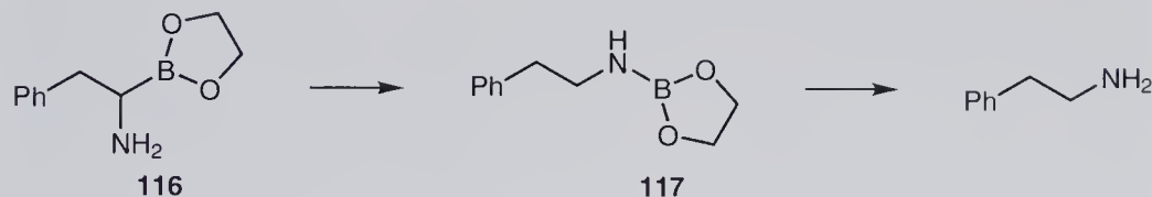
Scheme 8.27 Decomposition of an ( \alpha -aminoalkyl)boronic ester.
