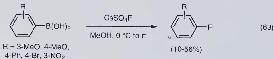
Figure 1.34 Halogenation of arylboronic acids.
