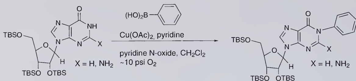
Scheme 5.20 N-1 Arylation of purine nucleosides.
