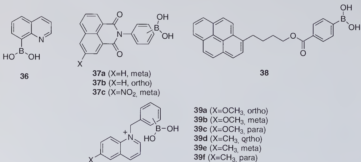
Figure 12.9 Monoboronic acid fluorescent sensors.
