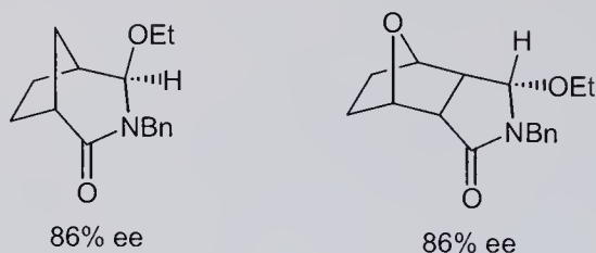
Scheme 11.10 Desymmetrization of meso-imides via 2a -catalyzed reduction.
