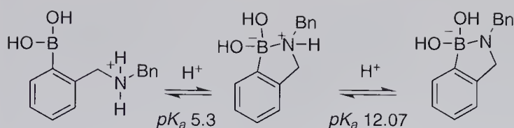
Scheme 12.2
