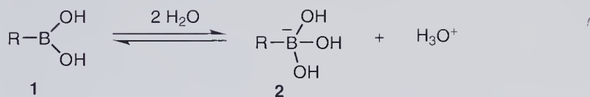
Scheme 13.1 Conversion from a neutral and trigonal planar sp^2 boron into an anionic tetrahedral sp^3 boron.
