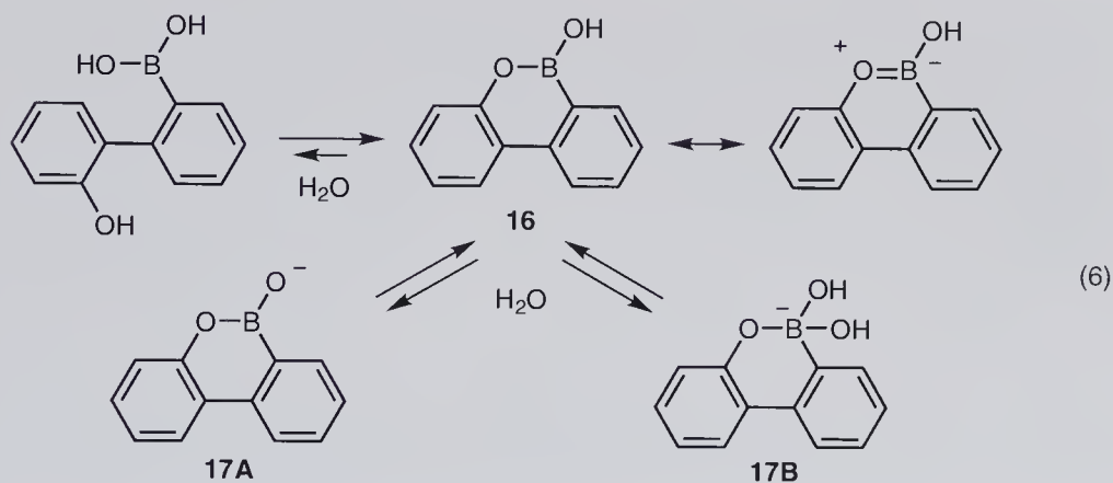
Figure 1.7 Ionization equilibrium for special types of boronic acids.
