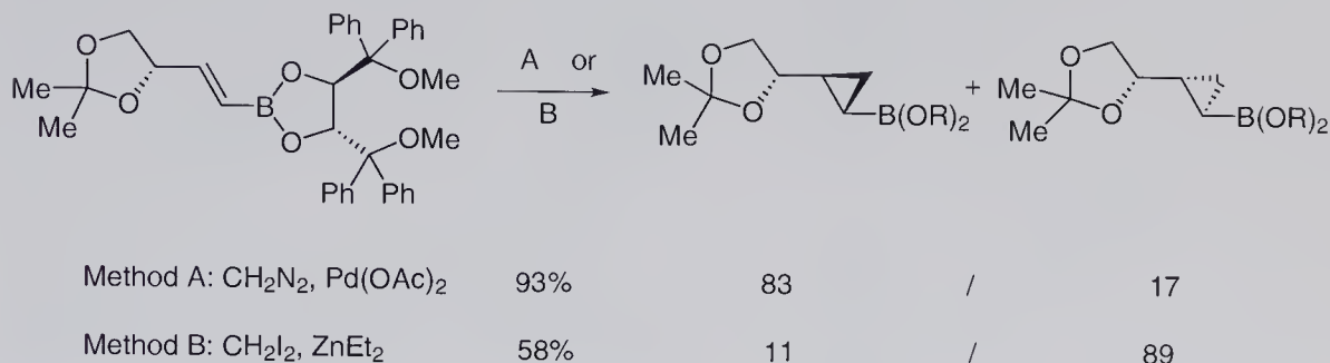
Scheme 9.17 Cyclopropanation of an alkenylboronic ester containing a chiral diol and an additional stereogenic center.
