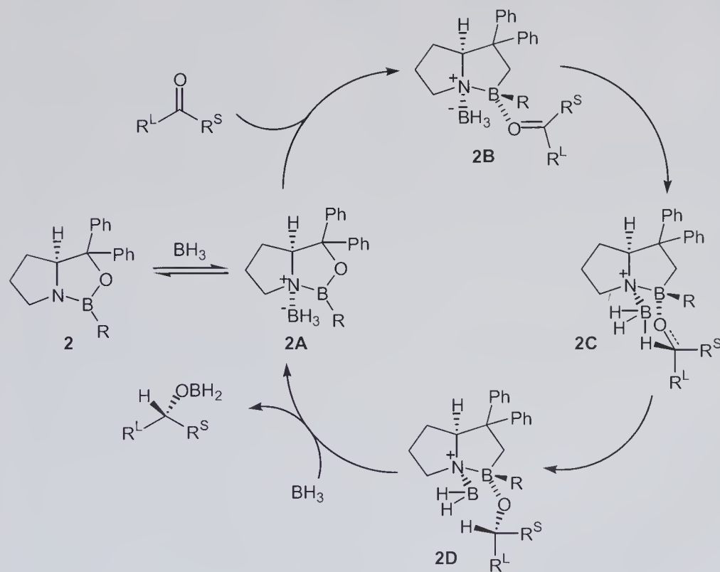
Scheme 11.3 Proposed mechanism of the 2 -catalyzed reduction of ketones.
