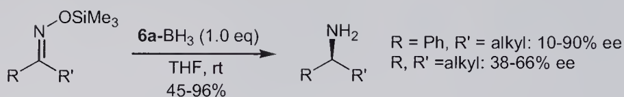
Scheme 11.19 OAB-induced reduction of ketoxime ether derivatives.
