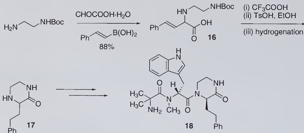
Scheme 7.4 Synthesis of 2-piperazinones using the Petasis borono-Mannich reaction.
