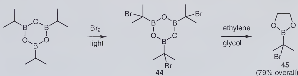
Scheme 8.9 Bromination of 2,4,6-(triisopropyl)boroxine.
