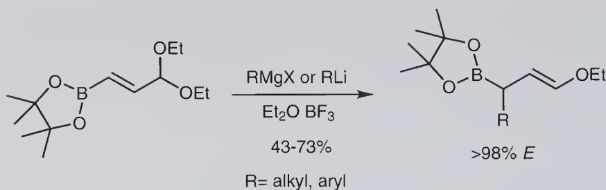
Scheme 9.7 Stereoselective synthesis of \gamma -alkoxyallylboronates.
