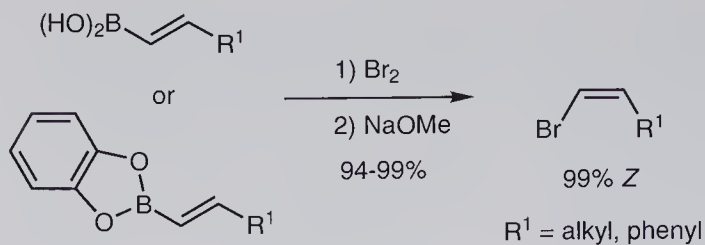
Scheme 9.1 Bromination of alkenylboronic acids and esters.
