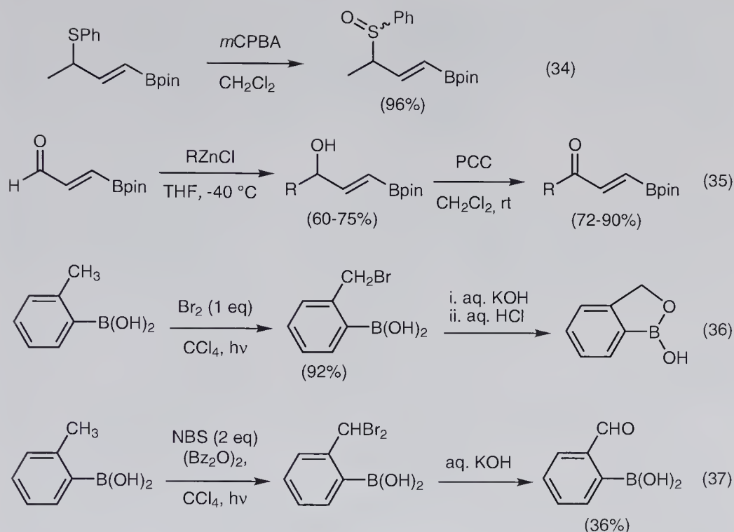
Figure 1.24 Chemoselective oxidation reactions involving boronic acid derivatives.
