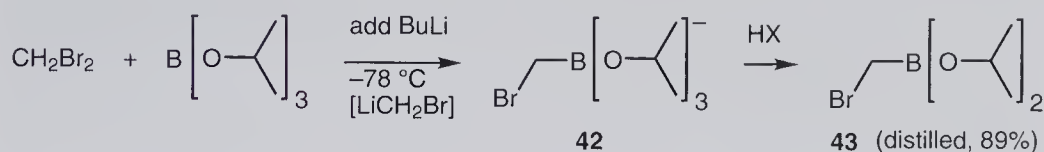
Scheme 8.8 Preparation of diisopropyl(bromomethyl)boronate.
