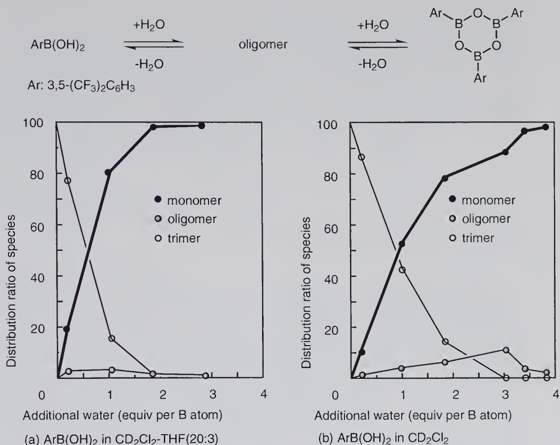
Figure 10.6 Plot of the distribution of species in a solution of 3,5-(CF 3 ) 2 C 6 H 3 B(OH) 2 versus additional water.
