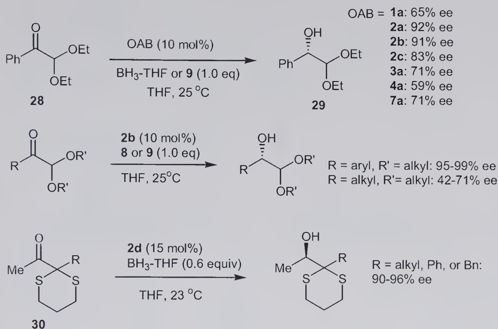
Scheme 11.8 OAB-catalyzed reduction of \alpha -keto acetals and thioketals.
