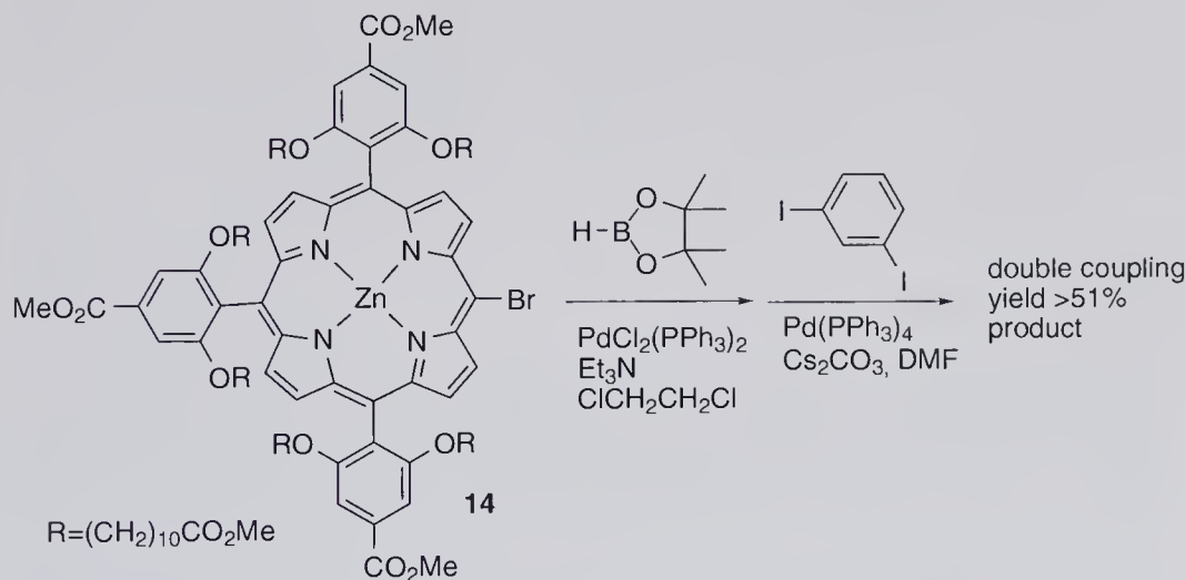
Scheme 2.2 Arylboron compounds via coupling reaction of pinacolborane.
