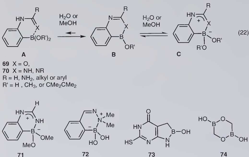
Figure 1.16 Hemi-heterocyclic “internal” boronic ester derivatives.
