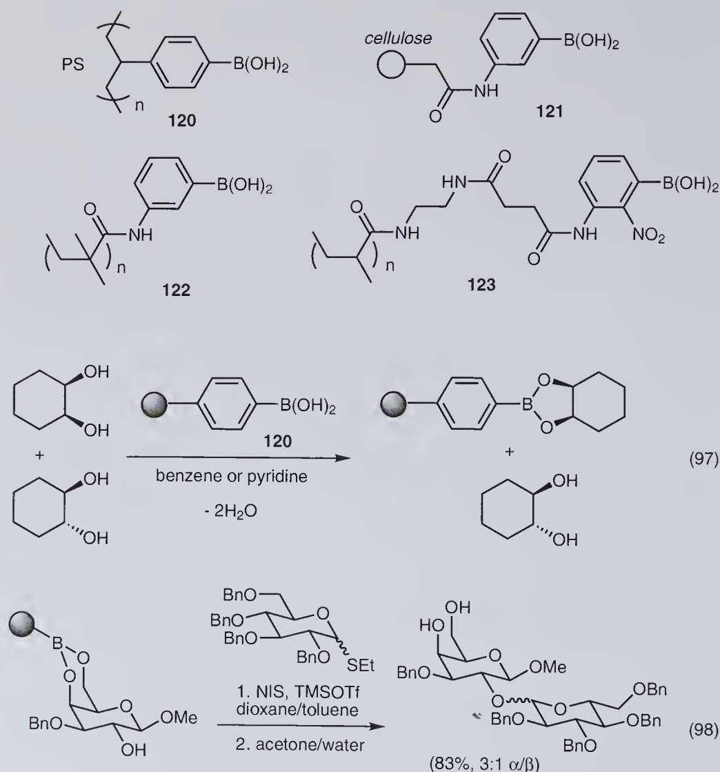
Figure 1.44 Boronic acid supports for diol compounds.
