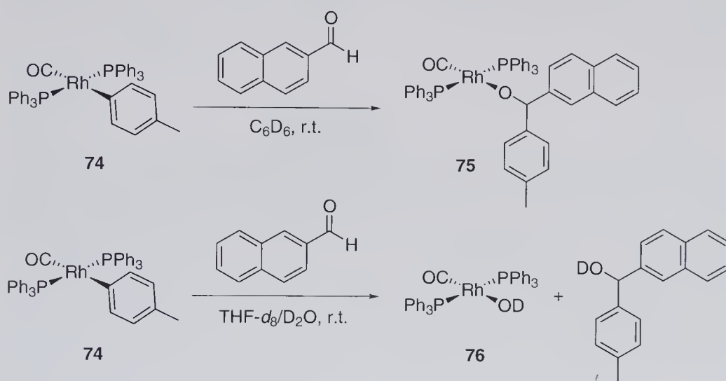
Scheme 4.36 Control reactions of arylrhodium complex 74 with 2-naphthaldehyde.
