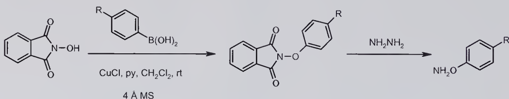
Scheme 5.4 Application of O -arylation in aryloxyamine syntheses.
