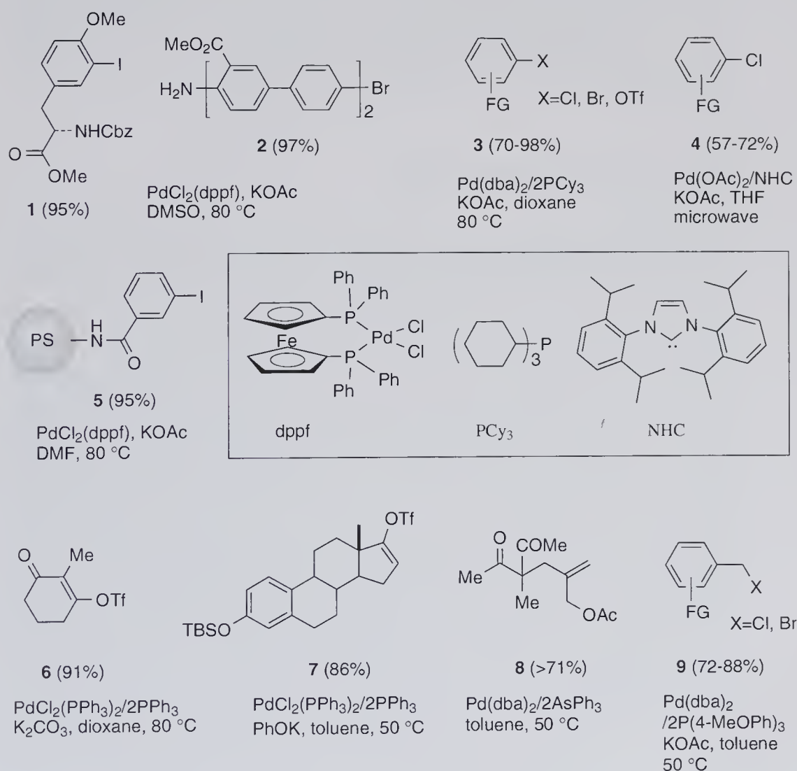
Scheme 2.1 Organoboron compounds via cross-coupling reactions of diborons.
