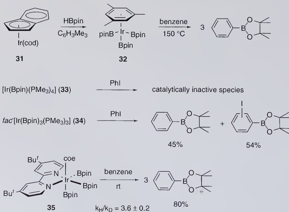
Scheme 2.13 tris(Boryl)Ir(III) intermediates involved in the catalytic cycle.
