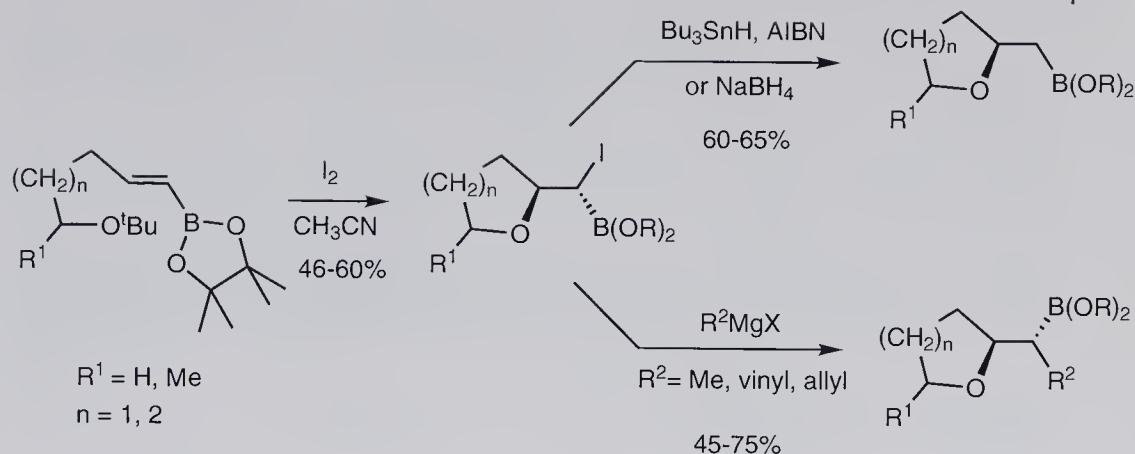
Scheme 9.4 Intramolecular iodoetherification of alkenylboronic esters.
