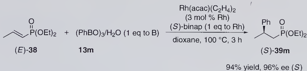
Scheme 4.15 Catalytic asymmetric conjugate addition to propenylphosphonate 38 .
