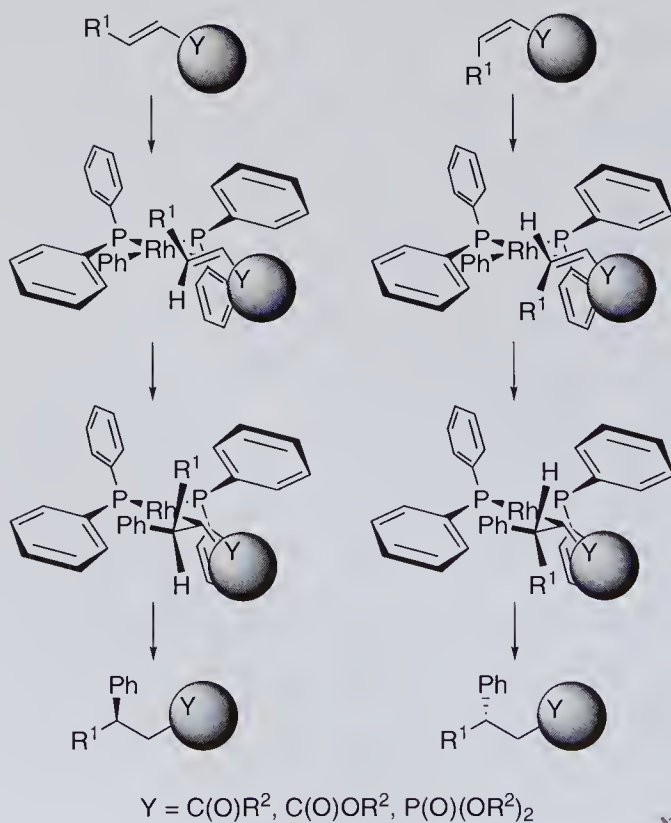
Scheme 4.8 Proposed stereochemical pathway in the conjugate addition catalyzed by rhodium ( S )-binap complex.
