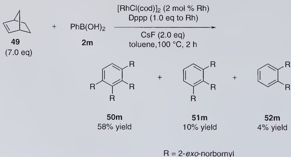
Scheme 4.21 Rhodium-catalyzed multiple alkylation of phenylboronic acid.
