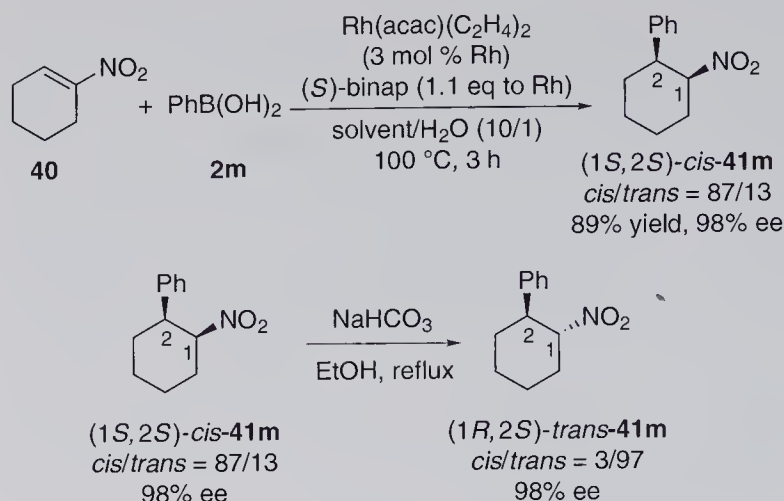
Scheme 4.16 Catalytic asymmetric conjugate addition to nitrocyclohexene 40.
