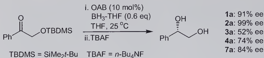
Scheme 11.6 OAB-catalyzed reduction of \alpha -silyloxy ketones.
