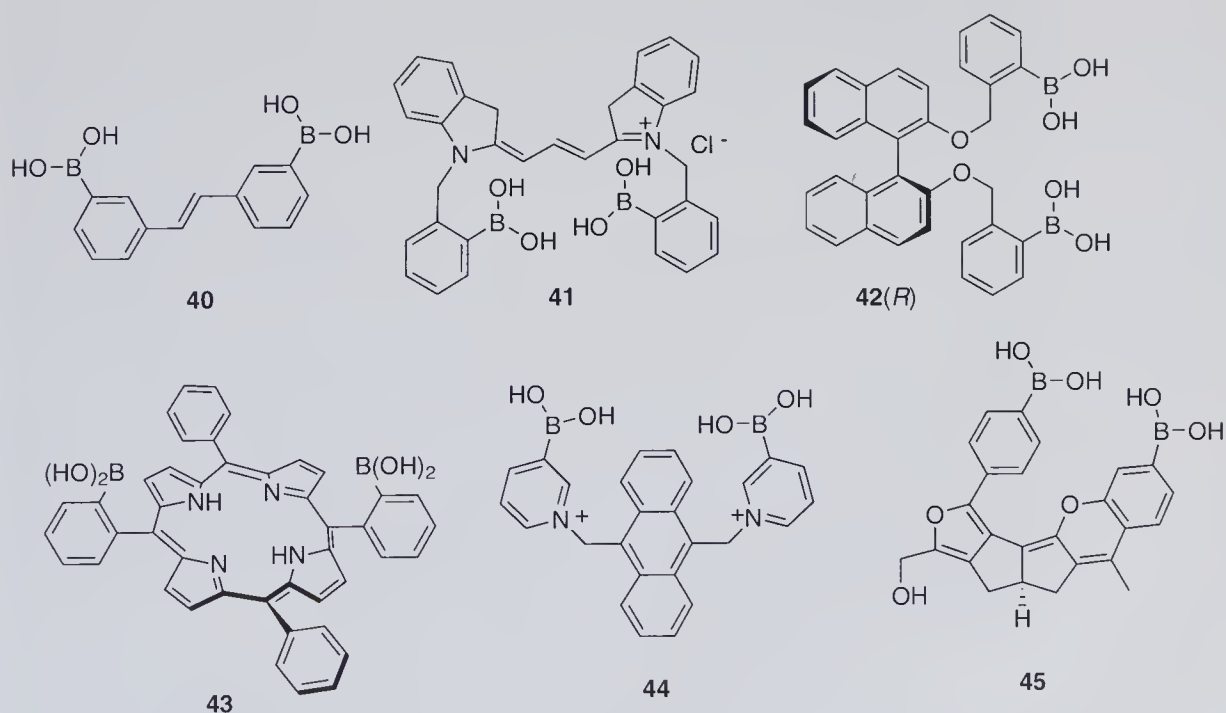
Figure 12.10 Diboronic acid fluorescent sensors.
