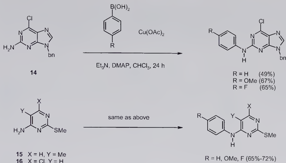
Scheme 5.7 C–N cross-coupling of aminapurines and aminopyrimidines.
