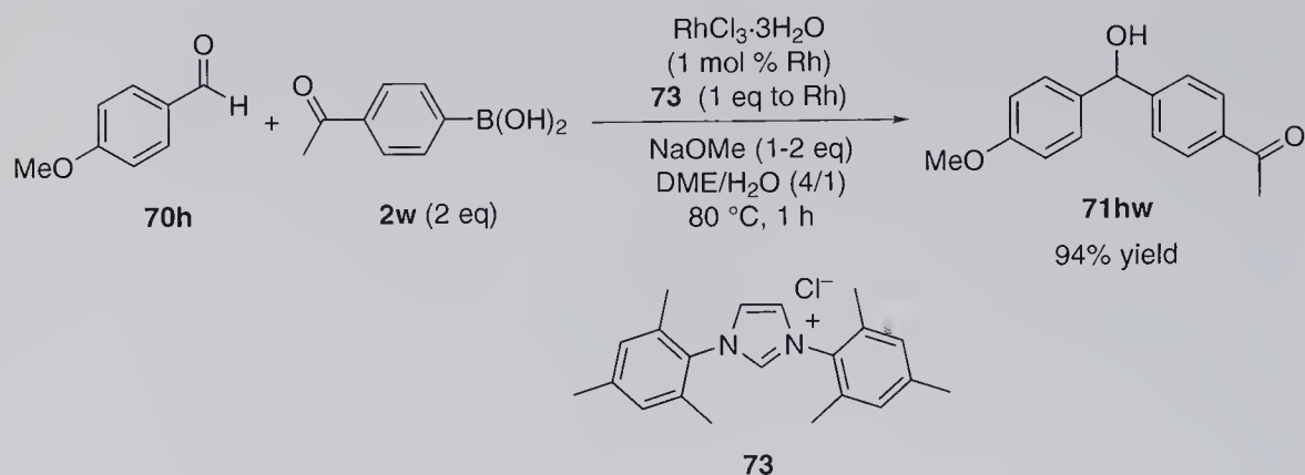
Scheme 4.33 Continued.
