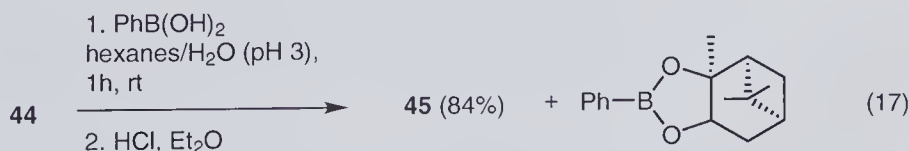
Figure 1.11 Cleavage of pinanediol boronic esters.
