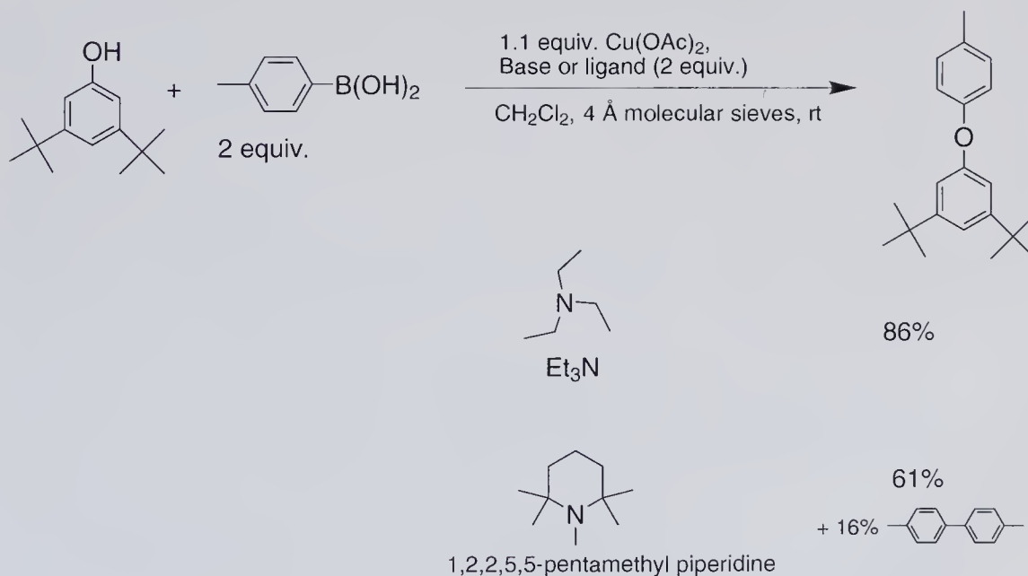
Scheme 5.32 Study on the role of base/ligand.
