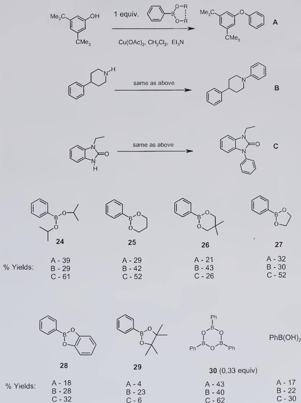
Scheme 5.26 N- and O-Arylation with phenylboronic acid esters.
