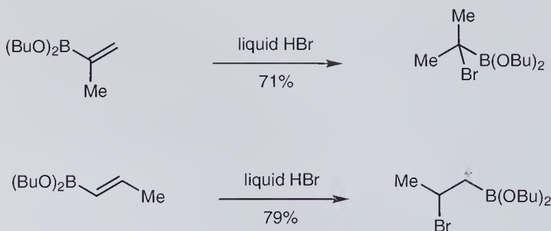
Scheme 9.3 Addition of hydrogen bromide to alkenylboronic esters.
