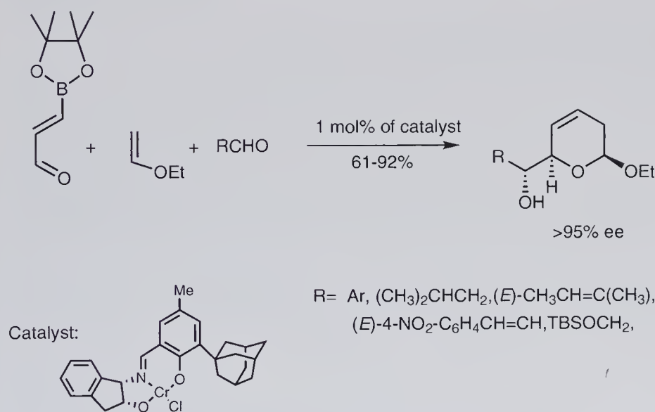
Scheme 9.37 Asymmetric synthesis of \alpha -hydroxylated dihydropyrans via a catalytic hetero-Diels–Alder cycloaddition/allylboration sequence.
