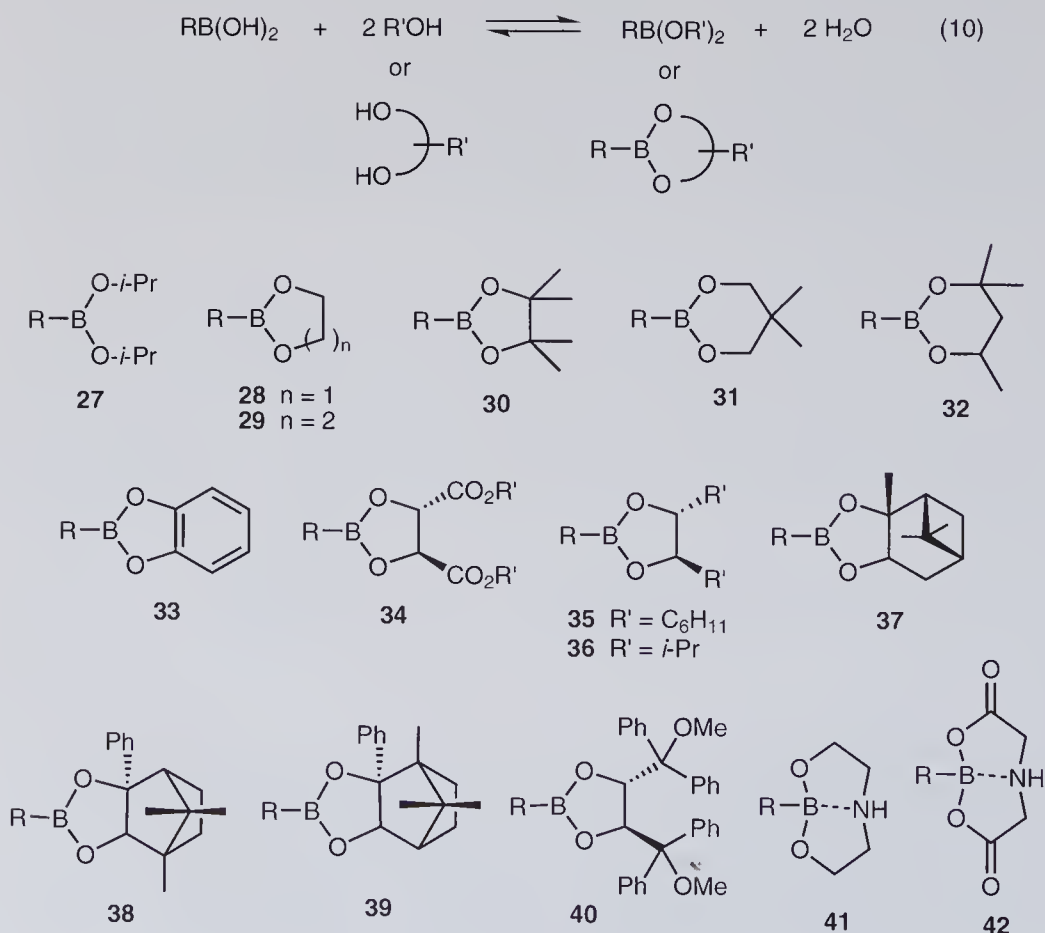
Figure 1.9 Common boronic esters.
