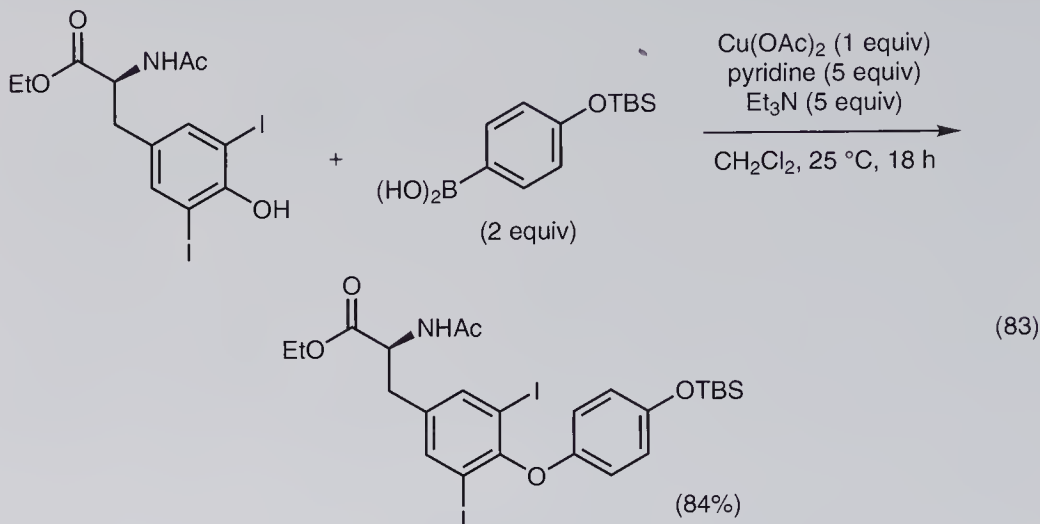
Figure 1.40 Copper-catalyzed coupling of boronic acids with nucleophilic oxygen and nitrogen-containing compounds.
