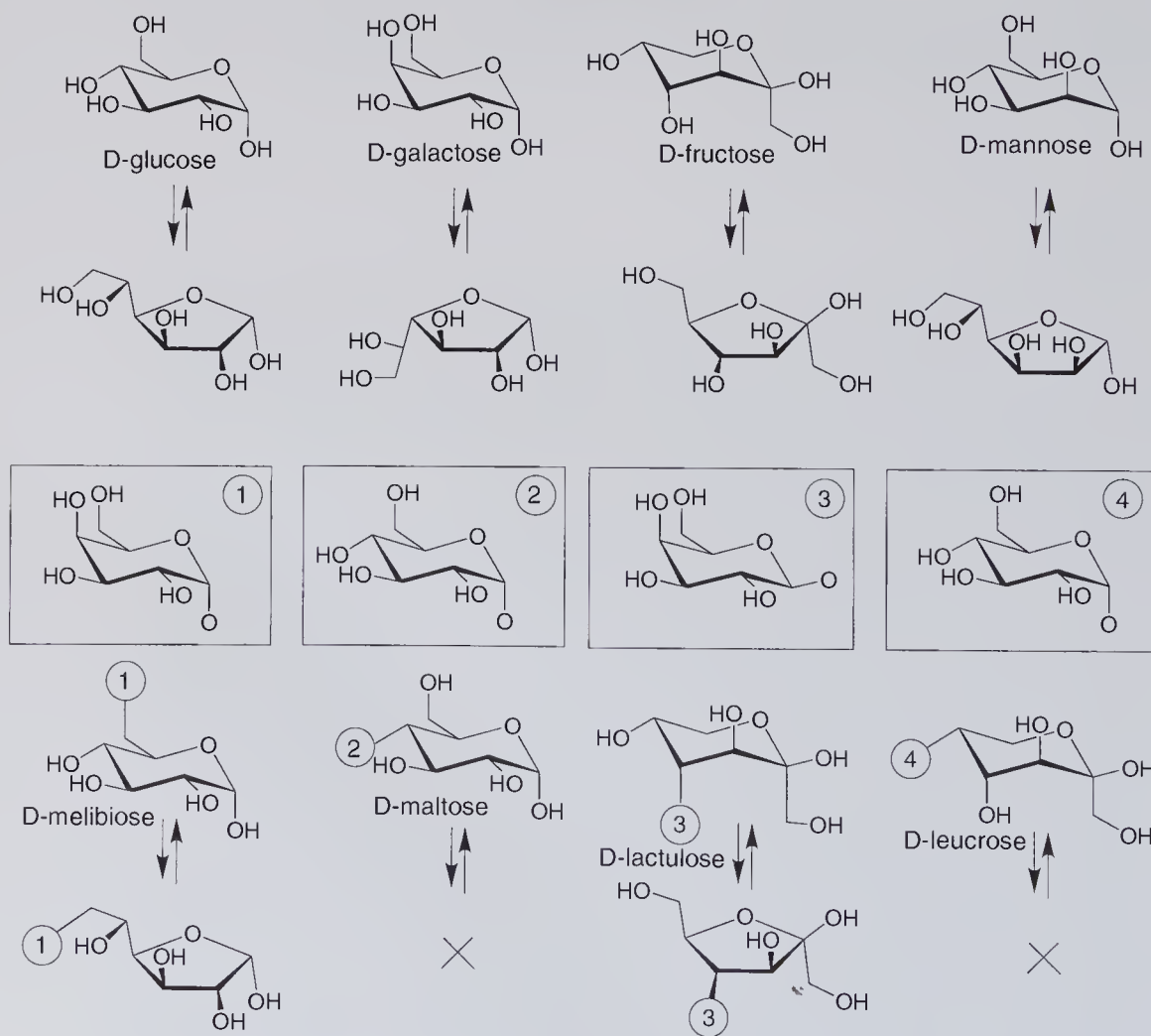
Figure 12.1 Pyranose to furanose isomerization for selected saccharides.
