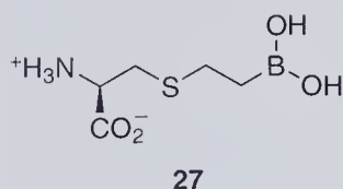
Figure 13.6 Structure of ( S )-(2-boronoethyl)-L-cysteine (BEC, 27 ).
