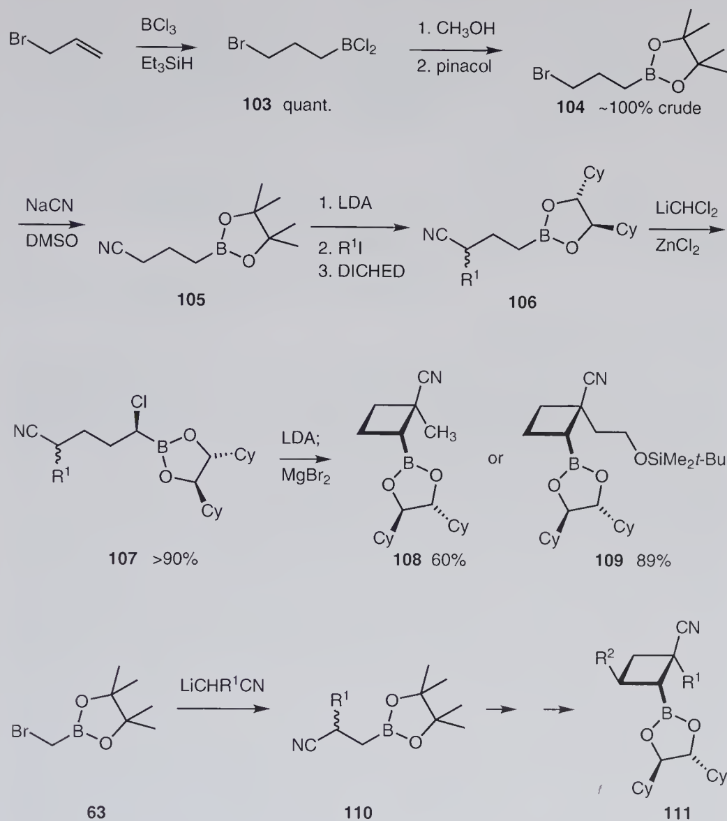
Scheme 8.24 Synthesis of di- and trisubstituted (cyclobutyl)boronic esters. Yields of 106 from 104 generally high, not reported in detail. Removal of \text{Et}_3\text{SiCl} from 104 by distillation was incomplete.
