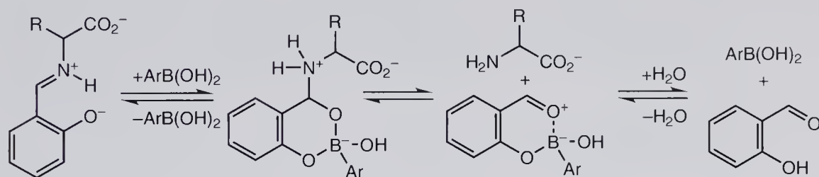
Scheme 10.3 Hydrolysis of salicylaldehyde imines catalyzed by \text{ArB(OH)}_2 .
