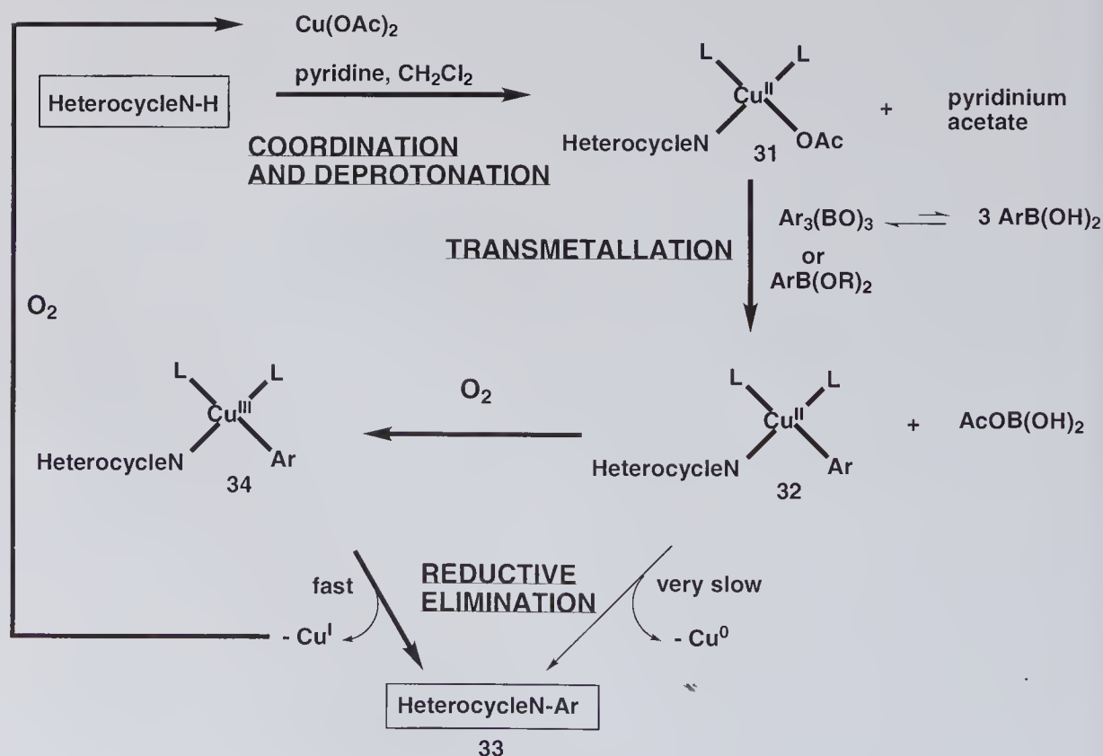
Scheme 5.33 Possible mechanism for copper-promoted N-arylation.
