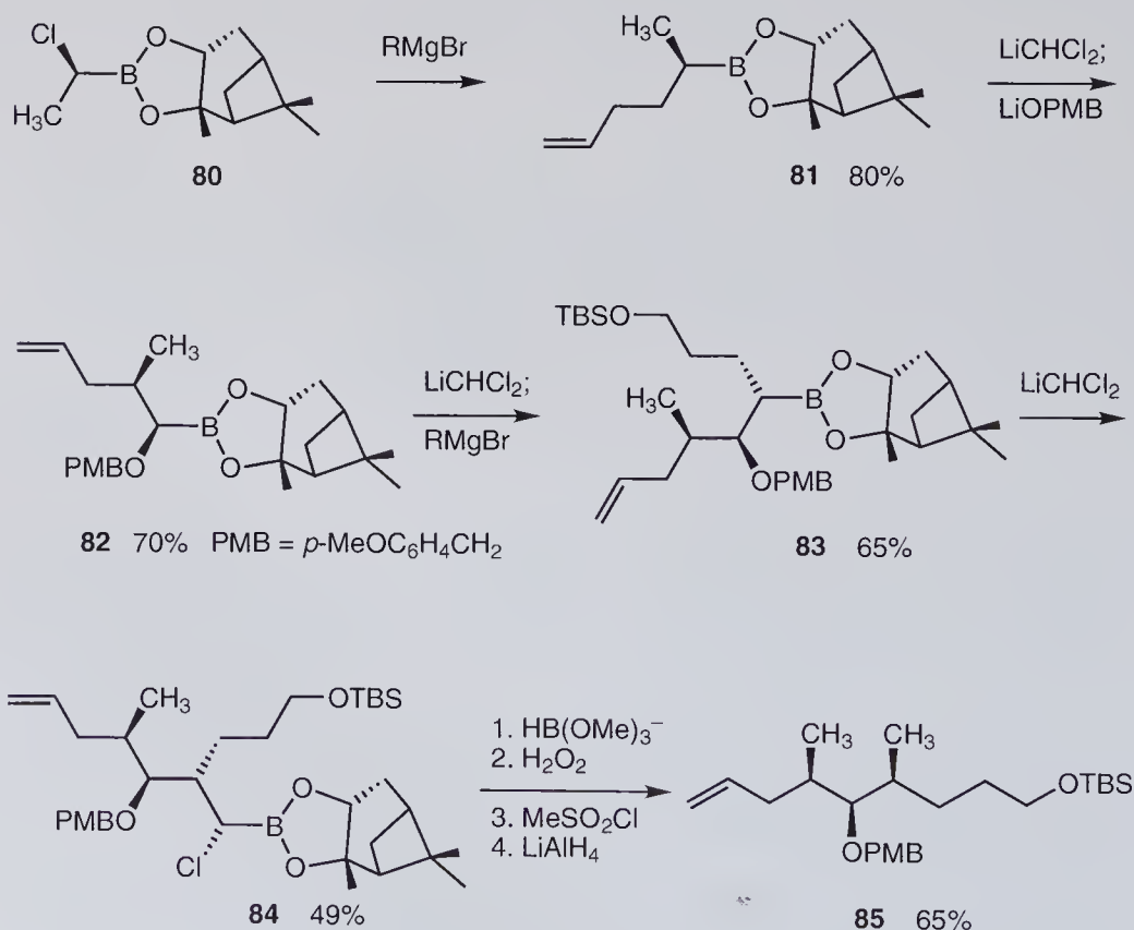
Scheme 8.17 Intermediates for synthesis of a tautomycin fragment. Conditions for reactions with LiCHCl 2 and replacement of chloride for conversion of 80 into 84 are similar to those outlined in Schemes 8.1 and 8.3.
