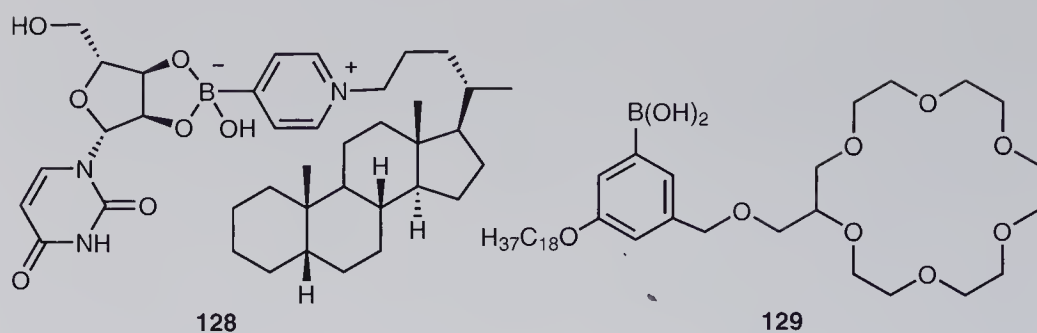
Figure 1.46 Examples of boronic acid based transporters.
