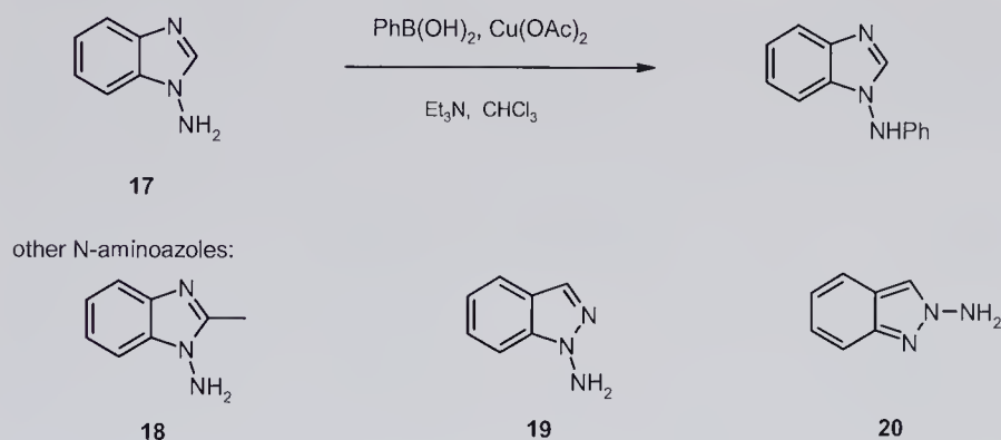
Scheme 5.8 C–N cross-coupling of N-aminoazoles.
