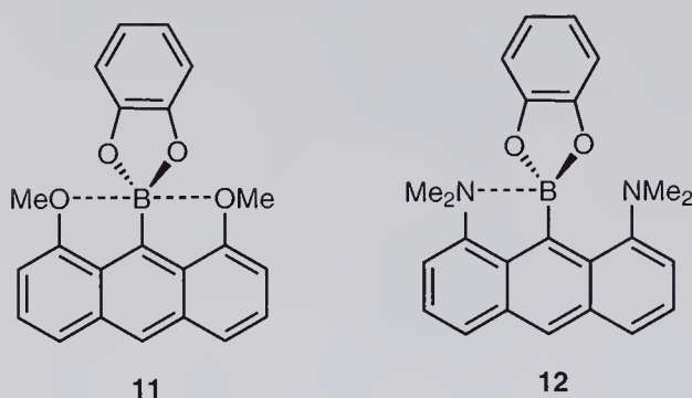
Figure 1.4 Model compounds for boronate hypercoordination.
