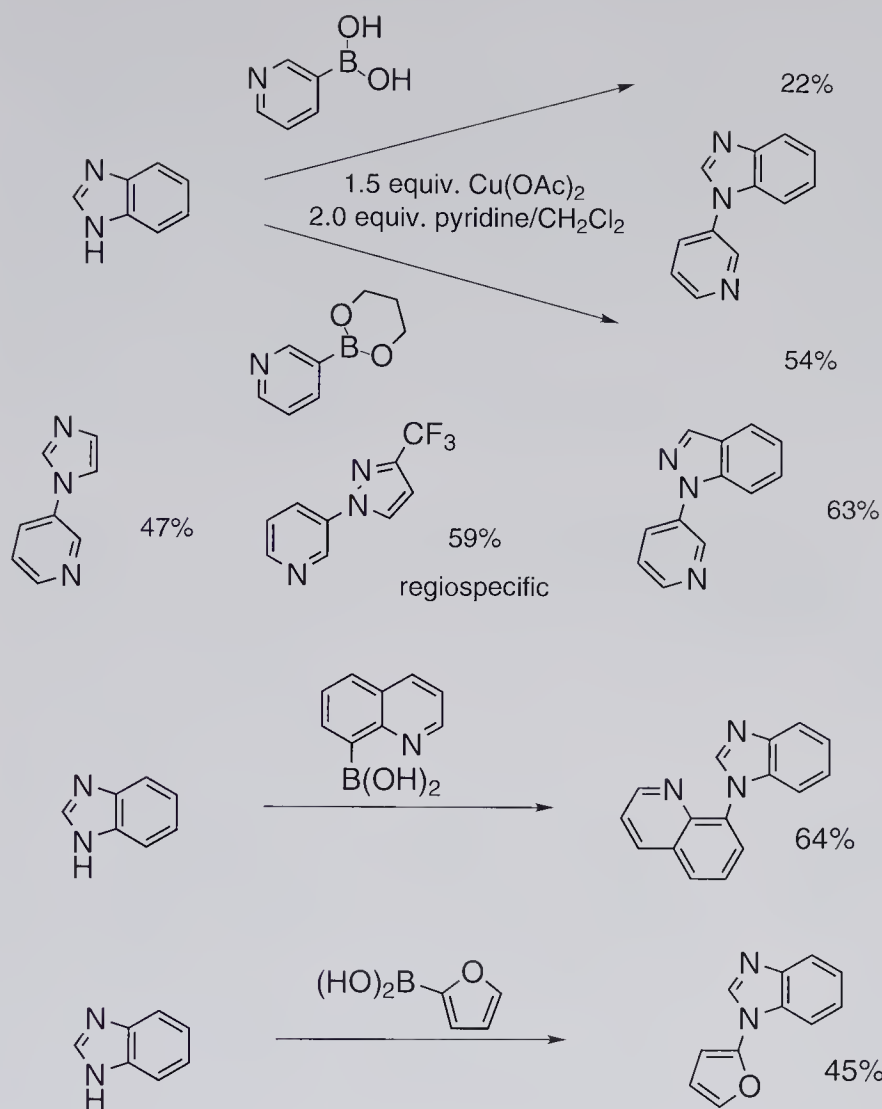
Scheme 5.21 Heteroarene–heteroarene C–N cross-couplings.
