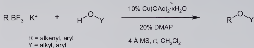
Scheme 5.27 Cu(II)-catalyzed ether synthesis with organotrifluoroborate salts.
