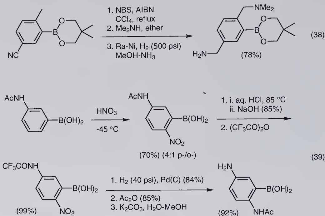
Figure 1.25 Chemoselective reduction reactions involving boronic acid derivatives.
