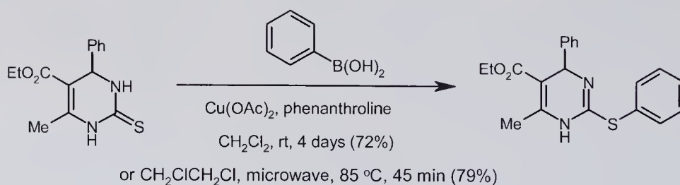
Scheme 5.25 S-Arylation with phenylboronic acid.
