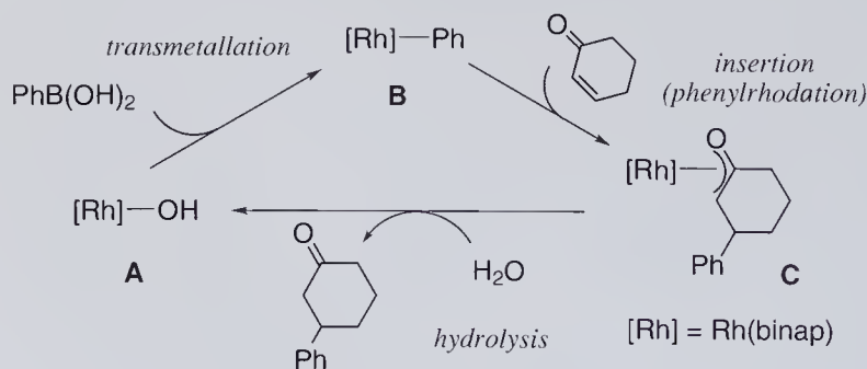
Scheme 4.4 Catalytic cycle for the rhodium-catalyzed conjugate addition.
