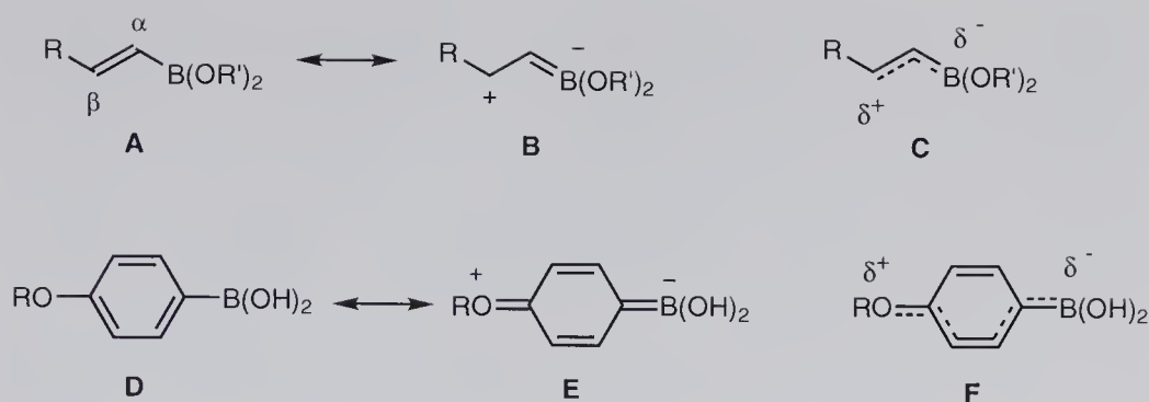
Figure 1.5 Limit mesomeric forms involving B–C \pi overlap.
