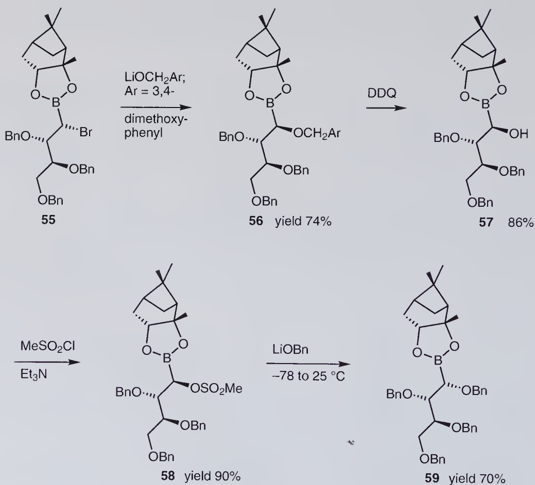
Scheme 8.13 Double inversion of an ( \alpha -bromoalkyl)boronic ester.
