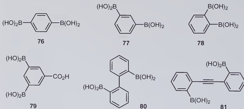
Figure 1.20 Selected examples of diboronic acids.
