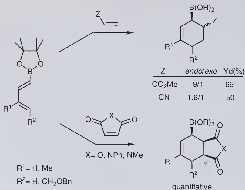
Scheme 9.29 Diels–Alder reactions of 1,3-dienylboronates.
