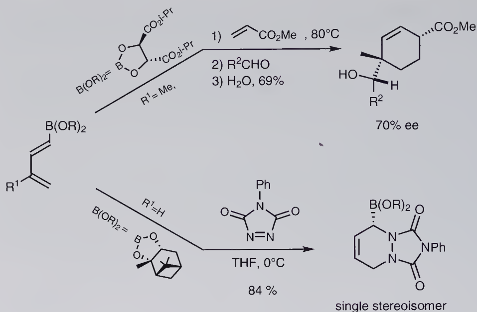
Scheme 9.35 Asymmetric Diels–Alder reaction of chiral 1,3-dienylboronates.
