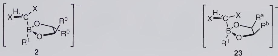
Scheme 8.4 Lack of diastereoselectivity in reactions of pinanediol ( \alpha -chloroalkyl)boronates.
