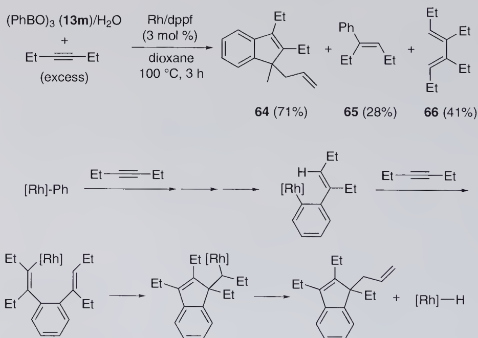
Scheme 4.30 Rhodium-catalyzed tandem hydroarylation–carbocyclization of 3-hexyne with phenylboronic acid.
