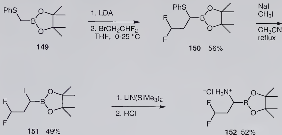
Scheme 8.35 Preparation of a fluorinated ( \alpha -aminoalkyl)boronic ester.
