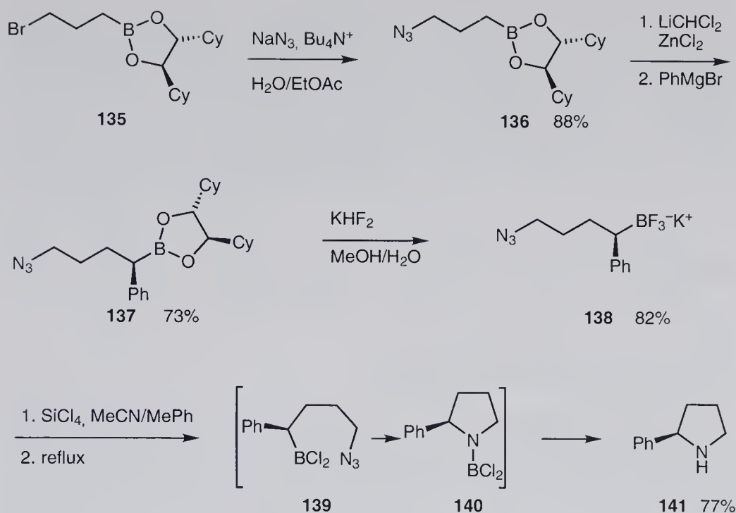
Scheme 8.32 Synthesis of ( R )-2-phenylpyrrolidine ( 141 ).
