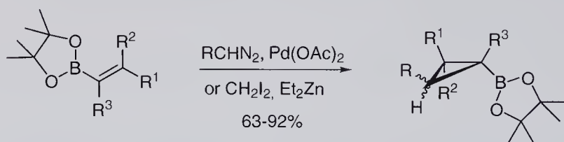
Scheme 9.15 Carbene additions to alkenylboronic esters.
