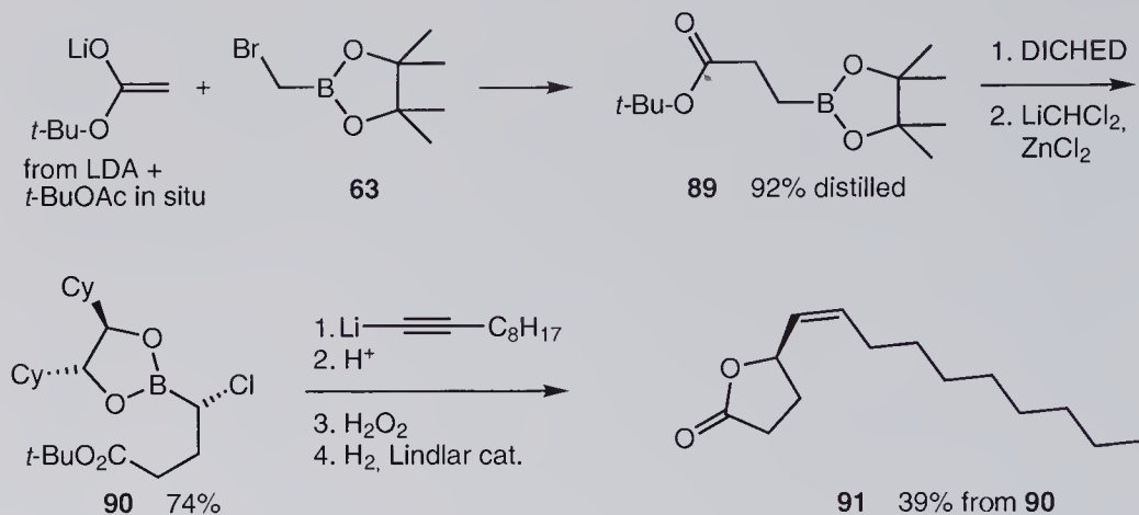
Scheme 8.19 Synthesis of japonilure ( 91 ).
