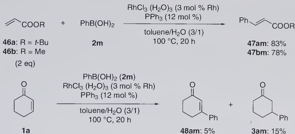
Scheme 4.19 Rhodium-catalyzed Heck-type reaction of \alpha,\beta -unsaturated olefins with organoboronic acids.
