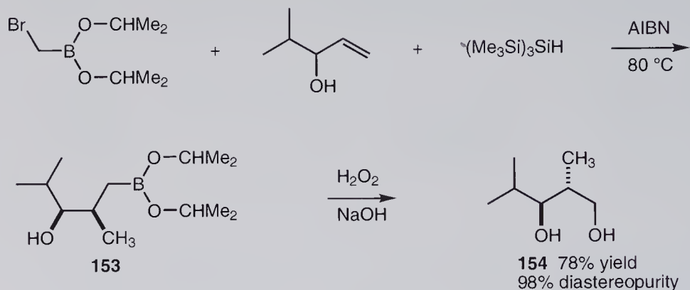
Scheme 8.36 Diastereoselective reaction of diisopropyl(bromomethyl)boronate with an al-
