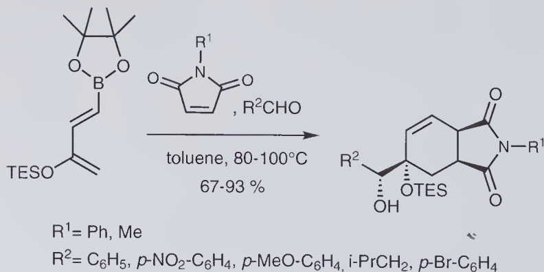
Scheme 9.33 Synthesis of hydroxylated cyclohexenes via tandem [4+2] cycloaddition/allylboration.
