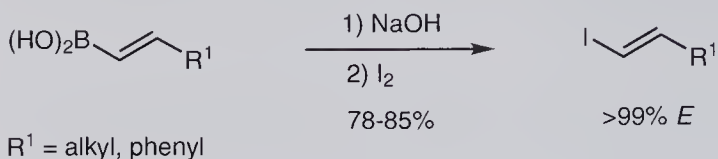
Scheme 9.2 Synthesis of 1-iodoalkenes from 1-alkenylboronic acids.
