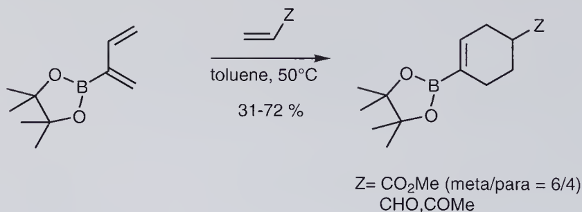
Scheme 9.39 Cycloaddition reaction of pinacol (1,3-butadien-2-yl)boronate to dienophiles.
