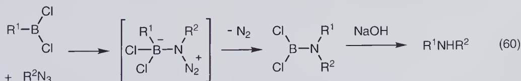
Figure 1.33 Oxidative amination of boronic acid derivatives.
