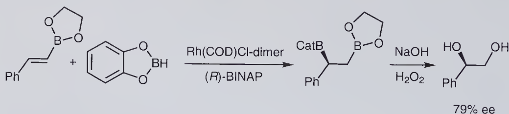
Scheme 9.55 Rhodium-catalyzed enantioselective hydroboration of an alkenylboronate.
