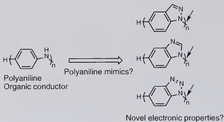
Scheme 5.12 Novel compounds containing heteroarene–arene C–N bonds.
