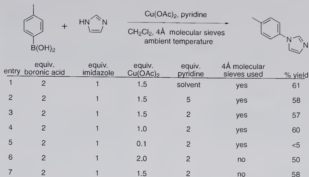
Scheme 5.36 Molecular sieves and base/ligand studies.
