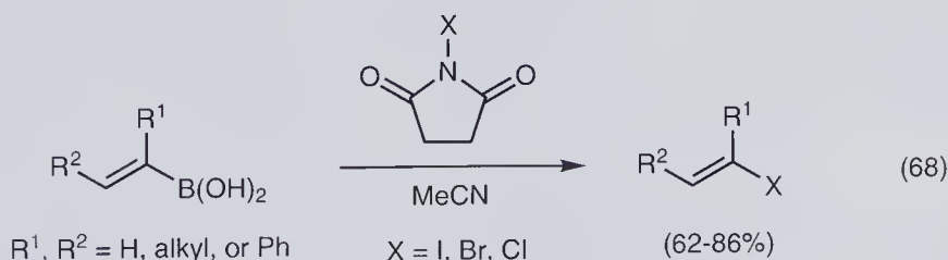
Figure 1.35 Halogenation of alkenylboronic acids (esters).
