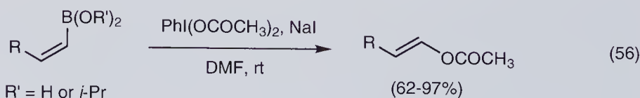
Figure 1.32 Oxidation of boronic acids (esters).
