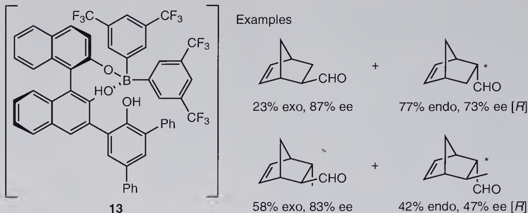
Figure 10.7 Diels–Alder reaction catalyzed by 5 mol% of 13 .
