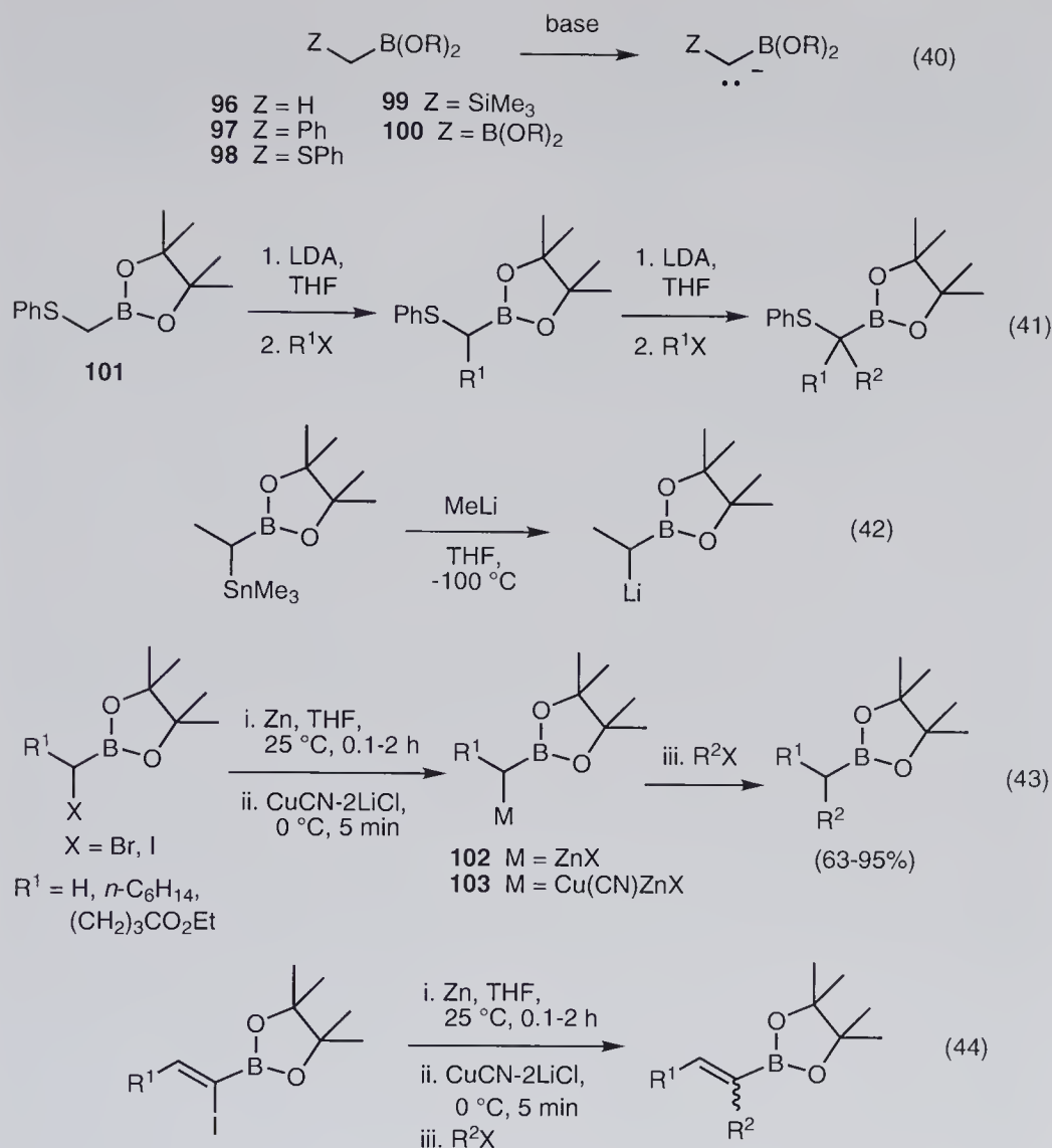
Figure 1.26 Formation and reactions of boronyl-substituted carbanions.
