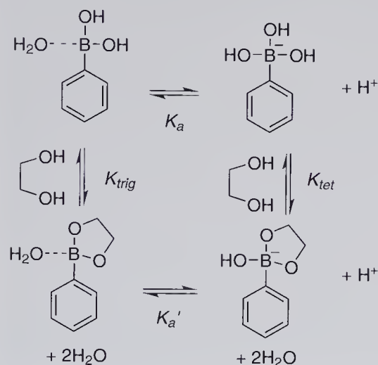
Scheme 12.1
