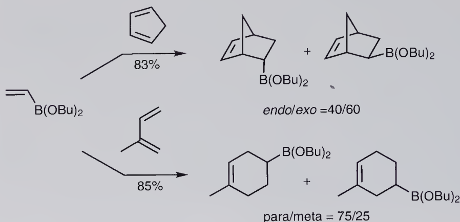
Scheme 9.19 [4+2] cycloaddition of dibutyl(ethylene)boronate to cyclopentadiene and isoprene.
