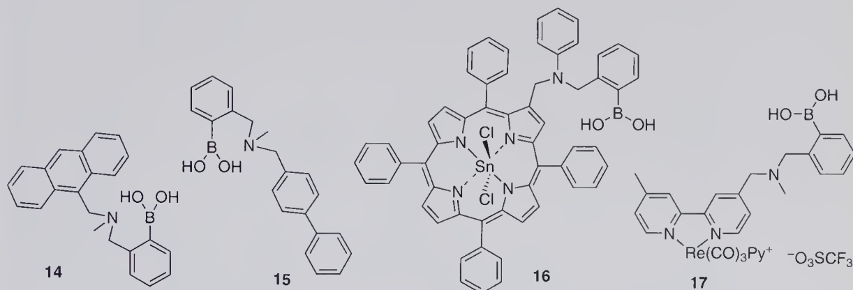
Figure 12.3 Monoboronic acid photoinduced electron transfer (PET) fluorescent sensors.
