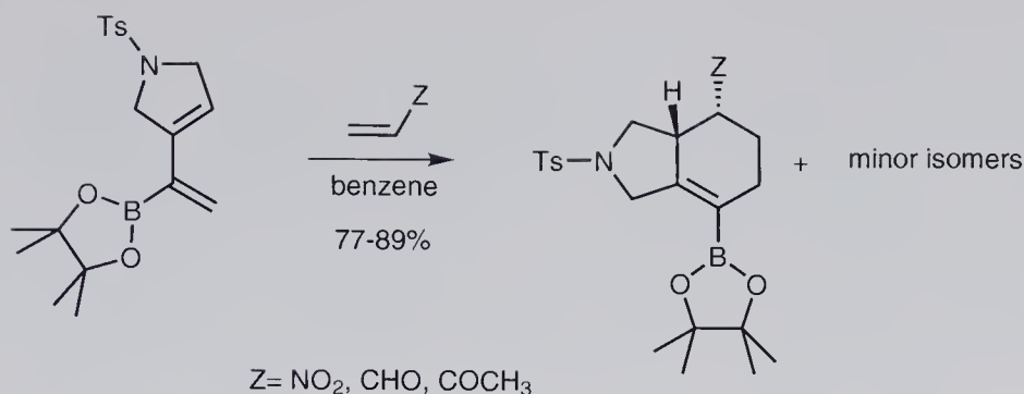
Scheme 9.40 Diels–Alder cycloaddition of a cyclic 1,3-dienyl-2-boronate.
