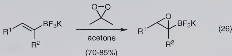
Figure 1.17 Synthesis of dichloroboranes, monoalkylboranes, and trifluoroborate salts.
