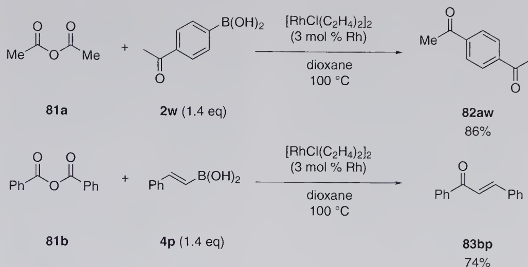
Scheme 4.39 Rhodium-catalyzed addition of organoboronic acids to anhydrides.
