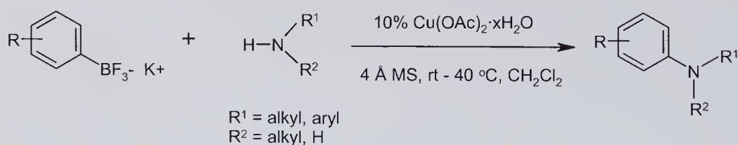
Scheme 5.28 Cu(II)-catalyzed C–N bond formation with organotrifluoroborate salts.
