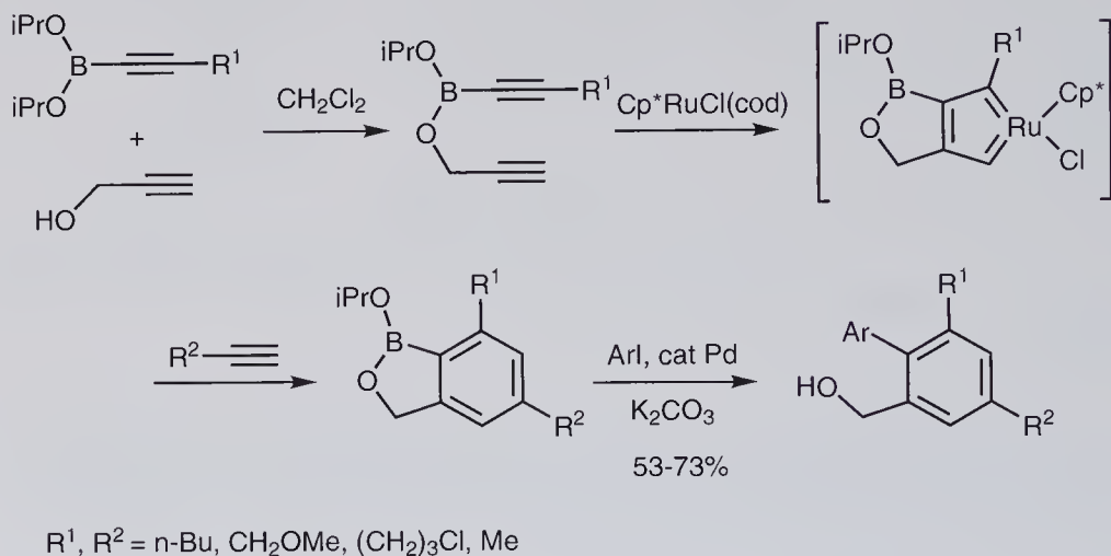
Scheme 9.50 One-pot four-component reactions via cyclotrimerization/Suzuki–Miyaura coupling.
