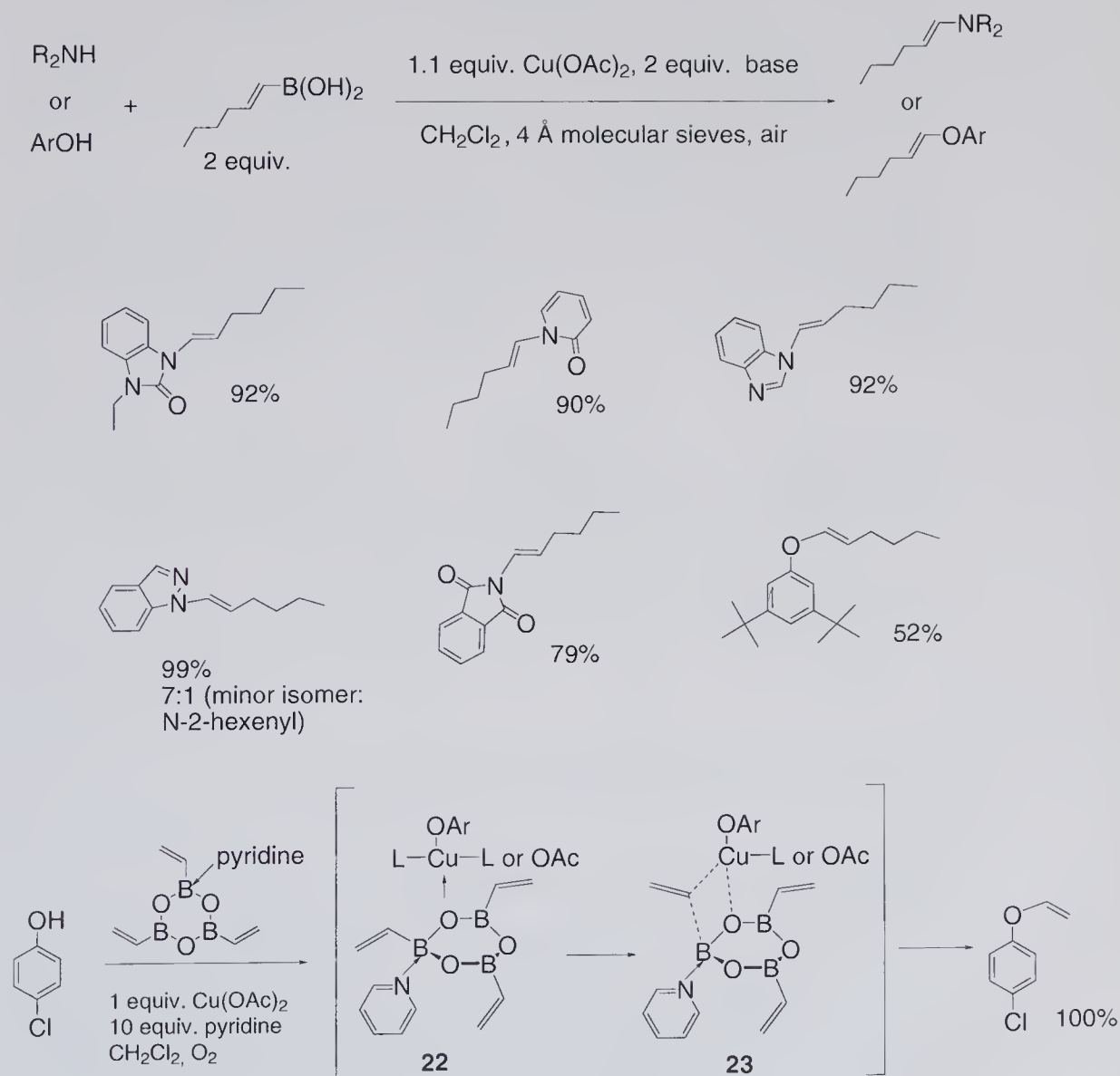
Scheme 5.24 N/O-Vinylation with trivinylboroxine-pyridine.
