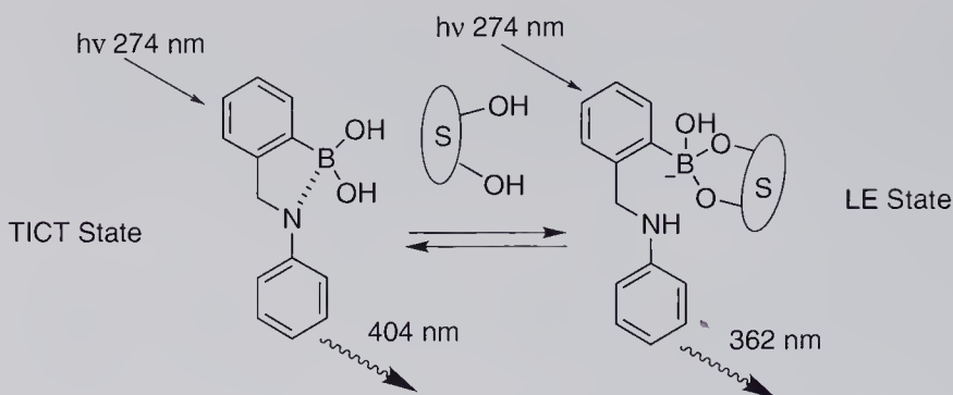
Scheme 12.3 Locally excited (LE) and twisted internal charge transfer (TICT) states of 12a .
