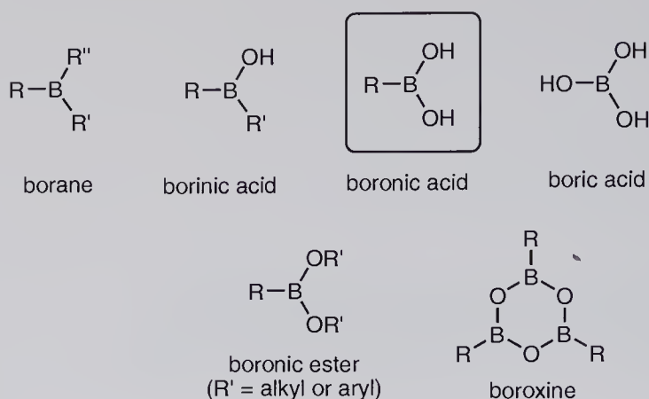
Figure 1.1 Oxygenated organoboron compounds.
