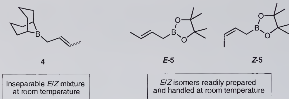
Figure 6.3 Comparison of the stereochemical stability of allylboranes vs. allylboronates.
