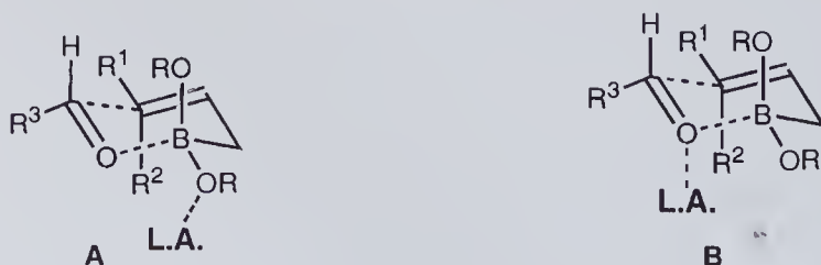
Figure 6.6 Possible transition structures for the Lewis acid-catalyzed allylboration. (A) Coordination of a boronate oxygen. (B) Double coordination of the aldehyde carbonyl.
