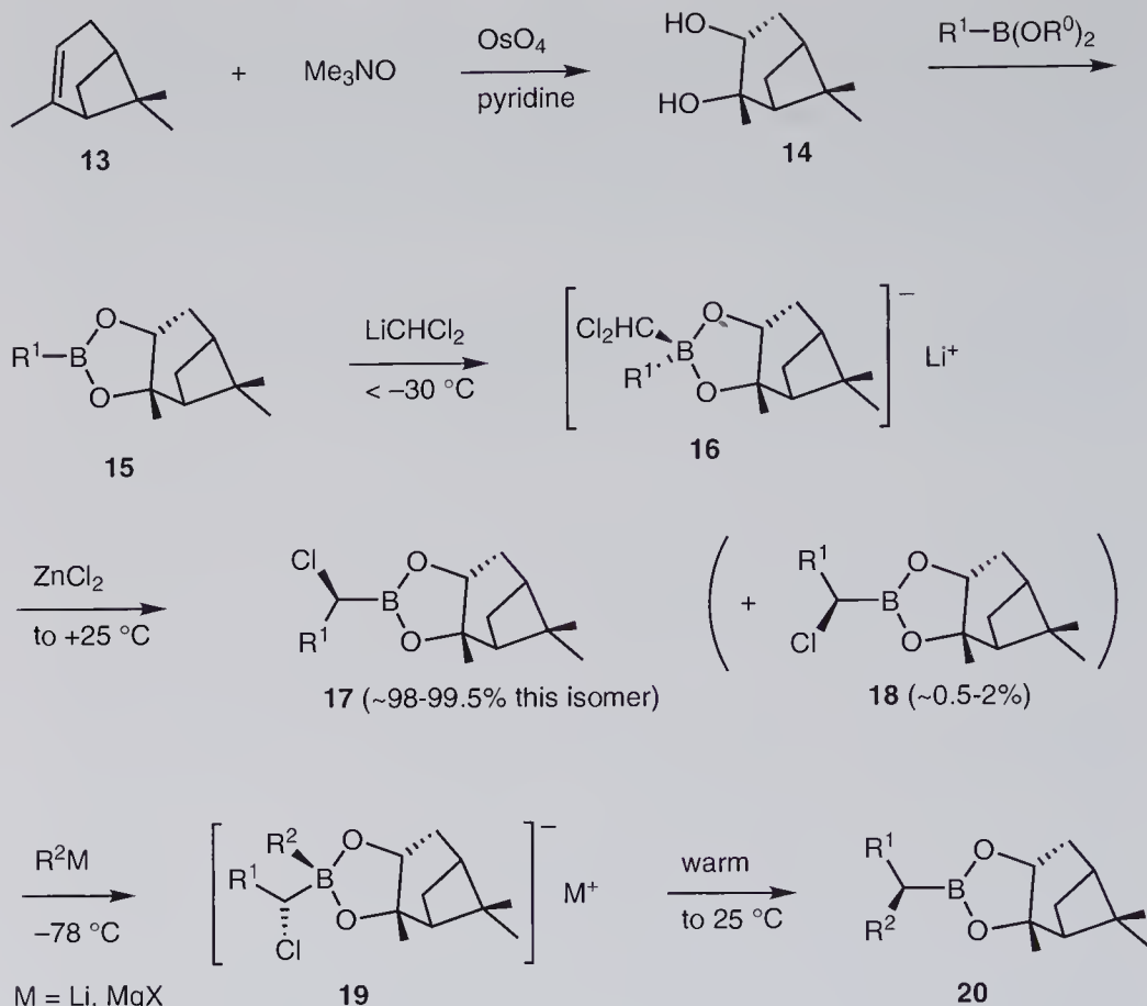
Scheme 8.3 General assembly of asymmetric carbon chains via pinanediol boronic esters. Structures 13 – 20 are drawn as slightly distorted planar projections of a three-dimensional computer model of the rigid terpenoid unit. For detailed reaction conditions, see Scheme 8.1.
