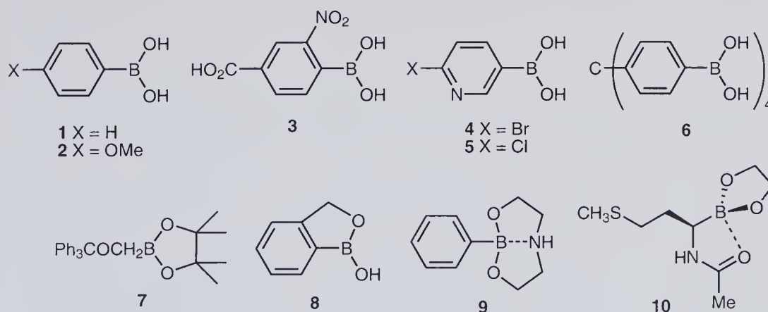
Figure 1.2 Boronic acid derivatives analyzed by X-ray crystallography.
