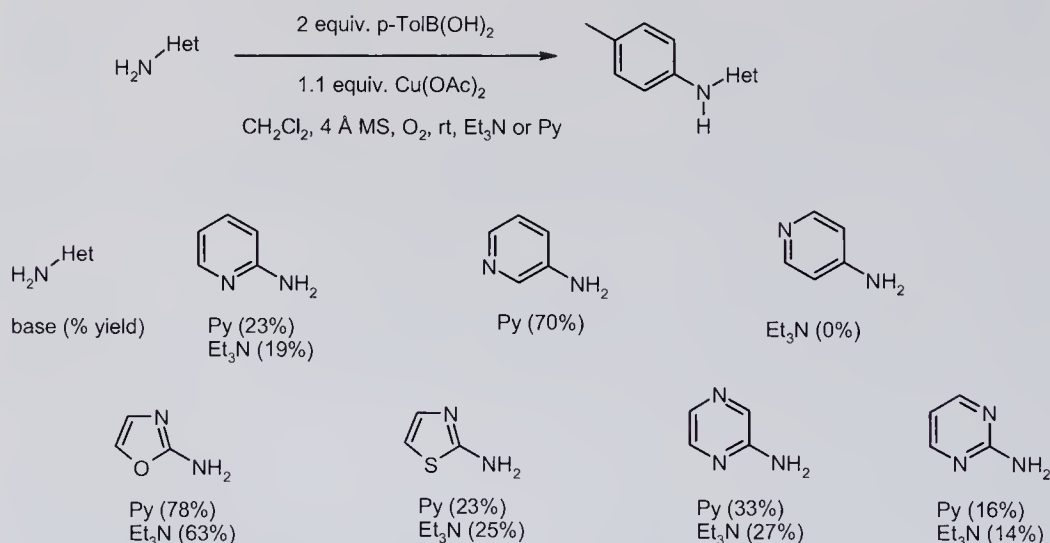
Scheme 5.6 C–N cross-coupling of heterocyclic amines.
