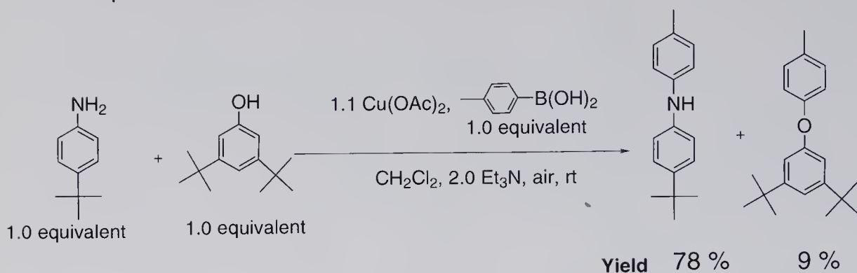
Scheme 5.22 Competition experiment of O- vs. N-arylation.
