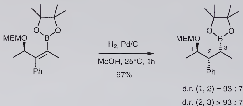
Scheme 9.54 Diastereoselective hydrogenation of an alkenylboronic ester.
