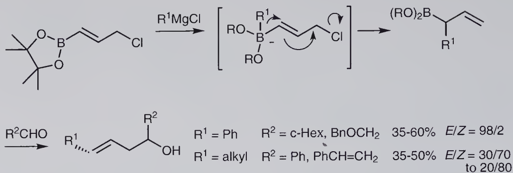
Scheme 9.6 Synthesis of homoallylic alcohols from (3-chloroprop-1-en-1-yl)boronate.
