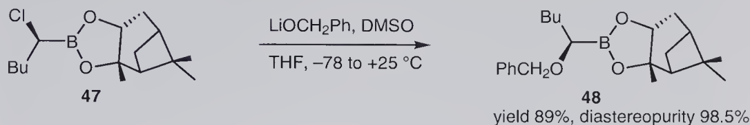
Scheme 8.11 Preparation of ( S )-pinanediol ( R )-[1-(benzyloxy)pentyl]boronate.
