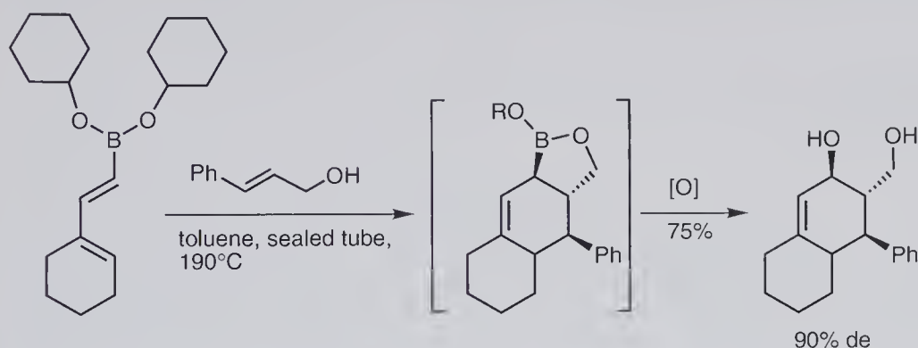
Scheme 9.34 Boron-tethered intramolecular Diels–Alder reaction of 1,3-dienylboronates.
