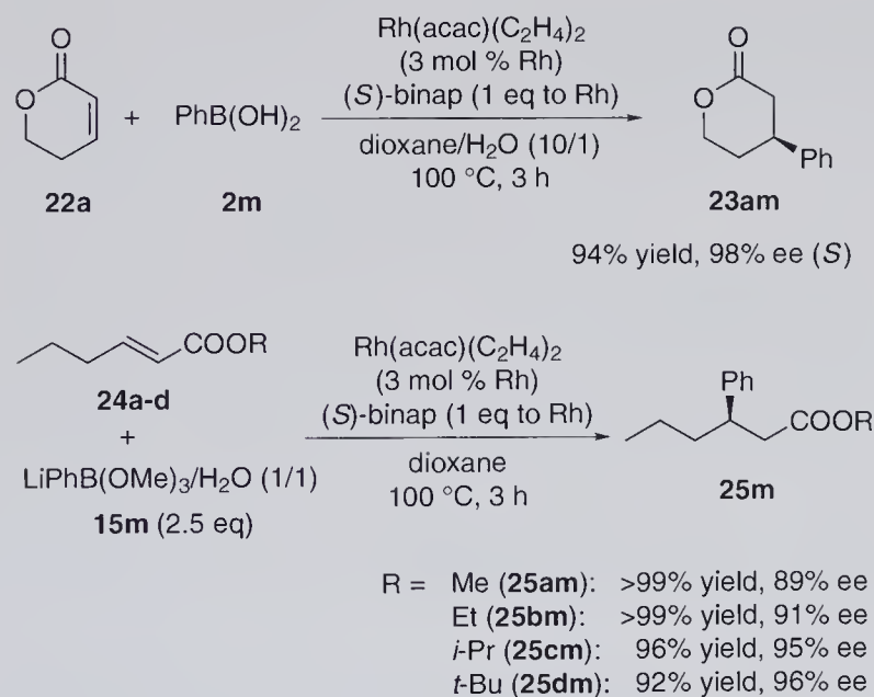
Scheme 4.9 Asymmetric conjugate addition of organoboron reagents to \alpha,\beta -unsaturated esters.
