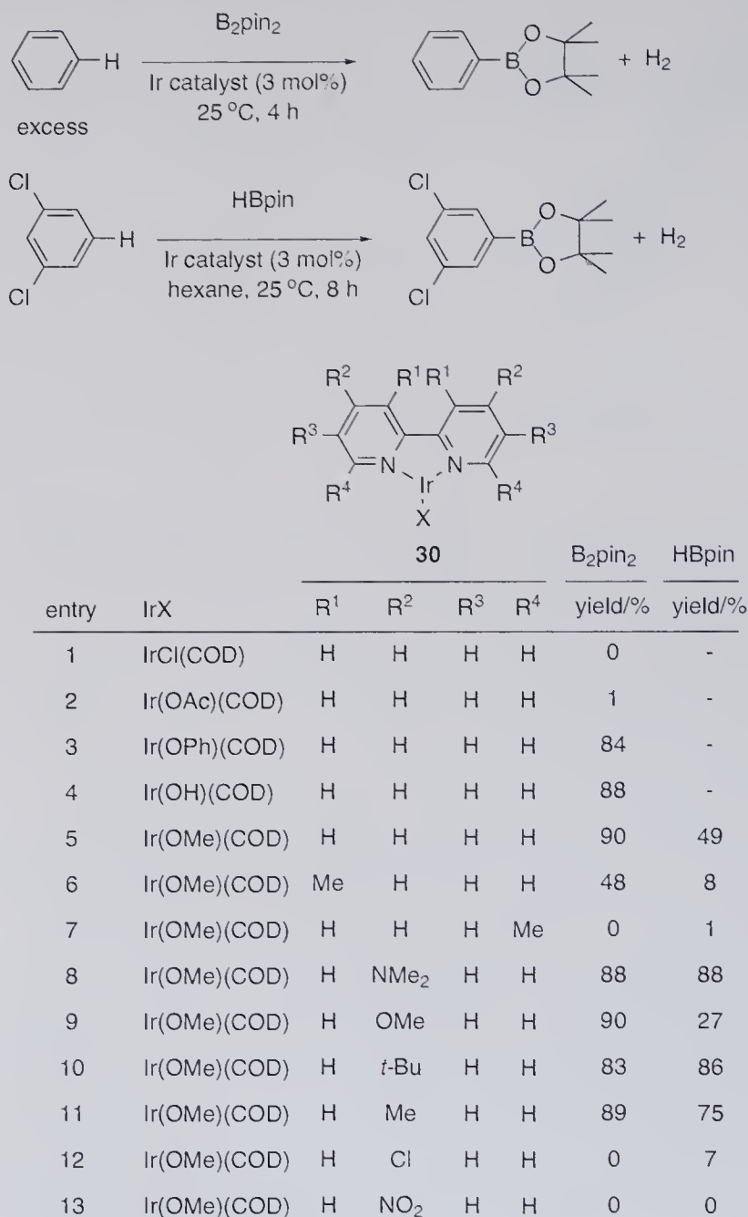
Scheme 2.9 Effect of ligands on the efficacy of Ir catalysts.
