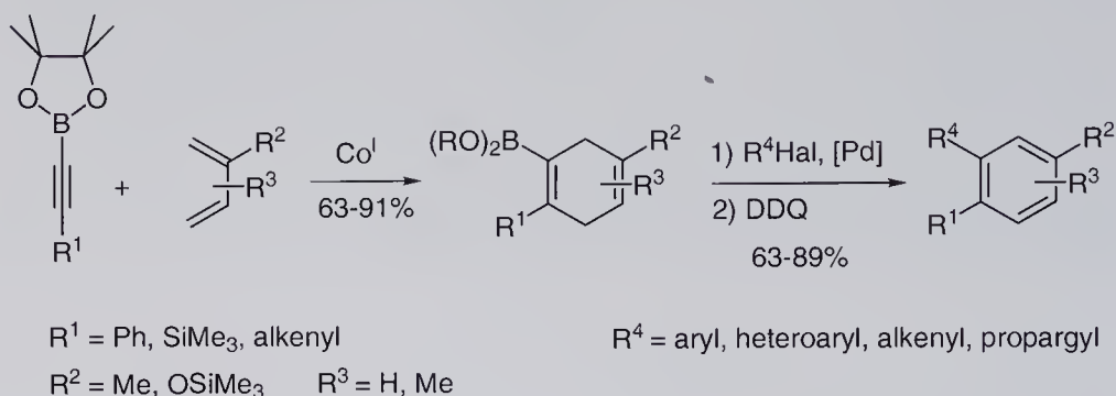
Scheme 9.28 Cobalt-catalyzed Diels–Alder reactions involving alkynylboronates.
