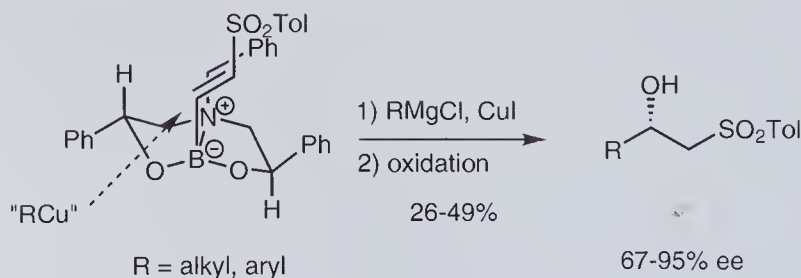
Scheme 9.8 Michael addition of organocuprates to activated alkenyldioxazaborocines.
