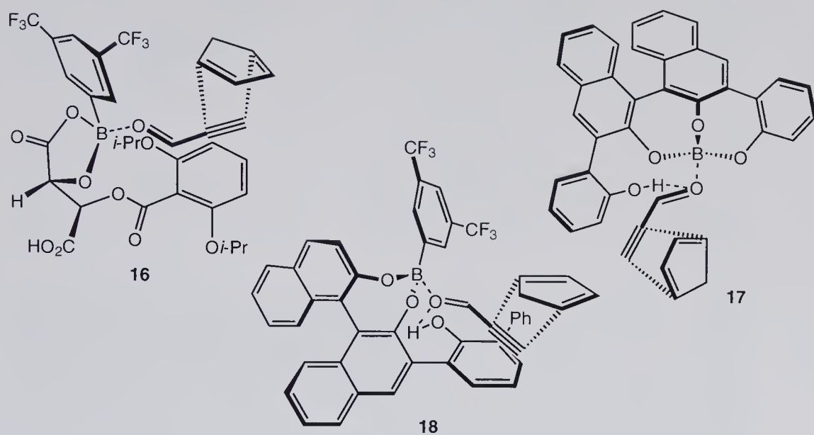
Figure 10.8 Proposed anti-exo-transition structures for the cycloaddition of cyclopentadiene and propynal.
