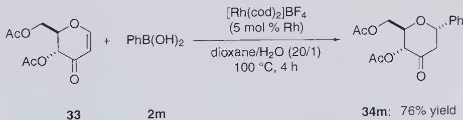
Scheme 4.13 Diastereoselective conjugate addition to enone 33 .
