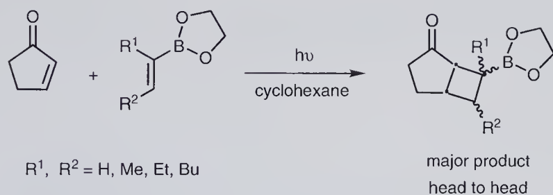
Scheme 9.48 Use of alkenylboronates in [2+2] enone-olefin photocycloadditions.
