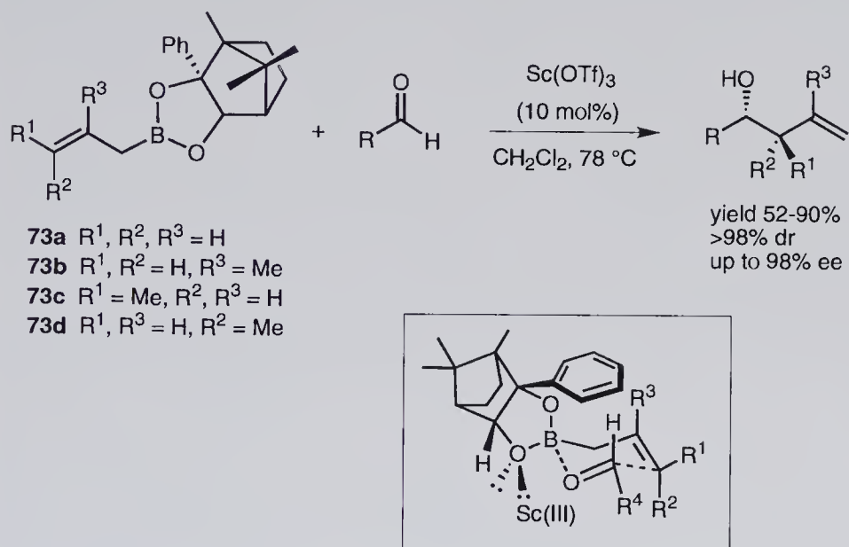
Figure 6.9 \text{Sc}(\text{OTf})_3 -catalyzed enantioselective addition of camphordiol allylboronates 73 .
