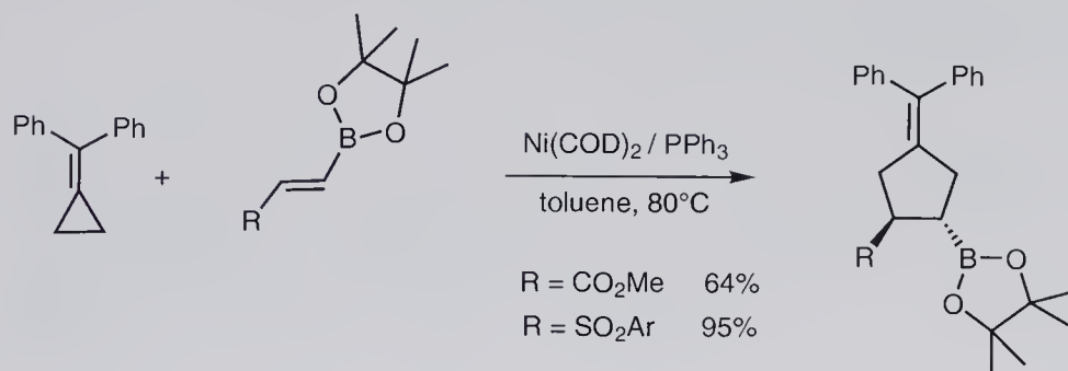
Scheme 9.47 Nickel(0)-catalyzed [3+2] cycloadditions to vinylboronates.
