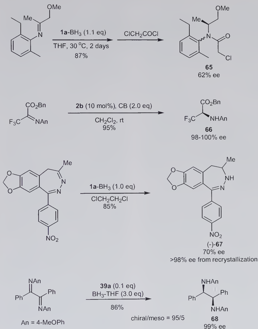
Scheme 11.21 Applications of the OAB-induced reduction of ketimines.
