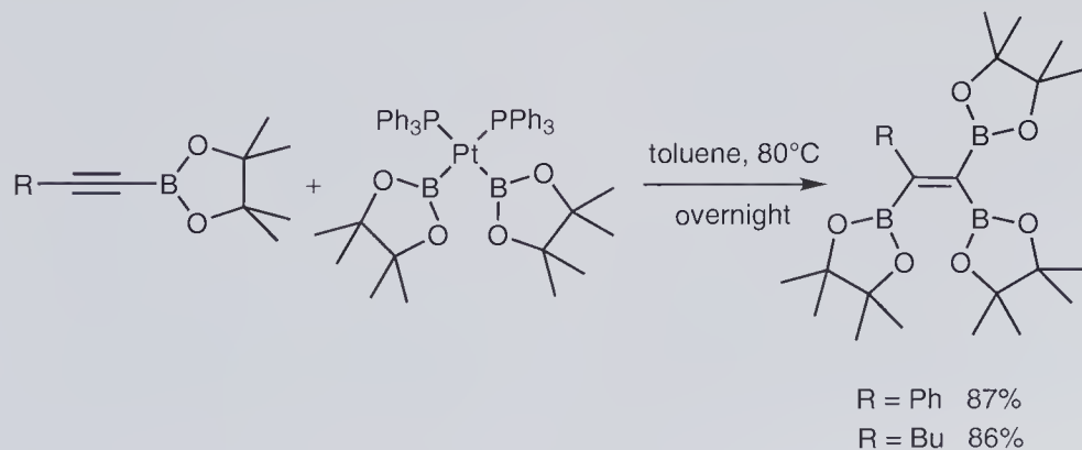
Scheme 9.58 Platinum(0)-catalyzed diboration of alkynylboronates.
