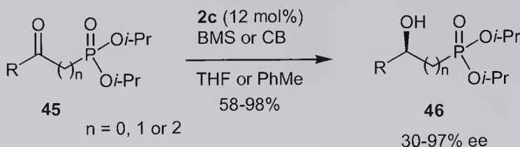
Scheme 11.14 2c-catalyzed reduction of keto phosphates.
