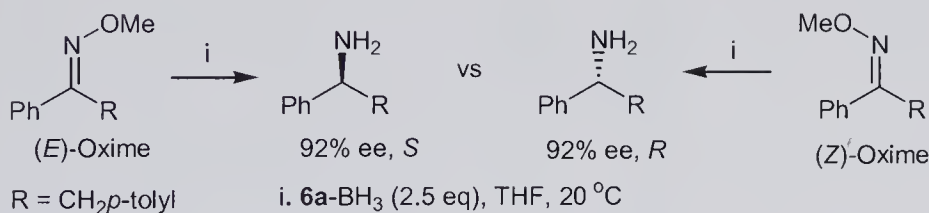
Scheme 11.18 Effect of oxime ether geometry on enantioselection.
