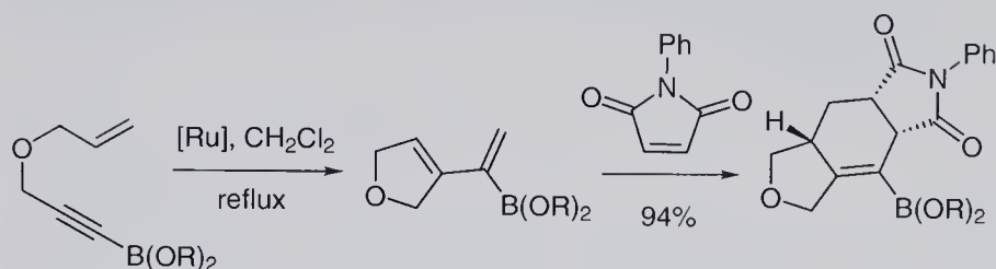
Scheme 9.51 Cyclic alkenyl- and dienyboronates via ring-closing metathesis.
