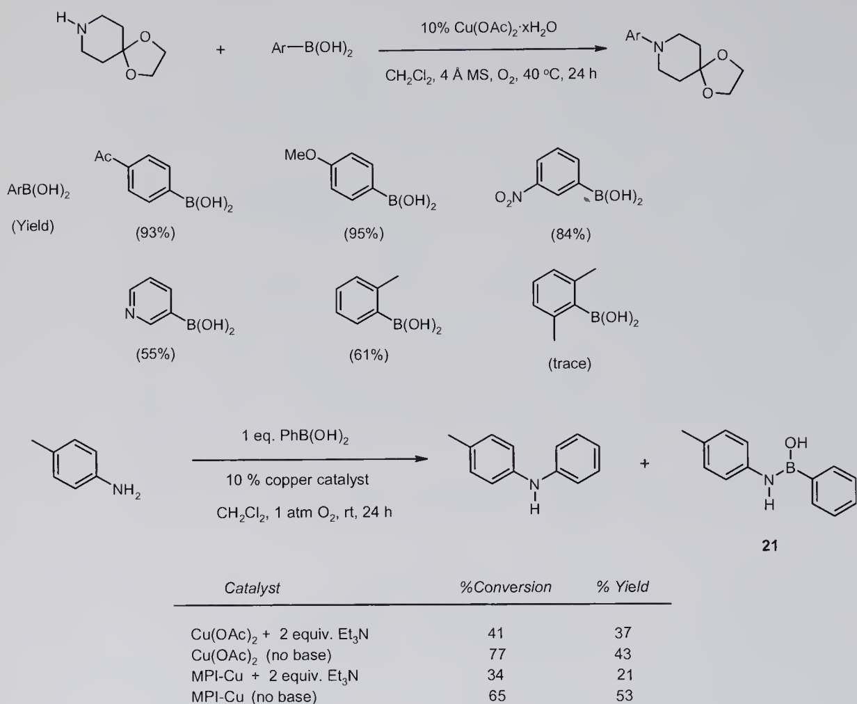
Scheme 5.10 Base/ligand free catalytic C–N cross-coupling.
