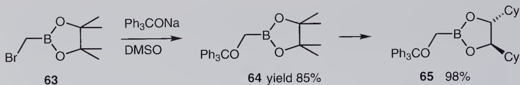
Scheme 8.15 Preparation of DICHED [(trityloxy)methyl]-boronate (65).
