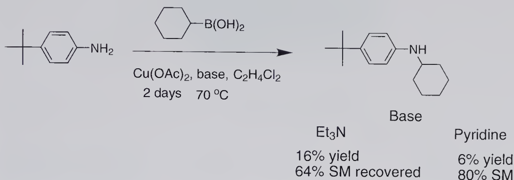
Scheme 5.29 N-Alkylation with cyclohexylboronic acid.
