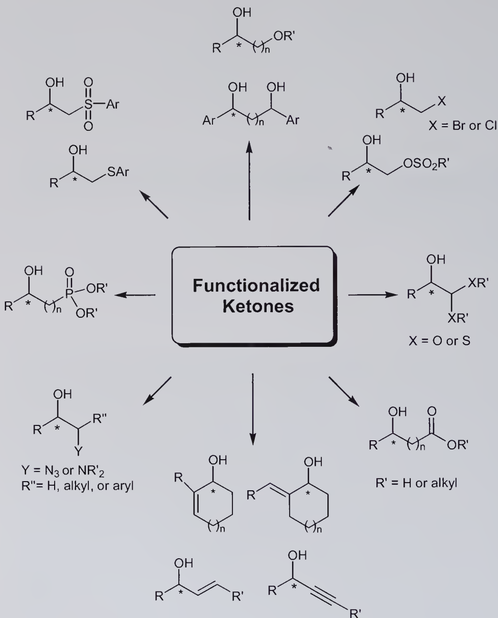
Figure 11.1 OAB-catalyzed asymmetric reduction of functionalized ketones.
