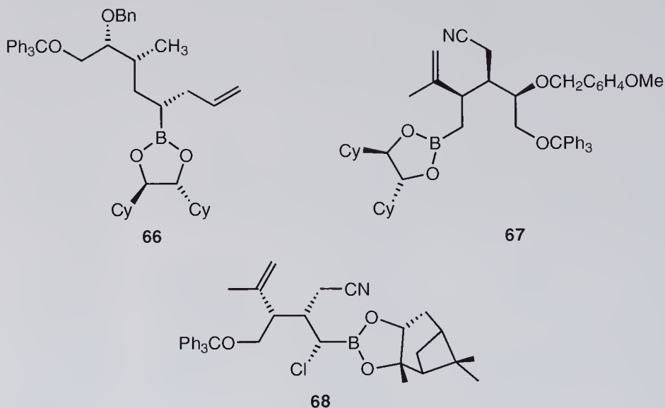
Figure 8.1 Miscellaneous boronic esters containing several stereocenters.
