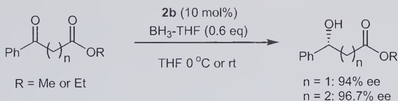
Scheme 11.9 2a -catalyzed reduction of keto esters.
