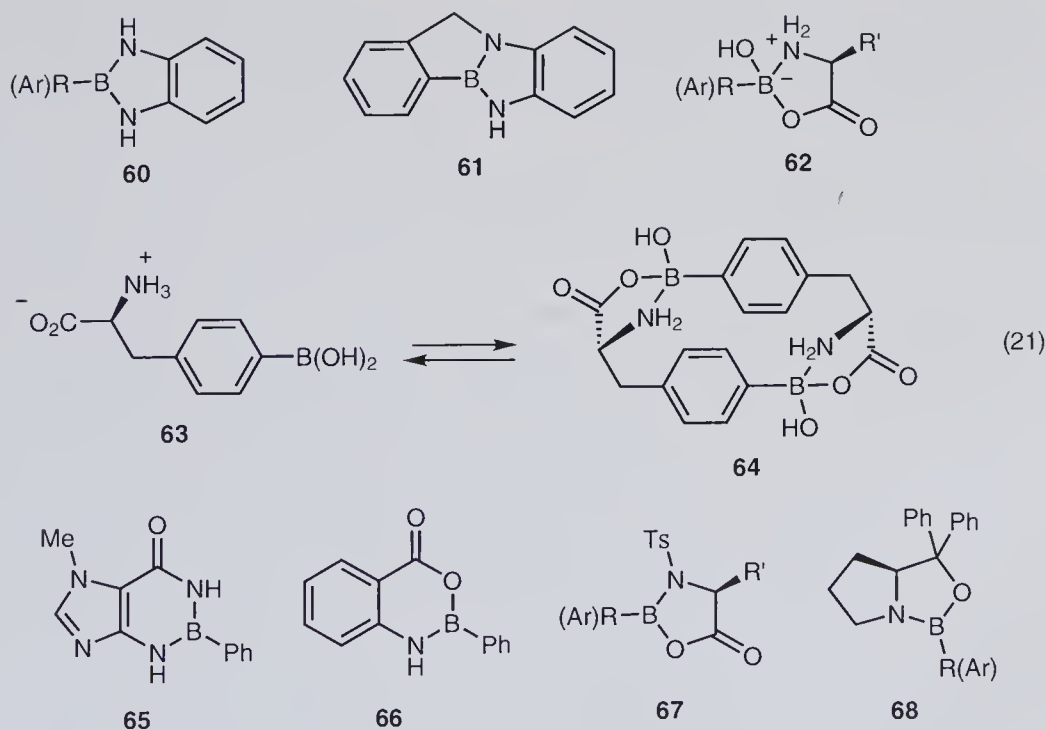
Figure 1.15 Examples of azaborolidines and other heterocyclic analogues.
