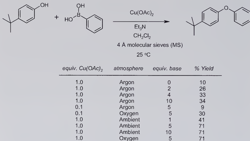
Scheme 5.2 Arylation of 4- t -butylphenol with phenylboronic acid.
