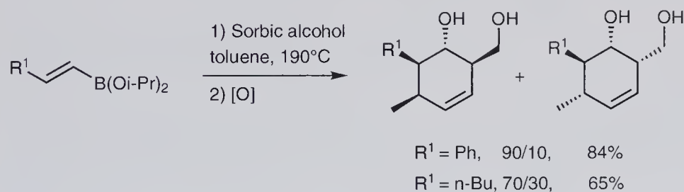
Scheme 9.22 Boron-tethered intramolecular Diels-Alder reactions.
