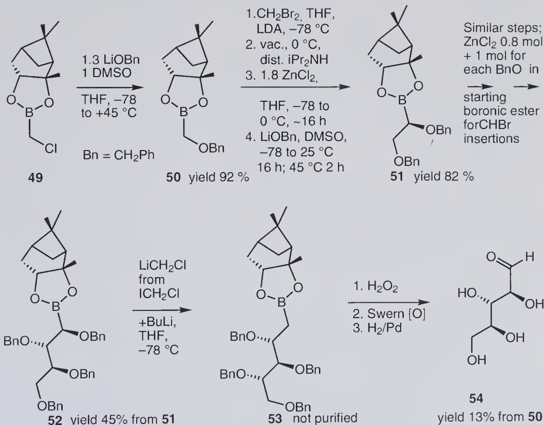
Scheme 8.12 Synthesis of L-ribose.
