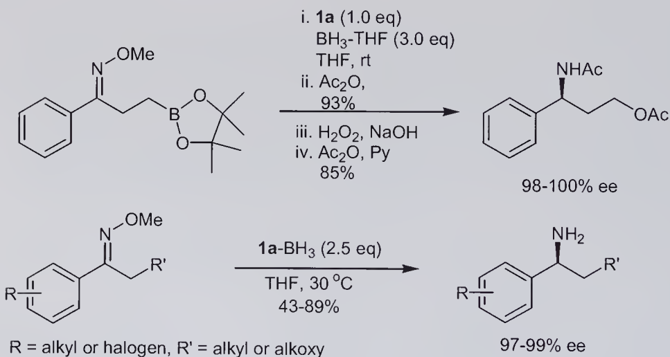
Scheme 11.19 OAB-induced reduction of ketoxime ether derivatives.
