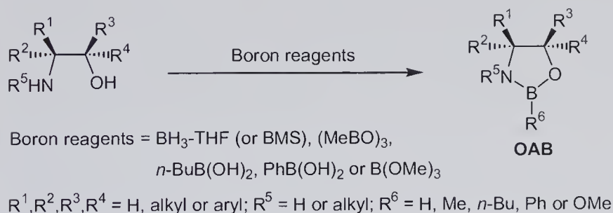
Scheme 11.1 Preparation of oxazaborolidines (OAB).
