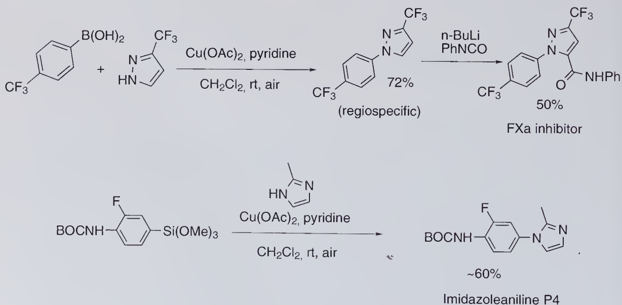
Scheme 5.17 Synthesis of Factor Xa inhibitors.
