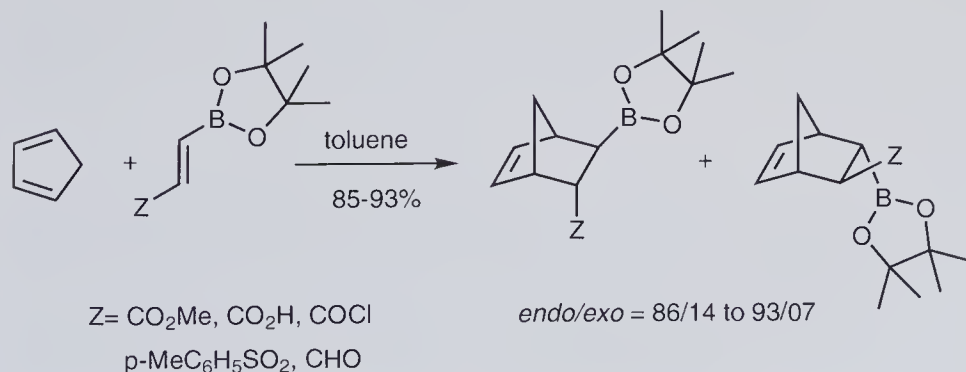
Scheme 9.23 Diels-Alder reactions of activated alkenylboronates with cyclopentadiene.
