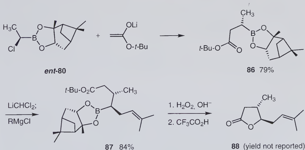
Scheme 8.18 Synthesis of African sugar cane borer pheromone. Conditions for \text{LiCHCl}_2 reactions and chloride substitutions as described in Schemes 8.1 and 8.3.
