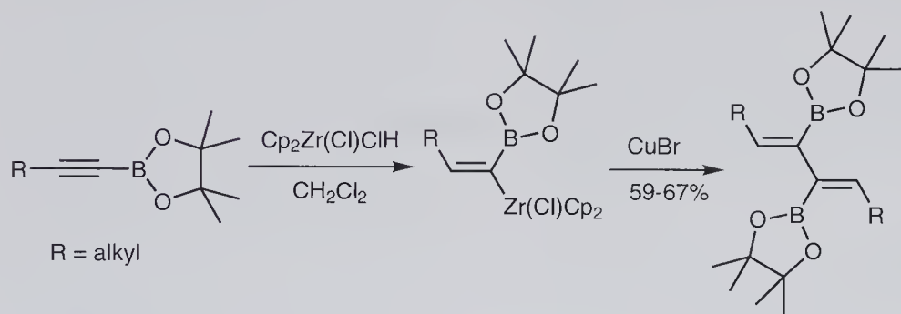
Scheme 9.57 Hydrozirconation of alkynylboronates and further homocoupling.
