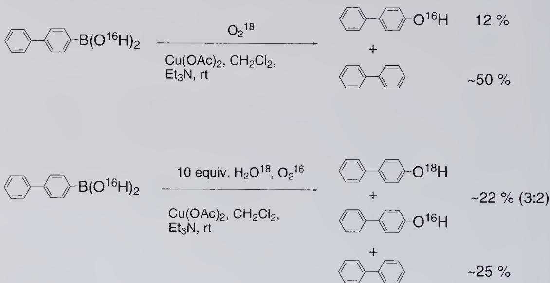
Scheme 5.35 Studies of the source of phenol byproduct.
