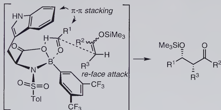
Figure 10.10 Proposed extended-transition state assembly.
