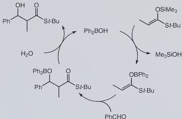
Scheme 10.1 Proposed boron enolate mechanism.
