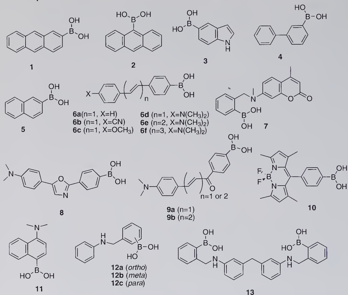
Figure 12.2 Internal charge transfer (ICT) fluorescence sensors.
