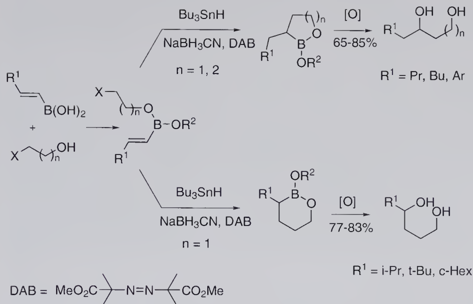
Scheme 9.13 Boron-tethered radical cyclizations.
