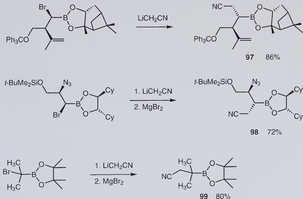
Scheme 8.22 Reactions of ( \alpha -bromoalkyl)boronic esters with lithioacetonitrile.
