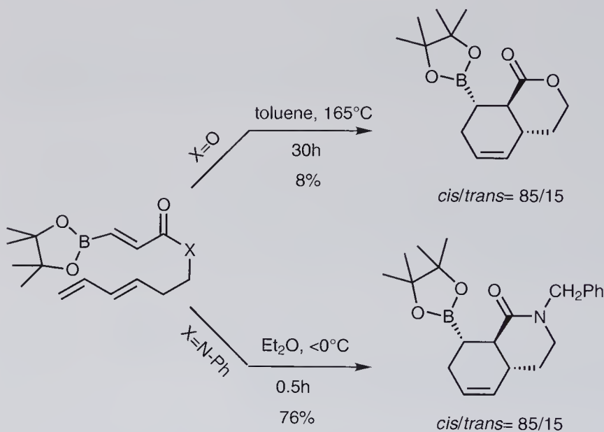
Scheme 9.24 Intramolecular Diels–Alder reactions involving 3-boronylpropenoic acid derivatives.
