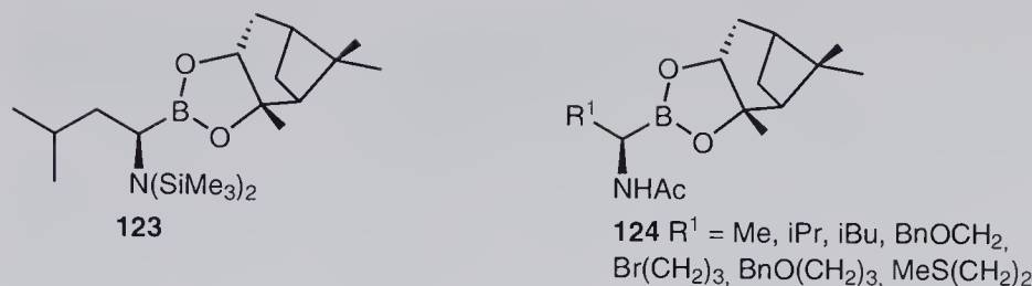
Figure 8.2 Significant silylated and acetylated ( \alpha -amidoalkyl)boronic esters.
