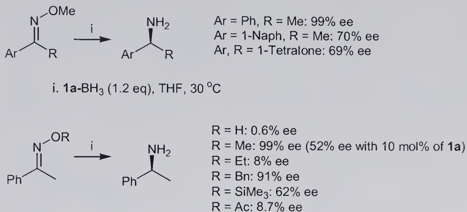
Scheme 11.17 1a -induced borane reduction of ketoxime derivatives.
