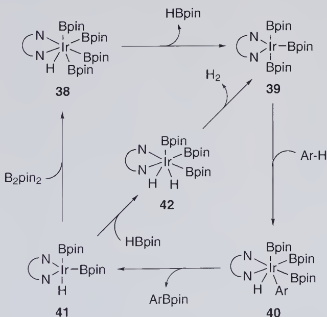
Scheme 2.14 Proposed catalytic cycle for aromatic C–H borylation.
