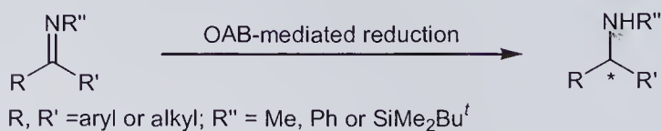
Figure 11.2 OAB-induced asymmetric reduction of ketimine derivatives.
