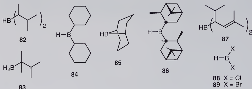
Figure 1.22 Common hydroborating agents for alkynes.
