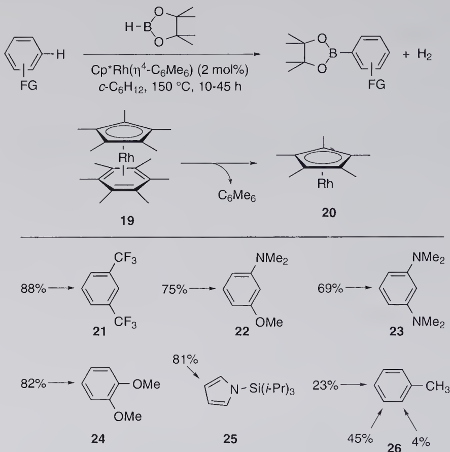
Scheme 2.7 Aromatic C–H borylation with \text{Cp}^*\text{Rh} complexes.
