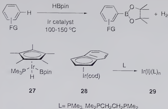
Scheme 2.8 Aromatic C–H borylation.
