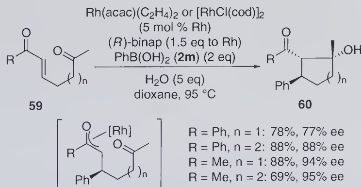
Scheme 4.26 Rhodium-catalyzed asymmetric intramolecular conjugate addition–aldol reaction.
