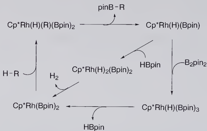
Scheme 2.5 Aliphatic C–H borylation with \text{Cp}^*\text{Rh} complexes.
