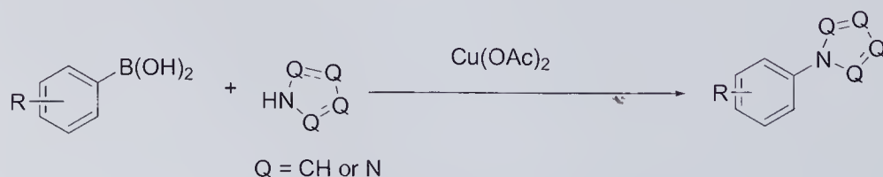
Scheme 5.14 Copper-promoted N-arylation of heteroarenes.
