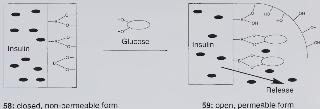
Scheme 13.5 A glucose-sensitive insulin release system using boronic acid polymer complexes ( 58 ).
