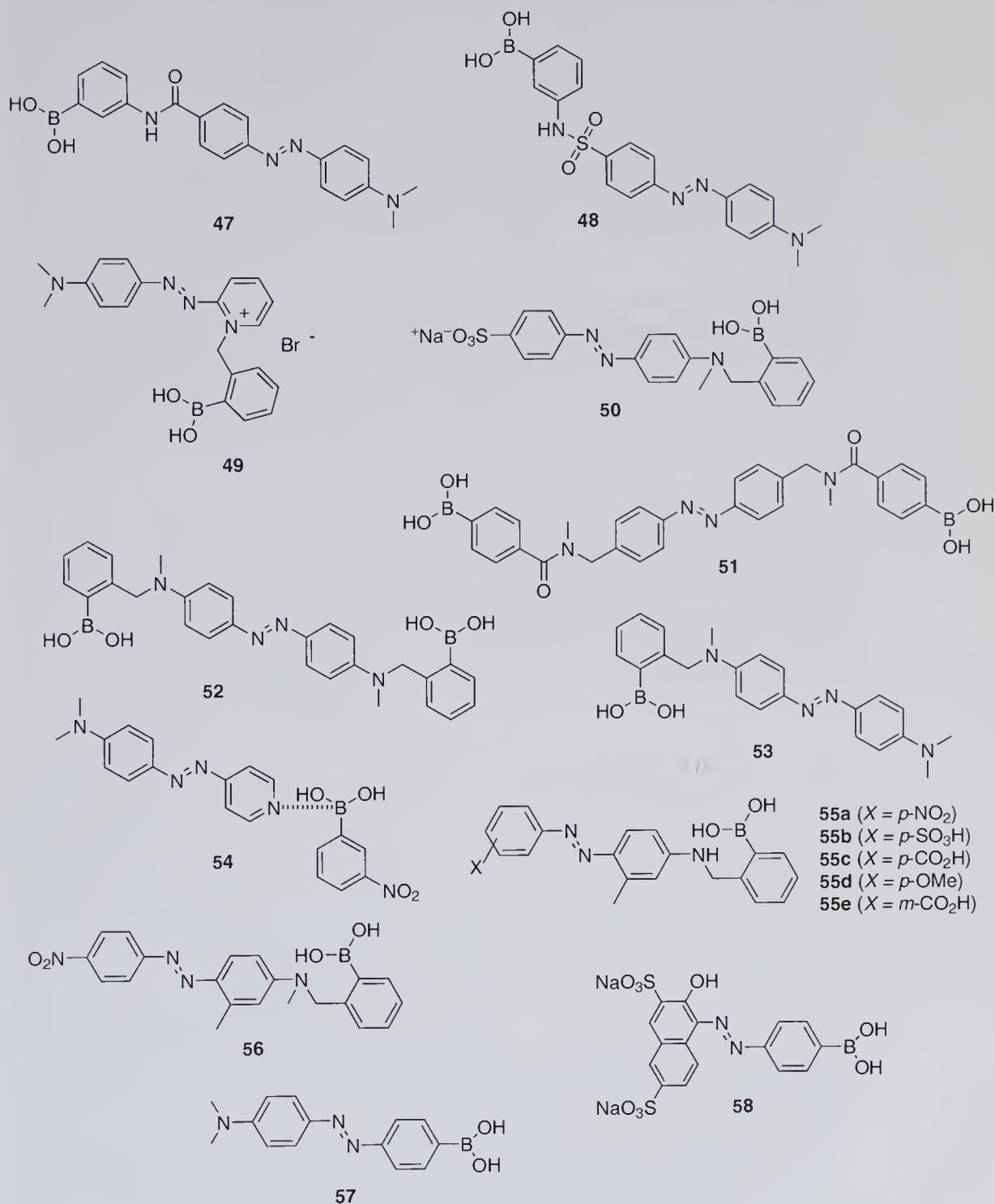
Figure 12.12 Azo-dye colorimetric sensors.
