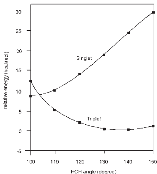
Figure 4. Change in the relative energy of singlet and triplet methylene with respect to \angle\text{HCH} at Becke 3LYP/TZ2P.
