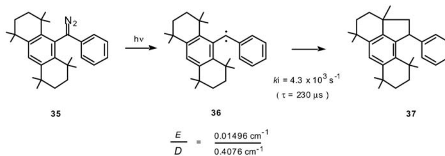
Scheme 10
