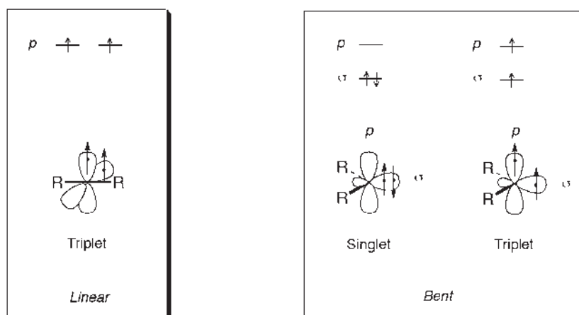
Figure 1. Linear and bent carbenes
