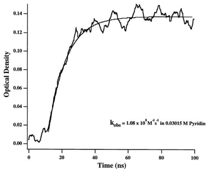
Figure 4. Growth of ylide 21 absorbance following laser flash photolysis of dimethyldiazirine in the presence of pyridine. Reprinted with permission from Ford, F.; Yuzawa, T.; Platz, M.S.; Matzinger, S.; Fülischer, M. J. Am. Chem. Soc. , 1998 , 120 , 4430
