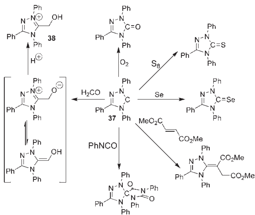
Scheme 12
