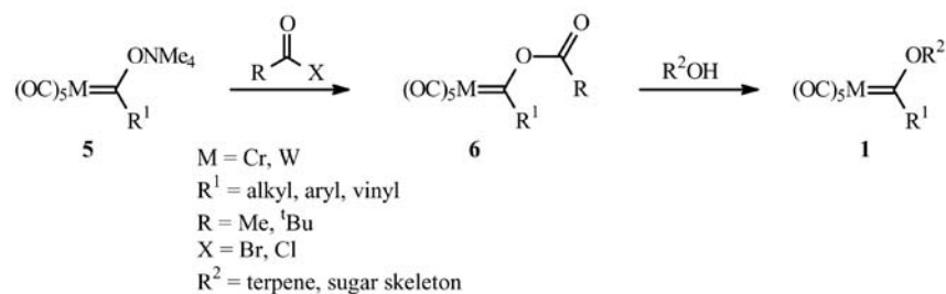
Scheme 2. Alkoxycarbene complexes via an acylation-alcoholysis sequence.
