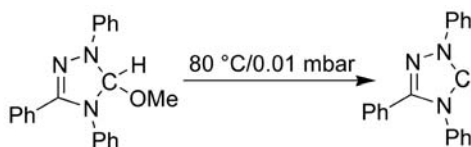
Scheme 7
