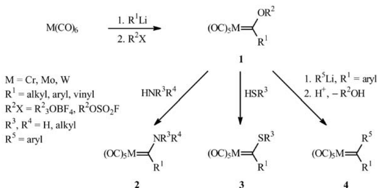
Scheme 1. Fischer route to metal carbene complexes.
