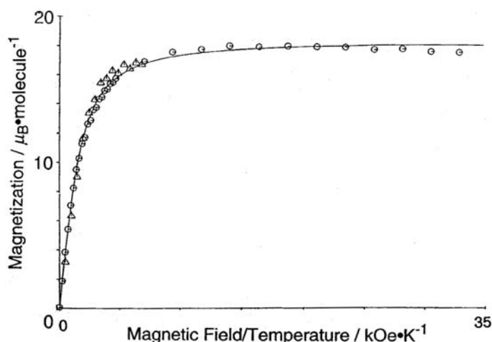
Figure 8. Field dependence of magnetization after irradiation of 11 in a frozen MTHF solution. The theoretical curve with S = 9 is shown by a solid line.
