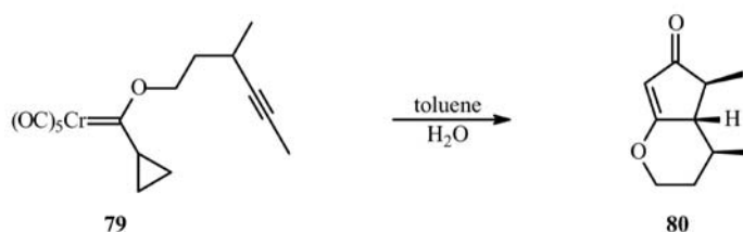
Scheme 36. Stereocontrolled intramolecular cycloaddition with a cyclopropylcarbene complex.
