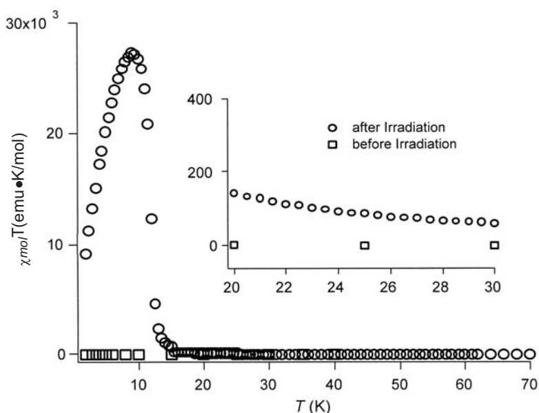
Figure 13. Temperature dependence of \chi_{mol}T values after irradiation of a 3:2 mixture (20 mM) of \text{Cu}(\text{hfac})_2 and 18 in a frozen solution. The inset shows the enlarged view in the temperature range of 20–30 K.
