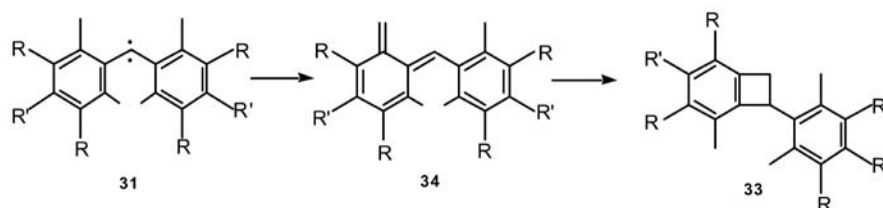
Scheme 7
