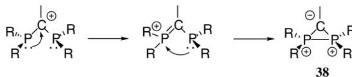
Scheme 17
