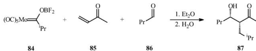
Scheme 38. Molybdenum difluoroboroxycarbene complexes in radical coupling reactions.
