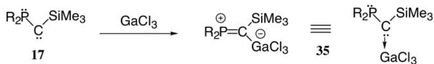
Scheme 13
