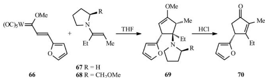
Scheme 33. Enantiocontrolled cycloaddition of enamines to alkenylcarbene complexes.
