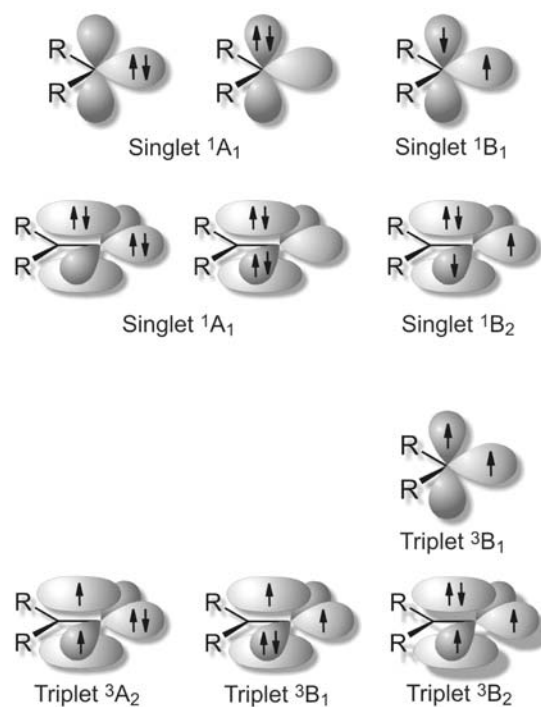
Figure 4. Important electronic configurations of carbenes and vinylidenes.
