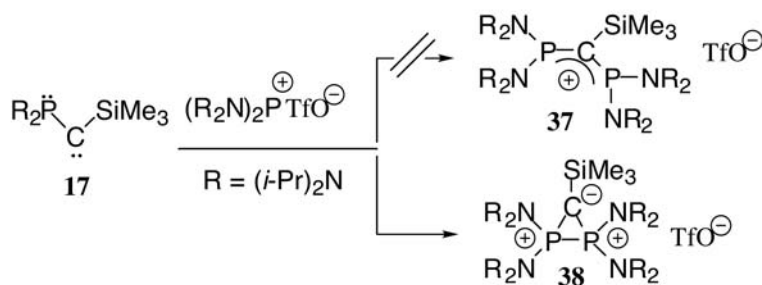
Scheme 16
