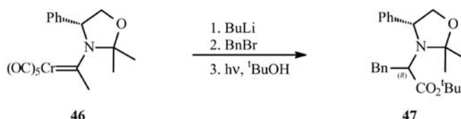
Scheme 25. Synthesis of enantiopure amino acids via photolysis of chromium carbene complexes.
