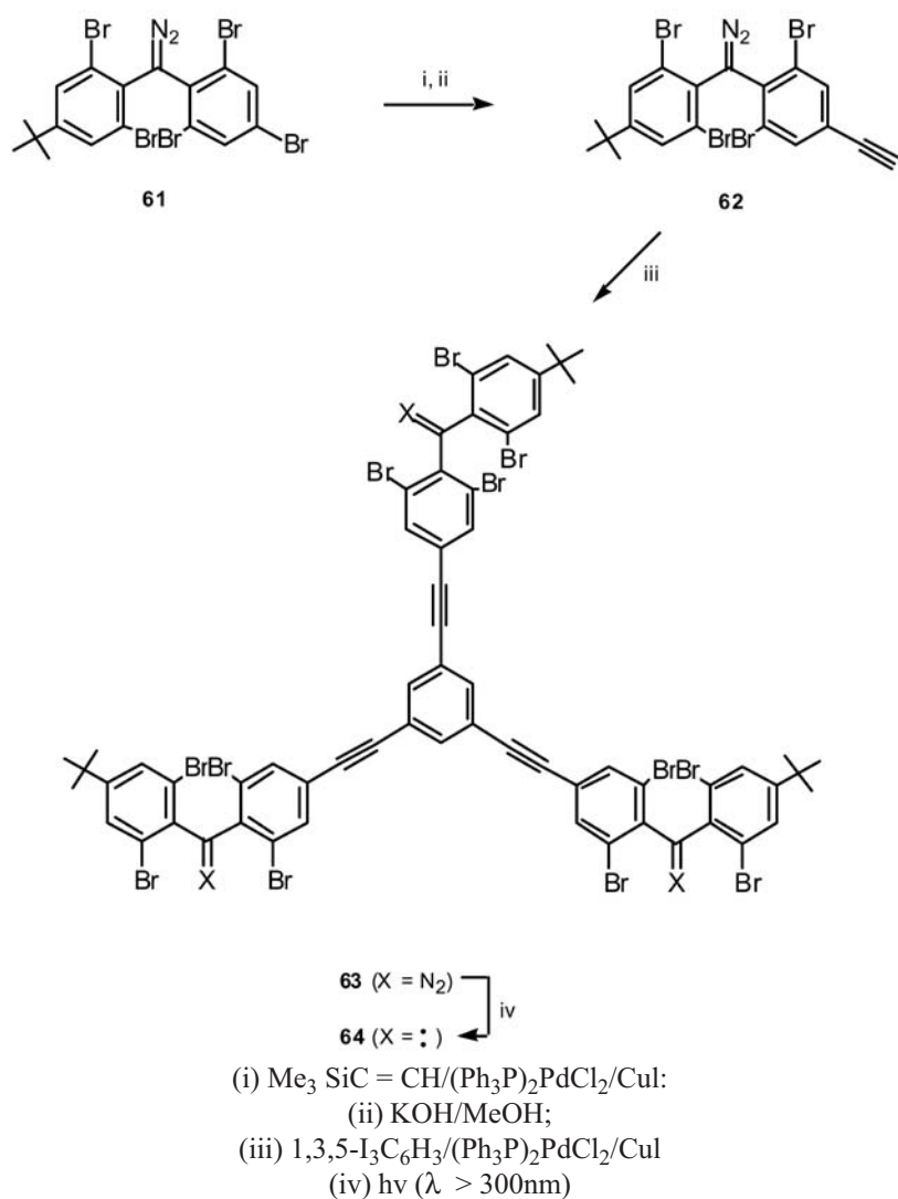
Scheme 22
