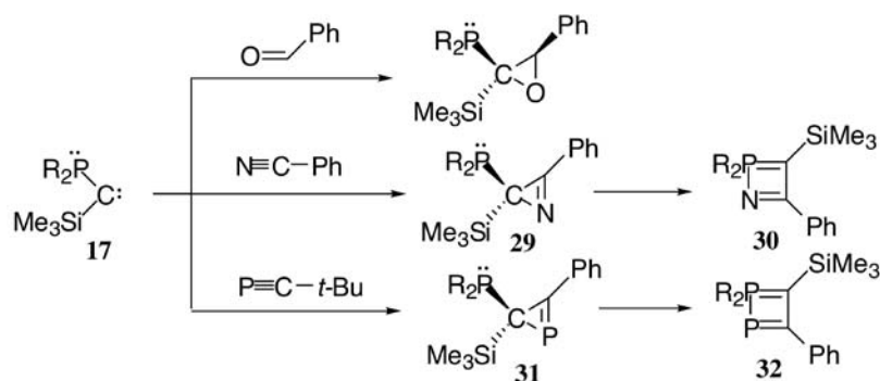
Scheme 10
