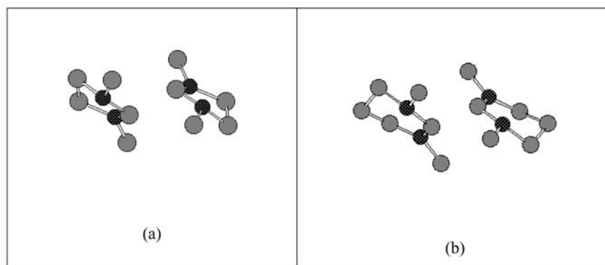
Figure 2 Transition states for dimerisation of (a) 1,3-dimethylimidazolidin-2-ylidene, ( 11 , R = Me) and (b) 1,3-dimethyltetrahydropyrimid-2-ylidene, 24 , from B3LYP/6-31G* calculations (hydrogen atoms have been omitted for clarity).
