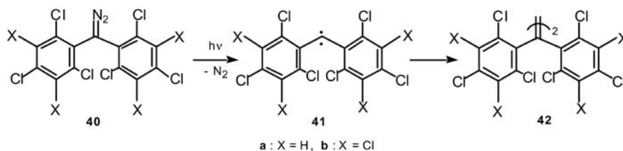
Scheme 12
