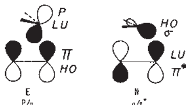
Figure 5. HOMO-LUMO interactions in carbene/alkene cycloadditions. Left, carbene p/alkene \pi ; right, carbene \sigma /alkene \pi^* . Reprinted with permission from ref. 66.
