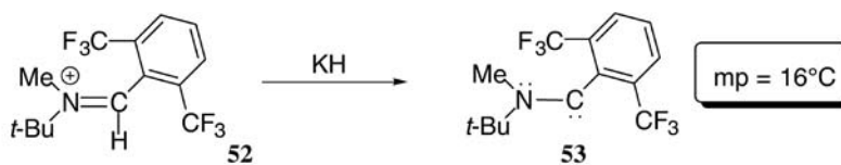
Scheme 22
