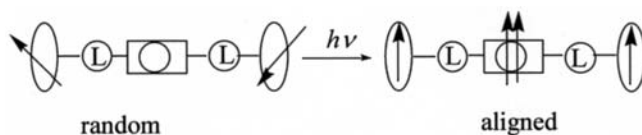
Figure 2. Role of carbene as a photoresponsive magnetic coupler (PMC).
