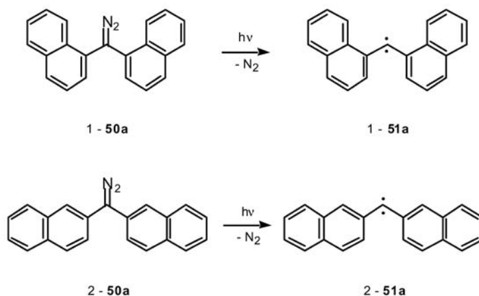
Scheme 17
