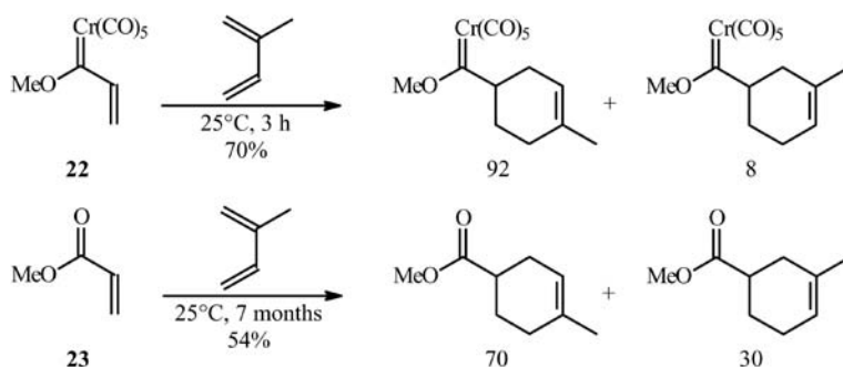
Scheme 12. Comparative Diels-Alder reaction of carbene complex 22 and its isolobal analogue.
