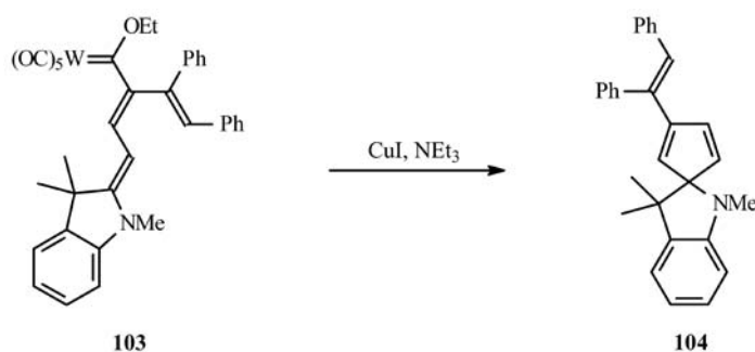
Scheme 45. Copper-catalyzed cyclization of a Fischer carbene to a spirocyclopentadiene.
