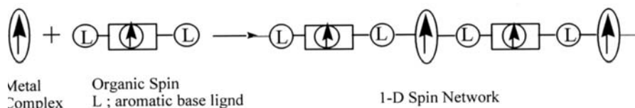
Figure 1. Strategy for the construction of 1D spin network in hetero-spin system.
