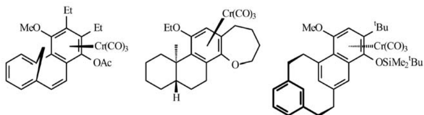
Figure 4. Asymmetric induction by chiral carbene carbon substituents.
