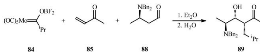
Scheme 39. Asymmetric radical coupling reaction with molybdenum boroxycarbenes.
