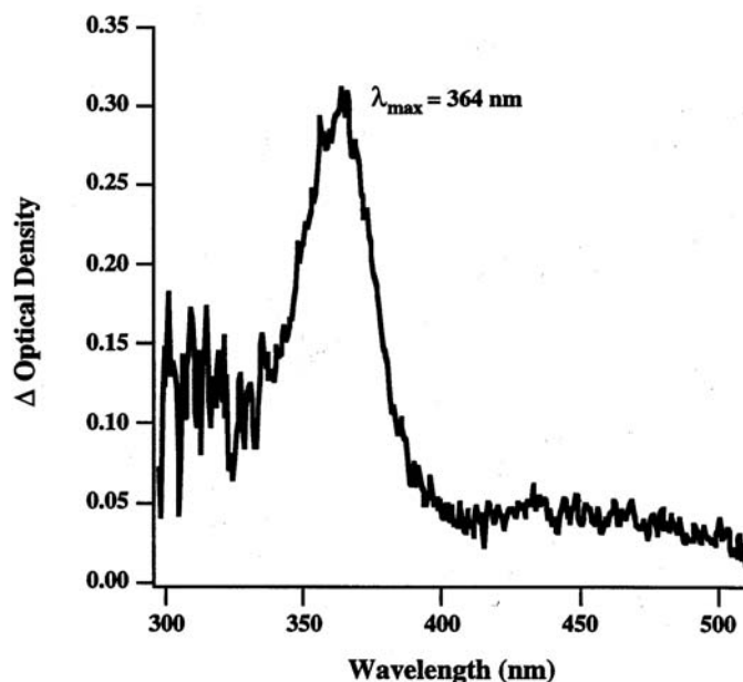
Figure 3. The transient absorption spectrum of ylide 21 produced by LFP of dimethyldiazirine in Freon-113 at ambient temperature. Reprinted with permission from Ford, F.; Yuzawa, T.; Platz, M.S.; Matzinger, S.; Fülischer, M. J. Am. Chem. Soc. , 1998 , 120 , 4430.
