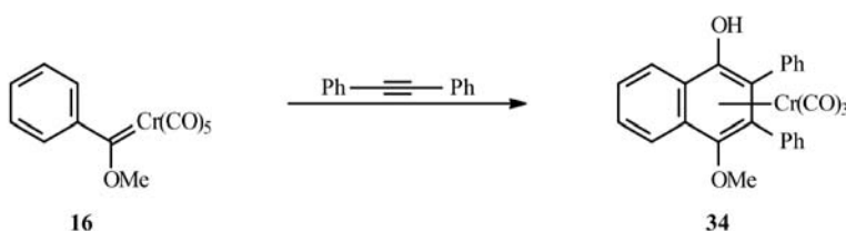
Scheme 20. Chromium-templated benzannulation of arylcarbenes.
