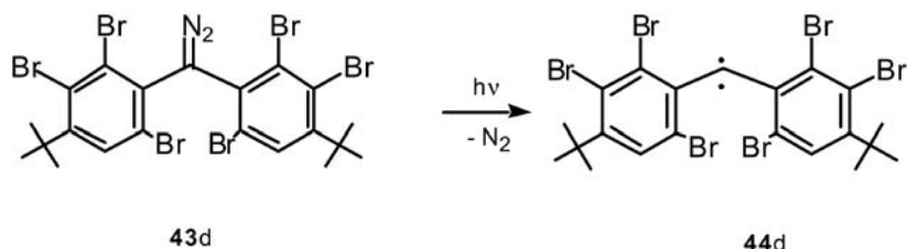
Scheme 14
