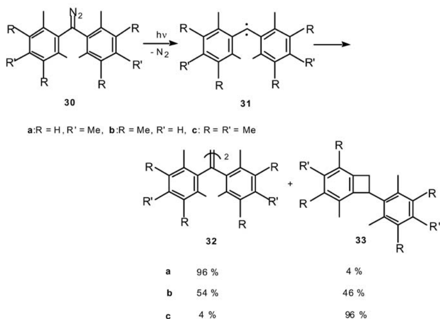
Scheme 6
