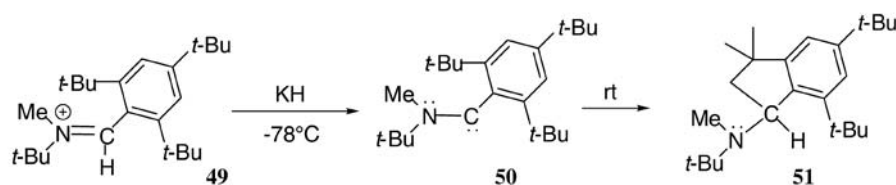
Scheme 21
