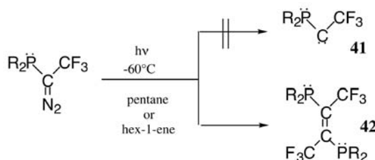
Scheme 18
