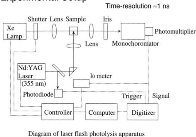
Figure 1. A typical apparatus for laser flash photolysis studies.
