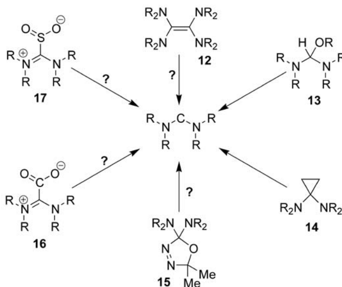
Scheme 6
