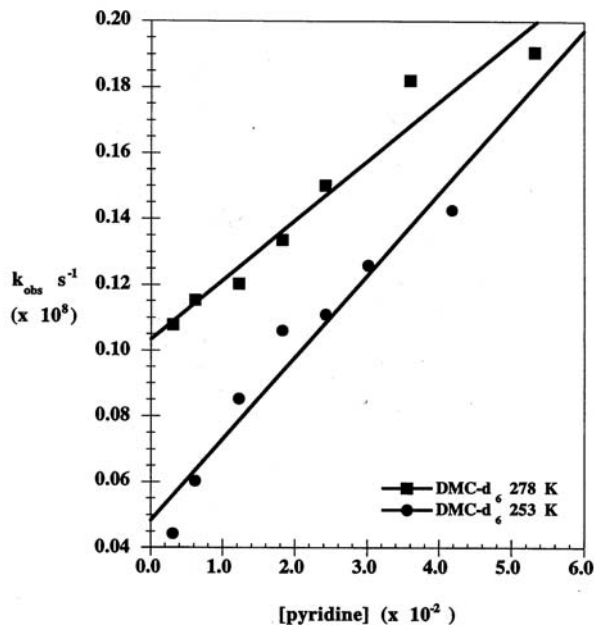
Figure 6. Plots of observed rate constant of ylide formation versus pyridine concentration obtained by LFP of dimethyldiazirine-d 6 in trifluoromethylbenzene at two temperatures. Reprinted with permission from Ford, F.; Yuzawa, T.; Platz, M.S.; Matzinger, S.; Fülischer, M. J. Am. Chem. Soc. , 1998 , 120 , 4430.
