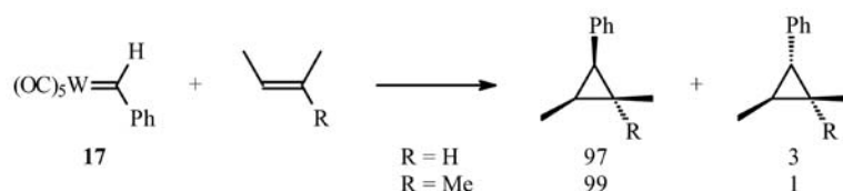
Scheme 18. Cyclopropanation of a non-functionalized alkene.
