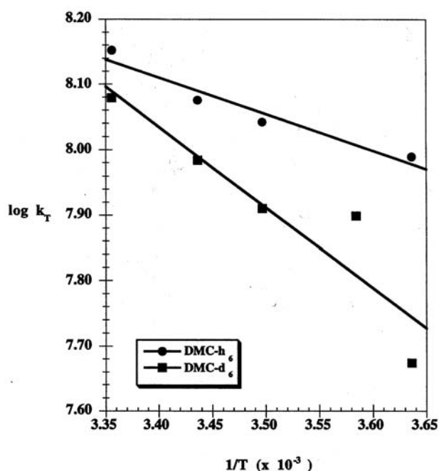
Figure 8. Arrhenius treatments of the intercepts of plots of the observed rate constant of ylide formation versus pyridine concentration obtained by LFP of dimethyldiazirine and dimethyldiazirine-d 6 in perfluorohexane. Reprinted with permission from Ford, F.; Yuzawa, T.; Platz, M.S.; Matzinger, S.; Fülischer, M. J. Am. Chem. Soc. , 1998 , 120 , 4430.
