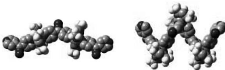
Figure 10. Crystal Structures of 1:1 Complexes [\text{Mn}(\text{hfac})_2\cdot\mathbf{16}] in a trans (left) and b cis (right) Conformations
