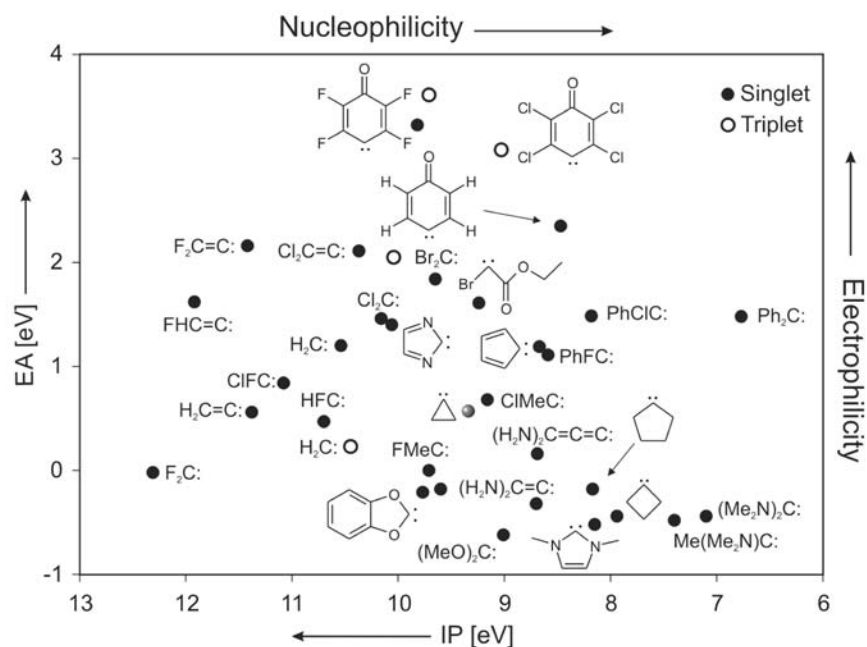
Figure 2. EA and IP of a series of carbenes calculated at the B3LYP/6-311++G(d,p) level of theory.
