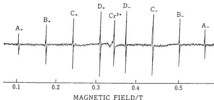
Figure 5. Oriented X-band epr spectrum after irradiation of tetradiazo compound, a precursor of 2 ( n = 4 ) in a benzophenone crystal.
