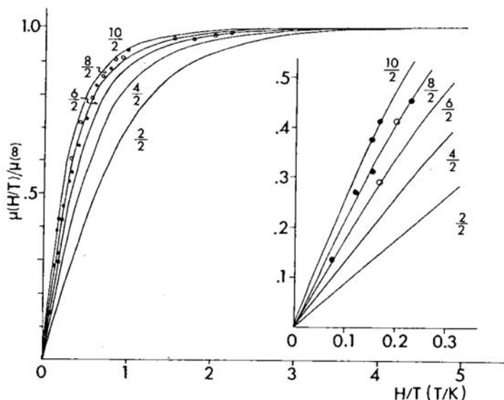
Figure 6. Field dependence of magnetization ( M ) at 2.1 (●) and 4.2 (○) K after irradiation of tetradiazo compound, a precursor to 2 ( n = 4 ) in a benzophenone crystal.
