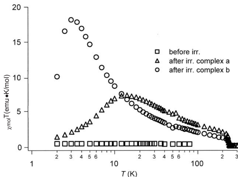
Figure 11. Temperature dependence of \chi_{mol}T for 1:1 complex a and b of [\text{Cu}(\text{hfac})_2 \cdot \mathbf{16}] before and after irradiation.
