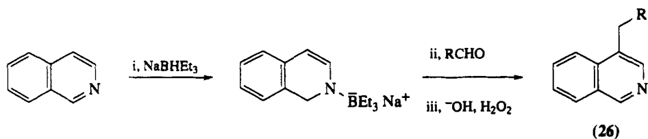
Scheme 11
