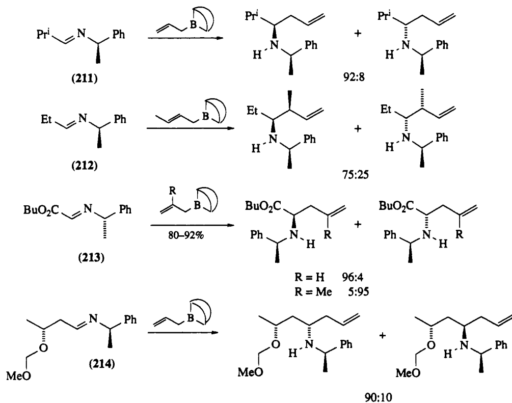
Scheme 35
