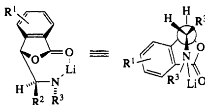
Figure 6 Proposed transition state involved in the addition of phthalide enolates to imines 122
