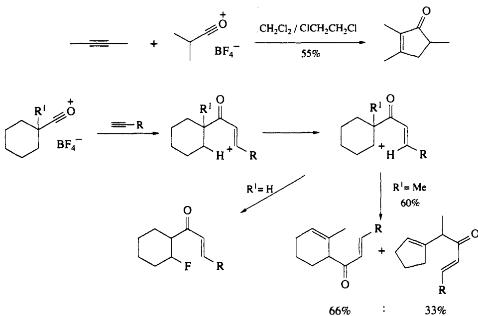
Scheme 24
