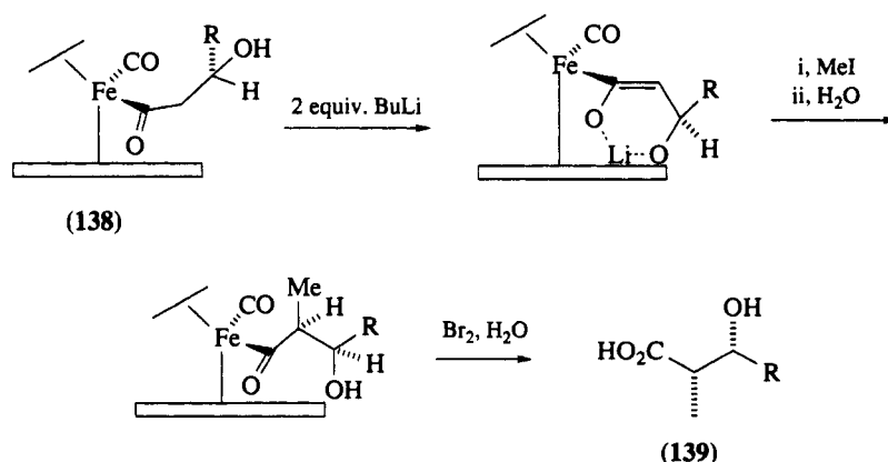
Scheme 61
