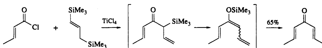
Scheme 12
