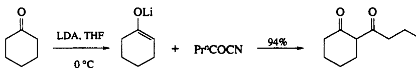
Scheme 50
