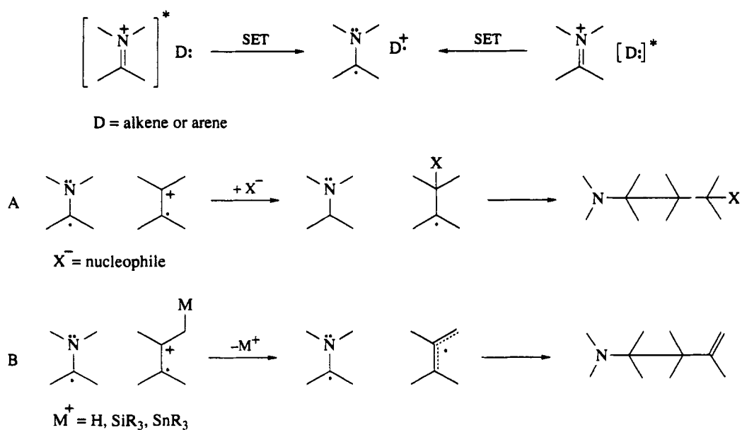
Scheme 46
