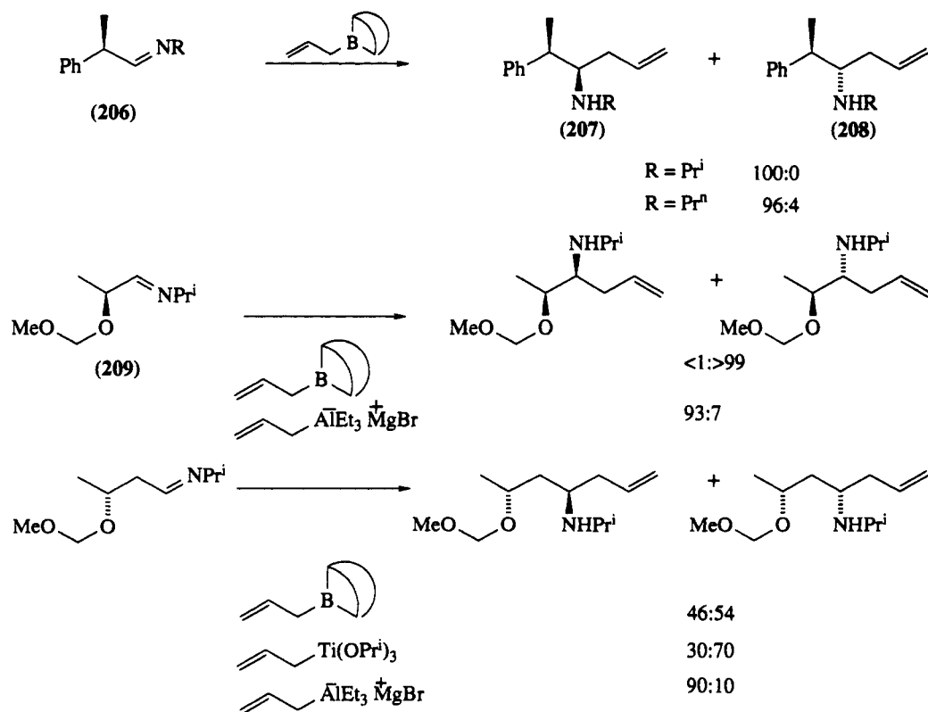
Scheme 34
