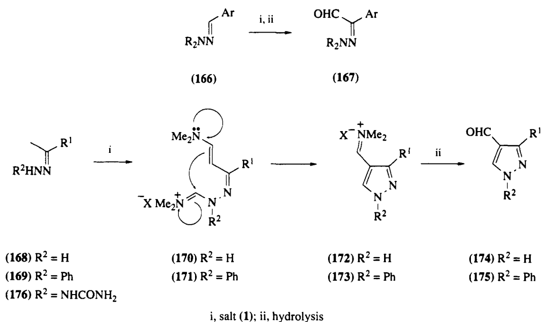
Scheme 13
