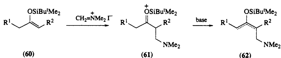
Scheme 12
