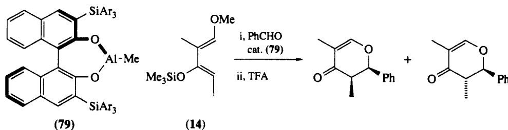
Scheme 28
