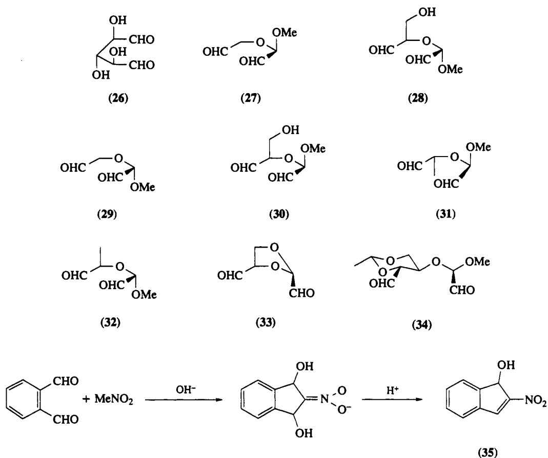
Scheme 6
