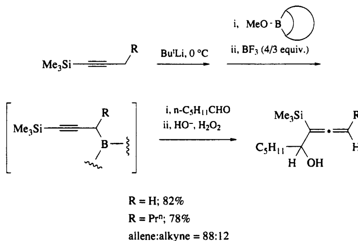
Scheme 7
