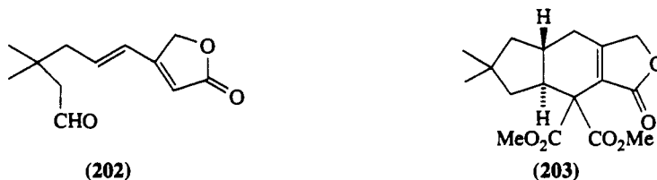
Scheme 36
