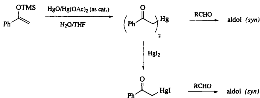
Scheme 69
