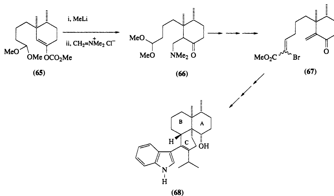
Scheme 15
