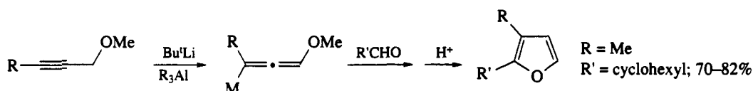
Scheme 18
