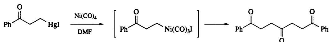
Scheme 26
