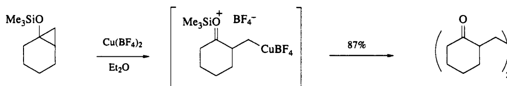
Scheme 10
