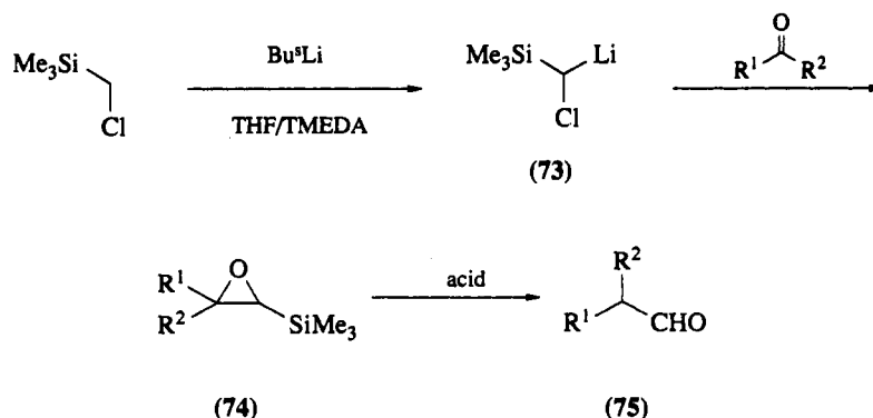
Scheme 18
