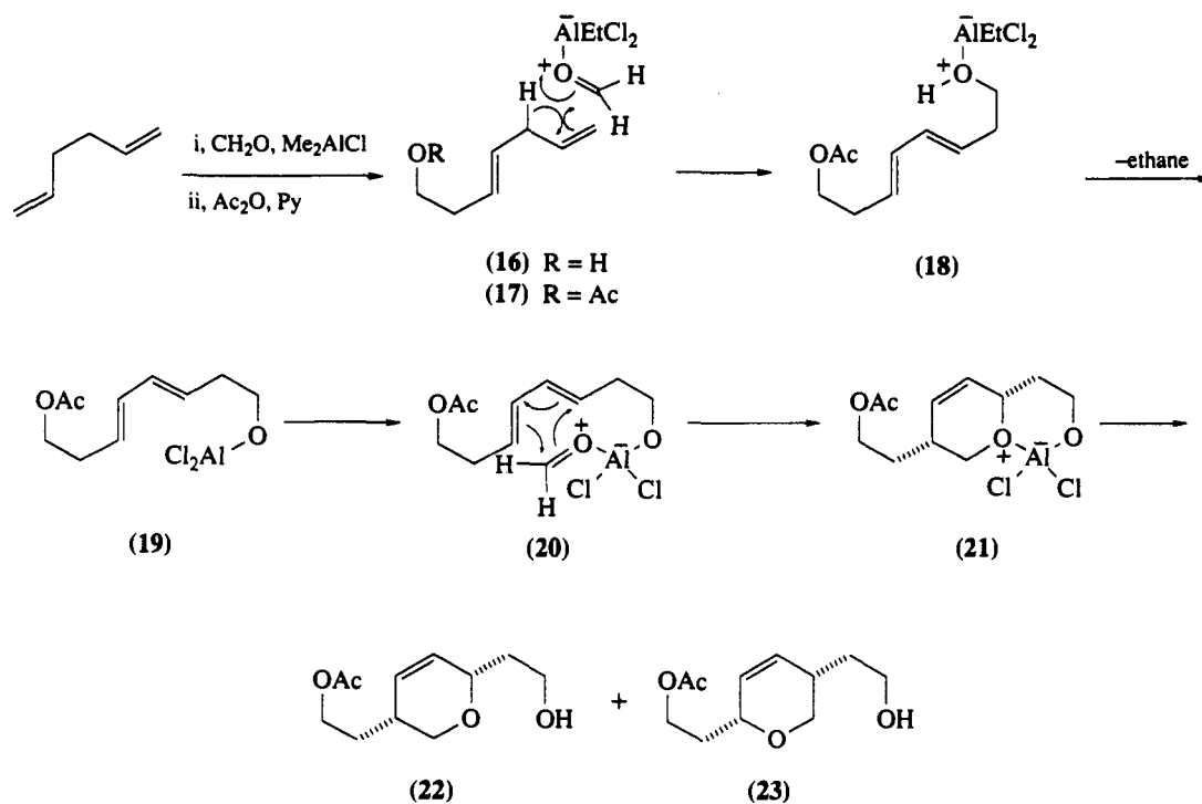
Scheme 5
