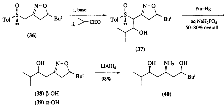
Scheme 17
