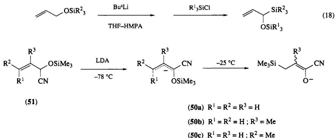
Scheme 29
