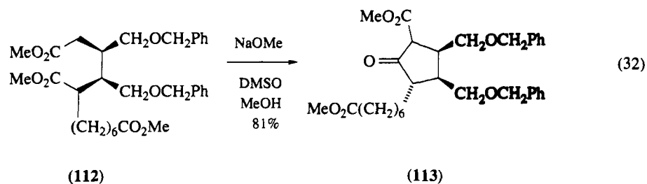
Scheme 39
