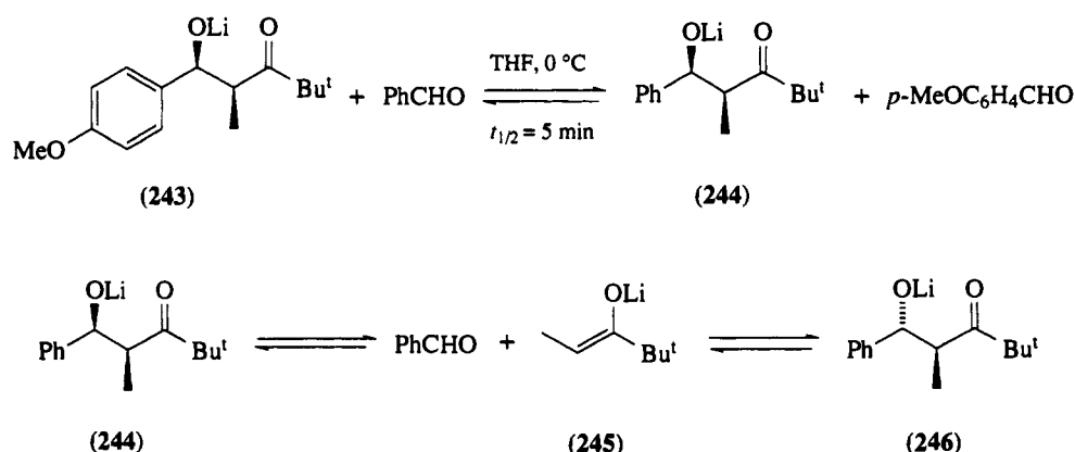
Scheme 16
