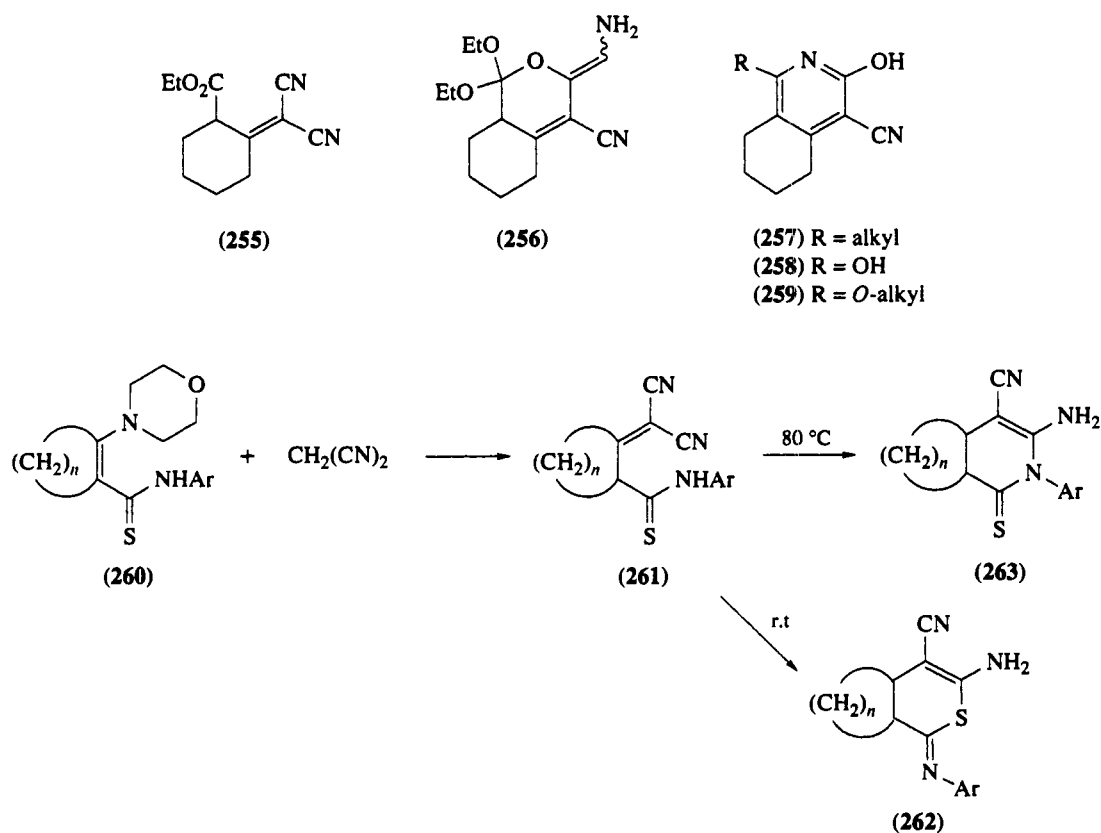
Scheme 52
