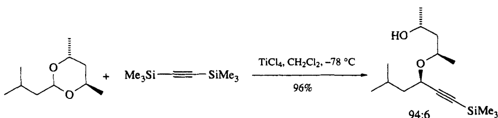
Scheme 52
