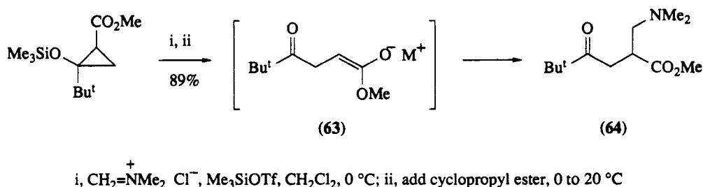
Scheme 14
