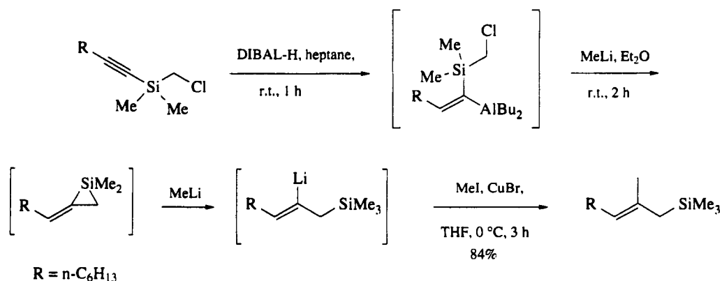
Scheme 74
