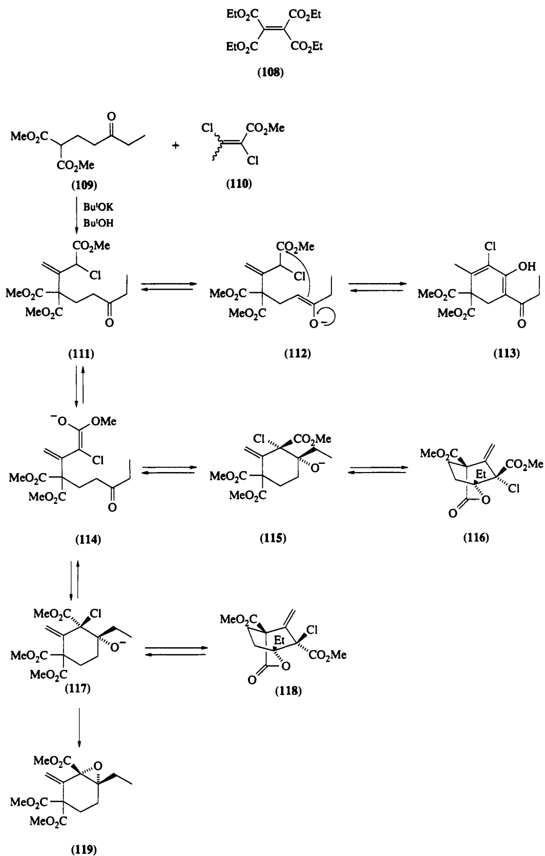
Scheme 23
