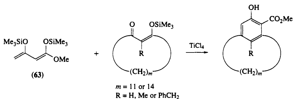
Scheme 49
