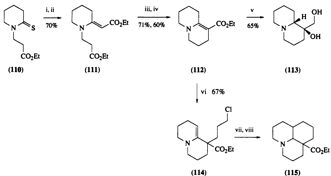
Scheme 23
