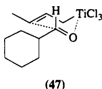
Scheme 25
