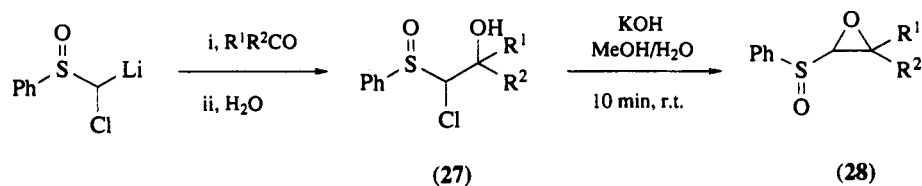
Scheme 7
