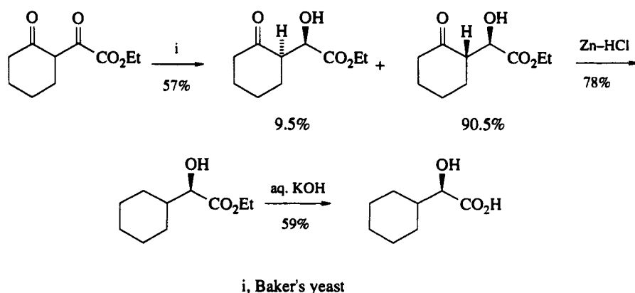
Scheme 67
