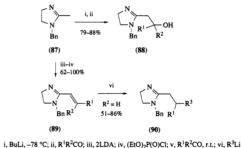
Scheme 33
