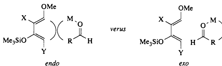
Figure 4 Steric interactions between metal, aldehyde and the diene disfavor the endo transition state. Chelation control should prefer the exo transition state in the Diels–Alder cycloaddition pathway
