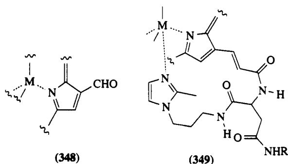
Scheme 62
