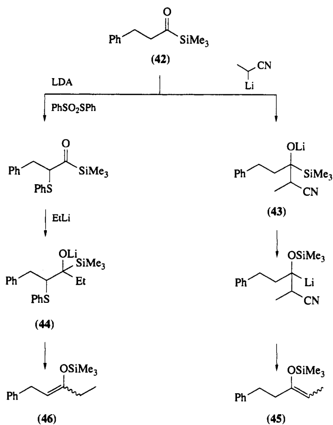
Scheme 15
