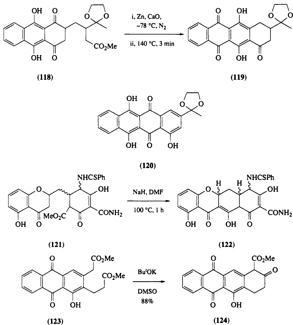
Scheme 41
