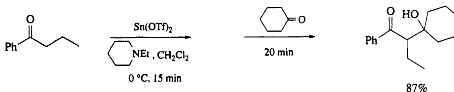
Scheme 31
