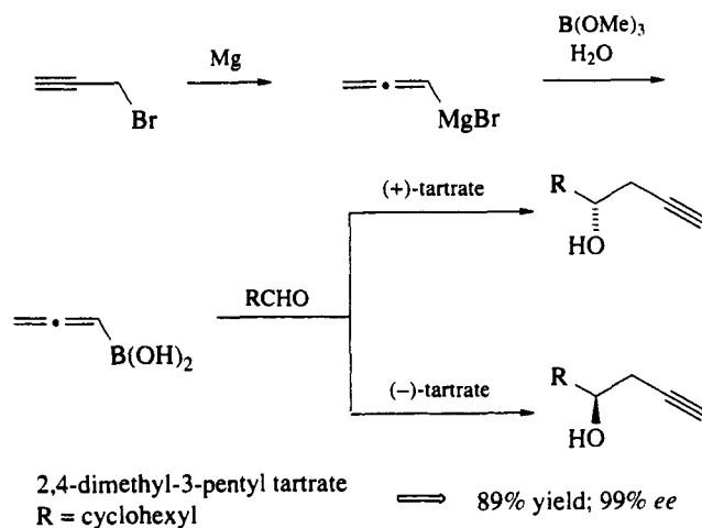
Scheme 38
