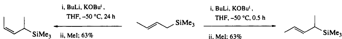
Scheme 78
