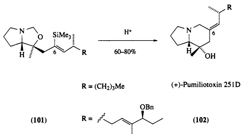
Scheme 36
