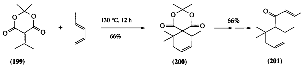
Scheme 36
