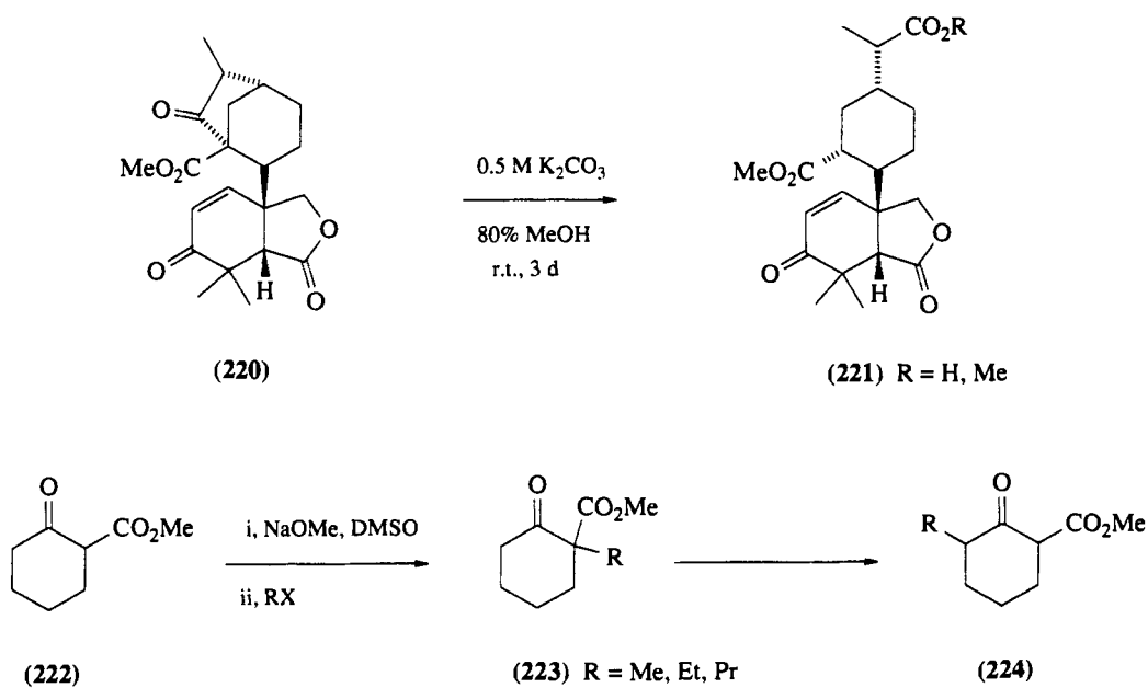
Scheme 95
