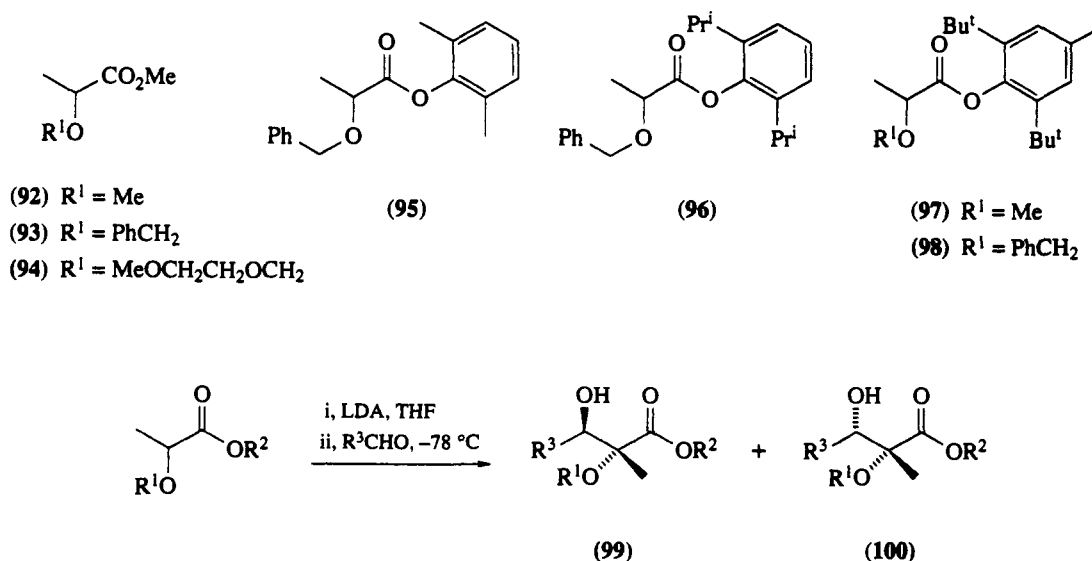
Scheme 5
