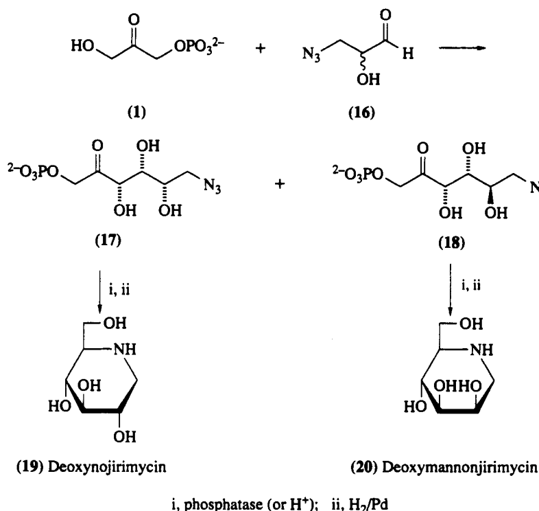
Scheme 5
