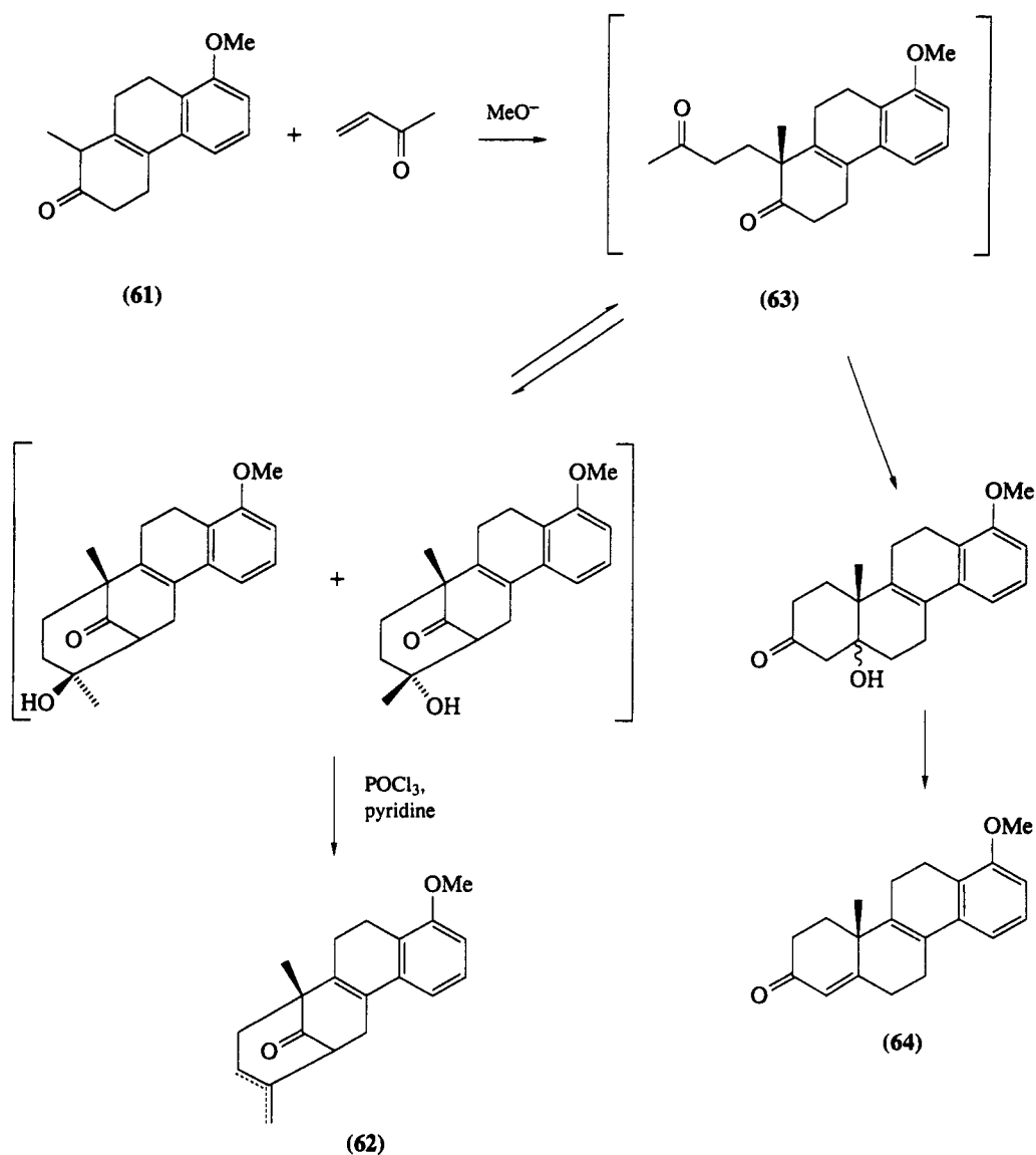
Scheme 3
