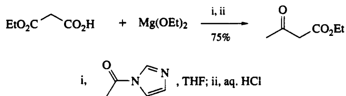
Scheme 8
