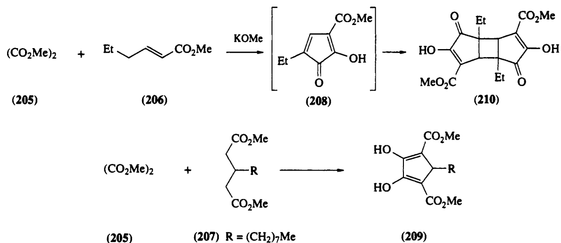
Scheme 91
