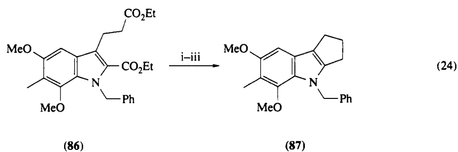
Scheme 35
