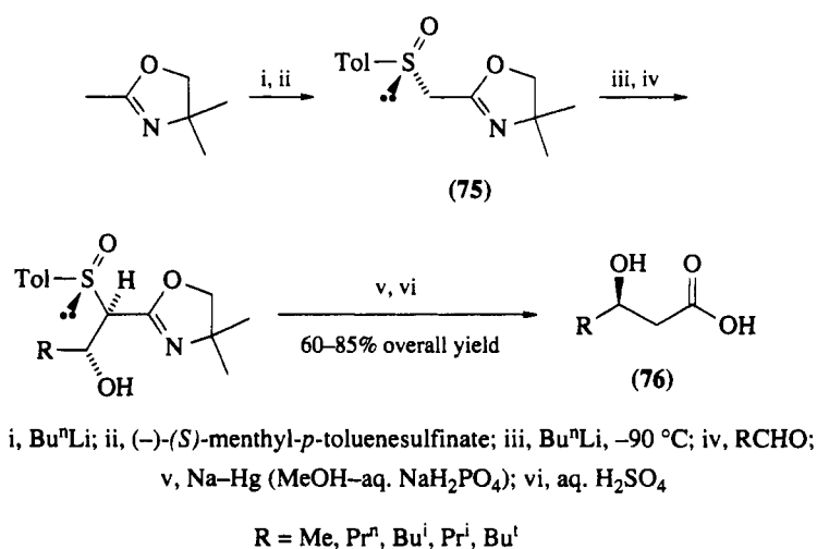
Scheme 28
