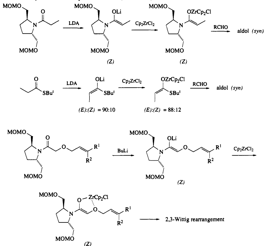
Scheme 44
