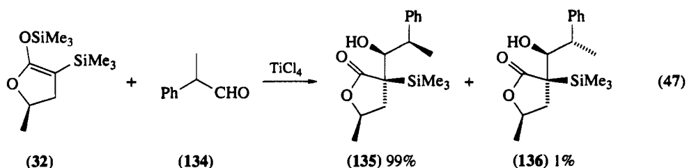
Scheme 13
