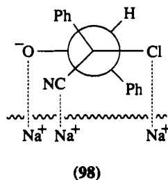
Scheme 21
