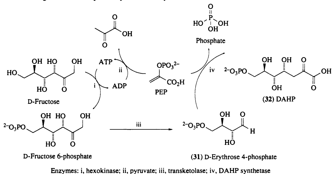
Scheme 10
