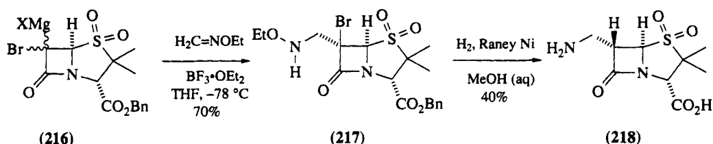
Scheme 45
