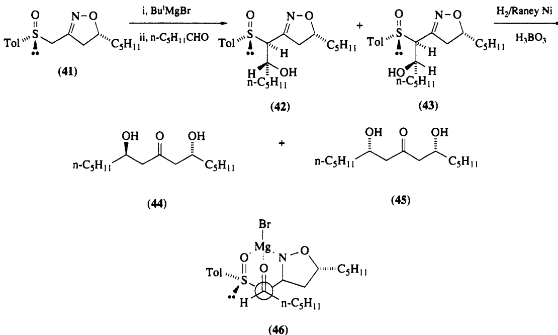
Scheme 18
