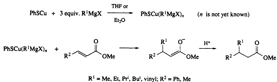
Scheme 50
