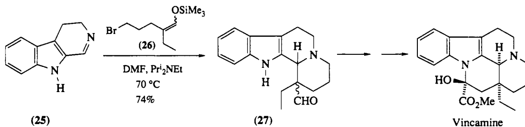
Scheme 14
