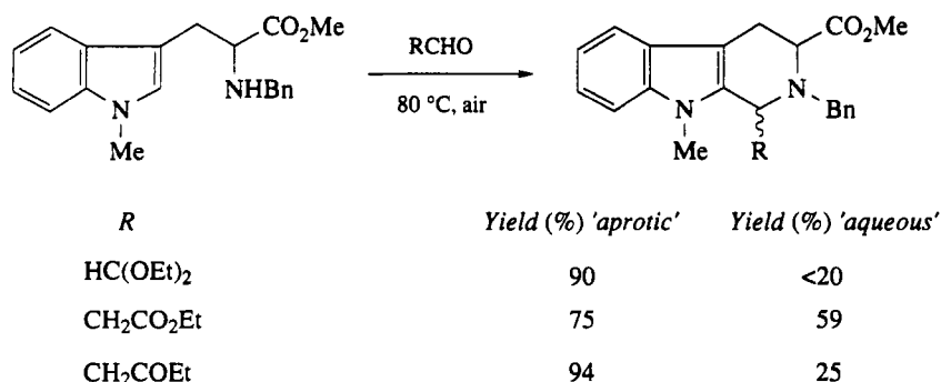
Scheme 17
