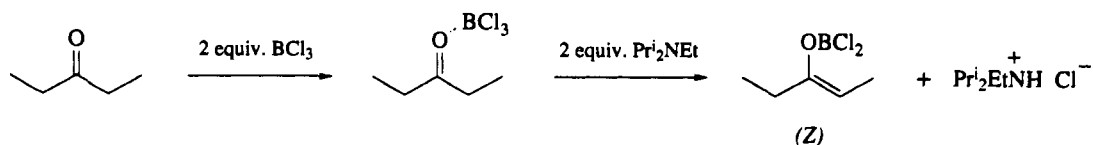
Scheme 27
