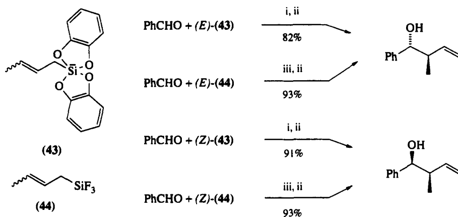
Scheme 20
