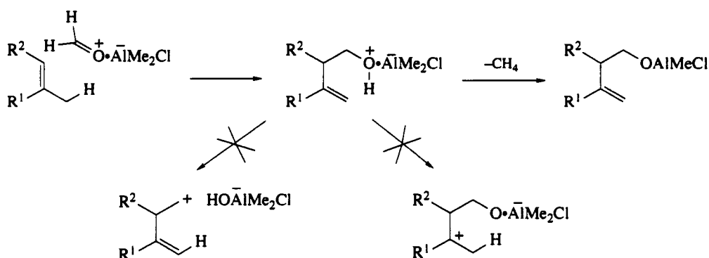
Scheme 3
