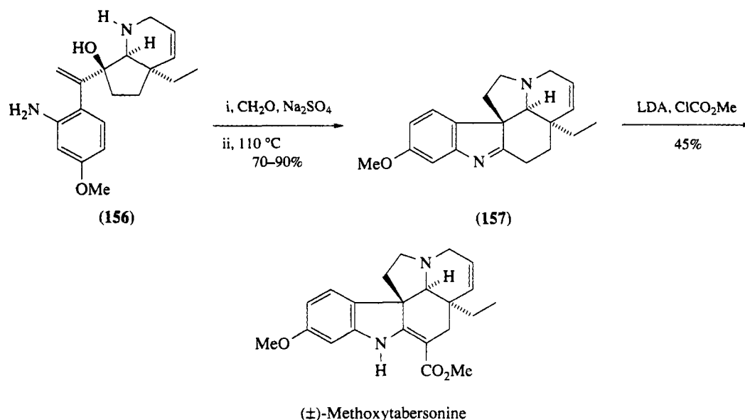
Scheme 56
