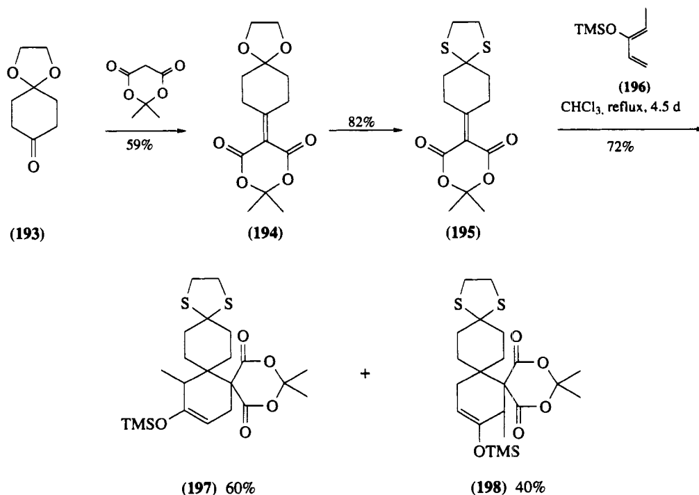
Scheme 35
