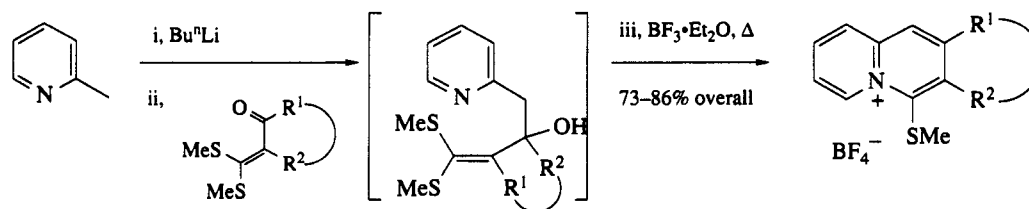
Scheme 35 62
