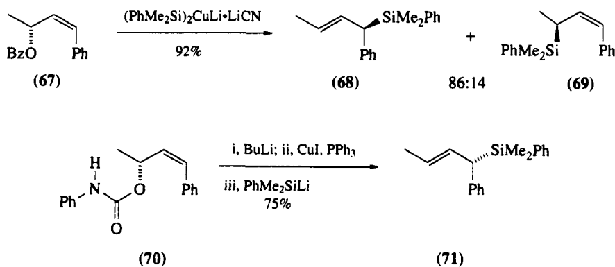
Scheme 65
