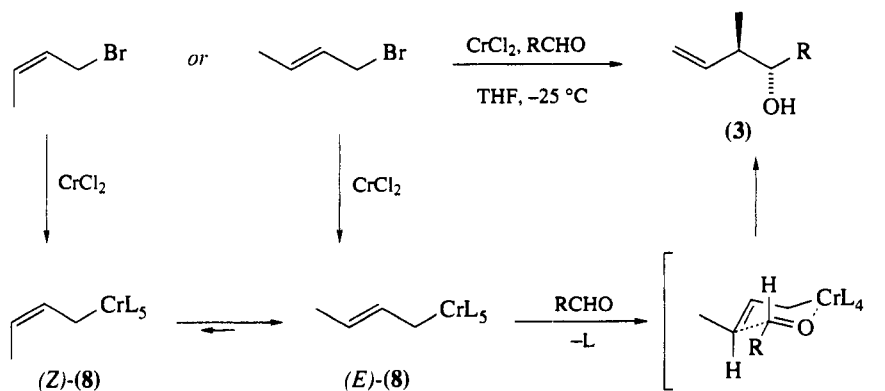
Scheme 5 Type III reactivity of crotylchromium(II) reagents
