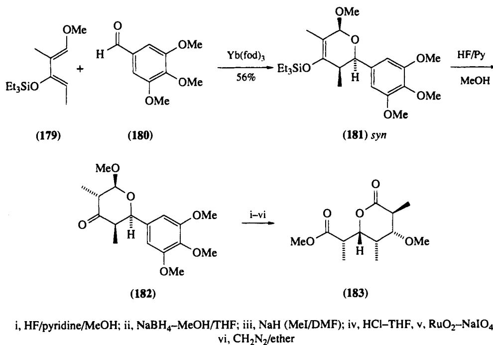
Scheme 50
