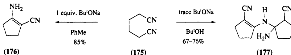
Scheme 84
