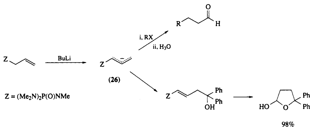
Scheme 11
