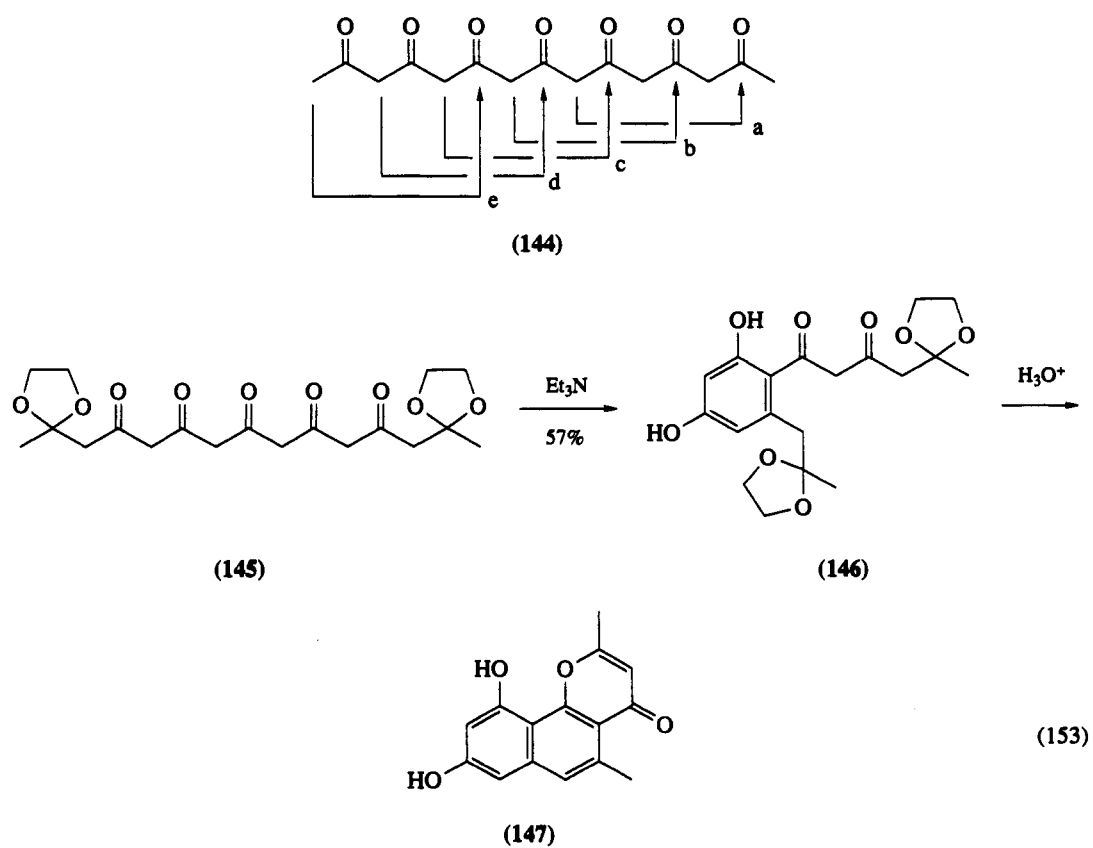
Scheme 5
