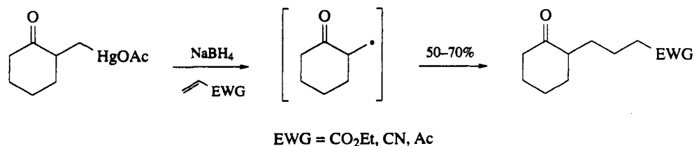
Scheme 19
