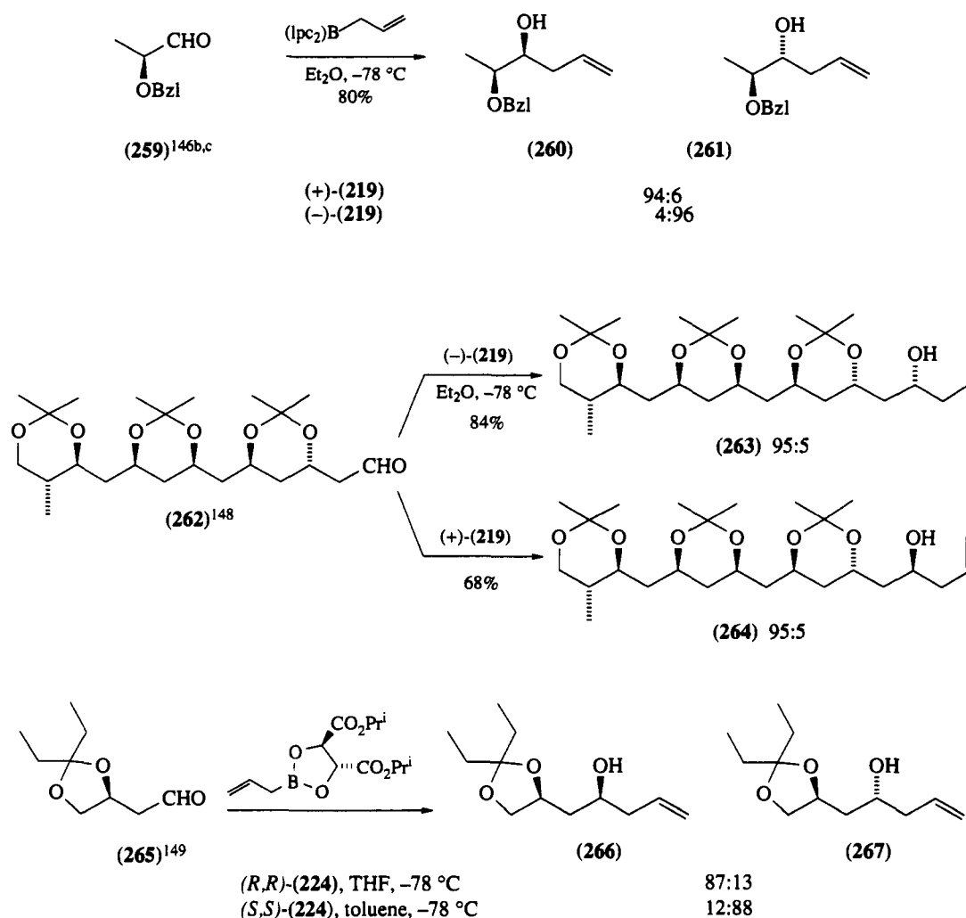
Scheme 49
