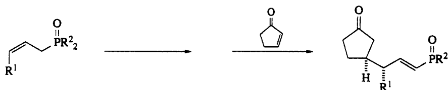
Scheme 20
