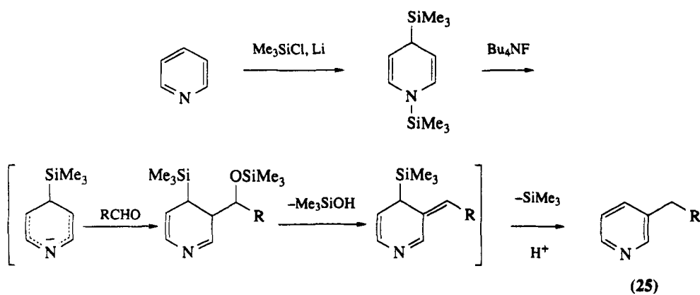
Scheme 11
