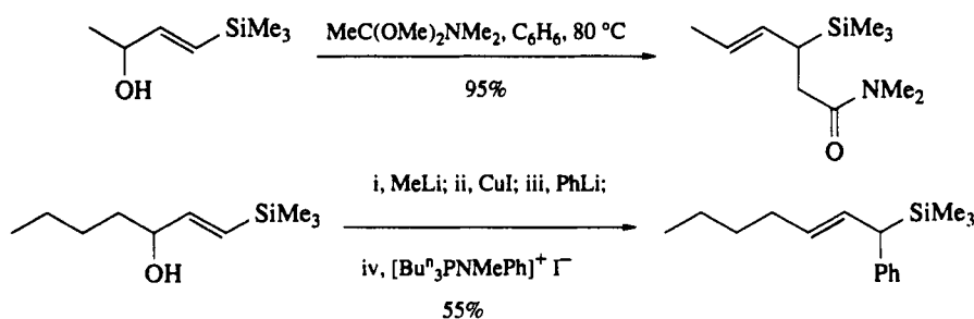
Scheme 80
