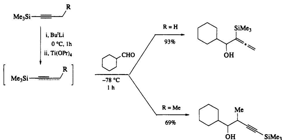
Scheme 30
