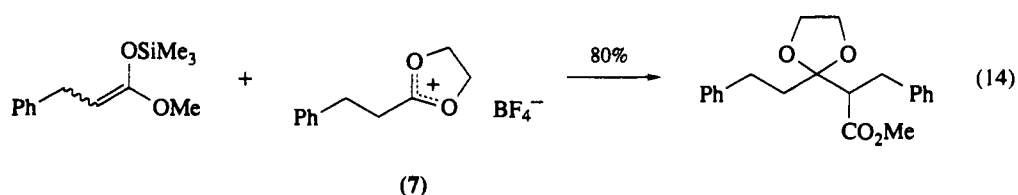
Scheme 12
