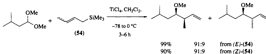
Scheme 40
