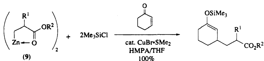
Scheme 21
