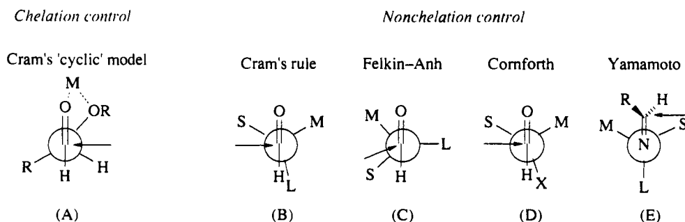
Figure 7 Models used to explain diastereofacial selectivity in the addition of nucleophiles to C=X
