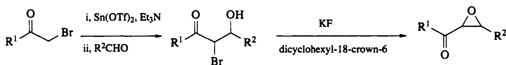
Scheme 16
