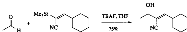
Scheme 34
