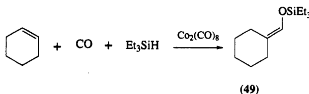
Scheme 17
