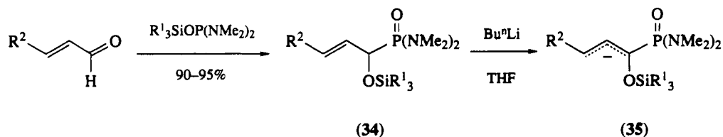
Scheme 17
