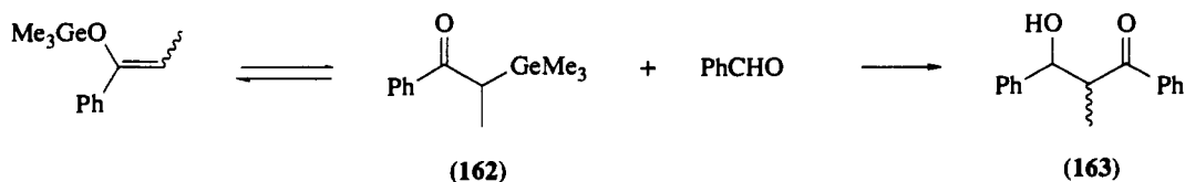
Scheme 53
