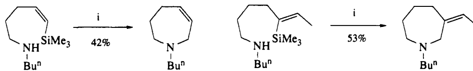
Scheme 39
