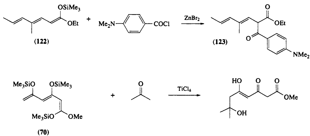
Scheme 44
