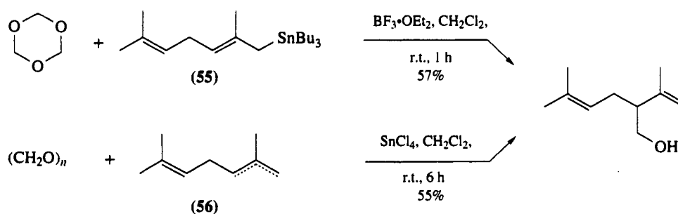
Scheme 46
