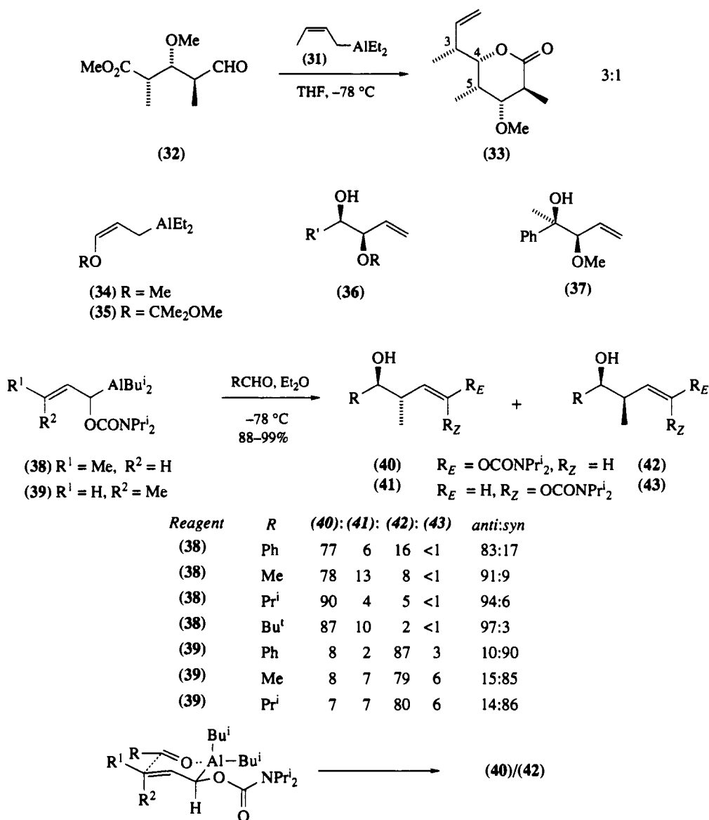
Scheme 9
