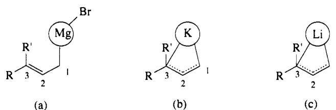
Figure 4 Structures of allyl- and crotyl-magnesium, -lithium and -potassium reagents as determined by isotopic perturbation studies. 6 The magnesium reagent (a) exists as a \sigma -structure and the potassium (b) and lithium (c) reagents exist as \pi -structures
