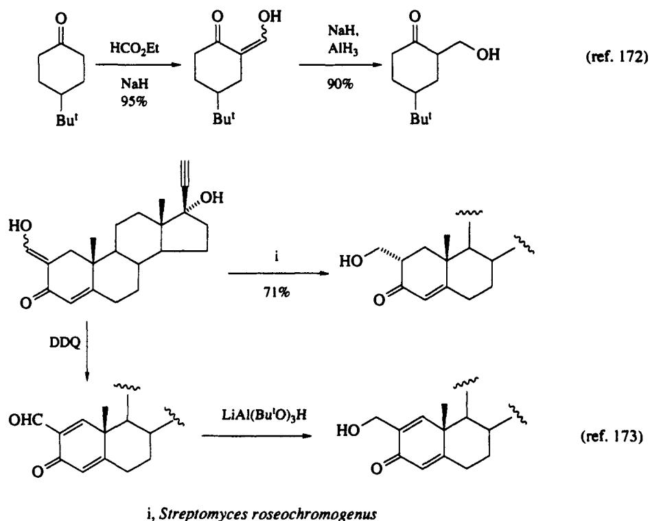
Scheme 65
