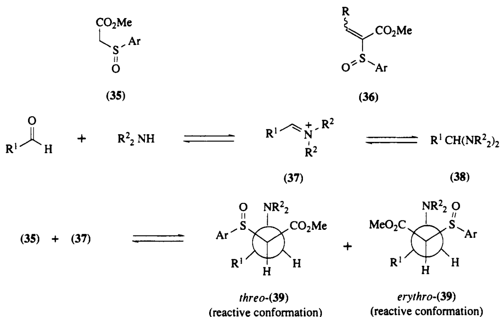
Scheme 11
