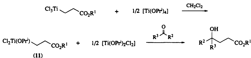
Scheme 12
