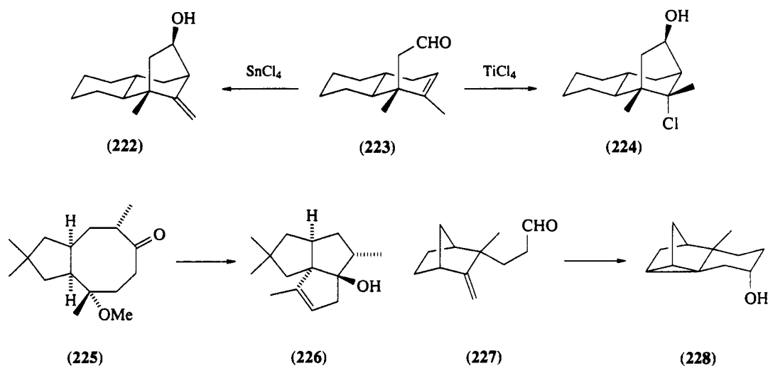
Scheme 33
