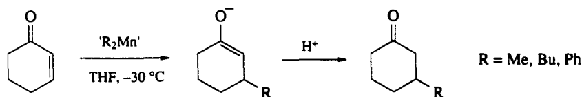
Scheme 66
