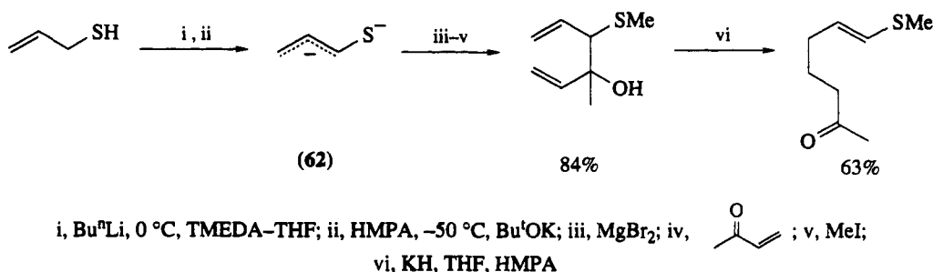
Scheme 35
