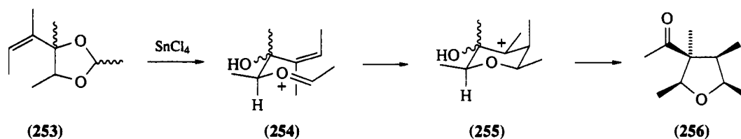
Scheme 37
