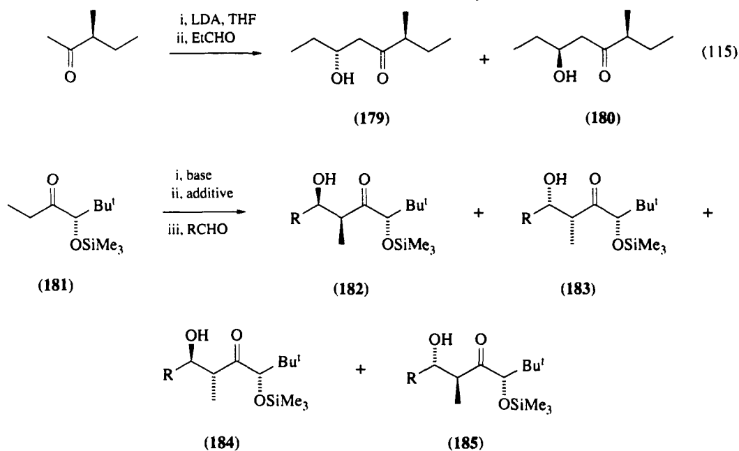
Scheme 11
