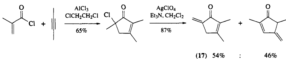
Scheme 23
