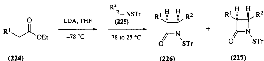
Scheme 47
