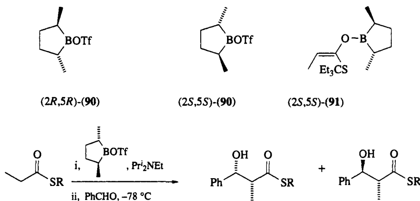
Scheme 37
