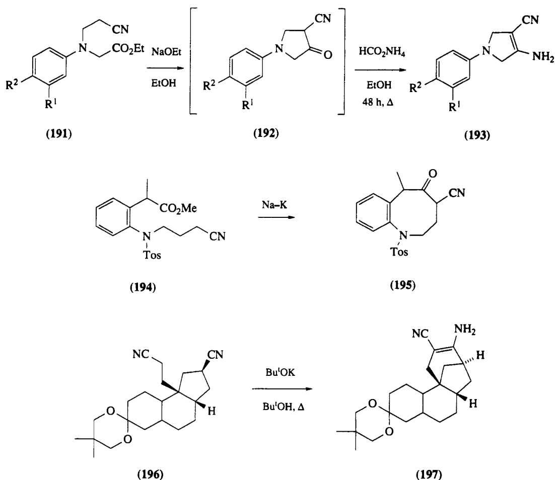
Scheme 88 (continued)
