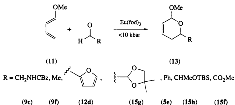
Scheme 15
