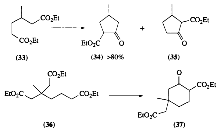
Scheme 24
