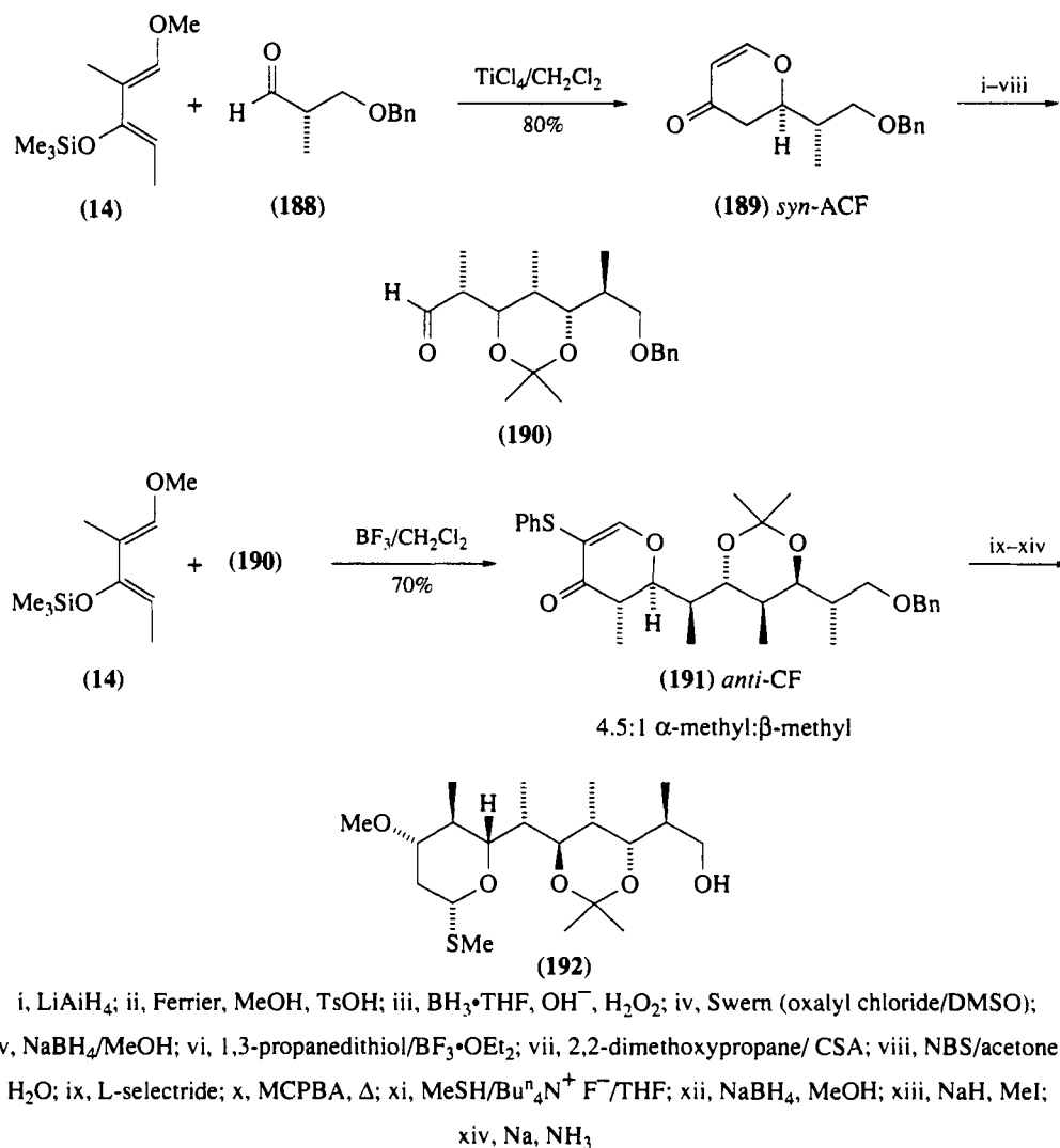
Scheme 52
