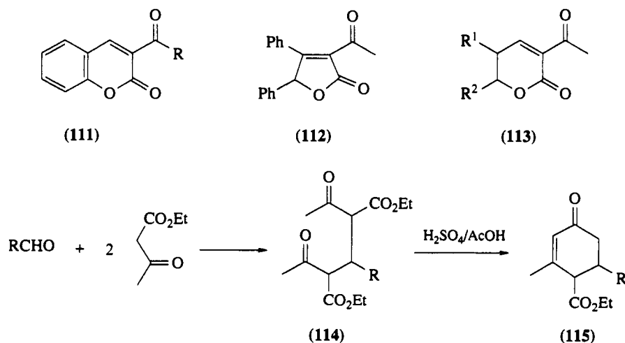
Scheme 17
