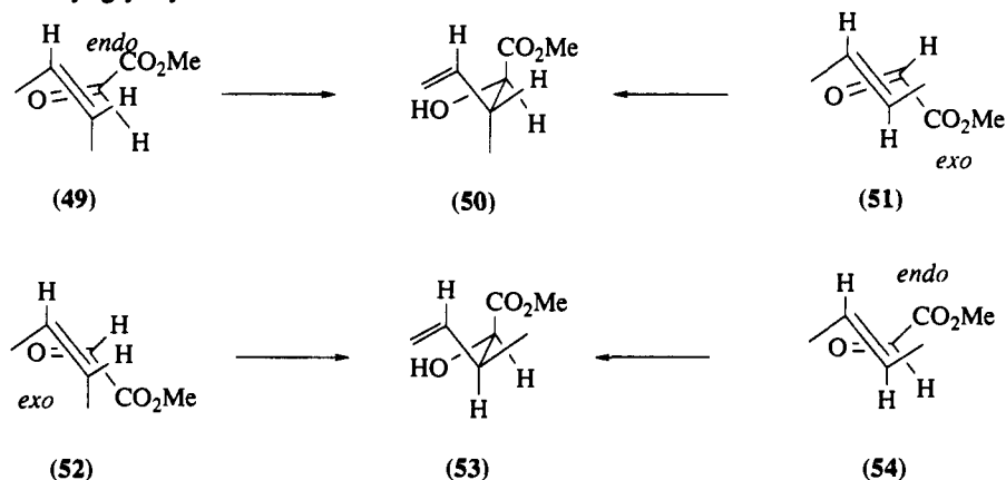
Scheme 10
