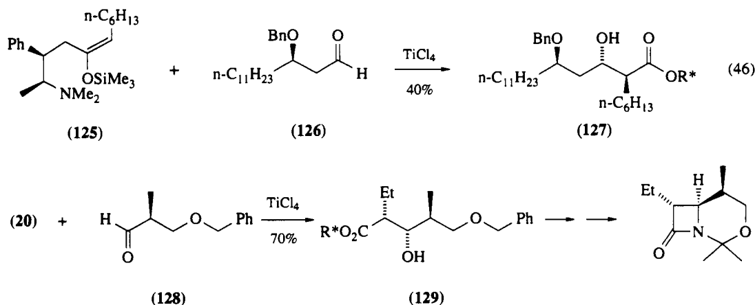
Scheme 10
