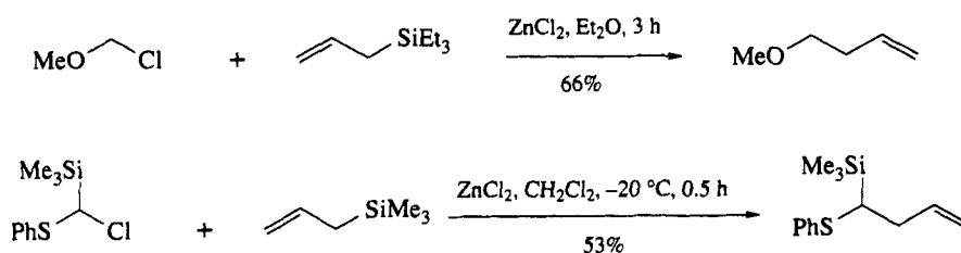
Scheme 53
