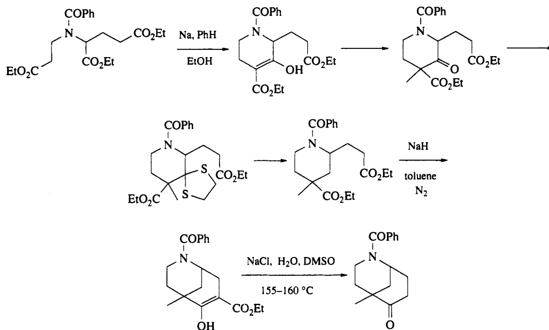
Scheme 35
