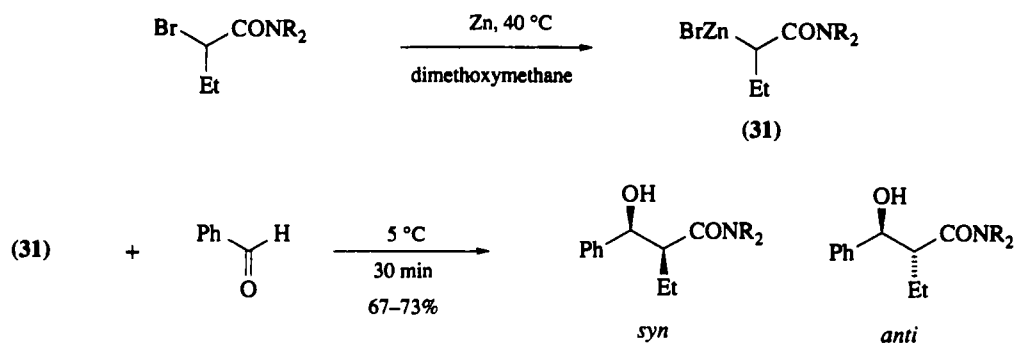
Scheme 12
