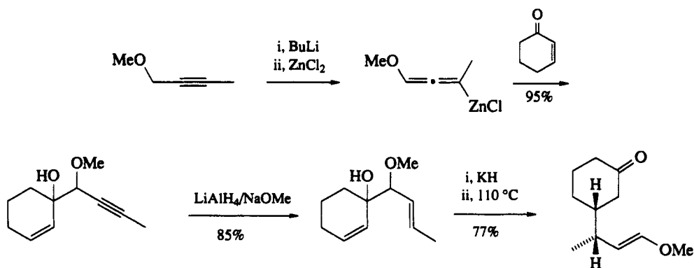
Scheme 28
