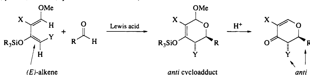
Scheme 20
