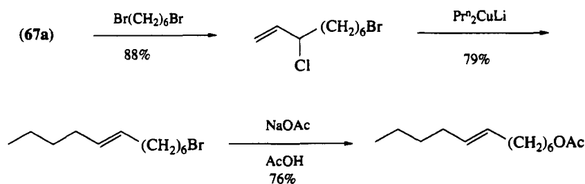
Scheme 47
