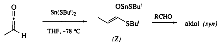
Scheme 38
