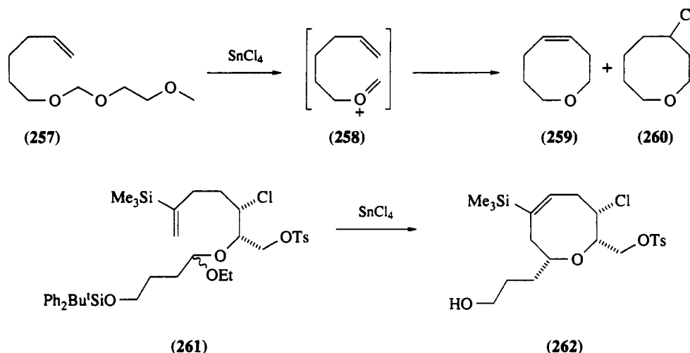
Scheme 38
