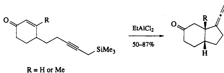
Scheme 20
