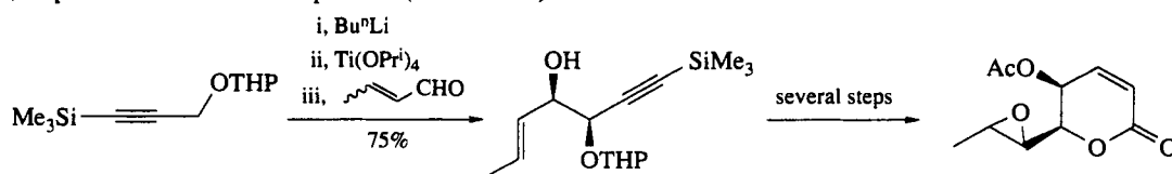
Scheme 32
