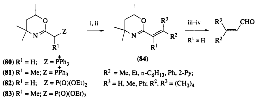
Scheme 30
