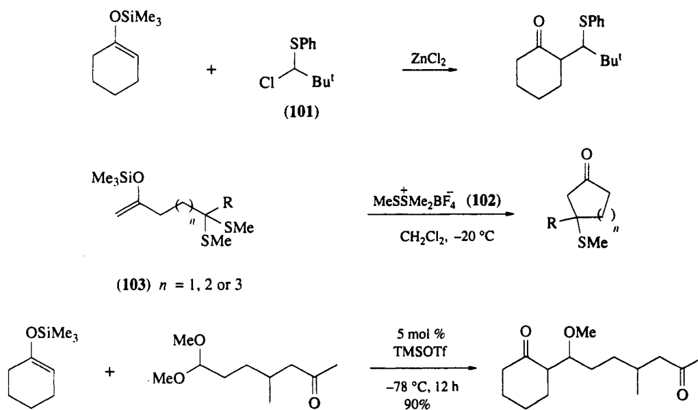
Scheme 37
