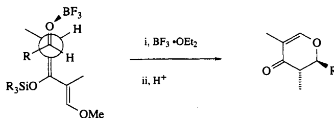
Scheme 16
