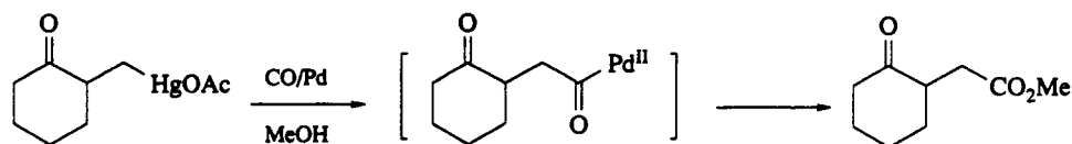
Scheme 26
