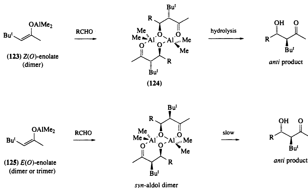
Scheme 51
