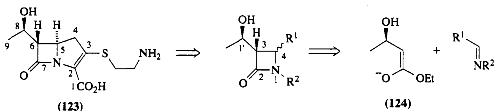
Scheme 25
