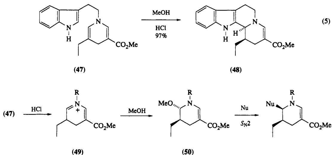
Scheme 22
