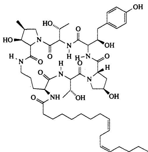
(75) Echinocandin D
