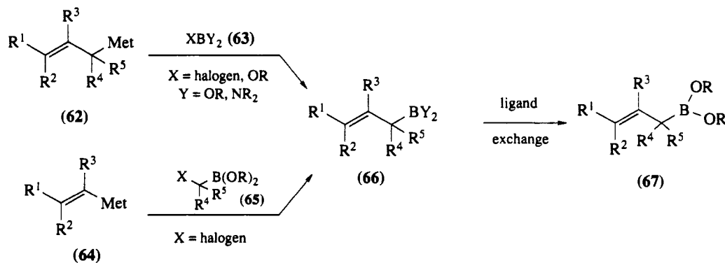
Scheme 13
