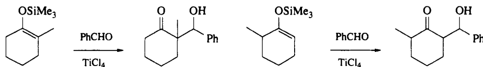
Scheme 34
