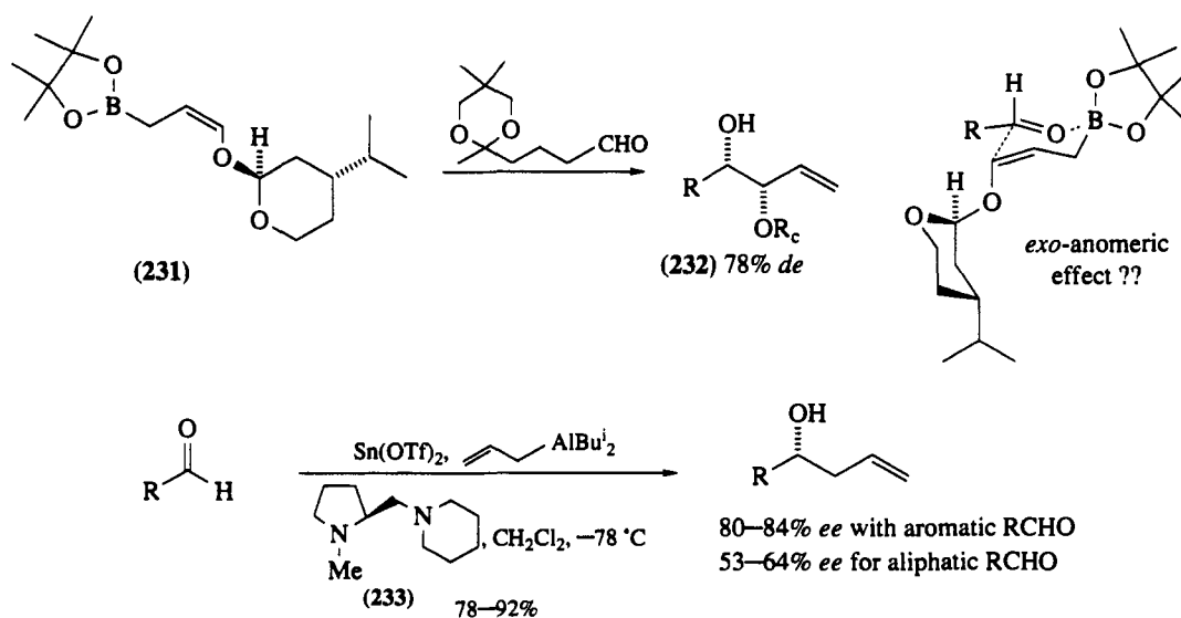
Scheme 42
