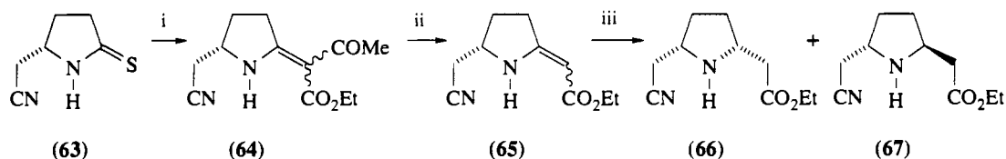
Scheme 15
