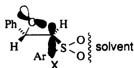
Figure 2 Solvation of the sulfonyl group, enhancing the negative steric interaction in (26)
