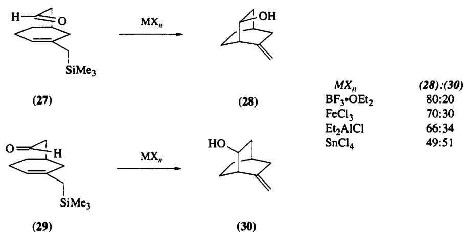
Scheme 12
