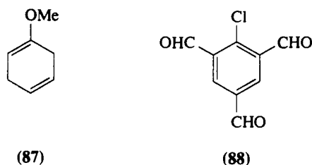
Scheme 6
