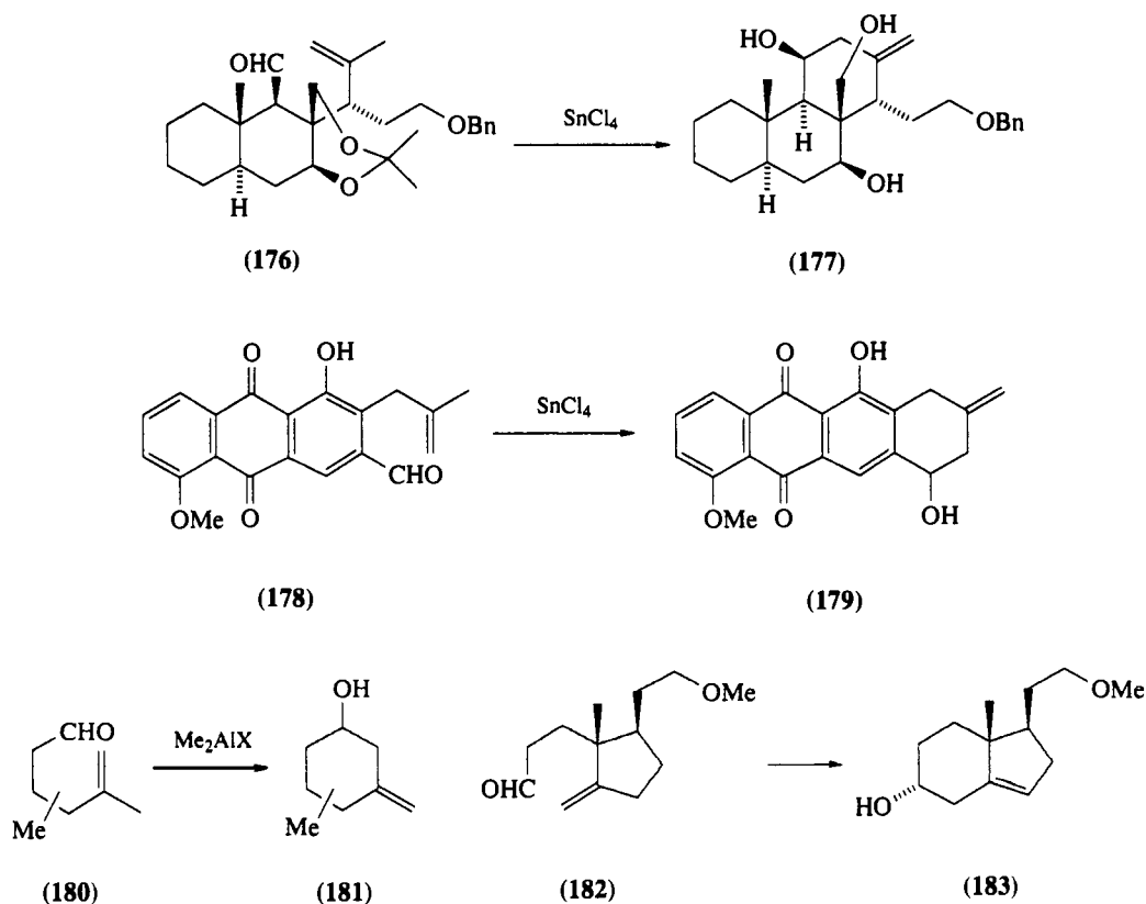
Scheme 29
