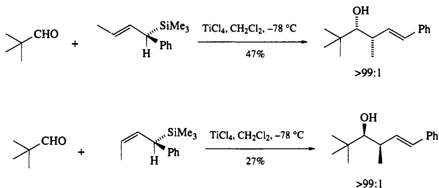
Scheme 13
