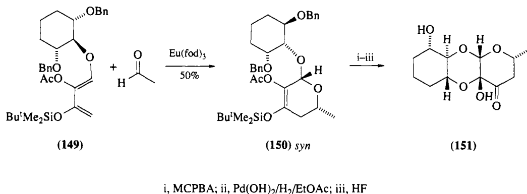
Scheme 42
