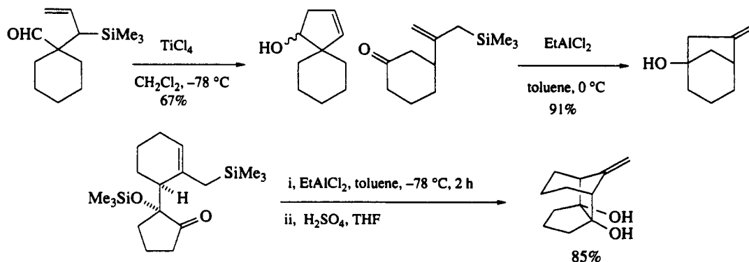
Scheme 10
