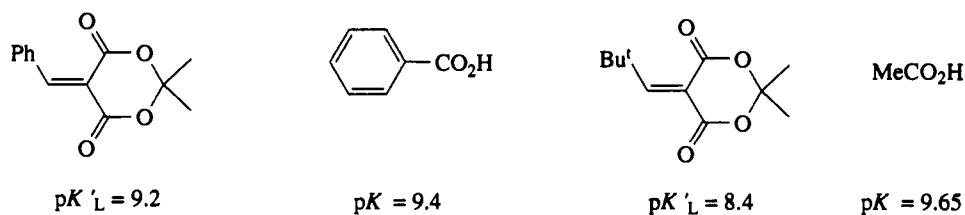
Scheme 7
