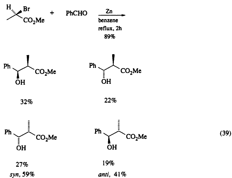
Scheme 13
