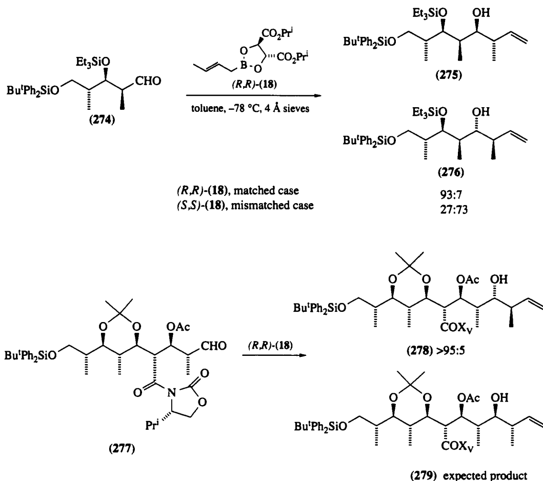
Scheme 51
