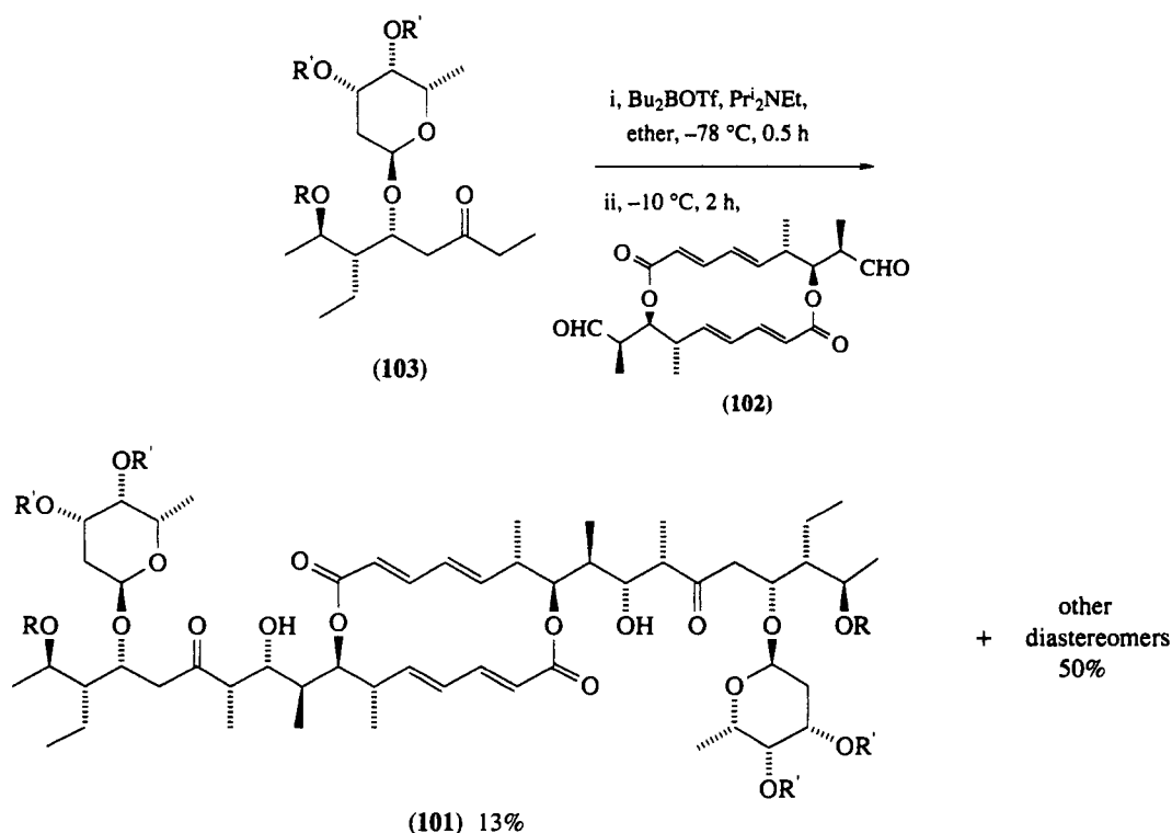
Scheme 43
