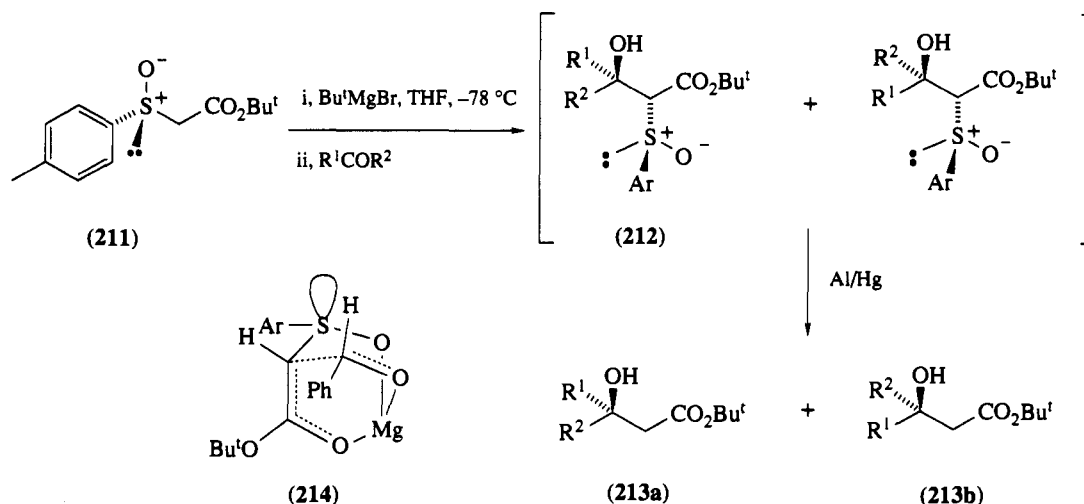
Scheme 13
