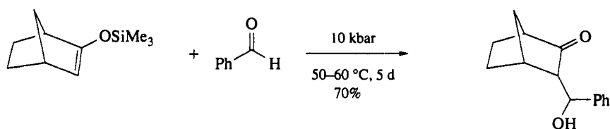
Scheme 32
