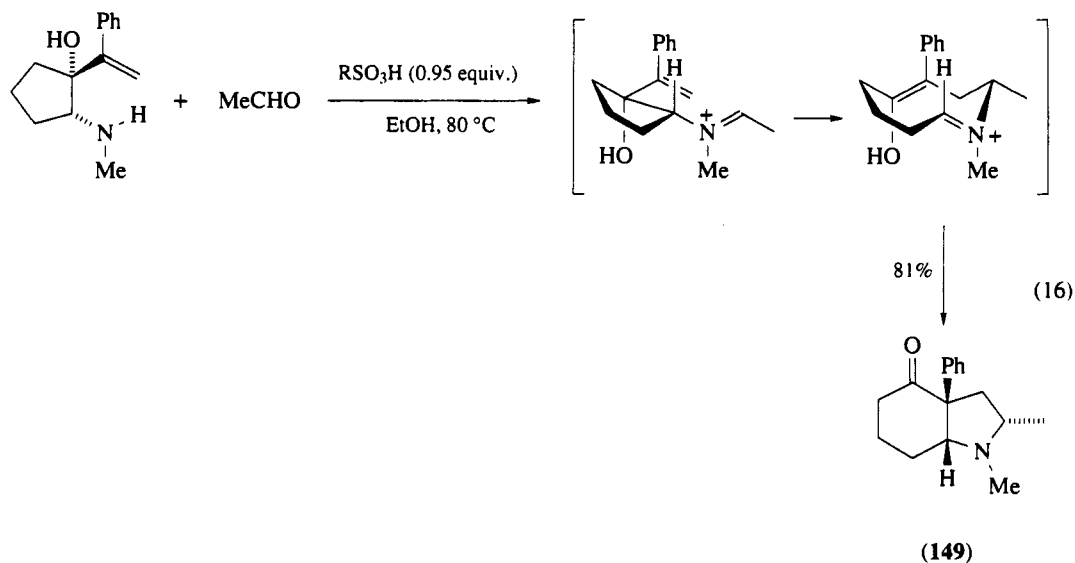
Scheme 53
