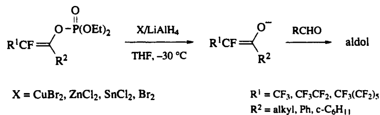
Scheme 34
