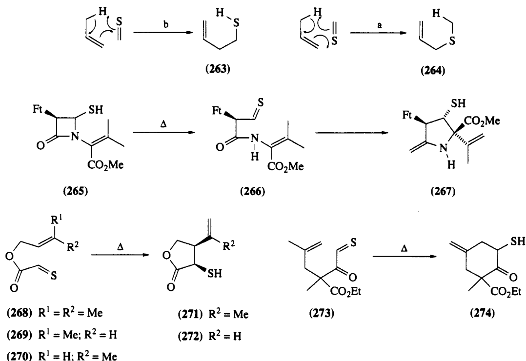
Scheme 39
