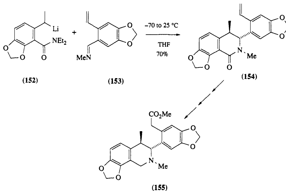
Scheme 32
