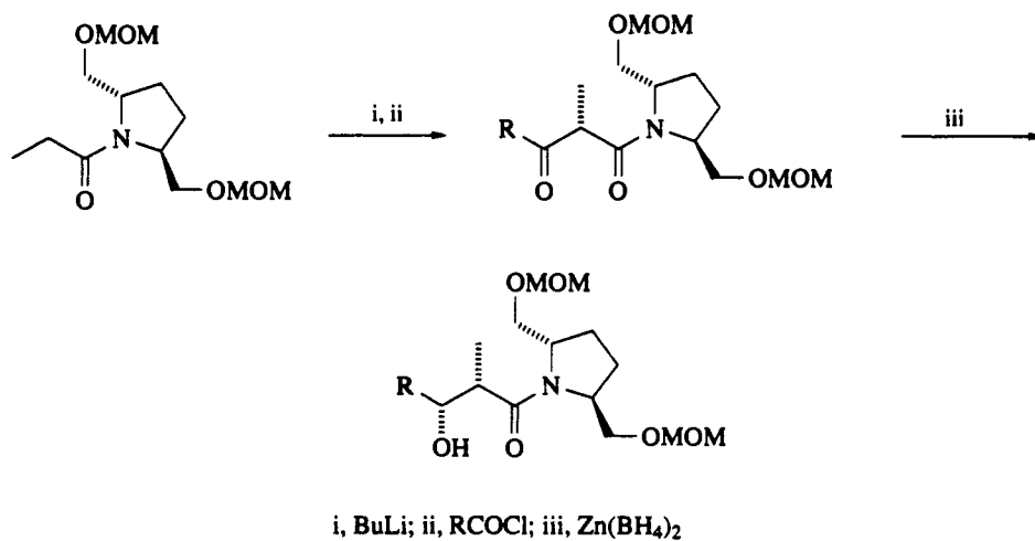
Scheme 81
