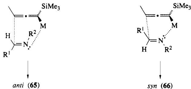
Figure 12 Proposed transition states for the formation of diastereomeric syn and anti alkynic amines in reactions of \alpha -silylallenic reagent ( 63 ) with aldimines 37
