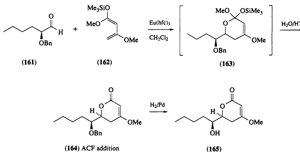
Scheme 45
