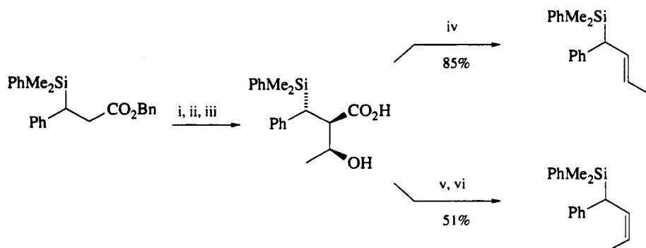
Scheme 76
