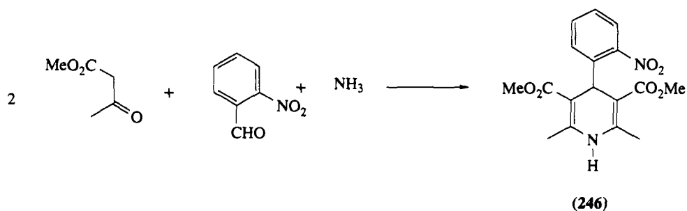
Scheme 50
