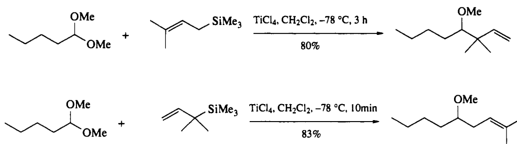
Scheme 37
