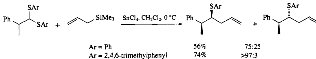
Scheme 54
