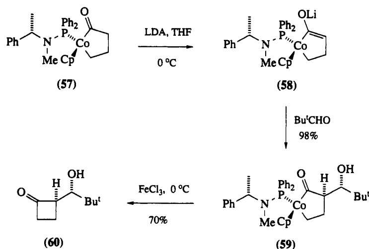
Scheme 7
