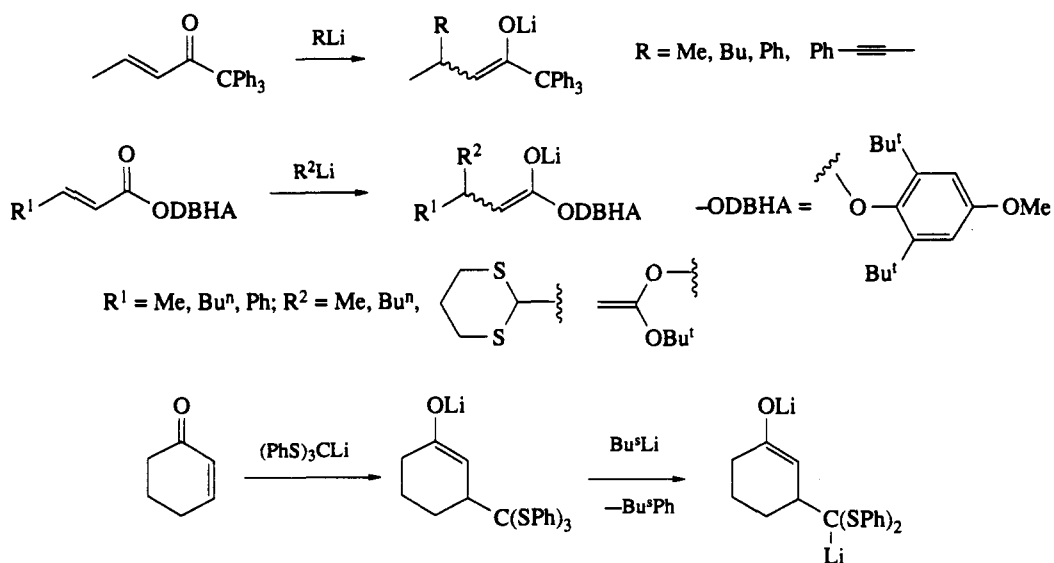
Scheme 17
