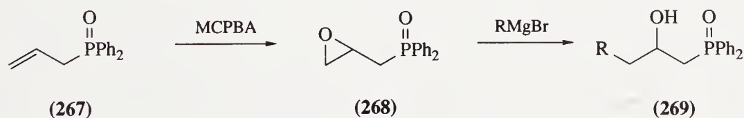
Scheme 36
