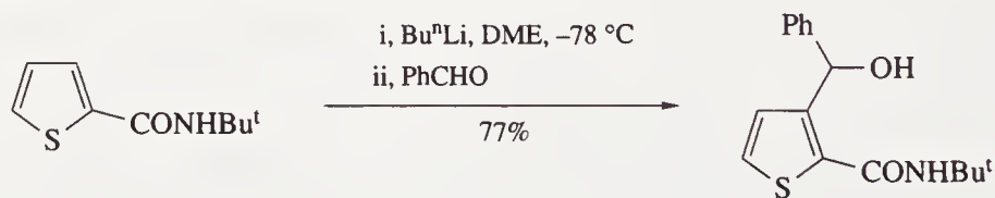
Scheme 23
