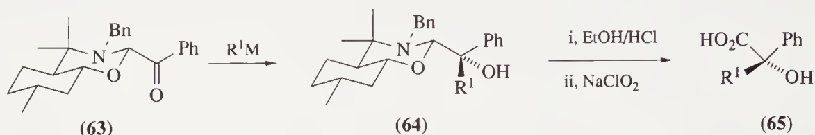
Scheme 5
