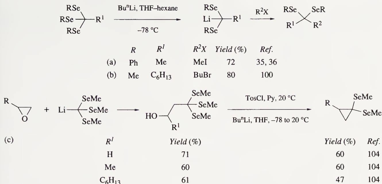
Scheme 77
