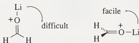
Figure 6 Relative ease of distortions for the \text{Li}^+ /formaldehyde complex
