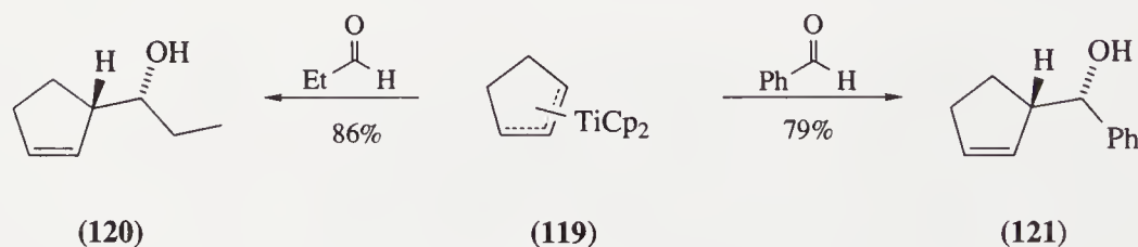
Scheme 13
