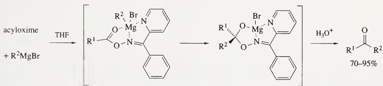
Scheme 23
