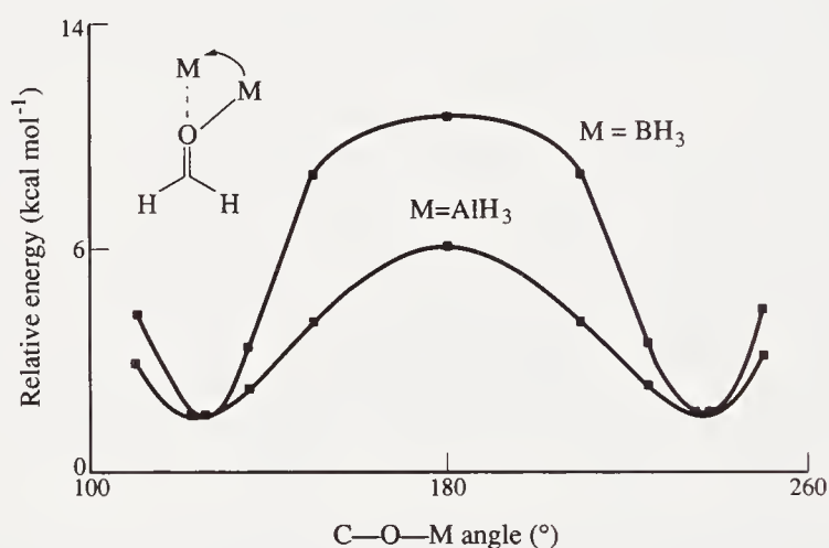
Figure 8 Rotational profile for formaldehyde complexes of BH 3 and AlH 3 [ \tau(\text{H}-\text{C}-\text{O}-\text{M}) = 0^\circ ]
