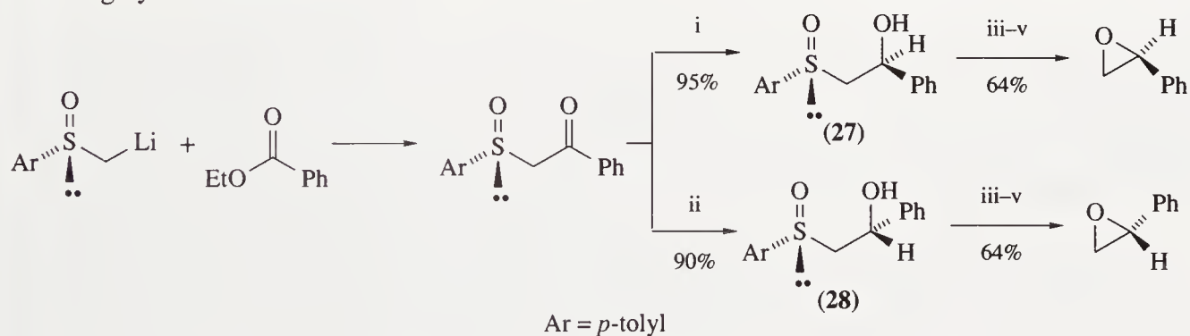
Scheme 16
