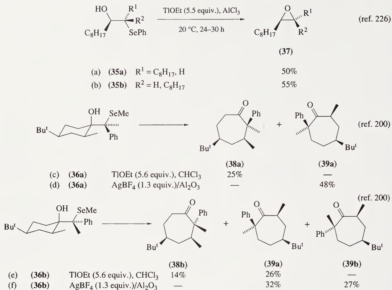
Scheme 196
