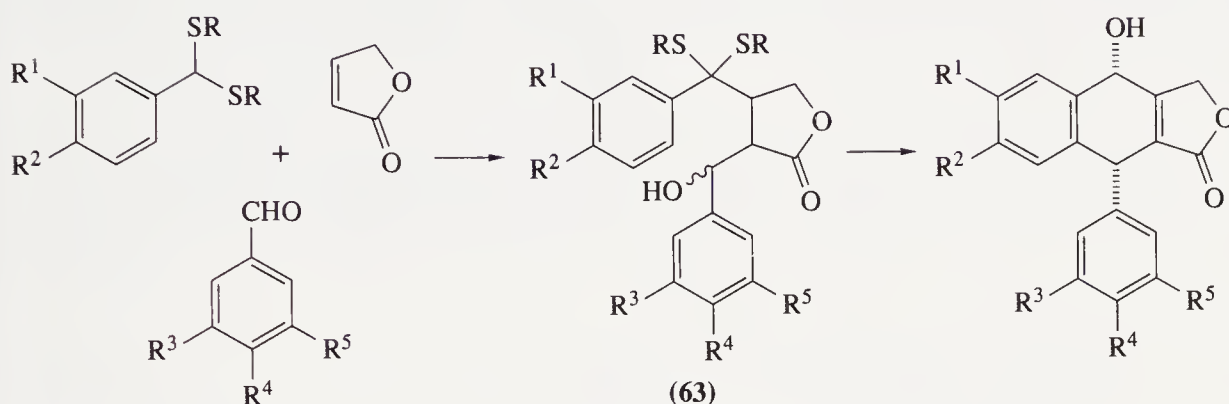
Scheme 37
