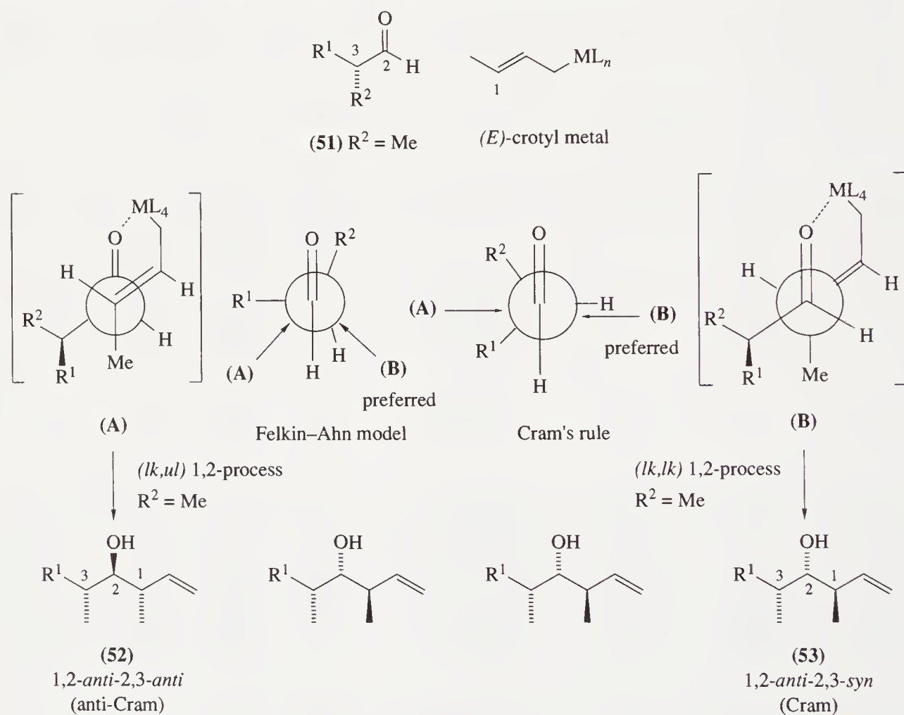
Scheme 4
