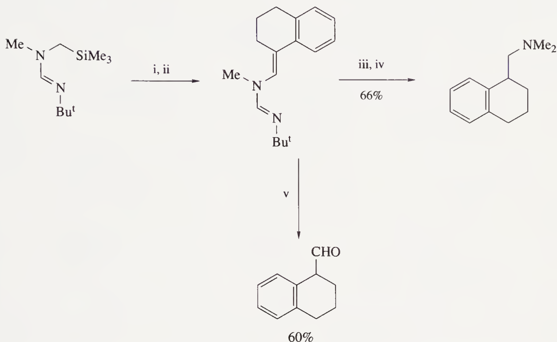
Scheme 39
