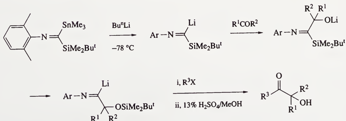
Scheme 7
