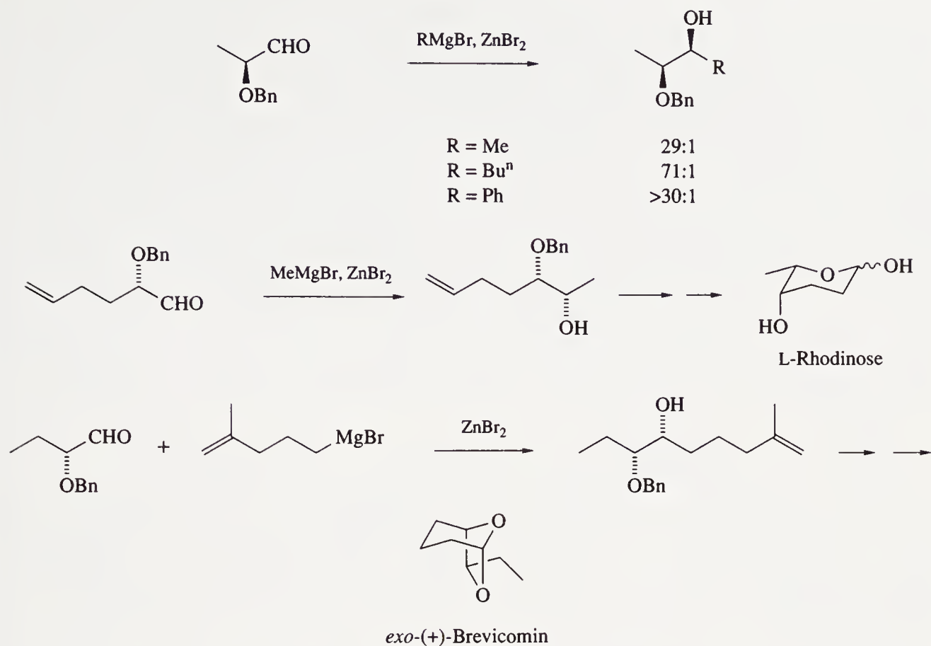
Scheme 9
