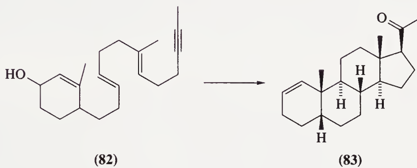
Scheme 40
