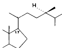
(3.105) Campesterol (24- \alpha -methyl-cholesterol) (3.107)
