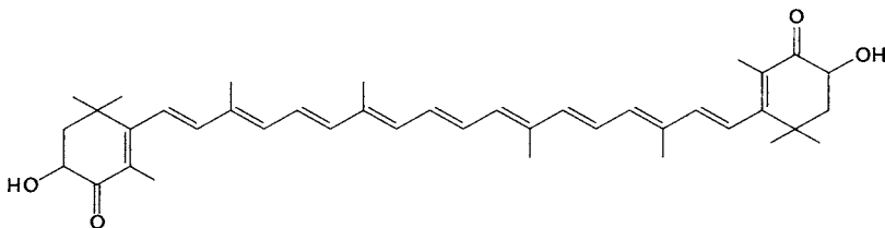
Astaxanthin (XI)
