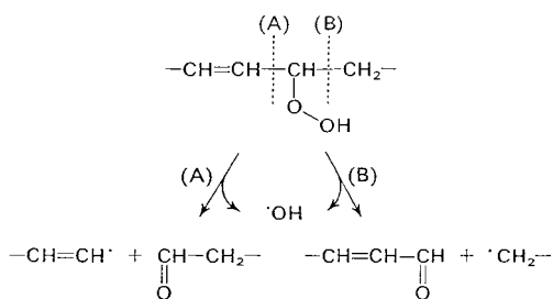
Fig. 3.26. \beta -Scission of monohydroperoxides (according to Badings , 1970)
