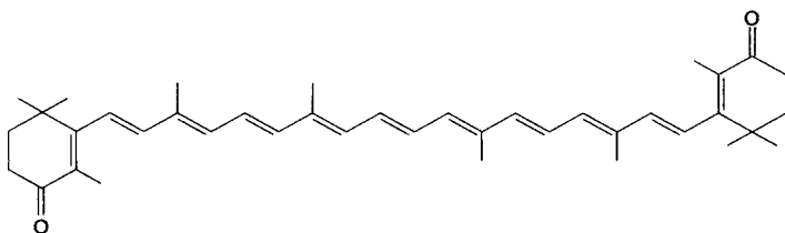
Canthaxanthin (XII)
