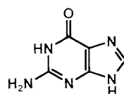
Guanine (G)
