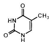
Thymine (T)
