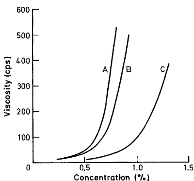
Fig. 4.20. Viscosity curves of carrageenan aqueous solutions. A: Euclidean spinosum , C: Chondrus crispus , B: A and C in a ratio of 2:1, 40 °C, 20 rpm (according to Whistler, 1973)
