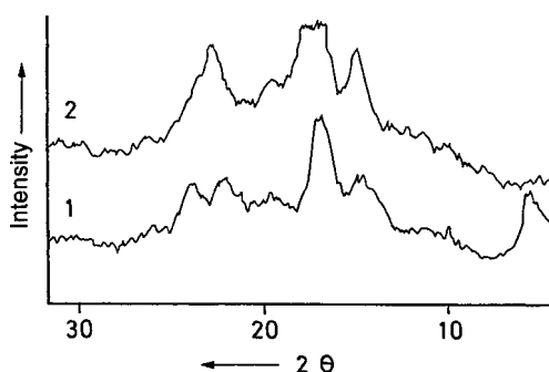
Fig. 4.28. X-ray diffraction diagrams of potato starch before (1) and after (2) thermal treatment ( 102^{\circ}\text{C}/16\text{ h} ) at a water content of 40%. The pattern of native starch (18.3% of water) corresponds to the B-type and that of treated starch (24.2% of water) to the A-type (according to Galliard , 1987)
