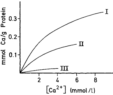
Fig. 10.1. Calcium binding by I: \alpha_{s1} -casein (0.38), II: \beta -casein (0.21) and III: \kappa -casein (0.05). The bound phosphate residues in mmol/g of casein are given in brackets (according to Walstra and Jenness, 1984)
