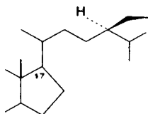
\beta -Sitosterol (24- \alpha -ethyl-cholesterol)
