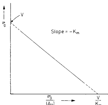
Fig. 2.24. Determination of K_m and V (according to Hofstee )
