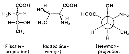
(Fischer-projection) (dotted line-wedge) (Newman-projection) L-Threonine, (2S:3R)-Threonine (Common in proteins)
