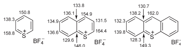
Figure 17 ^{13}\text{C} chemical shifts for thiinium salts.
