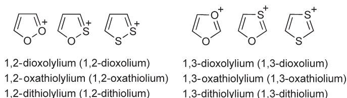
Figure 5 Structure and nomenclature of oxygen/sulfur five-membered cations.
