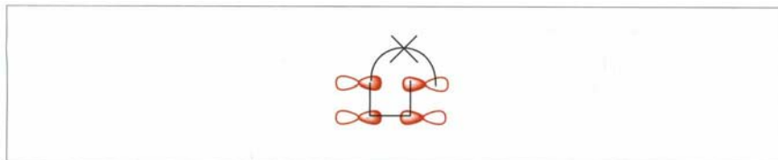
Figure 7.15 Impossibility of antarafacial attack in ethene dimerization
