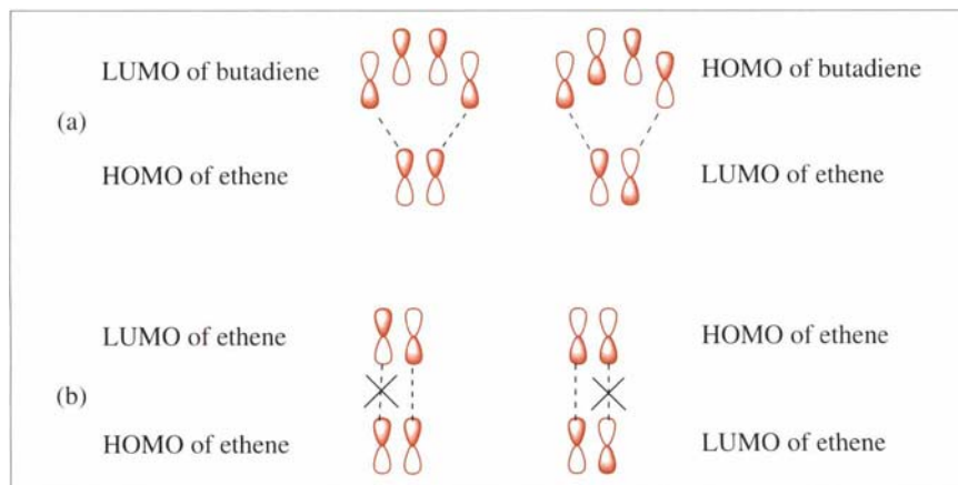
Figure 7.6 HOMO–LUMO interactions for (a) ethene with buta-1,3-diene and (b) ethene with ethene
