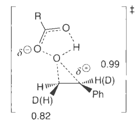
Unsymmetrical transition state
