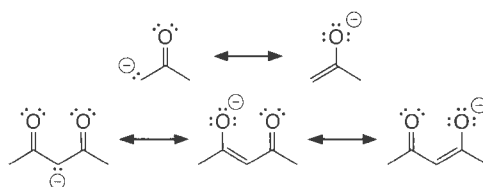
Resonance structures for enolates
