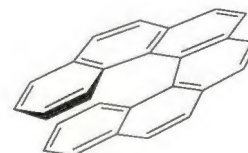
[6]Helicene
