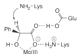
Mandelate racemase active site
