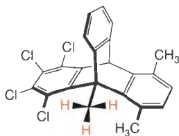
Slowed rotation in a methyl group
