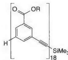
Foldamer structure
