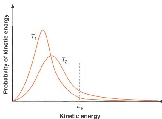
Figure 7.5 Diagram showing the Boltzmann distribution of molecules as a function of kinetic energy for two different temperatures. T_1 is the lower temperature and T_2 is a higher temperature.
