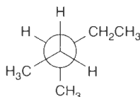
3-Methylpentane
