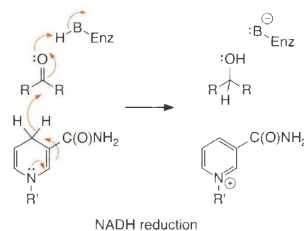
NADH reduction
