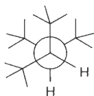
1,1,2,2-Tetrakis( t -butyl)ethane
