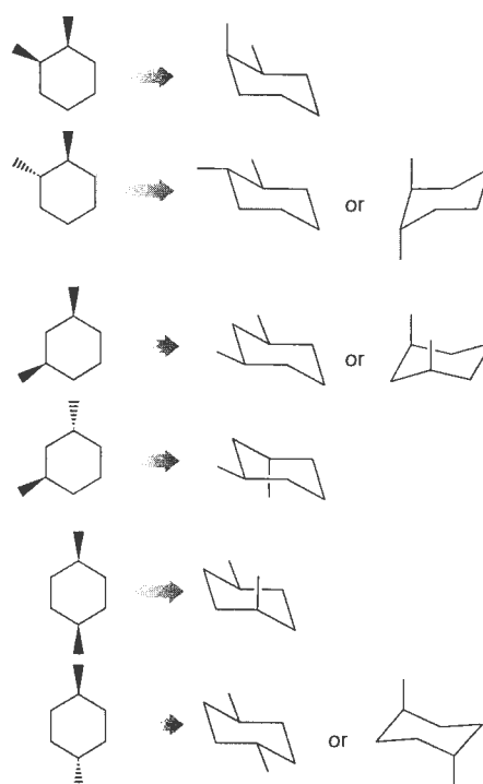
Dimethyl cyclohexanes
