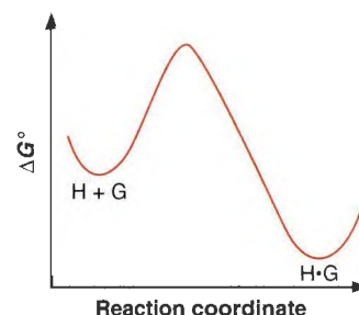
Figure 4.1 A normal reaction coordinate diagram for an exergonic binding process.
