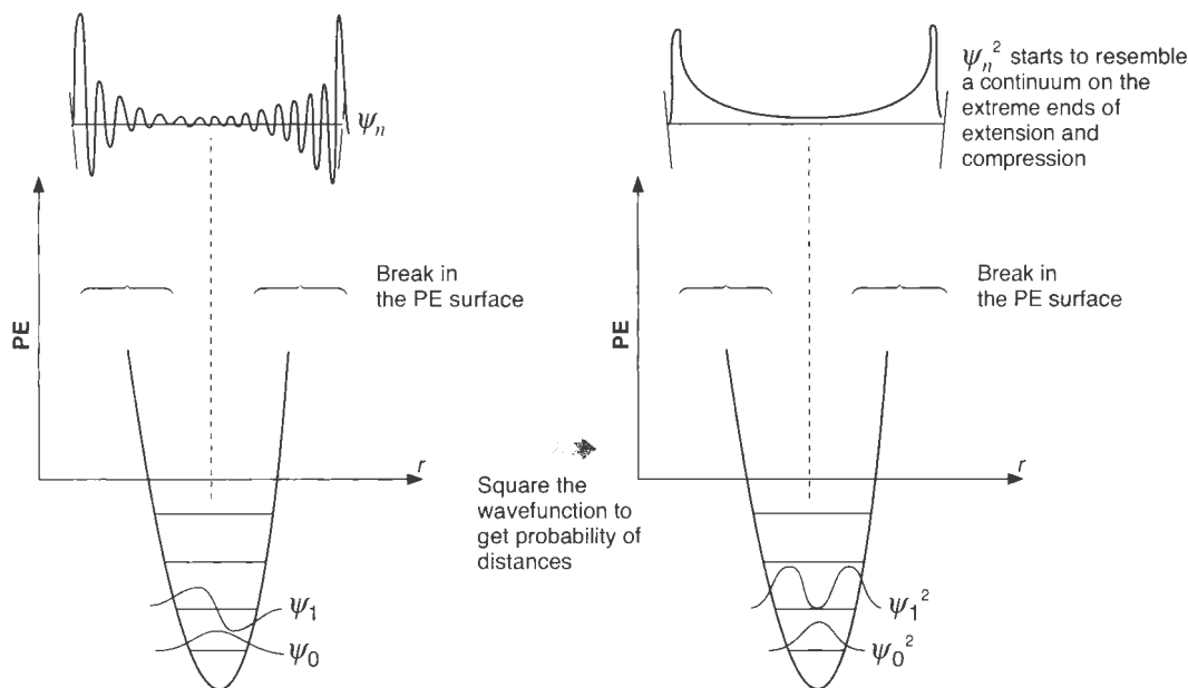
The harmonic oscillator, showing \psi and \psi^2
