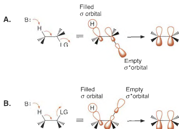
Figure 10.13 Stereoelectronically-controlled E2 pathways. A. Antiperiplanar, and B. Synperiplanar.
