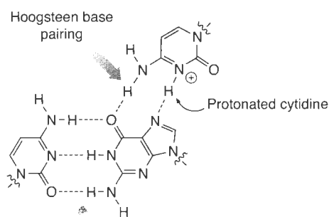
Watson–Crick base pairing
