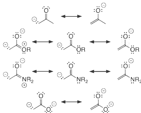
Resonance structures for enolates
