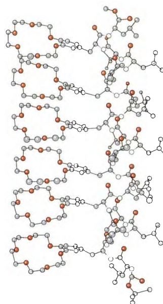
An artificial ion channel
