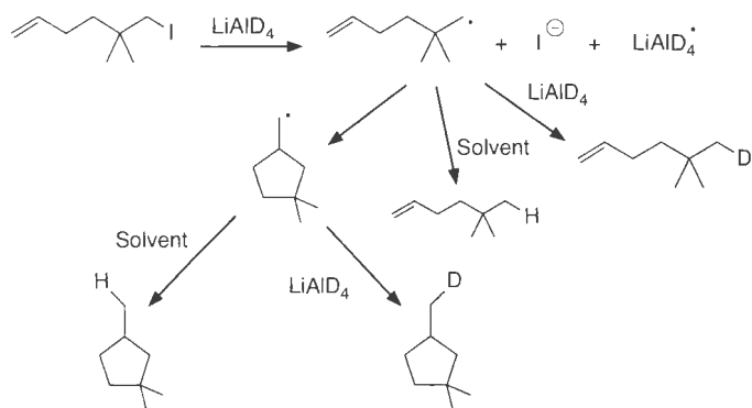
Figure 11.13 Pathway undertaken in the reduction of 6-iodo-5,5-dimethyl-1-hexene with \text{LiAlD}_4 .
