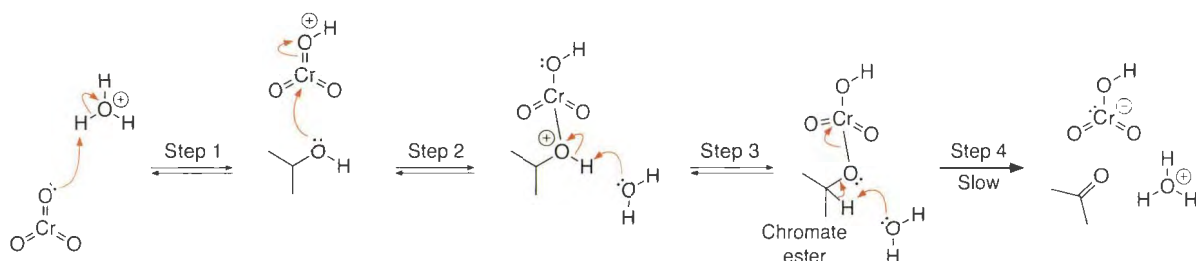
Scheme 10.13 Electron pushing for the \text{CrO}_3 oxidation of a secondary alcohol.
