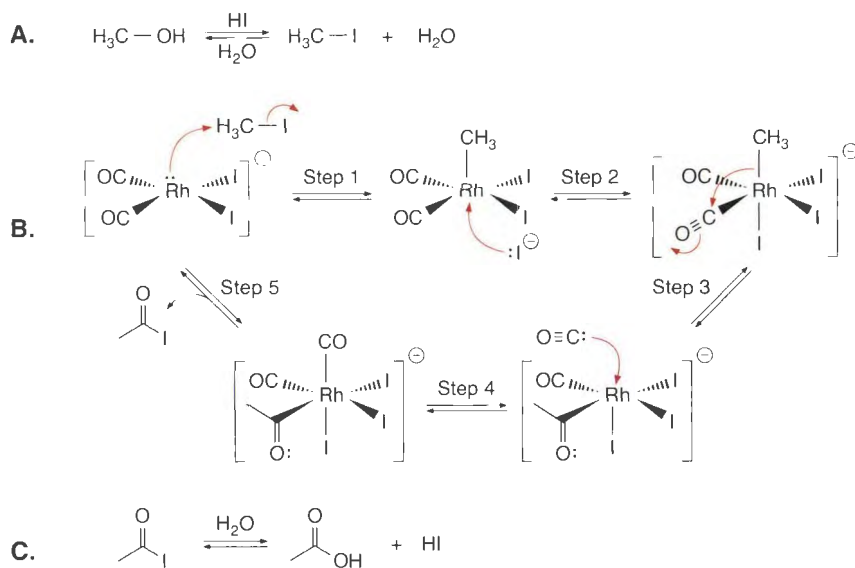
Figure 12.12 The catalytic cycle involved in the Monsanto acetic acid synthesis. A. An equilibrium established in solution that supplies \text{CH}_3\text{I} . B. The organometallic portion of the reaction. C. Conversion of the acetyl iodide to acetic acid.
