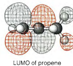
LUMO of propene
