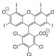
Rose bengal
