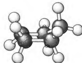
Cyclopentane envelope conformation
