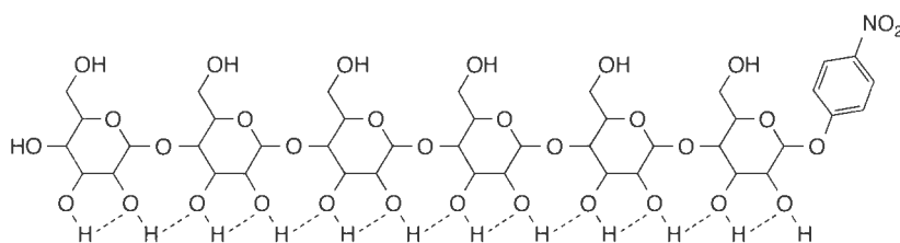
Intramolecular hydrogen bonding in oligosaccharides
