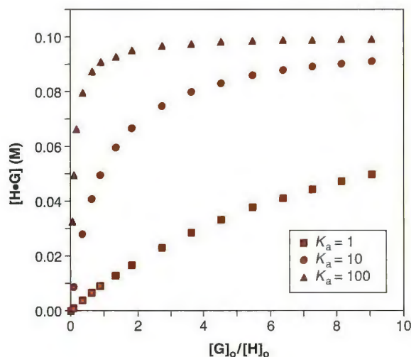
Figure 4.4 Binding isotherms for varying K_a with [H]_o = 0.1 M. ■ K_a = 1 \text{ M}^{-1} (hence K_d = 1 \text{ M} and is above [H]_o ), ● K_a = 10 \text{ M}^{-1} (hence K_d = 0.1 \text{ M} and is equal to [H]_o ), and ▲ K_a = 100 \text{ M}^{-1} (hence K_d = 0.01 \text{ M} and is below [H]_o ).
