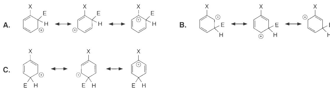
Figure 10.20 Resonance structures resulting from electrophilic addition to a substituted benzene ring. A. Ortho, B. Meta, and C. Para.
