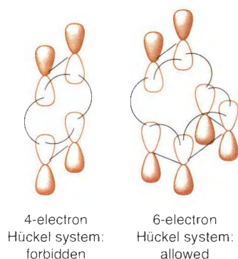
Figure 15.8 The application of aromatic transition state theory to cycloadditions.
