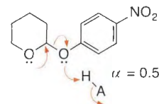
General-acid catalysis
