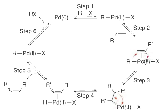
Proposed mechanism of the Heck reaction
