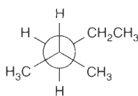
2-Methylpentane
