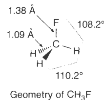
Geometry of \text{CH}_3\text{F}
