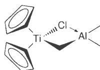
Tebbe's reagent
