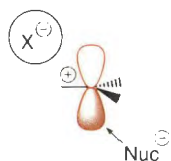
More nucleophilic attack from one face of the carbocation in an ion pair
