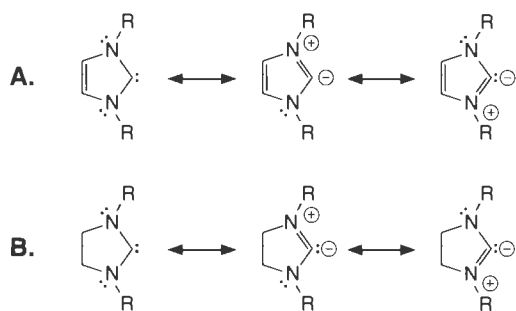
Stable carbenes
