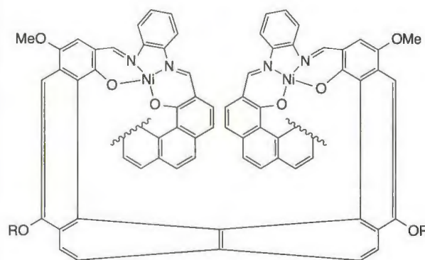
[6]Helicene
