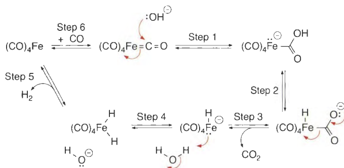
Figure 12.14 Catalytic cycle for the water-gas shift reaction.
