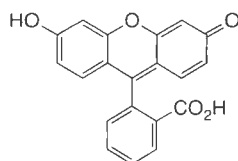
Fluorescein
