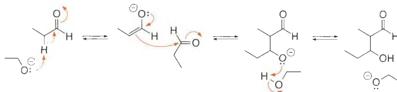
Scheme 11.4 The electron-pushing scheme for the aldol reaction.
