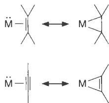
Alternative bonding schemes
