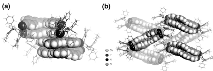
Fig. 11.14 a Supramolecular dimer observed in single crystals of metallacycle 31a 1 ; b organization of the neighboring metallacycles in the single crystals of supramolecular assembly 32a 1
