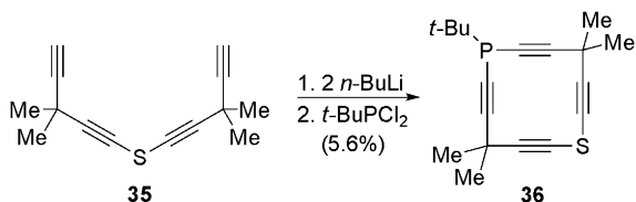
Fig. 2.12 Phosphathio[4]pericycline 36
