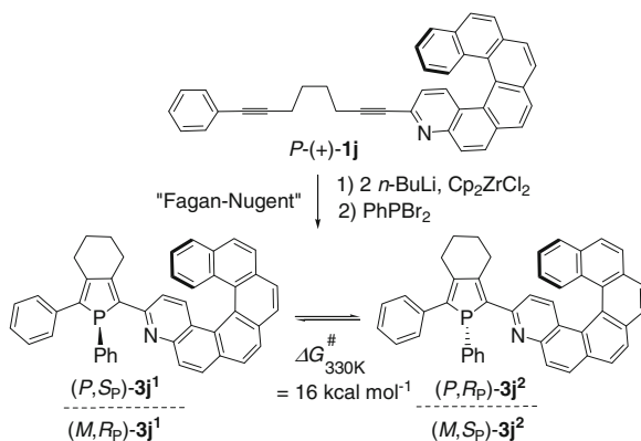
Scheme 11.2 Synthesis of (P,S_p)\text{-}3j^1 and (P,R_p)\text{-}3j^2 diastereomers from one diyne P-1j enantiomer
