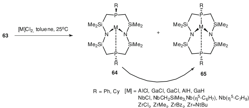
Scheme 12.24 Synthesis of complexes of the macrocycle 63
