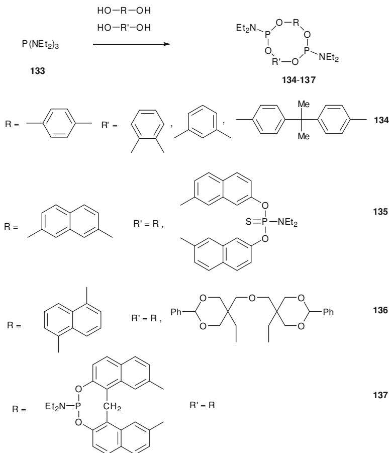
Scheme 12.52 Covalent self-assembly of macrocyclic phosphites 134–137
