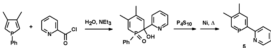
Scheme 6.4 Synthesis of phosphinines via ring-expansion
