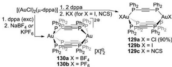
Fig. 2.52 Formation of gold-dppa cages 129 and 130
