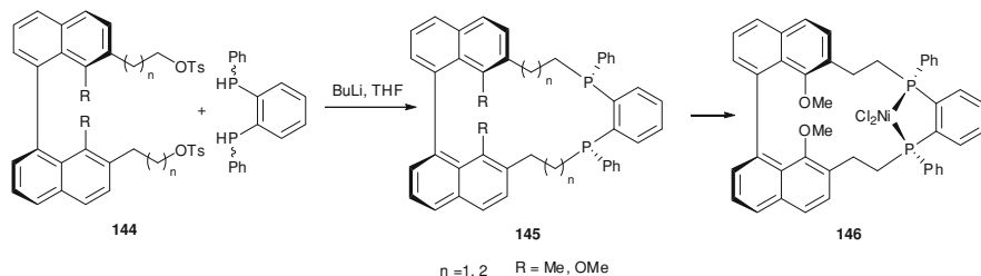
Scheme 12.54 Synthesis under high-dilution conditions of binaphthyl-based macrocyclic diphosphines 145
