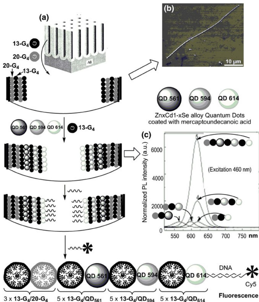
Fig. 9.20 a Functionalization of alumina template by LbL deposition of charged dendrimers; b nanotubes of dendrimers obtained after removal of the template; c nanotubes including one, two, or three types of quantum dots c and their use for the detection of trace amounts of DNA
