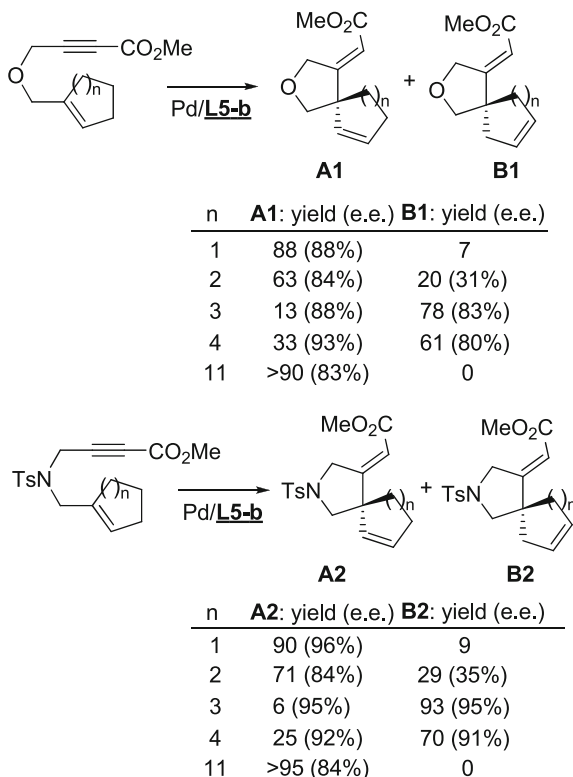
Fig. 10.8 Ene-type spiro-cyclization of 1,6-enyne ethers and tosylamides promoted by the palladium-phosphino-oxazoline complexes L5-b (see Fig. 10.7) [22, 23]
