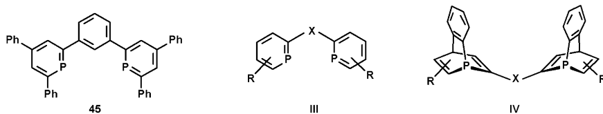
Fig. 6.18 Di-phosphinines and phosphabarrelenes
