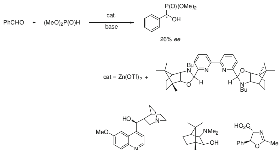
Scheme 8.66 Zn-catalyzed hydrophosphorylation of benzaldehyde
