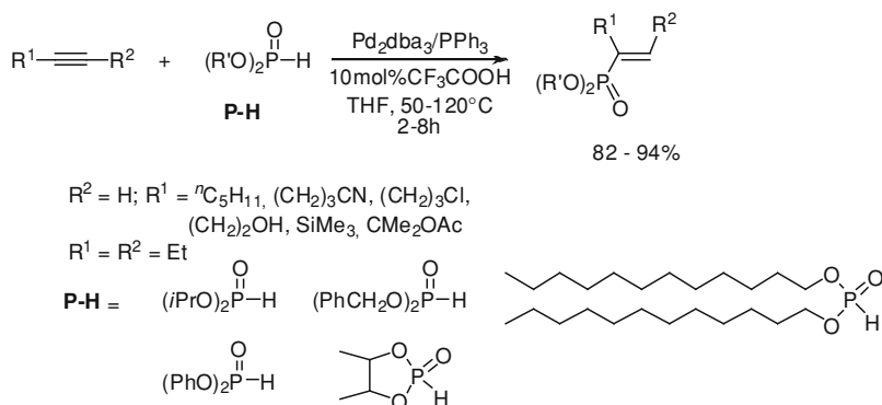
Scheme 8.14 Regioselective hydrophosphorylation of alkynes using [Pd]/CF 3 COOH system
