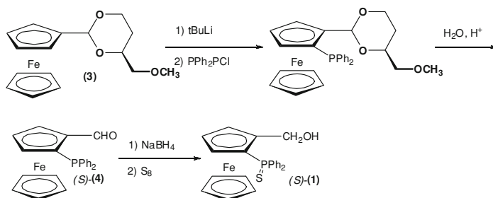
Scheme 5.2 Synthesis of the enantiomerically pure ( S )- 1 via Kagan's acetal
