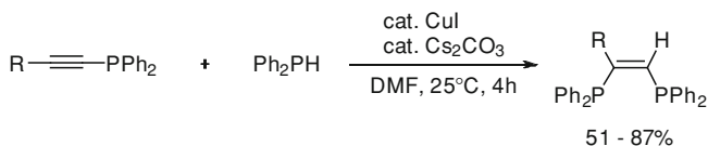
Scheme 8.60 Cu-catalyzed hydrophosphination of 1-alkynylphosphines
