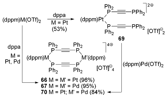
Fig. 2.24 Synthesis of dppm-ligated macrocycles 66 , 67 and 70
