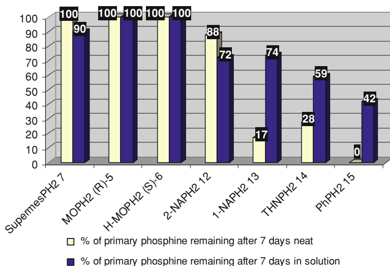
Fig. 1.6 The 7 day neat (left bar) and d -chloroform solution (right bar) oxidation profiles of selected primary phosphines; increasing \pi -conjugation stabilizes the -PH_2 group to air-oxidation
