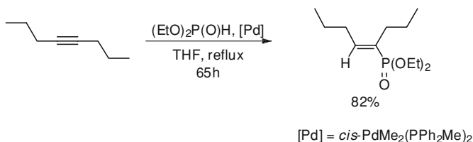
Scheme 8.4 Pd-catalyzed hydrophosphorylation of 4-octyne
