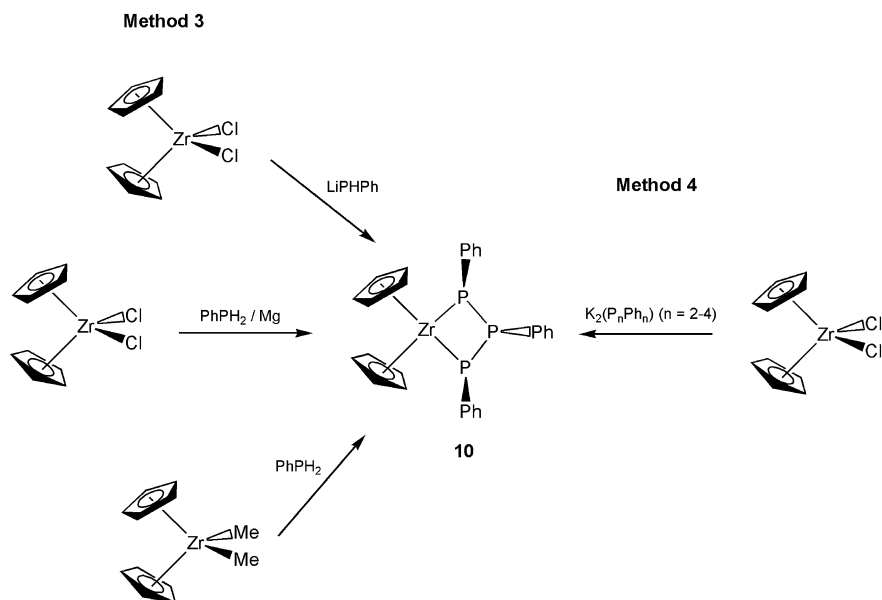
Fig. 4.3 Synthesis of [\text{Zr}(\eta^5\text{-C}_5\text{H}_5)_2(\text{P}_3\text{Ph}_3)] ( 10 ) by methods 3 and 4
