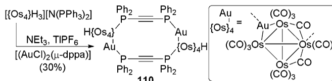
Fig. 2.41 Two \text{Os}_4\text{Au} clusters ( 110 ) doubly bridged by dppe
