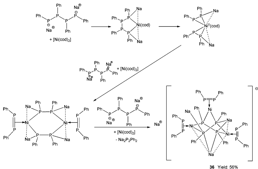
Fig. 4.15 Proposed mechanism for the formation of [\text{Na}(\text{Et}_2\text{O})_3][\text{Na}_3(\text{Et}_2\text{O})_2\text{Ni}_3(\mu\text{-P}_2\text{Ph}_2)_2(\eta^2\text{-P}_2\text{Ph}_2)_3] ( 36 )
