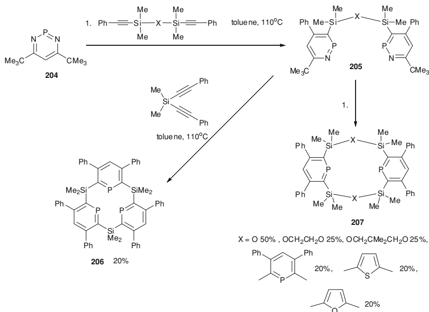
Scheme 12.69 Synthesis of cyclophanes 206 – 207 with phosphinine units incorporated into the macrocyclic framework
