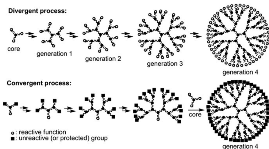
Fig. 9.1 Illustration of the divergent and convergent processes, both usable for the synthesis of dendrimers
