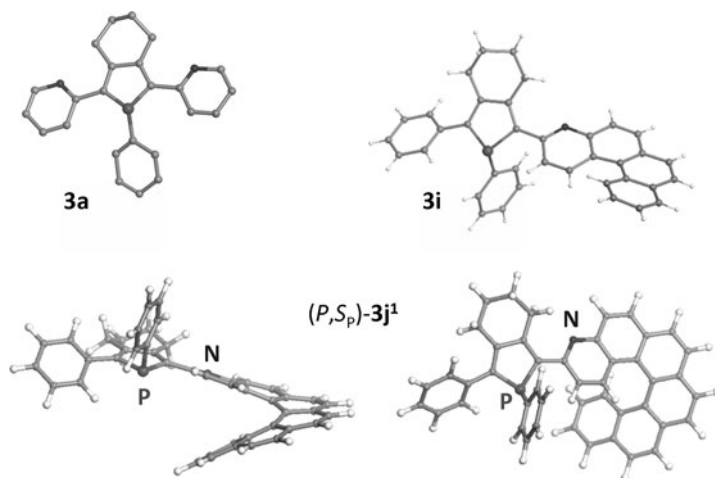
Fig. 11.4 X-ray structures of phospholes 3a,i,j
