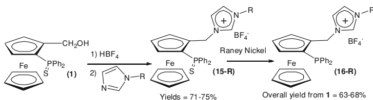
Scheme 5.10 Synthesis of phosphine- N -heterocyclic carbene ligand precursors
