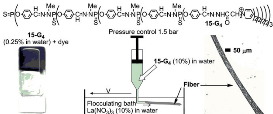
Fig. 9.14 Hydrogels and fibers obtained from pyridinium-ended dendrimers 15-G n
