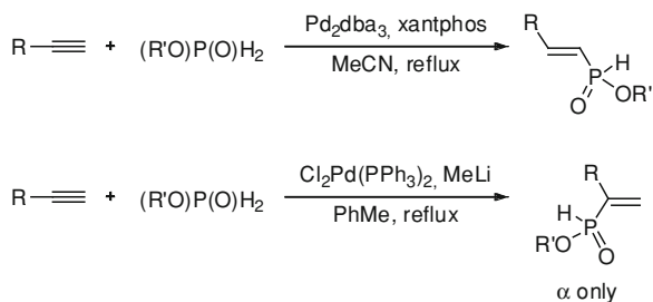
Scheme 8.37 Pd-catalyzed addition of phosphinates to terminal alkynes
