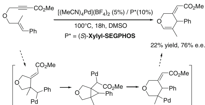
Fig. 10.12 Enantioselective formation of a tetrahydropyran ring from a 1,6-enyne, promoted by a Pd-Xylyl-SEGPPOS catalyst [24]
