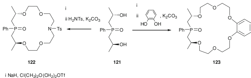
Scheme 12.47 Synthesis of chiral P,O,N- and P,O-containing macrocycles 122 and 123
