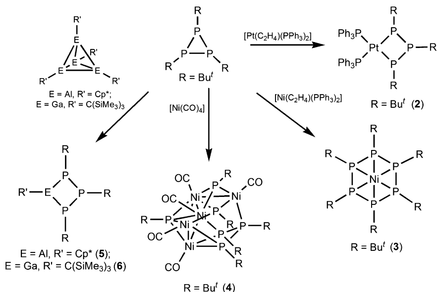
Fig. 4.1 Method 1 for the preparation of metal oligophosphanides
