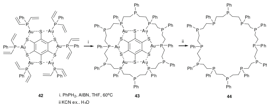
Scheme 12.18 Template synthesis of 36-membered macrocycle 44
