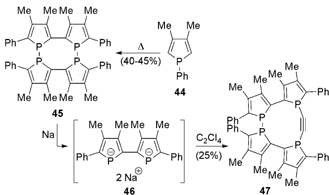
Fig. 2.16 Synthesis of phosphole-based acetylenic macrocycle 47
