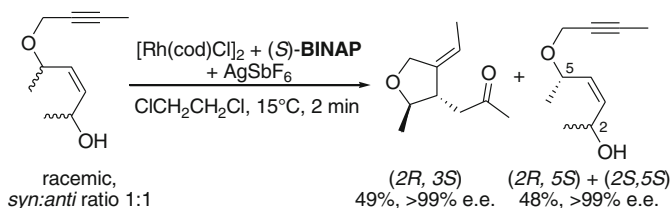
Fig. 10.19 Kinetic resolution of an enyne with stereogenic carbons at the allylic positions [32, 33]
