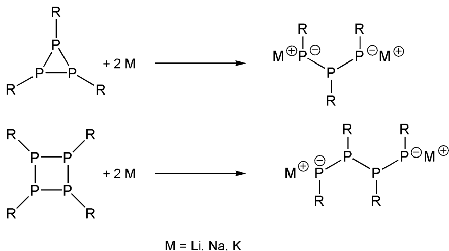
Fig. 4.6 General scheme for the preparation of linear (\text{P}_3\text{R}_3)^{2-} and (\text{P}_4\text{R}_4)^{2-} ions
