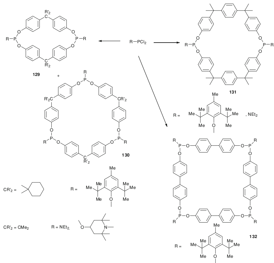
Scheme 12.51 Covalent self-assembly of macrocyclic phosphites 130–132
