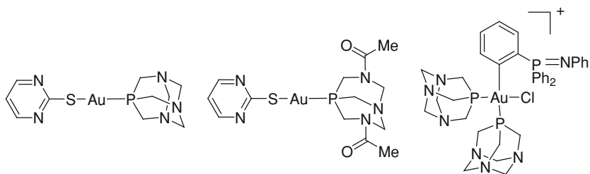
Fig. 13.18 Examples of PTA based Au complexes
