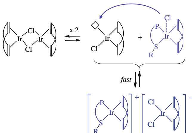
Scheme 5.13 Coordination equilibria of iridium complex 7-Ph in solution
