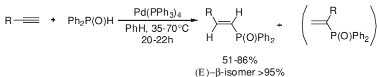
Scheme 8.24 Pd-catalyzed hydrophosphinylation of terminal alkynes
