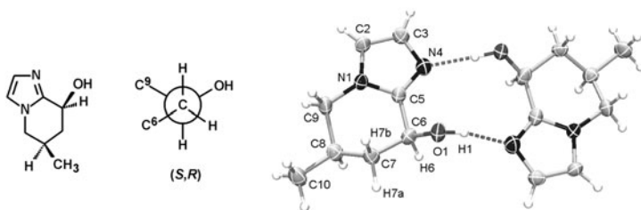
Fig. 6.16 Hydroxy-functionalized bicyclic imidazole and molecular structure in the crystal
