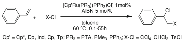
Scheme 7.14 Ru-catalyzed Kharasch addition of chloro substrates to styrene
