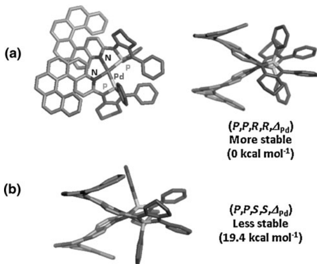
Fig. 11.7 Optimized structures and relative energies for 7j ( [\text{Pd}(\mathbf{3j}^1)_2]^{2+} (a) and [\text{Pd}(\mathbf{3j}^2)_2]^{2+} (b)) by DFT calculations
