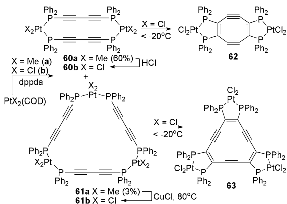
Fig. 2.23 Exploded platinacycles 60 and 61 and their rearranged products
