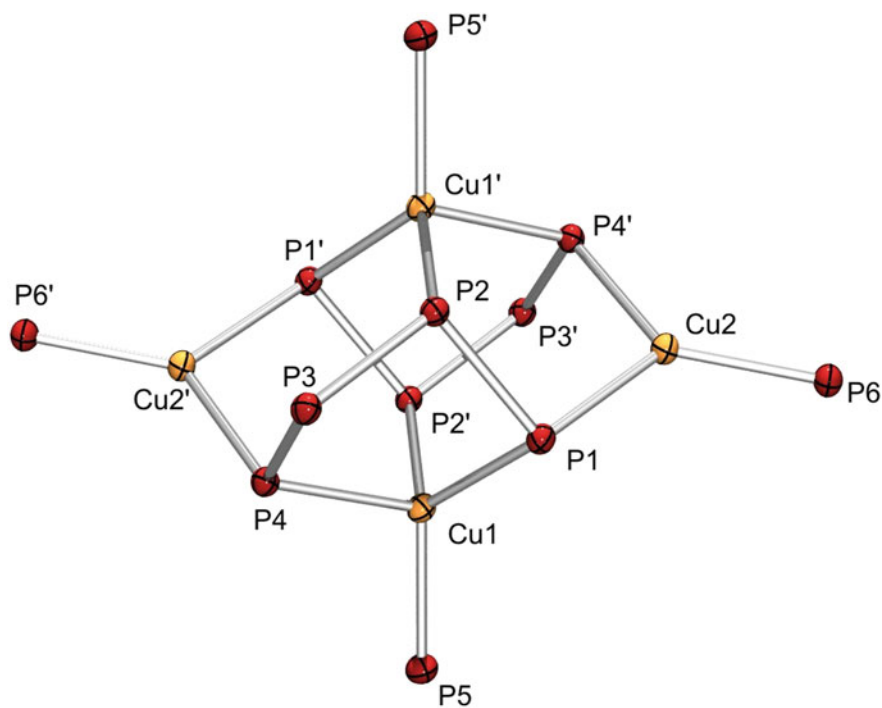
Fig. 4.11 Cu 4 P 12 core structure of [Cu 4 (P 4 Ph 4 ) 2 (PH 2 Ph) 2 (PCyp 3 ) 2 ] ( 29 )
