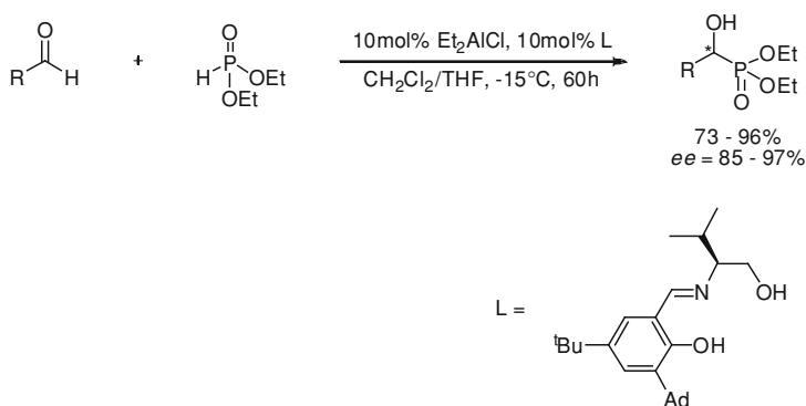
Scheme 8.74 Hydrophosphonylation of aldehydes using [Al]/Schiff base catalytic system
