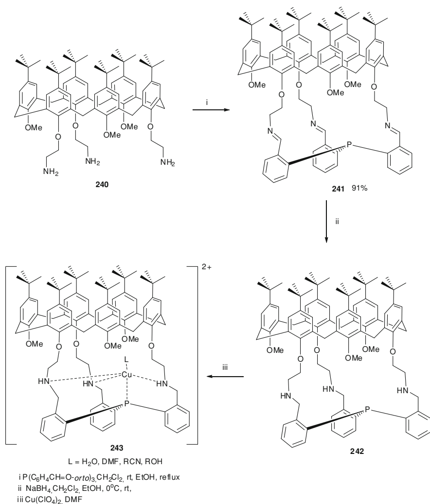
Scheme 12.85 Synthesis of \text{PN}_3 -calix[6]cryptands 241–242 and copper complexes 243
