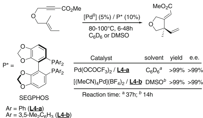
Fig. 10.5 Mikami's catalysts for the enantioselective ene-type cycloisomerizations of a 1,6-enyne [20]
