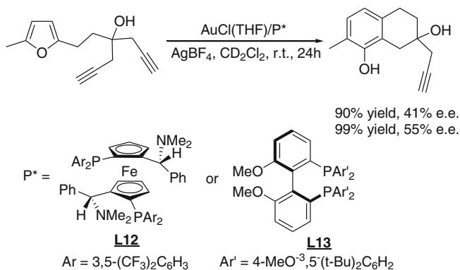
Fig. 10.53 Enantioselective cycloisomerization of prochiral en-diynes [71]
