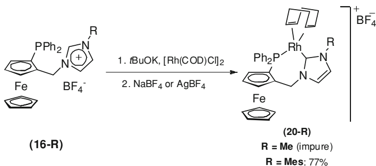
Scheme 5.12 Synthesis of phosphine-carbene rhodium complexes
