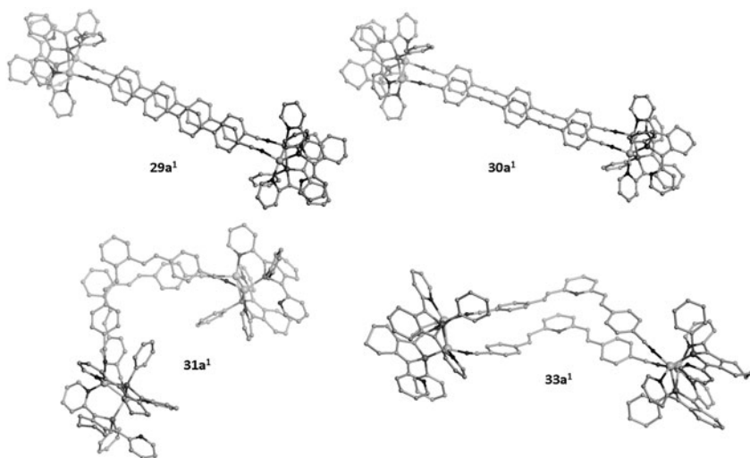
Fig. 11.11 X-ray molecular structures of the tetracationic assemblies 29a 1 –31a 1 and 33a 1 (H atoms, counteranions and solvents have been omitted for clarity)
