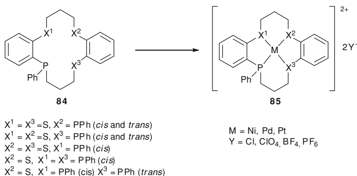
Scheme 12.33 Transition metal complexes 85 of 14-membered P,S-containing macrocyclic ligands 84
