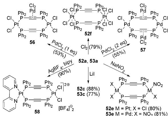
Fig. 2.22 Modifications of platinacycle 52a and palladacycle 53a
