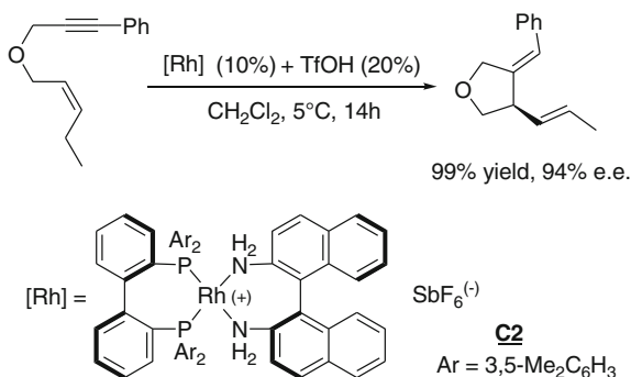
Fig. 10.28 Enantioselective ene-type cyclizations promoted by tropos Rh complexes of the conformationally flexible Xylyl-BIPHEP ligand [42]
