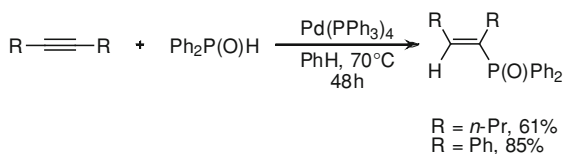
Scheme 8.26 Pd-catalyzed hydrophosphinylation of internal alkynes
