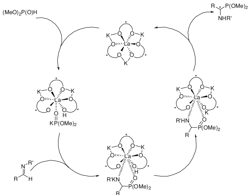
Scheme 8.78 Proposed mechanism of hydrophosphorylation of imines using (R)-LPB catalyst
