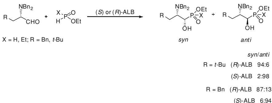
Scheme 8.63 Hydrophosphonylation of chiral \alpha -amino aldehydes using (ALB) catalyst
