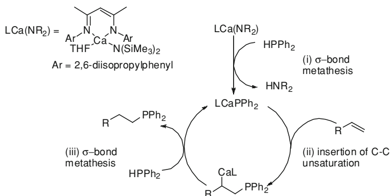
Scheme 8.48 Proposed mechanism of Ca-catalyzed hydrophosphination of alkenes
