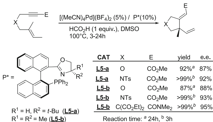
Fig. 10.7 Ene-type isomerizations of 1,6-enynes promoted by a phosphine–oxazoline palladium complex [21]
