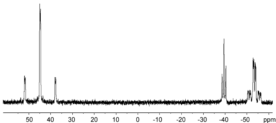
Fig. 4.20 ^{31}\text{P}\{^1\text{H}\} NMR spectrum of [\text{Pt}(\text{P}_4\text{Mes}_4)(\text{dppe})] ( 39 )
