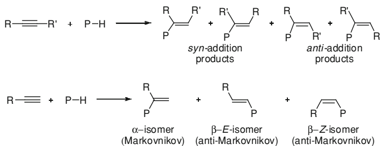
Scheme 8.1 Possible products in a P–H bond addition reaction to alkynes
