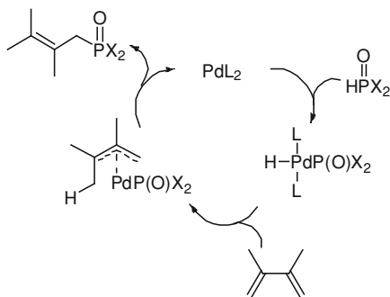
Scheme 8.22 Pd-catalyzed hydrophosphorylation of 1,3-dienes
