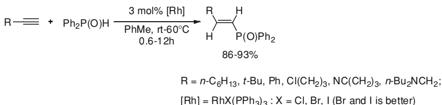
Scheme 8.30 Rh-catalyzed hydrophosphinylation of terminal alkynes
