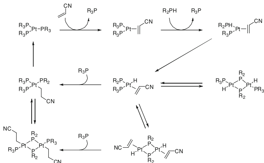
Scheme 8.43 Proposed mechanism of Pt-catalyzed hydrophosphination of acrylonitrile
