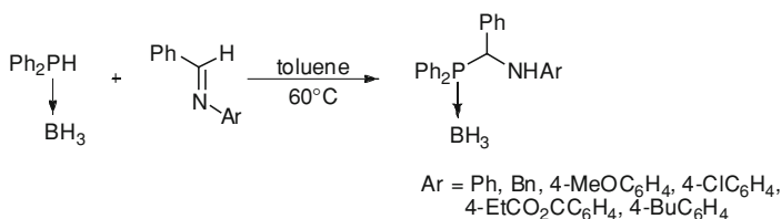
Scheme 8.82 BH 3 -mediated transition-metal-free hydrophosphination of aldehydes and imines
