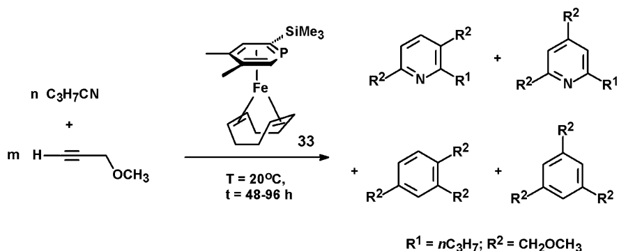
Scheme 6.8 Cyclotrimerization reaction with an \eta^6 -phosphinine-Fe(0) complex
