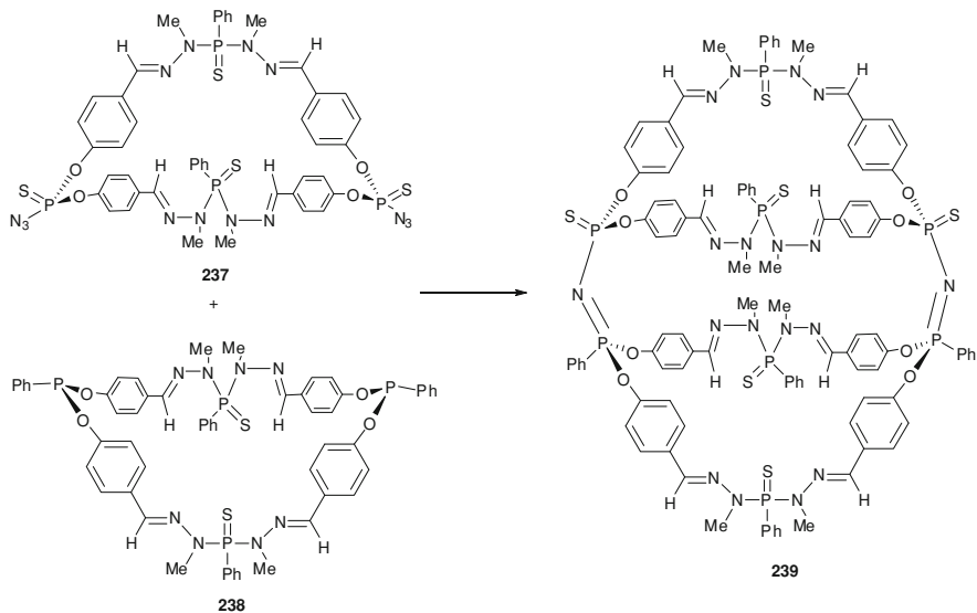
Scheme 12.84 Synthesis of 239
