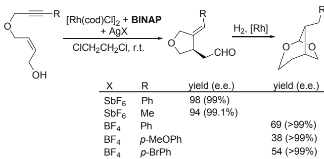
Fig. 10.18 Cycloisomerizations of 1,6-enynes substituted by an OH function at the allylic terminus [29], and subsequent synthesis of bicyclic acetals [31]
