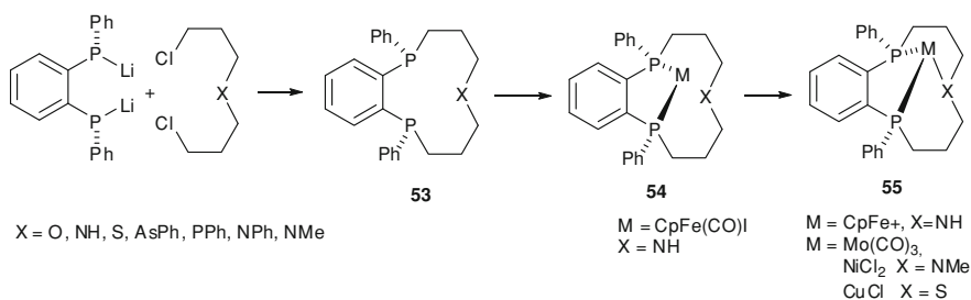
Scheme 12.21 Macrocyclization under high-dilution conditions and formation of transition metal complexes of 11-member macrocycles 53
