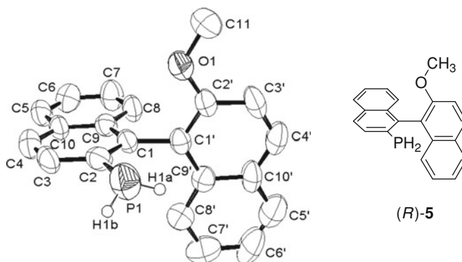
Fig. 1.3 The X-ray crystal structure of ( R )- 5 . Hydrogen atoms attached to carbon are omitted for clarity
