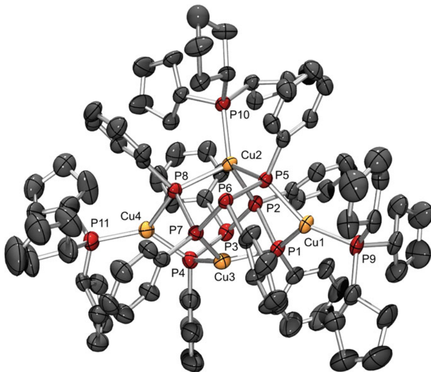
Fig. 4.10 Molecular structure of [\text{Cu}_4(\text{P}_4\text{Ph}_4)_2(\text{PCyp}_3)_3] ( 28 ). Hydrogen atoms are omitted for clarity
