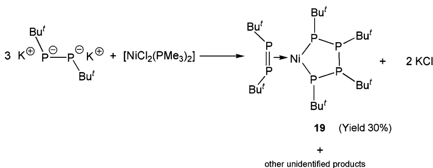
Fig. 4.5 Synthesis of [Ni( \eta^2 -P 2 Bu 2 t )(P 4 Bu 4 t )] ( 19 ) by method 4
