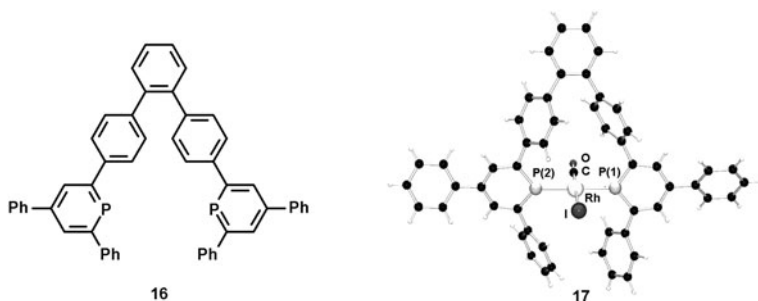
Fig. 6.8 Trans-coordinating di-phosphinine 16 and molecular structure of the corresponding Rh(I) complex 17 in the crystal
