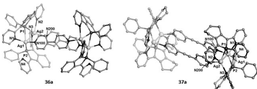
Fig. 11.15 X-ray crystal structures of the tetracationic assemblies 36a and 37a (H atoms, counteranions and solvents have been omitted for clarity)
