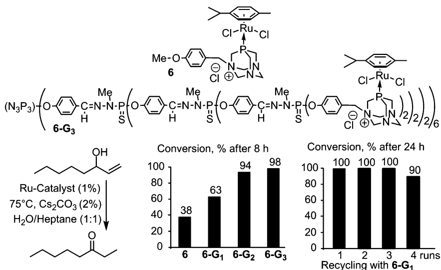
Fig. 9.7 Positive role of the generation and recycling in aqueous media for alcohol isomerisation
