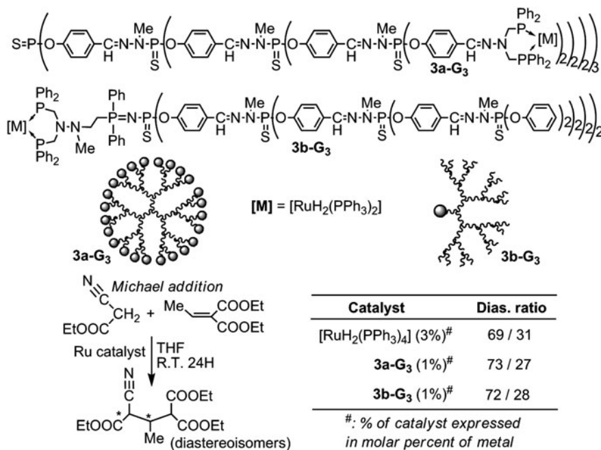
Fig. 9.4 Influence of the location of catalytic site(s) on Michael additions
