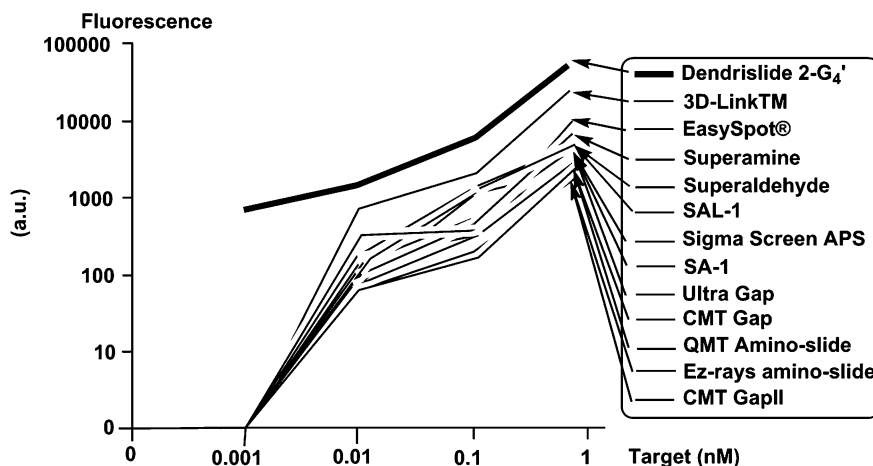
Fig. 9.23 Comparison of the efficiency of dendrislide 2-G 4 ' for the detection of fluorescent DNA complementary strand with twelve commercially available glass slides used as DNA chips
