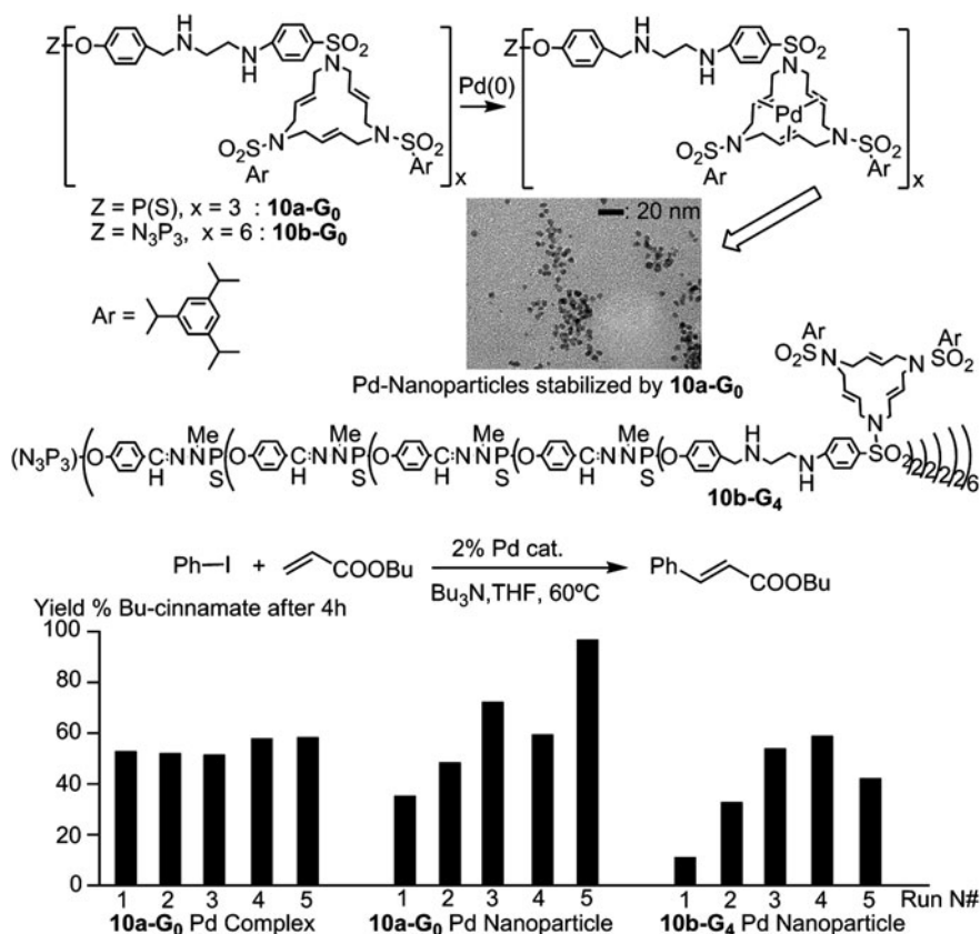
Fig. 9.11 Pd nanoparticles generated by dendrimers 10-G n and used in Mizoroki–Heck reactions
