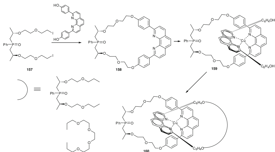
Scheme 12.59 Template synthesis of [2]catenane 160
