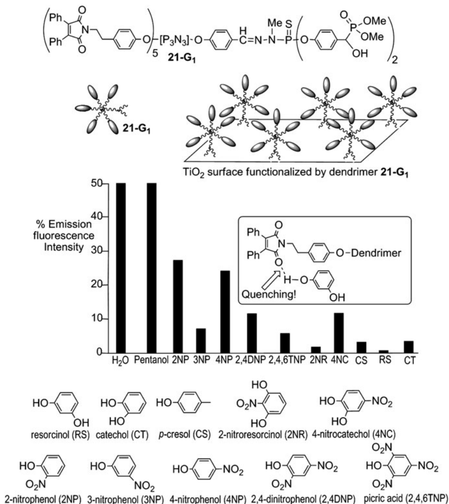
Fig. 9.21 A chemical sensor for phenols, elaborated with the fluorescent dendrimer 21-G 1
