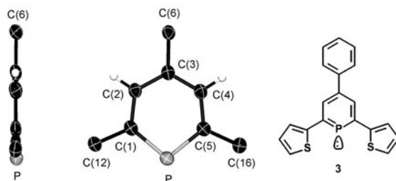
Fig. 6.3 Molecular structure of the bis-thienyl-substituted phosphinine 3 . Only part of the structure is shown. Side-view ( left ), front view ( middle ). Selected bond lengths (Å) and angles (°): P–C(1): 1.749, P–C(5): 1.750, C(1)–C(2): 1.398, C(2)–C(3): 1.394, C(3)–C(4): 1.394, C(4)–C(5): 1.392. C(1)–P–C(5): 101.37
