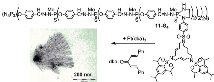
Fig. 9.12 Pt nanoparticles networks induced by the dendrimers 11-G n
