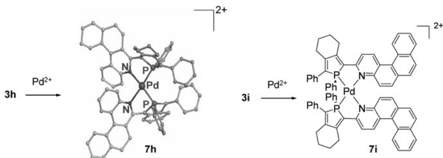
Scheme 11.6 Synthesis of \text{Pd}^{\text{II}} -complexes 7h and 7i from phosphophyl-aza[4]helicenes. View of the X-ray crystal structure of dicationic complex 7h (H atoms, counteranions and solvent molecules have been omitted)
