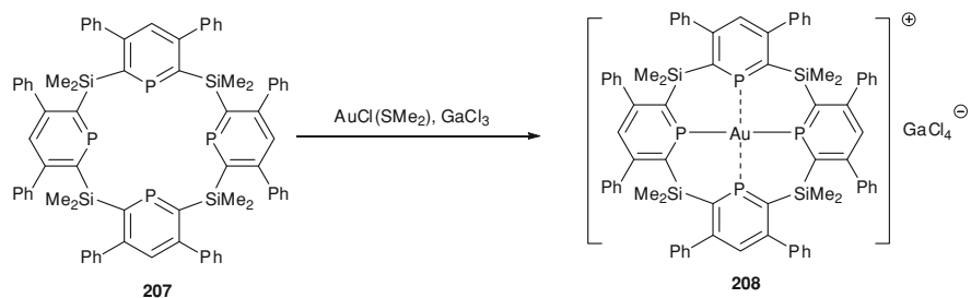
Scheme 12.70 Gold complex 208 of calix[4]phosphinines 207
