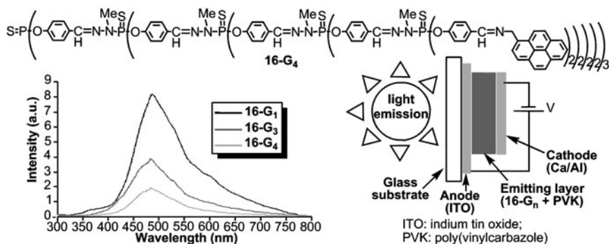
Fig. 9.15 OLEDs elaborated from the fluorescent dendrimers 16-G n . The fluorescence intensity is in arbitrary units, and cannot be compared within generations
