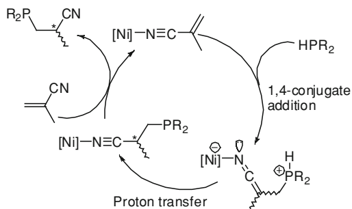
Scheme 8.49 Enantioselective hydrophosphination of methacrylonitrile using [Ni]/Pigiphos
