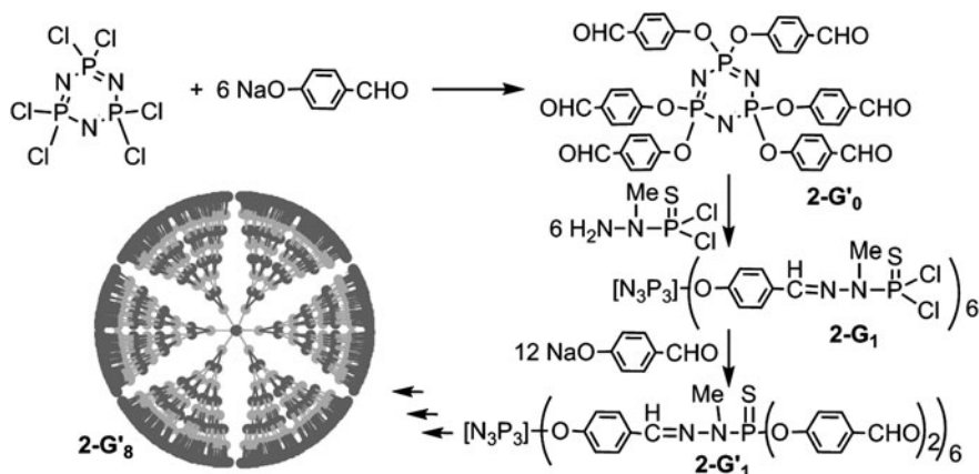
Fig. 9.3 The same method of synthesis as in Fig. 9.2, but applied to the cyclotriphosphazene core
