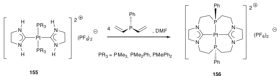
Scheme 12.58 Template synthesis of cyclophane 156
