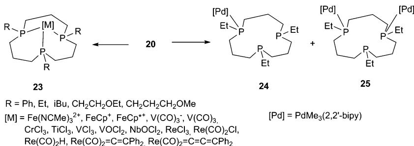
Scheme 12.9 Synthesis of transition metal complexes 23–25 of 12-membered triphosphorus macrocycles 20
