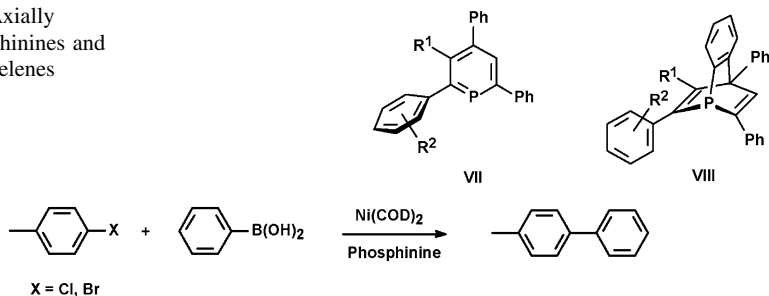
Scheme 6.28 Ni-catalyzed Suzuki–Miyaura reaction using phosphinine ligands
