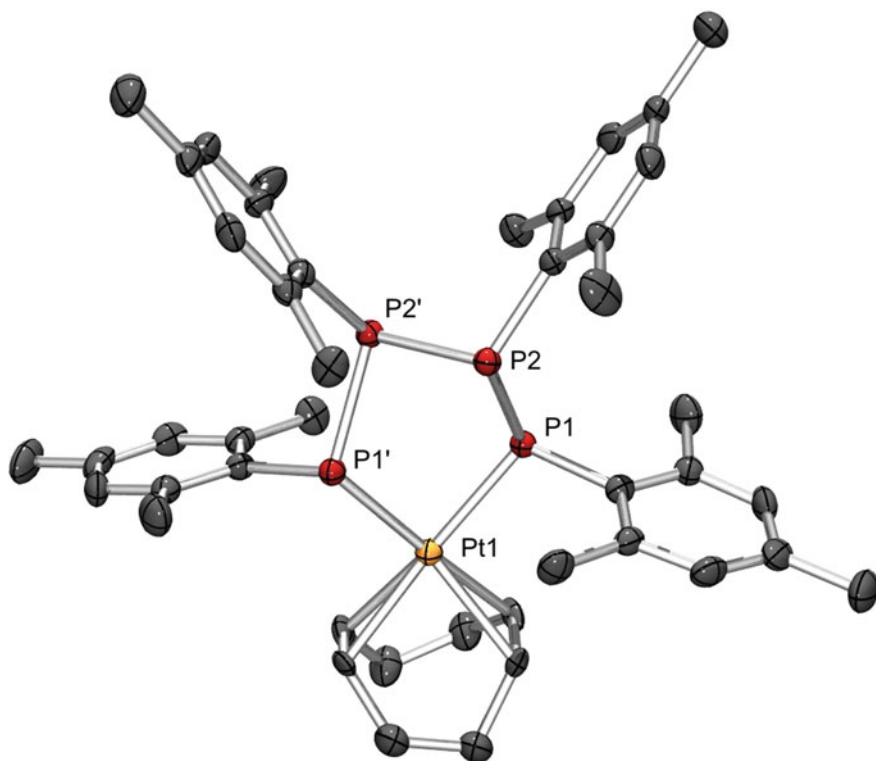
Fig. 4.21 Molecular structure of [\text{Pt}(\text{P}_4\text{Mes}_4)(\text{cod})] ( 38 ). Hydrogen atoms are omitted for clarity
