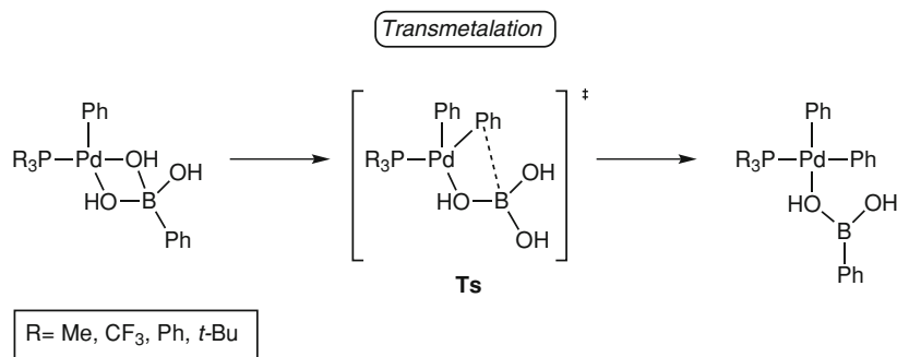
Fig. 3.11 Transmetalation process analyzed by Harvey et al. with different phosphine ligands
