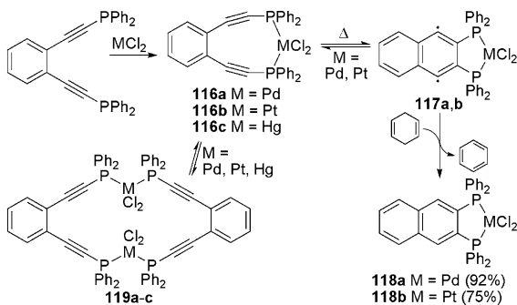
Fig. 2.46 Formation of monomeric ( 116a–c ) and dimeric ( 119a–c ) [MCl 2 ( o -dppeb)] macrocycles and subsequent Bergmann cyclization
