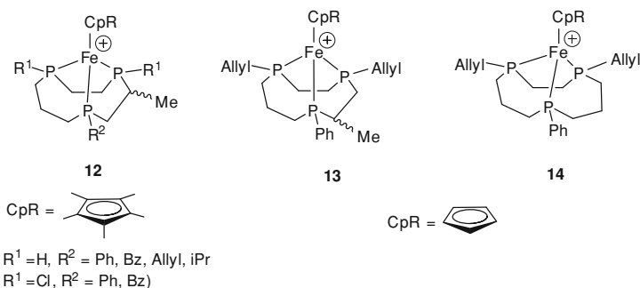
Scheme 12.5 10-Membered cyclic triphosphines 12–14
