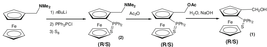
Scheme 5.1 Synthesis of the racemic thiophosphine-alcohol 1
