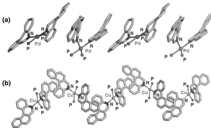
Fig. 11.6 Simplified views of the supramolecular arrangement of complexes 7h (a) and 8h (b)
