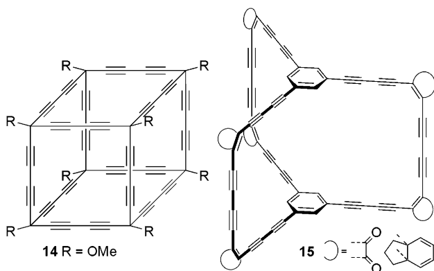
Fig. 2.5 Acetylenic carbon scaffolds
