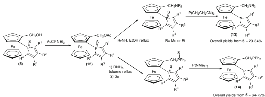
Scheme 5.9 Synthesis of the phosphole-amines 13 and phosphole-phosphines 14
