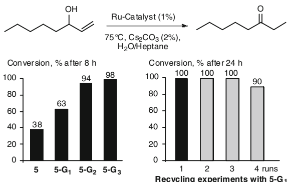
Fig. 7.9 Isomerization of 1-octen-3-ol using monomer 5 and dendrimers 5-G n ( n = 1-3 ) as catalysts (1 mol% based on Ru). On the right: recycling experiments with 5-G 1
