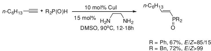
Scheme 8.35 Cu-catalyzed hydrophosphinylation of 1-octyne
