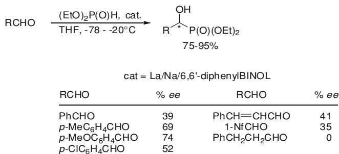
Scheme 8.68 Hydrophosphorylation of aldehydes using LSB catalyst
