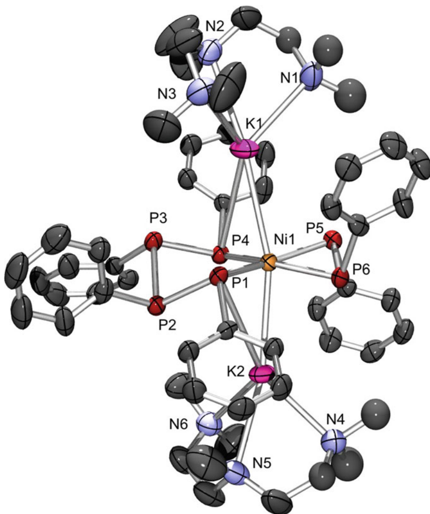
Fig. 4.18 Molecular structure of [\text{K}(\text{pmdeta})]_2[\text{Ni}(\text{P}_4\text{Ph}_4)(\eta^2\text{-P}_2\text{Ph}_2)] ( 37 ). Hydrogen atoms are omitted for clarity
