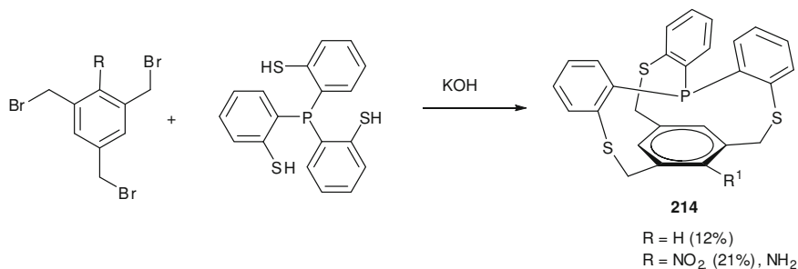
Scheme 12.74 Synthesis under high-dilution conditions of cryptand 214
