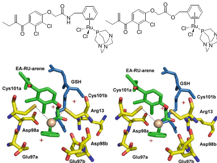
Fig. 13.13 Examples of RAPTA-type complexes containing the ethacrynic acid moiety ( top ) and views of the ruthenium complex at the GST P1-1 dimer interface ( bottom ). The PTA moiety and bonds between the Ru center and the arene ring have been omitted for clarity. Copyright Wiley-VCH Verlag GmbH & Co. KGaA. Reproduced with permission from Ref. [39]
