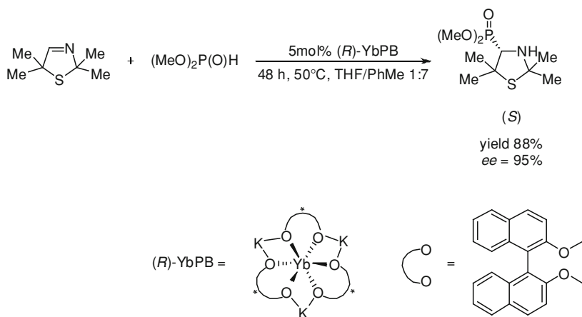
Scheme 8.79 Hydrophosphorylation of cyclic imines using (R)-YbPB catalyst
