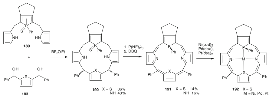
Scheme 12.66 Synthesis of calixpyrroles 190 and core-modified porphyrins 191
