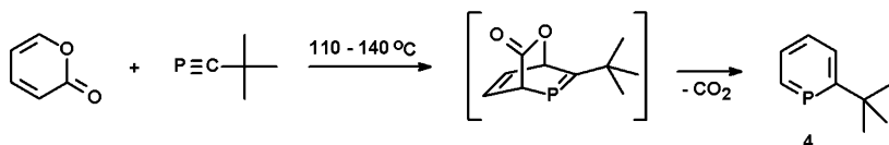
Scheme 6.3 Synthesis of phosphinines from pyrones
