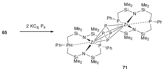
Scheme 12.27 White phosphorus activation by complex 65 containing diamidodiphosphine macrocycle 63
