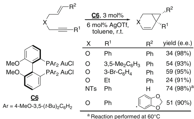
Fig. 10.50 Enantioselective cycloisomerizations of 1,6-enynes into bicyclo[4.1.0]heptenes promoted by gold-diphosphine complexes [69]
