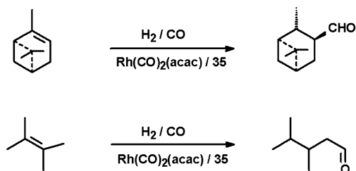
Scheme 6.11 Hydroformylation of substituted (less-reactive) alkenes
