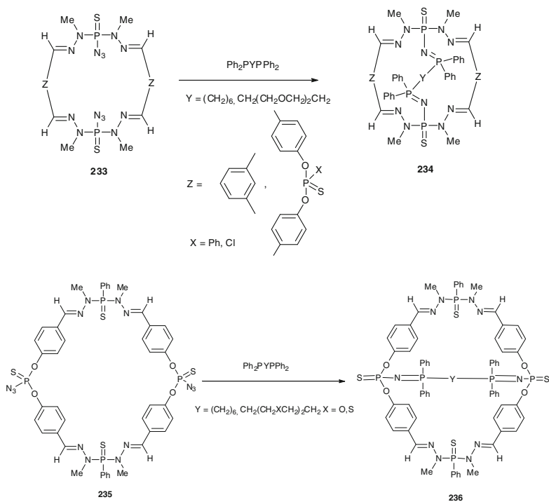
Scheme 12.83 Staudinger reactions of phosphorhydrazone-based macrocycles 233 and 235
