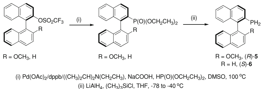
Fig. 1.2 The synthetic route to the chiral primary phosphines ( R )- 5 and ( S )- 6 ; note that the CIP rules determine the ( R ) and ( S ) stereochemistry of 5 and 6 respectively, despite their possession of identical axial configurations
