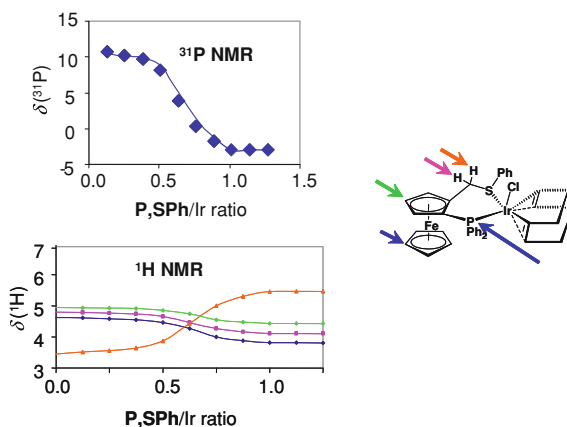
Fig. 5.4 ^{31}\text{P} and ^1\text{H} NMR titration of the addition of 7-Ph to [\text{IrCl}(\text{COD})]_2
