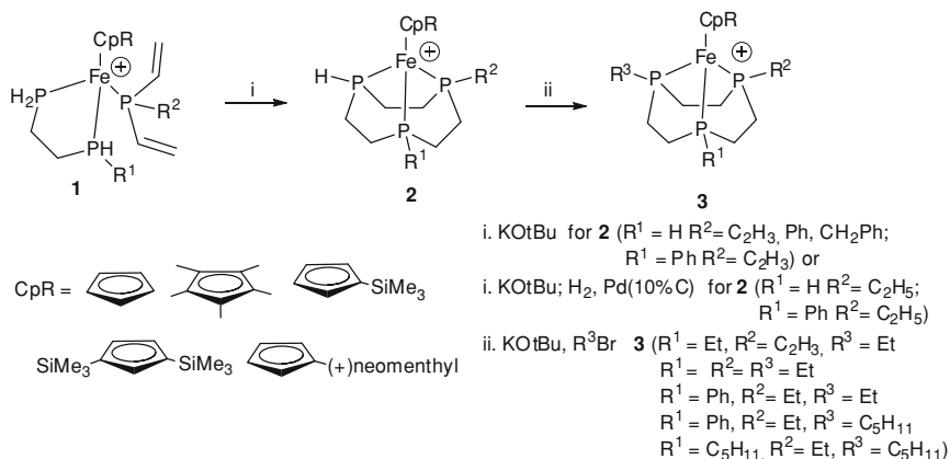
Scheme 12.1 Template synthesis of 1,4,7-triphosphacyclononanes 2 and 3
