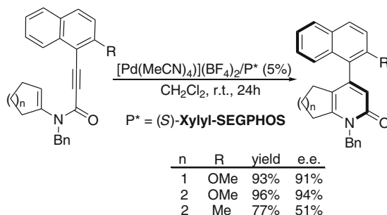
Fig. 10.13 Enantioselective construction of axially chiral compounds by enyne cycloisomerization [25]
