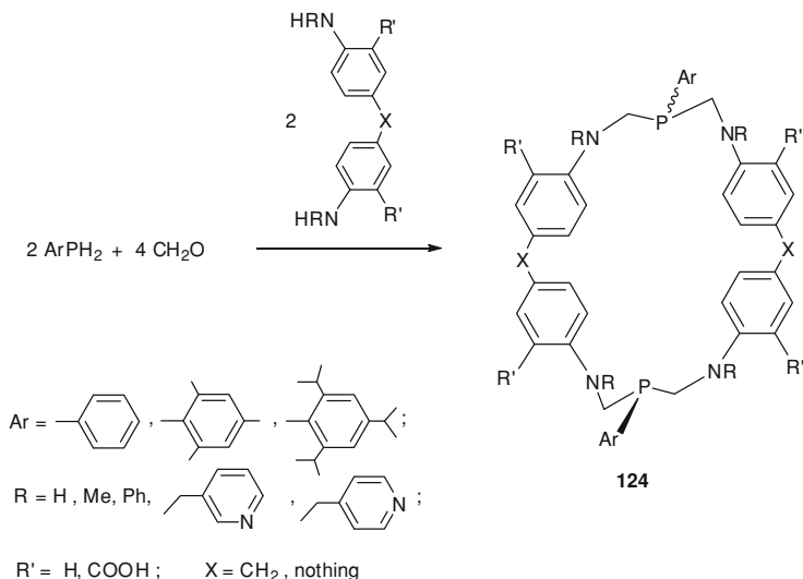
Scheme 12.48 Covalent self-assembly of P,N-containing cyclophanes with aminomethylphosphine backbone 124
