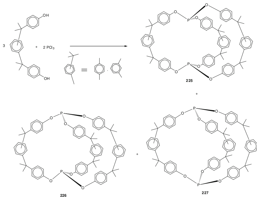
Scheme 12.80 Covalent self-assembly of P,O-cryptands 225–227
