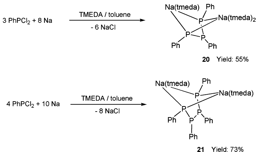
Fig. 4.7 Synthesis of [\text{Na}_2(\text{tmeda})_3(\text{P}_3\text{Ph}_3)] ( 20 ) and [\text{Na}_2(\text{tmeda})_2(\text{P}_4\text{Ph}_4)] ( 21 )
