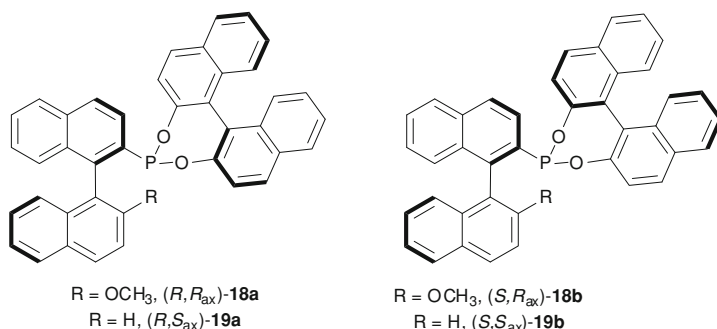
Fig. 1.10 The binol-derived MOP phosphonites prepared from ( R )- 5 and ( S )- 6
