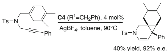
Fig. 10.45 Isomerization of a cyclic 1,6-dien-yne into a tricyclic compound [64]
