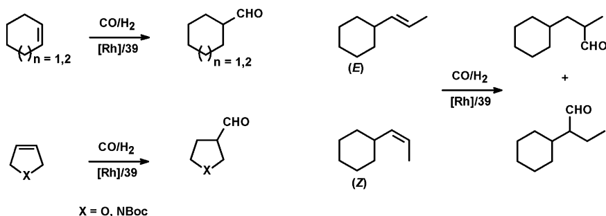
Scheme 6.22 Rh-catalyzed hydroformylation of internal and heterocyclic alkenes
