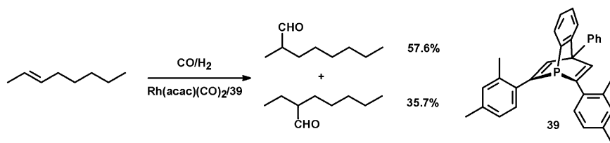
Scheme 6.21 Rh-catalyzed hydroformylation of 2-octene
