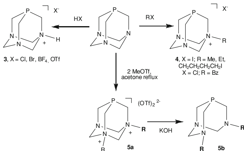
Scheme 7.2 “Lower rim” PTA functionalizations
