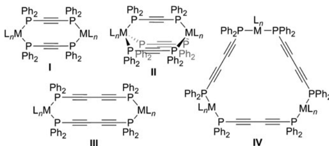
Fig. 2.1 Phosphine acetylenic macrocycles assembled through metal coordination
