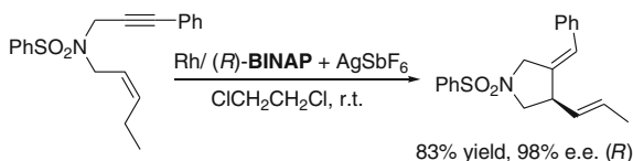
Fig. 10.17 Rh-BINAP promoted Alder-ene cycloisomerization of a sulfonamide tethered enyne [30]
