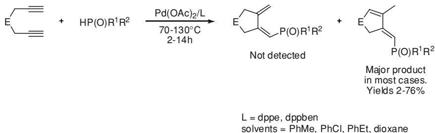
Scheme 8.36 Pd-catalyzed carbocyclization of \alpha,\omega -diynes
