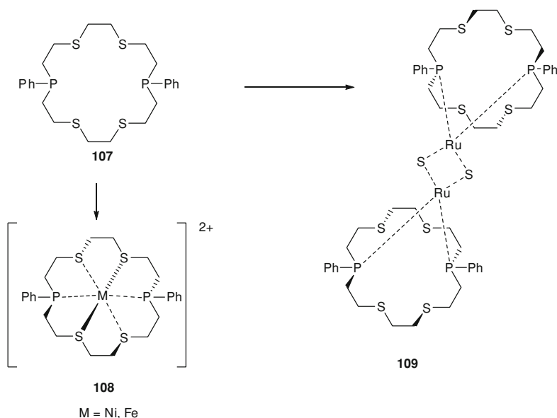
Scheme 12.43 Transition metal complexes 108–109 of 18-membered P,S-containing macrocyclic ligand 107
