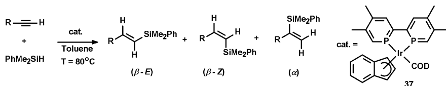
Scheme 6.18 Ir-catalyzed hydrosilylation of alkynes
