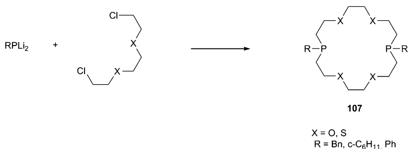
Scheme 12.42 Synthesis under high-dilution conditions of 18-membered P,S- and P,O-containing macrocycles 107
