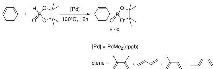
Scheme 8.22 Pd-catalyzed hydrophosphorylation of 1,3-dienes
