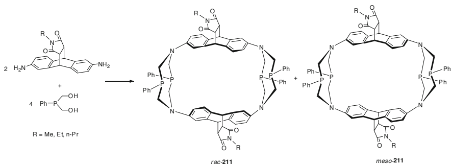
Scheme 12.72 Covalent self-assembly of cyclophanes 211 with chiral intramolecular cavity
