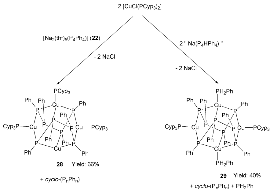
Fig. 4.9 Synthesis of [\text{Cu}_4(\text{P}_4\text{Ph}_4)_2(\text{PCyp}_3)_3] ( 28 ) and [\text{Cu}_4(\text{P}_4\text{Ph}_4)_2(\text{PH}_2\text{Ph})_2(\text{PCyp}_3)_2] ( 29 )
