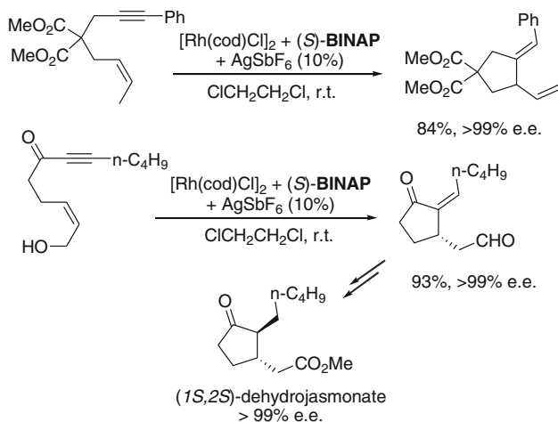
Fig. 10.23 Synthesis of cyclopentanes and cyclopentanones by Rh-promoted cycloisomerizations of 1,6-enynes [35]
