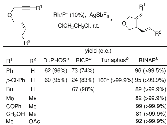
Fig. 10.16 Enantioselective synthesis of functionalized tetrahydrofurans by rhodium promoted Alder-ene type rearrangements of 1,6-enynes [28, 29]
