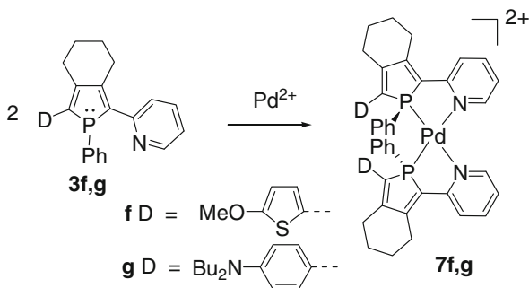
Scheme 11.5 Stereoselective synthesis of NLO-active complexes 7f,g
