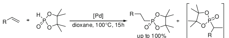
Scheme 8.14 Regioselective hydrophosphorylation of alkynes using [Pd]/CF 3 COOH system
