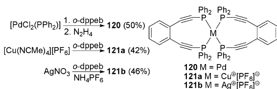
Fig. 2.47 d 10 Metal centers chelated by two o -dppeb moieties ( 120–121 )
