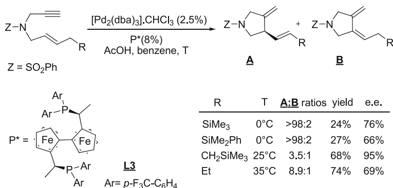
Fig. 10.4 Representative enyne-type isomerizations promoted by TRAP–palladium complexes [19]
