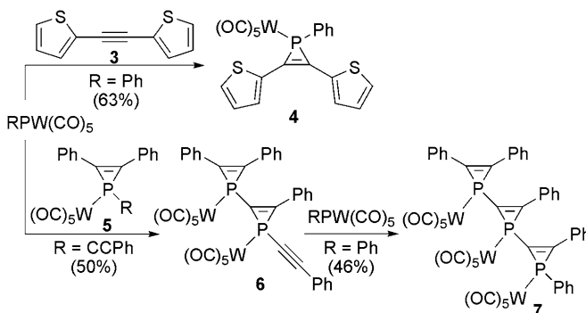
Fig. 2.3 P/C rings ( 4 , 6 , 7 ) obtained from phosphinidene addition to CC triple bonds
