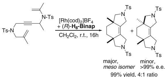
Fig. 10.36 Enantioselective cycloisomerization of dien-yne into tricyclic cyclohexenes [49]
