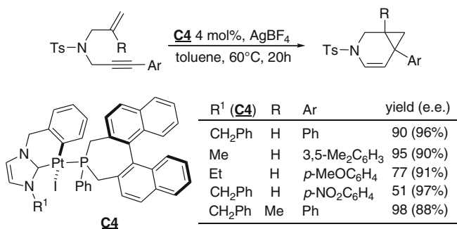
Fig. 10.44 Enantioselective cycloisomerizations of 1,6-enynes into bicyclo[4.1.0]heptenes promoted by platinumacyclic ( S )-Binerphos complexes [64]
