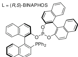
Scheme 8.17 Pd-catalyzed hydrophosphorylation of styrenes with ( R,S )-BINAPHOS as ligand
