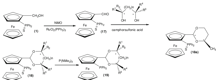
Scheme 5.11 Synthesis of phosphine-acetal ligands
