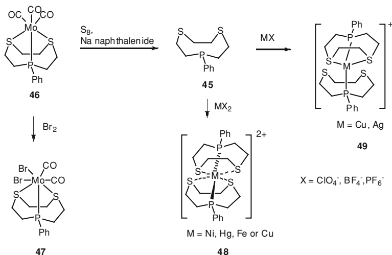
Scheme 12.19 Transition metal complexes 46–49 of 9-membered hybrid P,S,S-macrocycle 45
