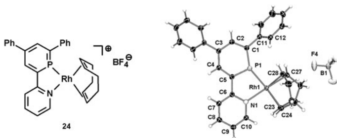
Fig. 6.11 Rh(I) complex containing a phosphinine derivative of 2,2'-bipyridine and the molecular structure of 24 in the crystal
