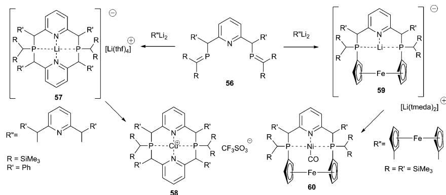
Scheme 12.22 Template synthesis of macrocyclic complexes 58 and 60
