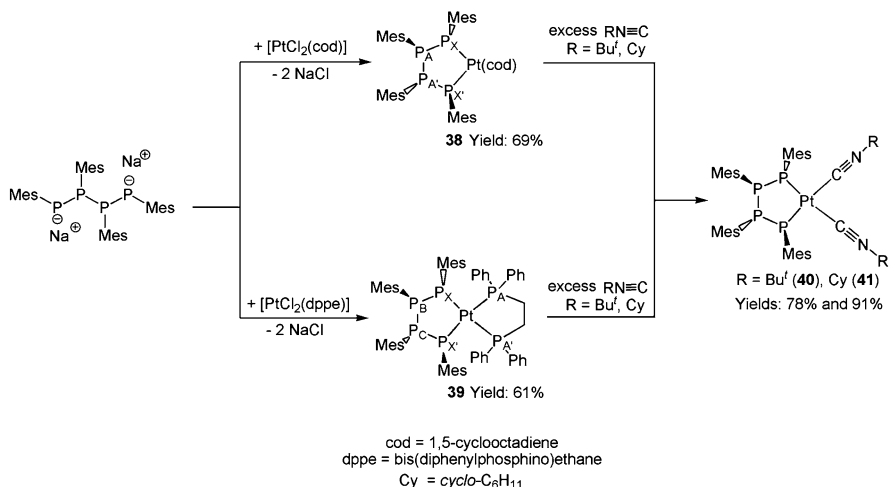
Fig. 4.19 Synthesis of platinum(II) complexes 38–41
