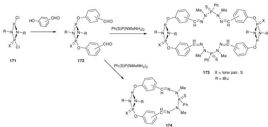
Scheme 12.62 Synthesis of cyclophanes containing 1,3-diaza-2,4-diphosphacyclobutane units 173–174
