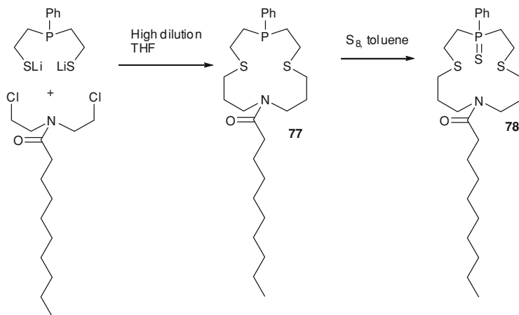
Scheme 12.29 Synthesis under high-dilution conditions of 14-membered P,S,N-containing macrocyclic ligand 77
