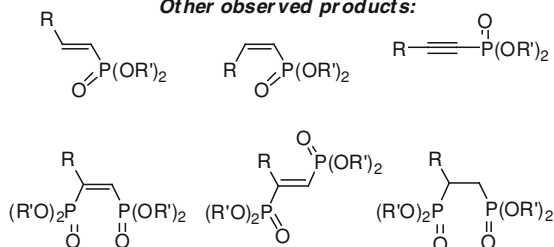
Scheme 8.13 Hydrophosphorylation of alkynes leading to \alpha -isomer and possible by-products
