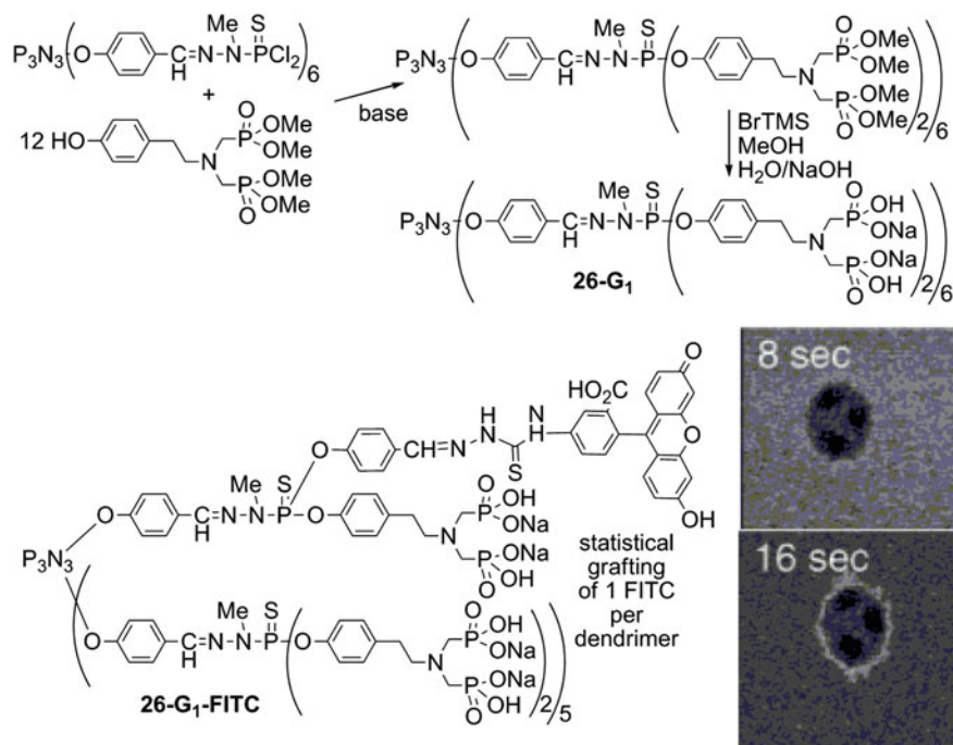
Fig. 9.29 Synthesis of the phosphonic acid salts ended dendrimer 26-G 1 , and use of its fluorescent analogue 26-G 1 -FITC for visualizing the interaction with monocytes
