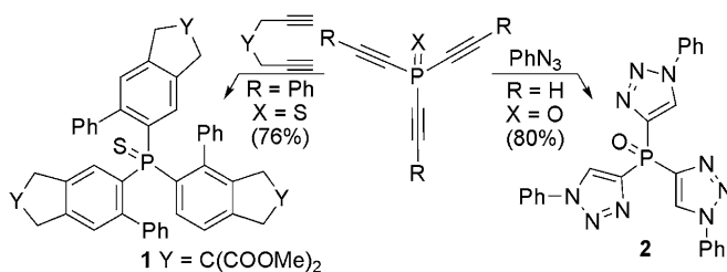
Fig. 2.2 Application of phosphine acetylenes in the construction of bulky arylphosphines ( 1 ) and phosphascorpinates ( 2 )
