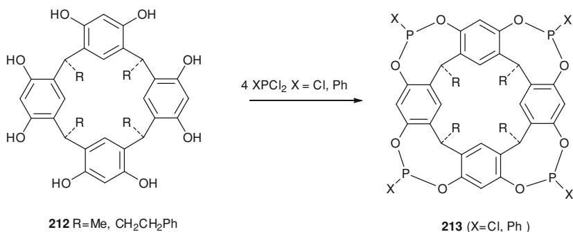
Scheme 12.73 Synthesis of cyclophanes 213 with with eight-membered P-containing rings incorporated into the cyclophane framework
