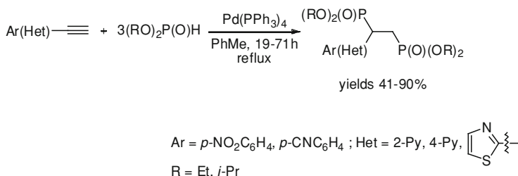
Scheme 8.6 Pd-catalyzed double hydrophosphorylation of aryl(hetaryl) substituted alkynes
