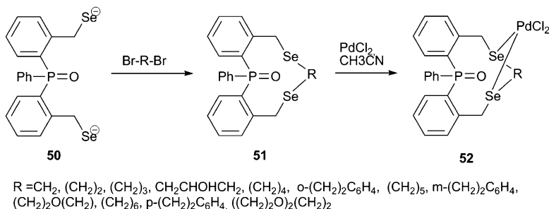
Scheme 12.20 Synthesis and formation of palladium (II) Se, Se-complexes of macrocycles 51
