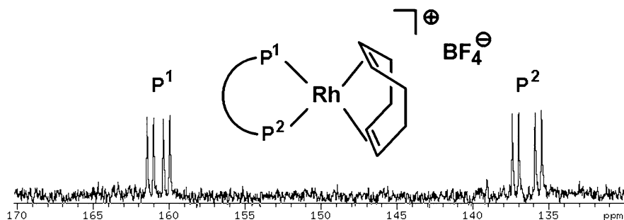
Fig. 6.15 ^{31}\text{P}\{^1\text{H}\} NMR spectrum of complex [(\mathbf{11})\text{Rh}(\text{cod})]\text{BF}_4
