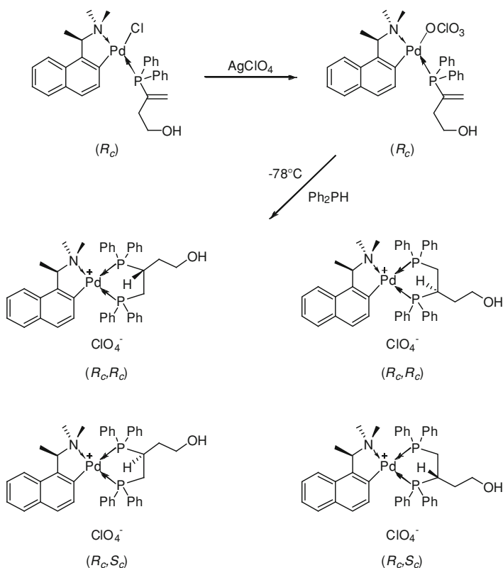
Scheme 8.58 Asymmetric hydrophosphination of diphenylphosphinoalkenols using organo palladium complex
