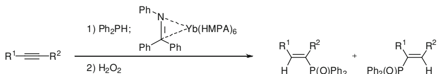
Scheme 8.54 Mechanistic difference in the hydrophosphination reactions using Pd(0)/Ni(0) or PdX 2 /NiX 2 species as catalyst precursors
