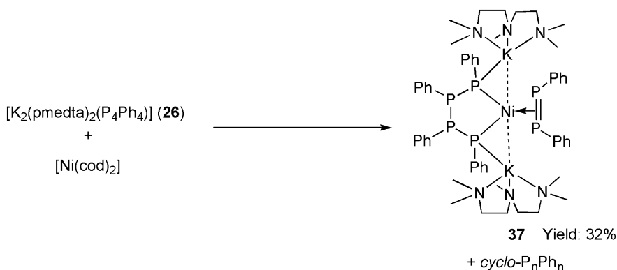
Fig. 4.16 Synthesis of [\text{K}(\text{pmdeta})]_2[\text{Ni}(\text{P}_4\text{Ph}_4)(\eta^2\text{-P}_2\text{Ph}_2)] ( 37 )
