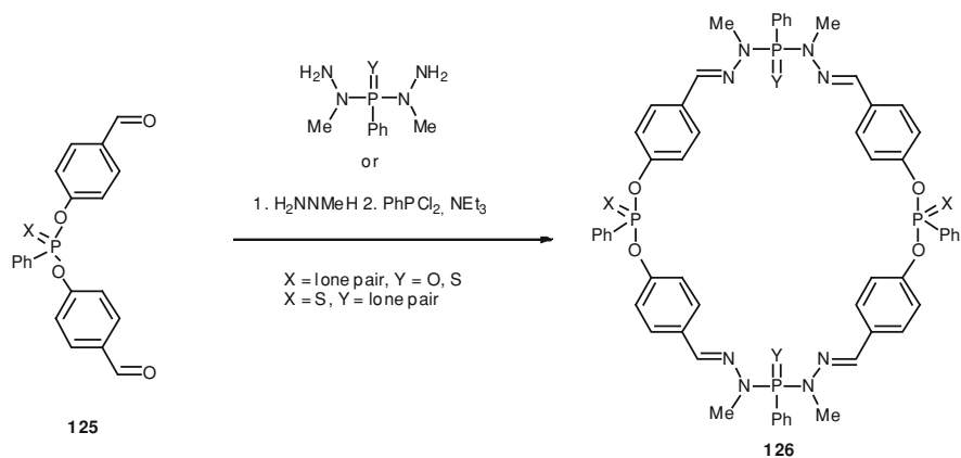
Scheme 12.49 Covalent self-assembly of P,N-containing cyclophanes 126
