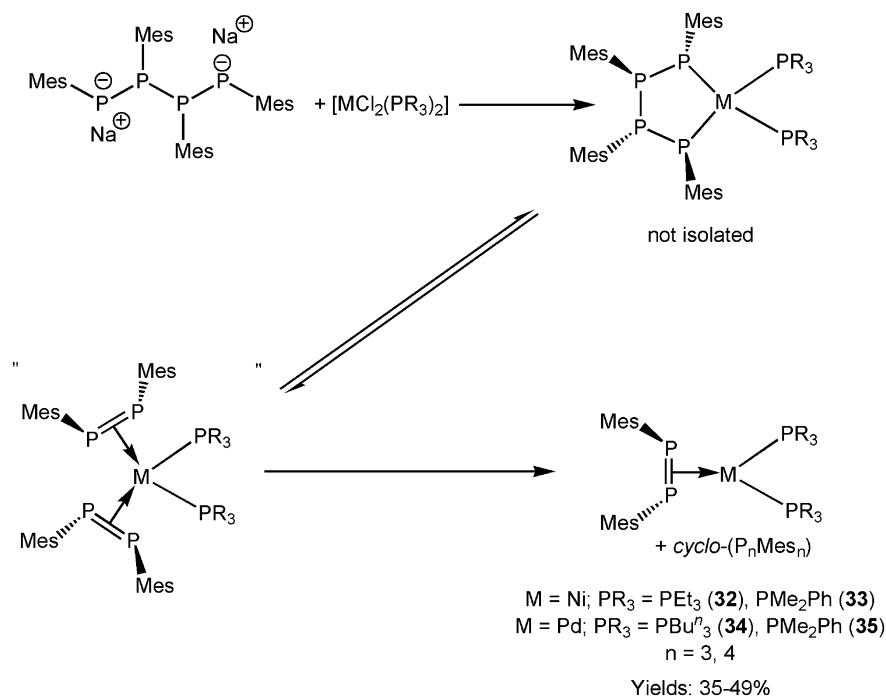
Fig. 4.14 Synthesis of Ni 0 and Pd 0 dimesityldiphosphene complexes 32–35
