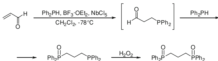
Scheme 8.83 Hydrophosphination of \alpha,\beta -unsaturated carbonyl compounds using NbCl 5 -BF 3 × Et 2 O
