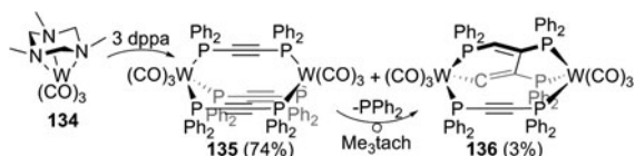
Fig. 2.55 Formation and rearrangement of W-cage 135
