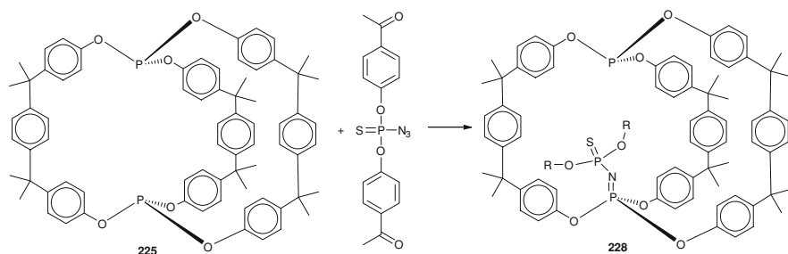
Scheme 12.81 Staudinger reaction of in,in -cryptand 225 with thiophosphorylazide
