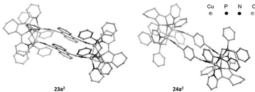
Fig. 11.9 X-ray crystal structures of the tetracationic assemblies 23a^2 and 24a^2 (H atoms, counteranions and solvents have been omitted for clarity)
