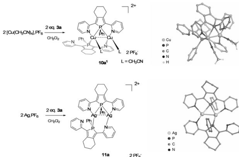
Scheme 11.9 Synthesis and view of the solid-state structure of dicationic complexes 10a 1 and 11a
