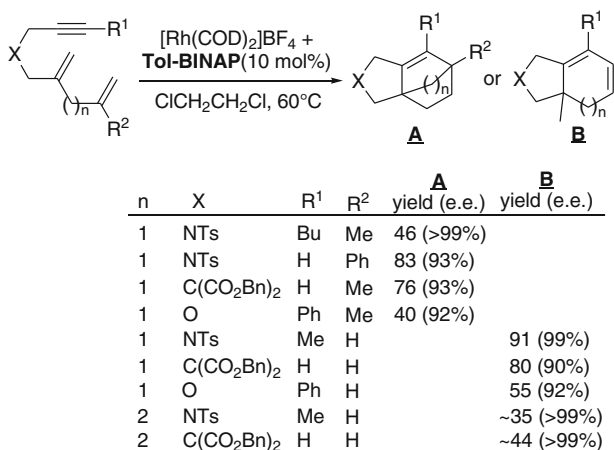
Fig. 10.32 Rhodium-TolBINAP promoted [2 + 2 + 2] annulations of dien-yne [47, 48]
