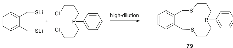
Scheme 12.30 Synthesis under high-dilution conditions of 13-membered P,S-containing macrocyclic ligand 79
