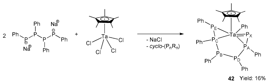
Fig. 4.22 Synthesis of [\text{Ta}(\eta^5\text{-C}_5\text{Me}_5)(\text{Ph})(\text{P}_6\text{Ph}_5)] ( 42 )
