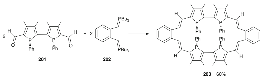
Scheme 12.68 Synthesis of macrocyclic tetraphosphole 203
