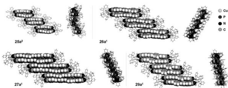
Fig. 11.12 ‘Side’ and ‘lateral’ views of the stacking patterns of \pi -stacked metallocyclophanes 25a 2 –27a 1 and 29a 1 observed in single crystals
