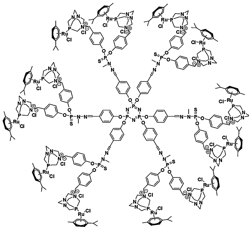
Fig. 7.7 A sketch view of [\text{RuCl}(\text{p-cymene})\text{PTA}] -decorated dendrimer 5-G 1
