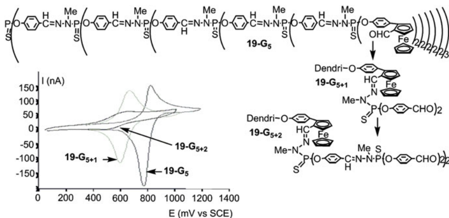
Fig. 9.17 Ferrocenes included at various places inside the structure of dendrimers, able to modify the surface of electrodes, and variation of the electrochemical response
