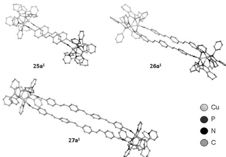
Fig. 11.10 Views of the solid state structures of the tetracationic supramolecular rectangles 25a 1 – 27a 1 (H atoms, counteranions and solvent molecules have been omitted for clarity)
