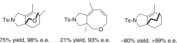
Fig. 10.34 Products from dien-yne cycloisomerizations promoted by Rh-TolBINAP complexes [48]
