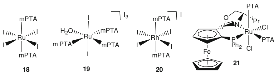
Fig. 7.1 Ru and Rh-PTA complexes 18–21 , active catalysts for C=O bond reduction
