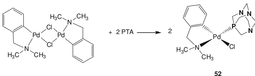
Scheme 7.12 Synthesis of [Pd(dmmba)Cl(PTA)] ( 52 )
