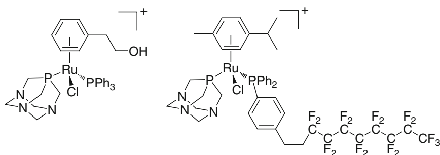
Fig. 13.14 RAPTA derivatives with an additional phosphine co-ligand
