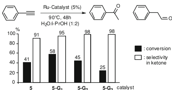
Fig. 7.8 Hydration of phenylacetylene using monomer 5 and dendrimers 5-G n ( n = 1-3 )
