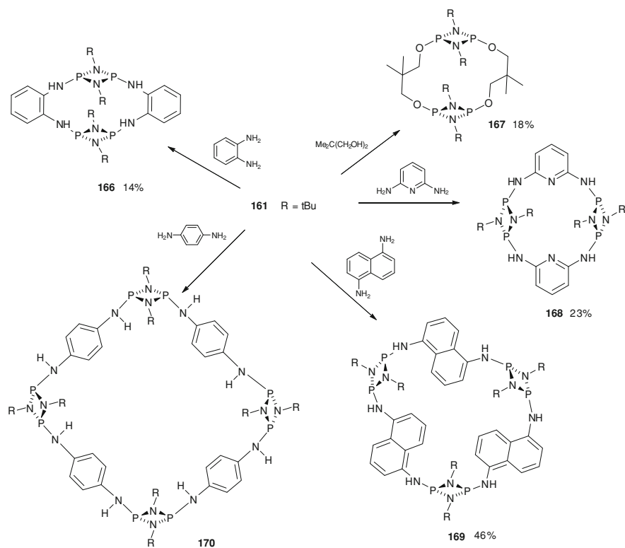
Scheme 12.61 Synthesis of cyclophanes formed by 1,3-diaza-2,4-diphosphacyclobutane units 166–170
