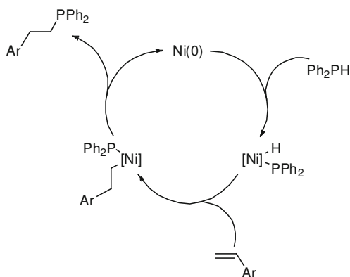
Scheme 8.44 Ni-catalyzed hydrophosphination of aryl(hetaryl) substituted alkenes
