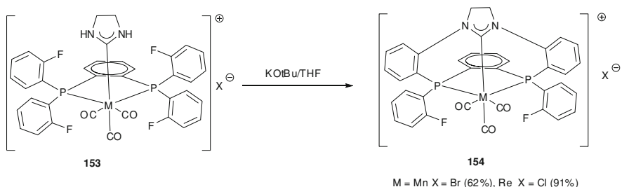
Scheme 12.57 Template synthesis of cyclophane 154
