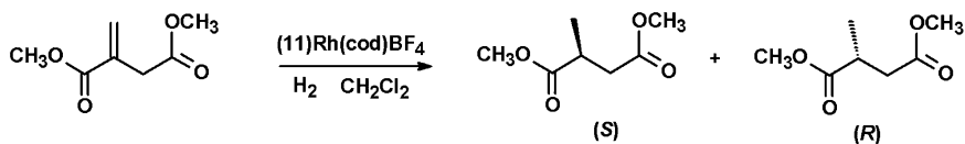
Scheme 6.16 Rh-catalyzed hydrogenation of dimethyl itaconate with [(11)Rh(cod)]BF 4
