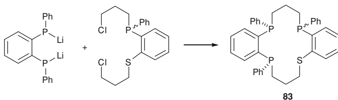
Scheme 12.32 Synthesis under high-dilution conditions of 14-membered P,S-containing macrocyclic ligand 83
