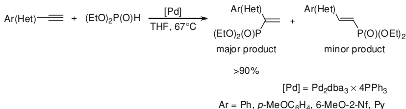
Scheme 8.5 Pd-catalyzed hydrophosphorylation of aryl(hetaryl) substituted alkynes
