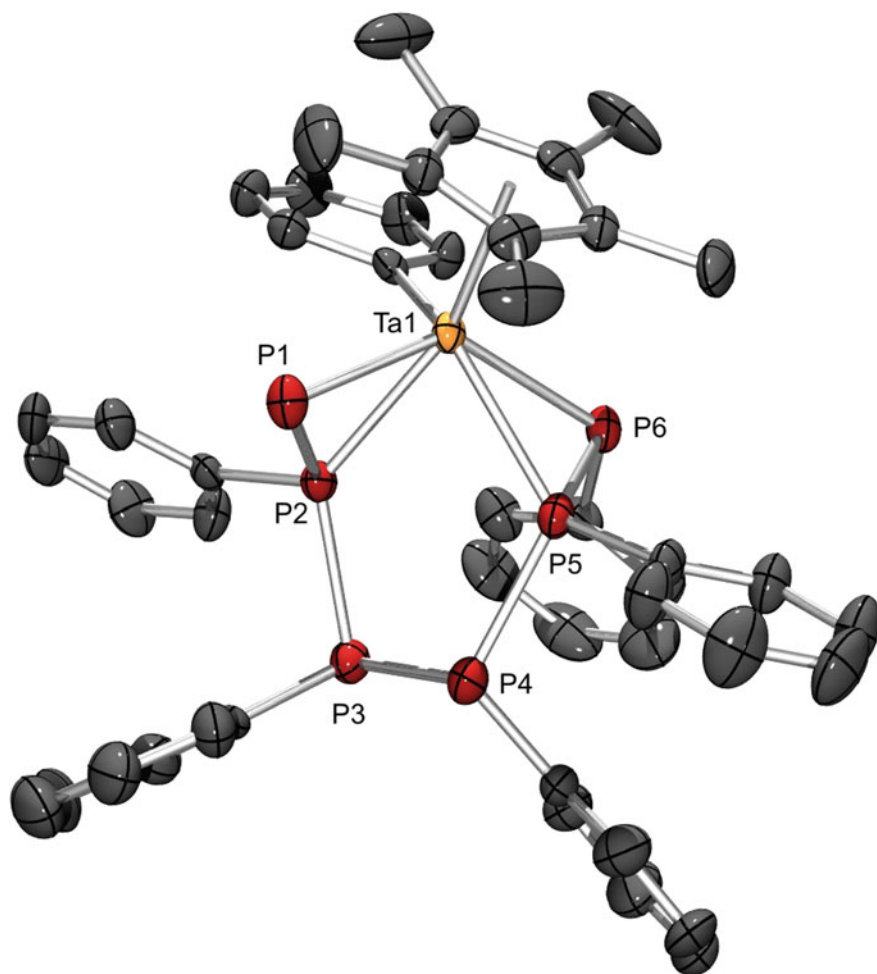
Fig. 4.23 Molecular structure of [\text{Ta}(\eta^5\text{-C}_5\text{Me}_5)(\text{Ph})(\text{P}_6\text{Ph}_5)] ( 42 ). Hydrogen atoms are omitted for clarity
