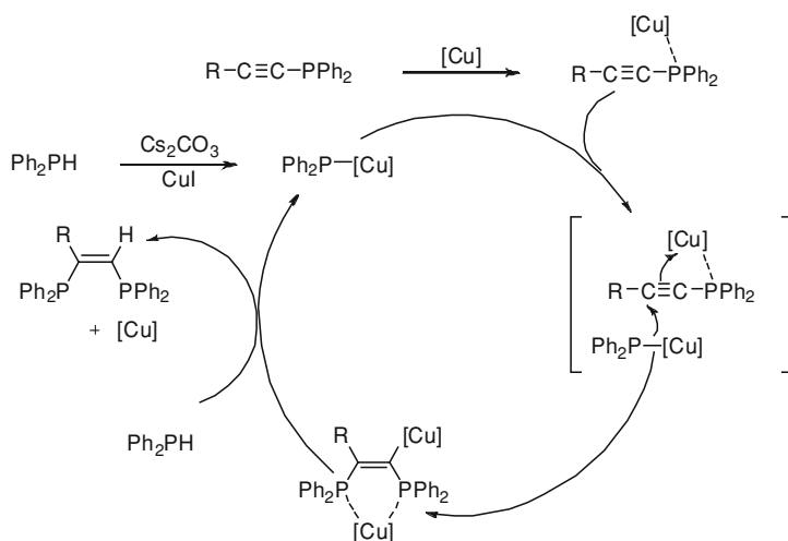
Scheme 8.61 Proposed mechanism of Cu-catalyzed hydrophosphination of 1-alkynylphosphines
