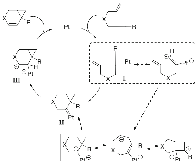
Fig. 10.41 Postulated mechanism for the cycloisomerization of enynes into bicyclo[n,1,0] derivatives
