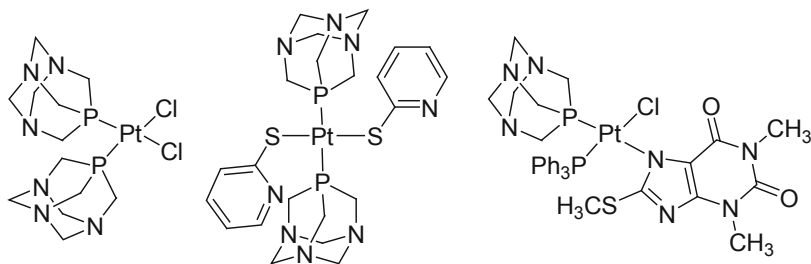
Fig. 13.3 PTA containing Pt(II) complexes
