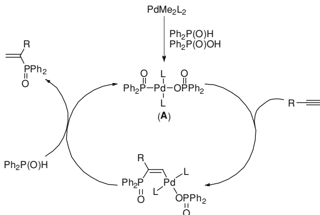
Scheme 8.29 Proposed mechanism of hydrophosphinylation of alkynes using [Pd]/Ph 2 P(O)OH catalytic system
