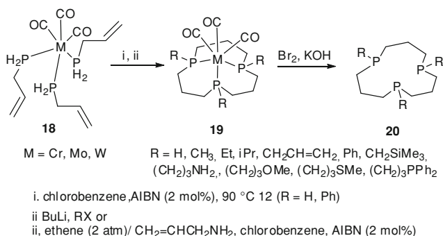
Scheme 12.7 Template synthesis of 12-membered macrocycles 20
