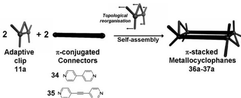
Scheme 11.12 Synthesis of \pi -stacked metallocyclophanes 36a , 37a using the adaptative \text{Ag}^{\text{I}} -dimer molecular clip 11a
