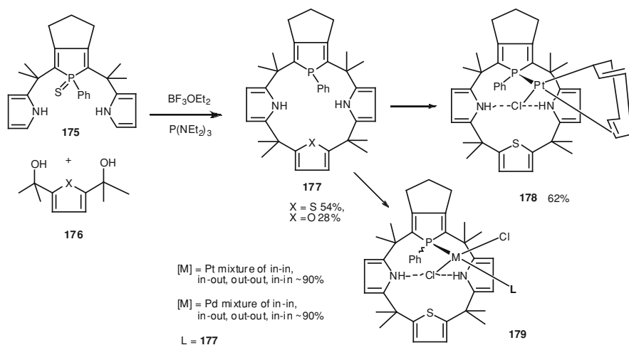
Scheme 12.63 Synthesis of phosphole-containing hybrid calixpyrroles 177 and their transition metal complexes- 178-179
