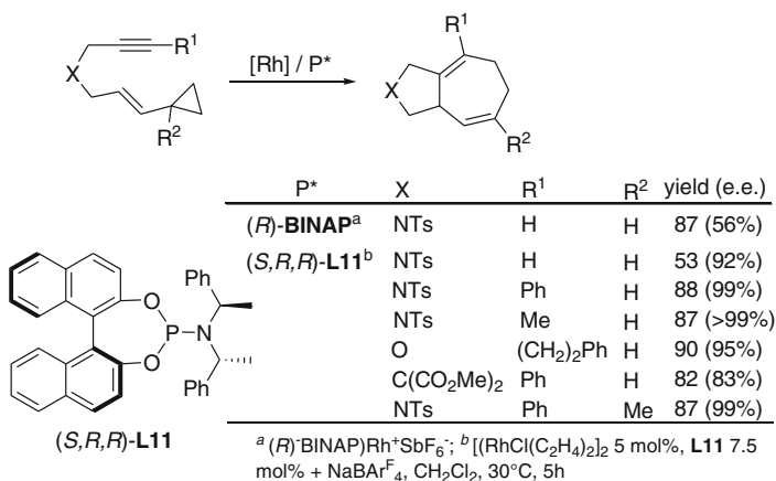
Fig. 10.39 Enantioselective [5 + 2] cycloadditions promoted by cationic rhodium complexes [38, 52]
