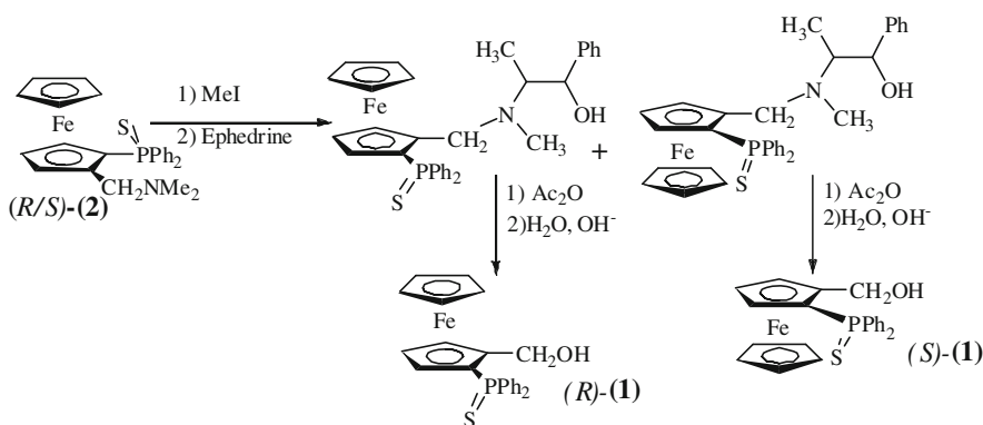
Scheme 5.4 Synthesis of the enantiomerically pure (S)- 1 and (R)- 1
