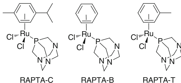
Fig. 13.9 Examples of RAPTA complexes
