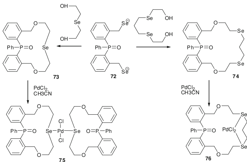
Scheme 12.28 Synthesis of 14-membered and 18-membered P,O,Se-containing macrocyclic ligands 73 and 74 and their palladium(II) complexes 75 and 76
