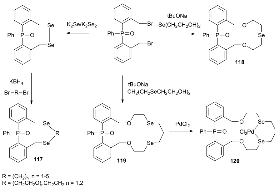
Scheme 12.46 Synthesis and transition metal complexes of P,Se- and P,O,Se-containing macrocycles 117 – 119
