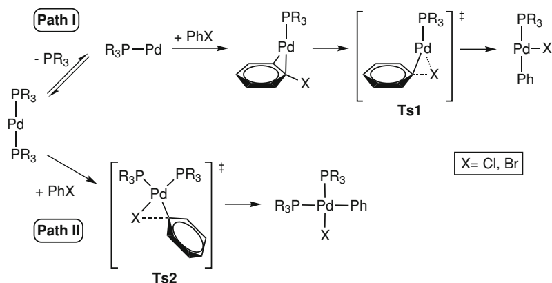
Fig. 3.3 Reaction mechanisms for the oxidative addition of PhX to [\text{Pd}(\text{PR}_3)_2] [53]
