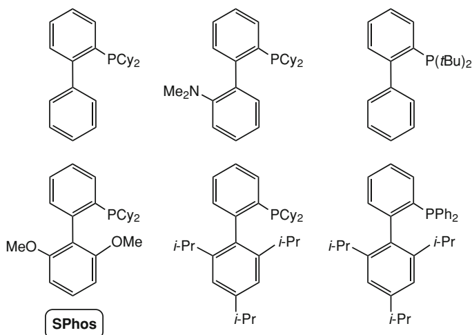
Fig. 3.9 Some examples of dialkylbiarylphosphines [76]
