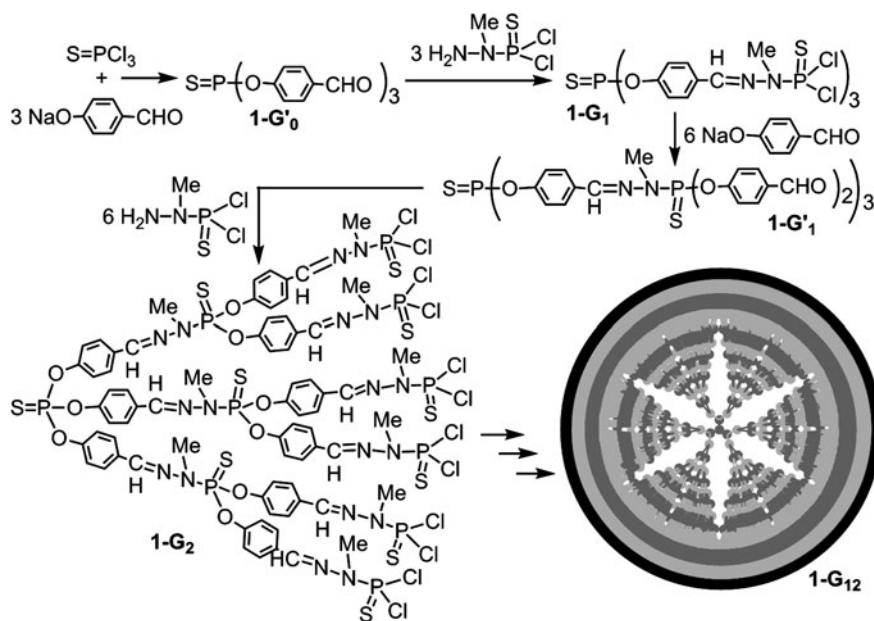
Fig. 9.2 The most widely used method of synthesis of phosphorus dendrimers, applied here to the trifunctional core \text{P}(\text{S})\text{Cl}_3 , and up to the twelfth generation 1\text{-G}_{12}
