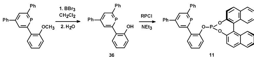
Scheme 6.15 Synthesis of chiral phosphinine-phosphites
