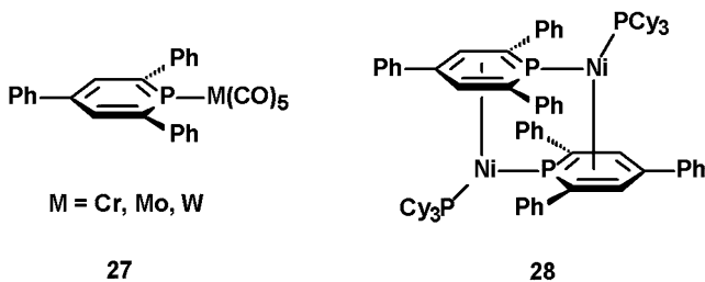
Fig. 6.13 Transition metal complexes of phosphinines ( \sigma - and \sigma/\pi -coordination mode)
