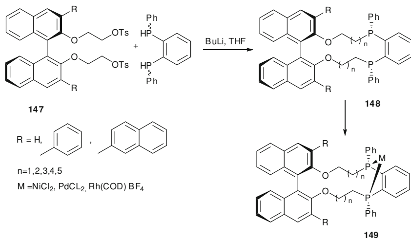
Scheme 12.55 Synthesis under high-dilution conditions of binaphthyl-based macrocyclic diphosphines 148 and chelate complexes 149
