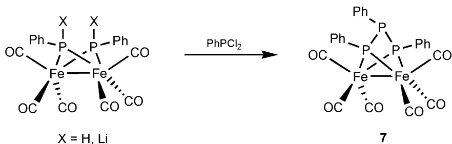
Fig. 4.2 An example of method 2 for the preparation of metal oligophosphanides
