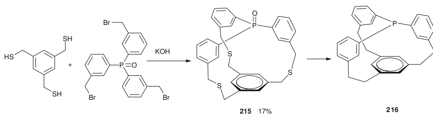
Scheme 12.75 Synthesis under high-dilution conditions of P,S-containing cryptand 215
