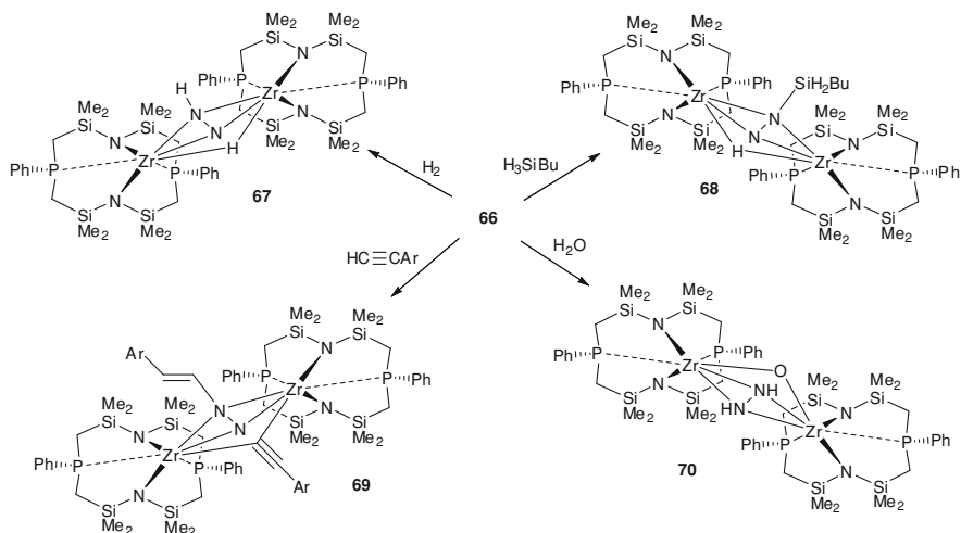
Scheme 12.26 Dinitrogen activation occurred in the coordination sphere of Zr complexes 66 with hybrid 12-membered macrocyclic ligand 63
