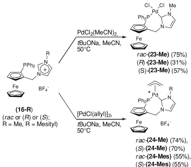
Scheme 5.15 Synthesis of phosphine-carbene palladium complexes 23 and 24
