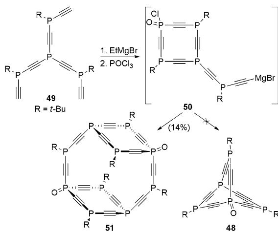
Fig. 2.17 Construction of phosphine-acetylenic Cage 51
