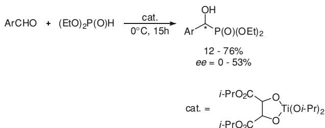
Scheme 8.67 Hydrophosphorylation of aromatic aldehydes using Sharpless catalyst
