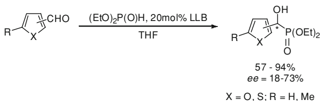
Scheme 8.72 LLB-catalyzed hydrophosphorylation of heteroaromatic aldehydes
