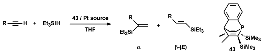
Scheme 6.26 Pt-catalyzed hydrosilylation of alkynes
