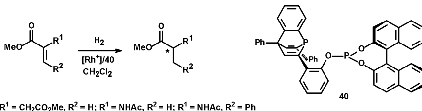
Scheme 6.23 Rh-catalyzed asymmetric hydrogenation of prochiral substrates
