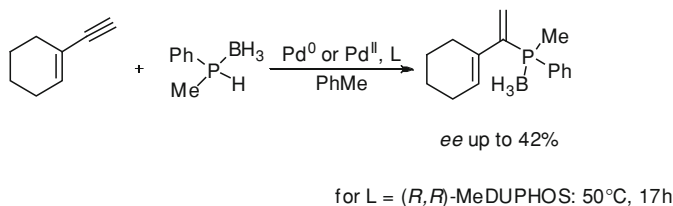
Scheme 8.56 Pd-catalyzed hydrophosphination of 1-ethynylcyclohexene
