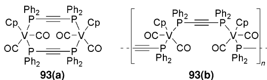
Fig. 2.34 [(\text{CpV}(\text{CO})_2)_2(\text{dppa})_2] ( 93 ); reported macrocyclic structure (a) and more probable polymeric structure (b)
