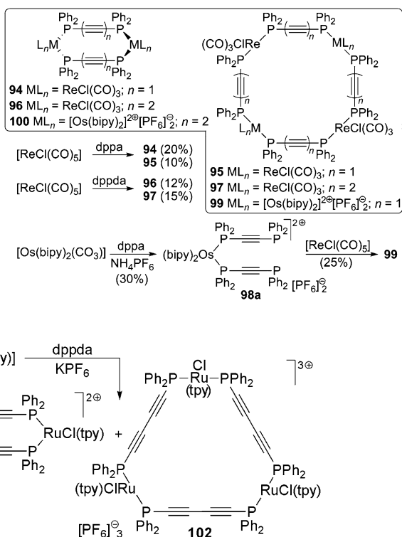
Fig. 2.36 Formation of Ru-dppda macrocycles 101 and 102
