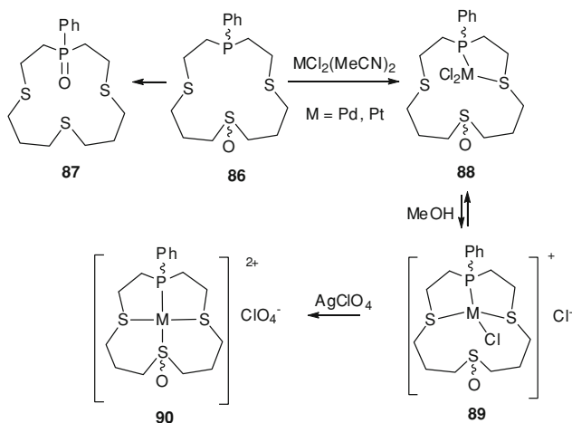
Scheme 12.34 Transition metal complexes 88–90 of 14-membered P,S,O-containing macrocyclic ligands 86
