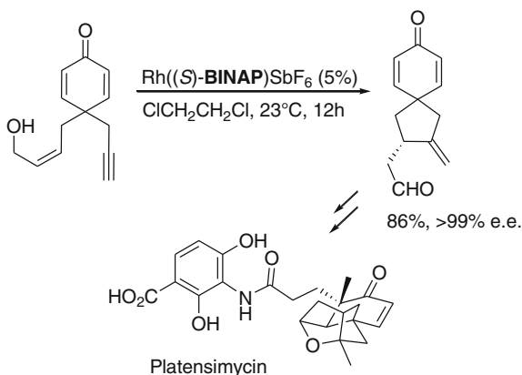
Fig. 10.25 Synthetic approach to Platensimycin [25]
