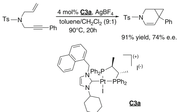
Fig. 10.43 Enantioselective cycloisomerization of 1,6-enynes promoted by cationic (NHC)Pt[( S,S )-chiraphos] complexes [63]
