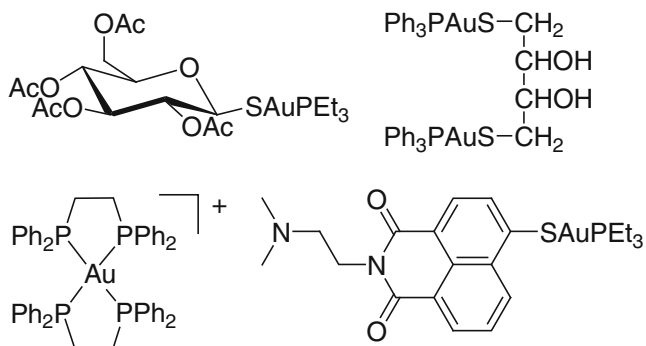
Fig. 13.16 Auranofin ( top left ) and examples of other Au(I) complexes with phosphine ligands
