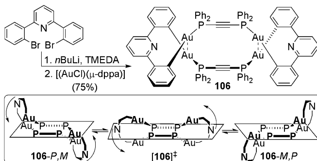
Fig. 2.39 Structure and conformations of 106 . The movement of the dppy ligands is indicated with arrows
