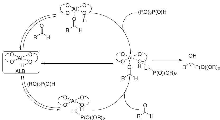
Scheme 8.70 Proposed mechanism of hydrophosphorylation of aldehydes using ALB catalyst
