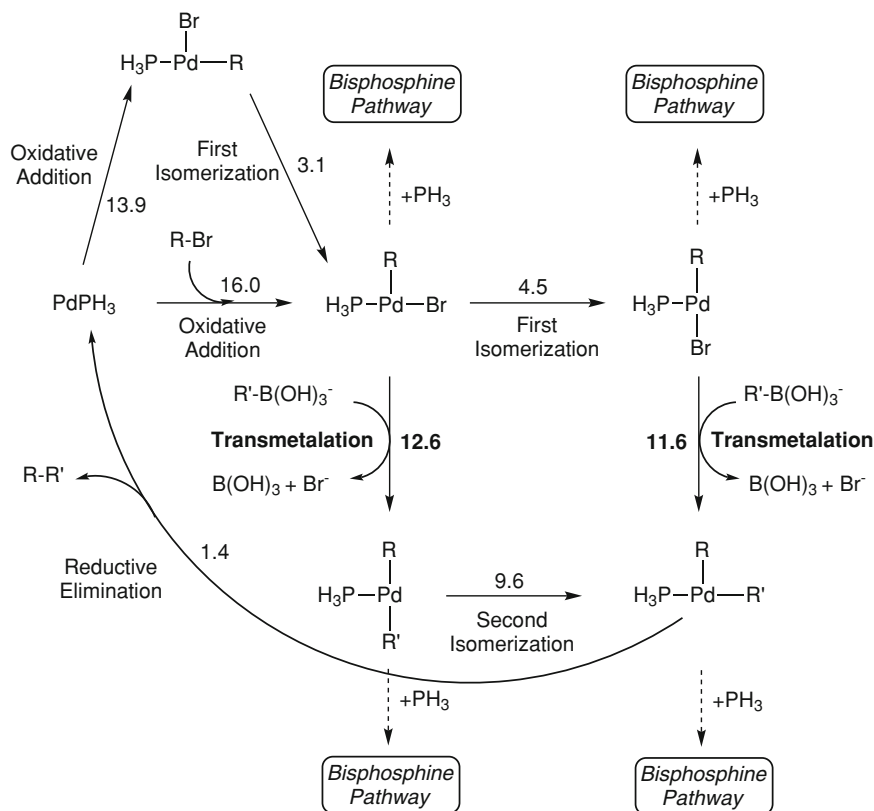
Fig. 3.8 Full reaction mechanism for the Suzuki reaction through monophosphine Pd complexes theoretically analyzed by Maseras et al. [71] (Energies in kcal/mol)
