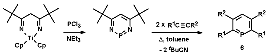
Scheme 6.5 Synthesis of phosphinines from diazaphosphinines
