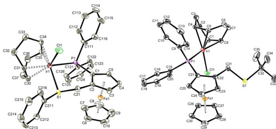
Fig. 5.3 Structure of [\text{IrCl}(\text{COD})(7\text{-R})] complexes. Left R = Ph. Right R = t Bu
