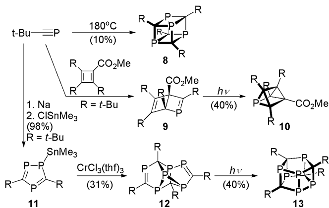
Fig. 2.4 P/C cages obtained by cyclooligomerization of phosphalkynes (11–13)
