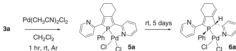
Scheme 11.4 Isomerization of phosphole complex 5a to 2-pyridyl-2-phospholene-Pd complex 6a
