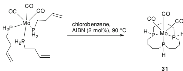
Scheme 12.13 Template synthesis of 15-membered macrocycle 31
