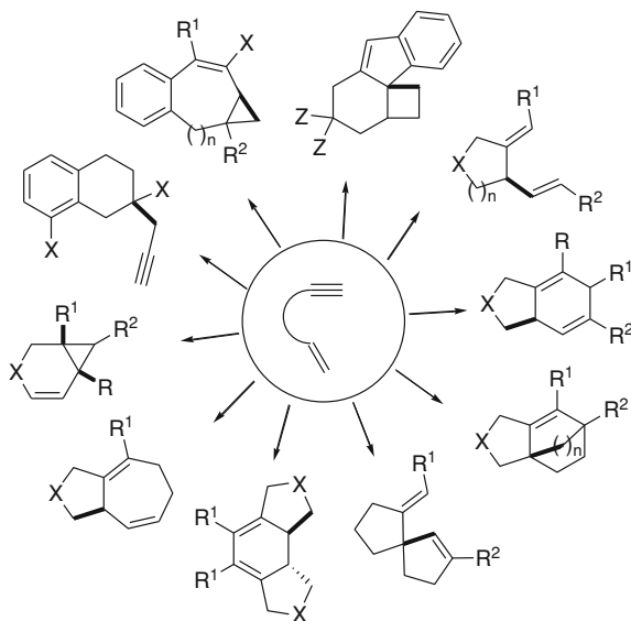
Fig. 10.1 Representative molecular scaffolds produced by enantioselective enyne cycloisomerization reactions
