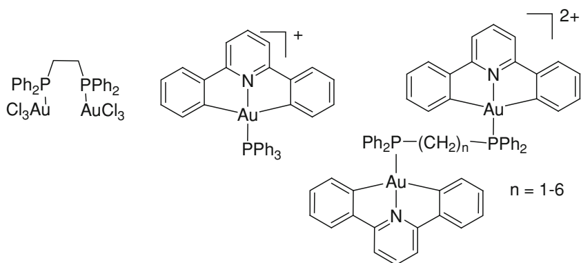
Fig. 13.20 Au(III) complexes with anticancer activity
