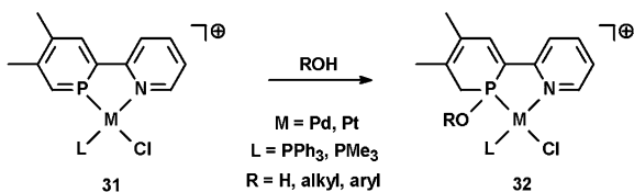
Scheme 6.7 Formation of dihydrophosphinines
