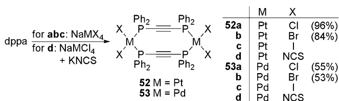
Fig. 2.19 First dppa-based macrocycles
