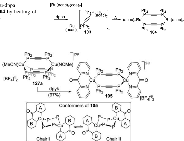
Fig. 2.38 Structure and conformation of Cu-dppa macrocycle 105
