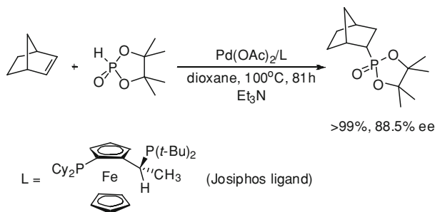
Scheme 8.19 Enantioselective Pd-catalyzed hydrophosphorylation of 2-norbornene
