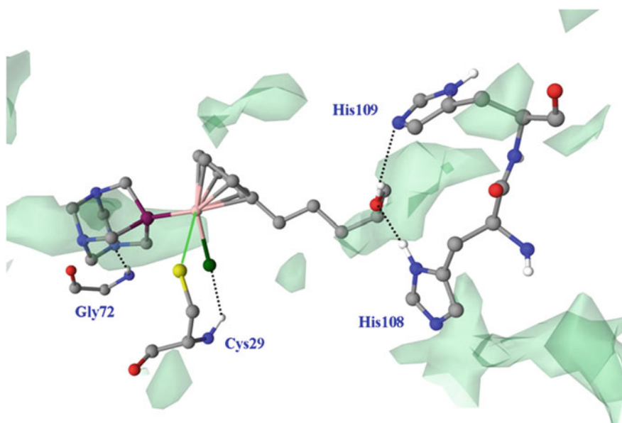
Fig. 13.12 Figure of cathepsin B docking studies showing the main interactions of the ligand with the residues flanking the active site. Adapted from Ref. [38]
