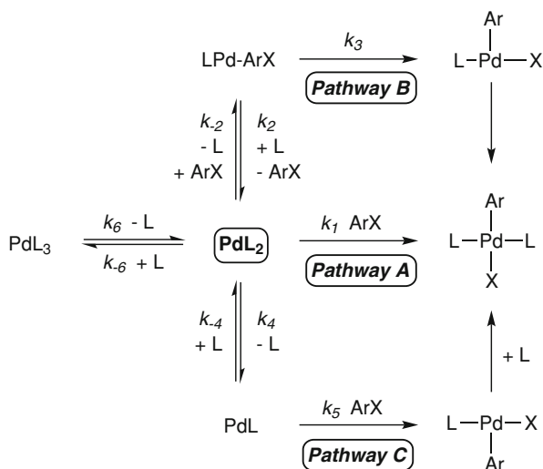
Fig. 3.4 Scheme of the three proposed mechanisms for the oxidative addition of ArX to [PdL_2] [55]
