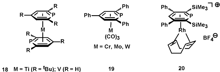
Fig. 6.9 Transition metal complexes of phosphinines ( \pi -coordination mode)
