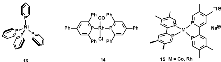
Fig. 6.7 Transition metal complexes of phosphinines ( \sigma -coordination mode)
