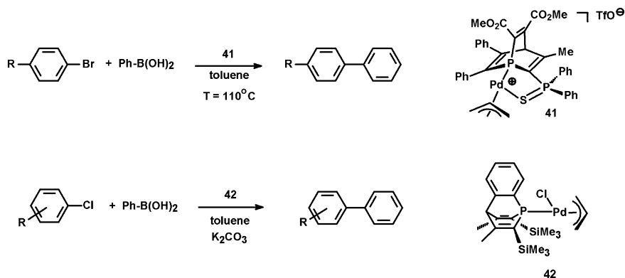
Scheme 6.24 Pd-catalyzed Suzuki–Miyaura cross-coupling reaction
