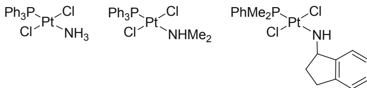
Fig. 13.5 Examples of trans -Pt(II) complexes
