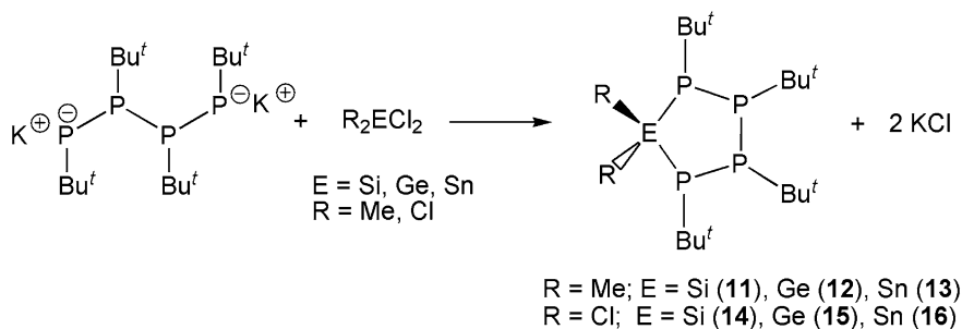
Fig. 4.4 Synthesis of complexes of the type cyclo -(P 4 Bu 4 t ER 2 ) (E = Si, Ge, Sn; R = Bu t , Cl) using method 4
