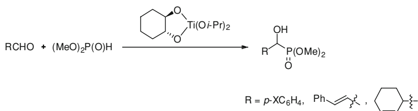
Scheme 8.65 Hydrophosphorylation of aromatic aldehydes using [\text{Ti}]/\text{cyclohexyl diol} catalytic system
