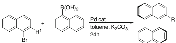
Scheme 5.18 Palladium-catalyzed asymmetric Suzuki coupling
