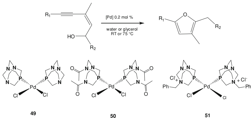
Scheme 7.11 Pd(II) catalysts for cycloisomerization of (Z)-2-en-4-yn-1-ols into furans
