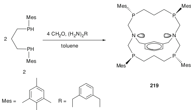
Scheme 12.77 Covalent self-assembly of P,N-containing cryptand 219
