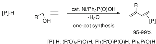
Scheme 8.12 Ni-catalyzed addition/dehydration reactions of P–H bond with propargyl alcohols
