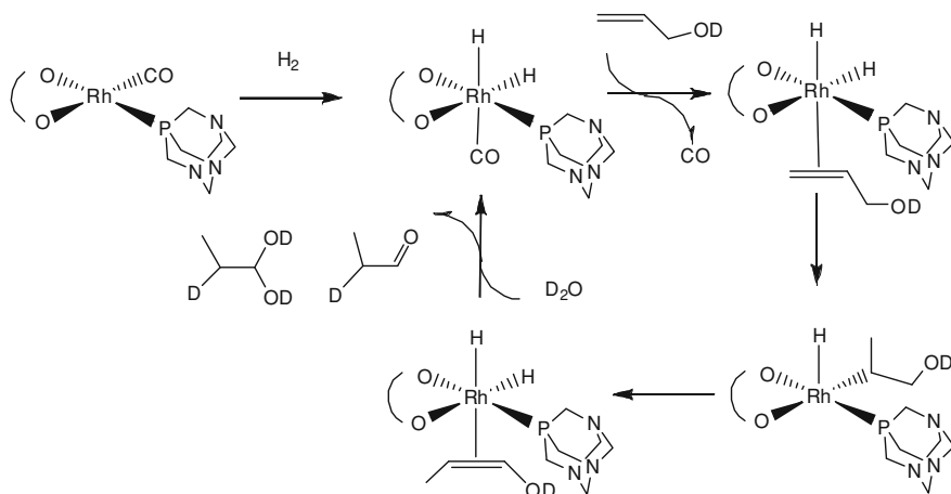
Scheme 7.7 Proposed mechanism for allyl alcohol hydrogenation in D 2 O in the presence of [Rh(acac)(CO)(PTA)] ( 32 )
