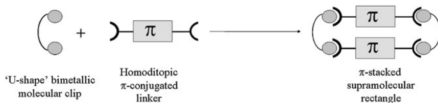
Scheme 11.10 Coordination-driven supramolecular synthesis of [2,2]-paracyclophanes analogues according to the directional bonding approach
