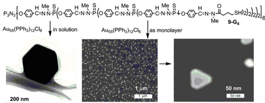
Fig. 9.10 Organization of \text{Au}_{55} clusters as nanocrystals induced by the dendrimer 9-G 4
