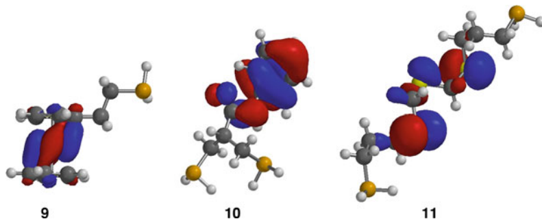
Fig. 1.8 Our DFT calculations for the ground state HOMO distribution of the air-stable primary phosphines 9 , 10 and 11 . Extensive conjugation and/or heteroatom presence reduces phosphorus incorporation from the HOMO and destabilizes the energy of the HOMO radical cation
