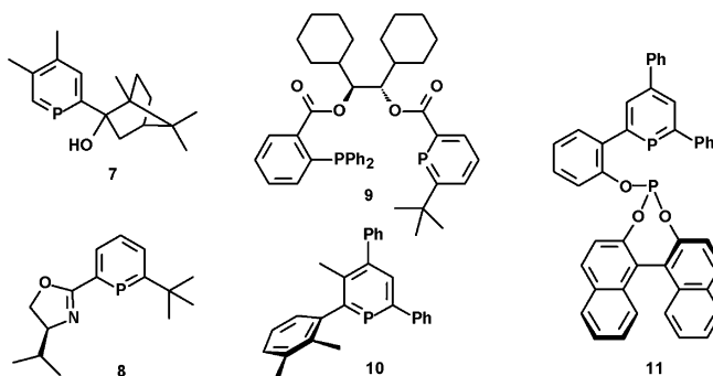
Fig. 6.5 Chiral phosphinines
