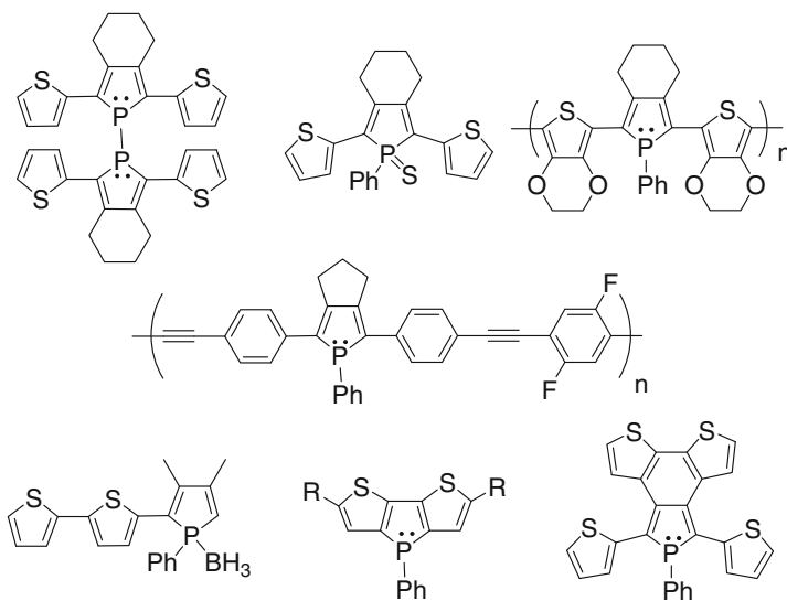
Fig. 11.2 Representative examples of phosphole-based \pi -conjugated systems
