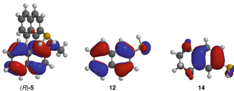
Fig. 1.7 DFT calculations indicating the ground state HOMO distribution for ( R )- 5 , 12 and 14 . Increasing conjugation reduces then eliminates phosphorus incorporation in the HOMO
