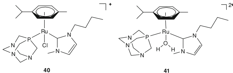
Fig. 7.5 Imidazolyl-arene Ru(II) PTA complexes 40 and 41
