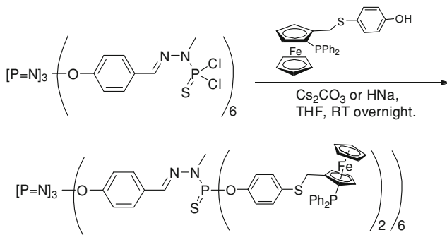
Scheme 5.7 Synthesis of the dendrimeric ligands G 1-7
