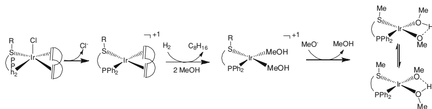
Scheme 5.21 Proposed pathway to the precatalyst
