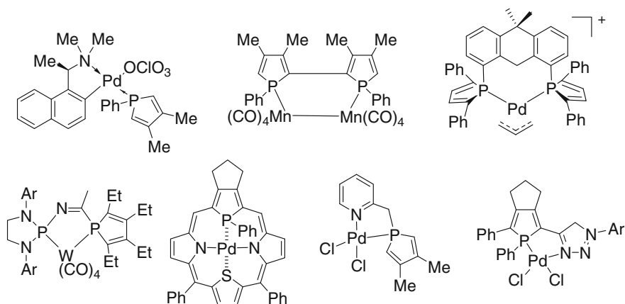
Fig. 11.1 Selected examples of complexes bearing phosphole-based ligands
