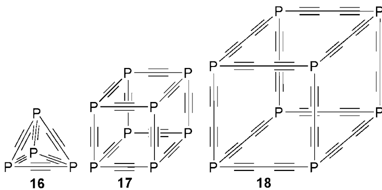
Fig. 2.6 Phosphine acetylenic scaffolding in 3-D
