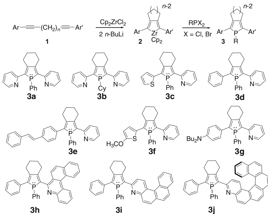
Scheme 11.1 Synthesis of 2-(2-pyridyl)phosphole derivatives by the Fagan–Nugent method
