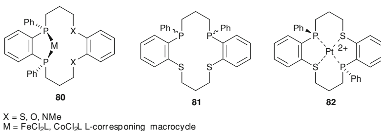
Scheme 12.31 Transition metal complexes 80–82 of 14-membered P,S-containing macrocyclic ligands
