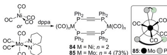
Fig. 2.29 Formation of \text{Ni}(\text{CO})_2 and \text{Mo}(\text{CO})_4 macrocycles 84 and 85 . Inset: Representation of 85 , viewed along the Mo-Mo vector. Phosphorus atoms of the same dppa bridge are connected
