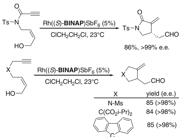
Fig. 10.24 Rh(BINAP)SbF 6 promoted cycloisomerization of terminal enynes [36, 37]
