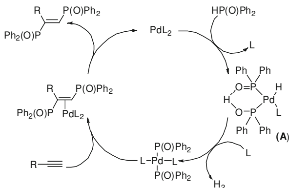
Scheme 8.34 Proposed mechanism of Pd-catalyzed dehydrogenative double phosphinylation of terminal alkynes with diphenylphosphine oxide
