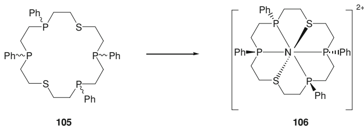
Scheme 12.41 Synthesis of nickel(II) complex 106 of 18-membered P,S-containing macrocycle 105
