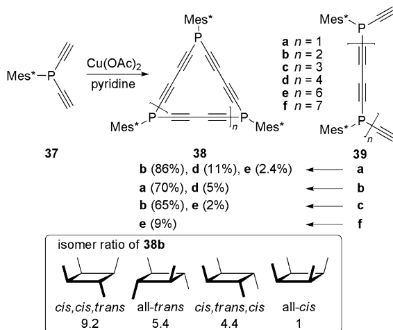
Fig. 2.13 Exploded phospha[n]pericyclines 38 via a one-pot approach from 37 and from linear precursors 39
