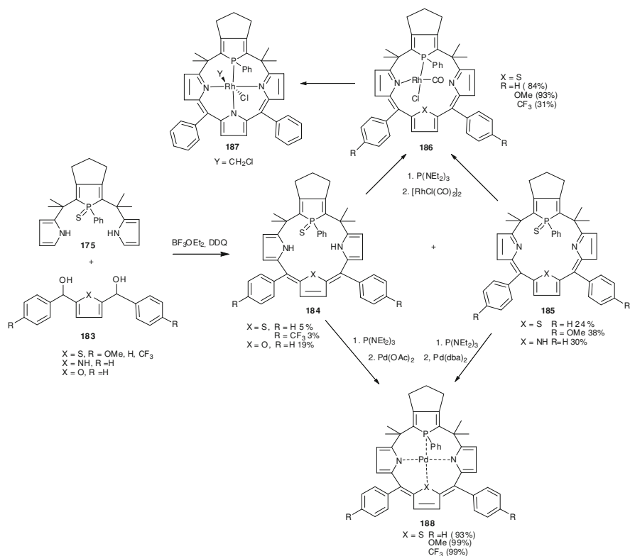
Scheme 12.65 Synthesis of calixphyrins 184 and 185 and their transition metal complexes 186–188
