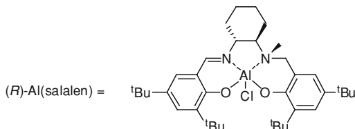
Scheme 8.73 Hydrophosphorylation of aldehydes using (R)-Al(salalen) complex
