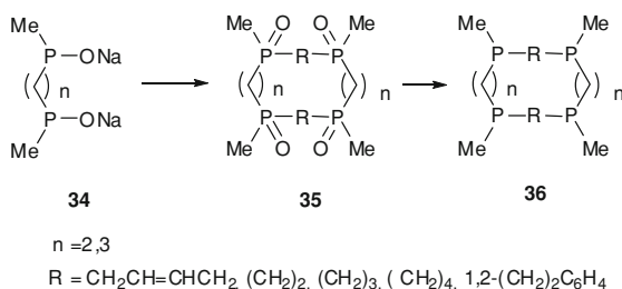
Scheme 12.14 Synthesis of 16-membered macrocycle 33
