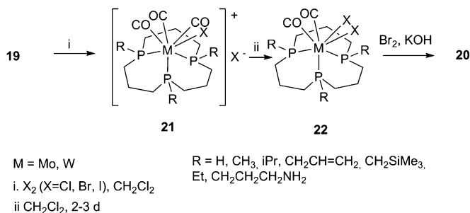
Scheme 12.8 Oxidative addition of halogens ( \text{Cl}_2 , \text{Br}_2 , \text{I}_2 ) to molybdenum and tungsten tricarbonyl complexes 19
