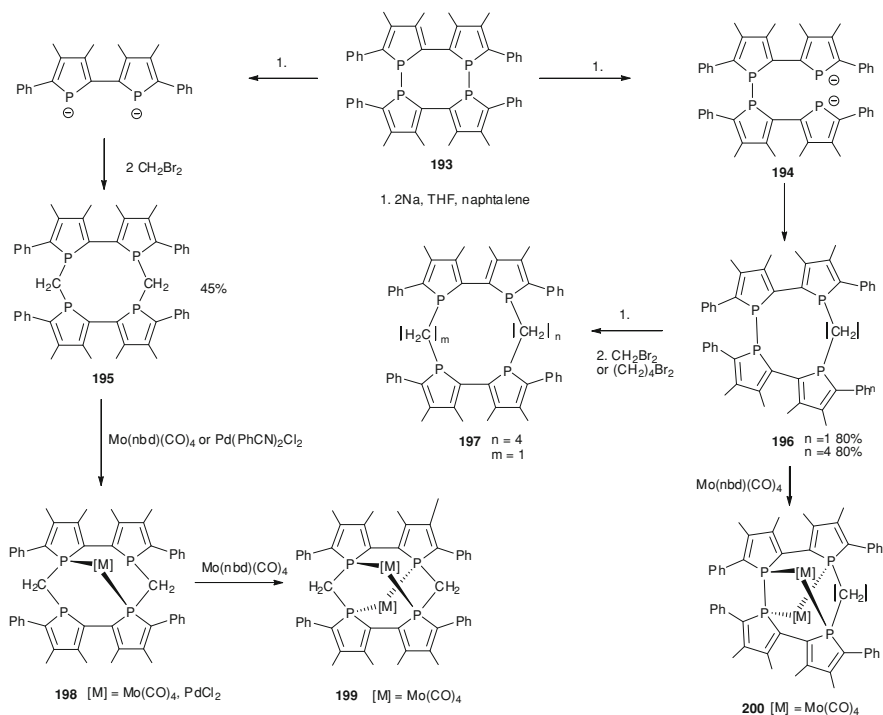
Scheme 12.67 Synthesis of phosphole based cyclophanes 193–197 and their transition metal complexes 198–200
