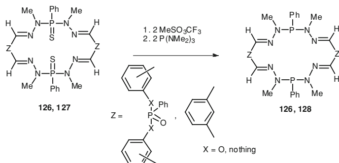
Scheme 12.50 Desulfurization of thiophosphonic macrocycles 126–127
