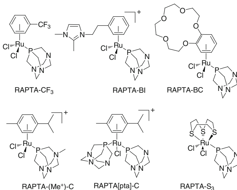
Fig. 13.10 Examples of RAPTA-type complexes explored as antitumor agents
