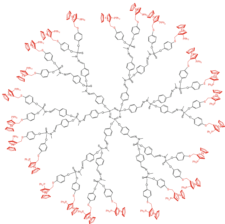
Scheme 5.8 Ligand G 2 -7
