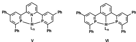
Fig. 6.18 Di-phosphinines and phosphabarrelenes
