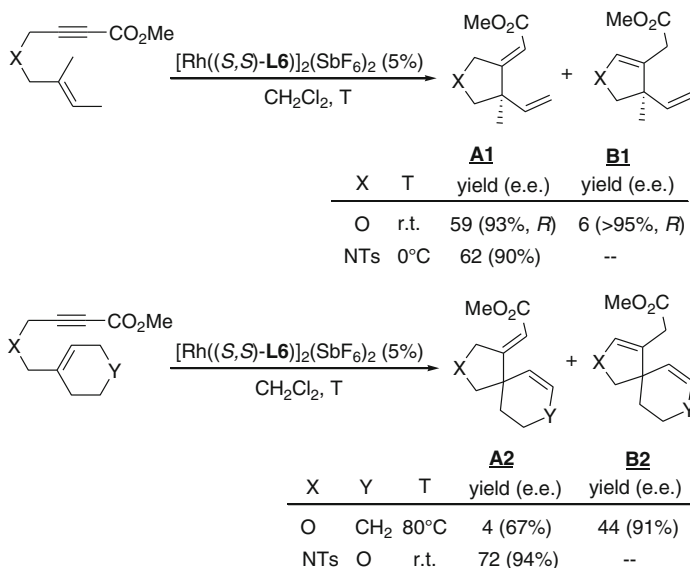
Fig. 10.27 Rh-Skewphos promoted cycloisomerization of 1,6-enynes with trisubstituted double bonds [40]
