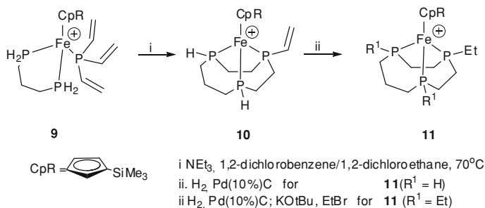
Scheme 12.4 Template synthesis 10-membered cyclic triphosphines 10 and 11
