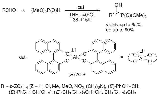
Scheme 8.69 Hydrophosphorylation of aldehydes using ALB catalyst
