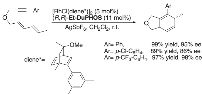
Fig. 10.31 Enantioselective [4 + 2] cyclizations of dienynes promoted by Rh-diphosphine-diene complexes [46]
