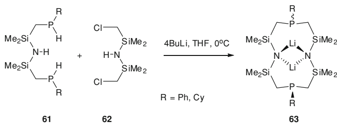
Scheme 12.23 Template synthesis of of 12-membered ring macrocycle 63
