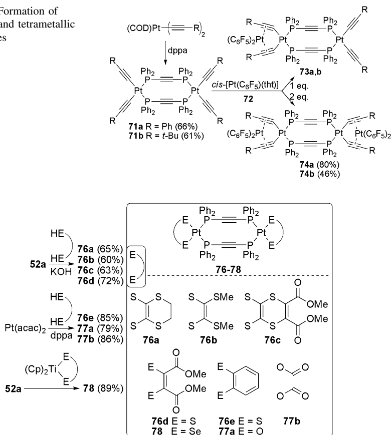
Fig. 2.26 Dichalcogenate complexes of [Pt 2 (μ-dppa) 2 ] ( 76–78 )
