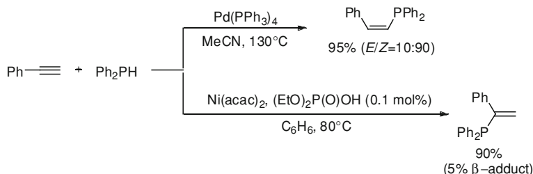
Scheme 8.51 Catalytic hydrophosphination of phenylacetylene
