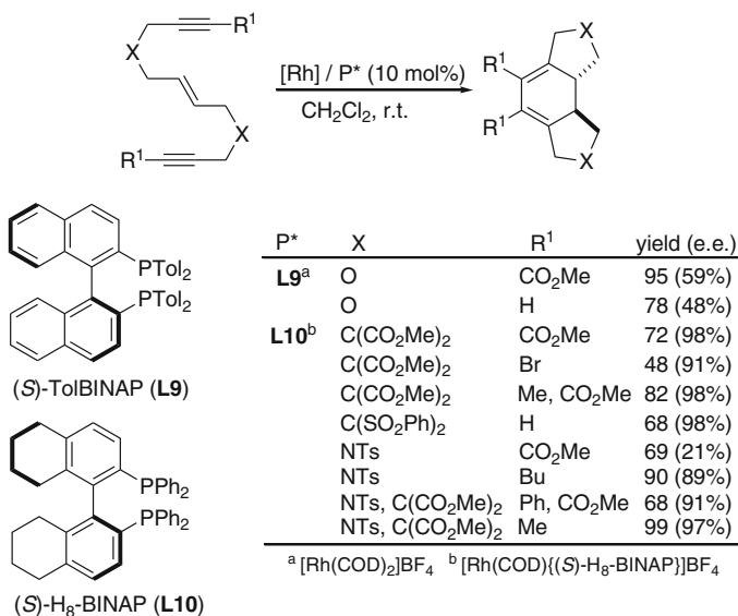
Fig. 10.37 Rhodium promoted [2 + 2 + 2] cycloadditions of ene-diyne [49, 50]
