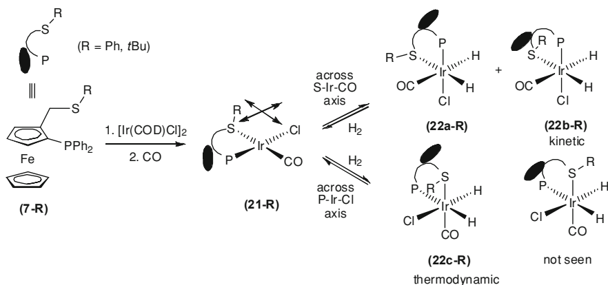
Scheme 5.14 Addition of pH_2 on iridium complexes 21-R
