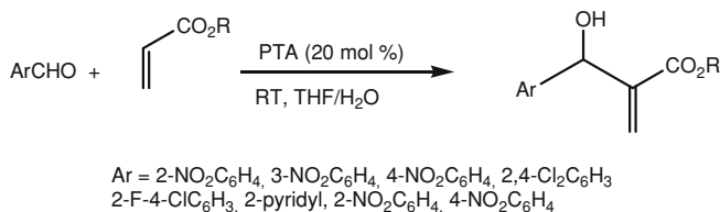
Scheme 7.9 Morita–Baylis–Hillman (MBH) reaction catalyzed by PTA
