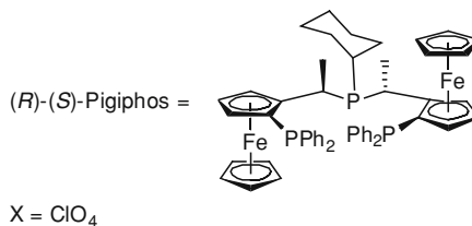
Scheme 8.49 Enantioselective hydrophosphination of methacrylonitrile using [Ni]/Pigiphos
