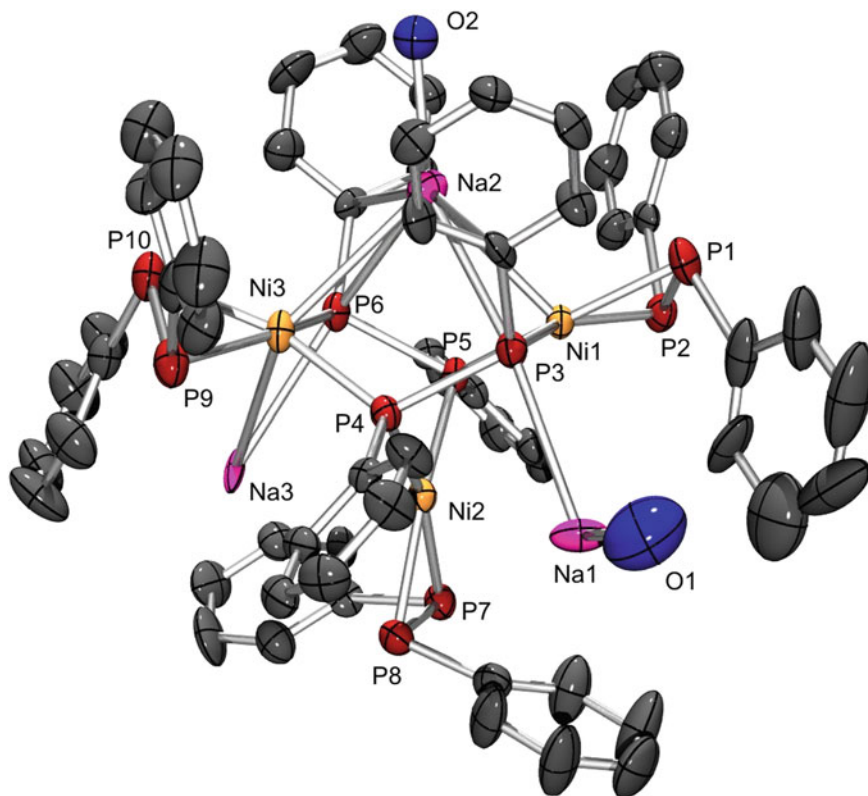
Fig. 4.17 Anionic part of the molecular structure of [\text{Na}(\text{Et}_2\text{O})_3][\text{Na}_3(\text{Et}_2\text{O})_2\text{Ni}_3(\mu\text{-P}_2\text{Ph}_2)_2(\eta^2\text{-P}_2\text{Ph}_2)_3] ( 36 ). Hydrogen atoms and carbon atoms of the coordinated ether molecules have been omitted for clarity
