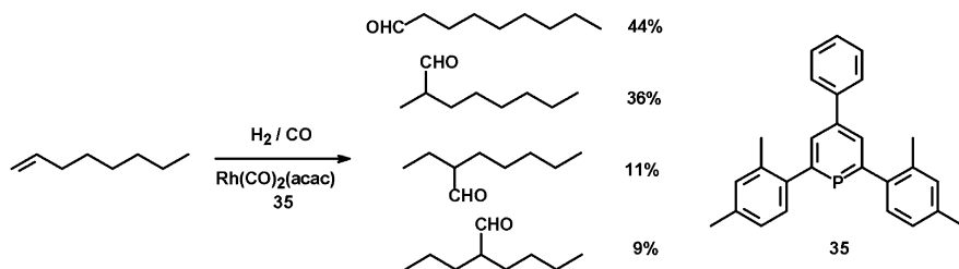
Scheme 6.10 Rh-catalyzed hydroformylation of 1-octene
