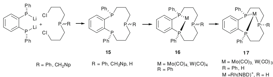
Scheme 12.6 Macrocyclization under high-dilution conditions and transition metal complexes of 11-membered cyclic triphosphines 15
