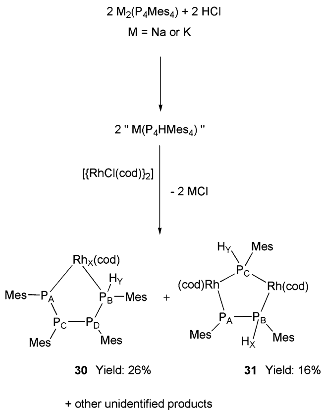
Fig. 4.12 Synthesis of [\text{Rh}(\text{P}_4\text{HMe}_4)(\text{cod})] ( 30 ) and [\text{Rh}_2(\mu\text{-P}_2\text{HMe}_2)(\mu\text{-PHMe})(\text{cod})_2] ( 31 )
