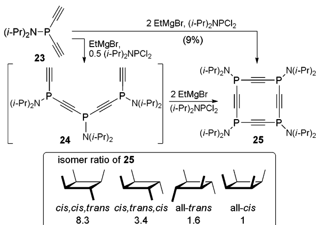
Fig. 2.8 One-step and stepwise synthesis of tetraphospha[4]pericycline 25
