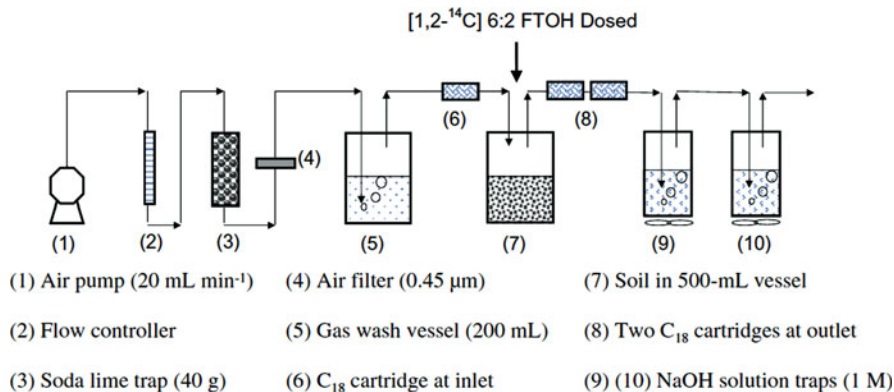
Fig. 2 Sophisticated biodegradation experimental setup allowing for constant aeration and capturing volatile transformation products on C 18 cartridges and basic traps. This setup was used to study biotransformation of 14 C 2 -labeled 6:2-FTOH. Taken from [29]
