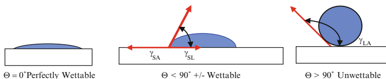
Fig. 2 Contact angle versus wettability of a substrate surface. When angle \Theta is > 90^\circ , liquid will not wet the surface; when angle \Theta is < 90^\circ , liquid will wet surface partially; when angle \Theta = 0^\circ , complete spreading & wetting of the surface by the liquid. Spreading occurs only if S > 0 . Spreading coefficient: S = \gamma_{SV} - (\gamma_{LV} + \gamma_{SL}) S = solid, L = liquid, A = air. where \gamma_{SA} = surface energy of the substrate (e.g., polymer surfaces), \gamma_{LA} = surface tension of the liquid and \gamma_{SL} = interfacial tension
