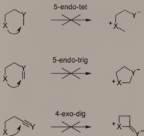
Scheme 9.1. Unfavorable processes according to Baldwin's rules.
