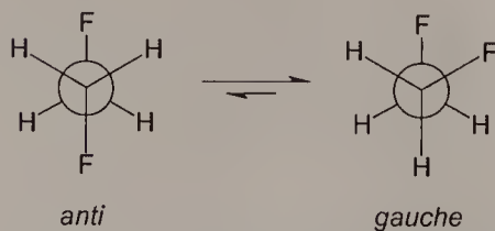
Scheme 2.2. Conformations of 1,2-difluoroethane.
