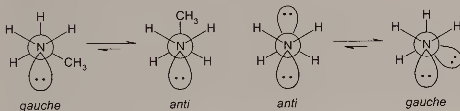
Scheme 2.3. Conformations of EtNH 2 (left [1]) and H 2 NNH 2 (right [13]).
