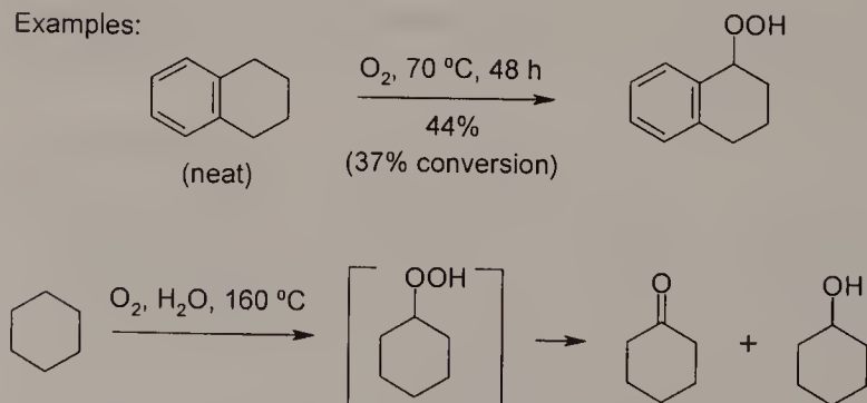
Scheme 3.15. Autoxidation of hydrocarbons [61, 62].
