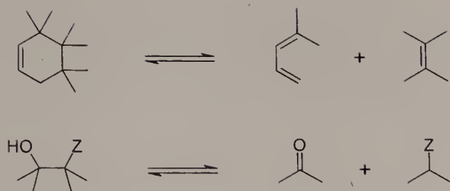
Scheme 3.2. Fragmentation via retro-Diels–Alder cycloaddition and retro-aldol addition.
