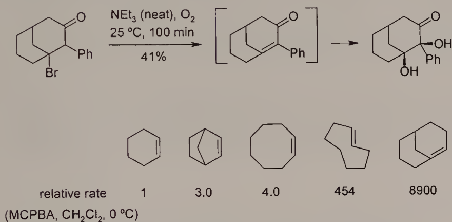
Scheme 3.6. Oxidation of a strained alkene by air [20] and relative rates of epoxidation of various cyclic alkenes [21].
