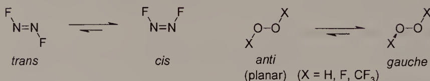
Scheme 2.5. Conformations of diazenes and peroxides.
