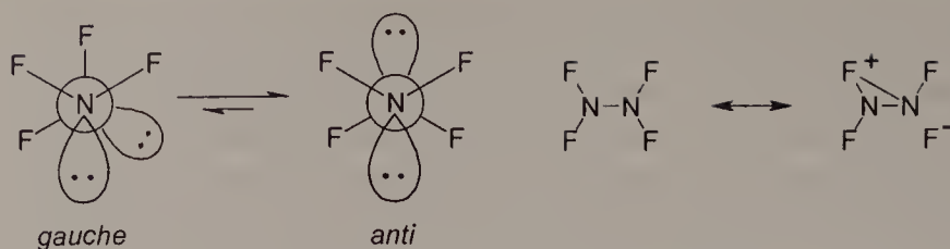
Scheme 2.4. Conformations and canonical forms of \text{F}_2\text{NNF}_2 [13].
