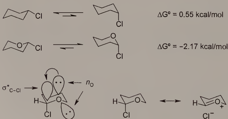
Scheme 2.6. The anomeric effect [16].
