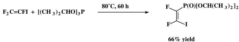
Figure 6.23 Direct replacement of fluoride by phosphorus at vinylic carbon.
