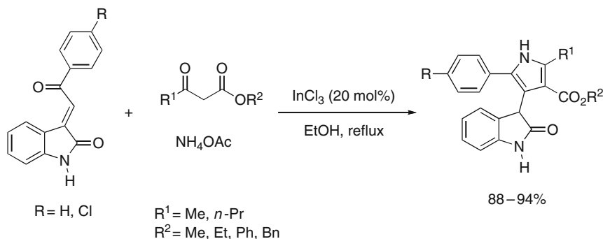
Scheme 47 \text{InCl}_3 -catalyzed three-component synthesis of 2-pyrrolo-3'-yloxindoles
