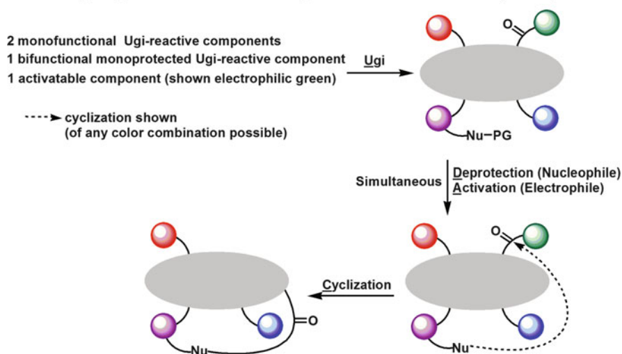
Fig. 3 The three most common modes to activate linear Ugi-products for cyclization, especially if the cyclization involves Ugi-reactive groups (e.g., acid, oxo-compound, or amine). Activation is mostly achieved with convertible isocyanides, i.e., activated amides (see text). Other MCRs follow similar concepts. With orthogonal second functionalities for cyclizations such deprotection and/or activation is not required (see below, e.g., RCM or cycloadditions)
