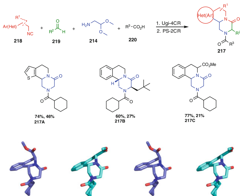
Scheme 39 Convergent MCR approach towards praziquantel derivatives 217 . Two representative diastereomers of 217C are drawn in blue and cyan
