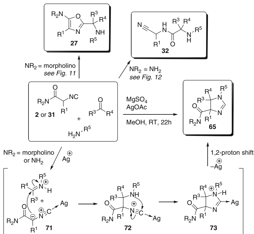
Fig. 22 Possible reaction paths for the reaction between \alpha -acidic isocyano amides (2 or 31), primary amines, and carbonyl components, including the Ag^I catalyzed formation of 2H-2-imidazolines (65)
