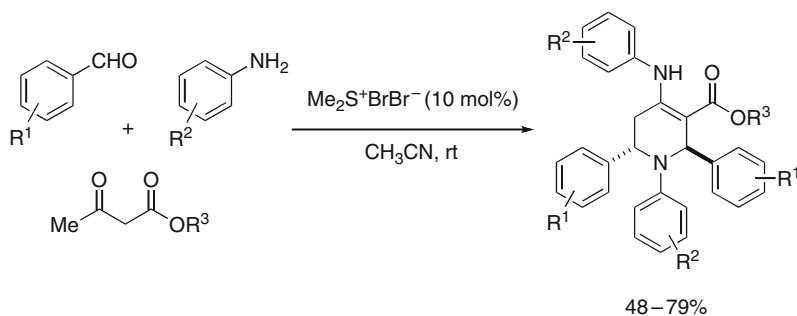
Scheme 24 BDMS-catalyzed multicomponent access to functionalized piperidines
