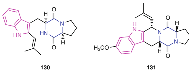
Fig. 8 Tryptophan moiety (magenta) containing piperazine natural products tryprostatin B 130 and fumitremorgin 131 are two inhibitors of mammalian cell progression at the G2/M transition
