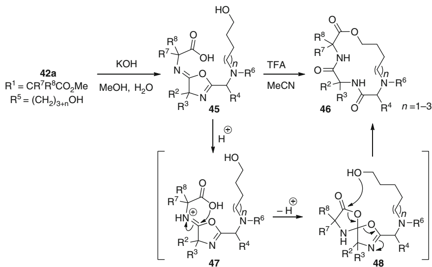
Fig. 16 Synthesis of macrocyclodepsipeptides from 5-iminooxazolines
