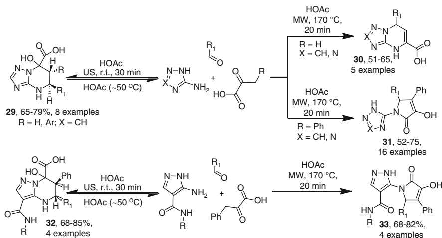
Scheme 13 MCRs under kinetic and thermodynamic control
