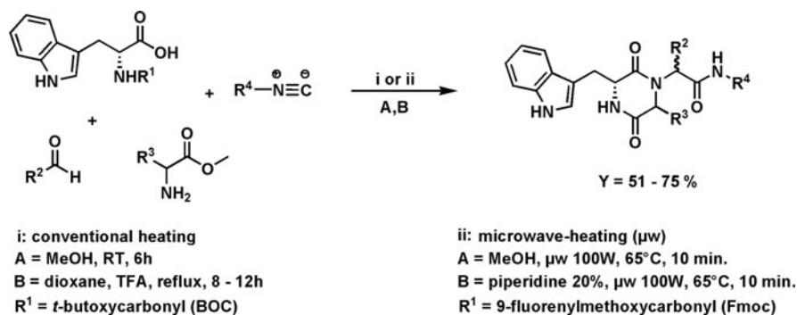
Scheme 4 Tryptophan derived diketopiperazines by microwave vs. conventional heating
