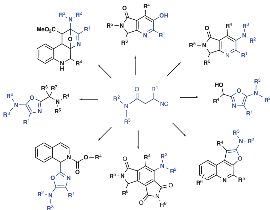
Fig. 3 \alpha -Isocyanoamides as the starting materials for a plethora of combinatorial scaffolds. The isocyanide borne moiety in the scaffolds is marked blue
