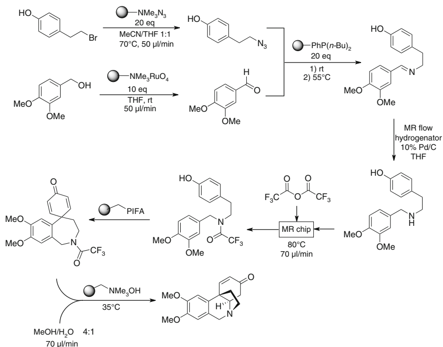
Scheme 34 A continuous flow synthesis of (±)-oxomaritidine [76]
