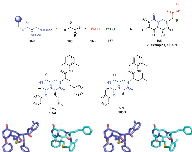
Scheme 28 Variations of bicyclic diketopiperazines 165 . Two representative diastereomers of 165A are drawn in blue and cyan and intramolecular hydrogen bonds are shown in red dots
