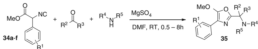
Fig. 13 Scope of isocyano esters in the MCR toward trisubstituted oxazoles
