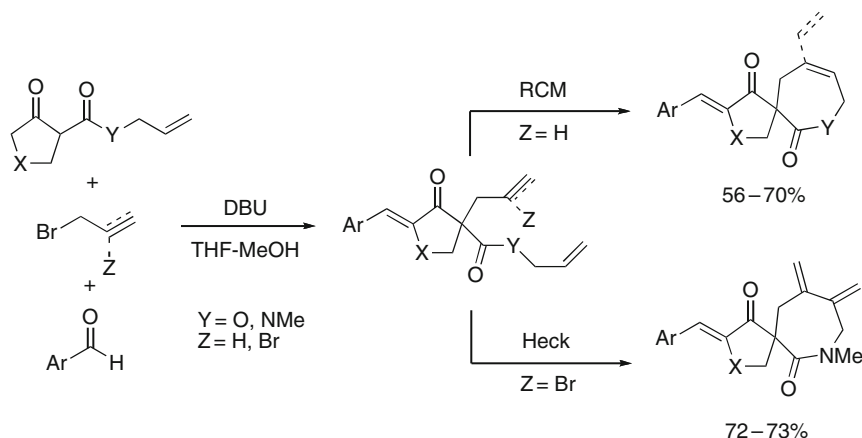
Scheme 62 Sequential multicomponent \alpha,\gamma -difunctionalization of 1,3-dicarbonyl/metal-catalyzed carbocyclization for the synthesis of spiro[4,6]-lactones and lactams
