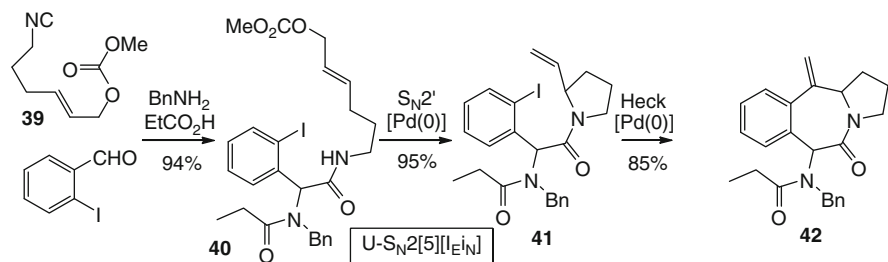
Fig. 7 Sequential Ugi- S_N2' -Heck
