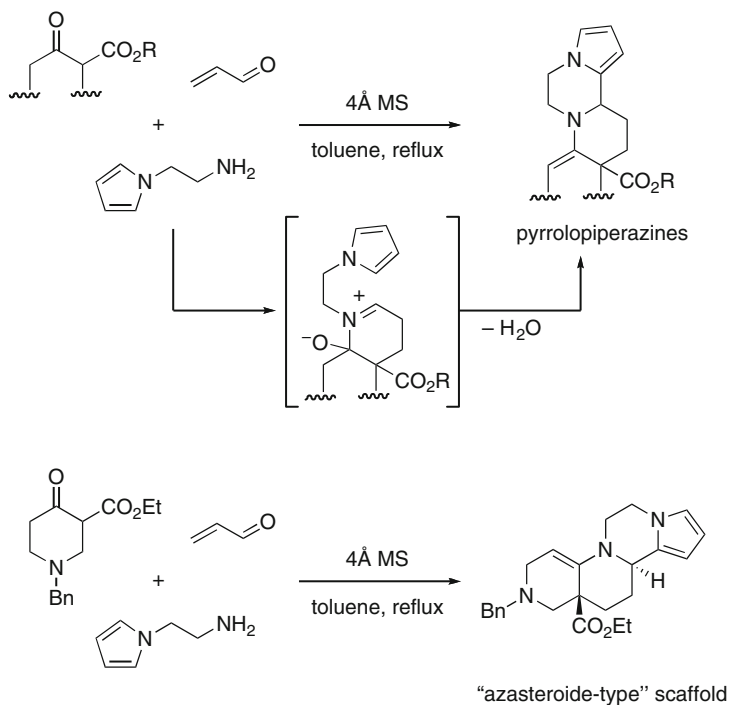
Scheme 60 Three-component synthesis of polycyclic pyrrolo piperazine scaffolds
