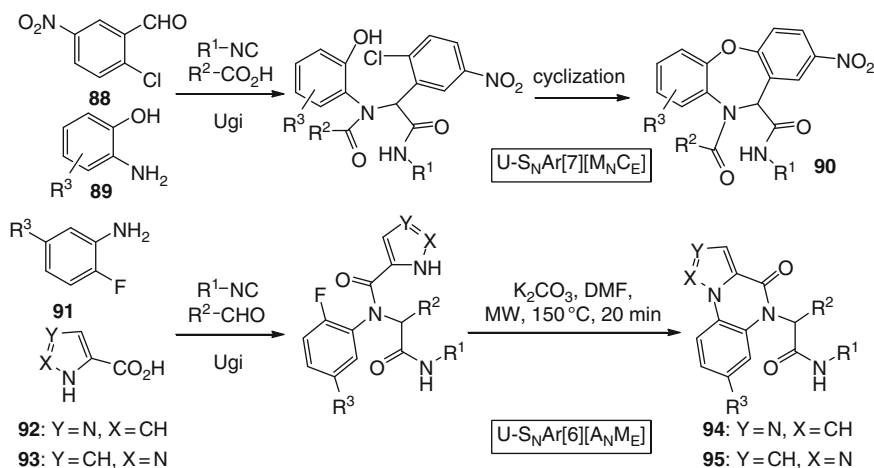
Fig. 18 Synthesis of medium-sized benzo-fused heterocycles through tandem Ugi-S N Ar processes
