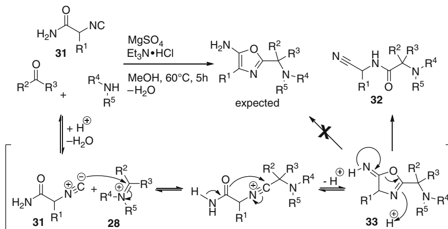
Fig. 12 Formation of N -(cyanomethyl)amides in the MCR between primary isocyano amides, aldehydes/ketones, and amines
