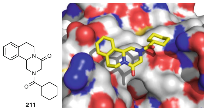
Fig. 10 X-ray co-crystal structure of praziquantel 211 and glutathione-S-peroxidase complex (PDB ID: 1GTB). Praziquantel is shown as yellow sticks and the receptor binding site is shown as hydrophobic surface
