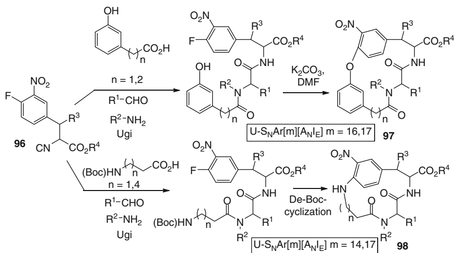
Fig. 19 Synthesis of para -cyclophanes through tandem Ugi-S N Ar processes
