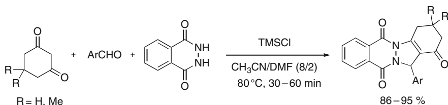
Scheme 32 TMSCl-catalyzed three-component route to indazolophthalazide-trione derivatives
