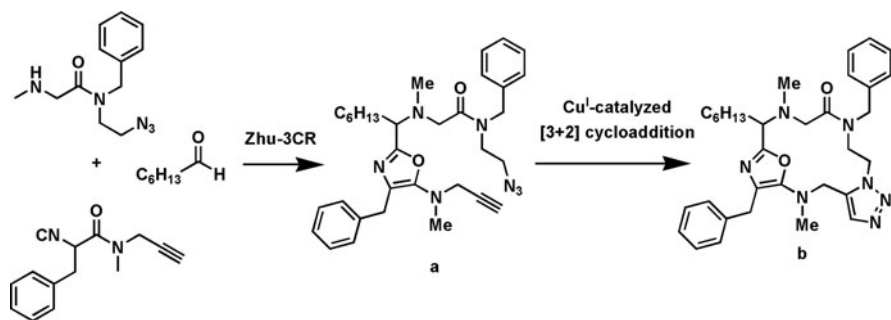
Scheme 17 Synthesis of cyclic peptidomimetics by sequential Zhu-3CR/azide-alkyne dipolar cycloaddition strategy
