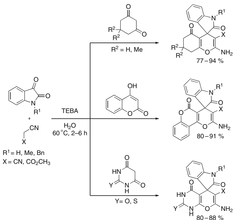
Scheme 36 Three-component synthesis of spirooxindole-containing tetrahydrochromene derivatives
