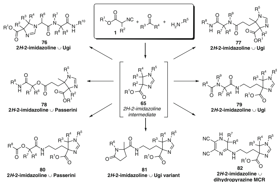
Fig. 24 Generation of higher order MCRs based on the 2H-2-imidazoline MCR
