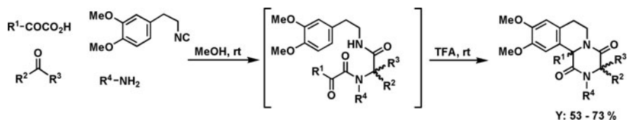
Scheme 2 El Kaïms synthesis of DKPs using an Ugi/Pictet–Spengler combination
