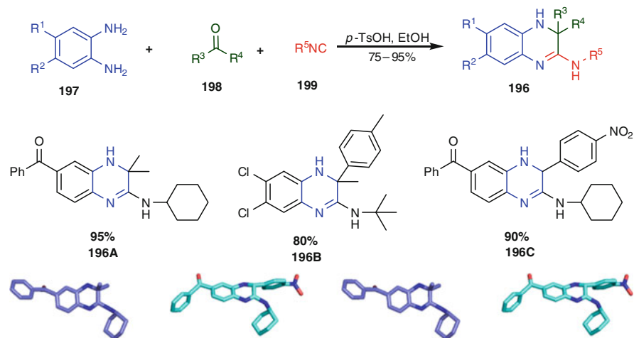
Scheme 35 Synthesis of 3,4-dihydroquinoxalin-2-amine derivatives 196 and two representative 3D conformations of 196A (blue) and 196C (cyan)
