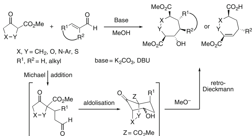
Scheme 58 General scheme for the MARDi cascade
