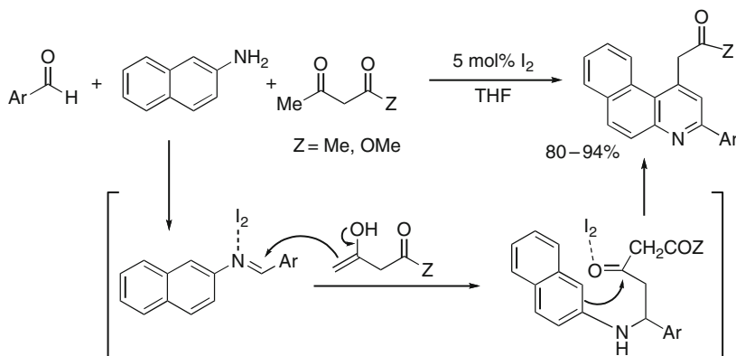
Scheme 25 \text{I}_2 -catalyzed three-component synthesis of benzo[ f ]quinoline derivatives
