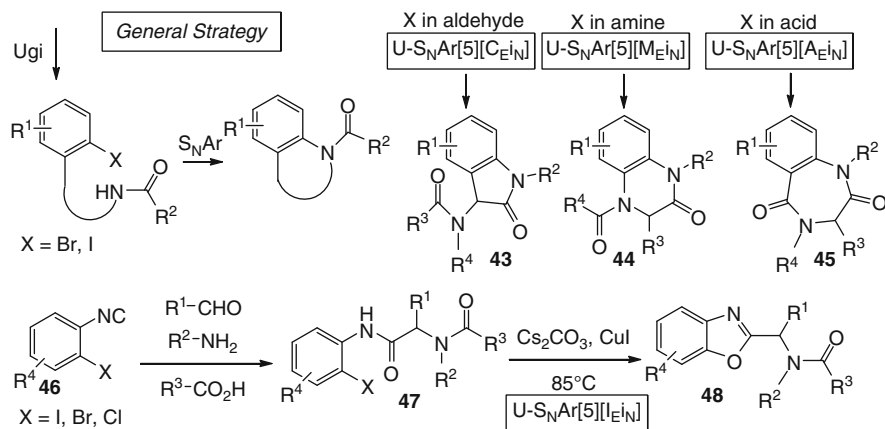
Fig. 8 Sequential Ugi-metal catalyzed S_NAr (Buchwald-Hartwig)
