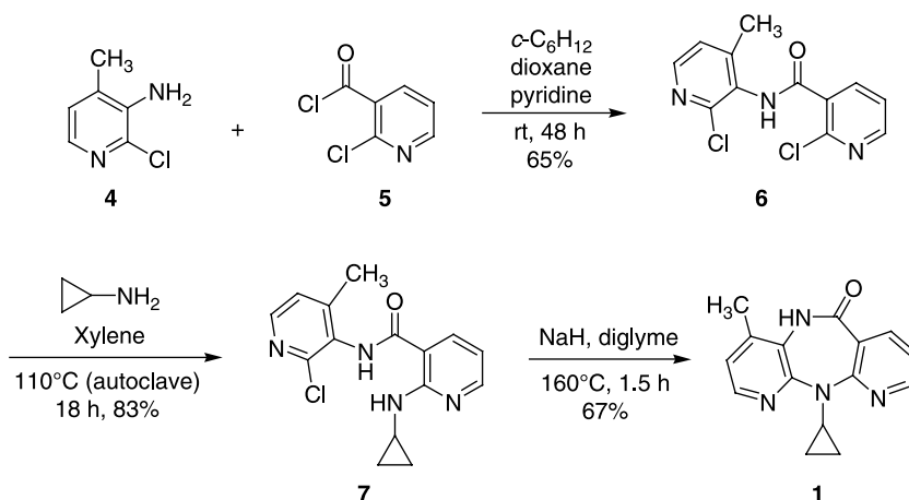
Scheme 6.1.
