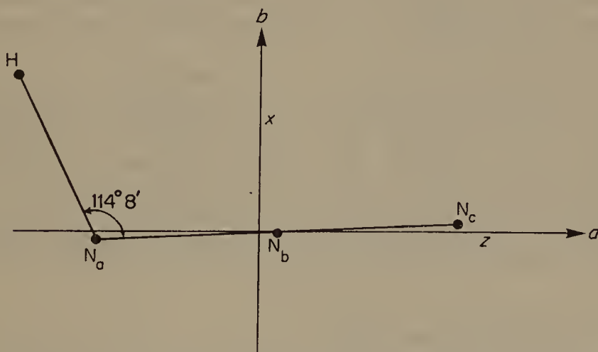
FIGURE 6. Positions of the atoms in the principal-axis system of \text{HN}_3 .
