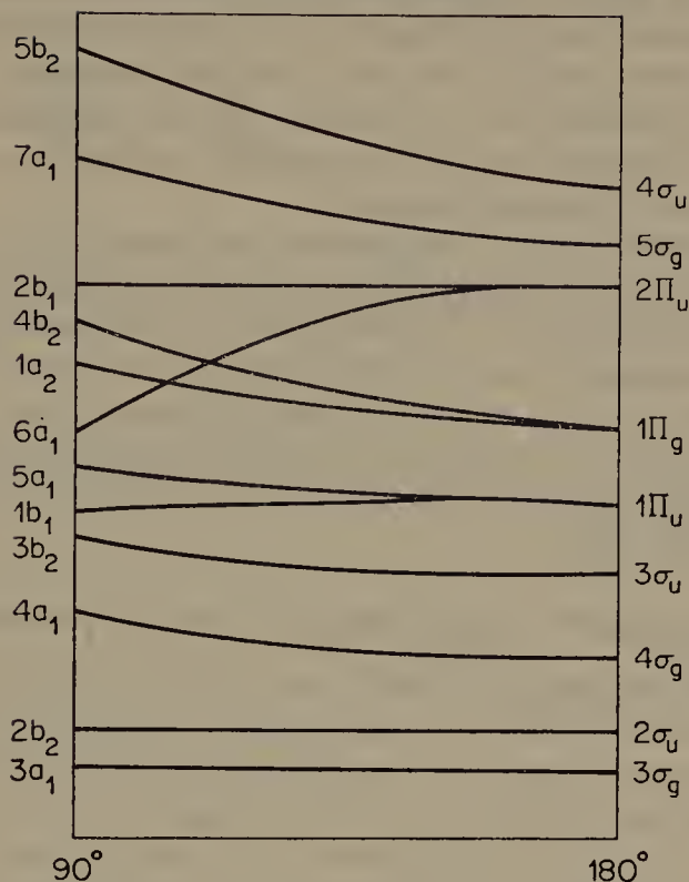
FIGURE 10. Walsh's diagram for ABA molecules (adapted from reference 71).
