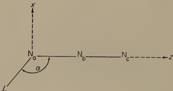
FIGURE 1. The geometry of covalent azides ( L is the atom to which \text{N}_a is bound; all the nuclei lie in the xz plane).
