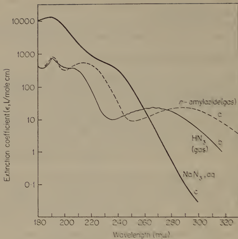
FIGURE 8. The electronic absorption spectra of n -amylozide gas (a), \text{HN}_3 gas (b) and \text{NaN}_3 in aqueous solution (c) (adapted from reference 9).
