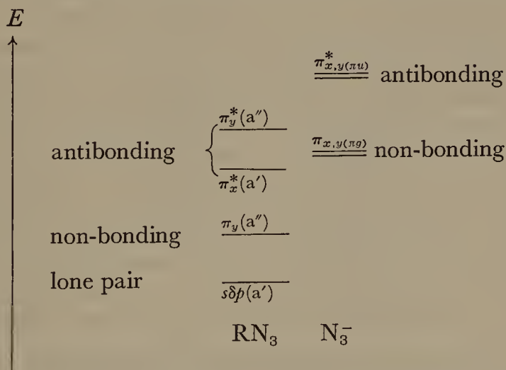
FIGURE 5. Energy levels of the highest-filled and lowest-unfilled orbitals of the azido group and of N_3^- .
