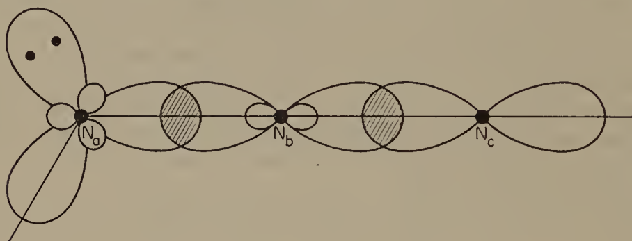
FIGURE 2. The \sigma -skeleton of azides.
