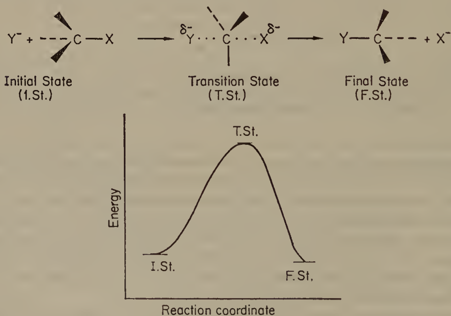
FIGURE 3. Walden Inversion during bimolecular substitution at a saturated carbon atom.
