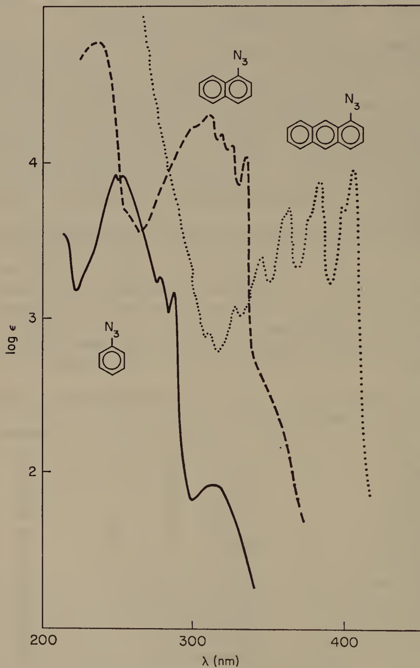
FIGURE 2. Absorption spectra of aromatic azides.
