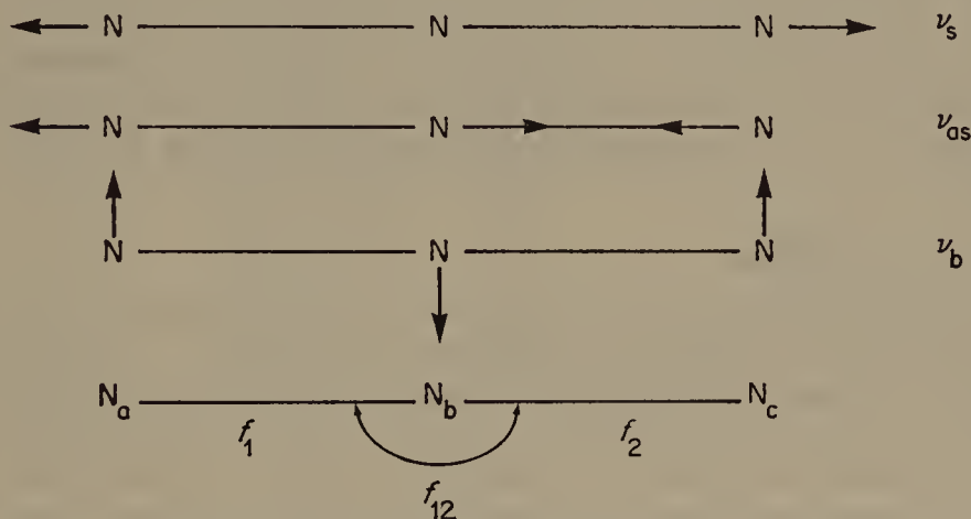
FIGURE 7. The fundamental vibration frequencies and bond-stretching force constants of molecules like \text{N}_3^- or \text{N}_3 .
