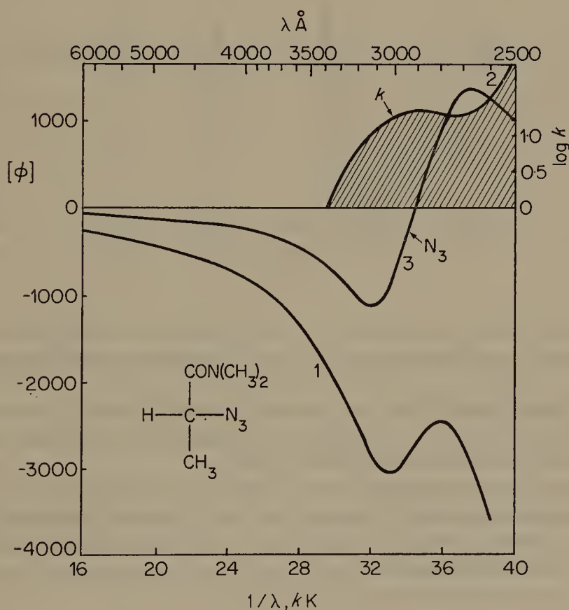
FIGURE 9A. Optical rotatory dispersion (1) and absorption spectrum (2) of \alpha -azidopropionic acid dimethylamide in ether. Curve 3: the rotatory contribution of the azido group.
