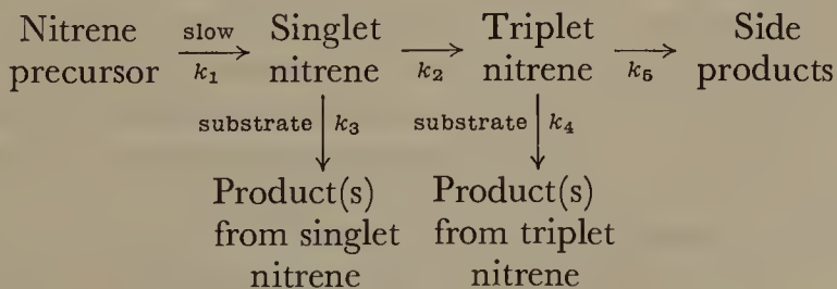
SCHEME 1. Singlet and triplet nitrene reactions
