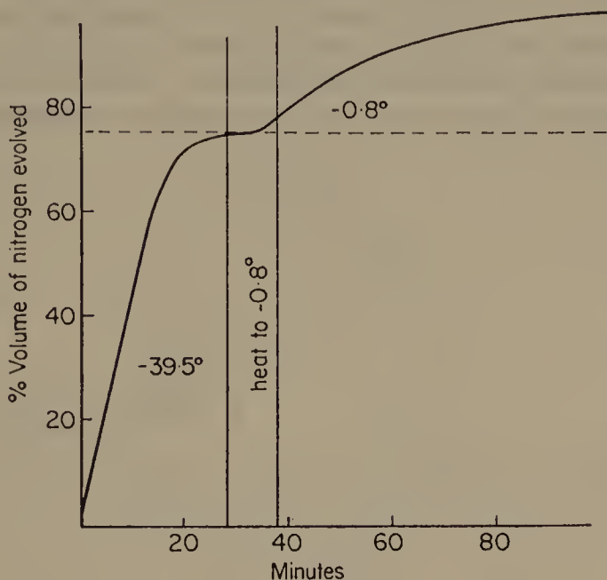
FIGURE 5. Plot of the volume of nitrogen evolved against time for the reaction of benzenediazonium chloride with lithium azide in methanol at -39.5^\circ and -0.8^\circ showing the two-path nature of the reaction.
