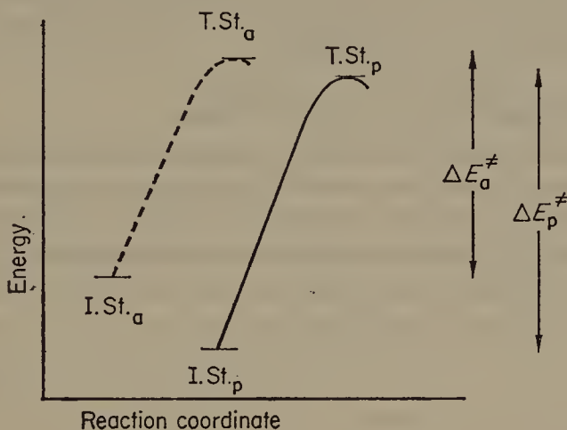
FIGURE 2. Effect of protic (p) and dipolar aprotic (a) solvents on the activation energy of S_N2 reactions and S_NAr reactions with the formation of T.St.1 rate-limiting. ---- dipolar aprotic solvent. — protic solvent.
