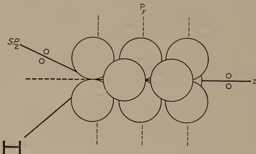
FIGURE 1. Atomic p -orbitals of \text{HN}_3 .
