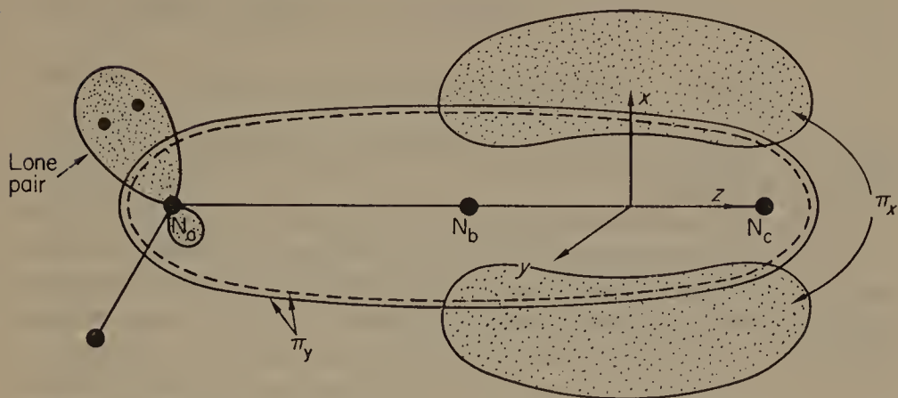
FIGURE 3. The bonding \pi orbitals of azides (the (s\delta p)^2 lone pair is also shown).
