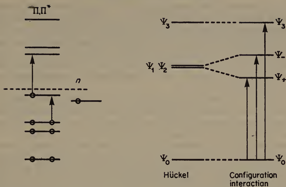
FIGURE 5. (a) Hückel MO-levels of phenyl nitrene; (b) Energy levels of excited states of phenyl nitrene.
