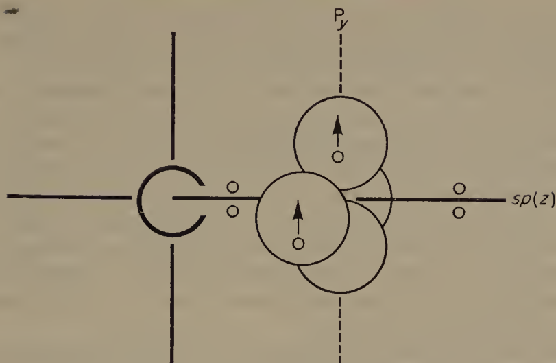
FIGURE 4. Electronic configuration of triplet nitrene.
