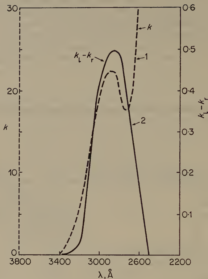
FIGURE 9B. Absorption spectrum (1) and circular dichroism (2) of \alpha -azidopropionic acid dimethylamide in hexane (adapted from reference 82).
