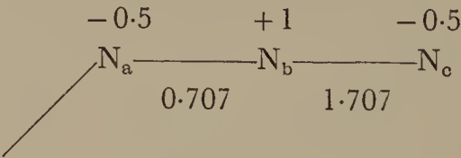
FIGURE 4. Primitive diagram of formal charges and bond orders of the \pi system in the azido group (based on single values for \alpha and \beta ).
