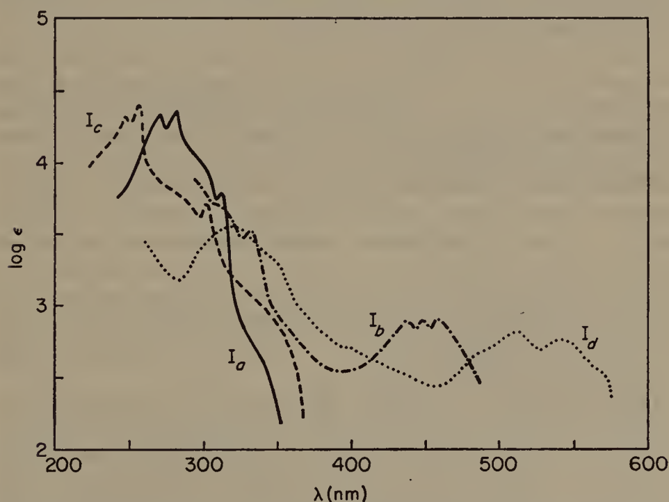
FIGURE 6. Absorption spectra of 1,4-diazidobenzene (I) and its photoproducts; matrix isolated at 77°K. I_a , diazide; I_b , azido-nitrene; I_c , dinitrene; I_d , dinitrene cation.
