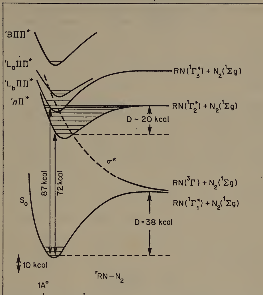
FIGURE 3. Potential energy diagram of the \text{RN}-\text{N}_2 bond in an aromatic azide.
