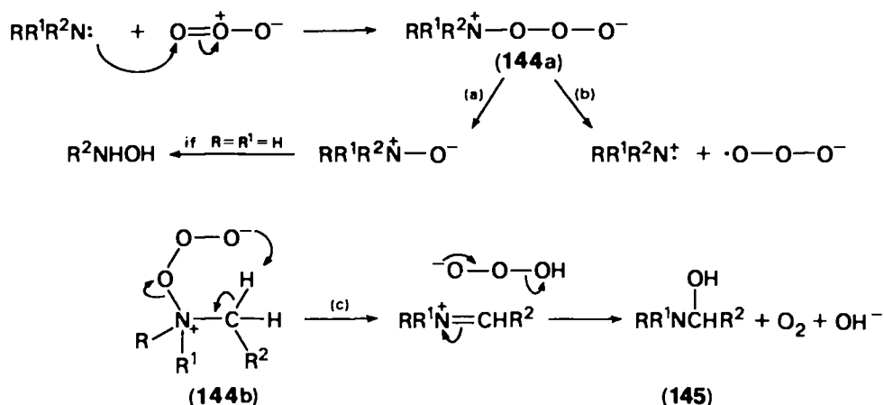
SCHEME 27
