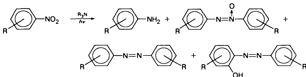
SCHEME 40
