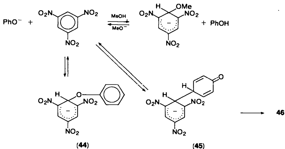
SCHEME 6
