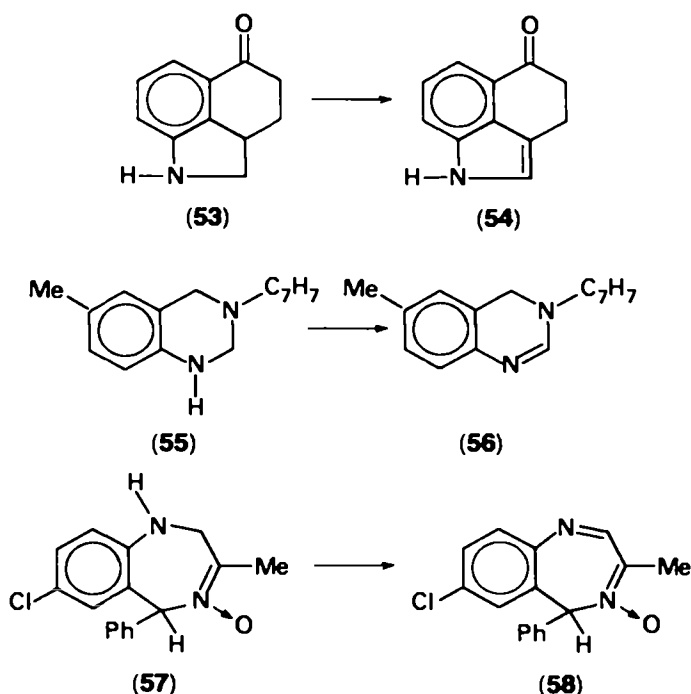
SCHEME 8
