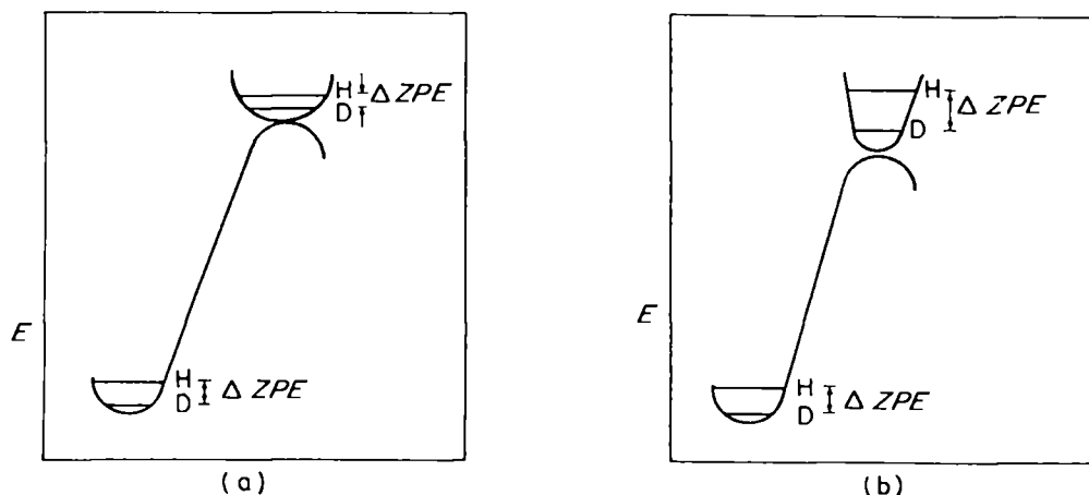
FIGURE 1. (a) Reaction where \Delta ZPE(\text{reactant}) is greater than \Delta ZPE(\text{transition state}) and k_H/k_D > 1 . (b) Reaction where \Delta ZPE(\text{reactant}) is less than \Delta ZPE(\text{transition state}) and k_H/k_D < 1 .
