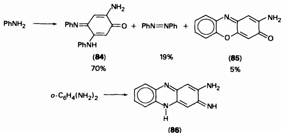
SCHEME 17
