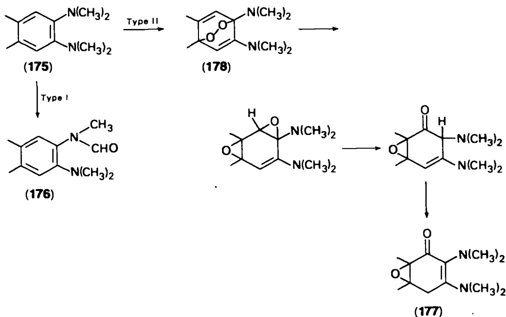
SCHEME 41
