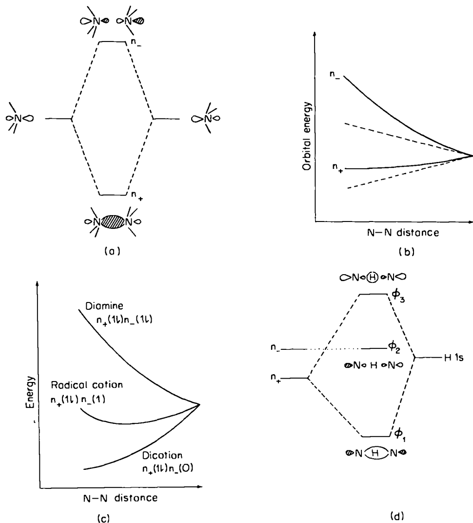
FIGURE 1. (a) Mixing of lone-pair orbitals to generate n_+ and n_- . (b) Orbital energies; without overlap n_+ is stabilized to the same extent than n_- is destabilized (dashed lines). Inclusion of overlap leads to greater destabilization of n_- . (c) Lone-pair interactions are always repulsive for diamines. The radical cation may have a weak three-electron bond, provided overlap is not too great ( s < \frac{1}{2} ) 2 . (d) The orbitals of a hydrogen bond, derived by mixing the hydrogen 1s orbital with n_+ . Note that for the \dot{N}-H\cdots N system, \phi_1(1\ell) \phi_2(1\ell) , the positive charge lowers all orbital energies.
