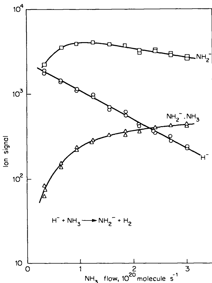
FIGURE 4. The variation of the H - , NH 2 - and NH 2 - ·NH 3 signals recorded upon the addition of NH 3 into a flowing He–NH 3 plasma in which H - is initially a major ion ( T = 297 K, P = 0.301 Torr). Reproduced by permission of the American Institute of Physics from D. K. Bohme, R. S. Hemsworth, H. W. Rundle and H. I. Schiff, J. Chem. Phys. , 59 , 77 (1973).
