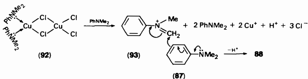
SCHEME 18
