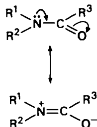
FIGURE 2. Comparison of resonance structures of secondary N -nitrosamines and tertiary amides.
