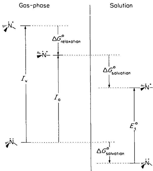
FIGURE 8. Relationships between I_v , the vertical ionization energy I_a , the adiabatic ionization energy, and E_1^{\circ} , the oxidation potential for the amine in solution.
