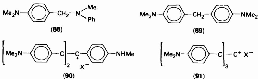
SCHEME 17
