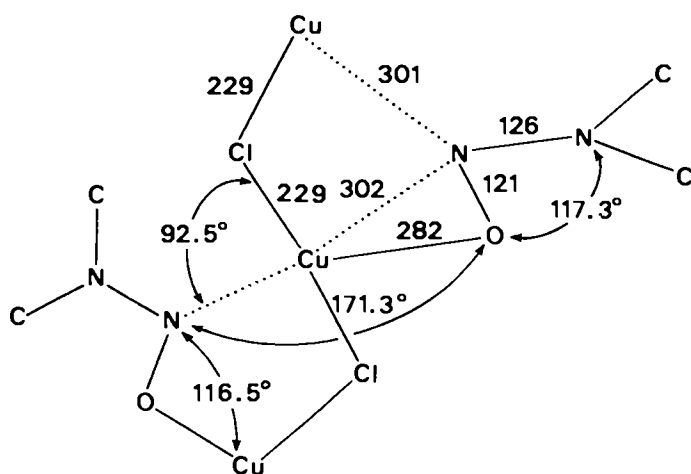
FIGURE 4. Structure of the 1:1 complex between N -nitrosodimethylamine and CuCl 2 . (From X-ray diffraction data 160 ; bond lengths in pm.)
