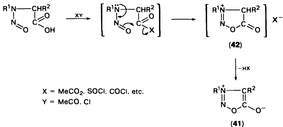
SCHEME 18. Intramolecular acylation of N -nitrosamines to give sydnone.
