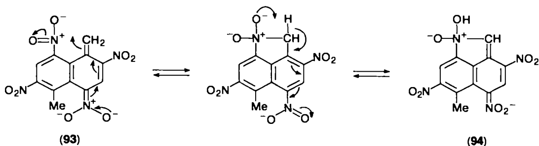
SCHEME 22
