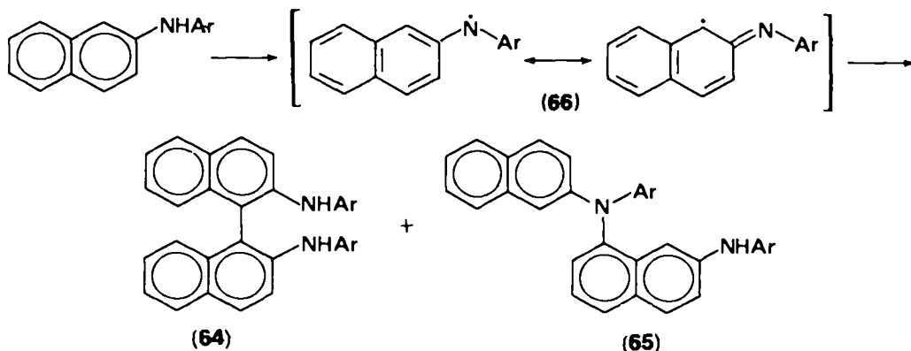
SCHEME 11
