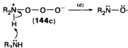
SCHEME 29
