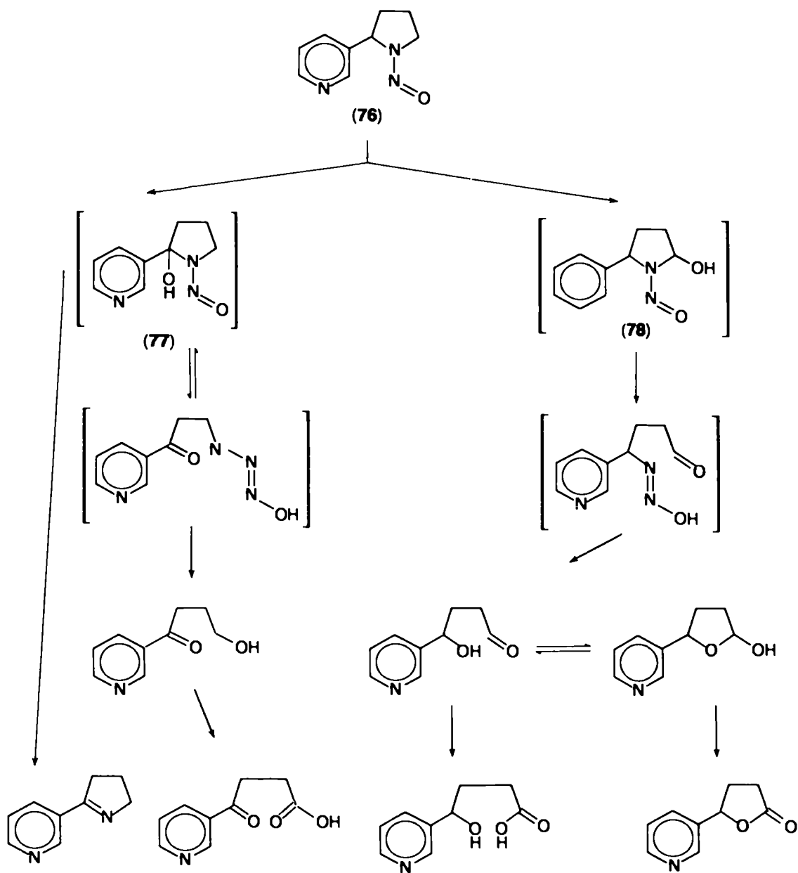
SCHEME 27. Pathways for product formation in the metabolic degradation of N -nitrosornornicotine. N -nitrosornornicotine.
