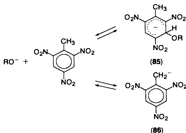
SCHEME 19
