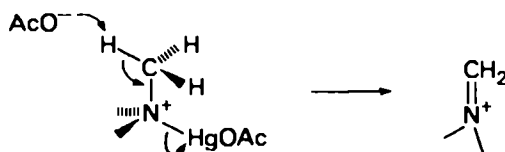
SCHEME 6
