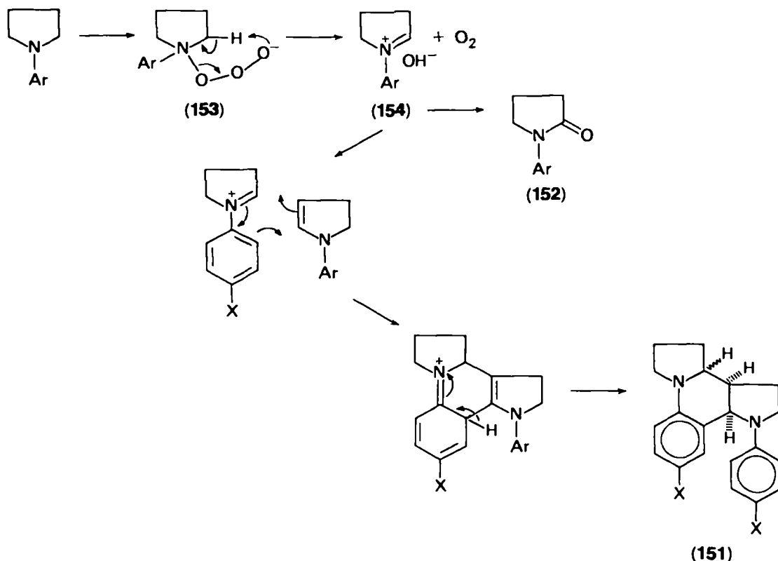
SCHEME 31
