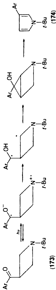
SCHEME 38
