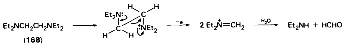
SCHEME 36
