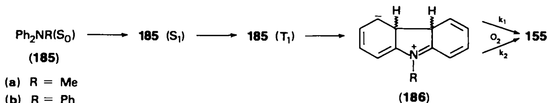
SCHEME 43
