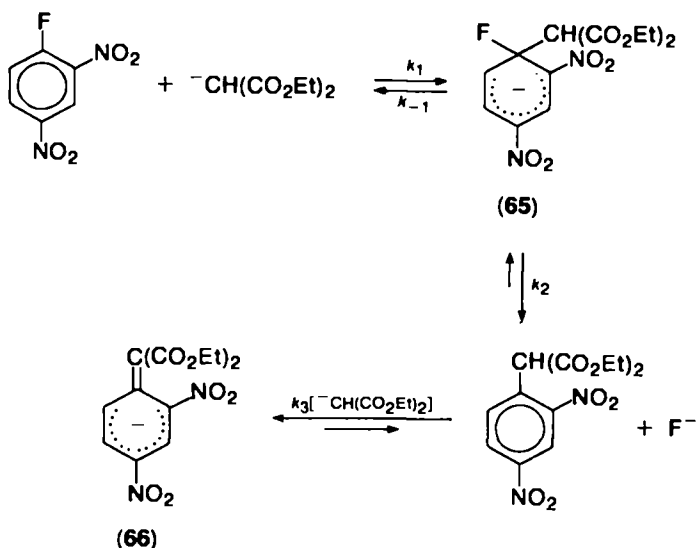
SCHEME 8
