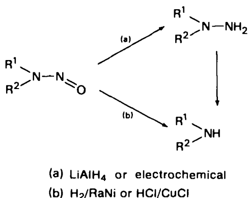
SCHEME 22. Usual products from the reduction of N -nitrosamines.
