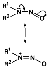
FIGURE 2. Comparison of resonance structures of secondary N -nitrosamines and tertiary amides.
