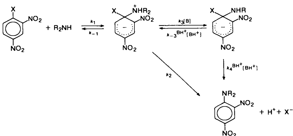
SCHEME 14
