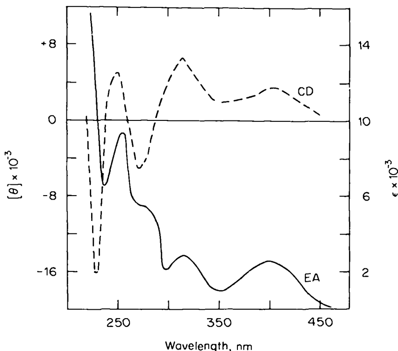
FIGURE 4. Electronic absorption (EA) and circular dichroism (CD) spectra of L-alanine (L-74) with a 15% molar excess of sodium salicylaldehyde (55) in methanol. Reproduced with permission from H. E. Smith, E. P. Burrows, M. J. Marks, R. D. Lynch and F.-M. Chen. J. Amer. Chem. Soc. , 99 , 707 (1977). Copyright by the American Chemical Society.
