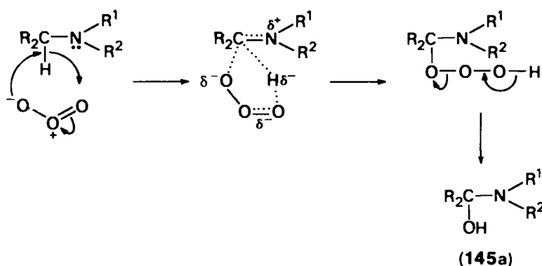
SCHEME 28
