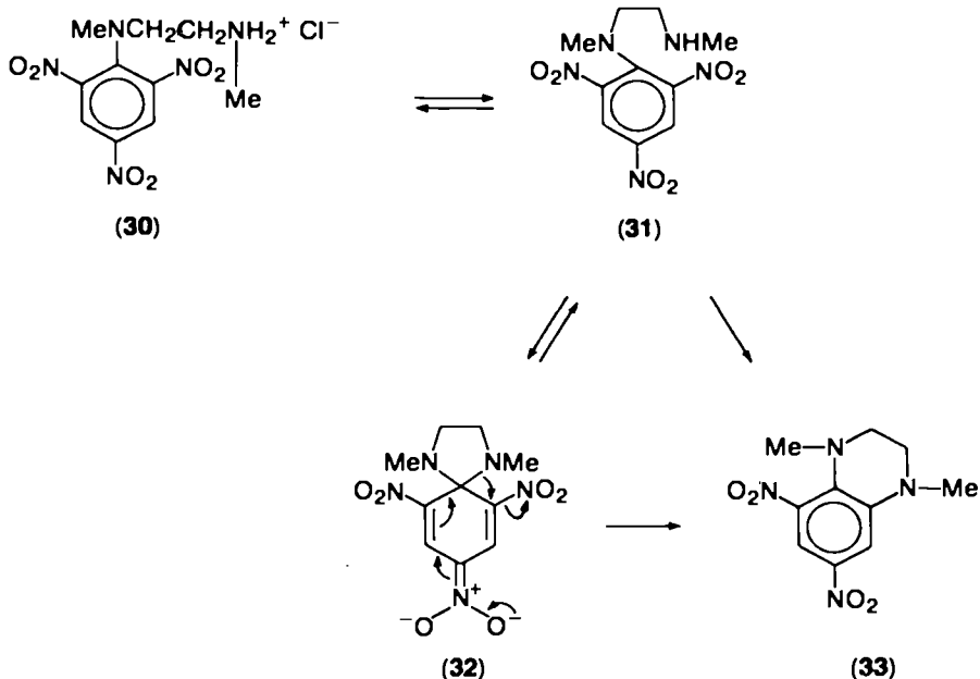
SCHEME 4
