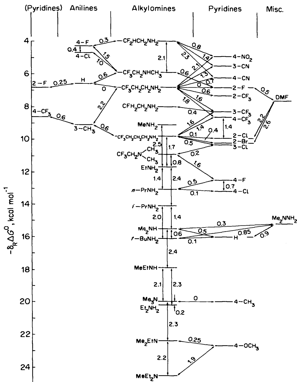
FIGURE 7. Summary of values of \Delta G^0 ( \text{kcal mol}^{-1} ) derived using low-pressure ICR techniques. Reproduced with permission from R. W. Taft in Proton-transfer Reactions (Eds. E. Caldwin and V. Gold), Chapman and Hall Ltd., London, 1975, p. 31.
