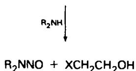
SCHEME 6. Catalysis of nitrosyl gas nitrosation of amines by \beta -hydroxyalkyl compounds.
