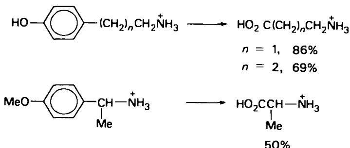
SCHEME 23
