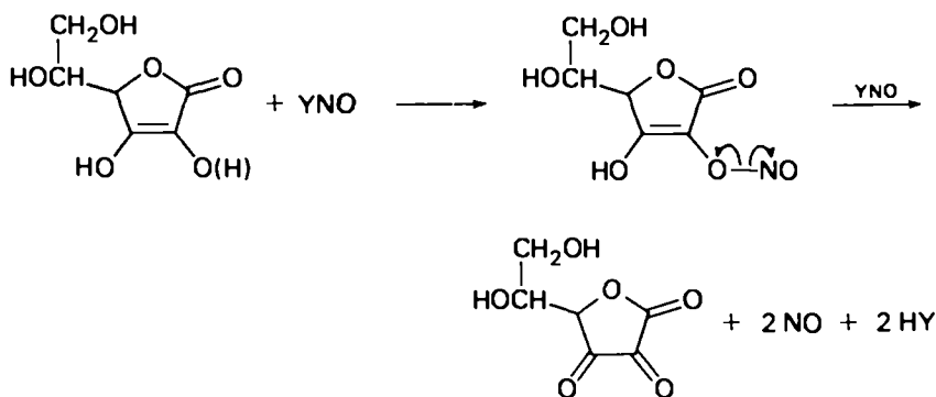
SCHEME 4. Reduction of \text{Y}-\text{NO} to \text{NO} by ascorbic acid.
