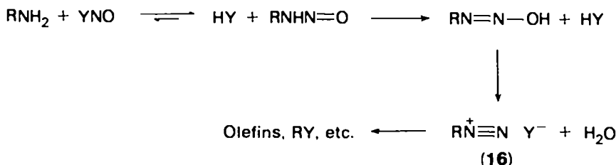
SCHEME 9. Nitrosation of primary aliphatic amines.
