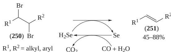
SCHEME 57. Reductive dehalogenation of vicinal dibromoalkanes
