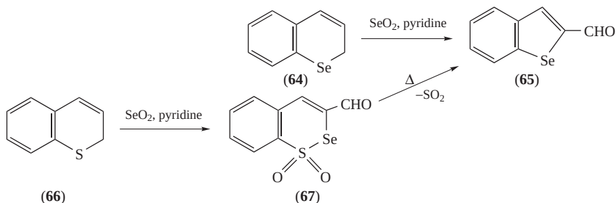
SCHEME 19. Oxidative ring contraction of selenachromene and thiachromene with \text{SeO}_2 .
