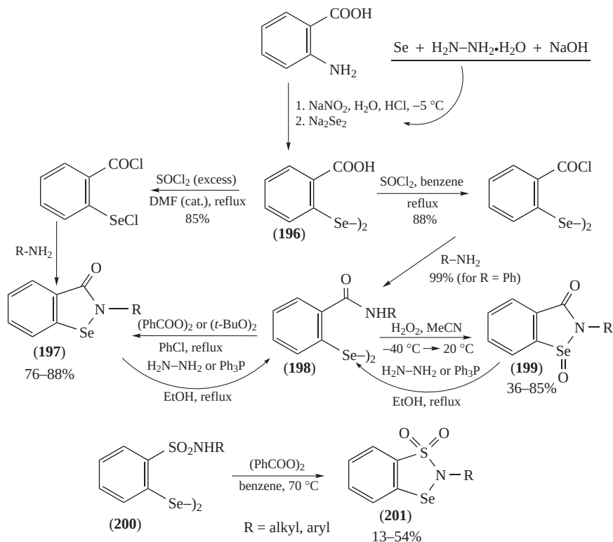
SCHEME 48. Oxidative cyclization of bis[(2-carbamoyl)phenyl] diselenides and 1,3,2-thiaselenazole 1,1-oxides
