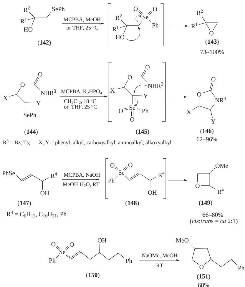
SCHEME 39. Nucleophilic intramolecular substitution of the \text{PhSeO}_2 group in selenones
