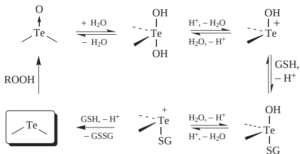
SCHEME 3 Mechanism for the Gpx -like behavior of diorganotellurides
