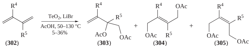
SCHEME 73. Diacetoxylation of alkenes and dienes with \text{TeO}_2/\text{LiBr}/\text{AcOH}
