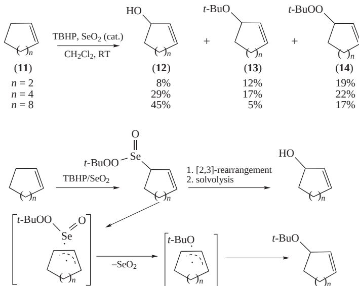
SCHEME 3. TBHP/SeO 2 oxidation of some cycloalkenes
