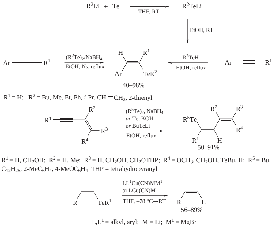
SCHEME 87. Hydrotelluration of alkynes and the coupling of Z -vinyllic tellurides with other organometallics
