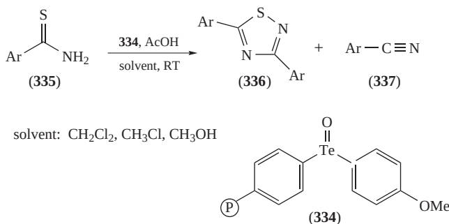
SCHEME 81. Oxidation of thioamides with polymer-supported diaryl telluroxide
