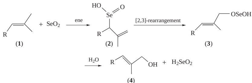
SCHEME 1. Mechanism of selenium(IV) oxide \alpha -hydroxyalkylation of alkenes
