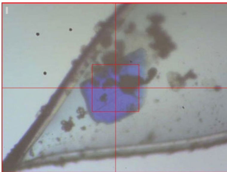
FIGURE 4 Mouse MDR3 CL P-gp co-crystallized with tellurorhodamine II ( TeRh II ). Image courtesy of Geoffrey Chang, The Scripps Research Institute
