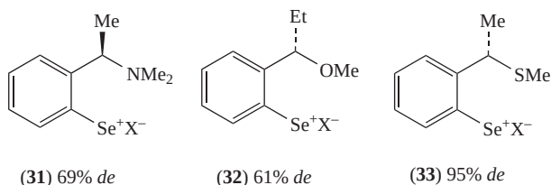
FIGURE 11. Chiral electrophiles 31 – 33 with different heteroatoms
