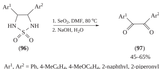
SCHEME 25. Conversion of 3,4-diaryl-1,2,5-thiazolidine 1,1-dioxides to diaryl 1,2-diketones
