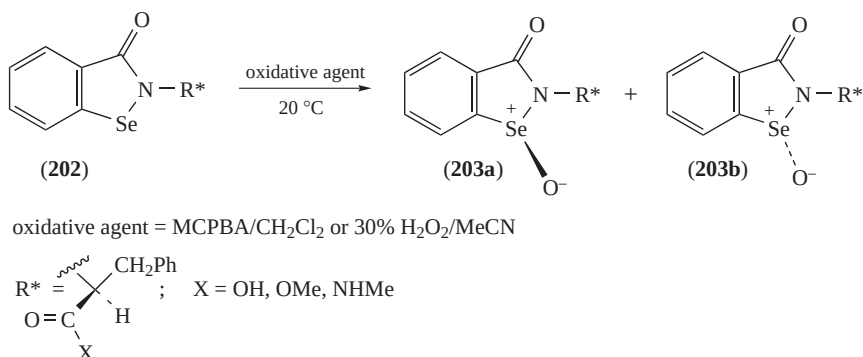
SCHEME 49. Stereoselective oxidation of cyclic selenenamides to seleninamides
