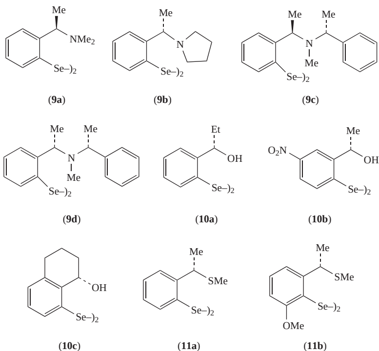
FIGURE 7. Structures of nitrogen-, oxygen and sulfur-containing diselenides 9a–9d , 10a–10c and 11a and 11b
