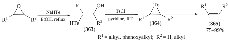
SCHEME 90. Deoxygenation of epoxides with sodium hydrogen telluride
