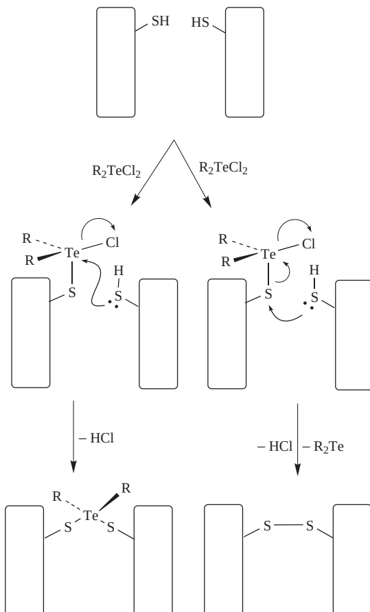
FIGURE 3 A mechanism for disulfide bridge formation and oligomerization of mitochondrial membrane proteins using protein thiol residues and organo pertelluranes
