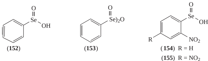
SCHEME 40. Areneseleninic acids and anhydride
