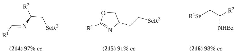
FIGURE 19. Seleno imines 214 , oxazoline-based selenides 215 and β-seleno amides 216 as chiral selenium-containing ligands
