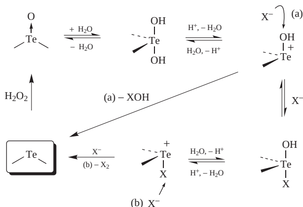
SCHEME 4 Mechanism for haloperoxidase-like behavior of diorganotellurides in the presence of hydrogen peroxide and halide ions
