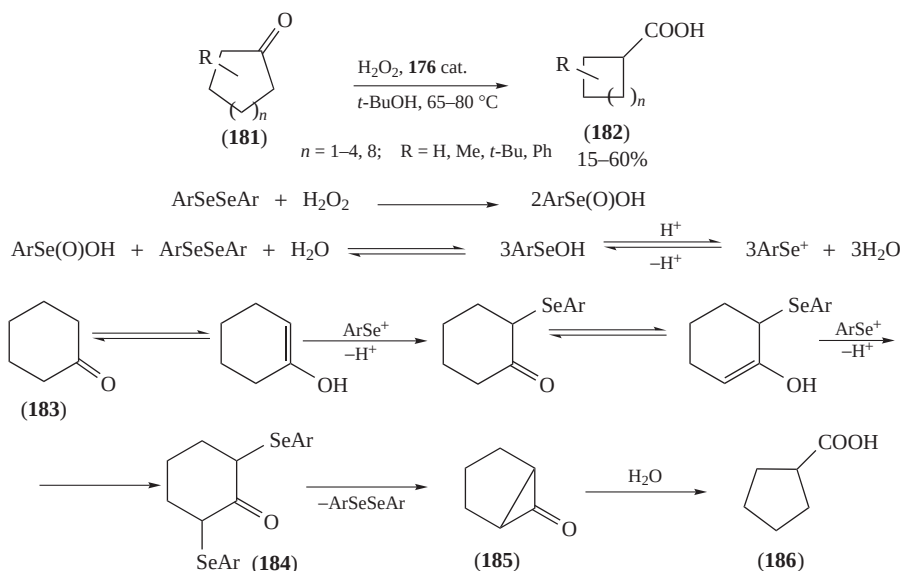
SCHEME 45. Oxidative conversion of cycloalkanones into cycloalkanecarboxylic acids catalyzed by poly(bis-9,10-anthracenylene) diselenide
