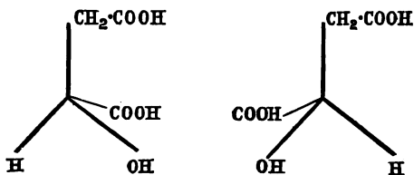
FIG. 51.—Space configuration of isomeric Malic acids.
