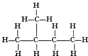
Isopentane.
