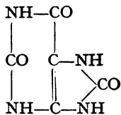
Formula of Uric acid.
