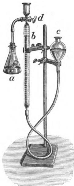
FIG. 56.—Lunge's Nitrometer for the estimation of urea.
