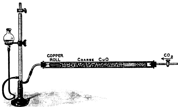
FIG. 57.—Dumas' apparatus for estimating nitrogen with Schiff's azotometer.
