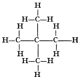
Neopentane.
