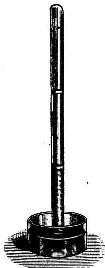
FIG. 35.—Action of chlorine on marsh-gas.
