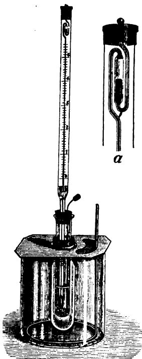
FIG. 12.—Beckmann's freezing-point apparatus.
