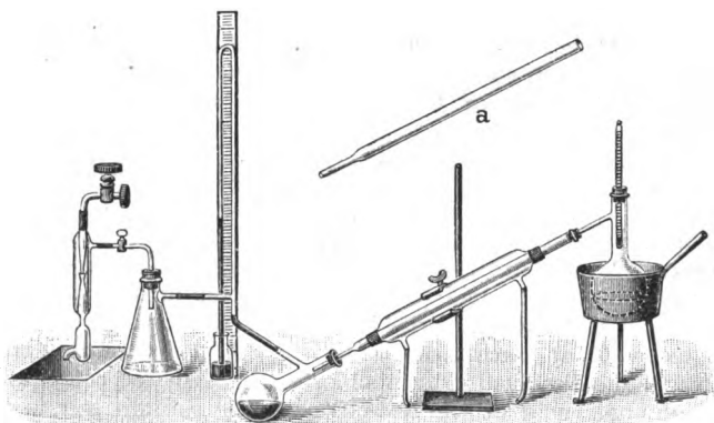
FIG. 62.—Apparatus for distillation under reduced pressure.
