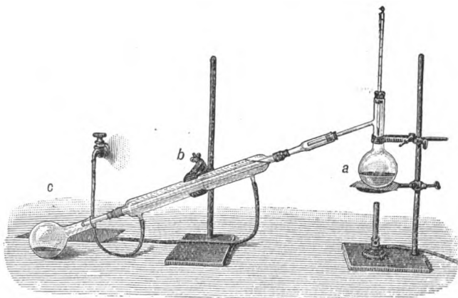
FIG. 4.—Distillation apparatus.
