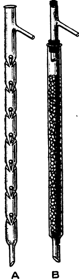
FIG. 6.—Fractionating columns.
