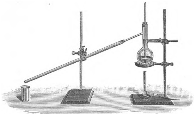
FIG. 55.—Preparation of Acetamide.
