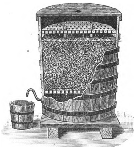
FIG. 28.—Quick vinegar process.
