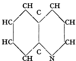
Quinoline.
