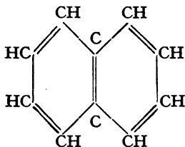
Formula for Naphthalene.
