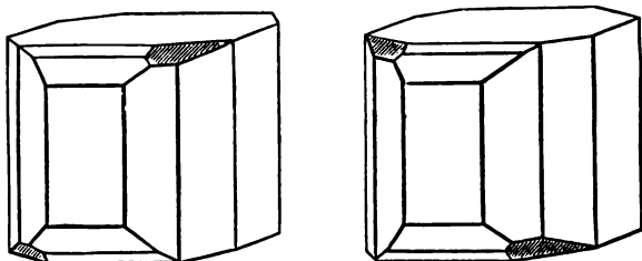
FIG. 52.—Enantiomorphous crystal forms of Sodium ammonium tartrate.
