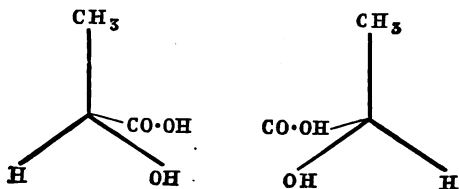
FIG. 50.—Stereo-isomeric forms of Lactic acid.
