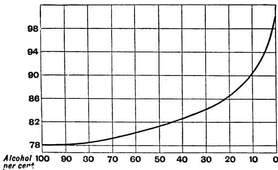
FIG. 5.—Boiling-point curve of alcohol and water mixtures.
