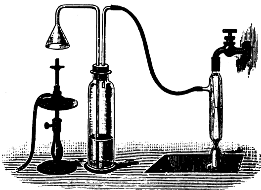
FIG. 41.—Acetylene formed by incomplete combustion of coal-gas.
