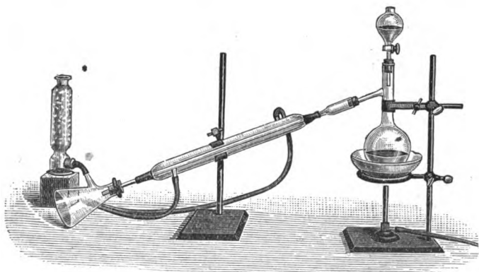
FIG. 16.—Preparation of ethyl bromide.
