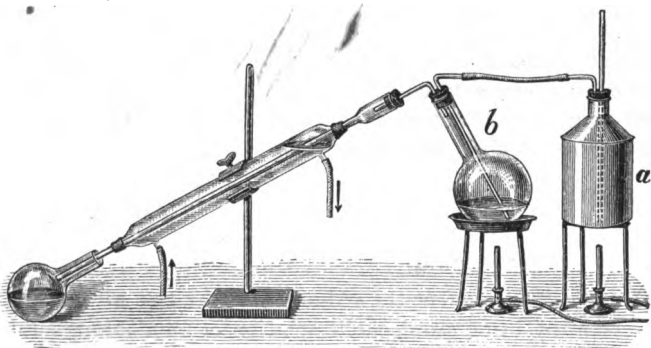
FIG. 61.—Distillation in steam.
