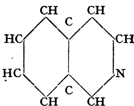
Isoquinoline.
