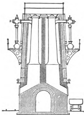
FIG. 31.—Shale retort.
