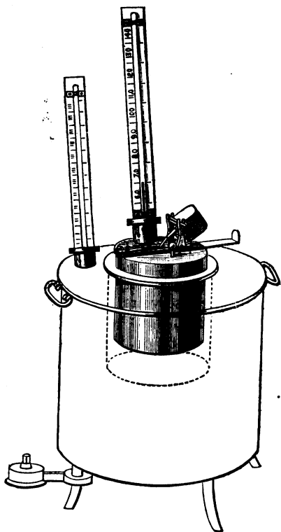
FIG. 34.—The Abel flash-point apparatus.
