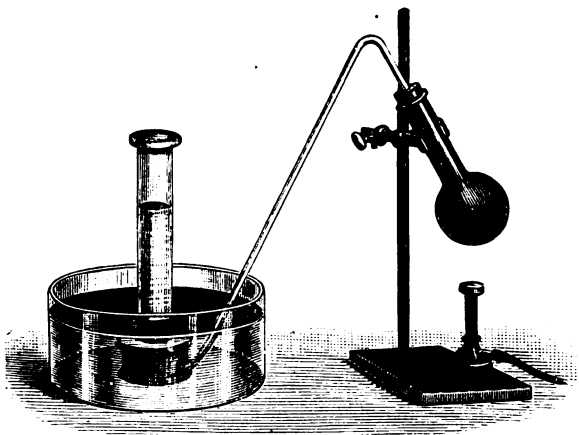
FIG. 29.—Preparation of marsh-gas from potassium acetate.
