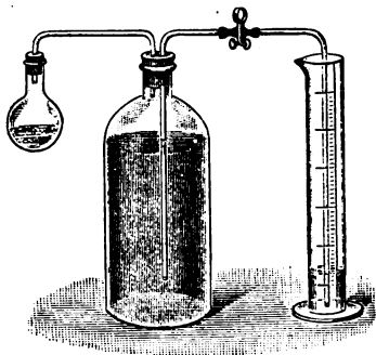
FIG. 15.—Measurement of the volume of hydrogen formed on dissolving a known weight of sodium in alcohol.
