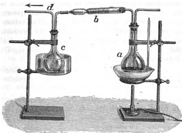
FIG. 30.—Preparation of formaldehyde.
