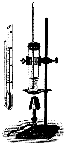
FIG. 2.—Apparatus for determining the melting-point.
