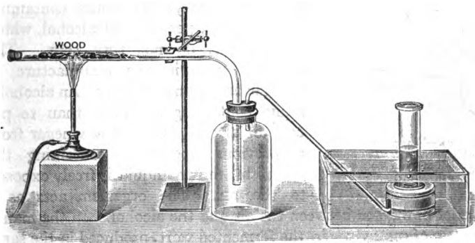
FIG. 26.—The destructive distillation of wood.
