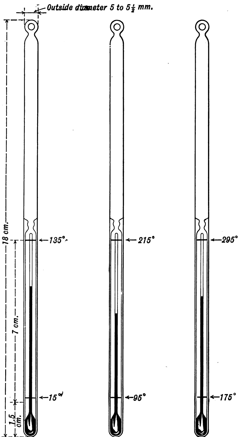
FIG. 1.—Short Scale Thermometers.
