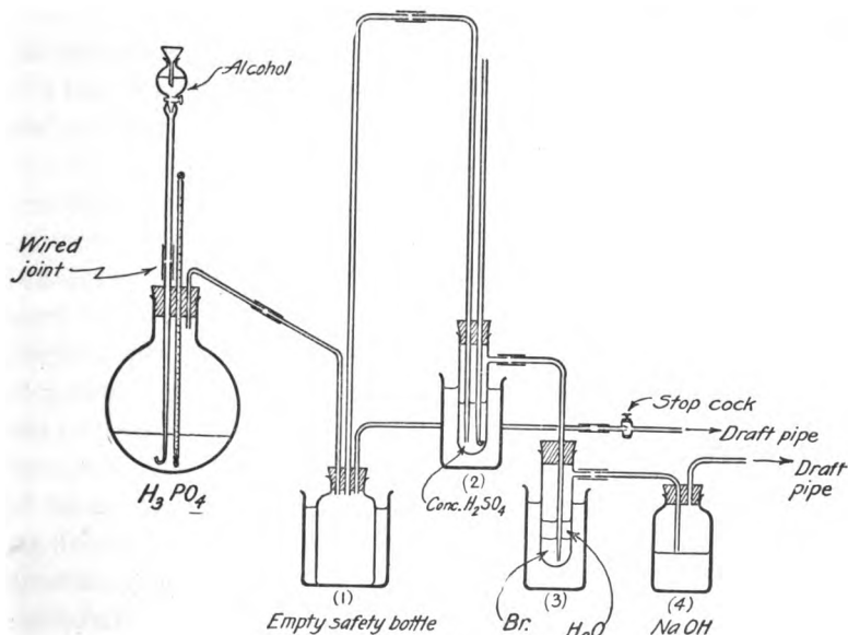
Diagram of Apparatus for Ethylene Dibromide
