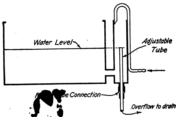
CONSTANT LEVEL WATER BATH CROSS SECTION
