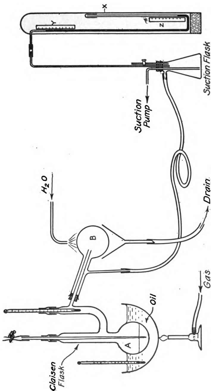
FIG. 11.—DISTILLATION IN VACUO
