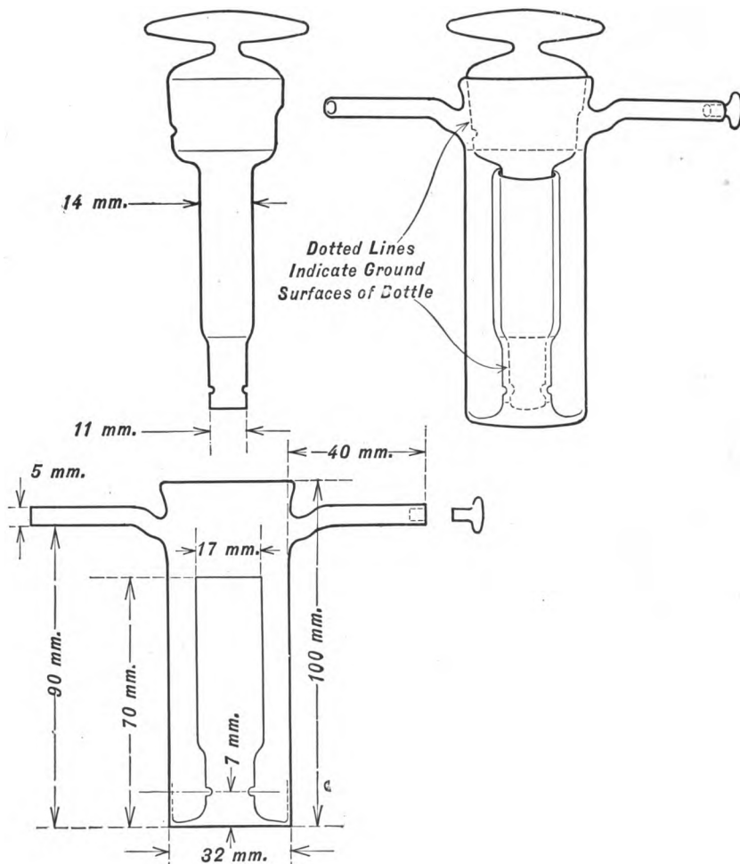
FIG. 17.—Fisher Absorption Bottle.
