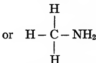
Amino-methane
